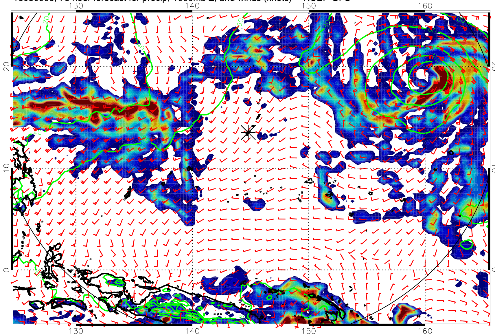
16080906, 78 hour forecast for precip, 1000mb Z, and winds (knots) -- NCEP GFS
