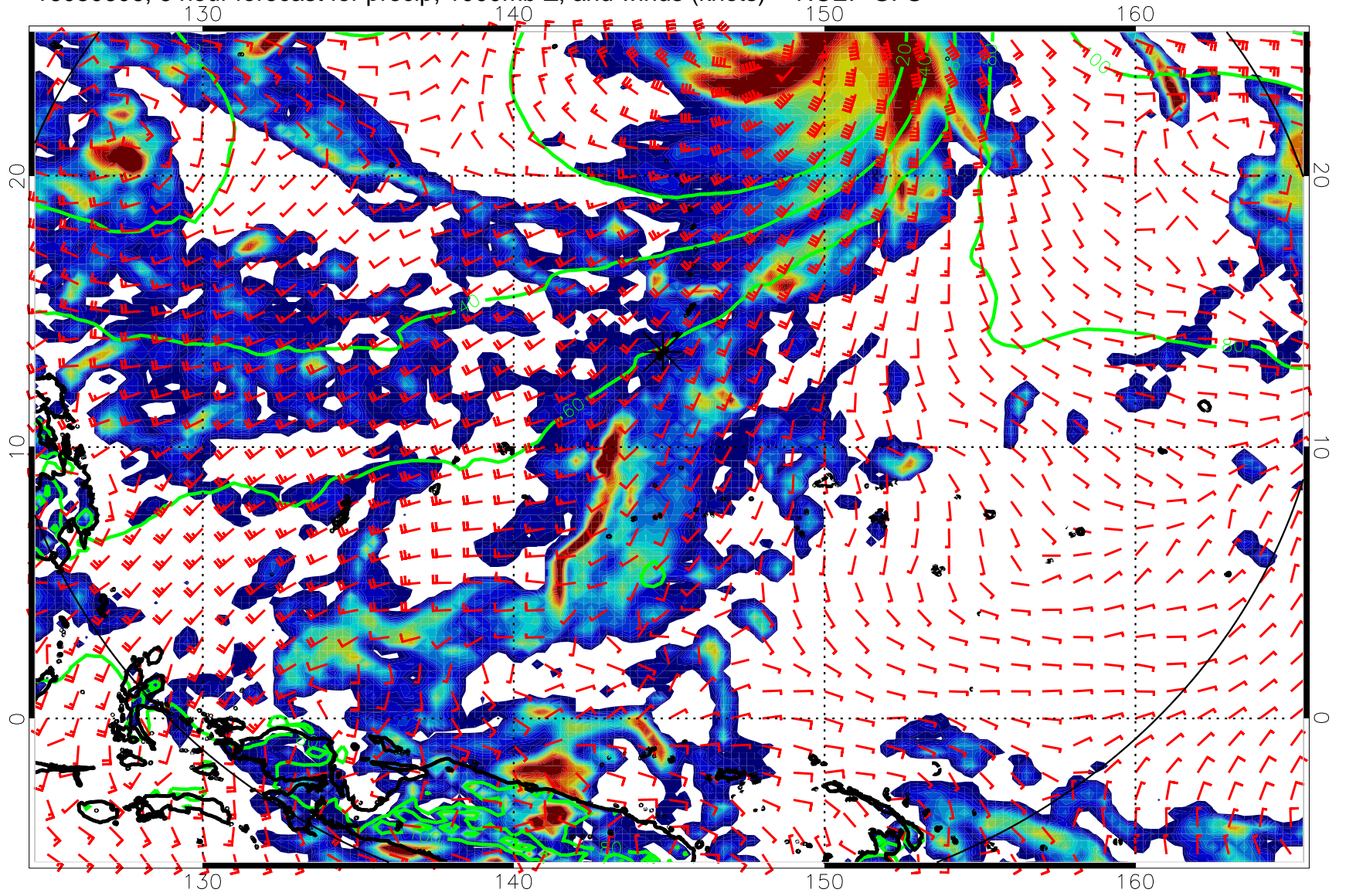
16080606, 6 hour forecast for precip, 1000mb Z, and winds (knots) -- NCEP GFS
