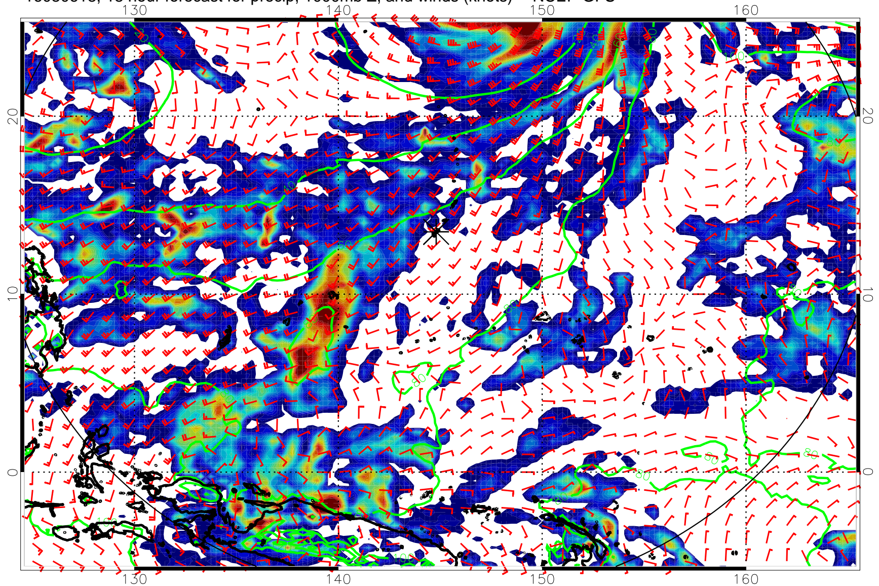
16080618, 18 hour forecast for precip, 1000mb Z, and winds (knots) -- NCEP GFS
