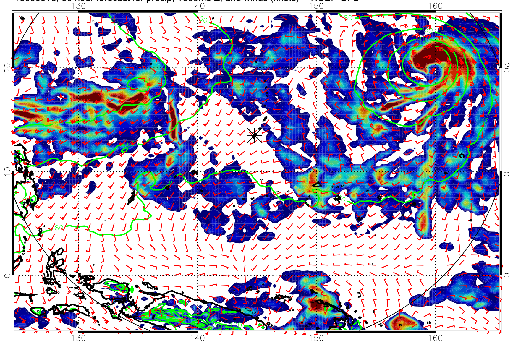
16080918, 90 hour forecast for precip, 1000mb Z, and winds (knots) -- NCEP GFS
