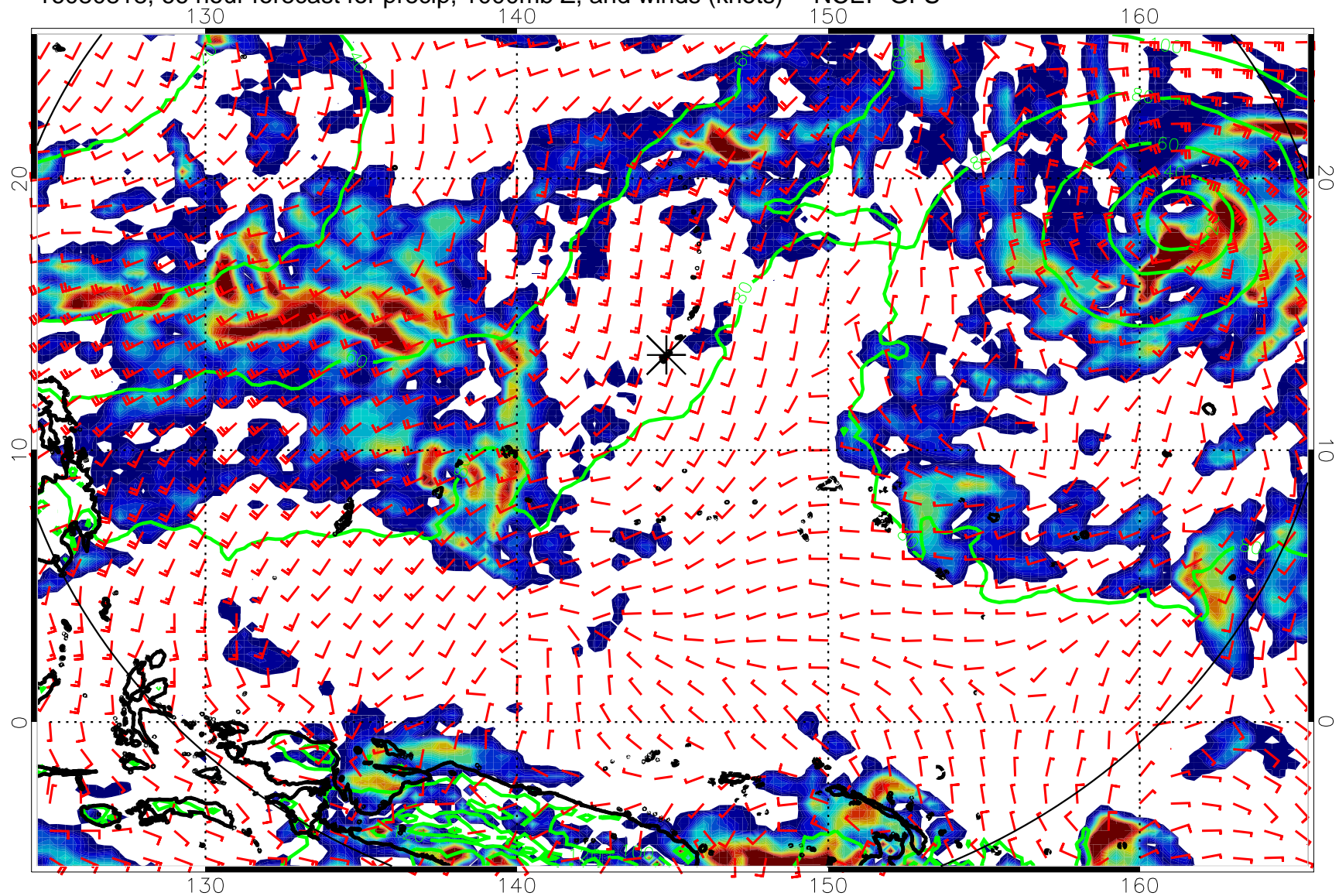
16080818, 66 hour forecast for precip, 1000mb Z, and winds (knots) -- NCEP GFS
