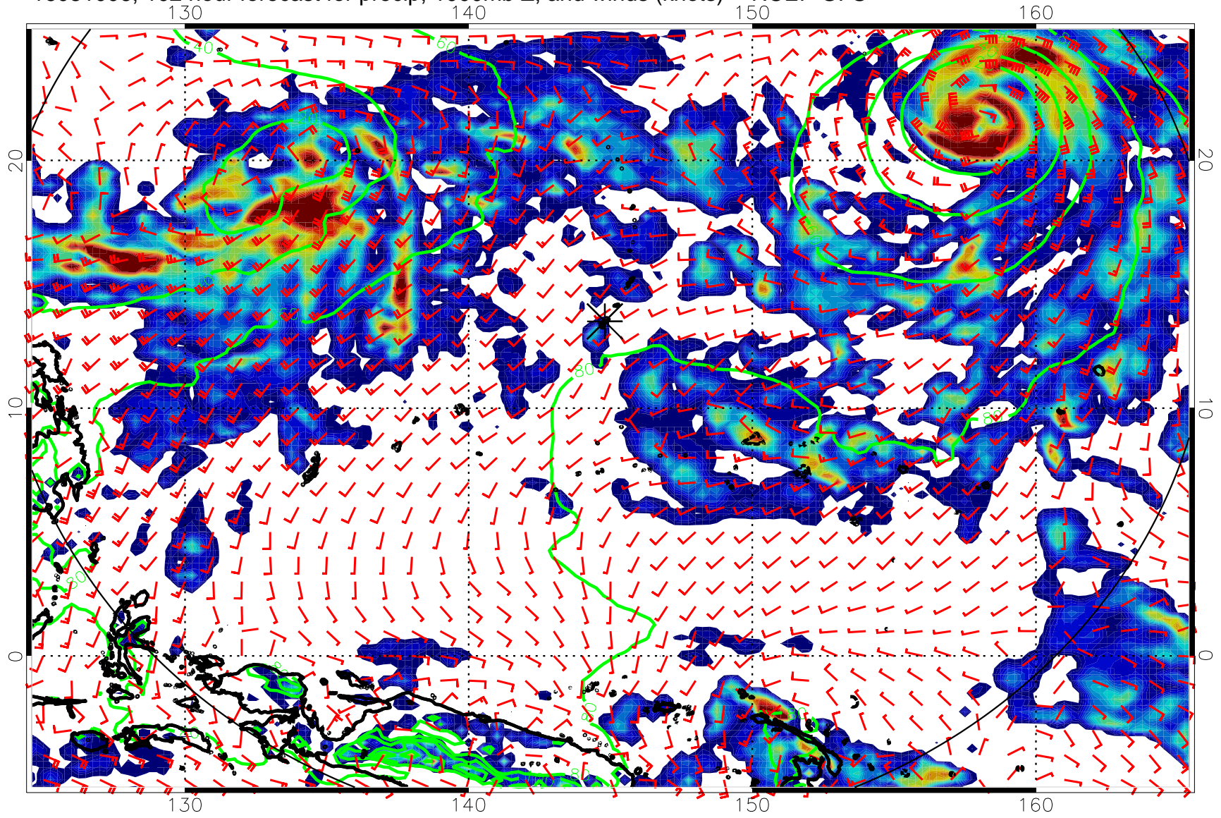
16081006, 102 hour forecast for precip, 1000mb Z, and winds (knots) -- NCEP GFS
