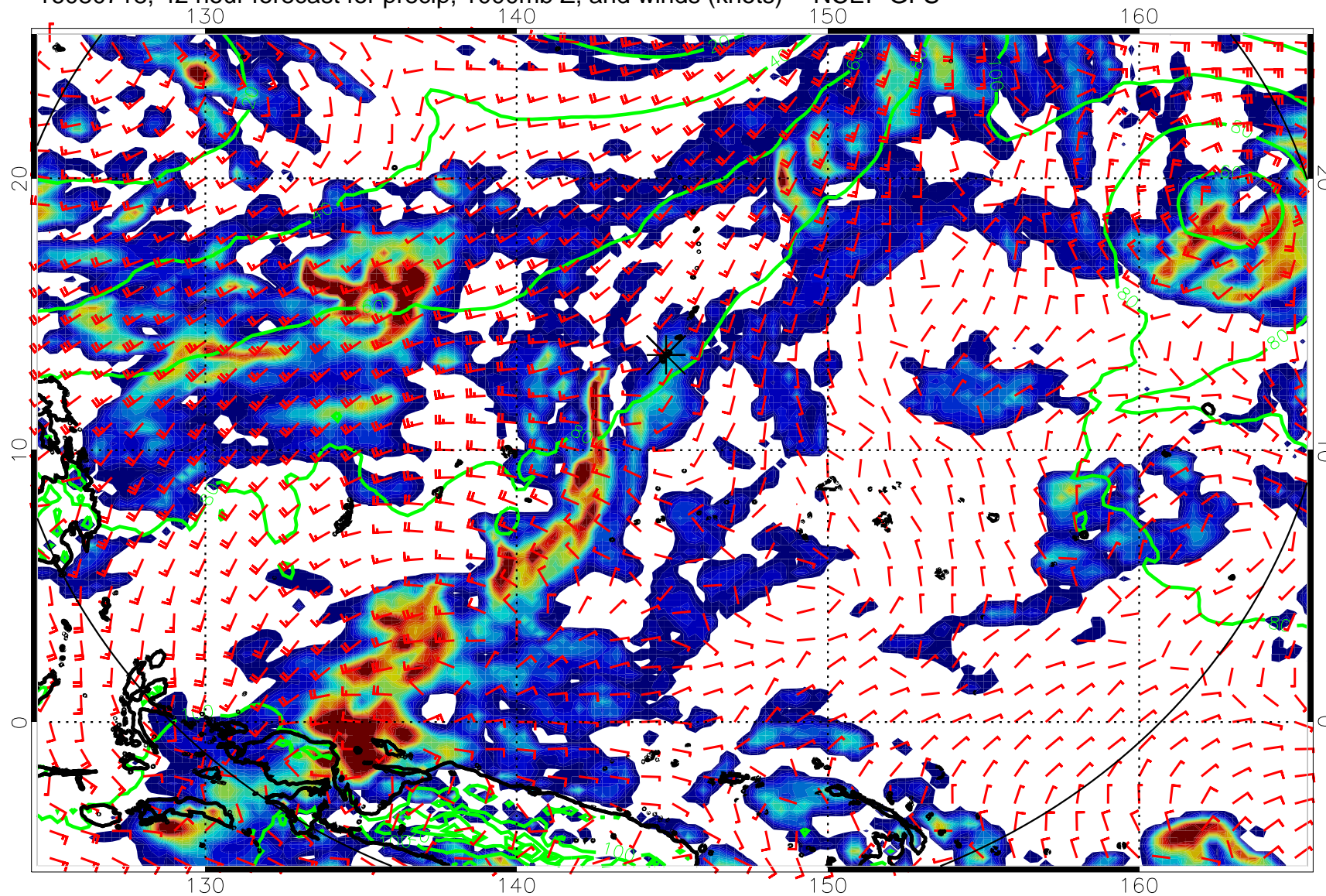
16080718, 42 hour forecast for precip, 1000mb Z, and winds (knots) -- NCEP GFS
