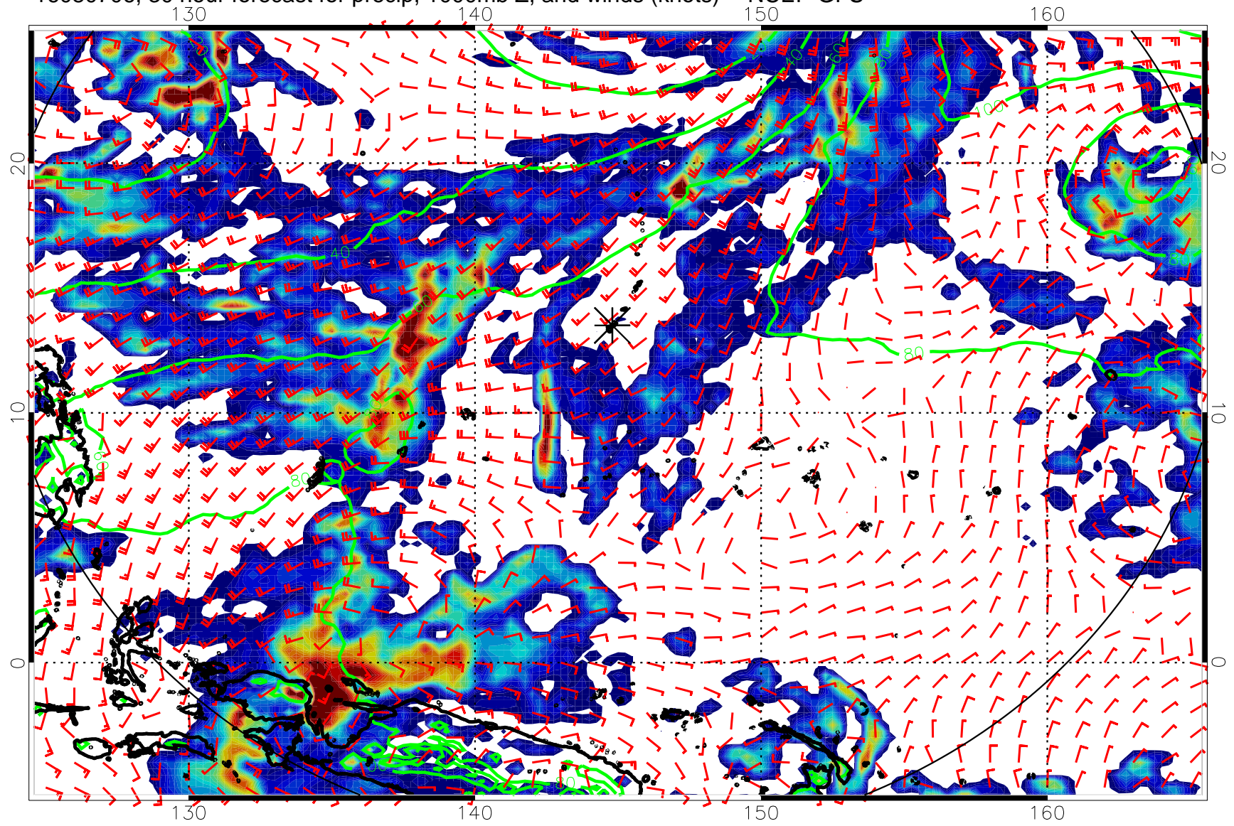
16080706, 30 hour forecast for precip, 1000mb Z, and winds (knots) -- NCEP GFS
