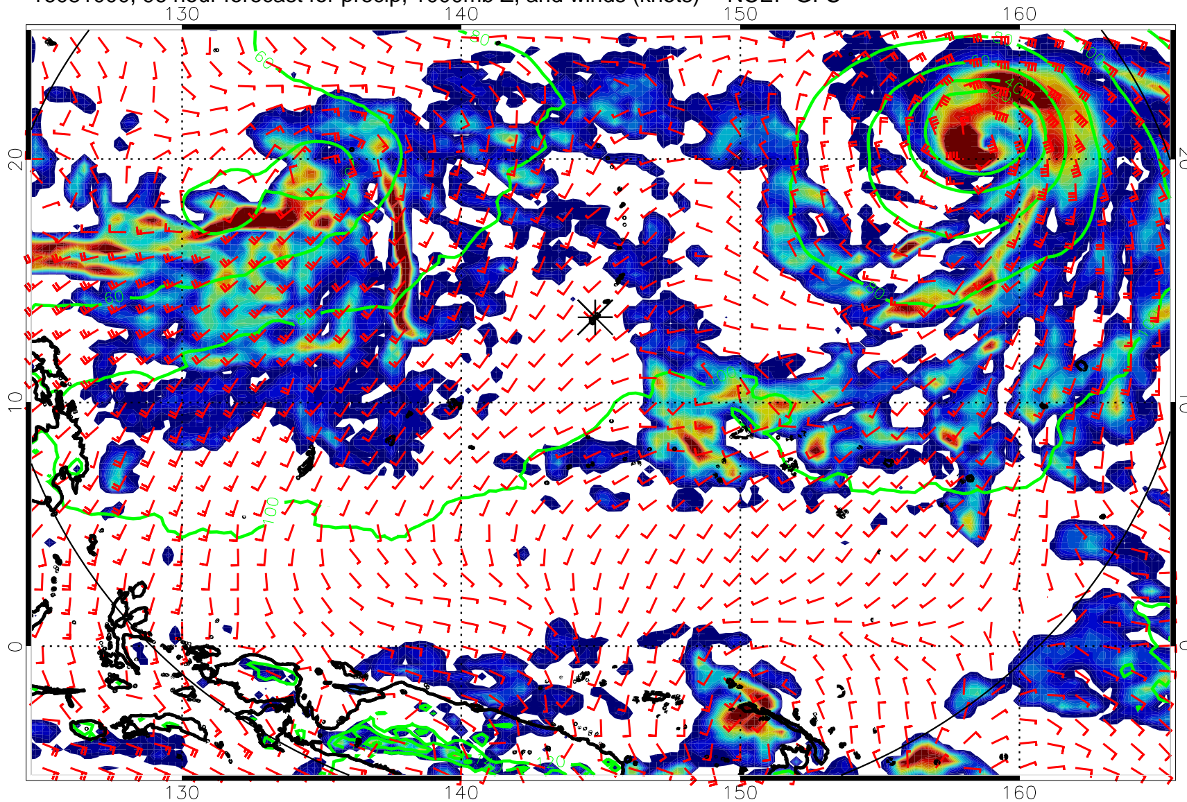
16081000, 96 hour forecast for precip, 1000mb Z, and winds (knots) -- NCEP GFS
