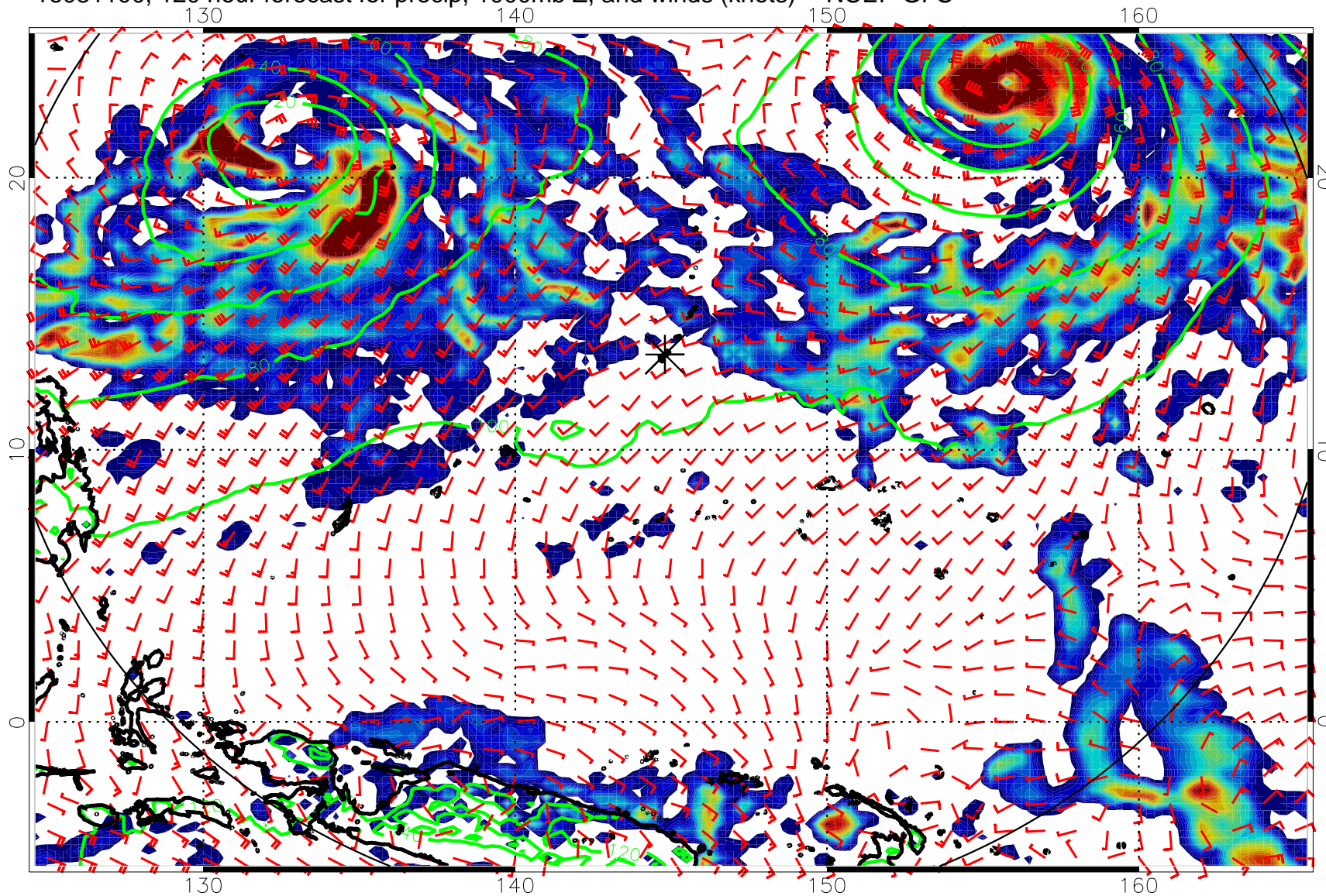
16081100, 120 hour forecast for precip, 1000mb Z, and winds (knots) -- NCEP GFS
