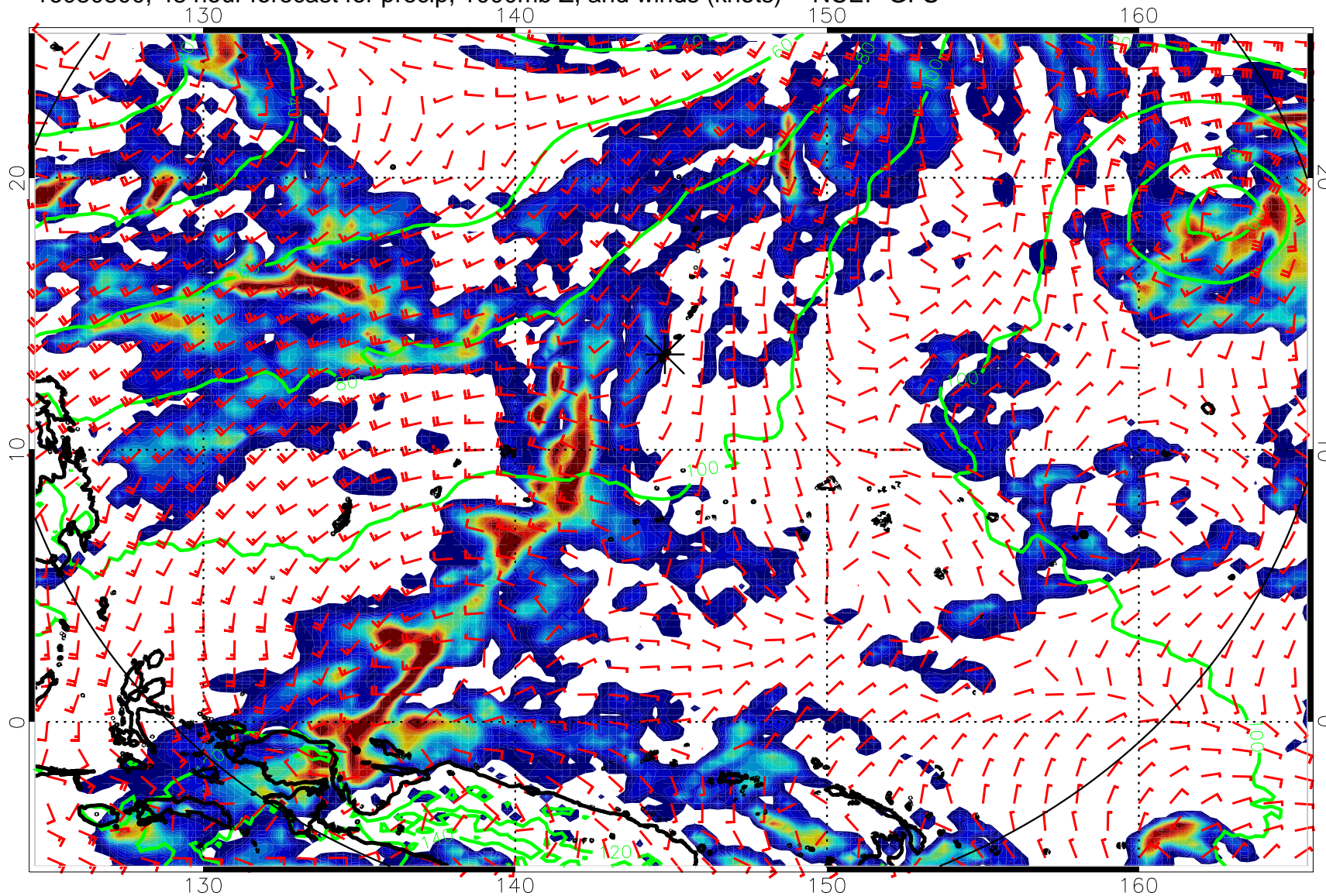
16080800, 48 hour forecast for precip, 1000mb Z, and winds (knots) -- NCEP GFS
