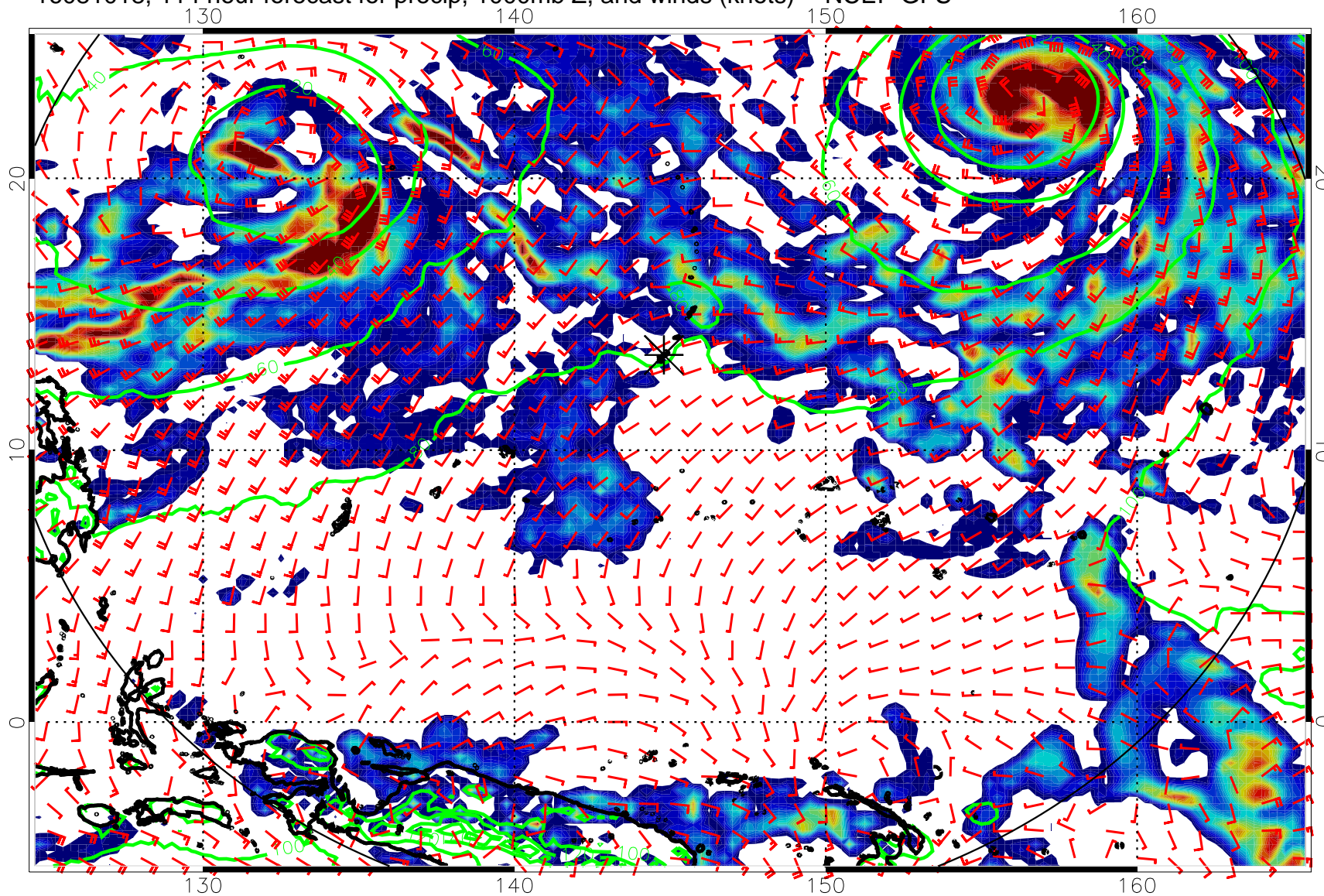
16081018, 114 hour forecast for precip, 1000mb Z, and winds (knots) -- NCEP GFS
