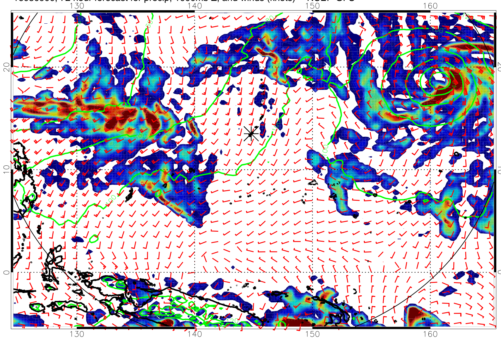
16080900, 72 hour forecast for precip, 1000mb Z, and winds (knots) -- NCEP GFS
