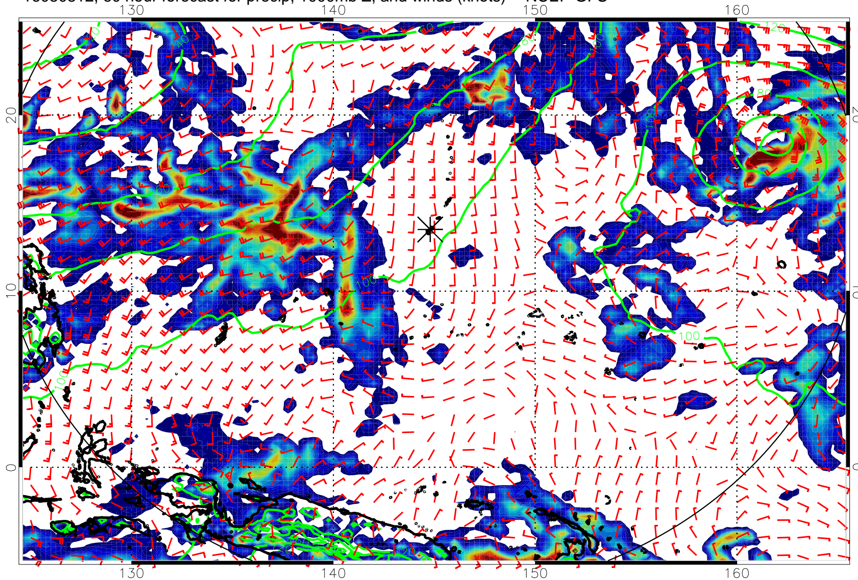
16080812, 60 hour forecast for precip, 1000mb Z, and winds (knots) -- NCEP GFS
