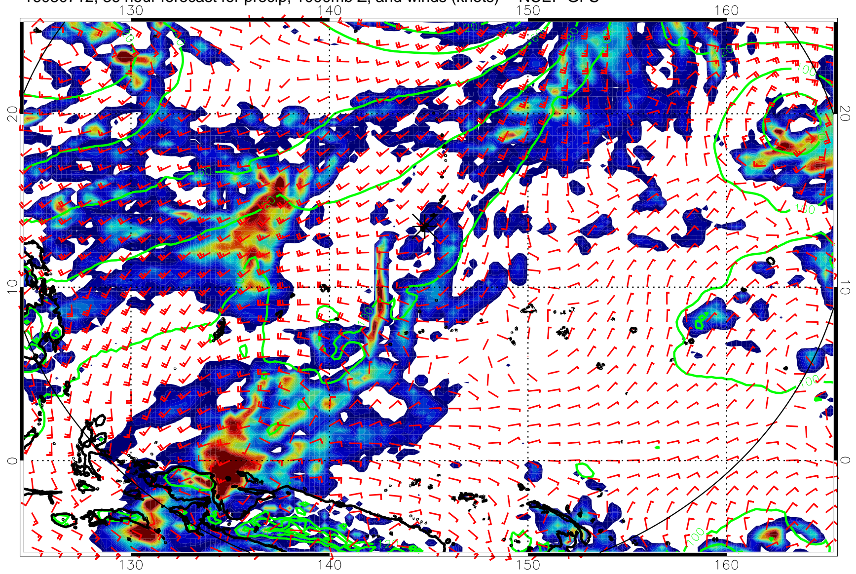
16080712, 36 hour forecast for precip, 1000mb Z, and winds (knots) -- NCEP GFS
