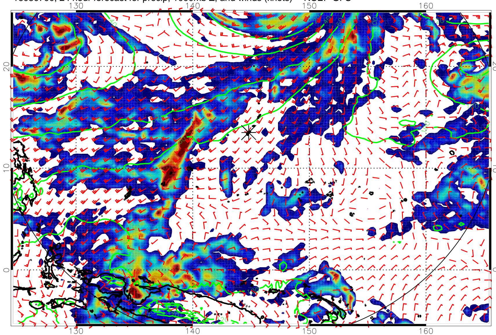
16080700, 24 hour forecast for precip, 1000mb Z, and winds (knots) -- NCEP GFS
