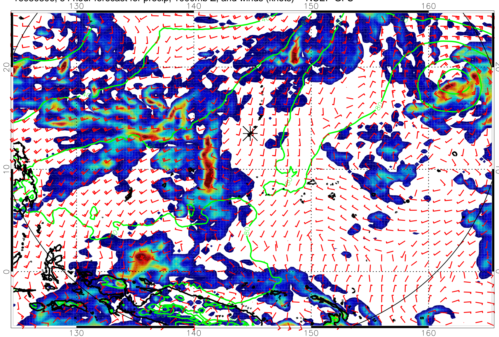
16080806, 54 hour forecast for precip, 1000mb Z, and winds (knots) -- NCEP GFS
