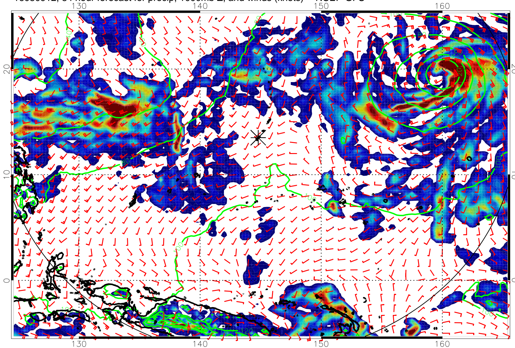
16080912, 84 hour forecast for precip, 1000mb Z, and winds (knots) -- NCEP GFS
