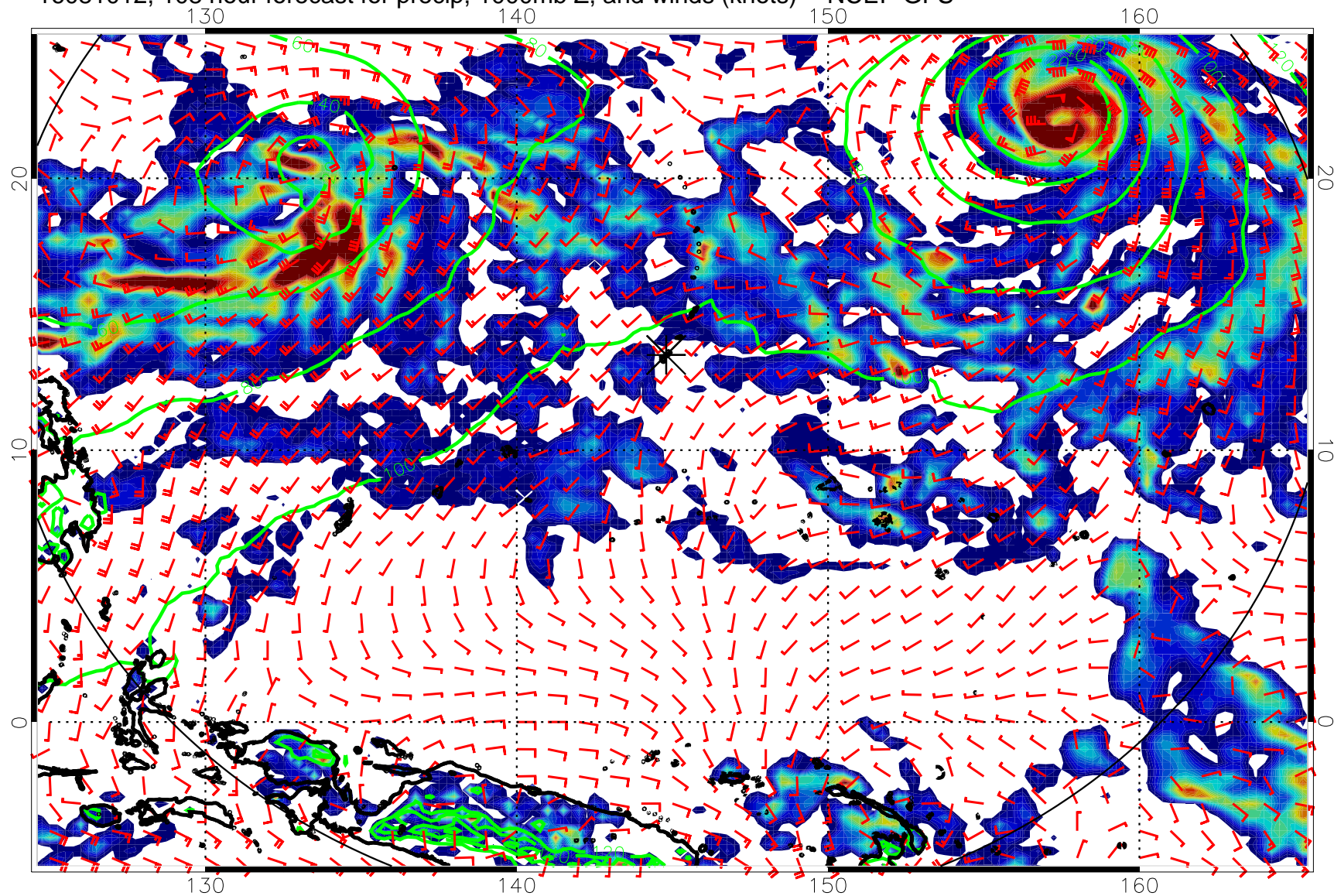
16081012, 108 hour forecast for precip, 1000mb Z, and winds (knots) -- NCEP GFS
