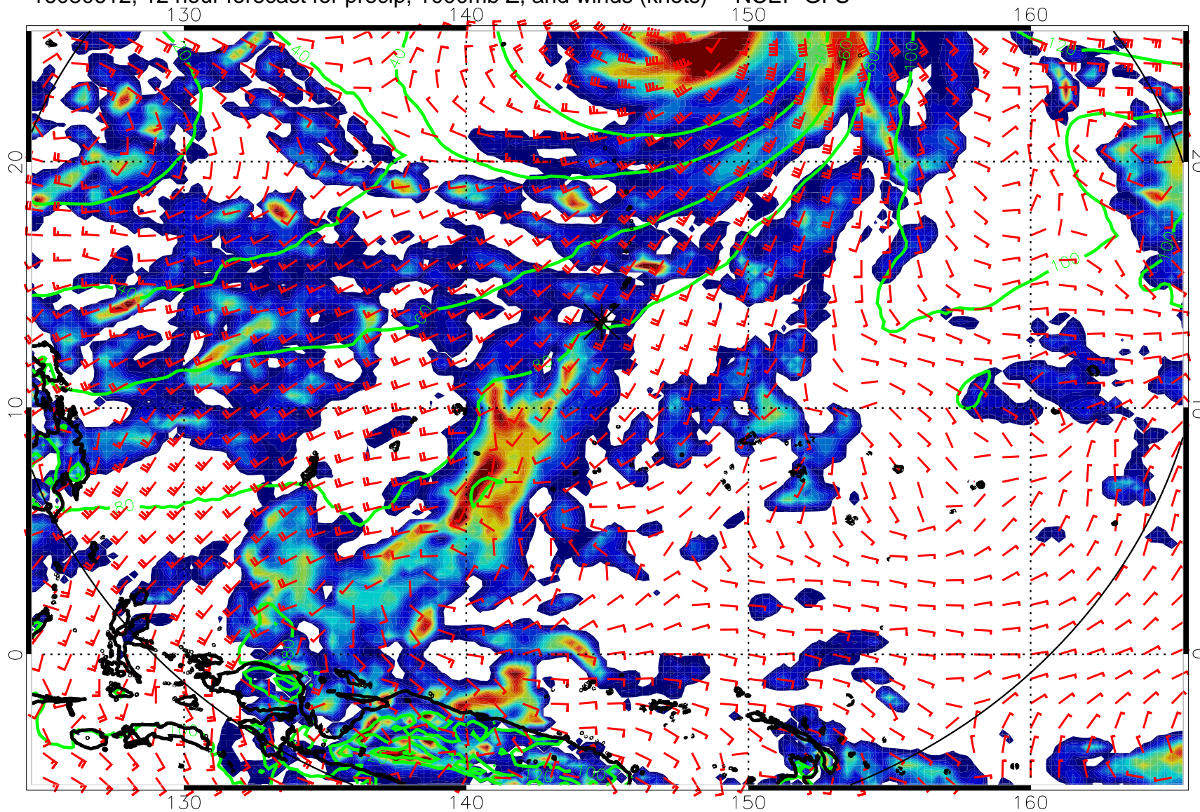
16080612, 12 hour forecast for precip, 1000mb Z, and winds (knots) -- NCEP GFS
