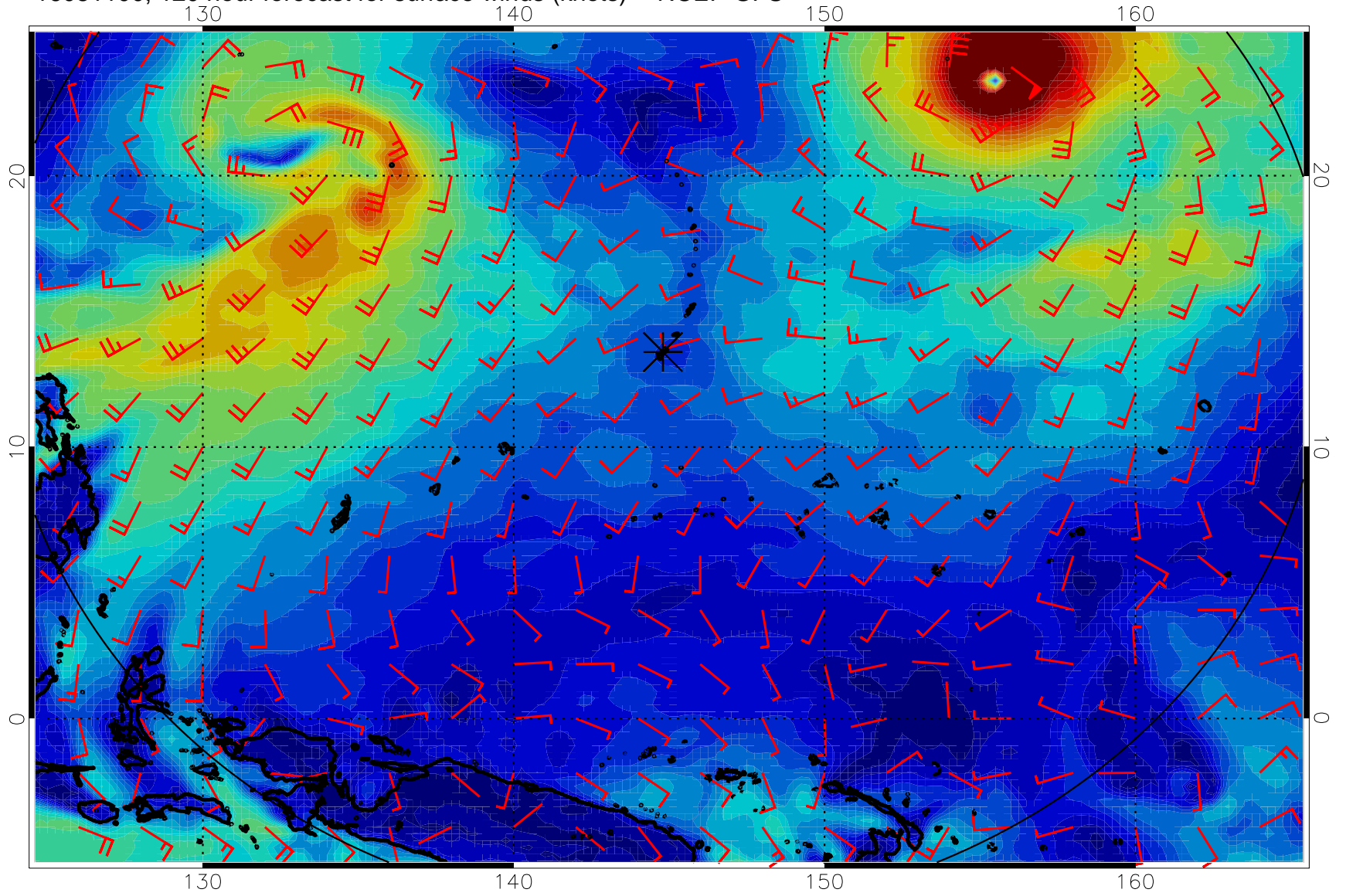
16081100, 120 hour forecast for surface winds (knots) -- NCEP GFS
