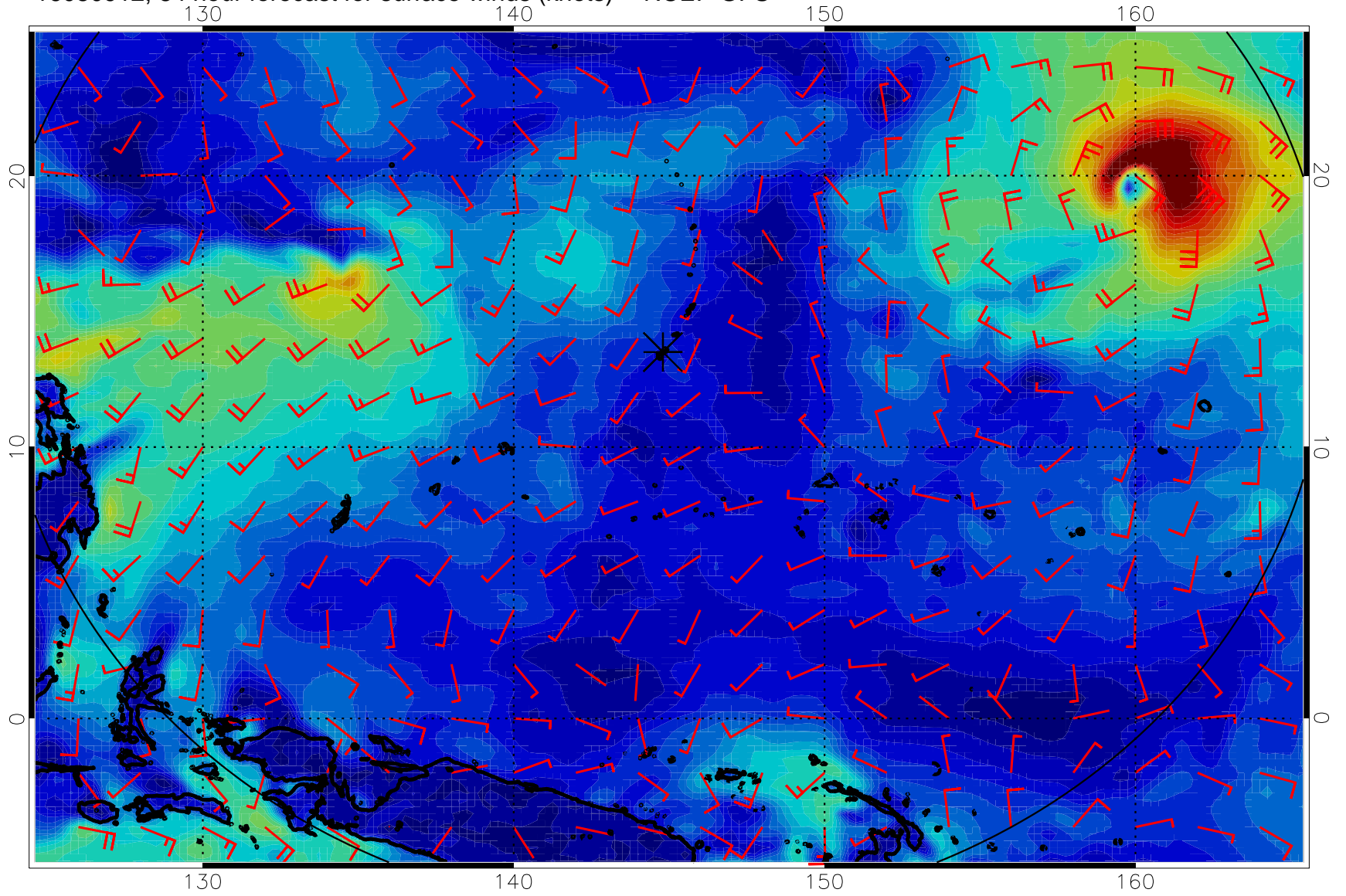
16080912, 84 hour forecast for surface winds (knots) -- NCEP GFS
