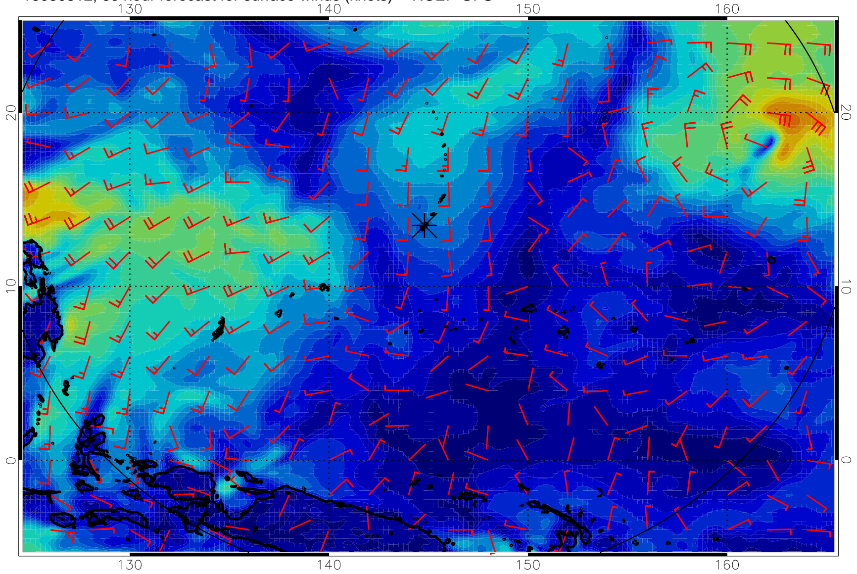
16080812, 60 hour forecast for surface winds (knots) -- NCEP GFS
