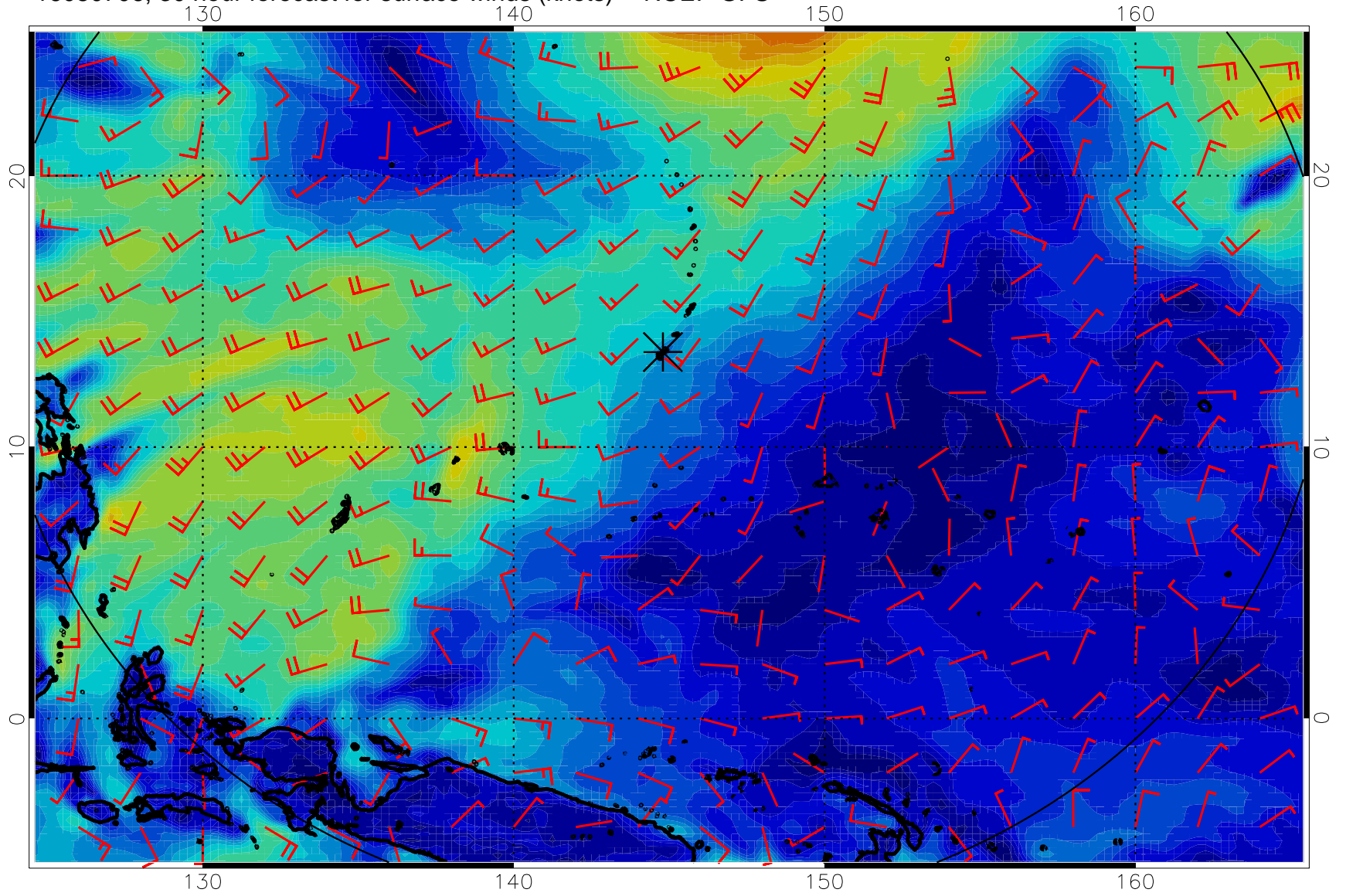
16080706, 30 hour forecast for surface winds (knots) -- NCEP GFS
