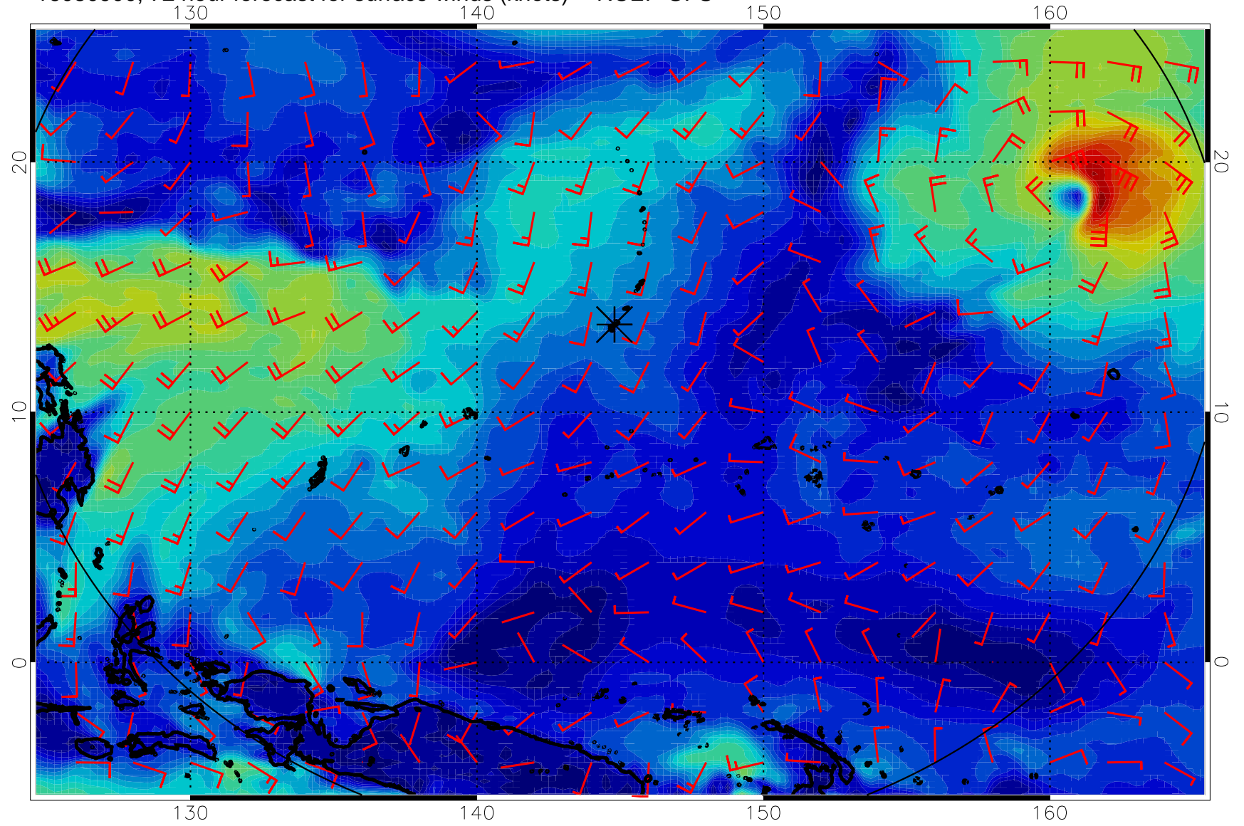
16080900, 72 hour forecast for surface winds (knots) -- NCEP GFS
