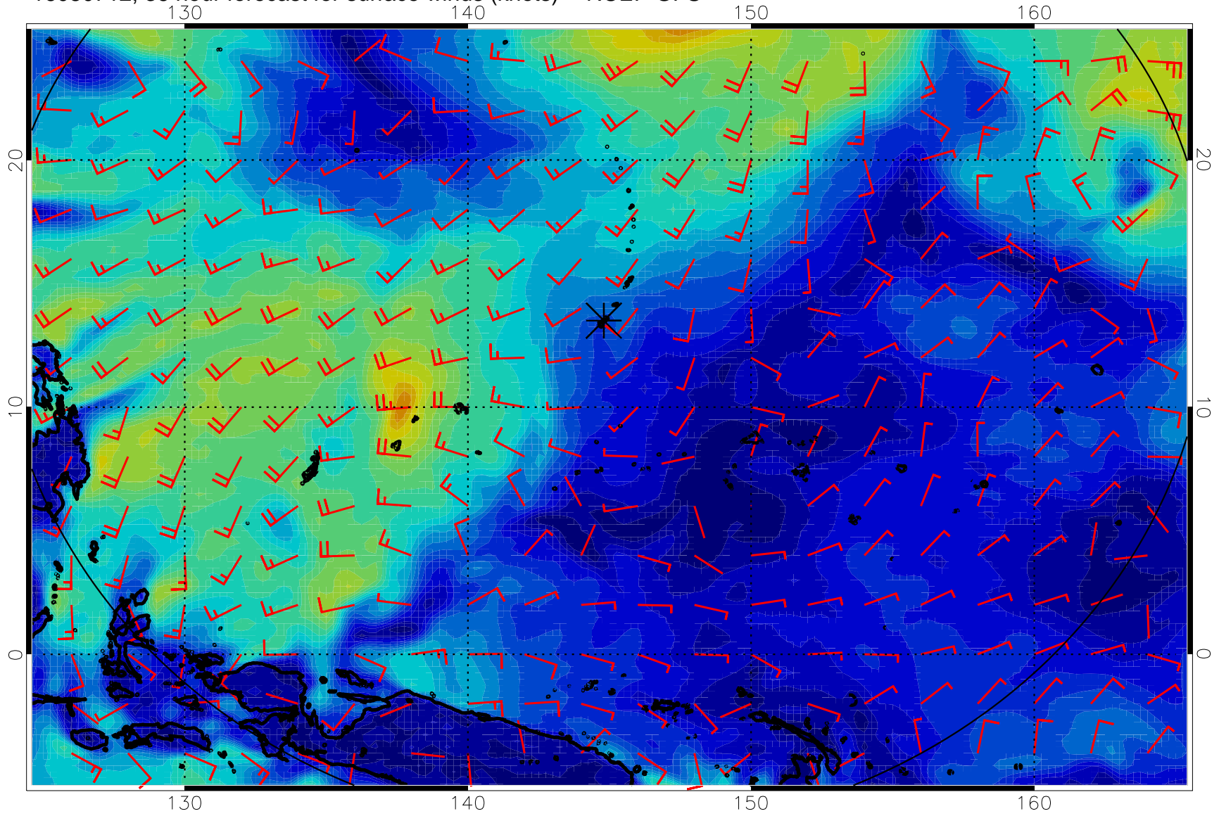
16080712, 36 hour forecast for surface winds (knots) -- NCEP GFS
