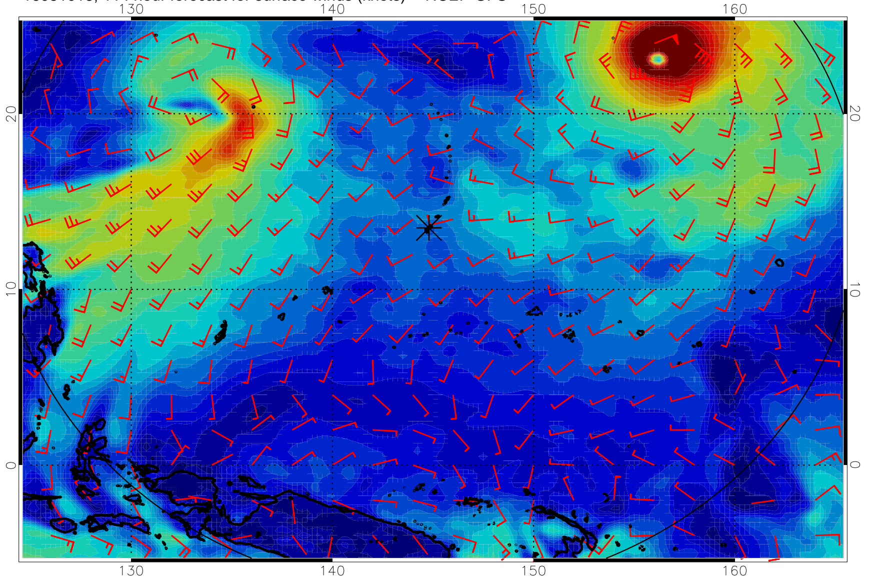
16081018, 114 hour forecast for surface winds (knots) -- NCEP GFS
