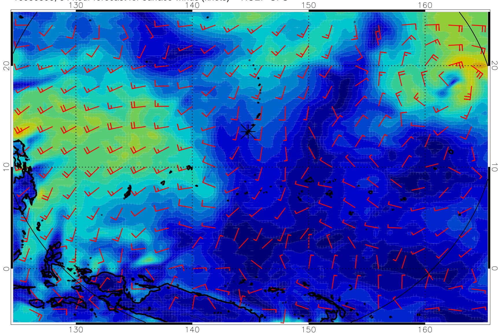
16080806, 54 hour forecast for surface winds (knots) -- NCEP GFS
