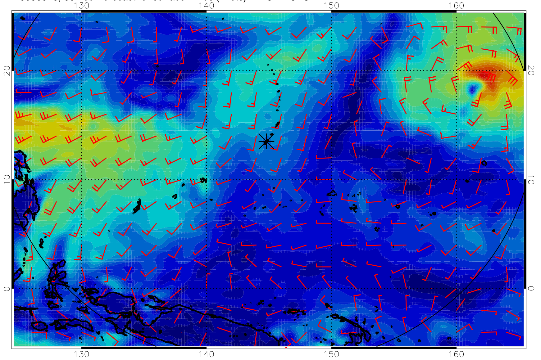
16080818, 66 hour forecast for surface winds (knots) -- NCEP GFS
