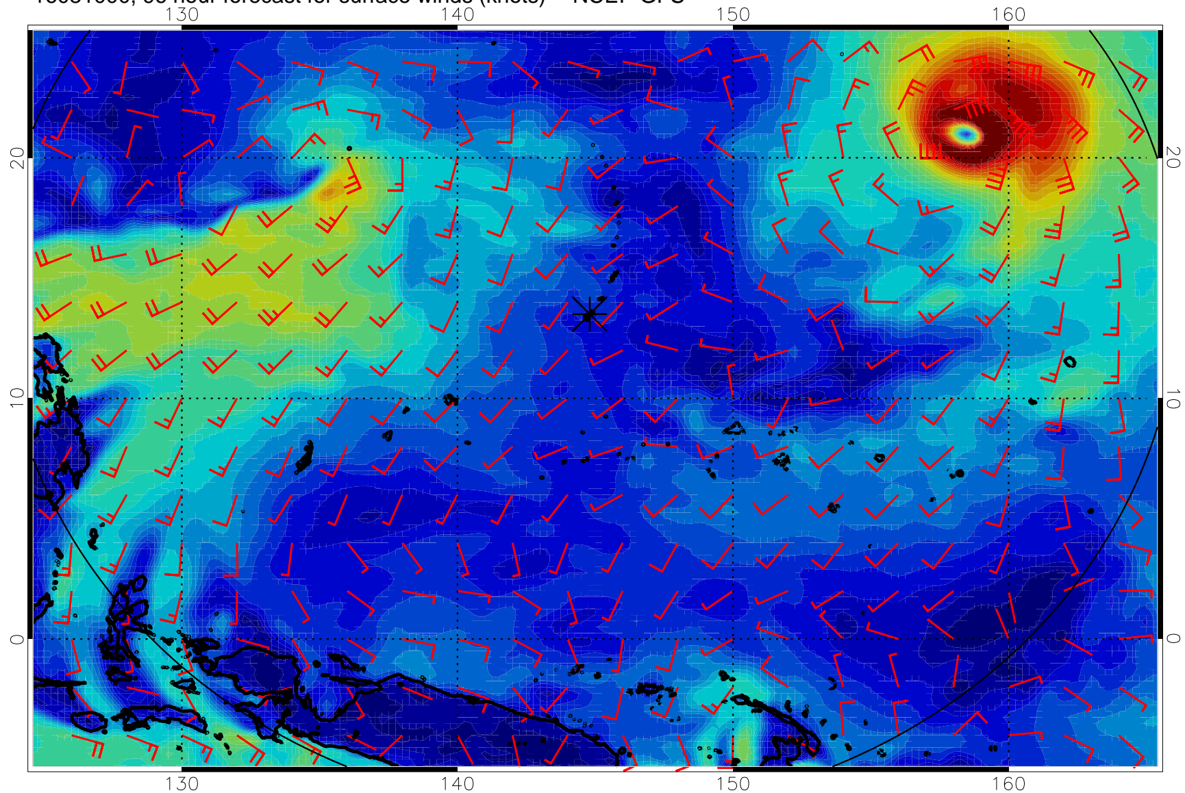
16081000, 96 hour forecast for surface winds (knots) -- NCEP GFS
