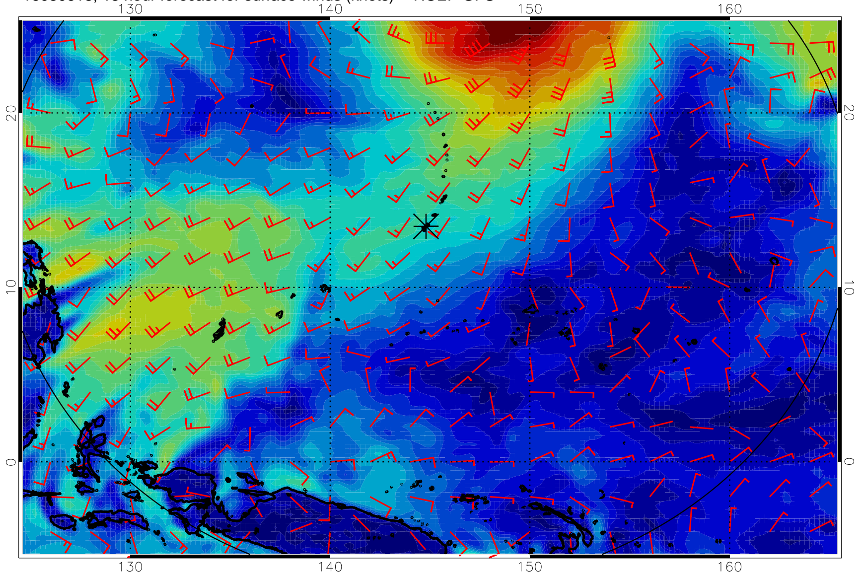
16080618, 18 hour forecast for surface winds (knots) -- NCEP GFS
