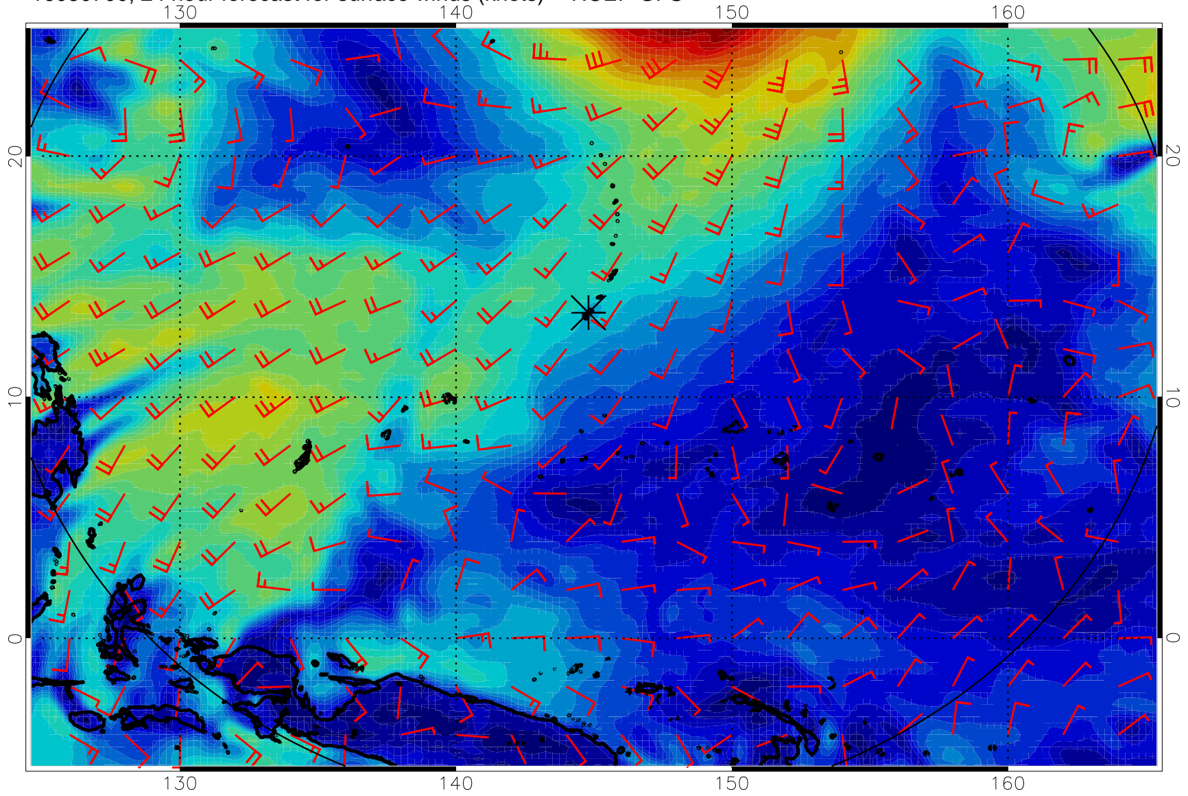
16080700, 24 hour forecast for surface winds (knots) -- NCEP GFS
