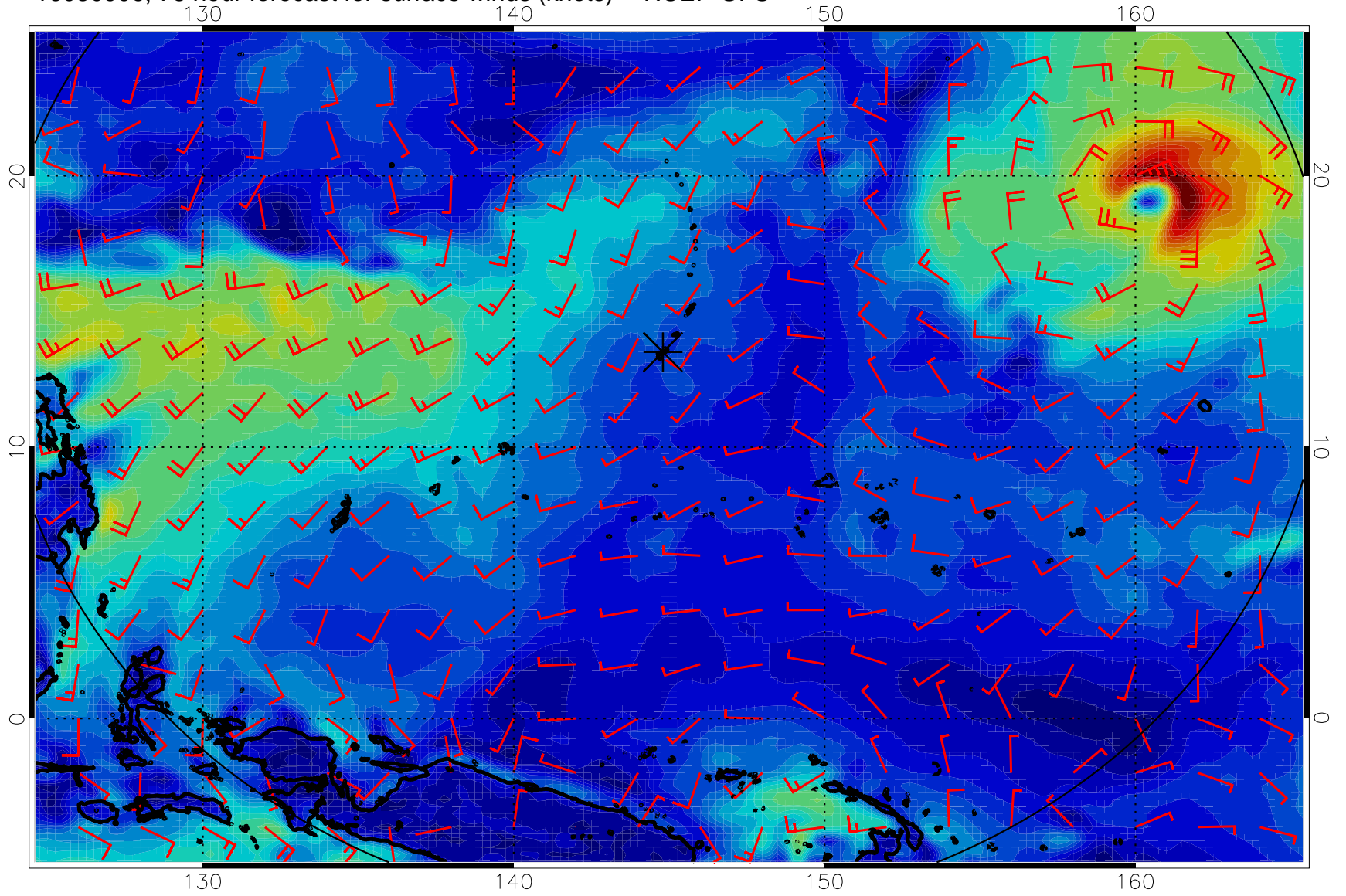
16080906, 78 hour forecast for surface winds (knots) -- NCEP GFS
