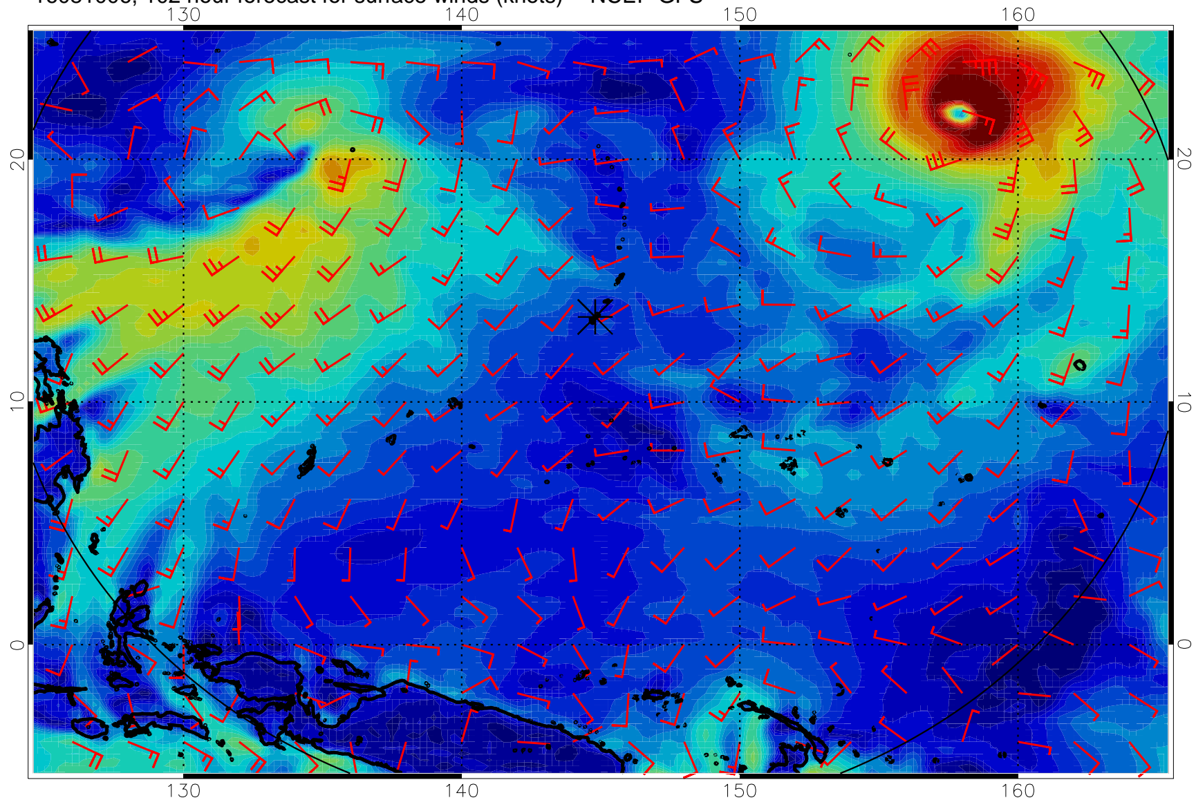
16081006, 102 hour forecast for surface winds (knots) -- NCEP GFS
