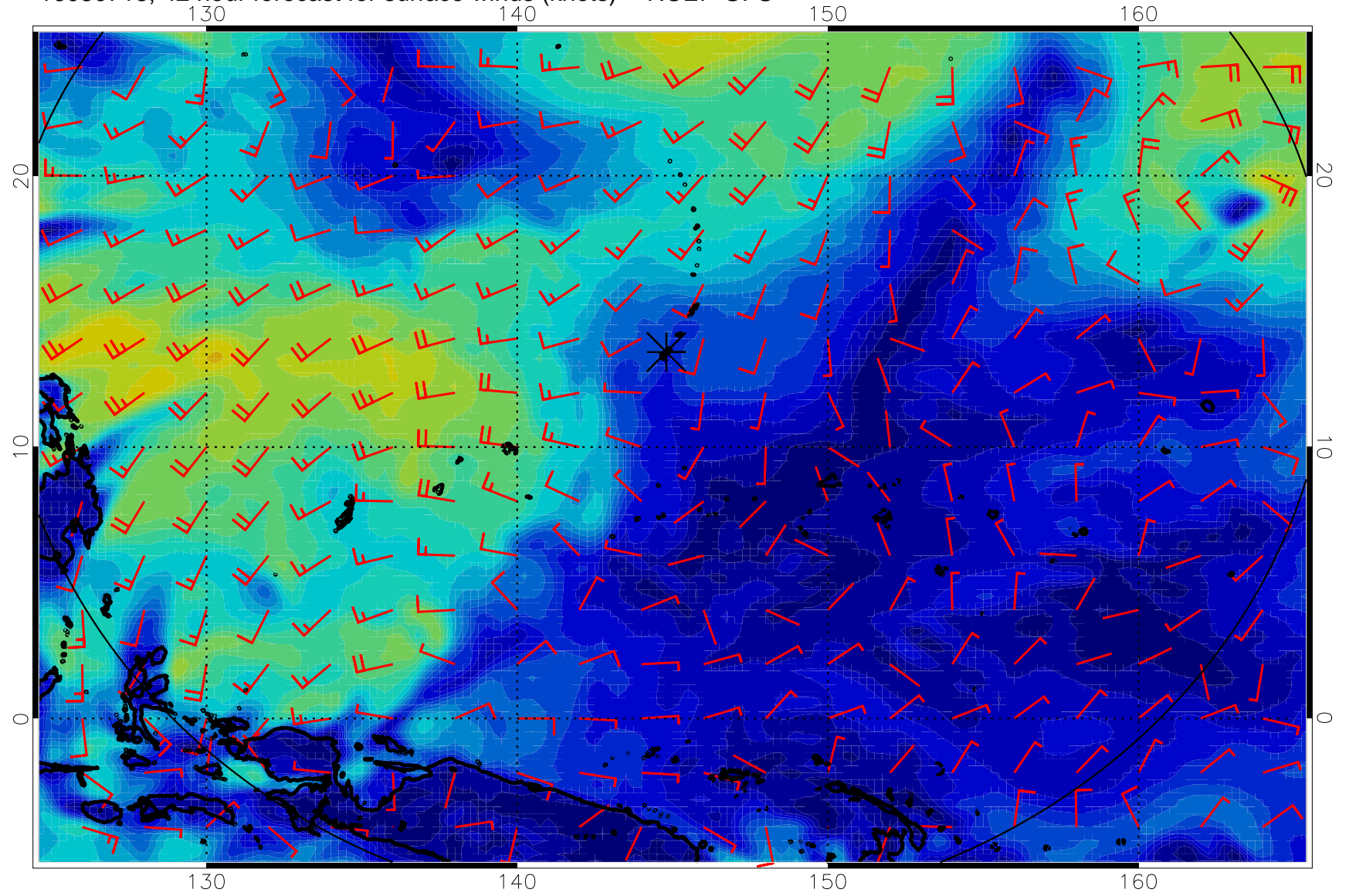
16080718, 42 hour forecast for surface winds (knots) -- NCEP GFS
