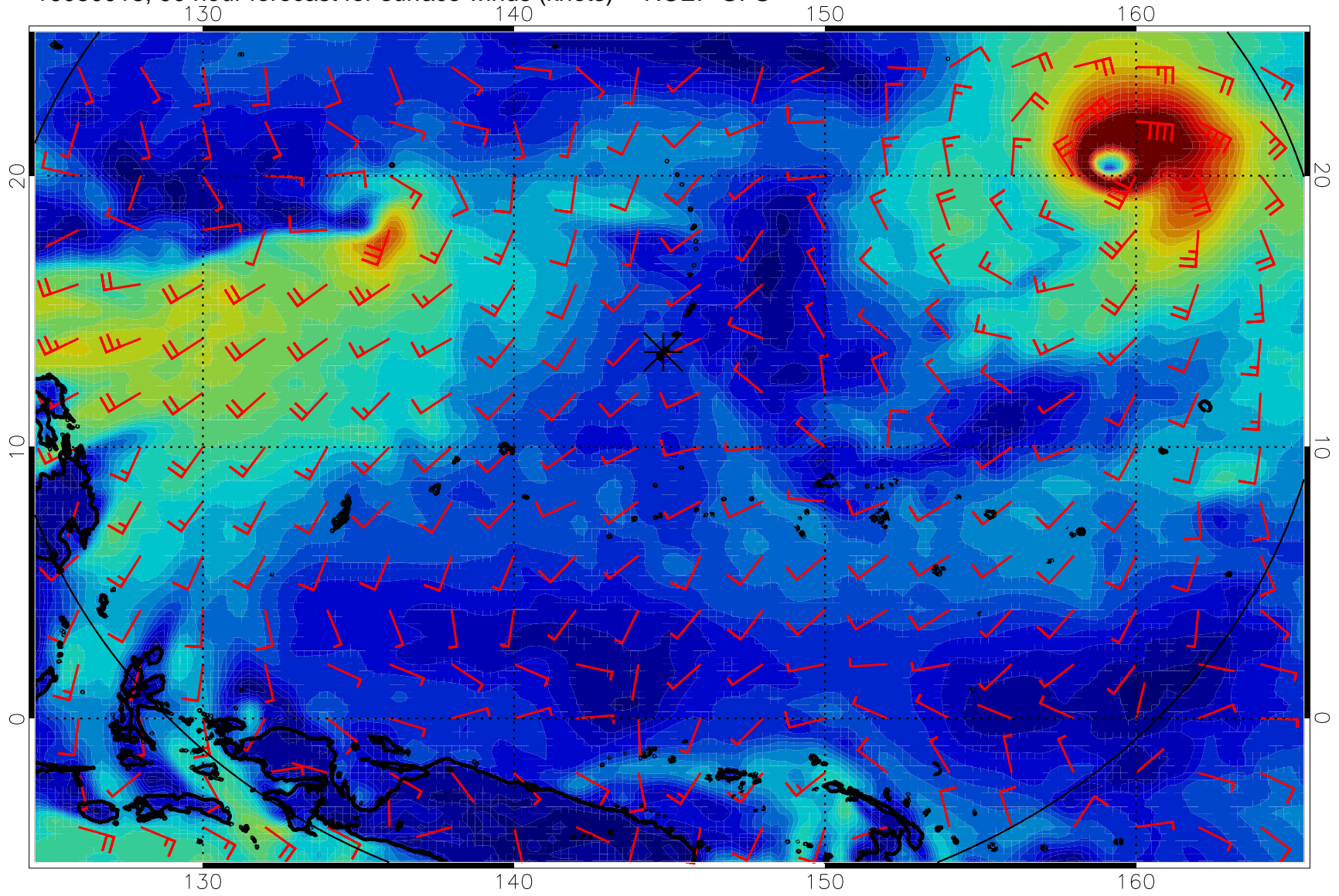
16080918, 90 hour forecast for surface winds (knots) -- NCEP GFS
