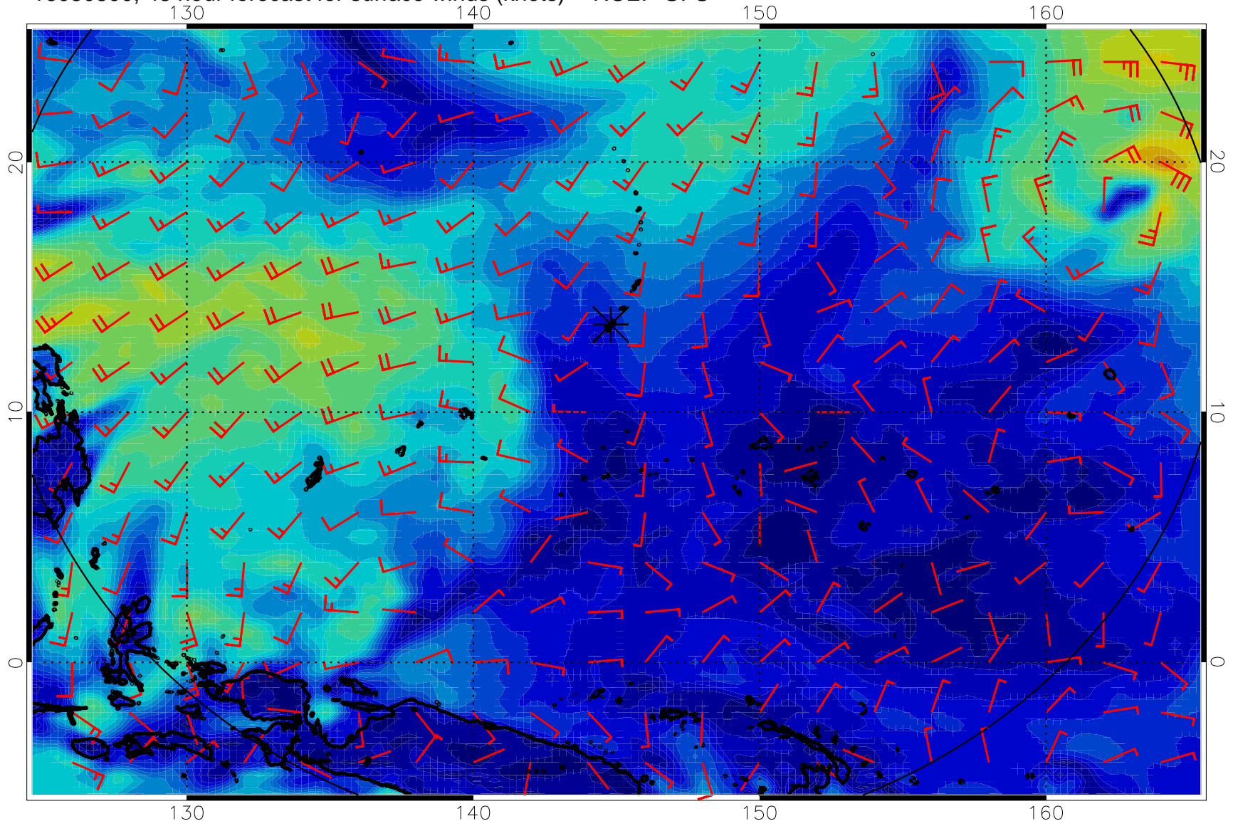
16080800, 48 hour forecast for surface winds (knots) -- NCEP GFS
