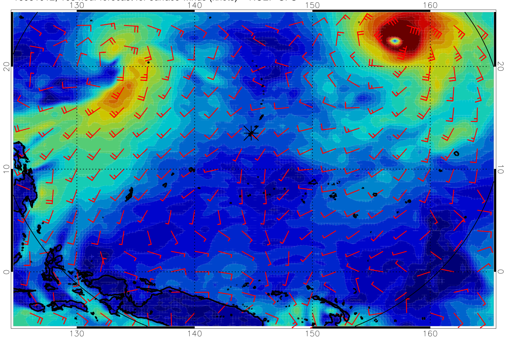
16081012, 108 hour forecast for surface winds (knots) -- NCEP GFS
