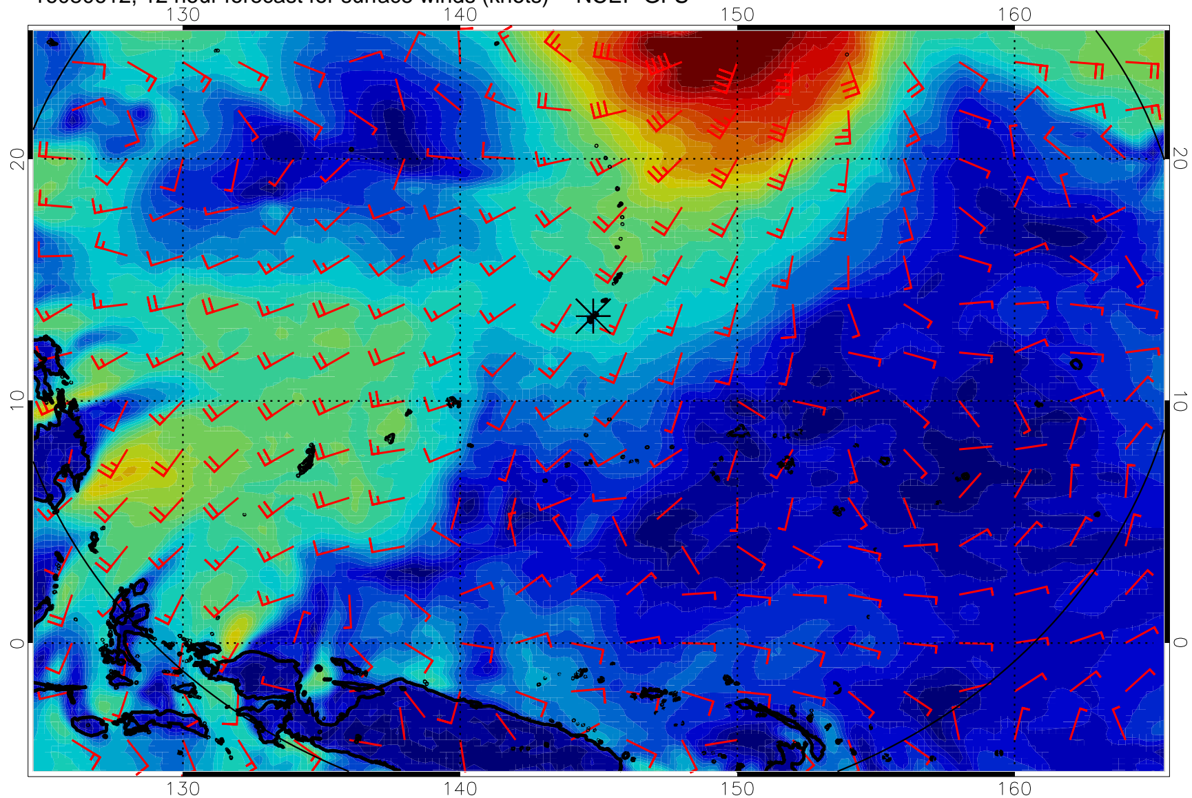
16080612, 12 hour forecast for surface winds (knots) -- NCEP GFS
