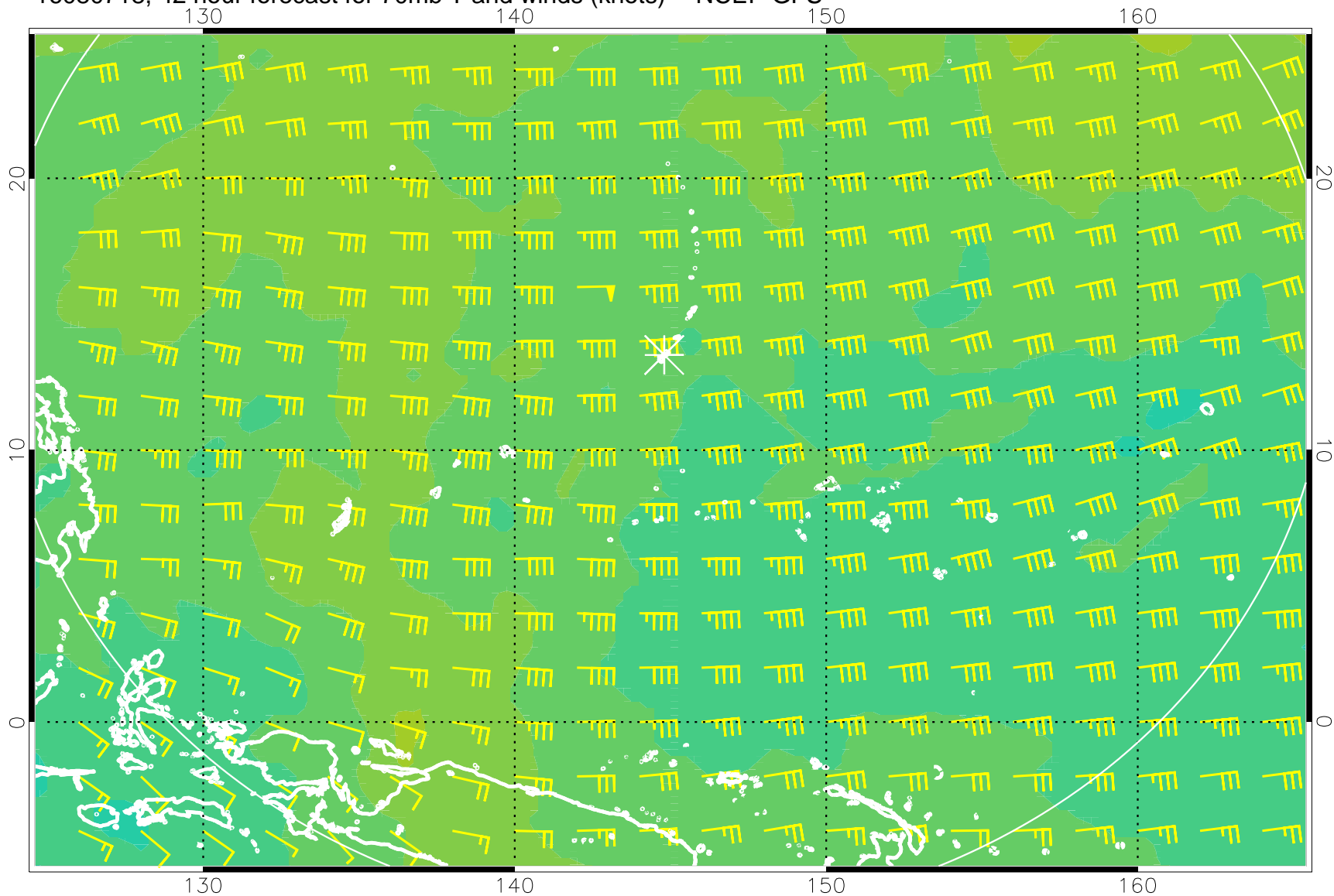
16080718, 42 hour forecast for 70mb T and winds (knots) -- NCEP GFS
