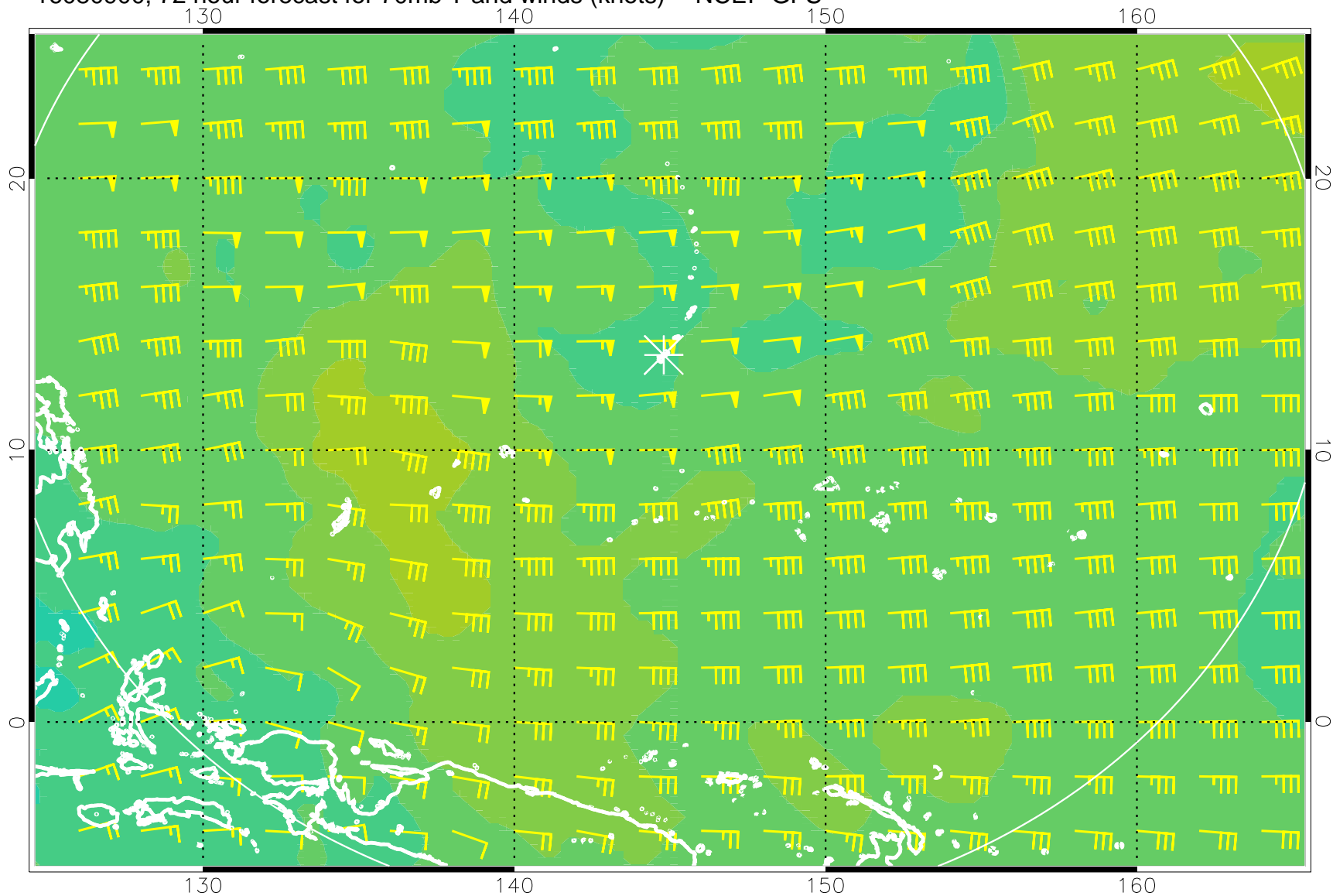
16080900, 72 hour forecast for 70mb T and winds (knots) -- NCEP GFS
