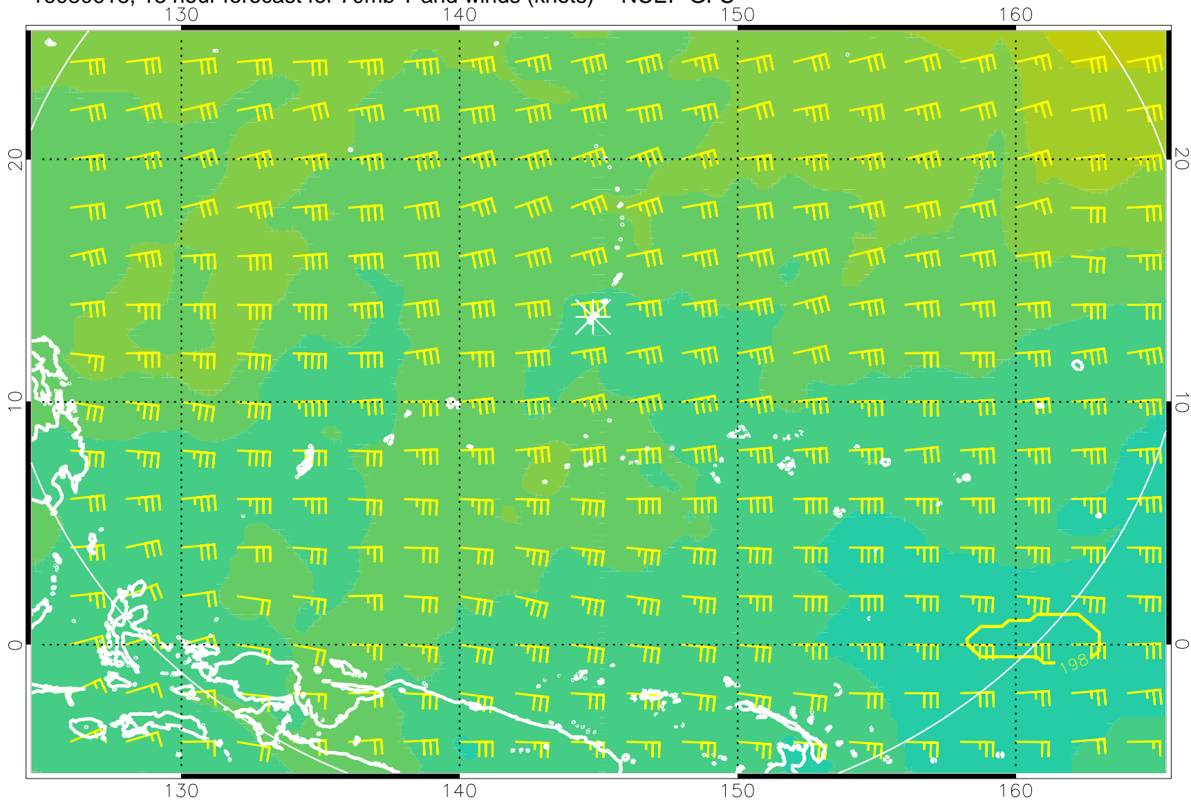
16080618, 18 hour forecast for 70mb T and winds (knots) -- NCEP GFS
