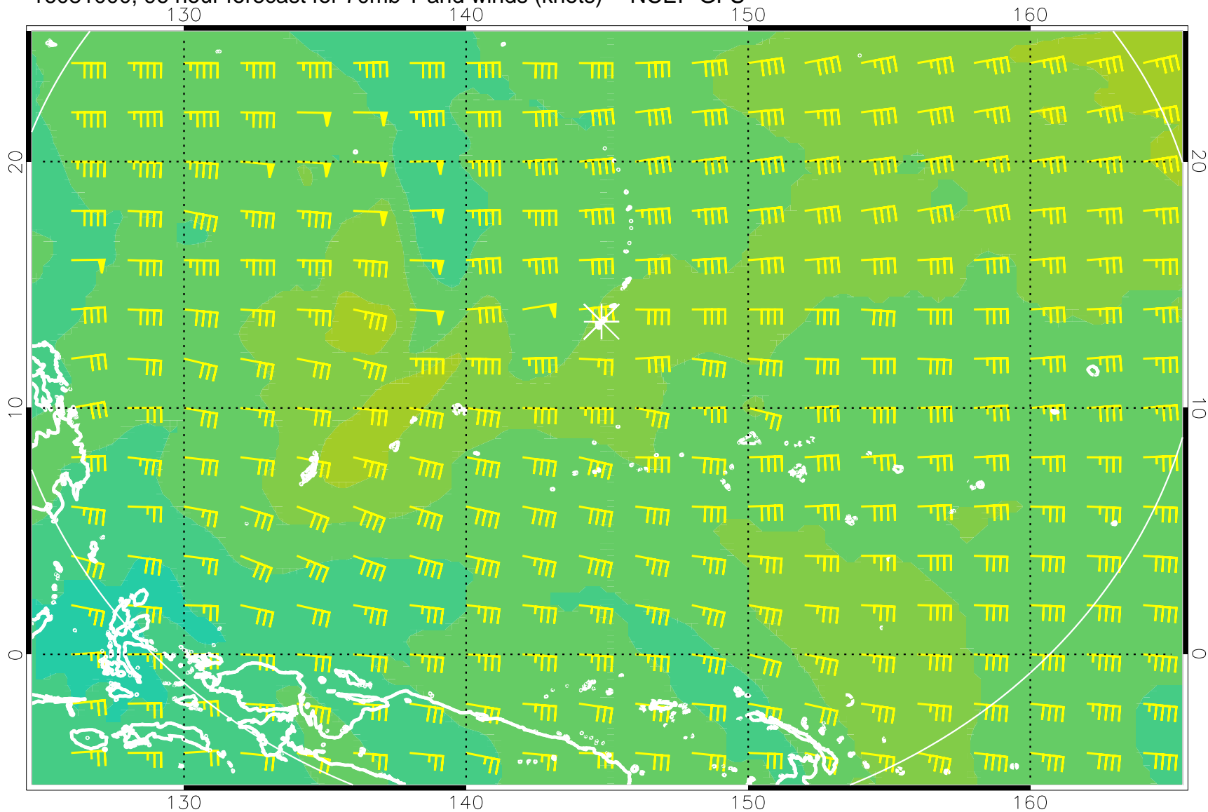
16081000, 96 hour forecast for 70mb T and winds (knots) -- NCEP GFS
