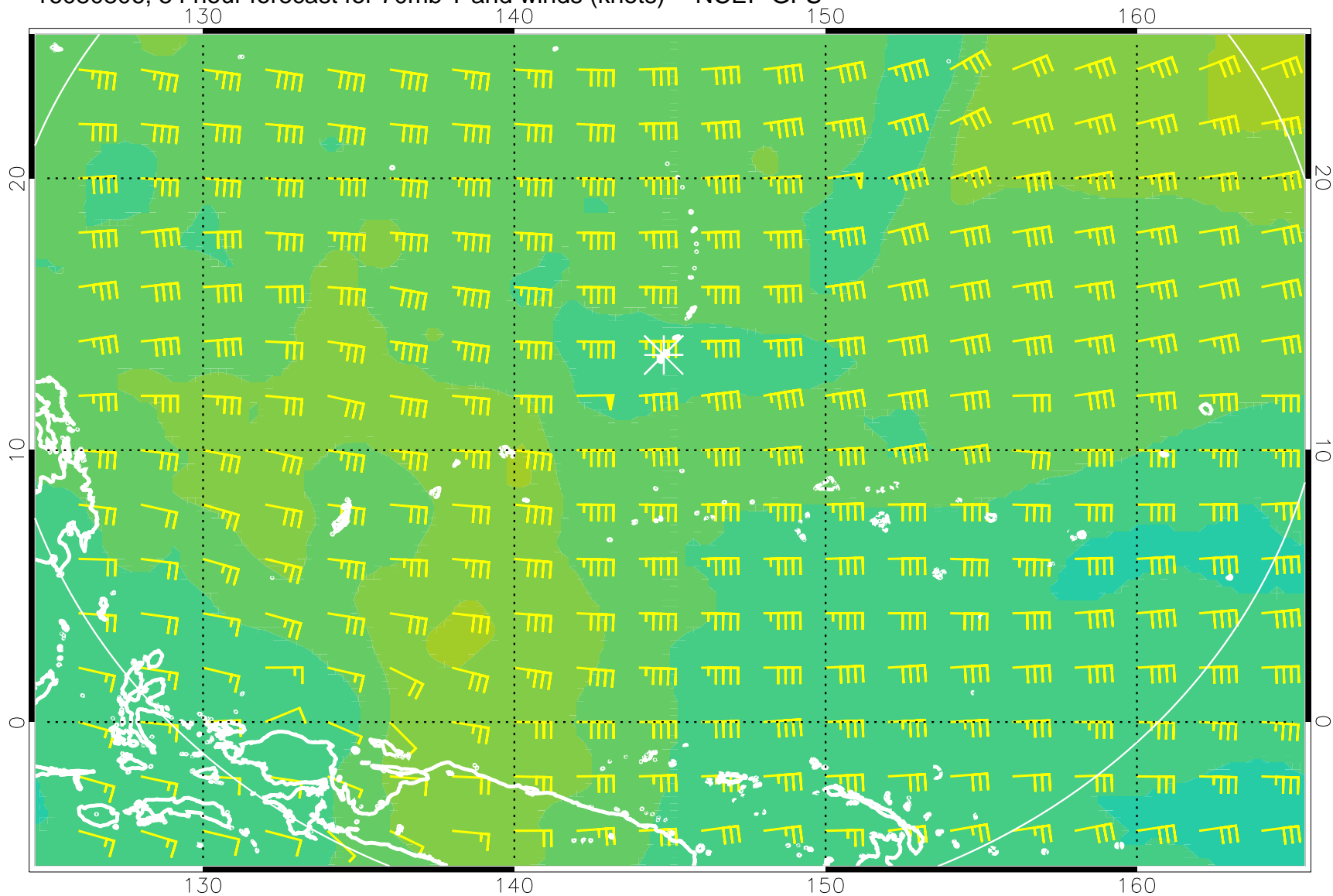
16080806, 54 hour forecast for 70mb T and winds (knots) -- NCEP GFS
