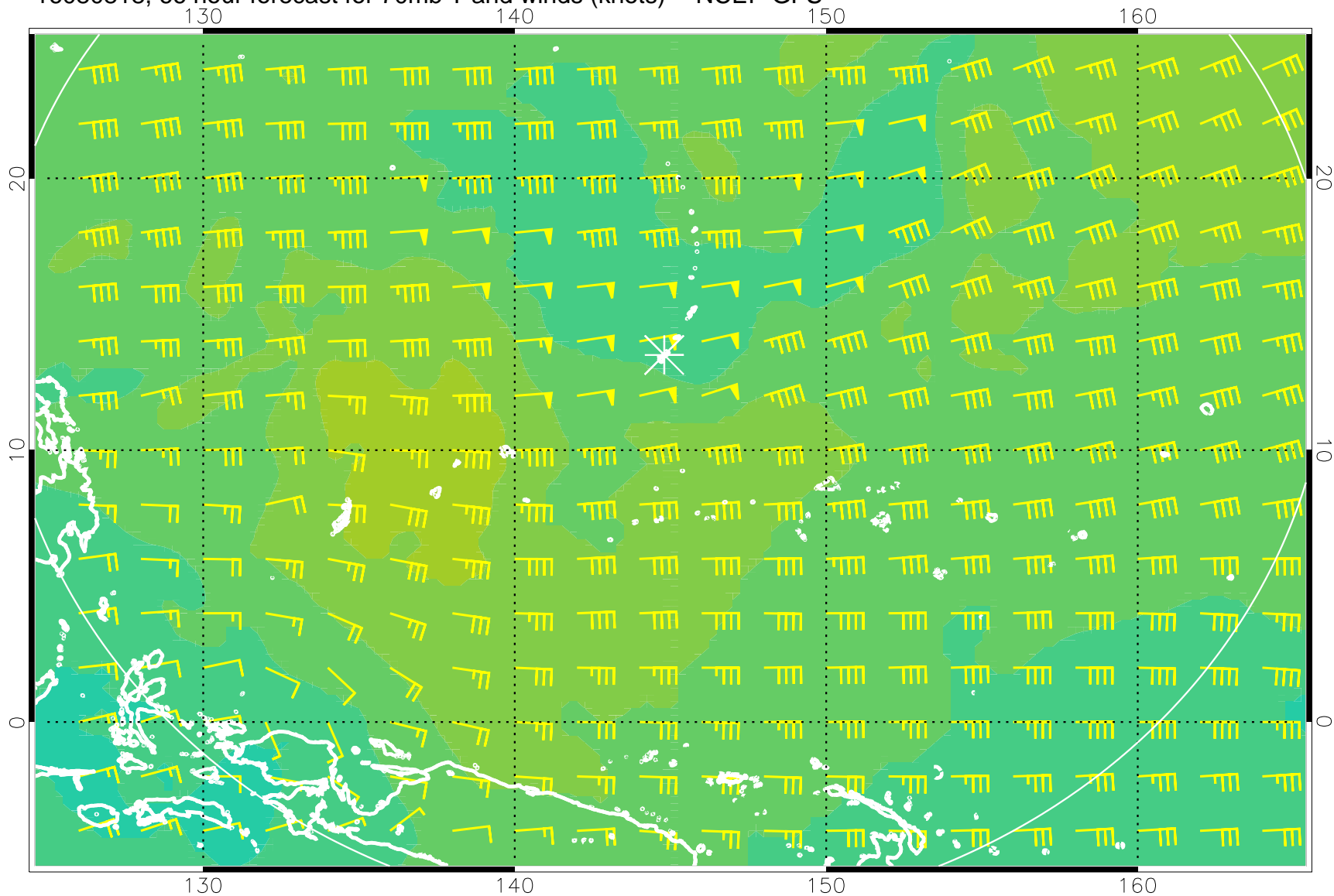
16080818, 66 hour forecast for 70mb T and winds (knots) -- NCEP GFS
