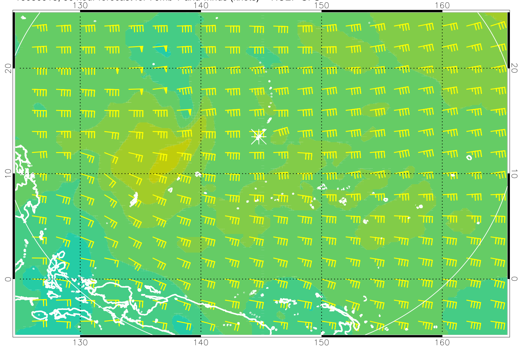
16080918, 90 hour forecast for 70mb T and winds (knots) -- NCEP GFS
