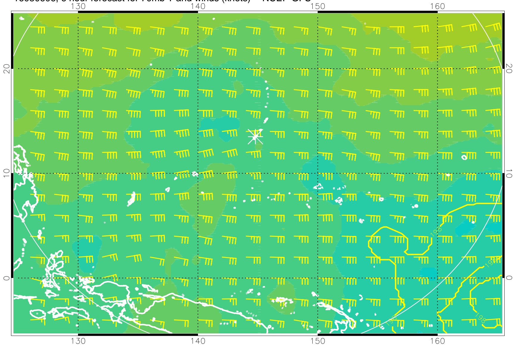
16080606, 6 hour forecast for 70mb T and winds (knots) -- NCEP GFS
