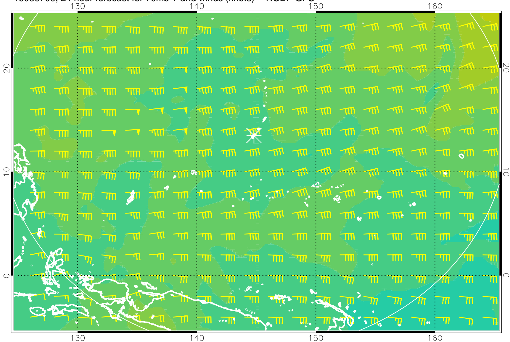
16080700, 24 hour forecast for 70mb T and winds (knots) -- NCEP GFS
