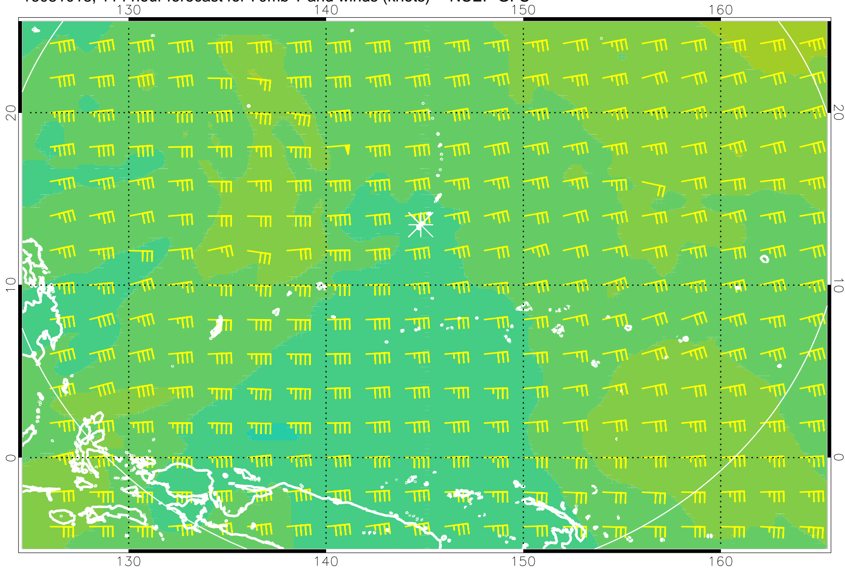
16081018, 114 hour forecast for 70mb T and winds (knots) -- NCEP GFS
