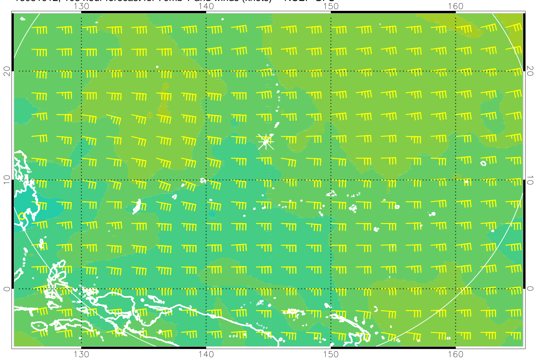
16081012, 108 hour forecast for 70mb T and winds (knots) -- NCEP GFS
