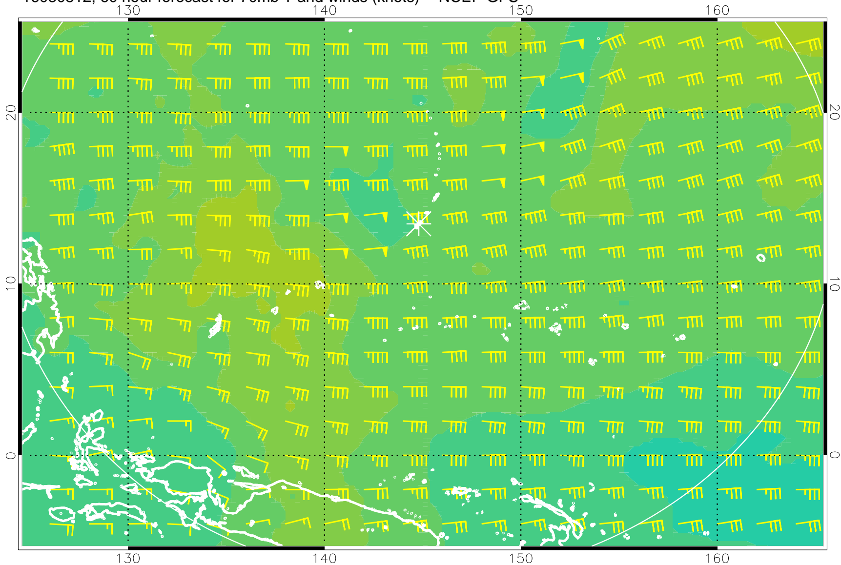
16080812, 60 hour forecast for 70mb T and winds (knots) -- NCEP GFS
