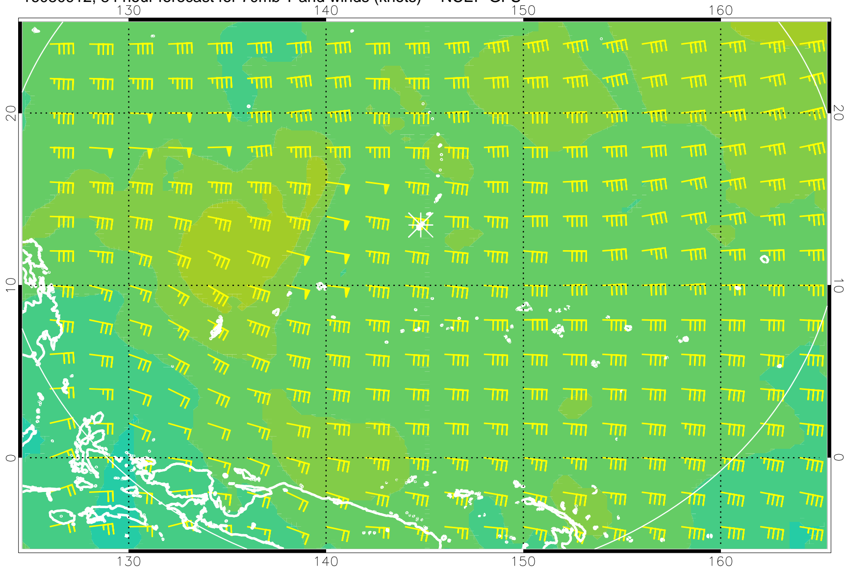
16080912, 84 hour forecast for 70mb T and winds (knots) -- NCEP GFS
