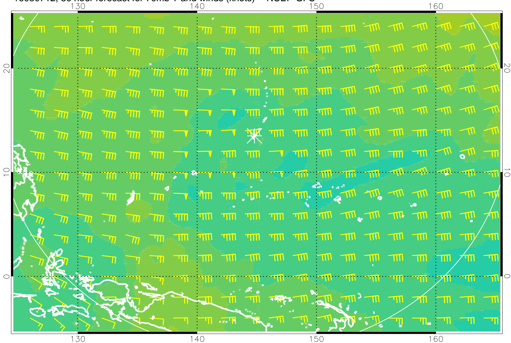
16080712, 36 hour forecast for 70mb T and winds (knots) -- NCEP GFS
