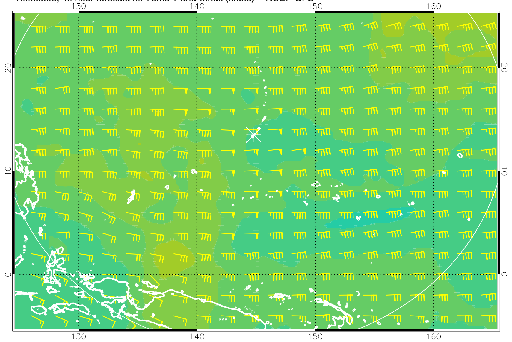
16080800, 48 hour forecast for 70mb T and winds (knots) -- NCEP GFS
