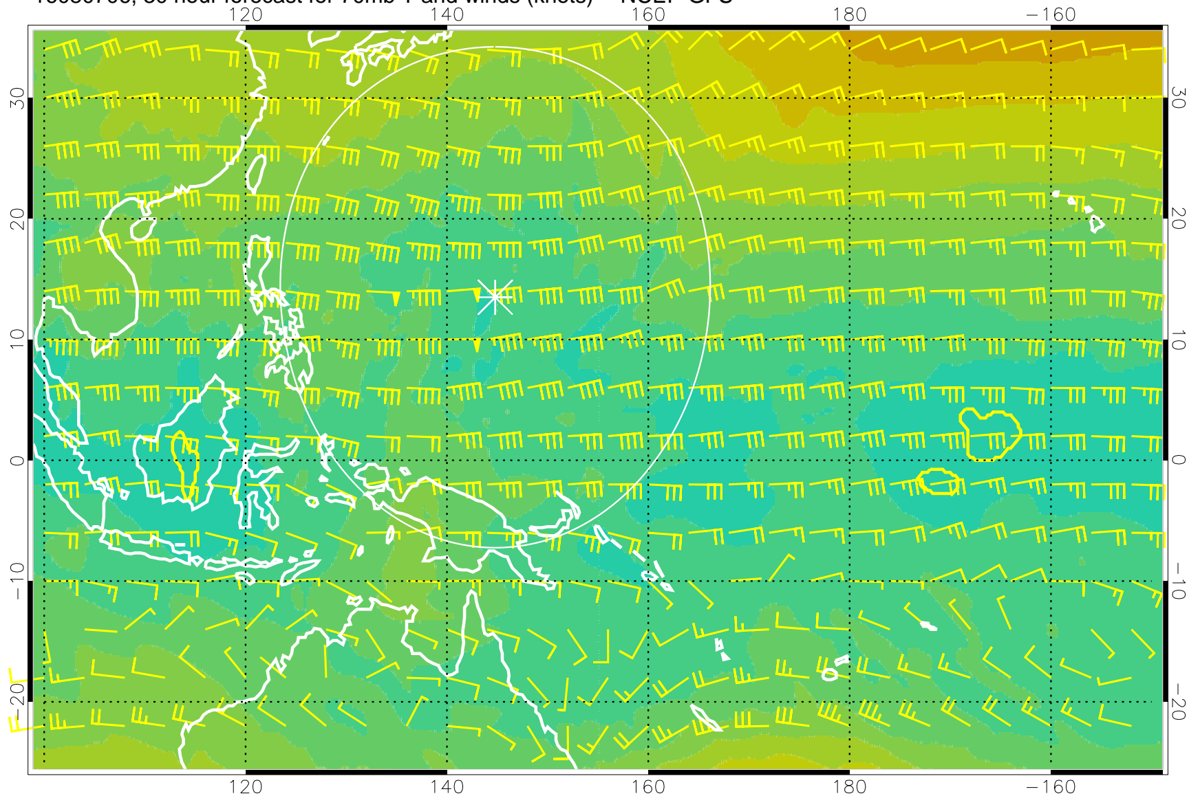
16080706, 30 hour forecast for 70mb T and winds (knots) -- NCEP GFS
