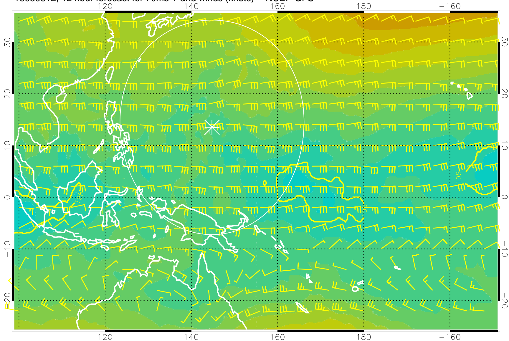
16080612, 12 hour forecast for 70mb T and winds (knots) -- NCEP GFS
