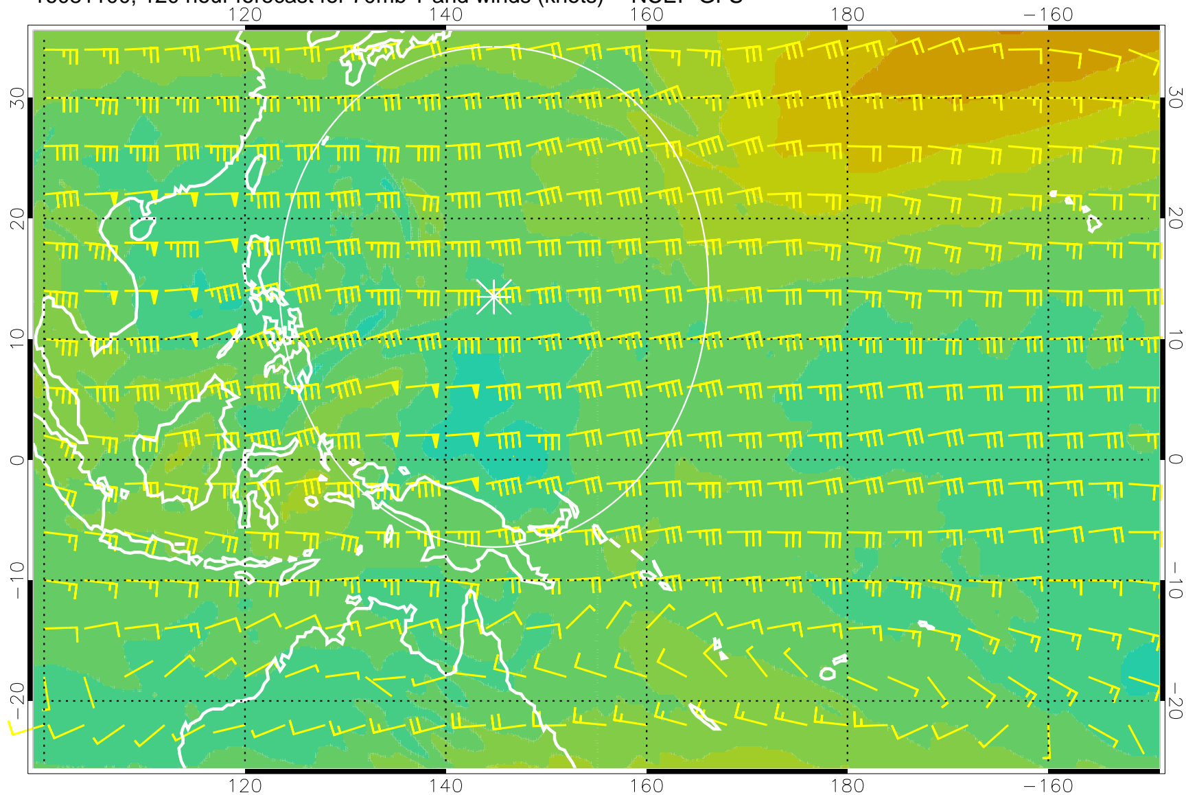
16081100, 120 hour forecast for 70mb T and winds (knots) -- NCEP GFS
