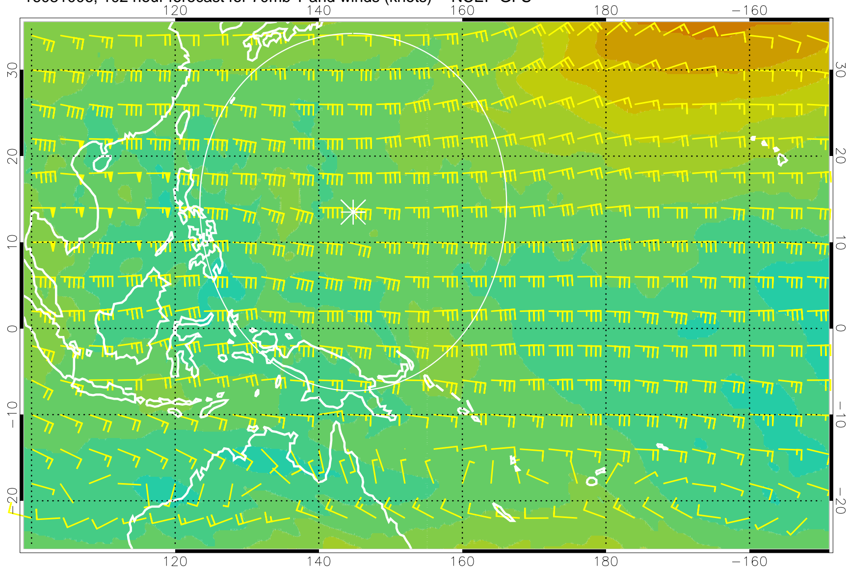
16081006, 102 hour forecast for 70mb T and winds (knots) -- NCEP GFS
