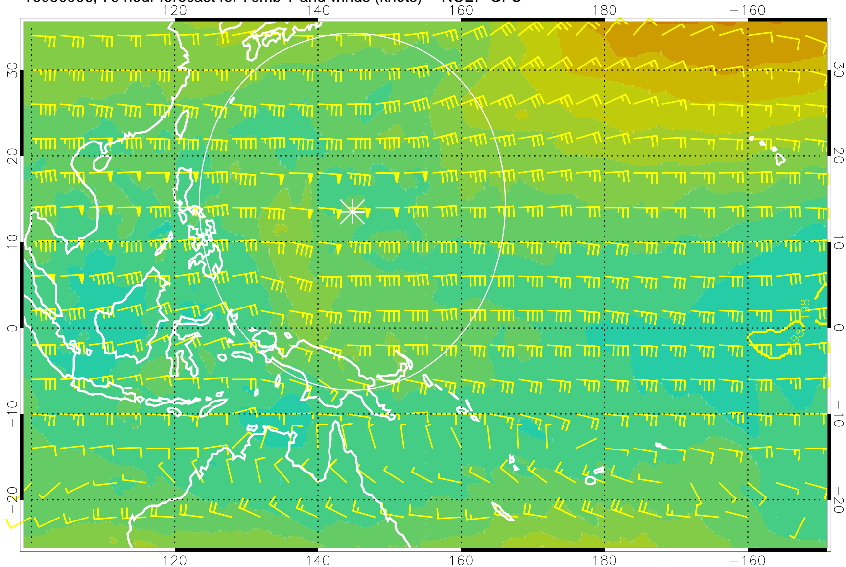
16080906, 78 hour forecast for 70mb T and winds (knots) -- NCEP GFS
