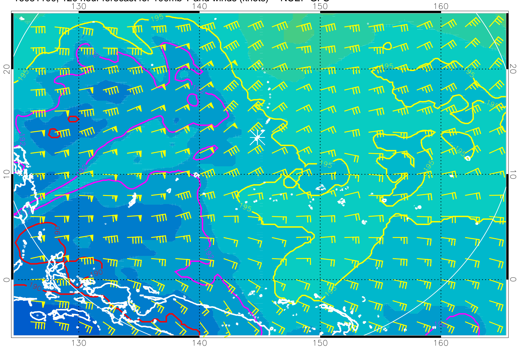
16081100, 120 hour forecast for 100mb T and winds (knots) -- NCEP GFS
