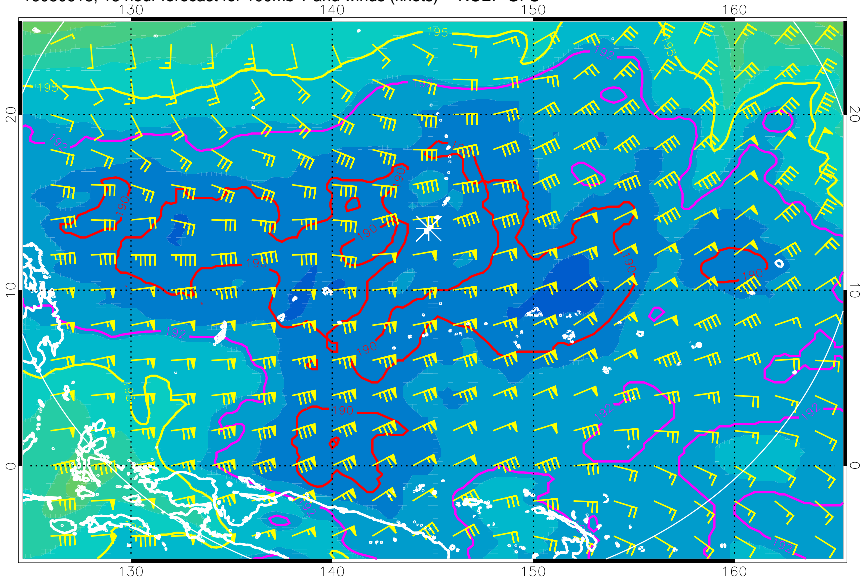
16080618, 18 hour forecast for 100mb T and winds (knots) -- NCEP GFS
