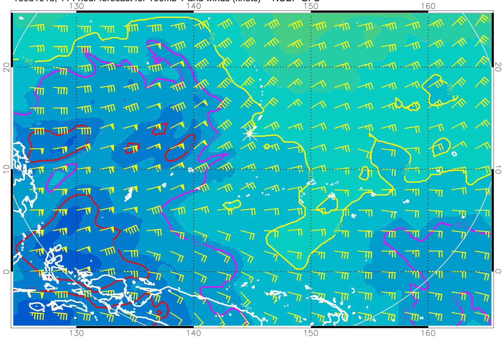
16081018, 114 hour forecast for 100mb T and winds (knots) -- NCEP GFS
