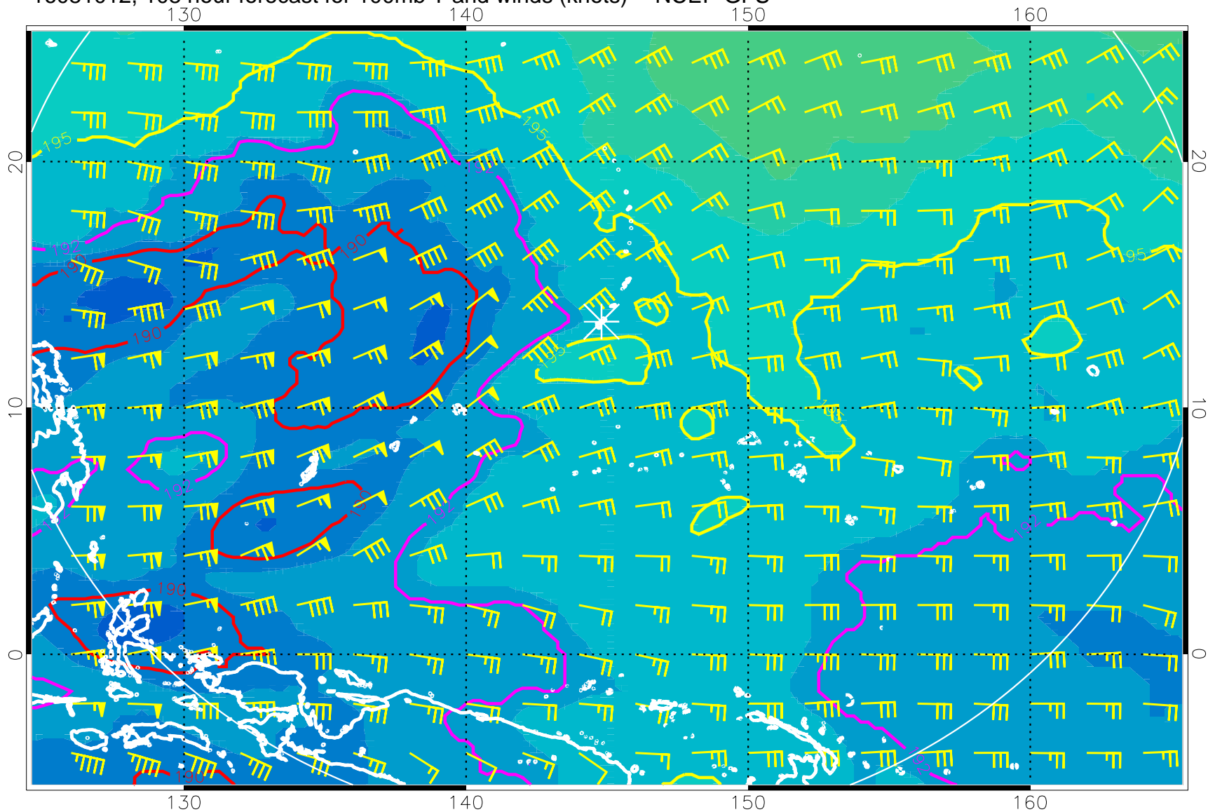
16081012, 108 hour forecast for 100mb T and winds (knots) -- NCEP GFS
