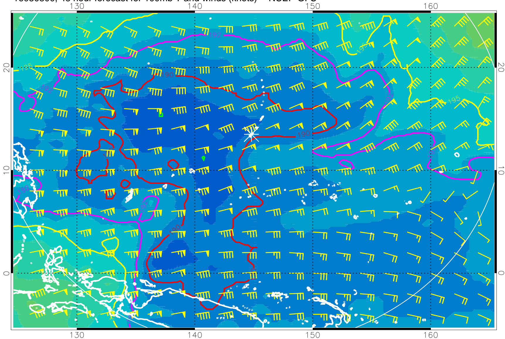
16080800, 48 hour forecast for 100mb T and winds (knots) -- NCEP GFS
