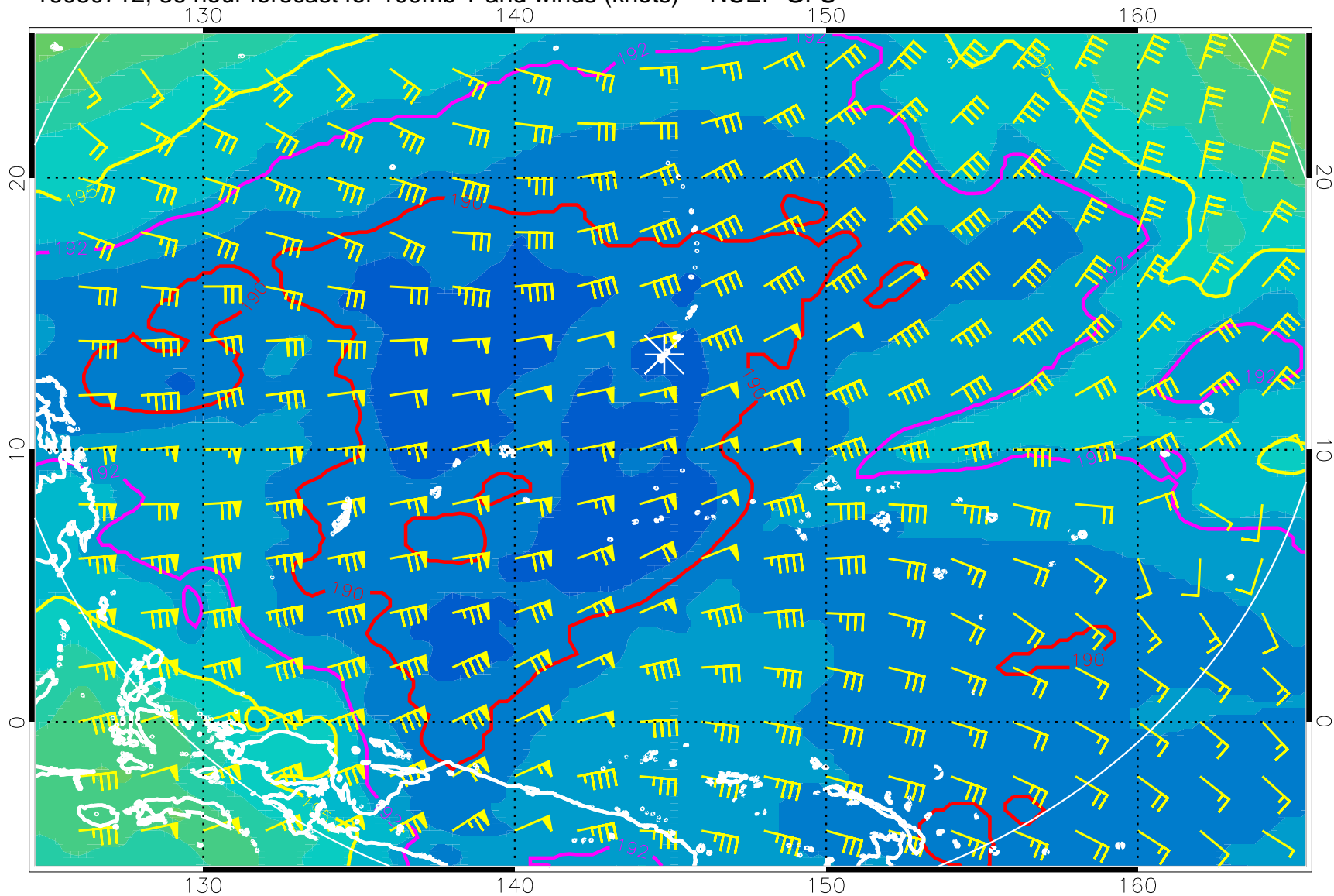
16080712, 36 hour forecast for 100mb T and winds (knots) -- NCEP GFS
