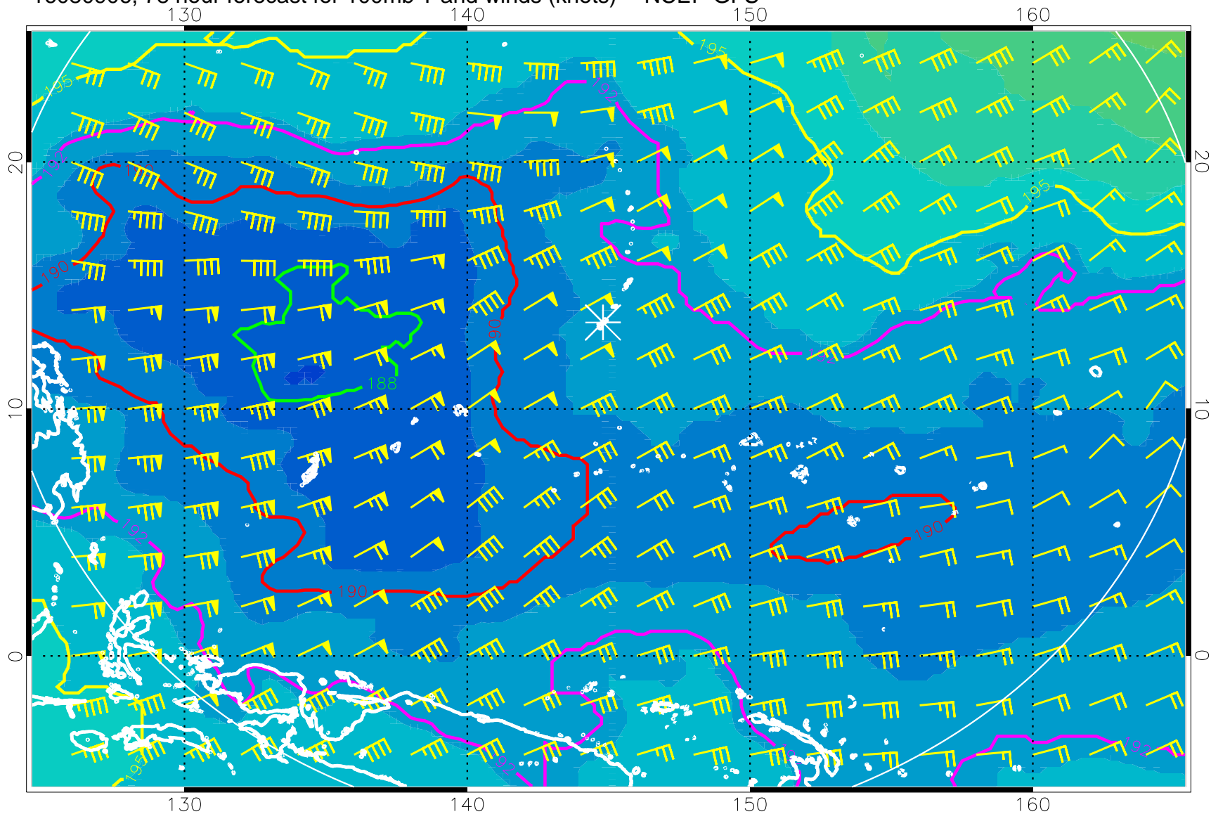
16080906, 78 hour forecast for 100mb T and winds (knots) -- NCEP GFS
