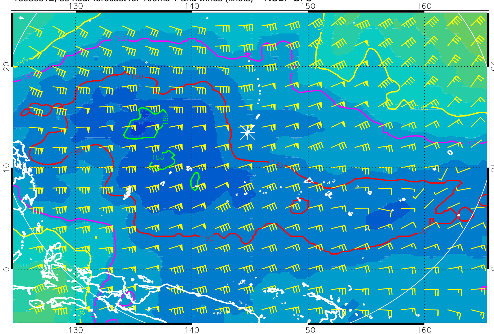
16080812, 60 hour forecast for 100mb T and winds (knots) -- NCEP GFS
