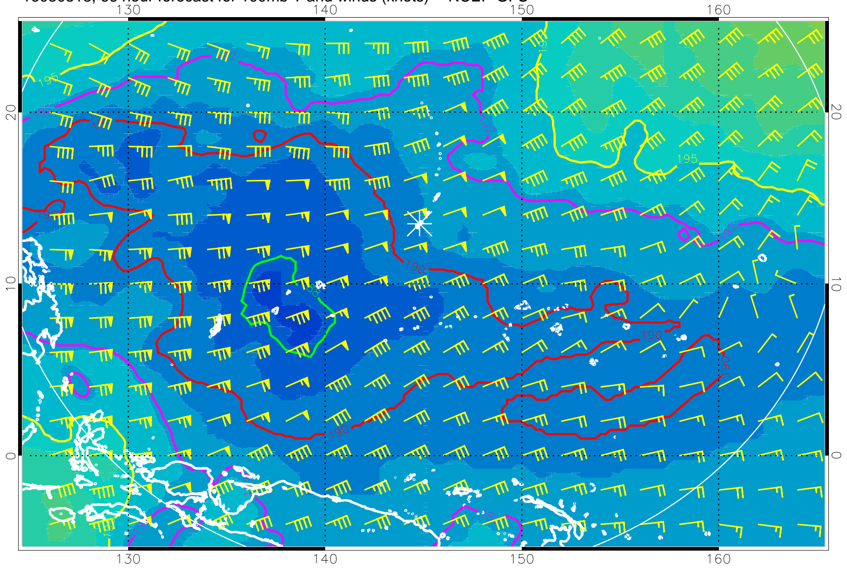
16080818, 66 hour forecast for 100mb T and winds (knots) -- NCEP GFS
