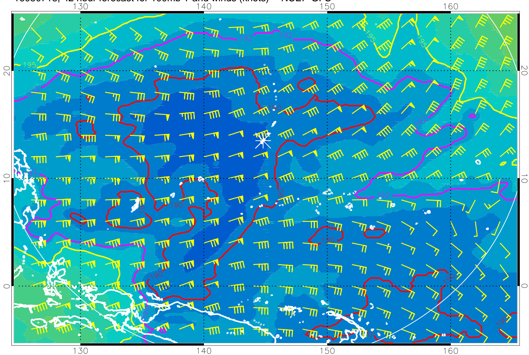
16080718, 42 hour forecast for 100mb T and winds (knots) -- NCEP GFS
