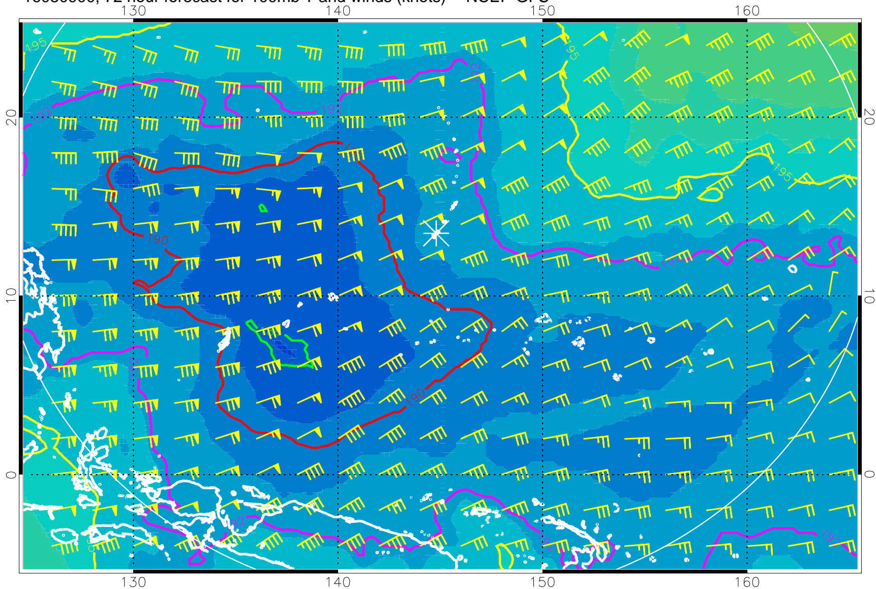
16080900, 72 hour forecast for 100mb T and winds (knots) -- NCEP GFS
