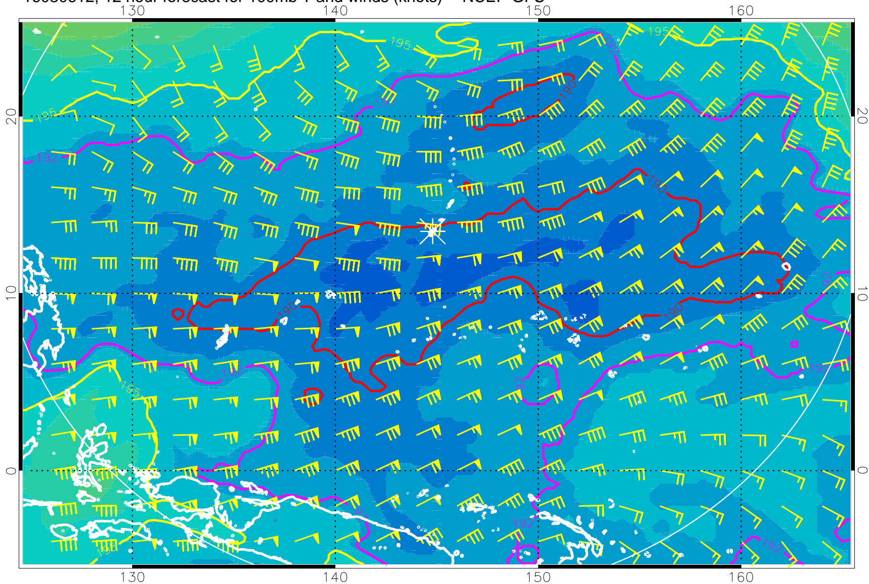
16080612, 12 hour forecast for 100mb T and winds (knots) -- NCEP GFS
