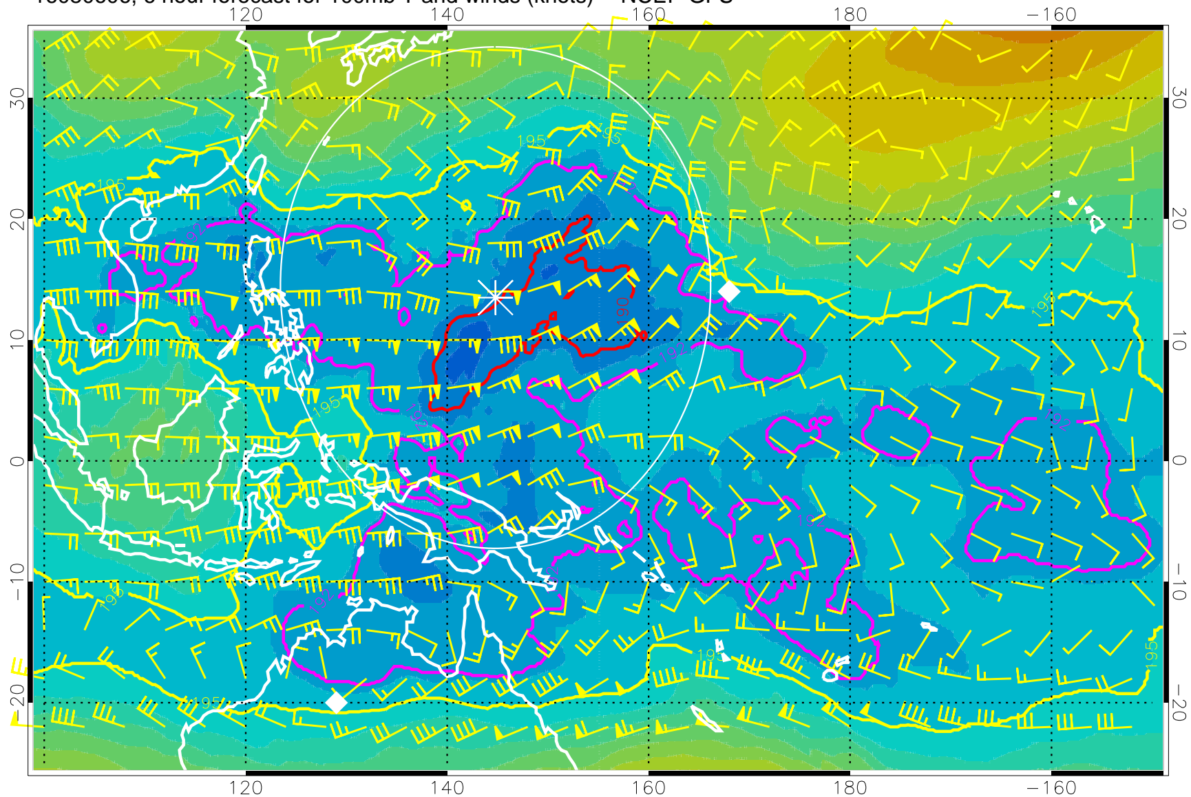
16080606, 6 hour forecast for 100mb T and winds (knots) -- NCEP GFS
