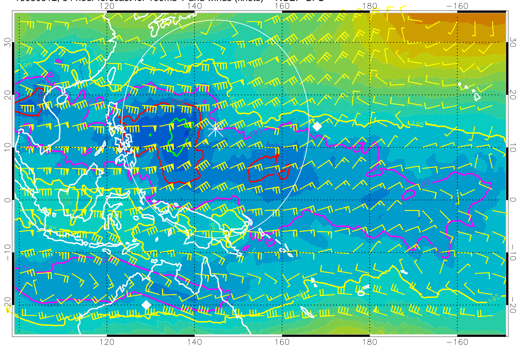
16080912, 84 hour forecast for 100mb T and winds (knots) -- NCEP GFS
