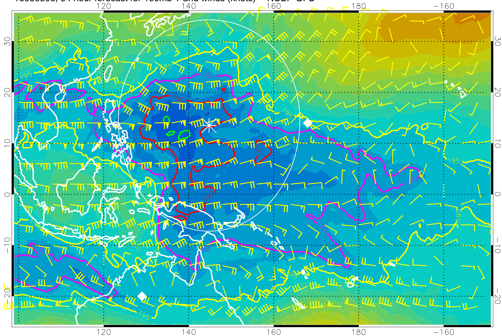
16080806, 54 hour forecast for 100mb T and winds (knots) -- NCEP GFS
