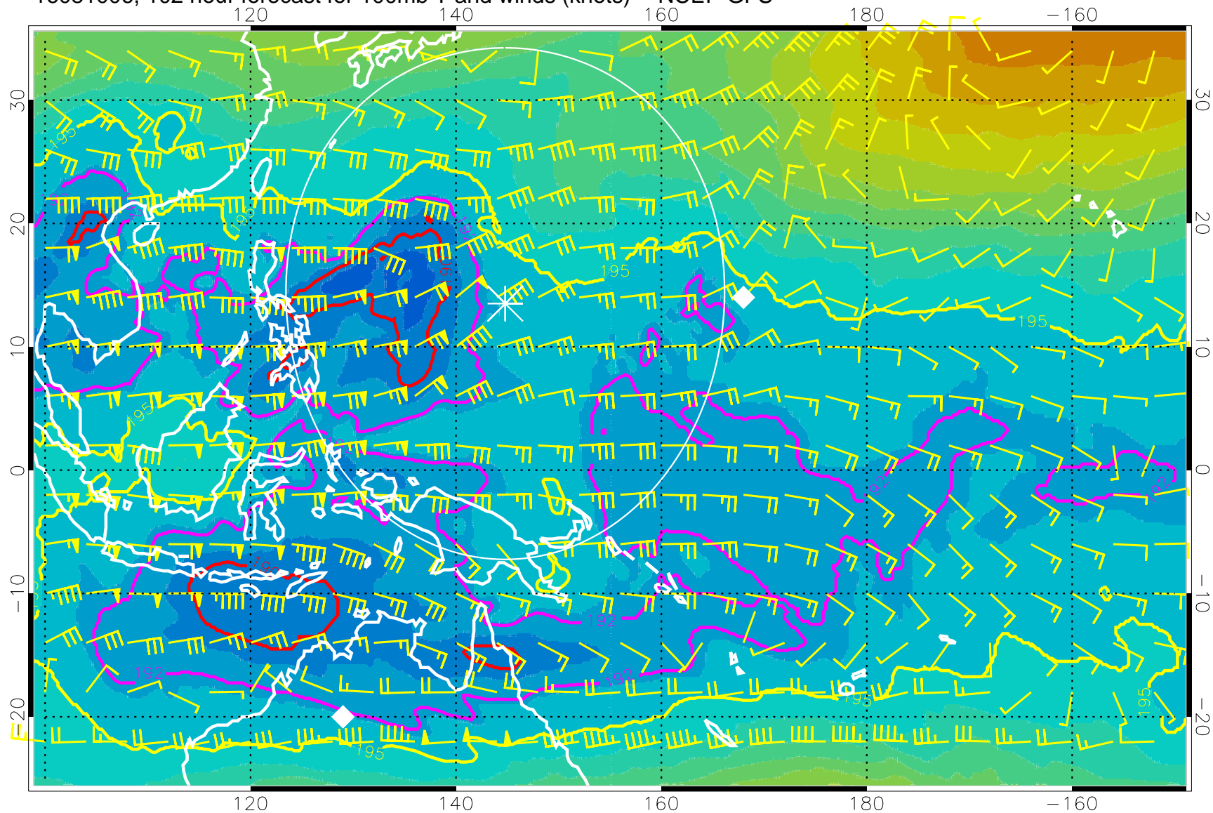
16081006, 102 hour forecast for 100mb T and winds (knots) -- NCEP GFS
