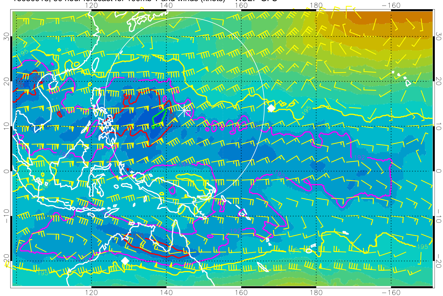
16080918, 90 hour forecast for 100mb T and winds (knots) -- NCEP GFS
