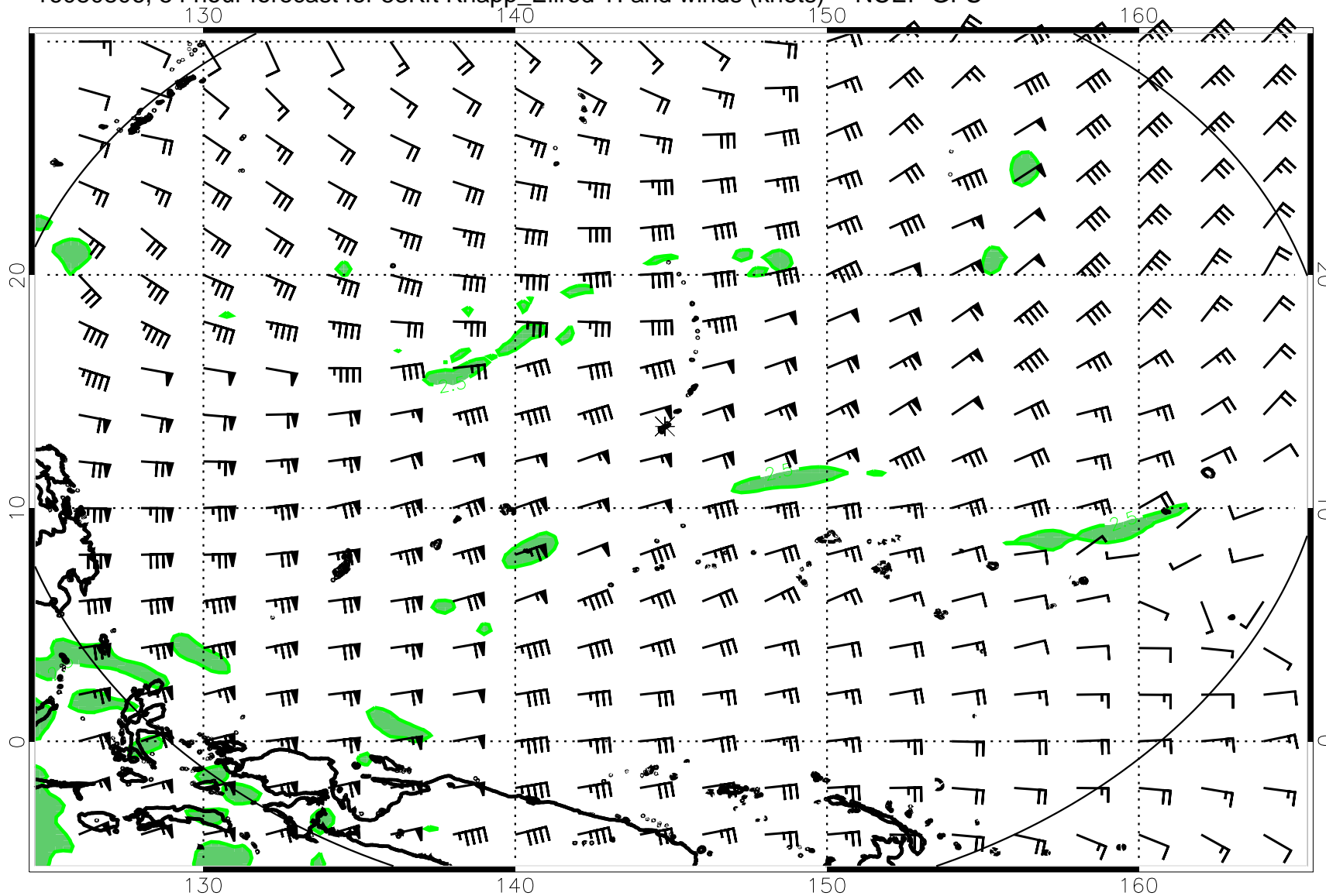
16080806, 54 hour forecast for 53Kft Knapp_Ellrod TI and winds (knots) -- NCEP GFS
