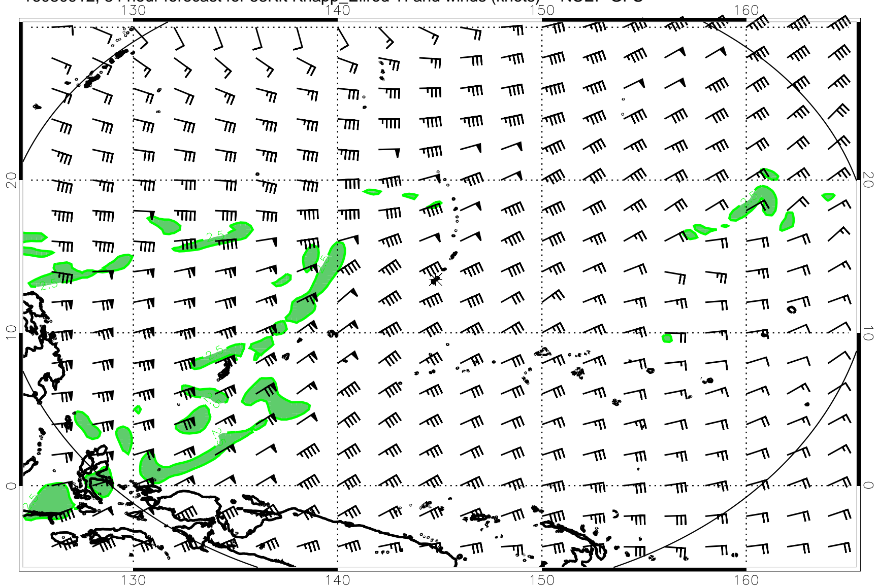
16080912, 84 hour forecast for 53Kft Knapp_Ellrod TI and winds (knots) -- NCEP GFS
