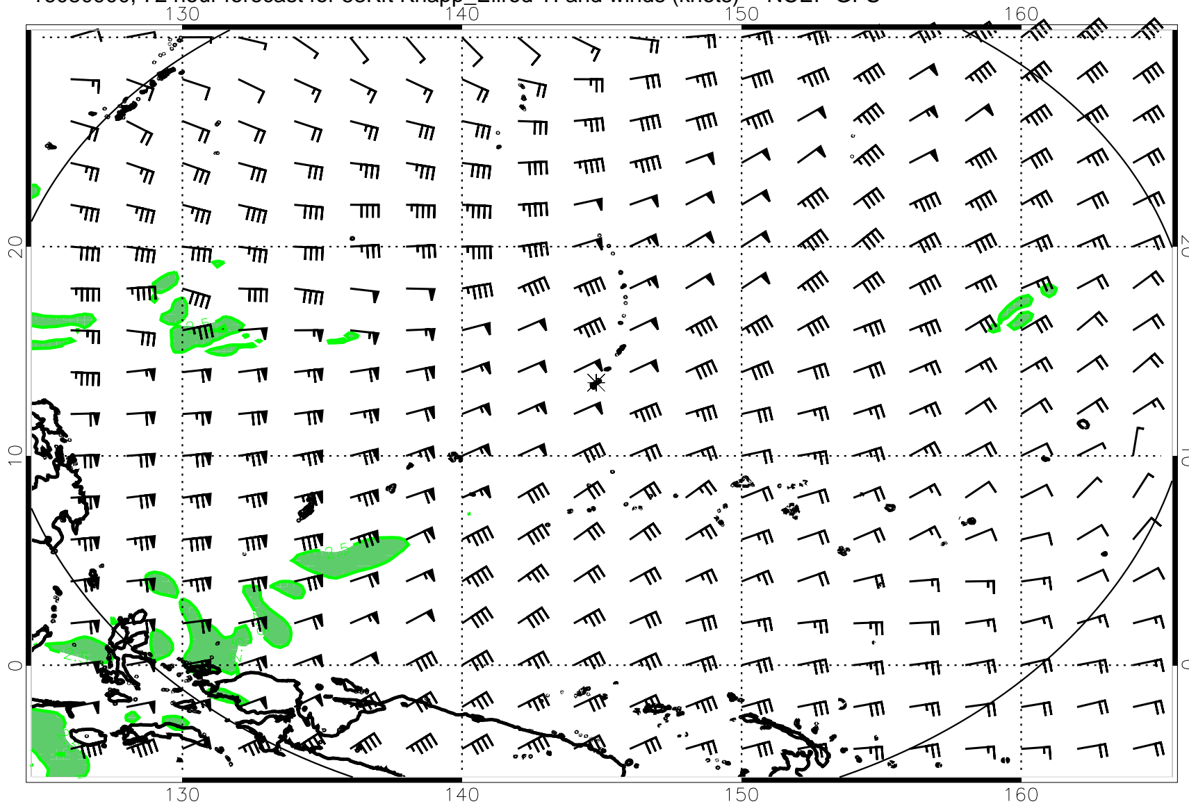
16080900, 72 hour forecast for 53Kft Knapp_Ellrod TI and winds (knots) -- NCEP GFS
