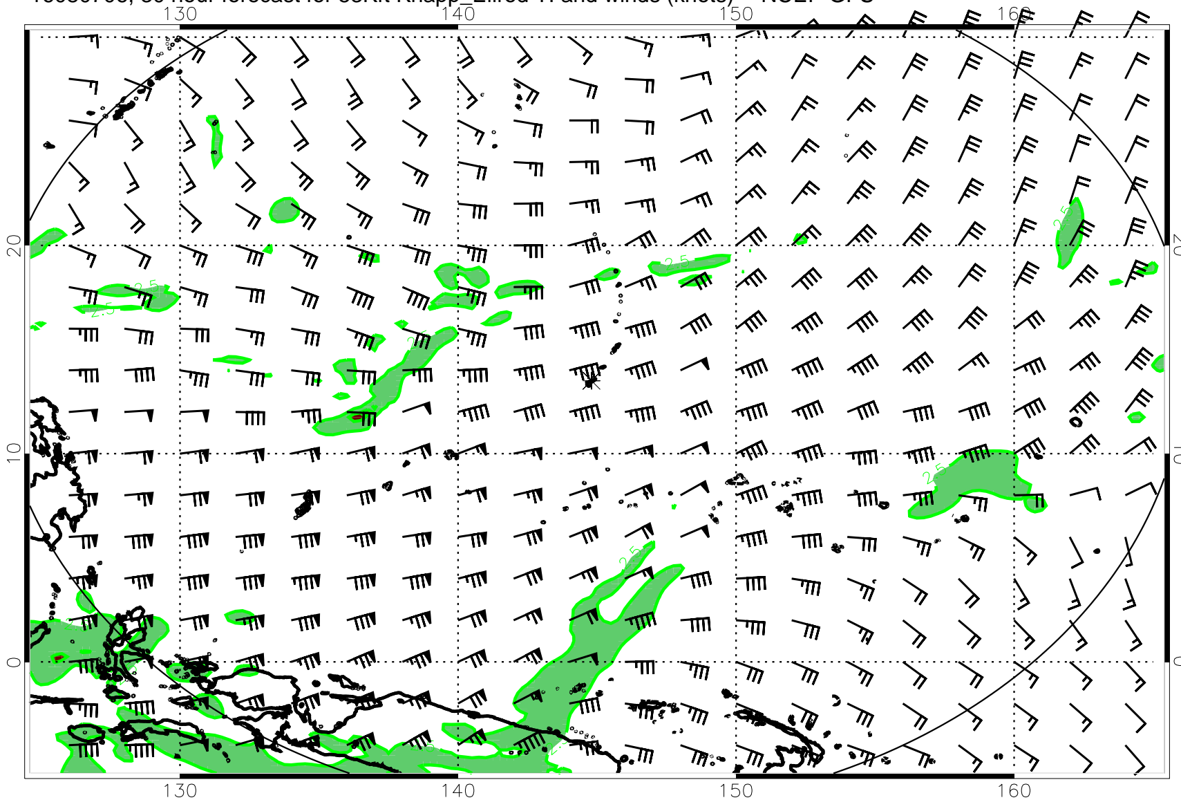
16080706, 30 hour forecast for 53Kft Knapp_Ellrod TI and winds (knots) -- NCEP GFS
