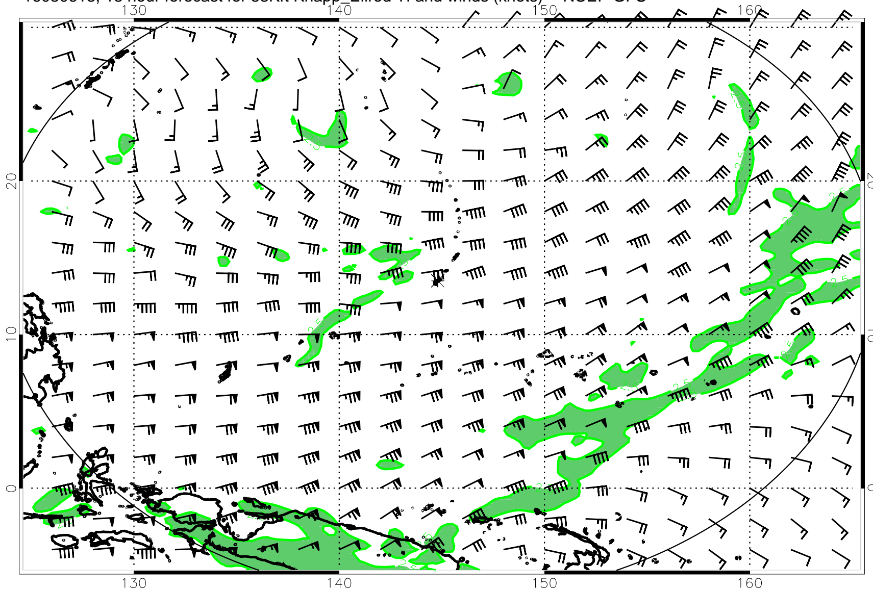
16080618, 18 hour forecast for 53Kft Knapp_Ellrod TI and winds (knots) -- NCEP GFS
