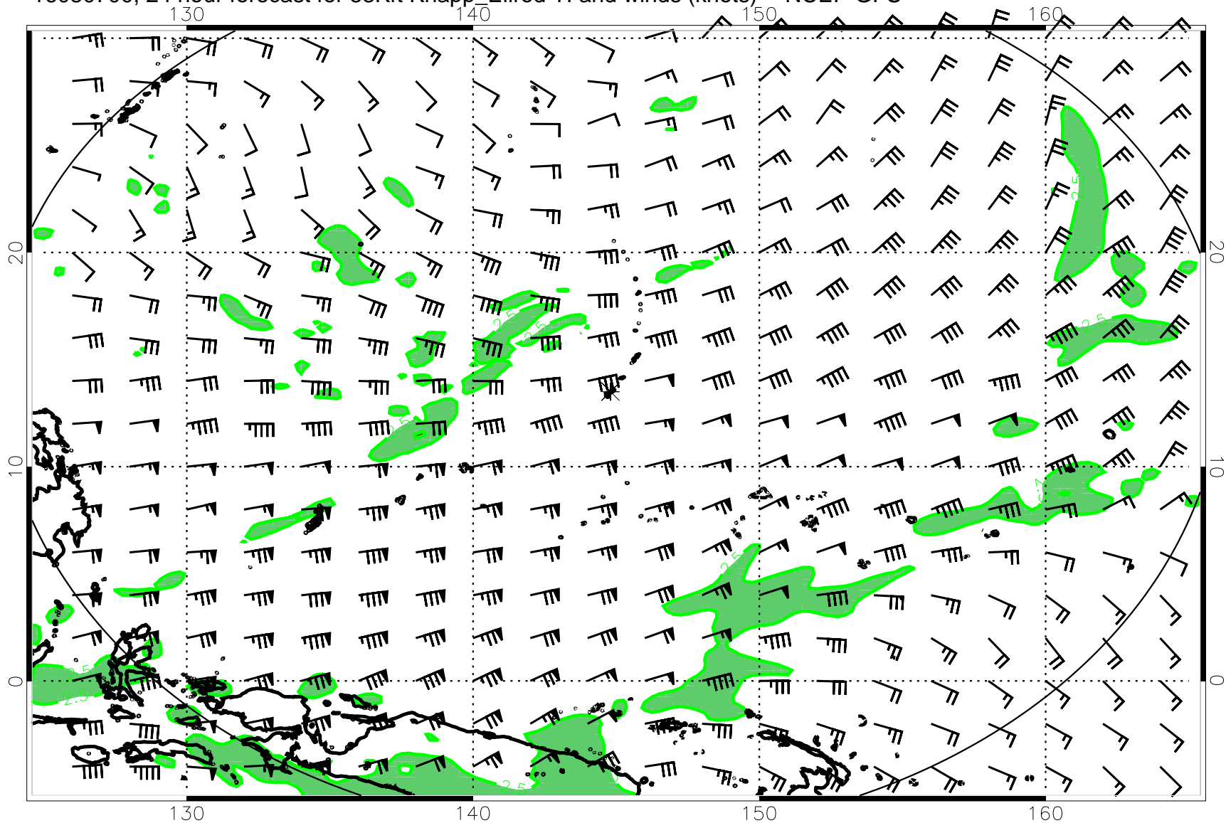
16080700, 24 hour forecast for 53Kft Knapp_Ellrod TI and winds (knots) -- NCEP GFS
