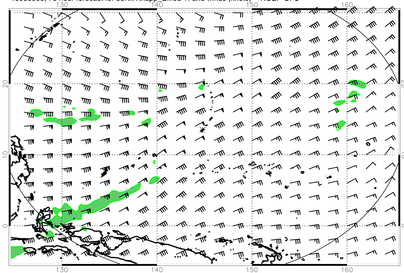
16080906, 78 hour forecast for 53Kft Knapp_Ellrod TI and winds (knots) -- NCEP GFS
