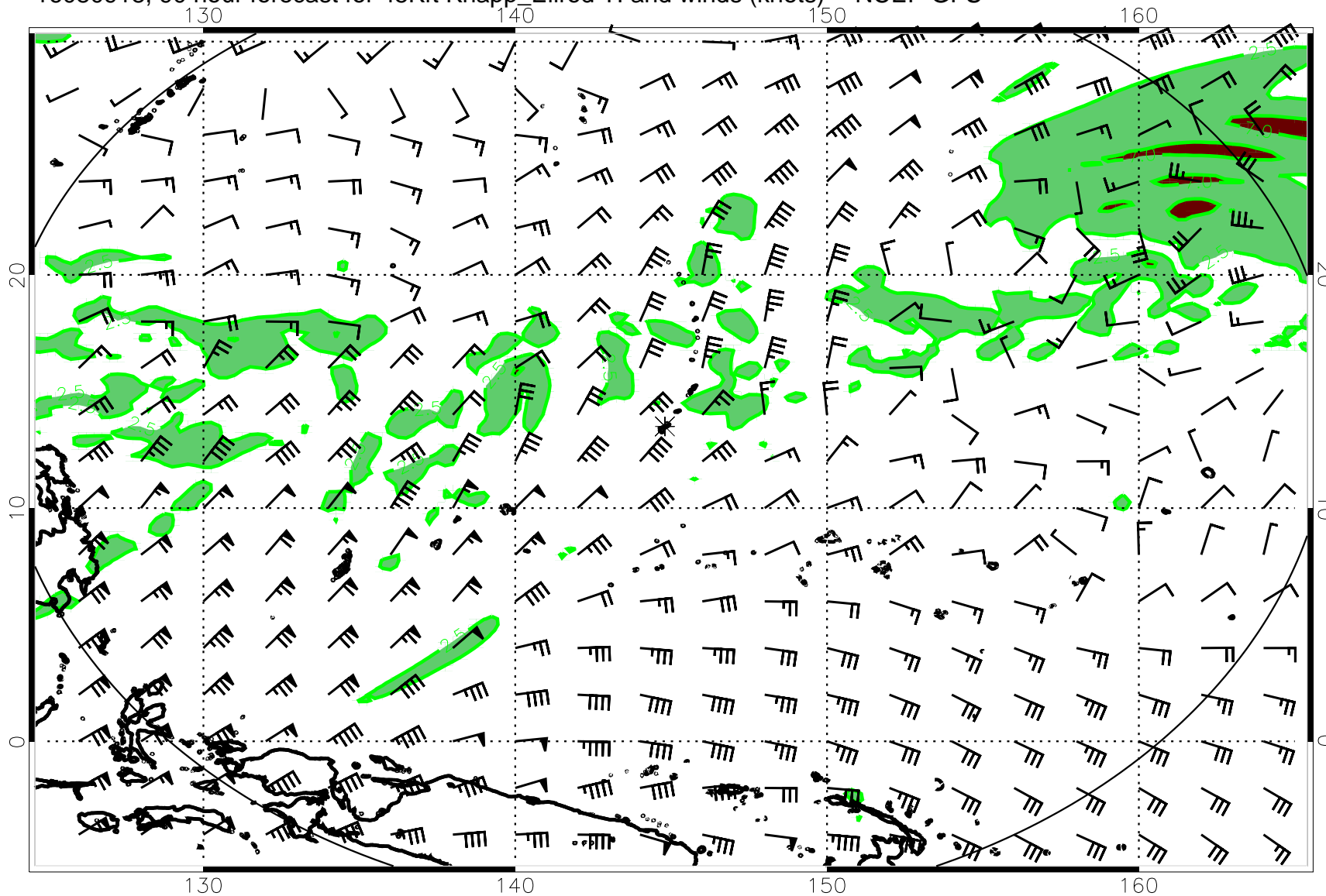
16080918, 90 hour forecast for 45Kft Knapp_Ellrod TI and winds (knots) -- NCEP GFS
