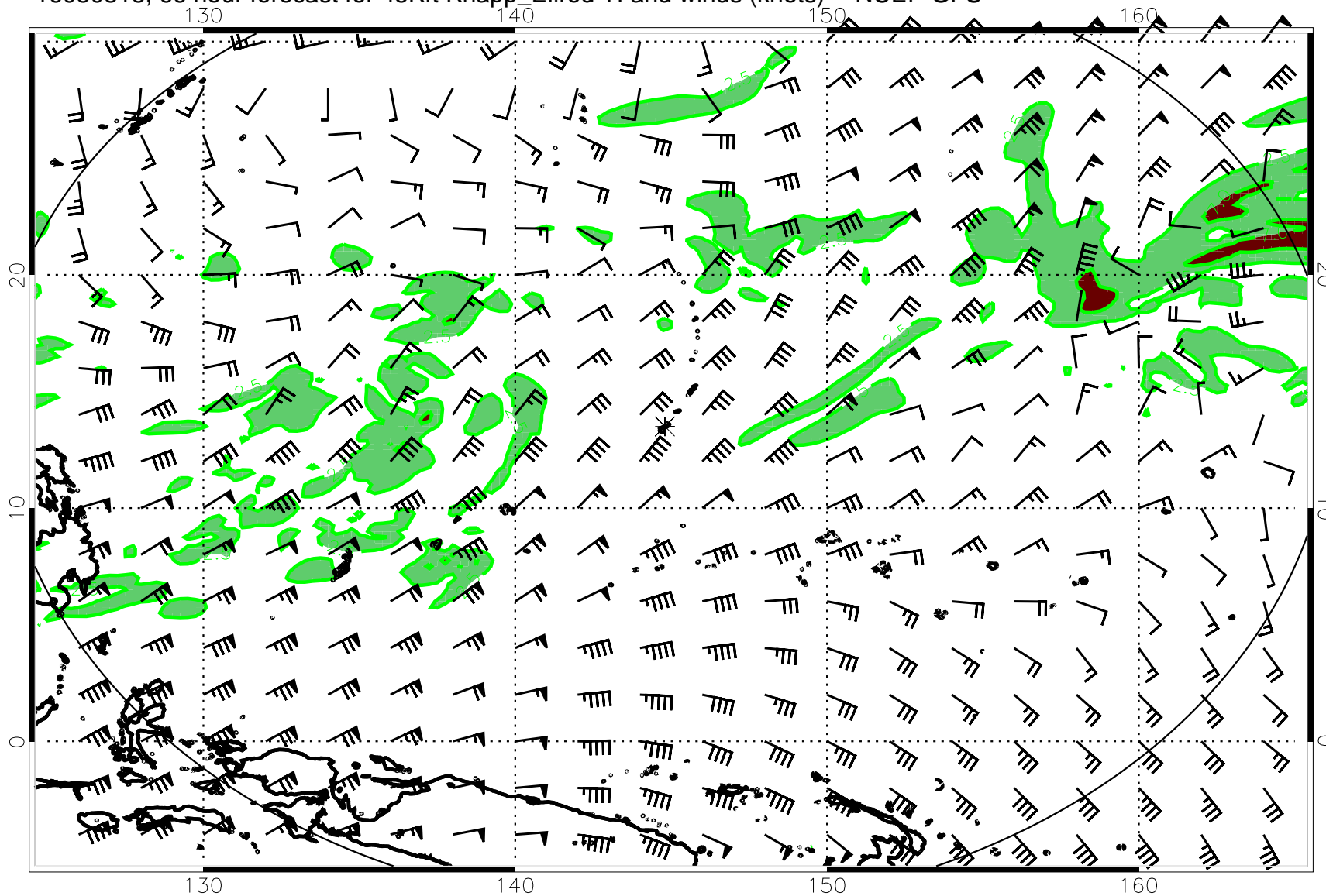
16080818, 66 hour forecast for 45Kft Knapp_Ellrod TI and winds (knots) -- NCEP GFS
