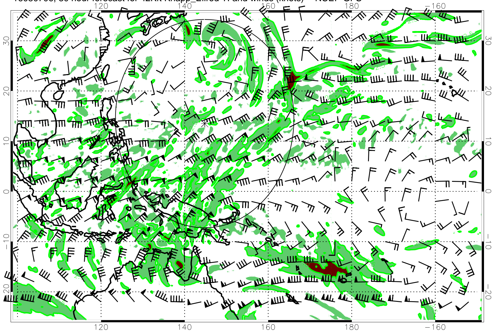
16080706, 30 hour forecast for 42Kft Knapp_Ellrod TI and winds (knots) -- NCEP GFS
