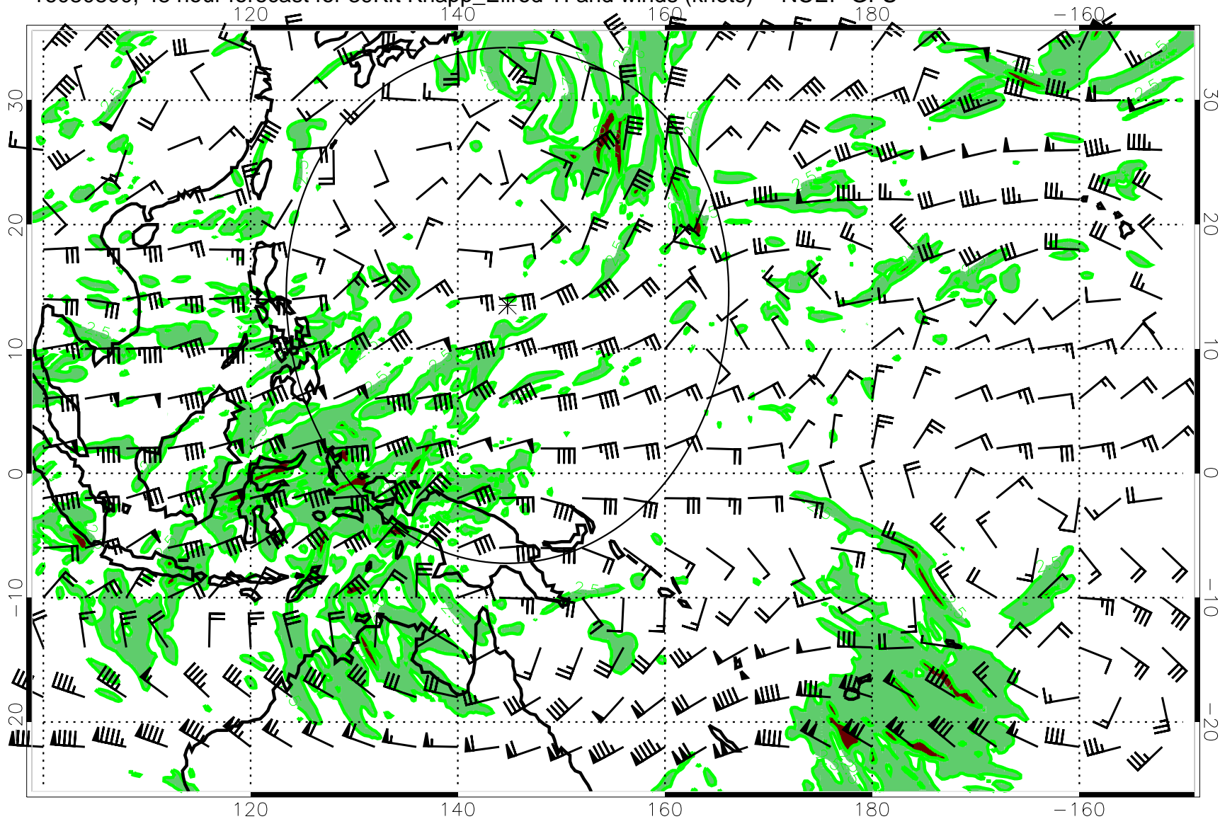
16080800, 48 hour forecast for 39Kft Knapp_Ellrod TI and winds (knots) -- NCEP GFS
