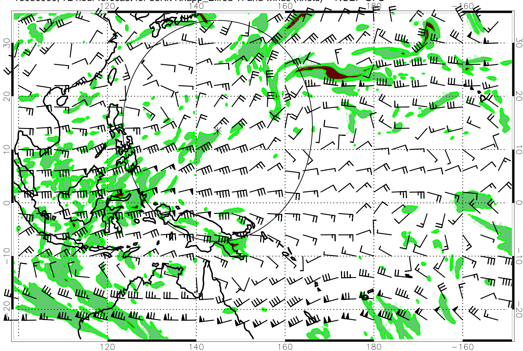
16080900, 72 hour forecast for 36Kft Knapp_Ellrod TI and winds (knots) -- NCEP GFS
