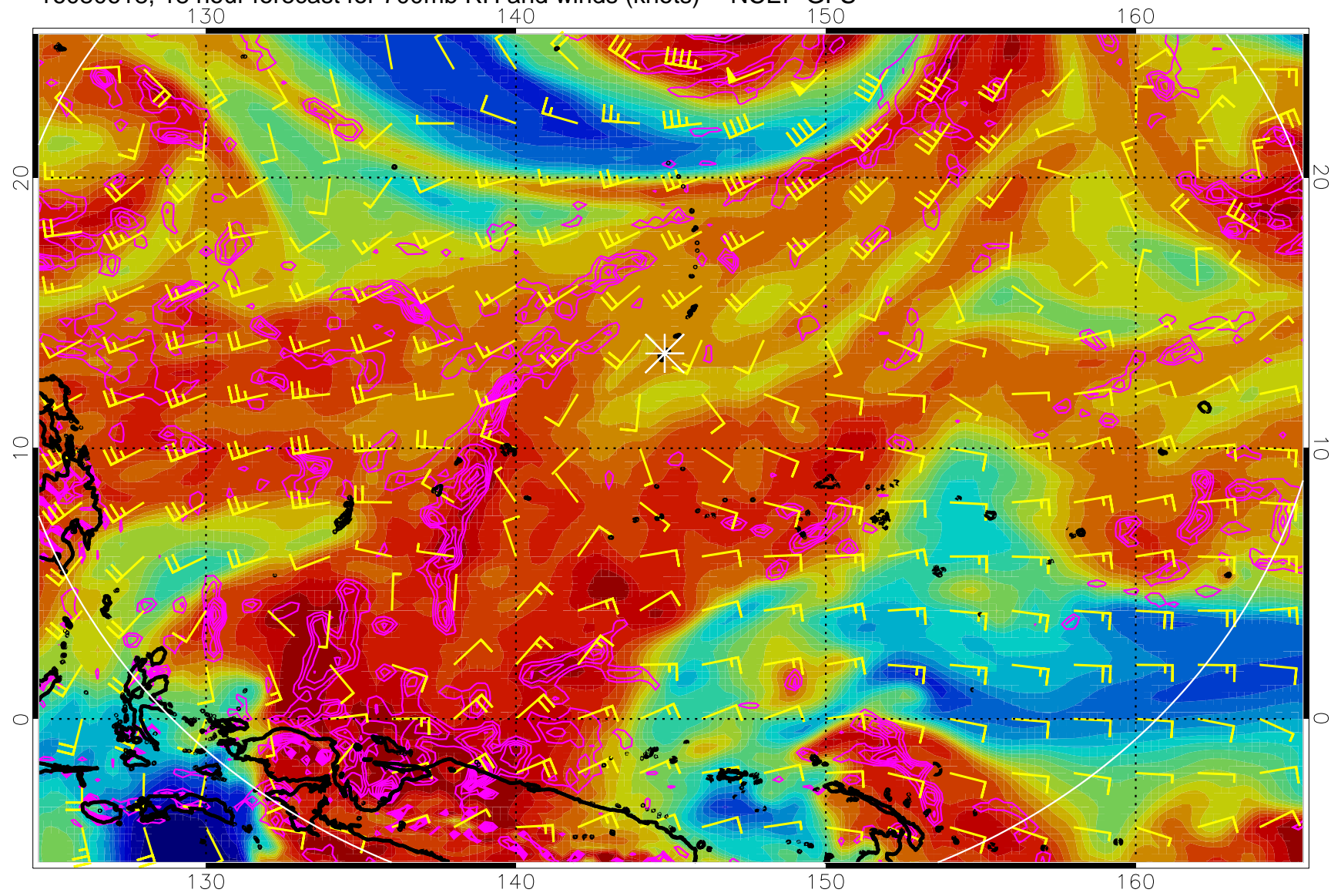
16080618, 18 hour forecast for 700mb RH and winds (knots) -- NCEP GFS
