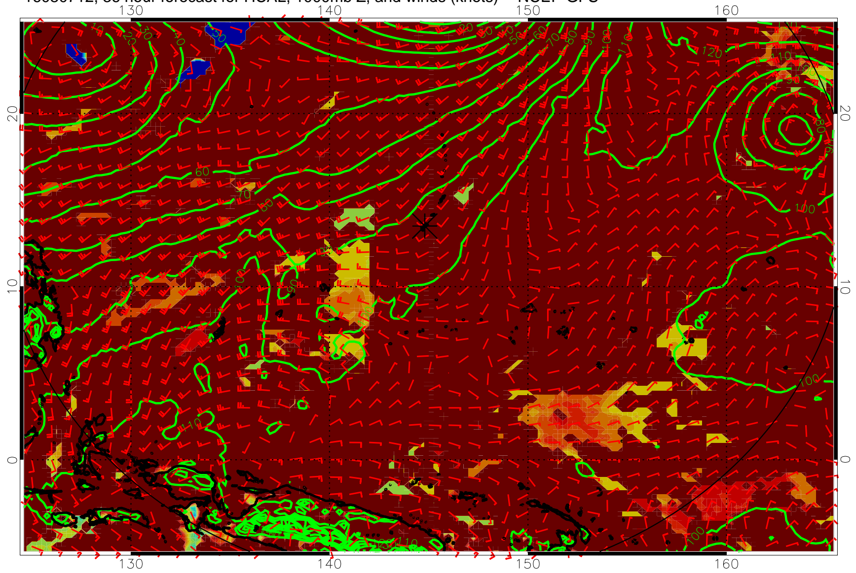
16080712, 36 hour forecast for HCAL, 1000mb Z, and winds (knots) -- NCEP GFS
