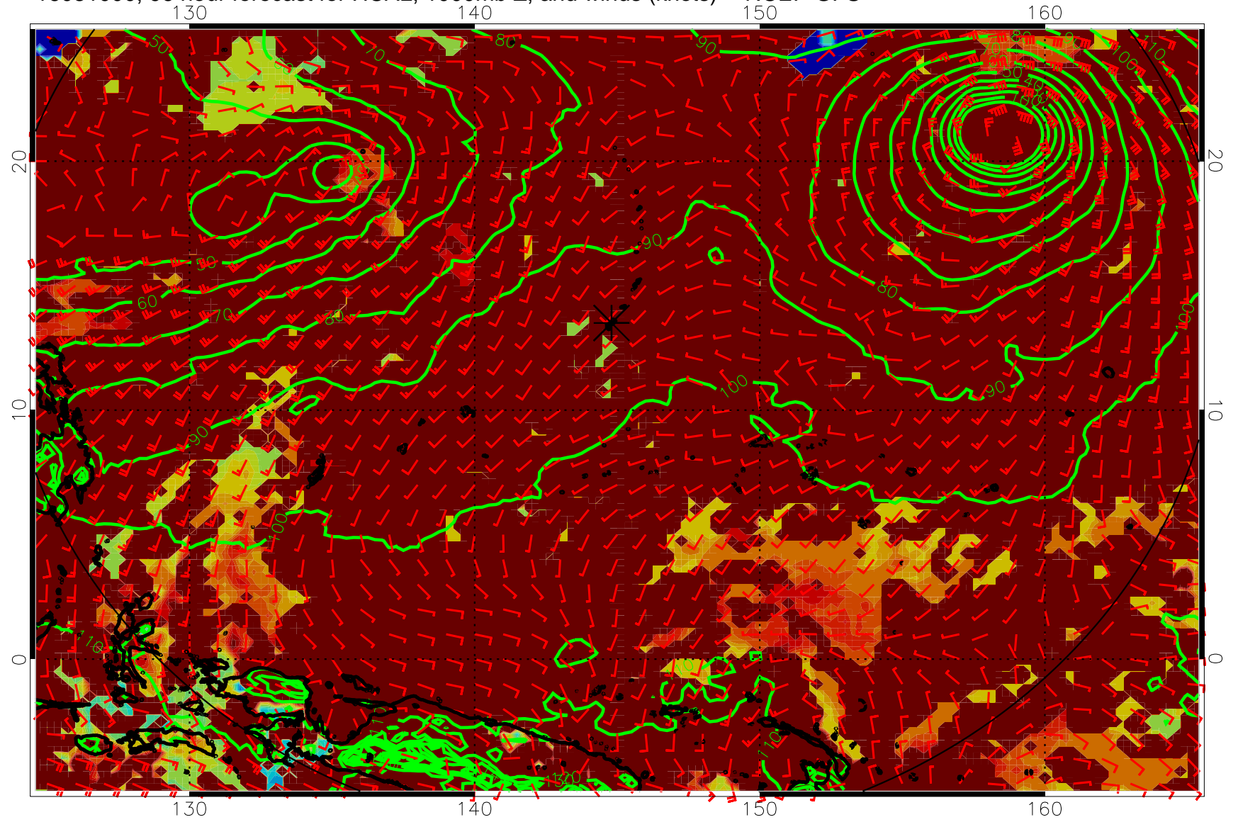
16081000, 96 hour forecast for HCAL, 1000mb Z, and winds (knots) -- NCEP GFS
