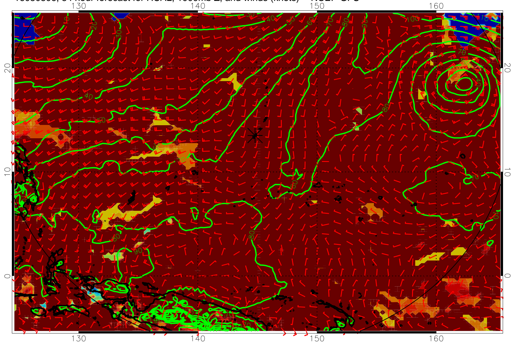
16080806, 54 hour forecast for HCAL, 1000mb Z, and winds (knots) -- NCEP GFS
