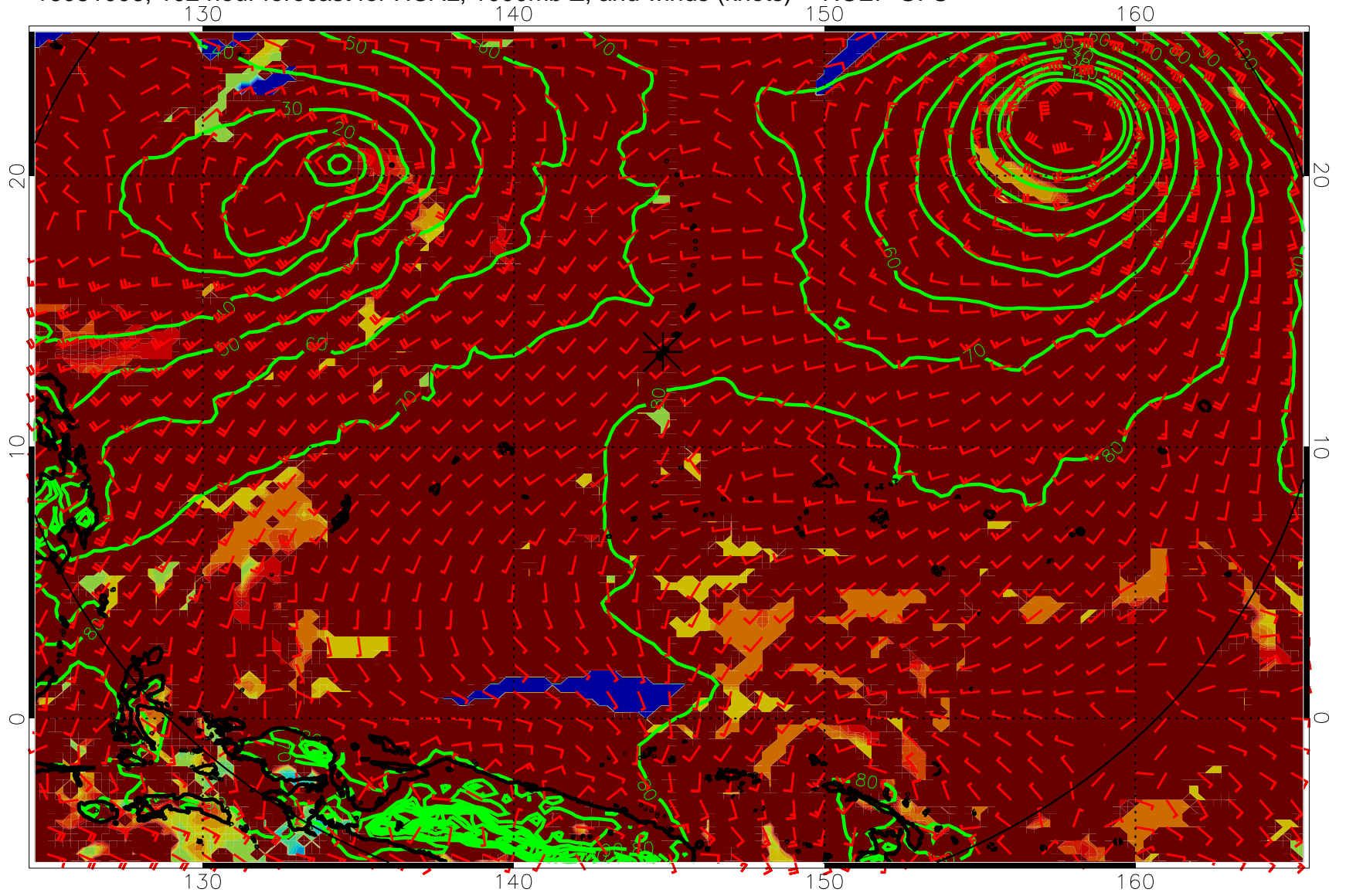
16081006, 102 hour forecast for HCAL, 1000mb Z, and winds (knots) -- NCEP GFS
