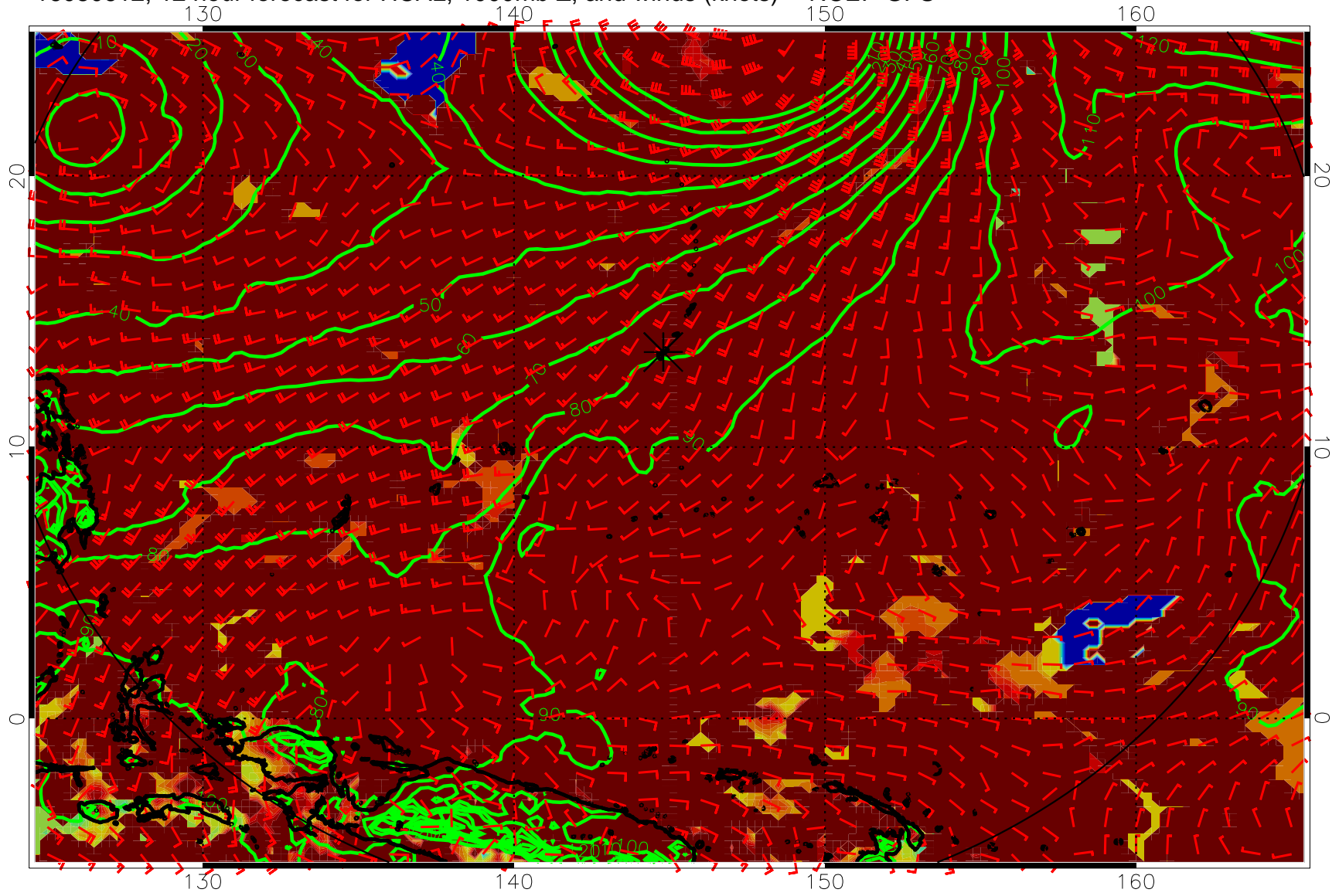
16080612, 12 hour forecast for HCAL, 1000mb Z, and winds (knots) -- NCEP GFS
