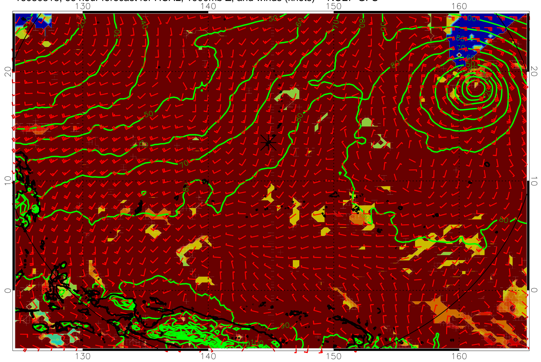
16080818, 66 hour forecast for HCAL, 1000mb Z, and winds (knots) -- NCEP GFS
