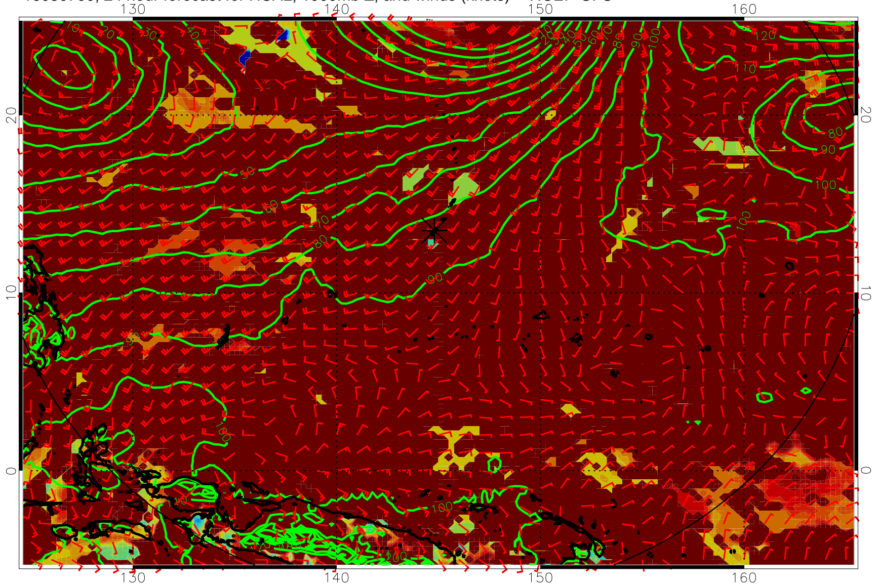
16080700, 24 hour forecast for HCAL, 1000mb Z, and winds (knots) -- NCEP GFS
