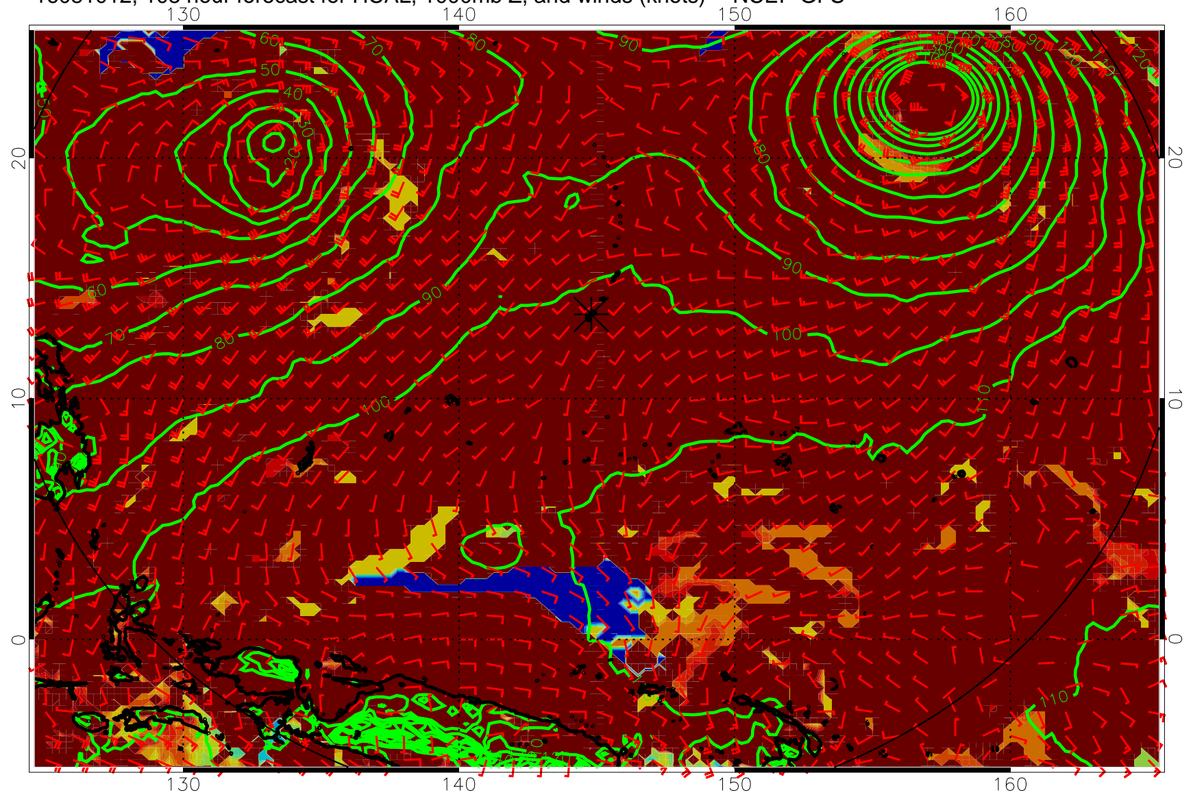
16081012, 108 hour forecast for HCAL, 1000mb Z, and winds (knots) -- NCEP GFS
