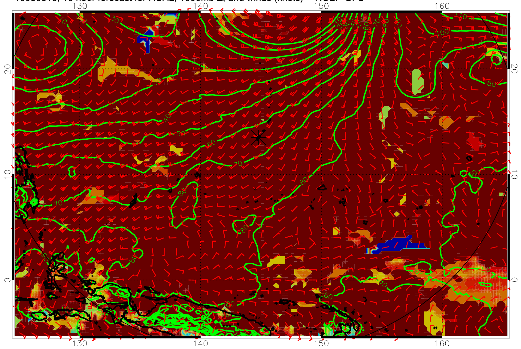
16080618, 18 hour forecast for HCAL, 1000mb Z, and winds (knots) -- NCEP GFS
