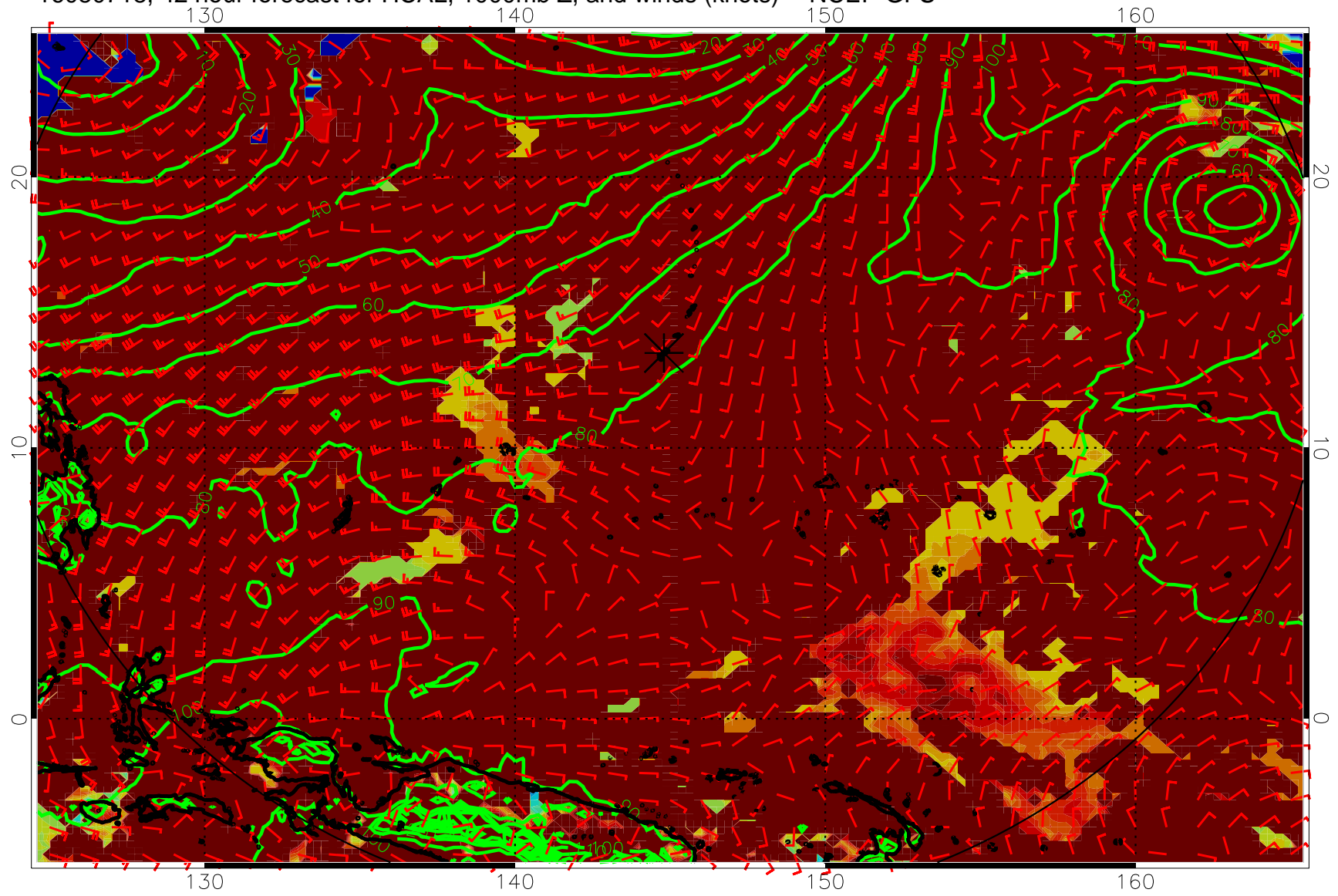
16080718, 42 hour forecast for HCAL, 1000mb Z, and winds (knots) -- NCEP GFS
