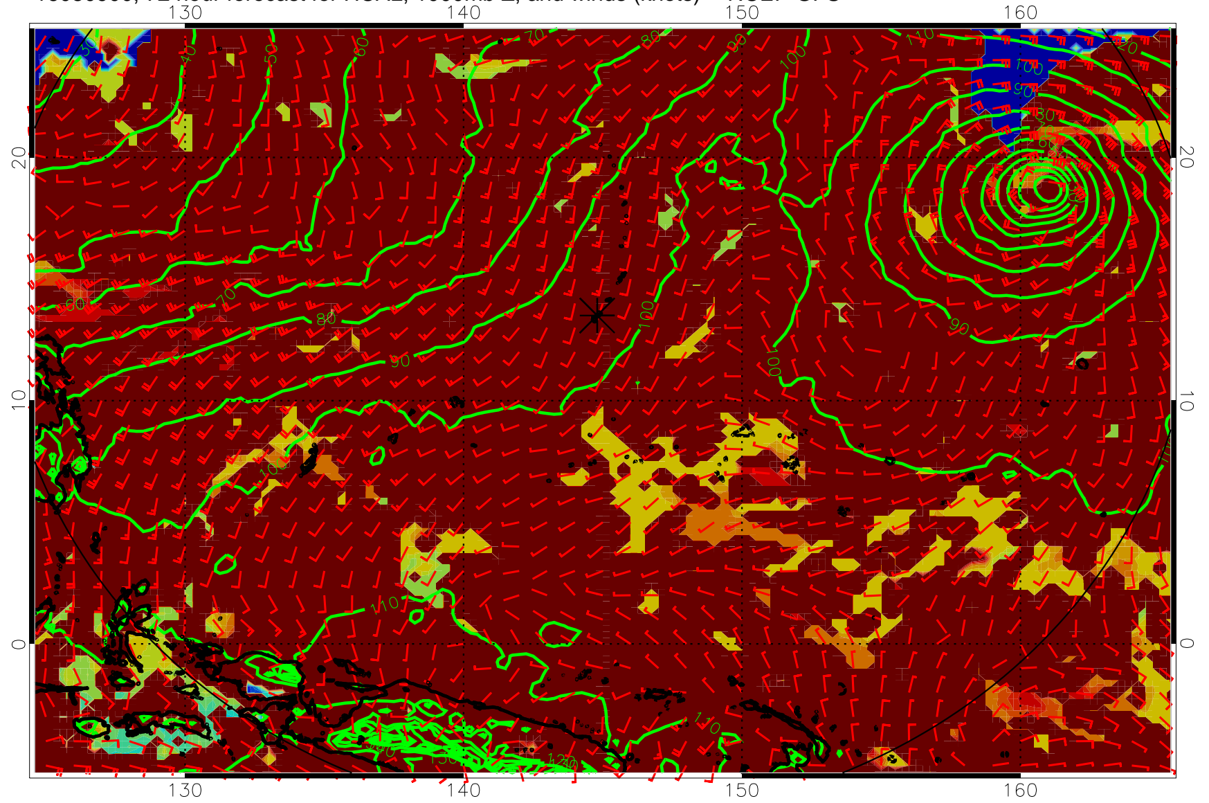
16080900, 72 hour forecast for HCAL, 1000mb Z, and winds (knots) -- NCEP GFS
