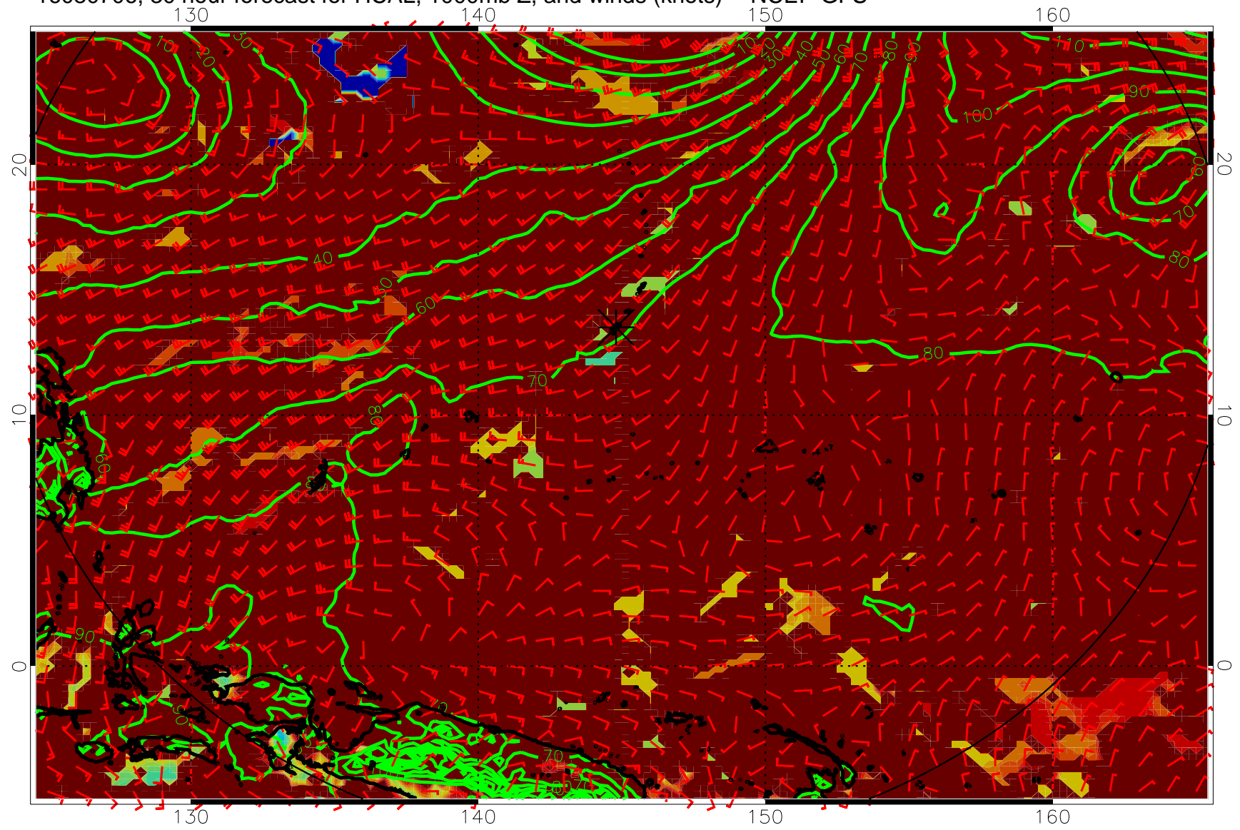
16080706, 30 hour forecast for HCAL, 1000mb Z, and winds (knots) -- NCEP GFS
