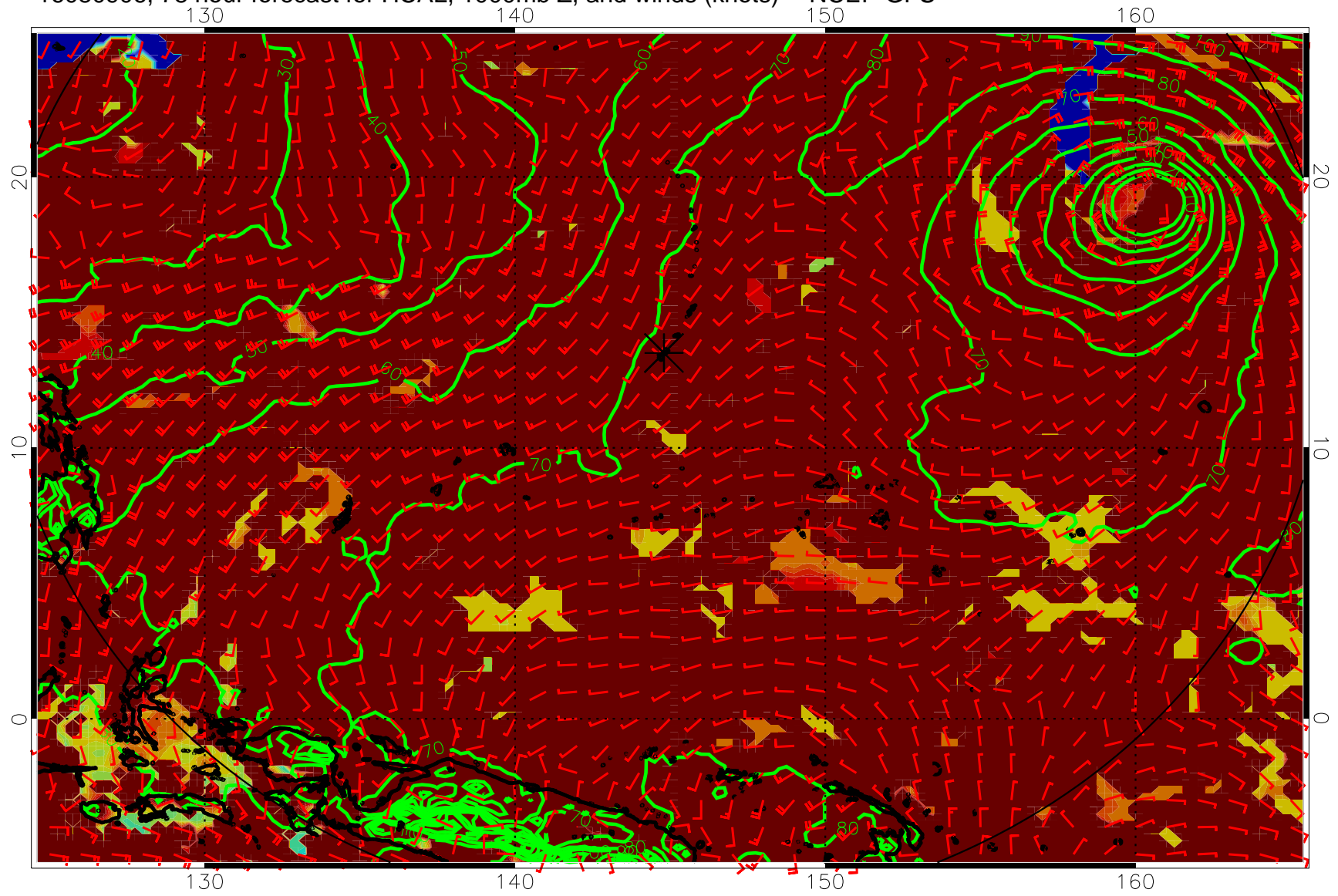
16080906, 78 hour forecast for HCAL, 1000mb Z, and winds (knots) -- NCEP GFS
