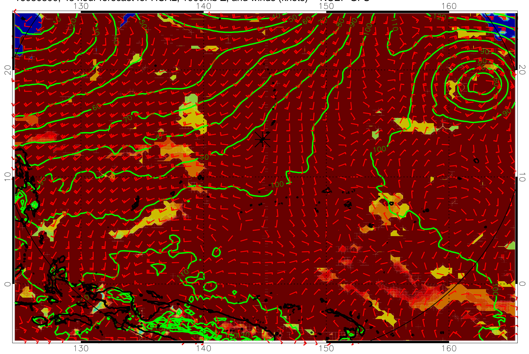
16080800, 48 hour forecast for HCAL, 1000mb Z, and winds (knots) -- NCEP GFS
