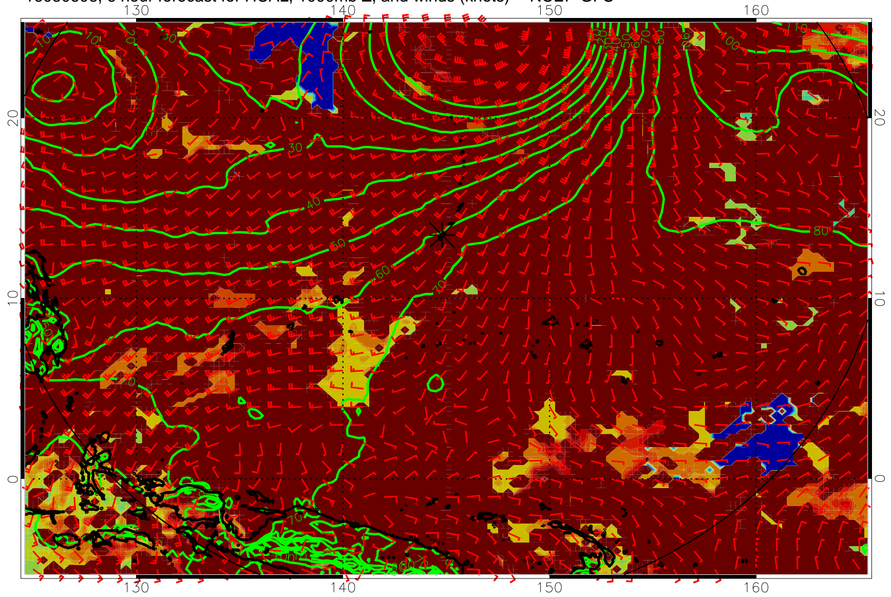
16080606, 6 hour forecast for HCAL, 1000mb Z, and winds (knots) -- NCEP GFS
