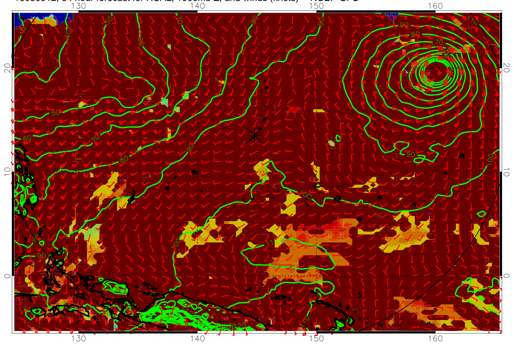
16080912, 84 hour forecast for HCAL, 1000mb Z, and winds (knots) -- NCEP GFS
