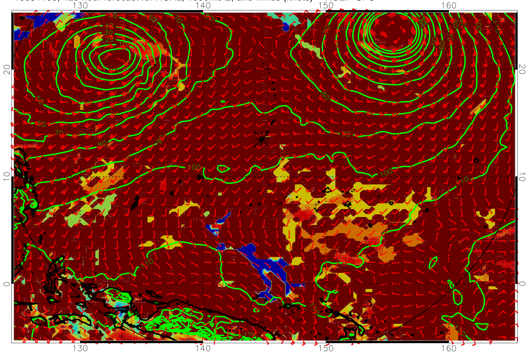
16081100, 120 hour forecast for HCAL, 1000mb Z, and winds (knots) -- NCEP GFS
