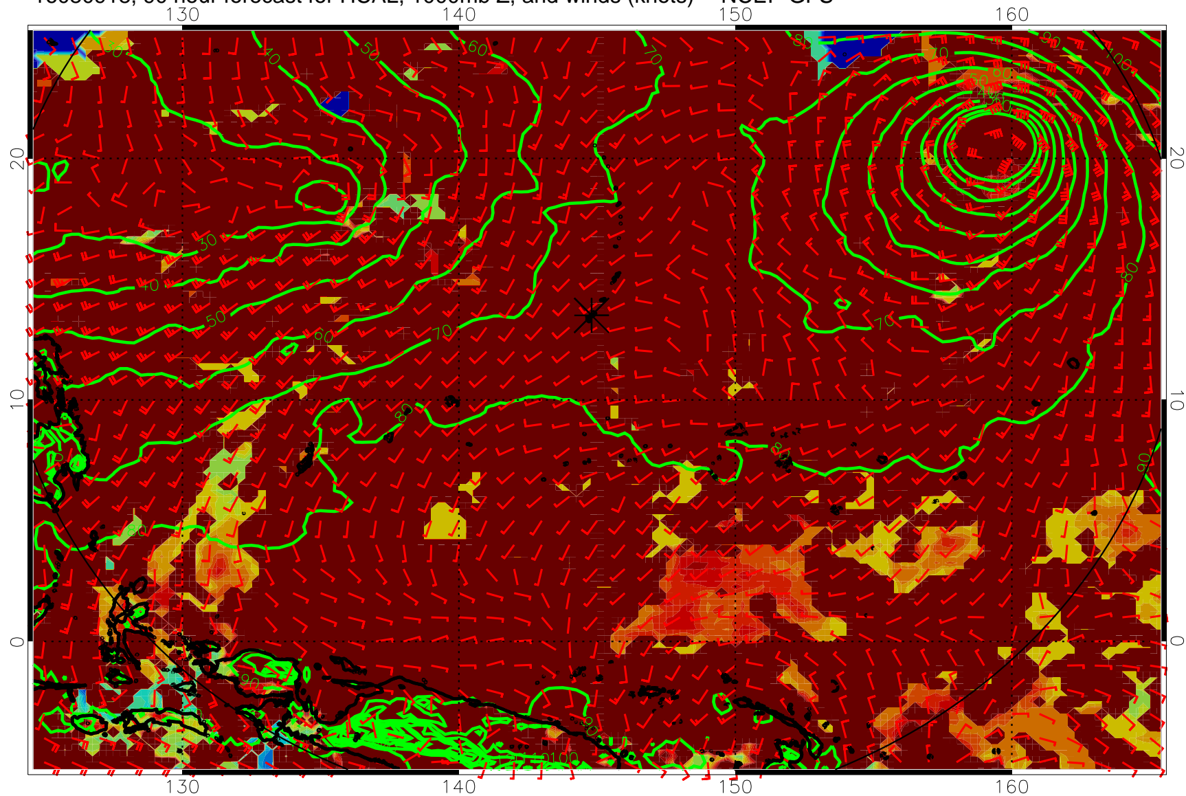
16080918, 90 hour forecast for HCAL, 1000mb Z, and winds (knots) -- NCEP GFS
