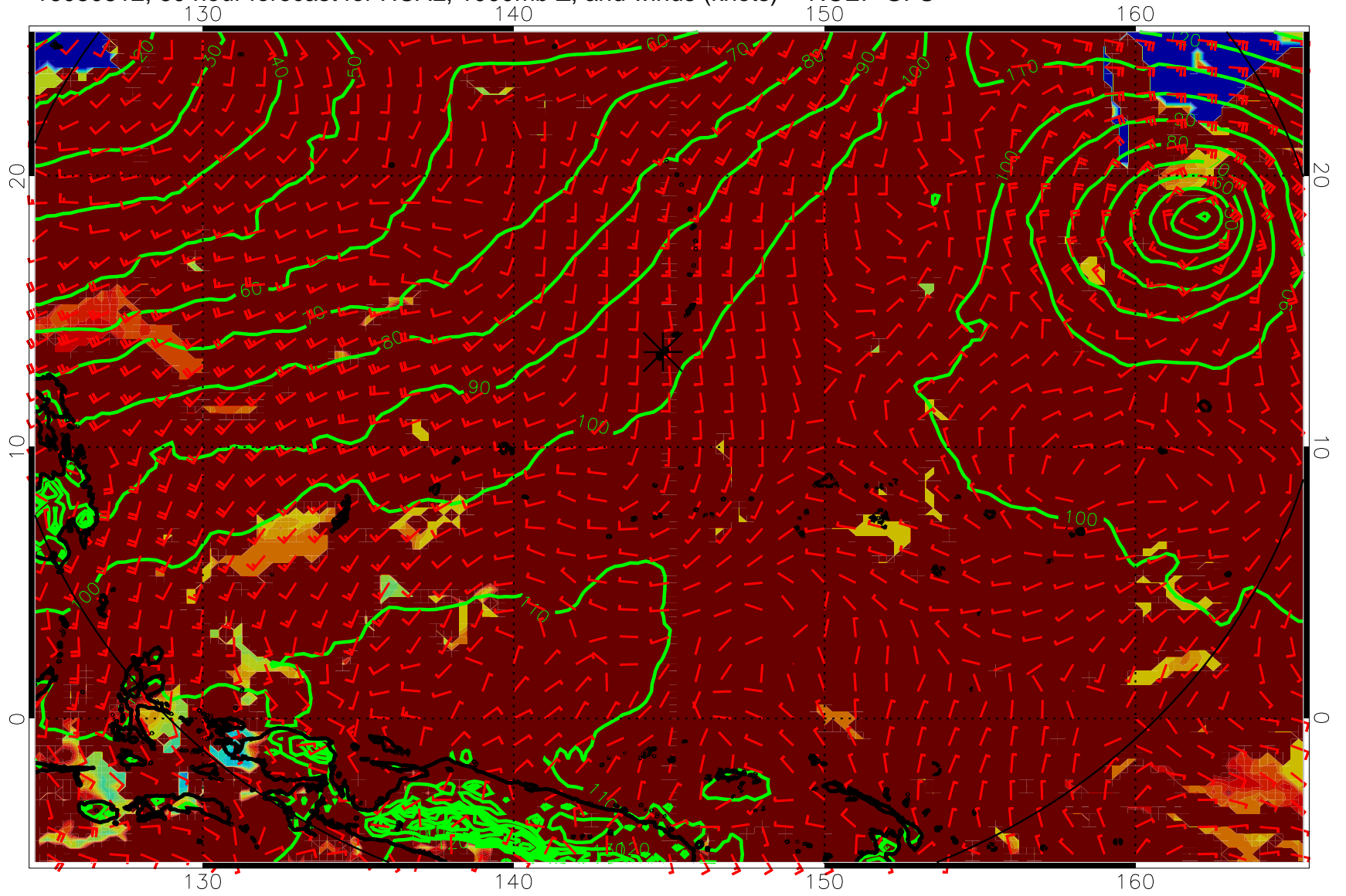
16080812, 60 hour forecast for HCAL, 1000mb Z, and winds (knots) -- NCEP GFS
