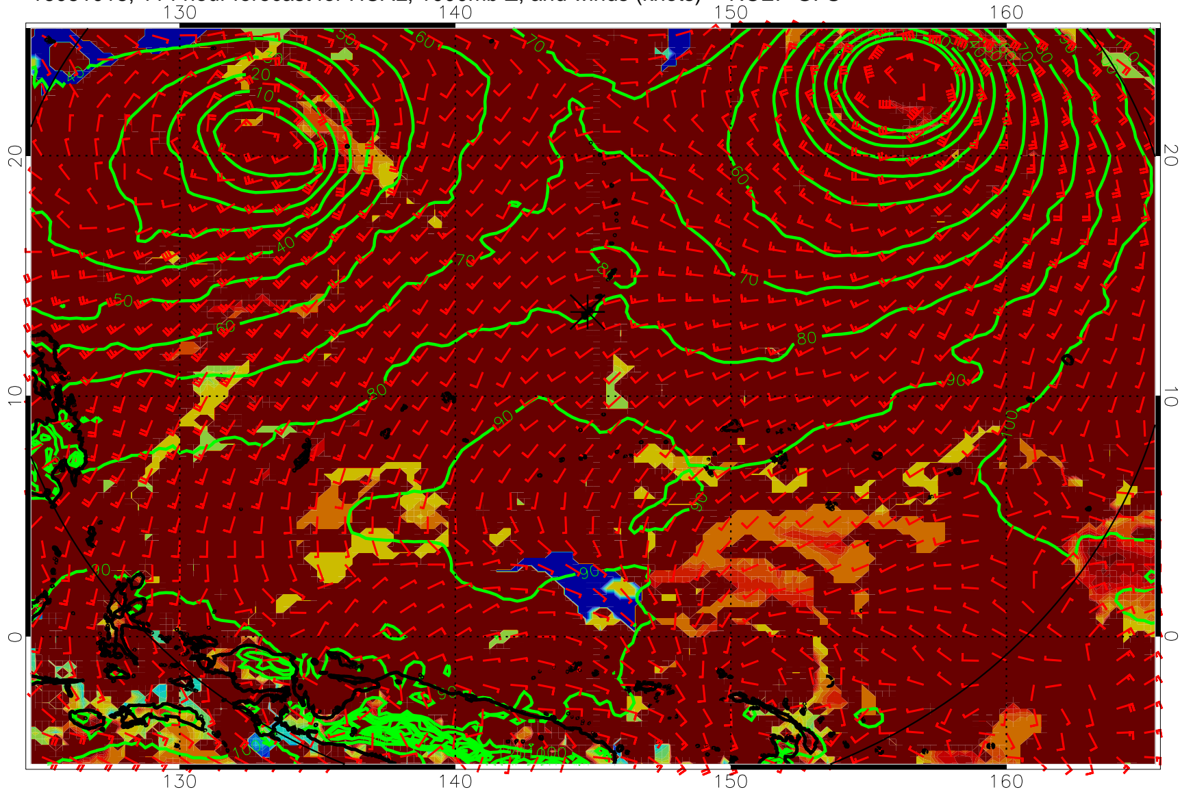
16081018, 114 hour forecast for HCAL, 1000mb Z, and winds (knots) -- NCEP GFS
