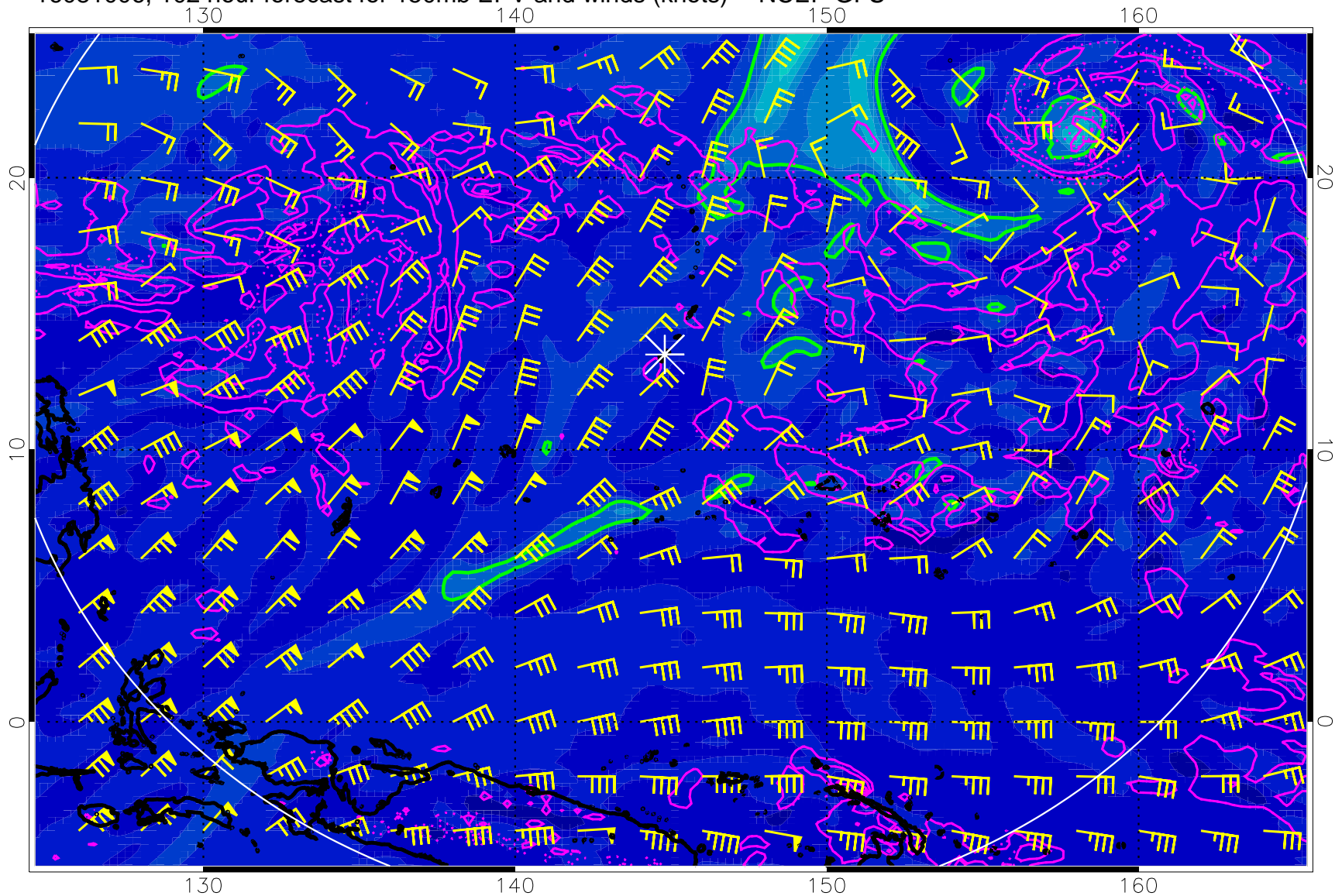
16081006, 102 hour forecast for 150mb EPV and winds (knots) -- NCEP GFS
