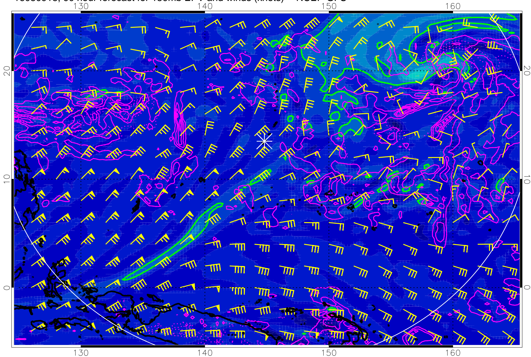
16080918, 90 hour forecast for 150mb EPV and winds (knots) -- NCEP GFS
