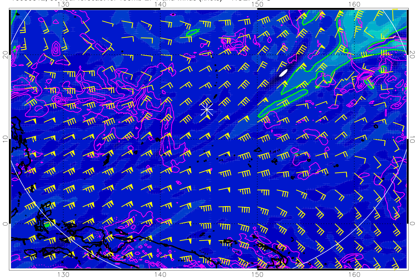
16080812, 60 hour forecast for 150mb EPV and winds (knots) -- NCEP GFS
