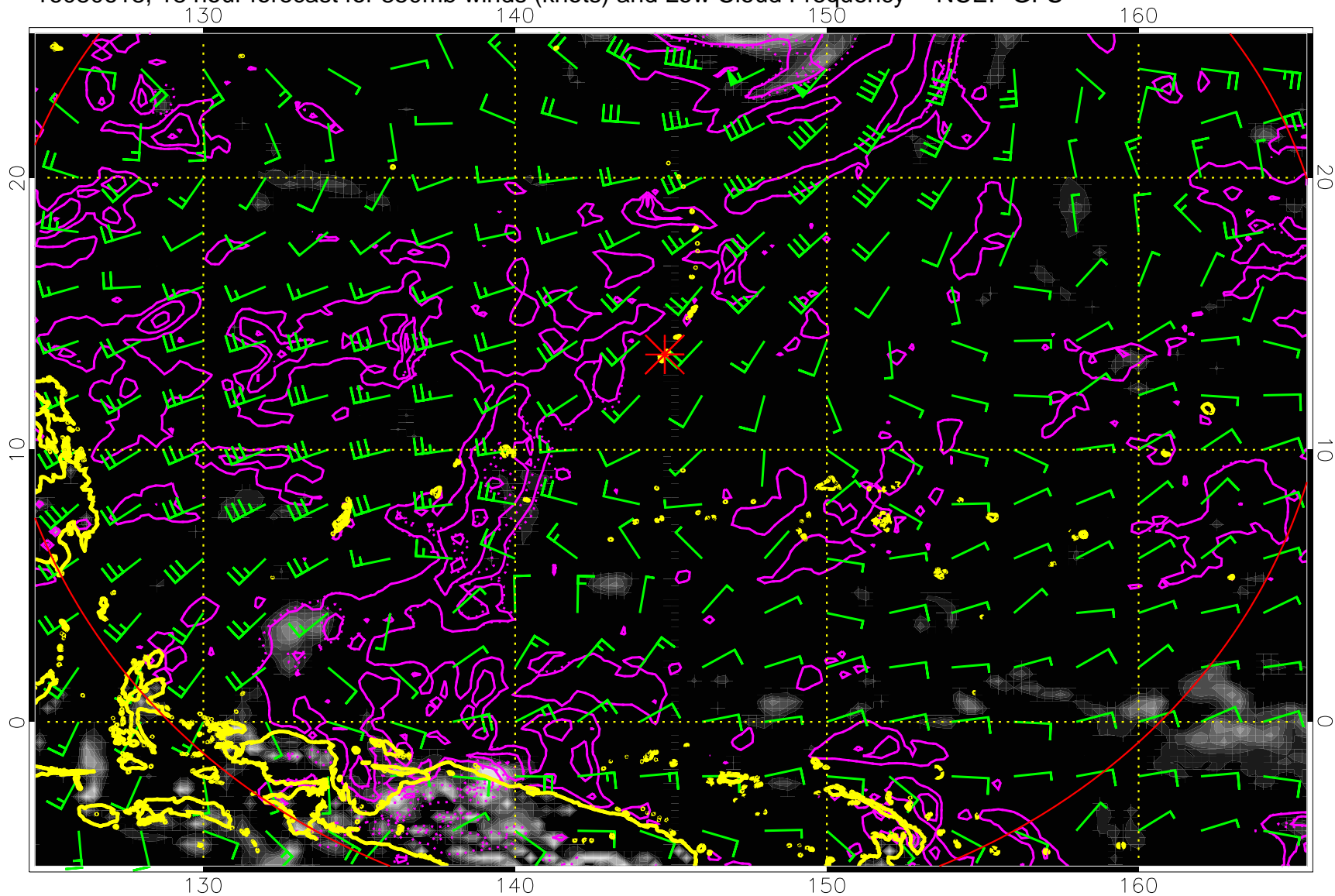
16080618, 18 hour forecast for 850mb winds (knots) and Low Cloud Frequency -- NCEP GFS
