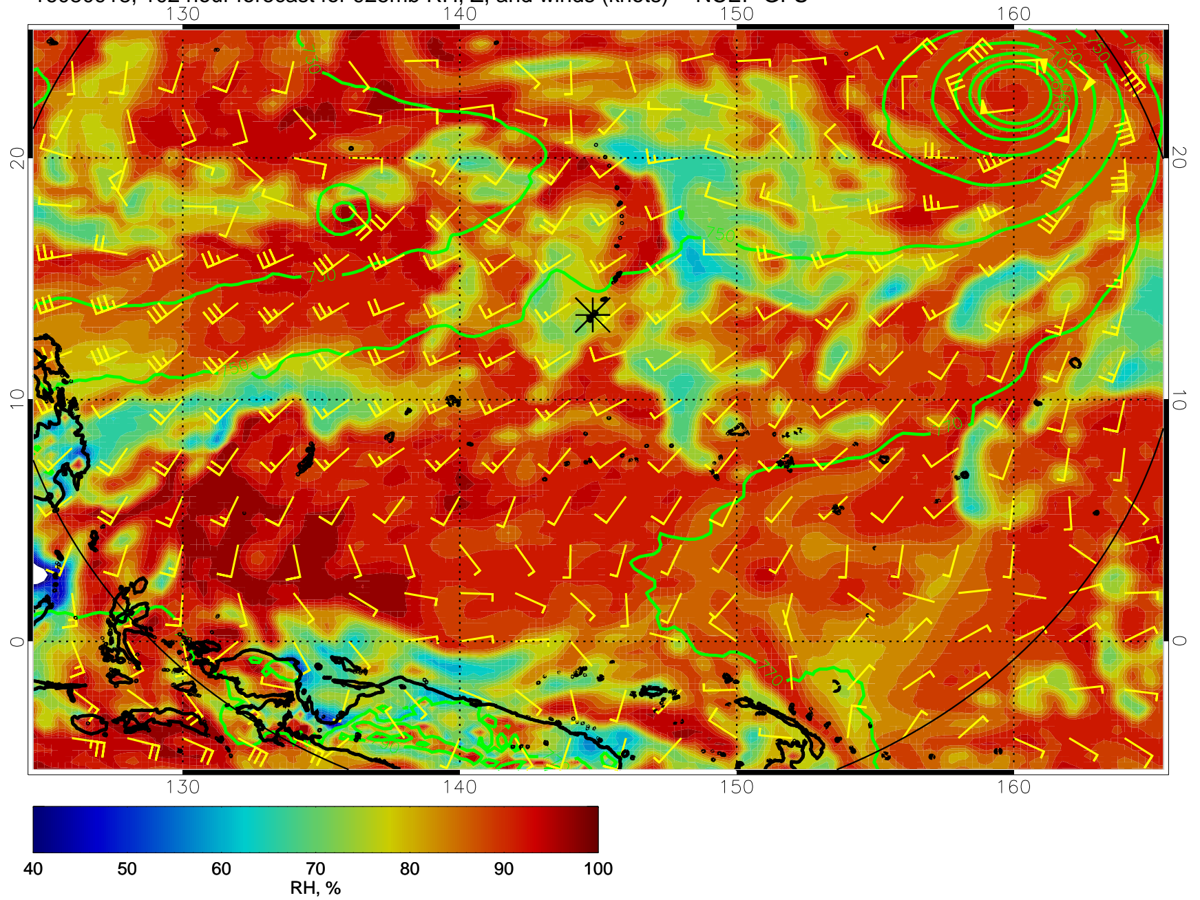
16080918, 102 hour forecast for 925mb RH, Z, and winds (knots) -- NCEP GFS
