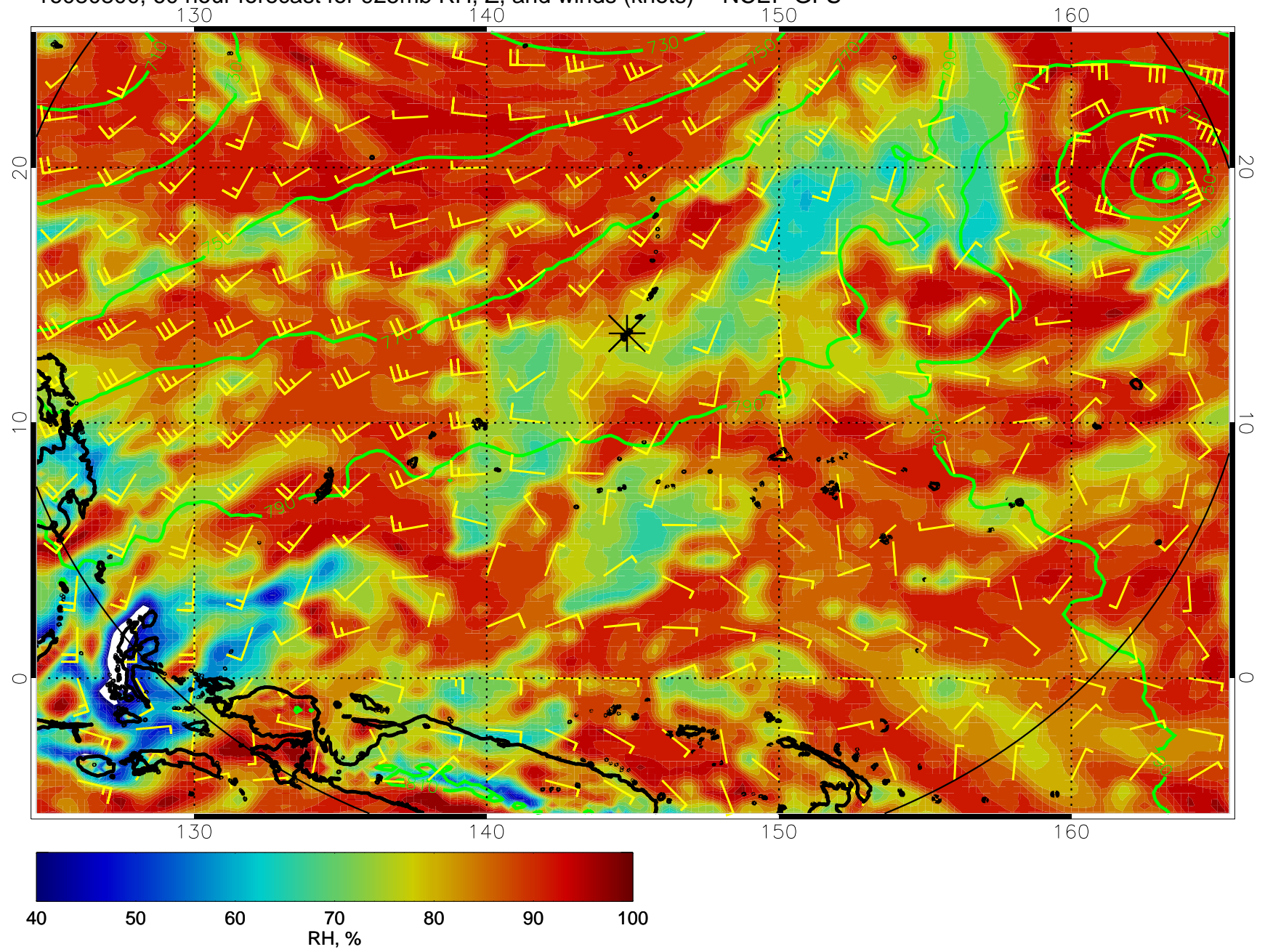
16080800, 60 hour forecast for 925mb RH, Z, and winds (knots) -- NCEP GFS
