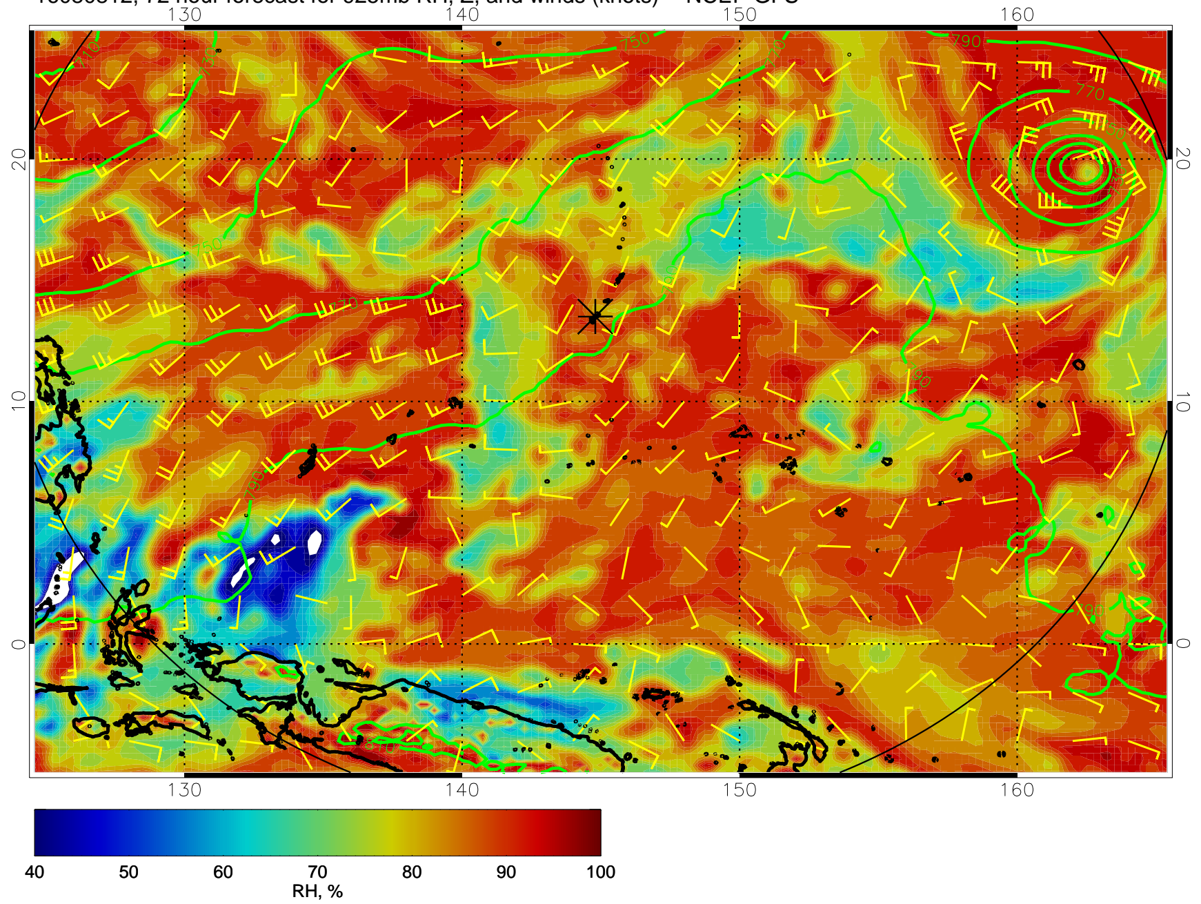
16080812, 72 hour forecast for 925mb RH, Z, and winds (knots) -- NCEP GFS
