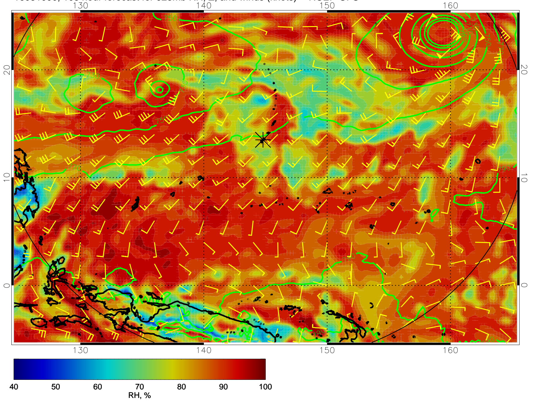
16081000, 108 hour forecast for 925mb RH, Z, and winds (knots) -- NCEP GFS
