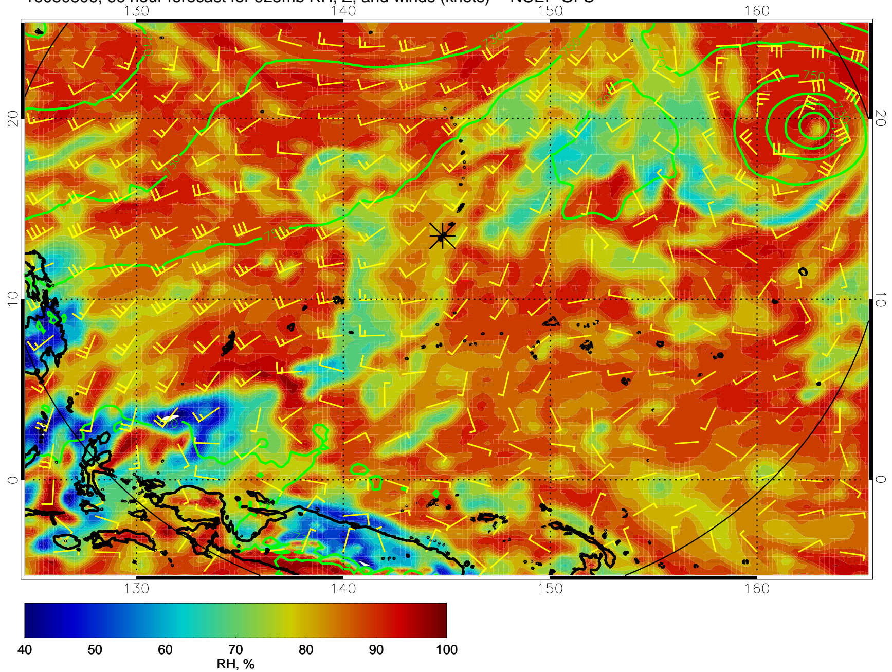
16080806, 66 hour forecast for 925mb RH, Z, and winds (knots) -- NCEP GFS
