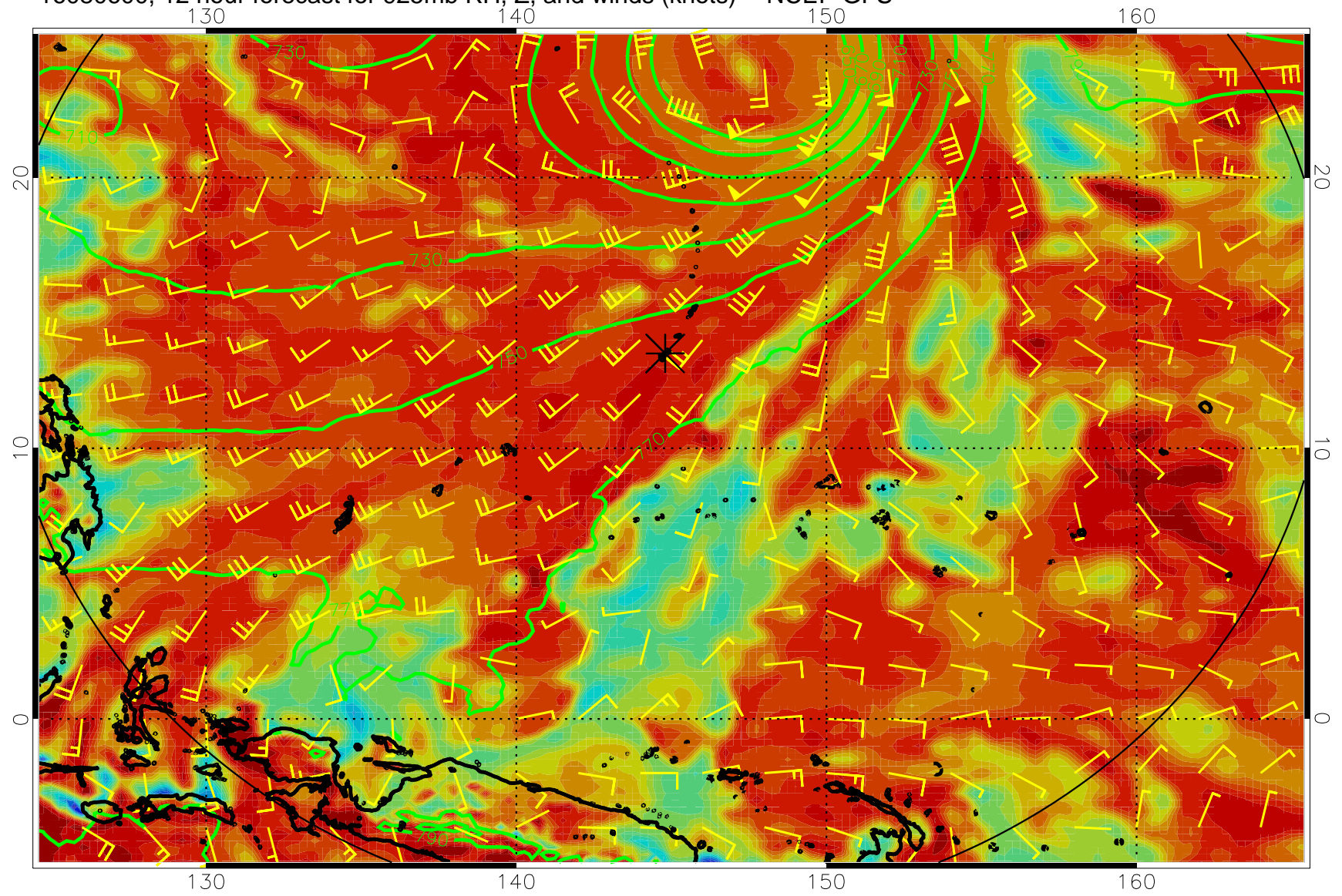
16080600, 12 hour forecast for 925mb RH, Z, and winds (knots) -- NCEP GFS
