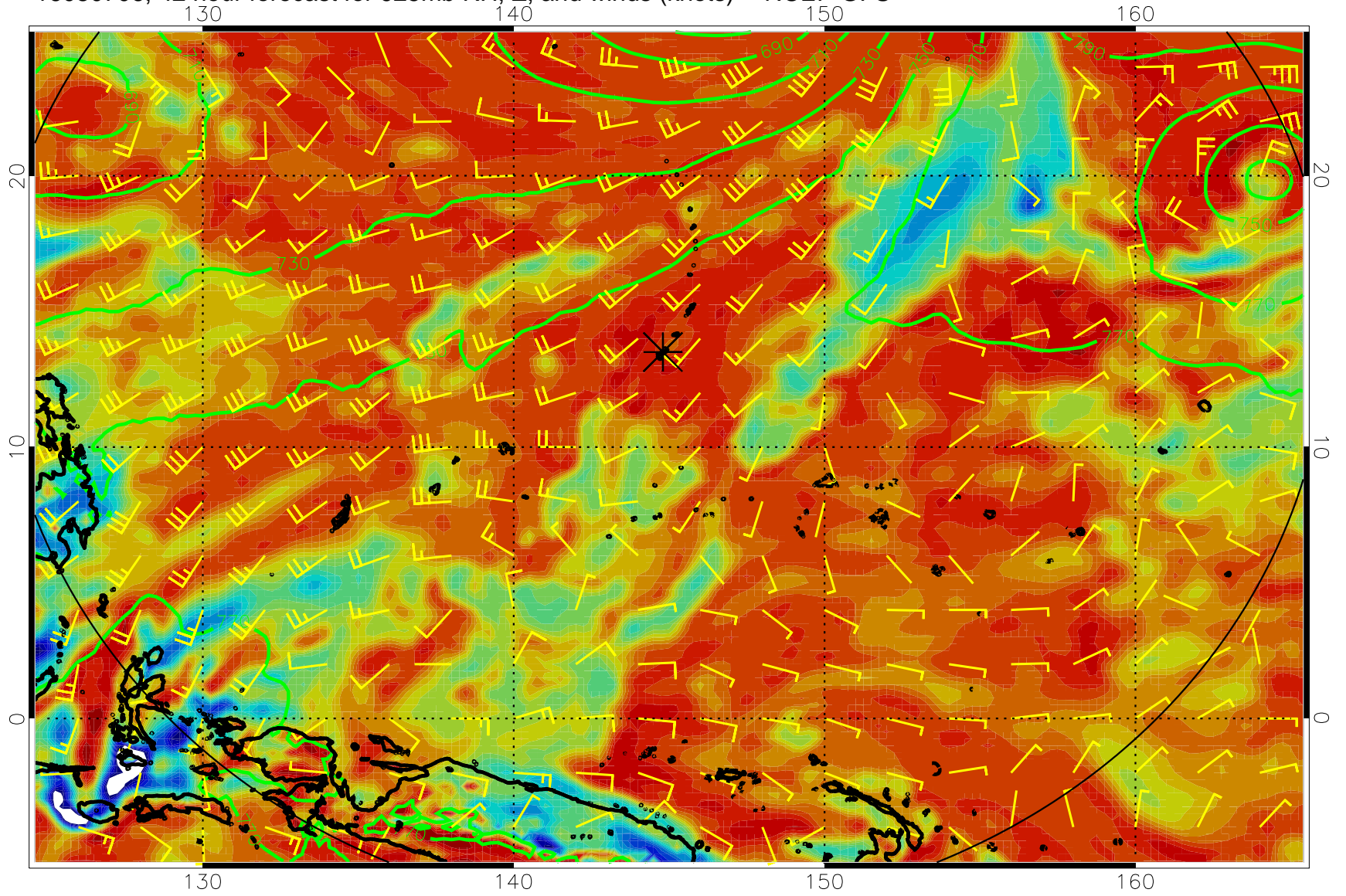
16080706, 42 hour forecast for 925mb RH, Z, and winds (knots) -- NCEP GFS
