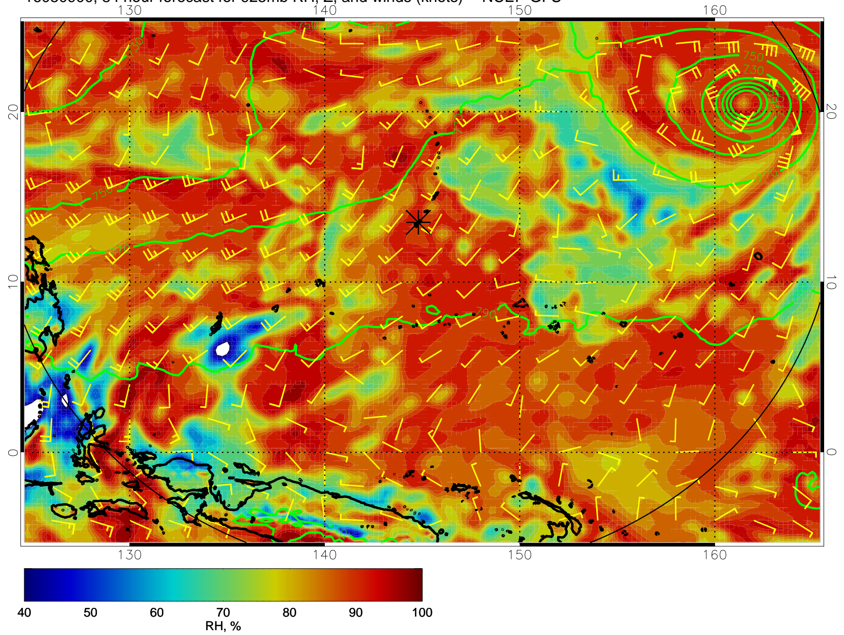
16080900, 84 hour forecast for 925mb RH, Z, and winds (knots) -- NCEP GFS
