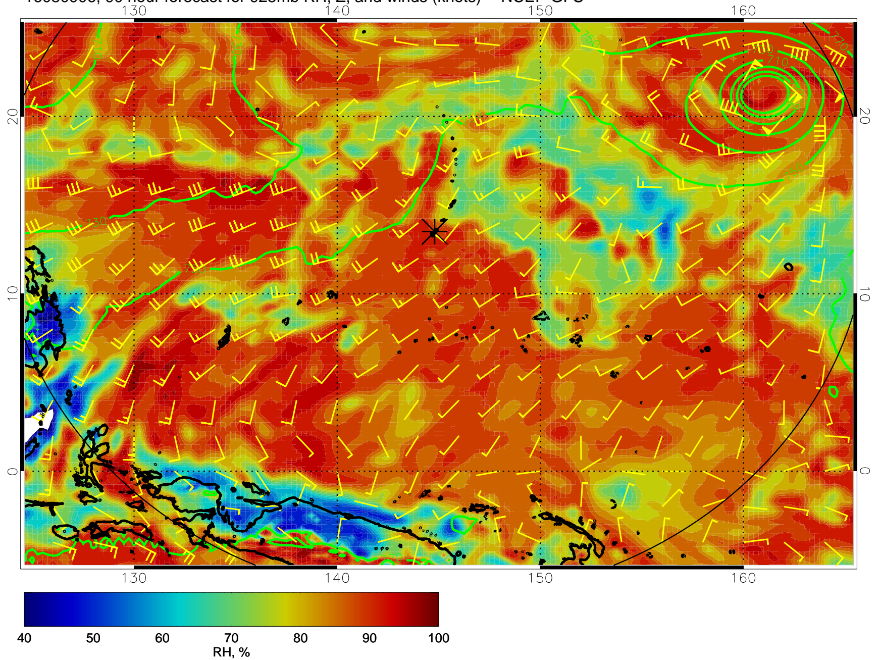
16080906, 90 hour forecast for 925mb RH, Z, and winds (knots) -- NCEP GFS
