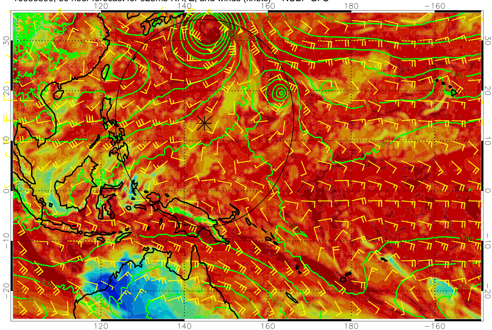
16080800, 60 hour forecast for 925mb RH, Z, and winds (knots) -- NCEP GFS
