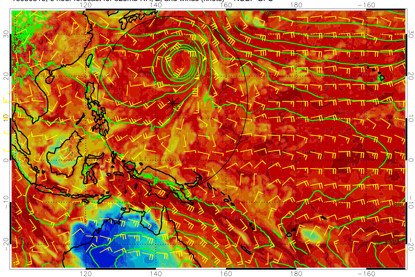
16080518, 6 hour forecast for 925mb RH, Z, and winds (knots) -- NCEP GFS
