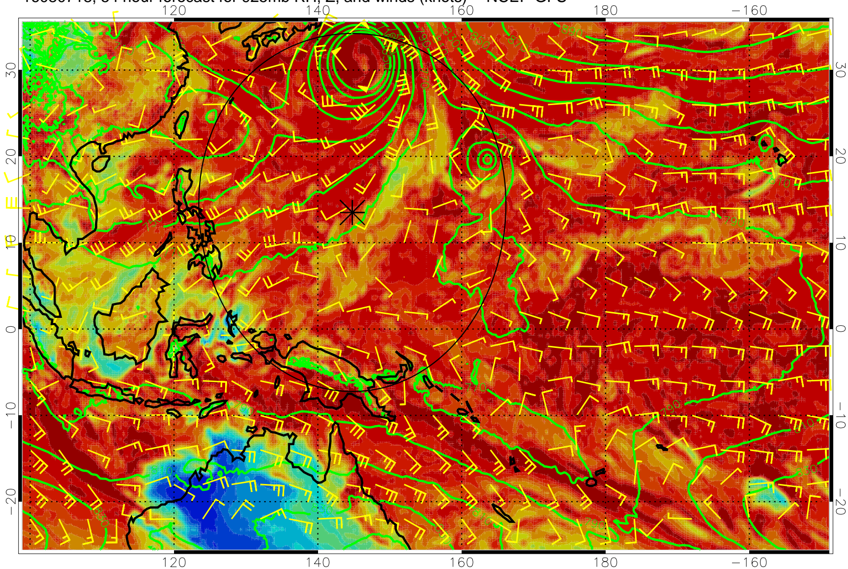
16080718, 54 hour forecast for 925mb RH, Z, and winds (knots) -- NCEP GFS
