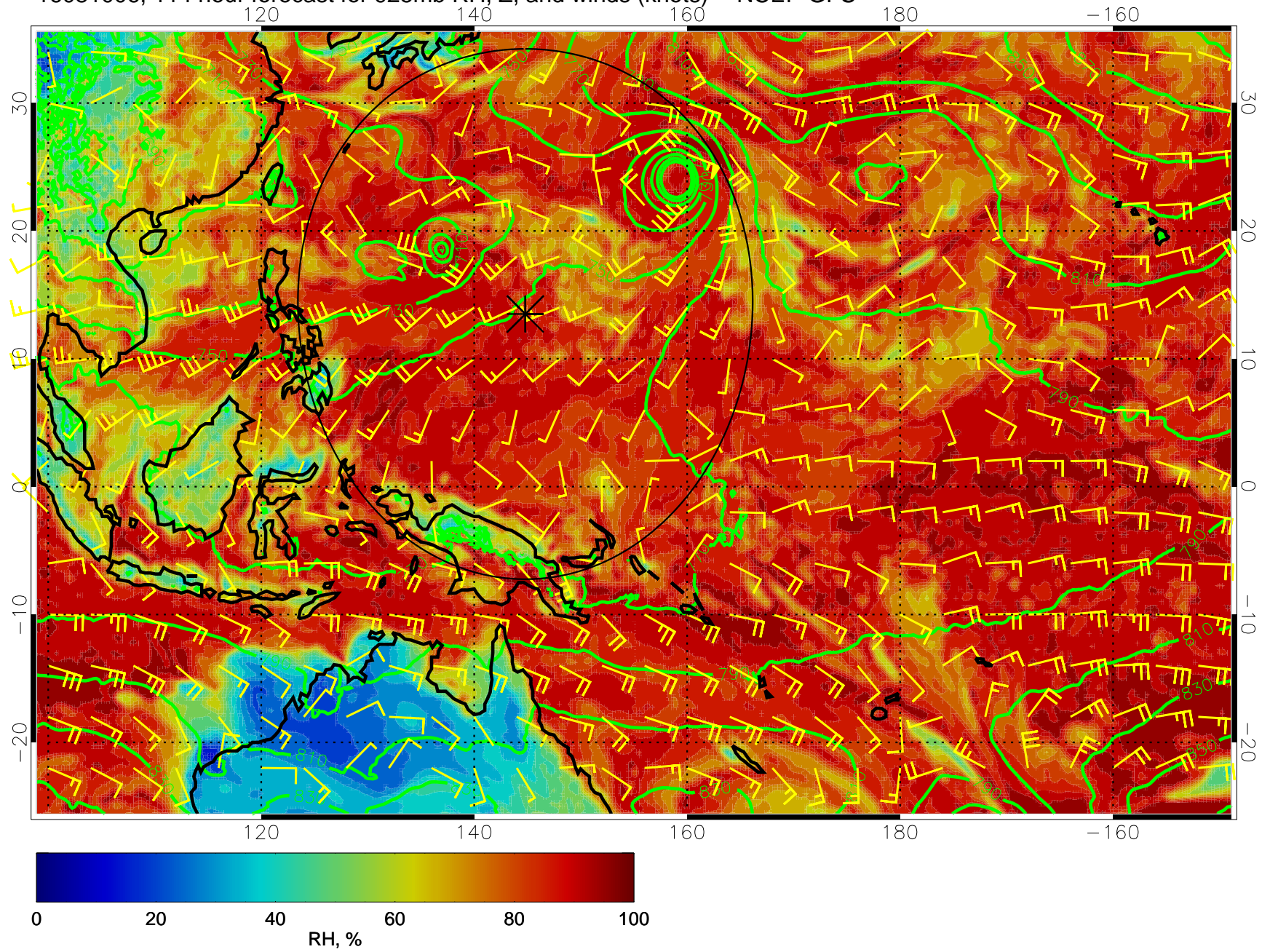
16081006, 114 hour forecast for 925mb RH, Z, and winds (knots) -- NCEP GFS
