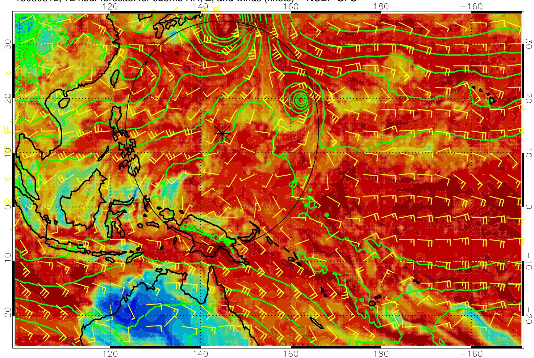
16080812, 72 hour forecast for 925mb RH, Z, and winds (knots) -- NCEP GFS
