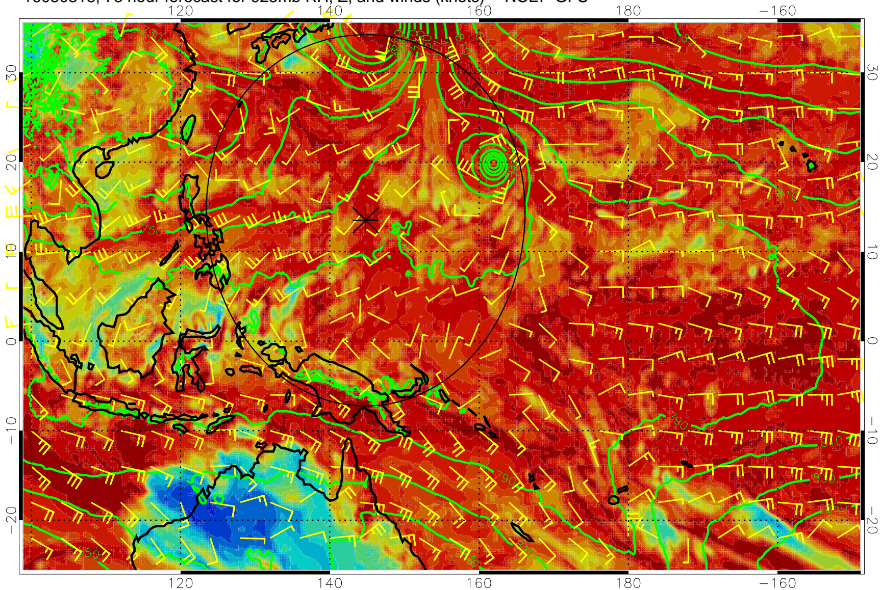
16080818, 78 hour forecast for 925mb RH, Z, and winds (knots) -- NCEP GFS
