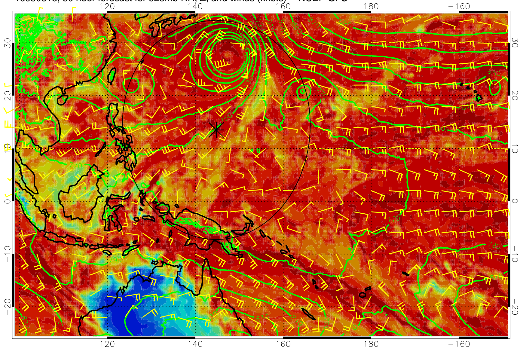
16080618, 30 hour forecast for 925mb RH, Z, and winds (knots) -- NCEP GFS
