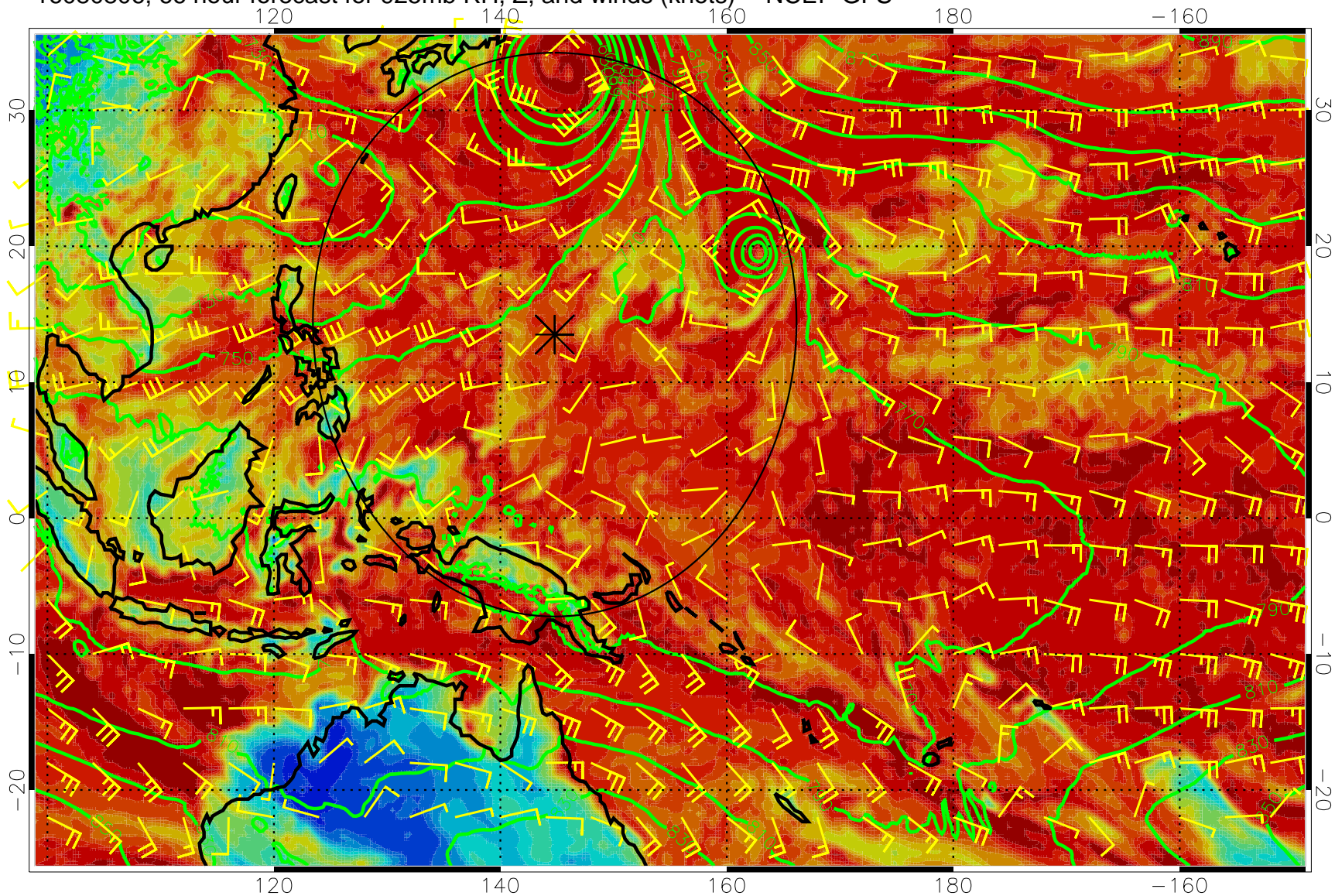
16080806, 66 hour forecast for 925mb RH, Z, and winds (knots) -- NCEP GFS
