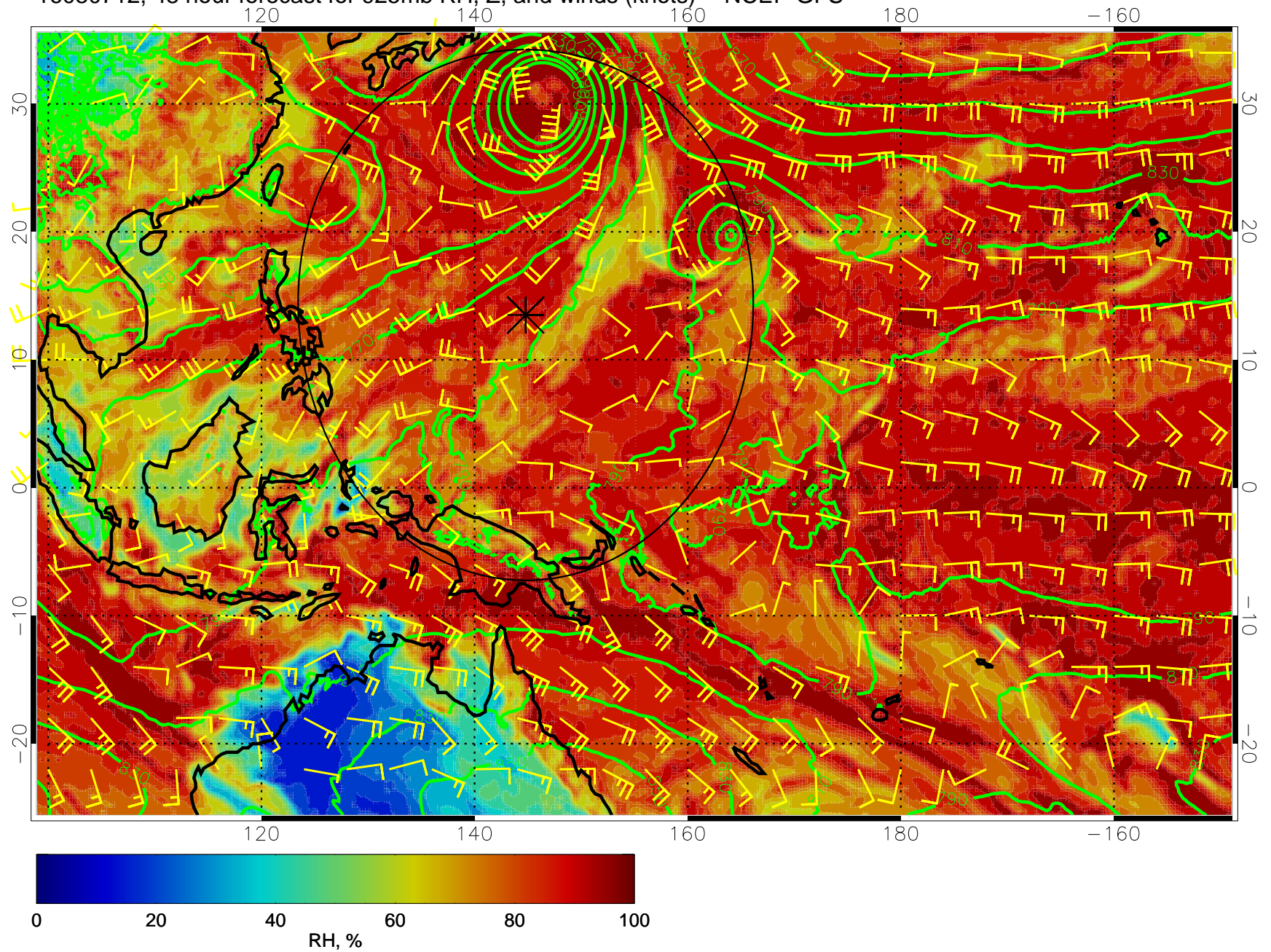
16080712, 48 hour forecast for 925mb RH, Z, and winds (knots) -- NCEP GFS
