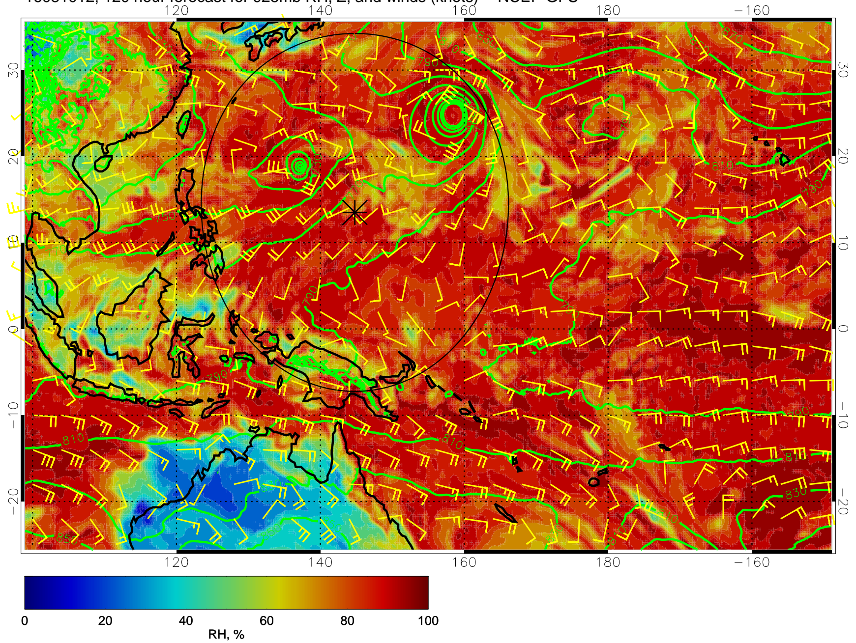
16081012, 120 hour forecast for 925mb RH, Z, and winds (knots) -- NCEP GFS
