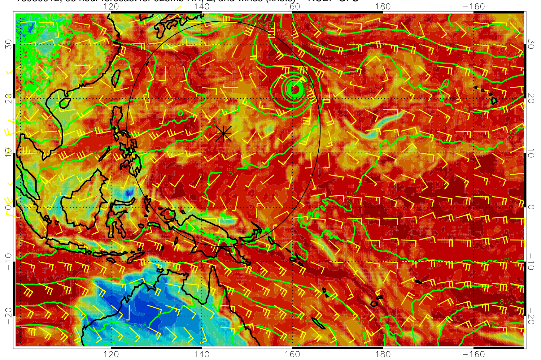
16080912, 96 hour forecast for 925mb RH, Z, and winds (knots) -- NCEP GFS
