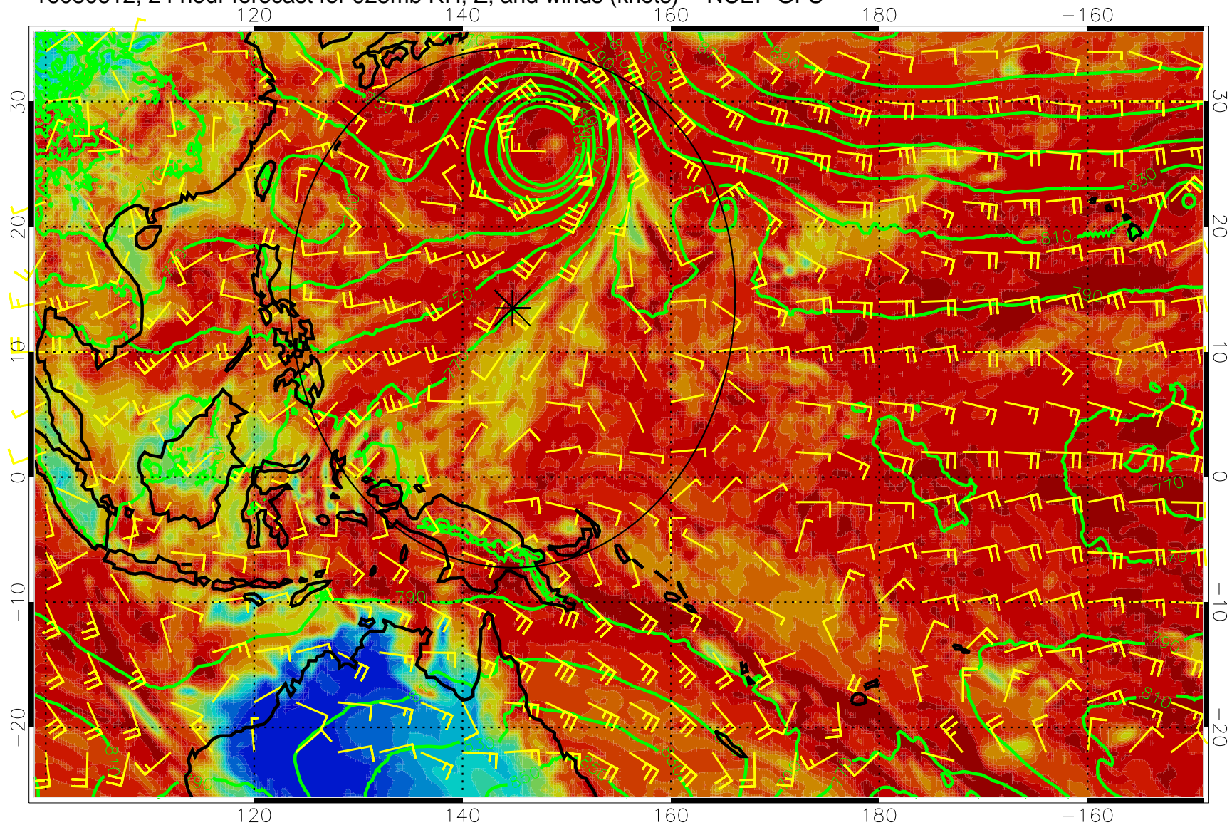
16080612, 24 hour forecast for 925mb RH, Z, and winds (knots) -- NCEP GFS
