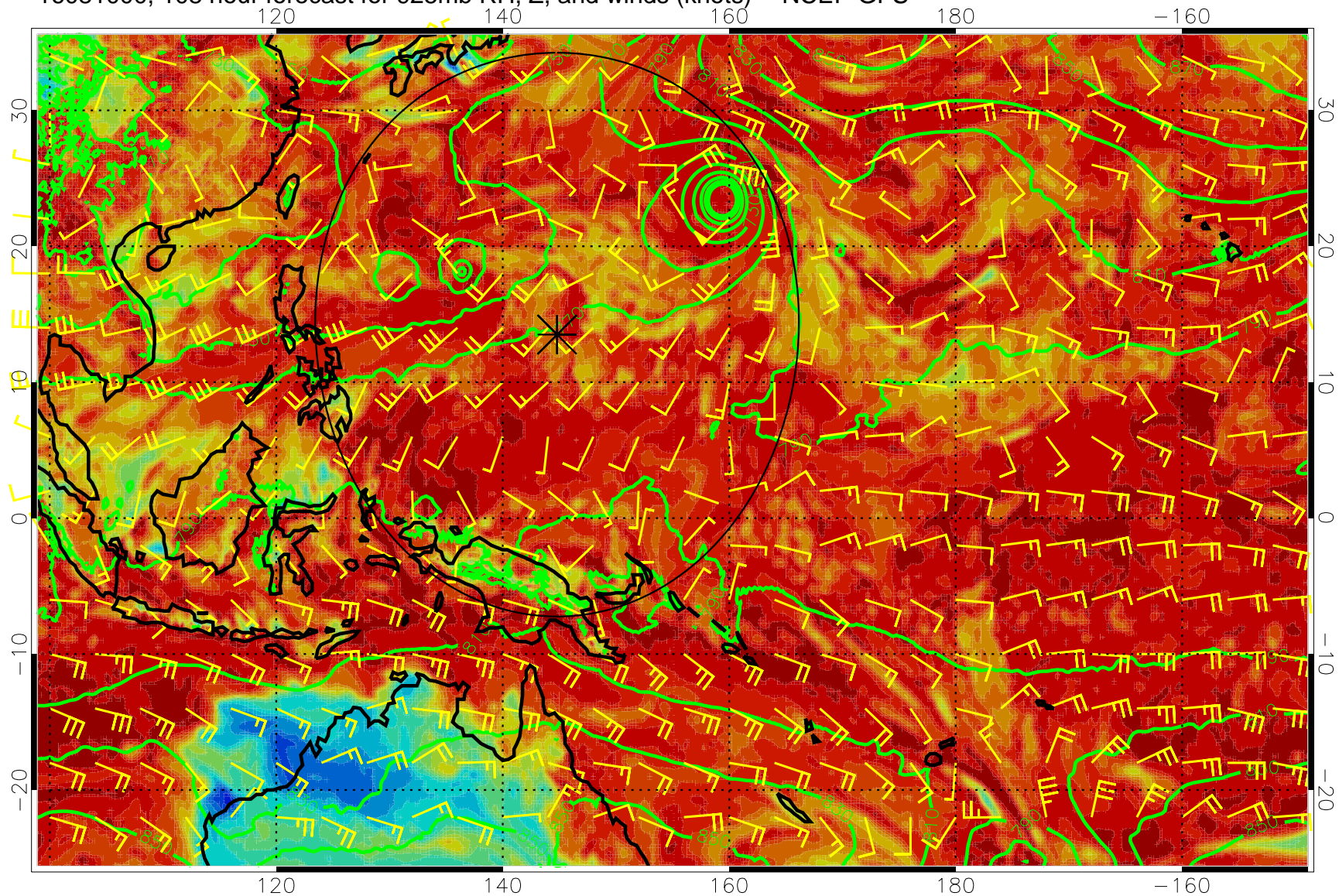
16081000, 108 hour forecast for 925mb RH, Z, and winds (knots) -- NCEP GFS
