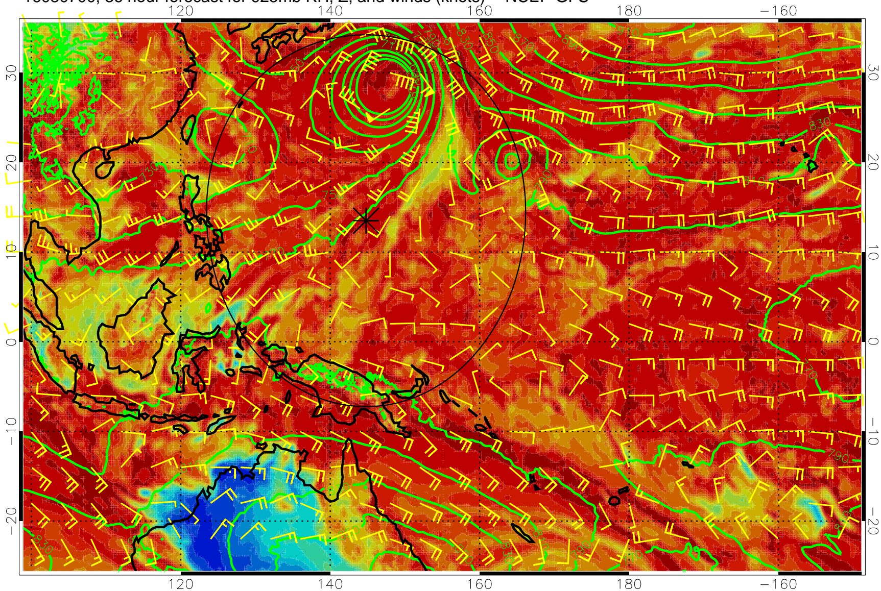
16080700, 36 hour forecast for 925mb RH, Z, and winds (knots) -- NCEP GFS
