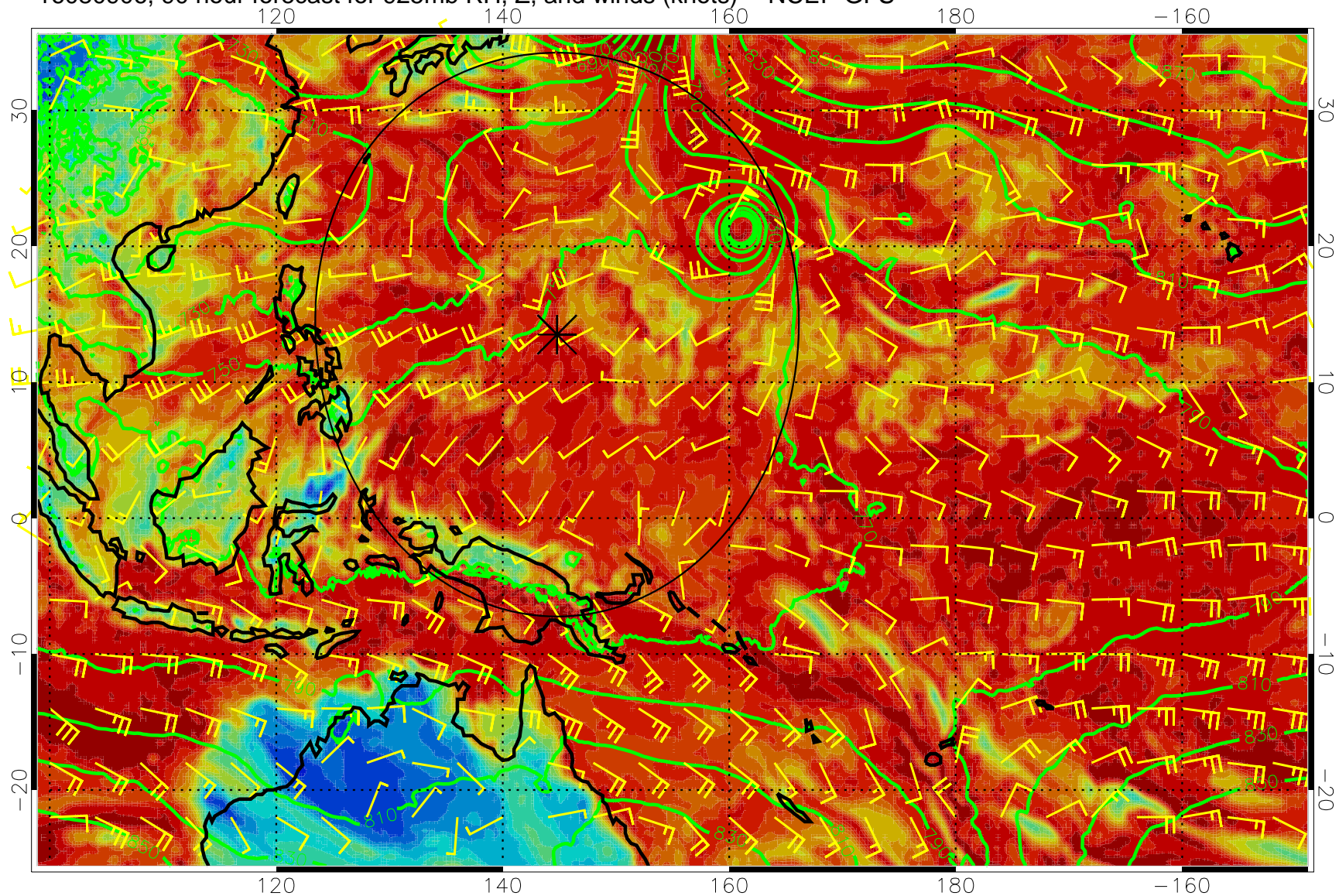
16080906, 90 hour forecast for 925mb RH, Z, and winds (knots) -- NCEP GFS
