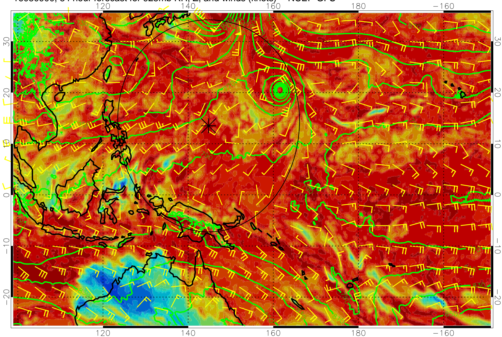
16080900, 84 hour forecast for 925mb RH, Z, and winds (knots) -- NCEP GFS
