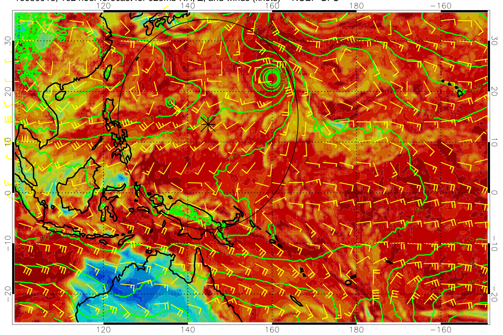
16080918, 102 hour forecast for 925mb RH, Z, and winds (knots) -- NCEP GFS
