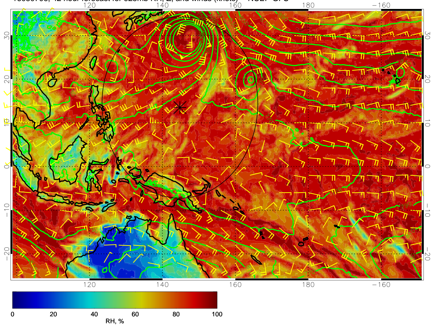
16080706, 42 hour forecast for 925mb RH, Z, and winds (knots) -- NCEP GFS
