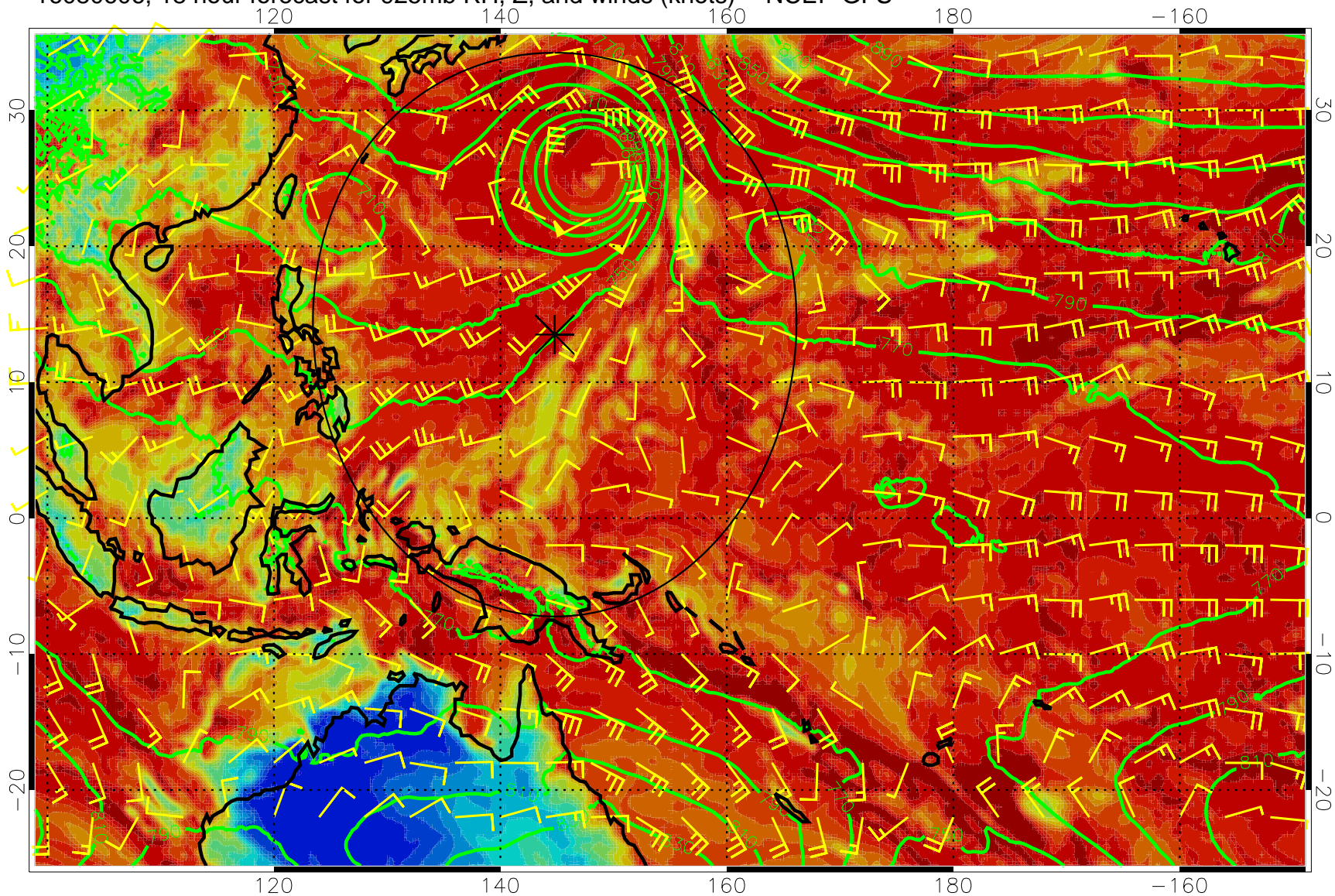
16080606, 18 hour forecast for 925mb RH, Z, and winds (knots) -- NCEP GFS
