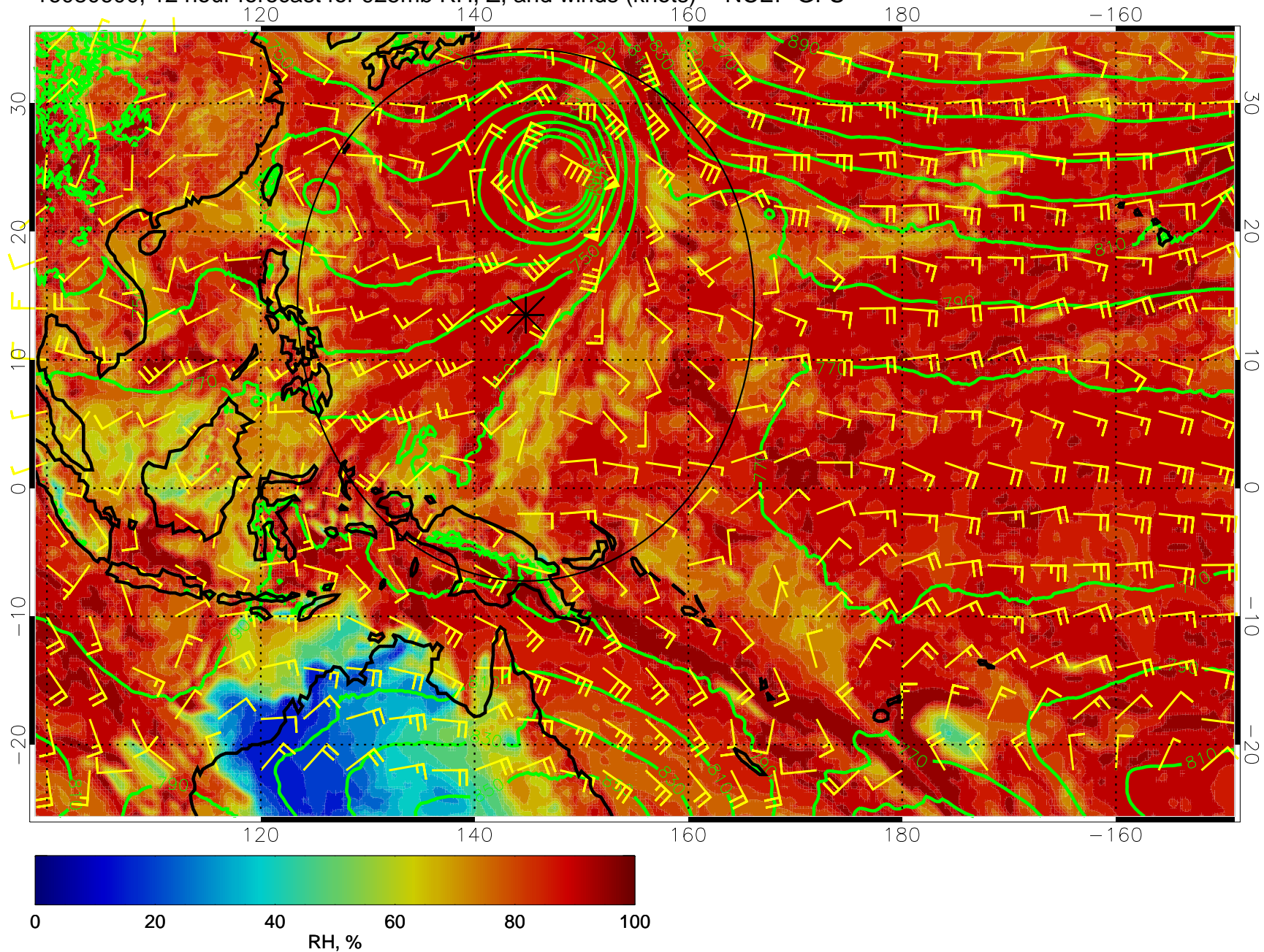
16080600, 12 hour forecast for 925mb RH, Z, and winds (knots) -- NCEP GFS
