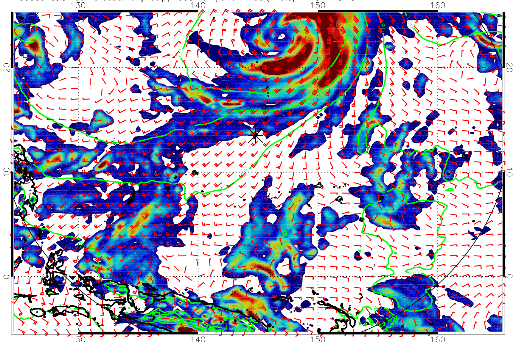
16080518, 6 hour forecast for precip, 1000mb Z, and winds (knots) -- NCEP GFS
