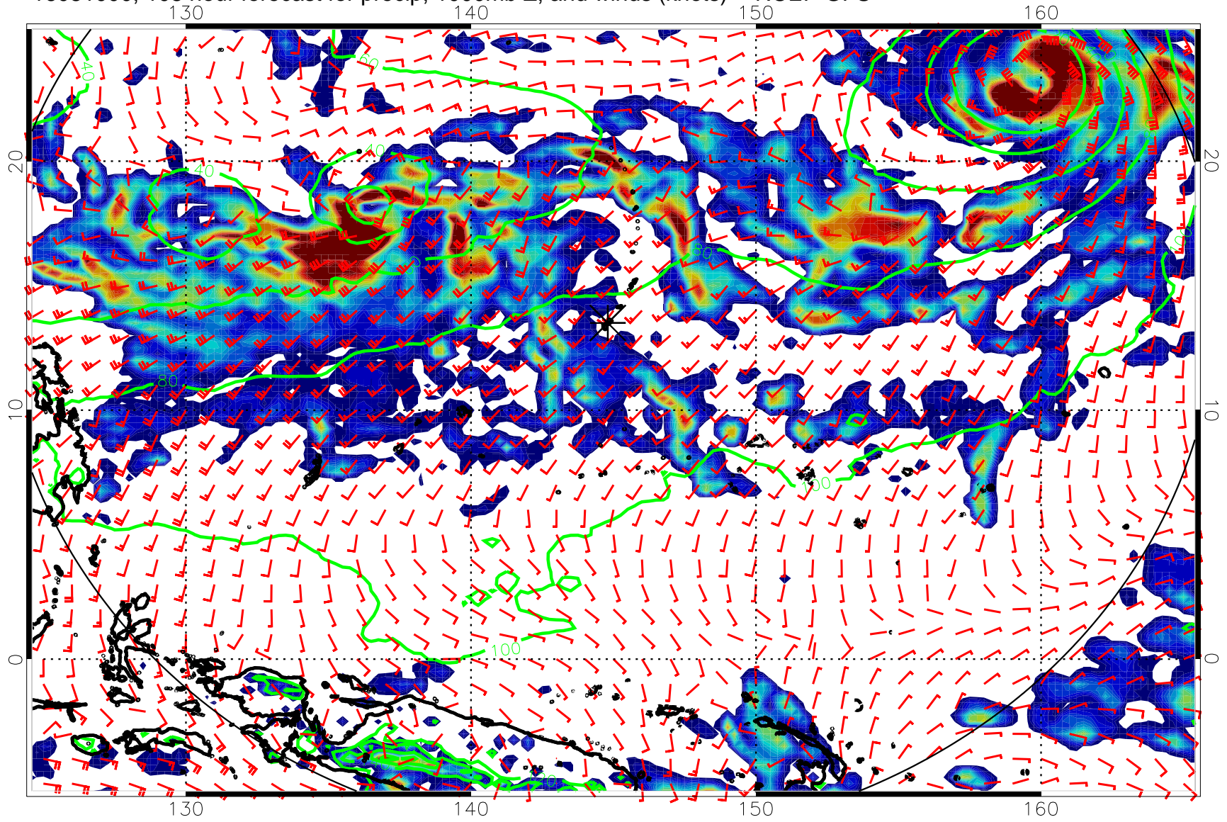
16081000, 108 hour forecast for precip, 1000mb Z, and winds (knots) -- NCEP GFS
