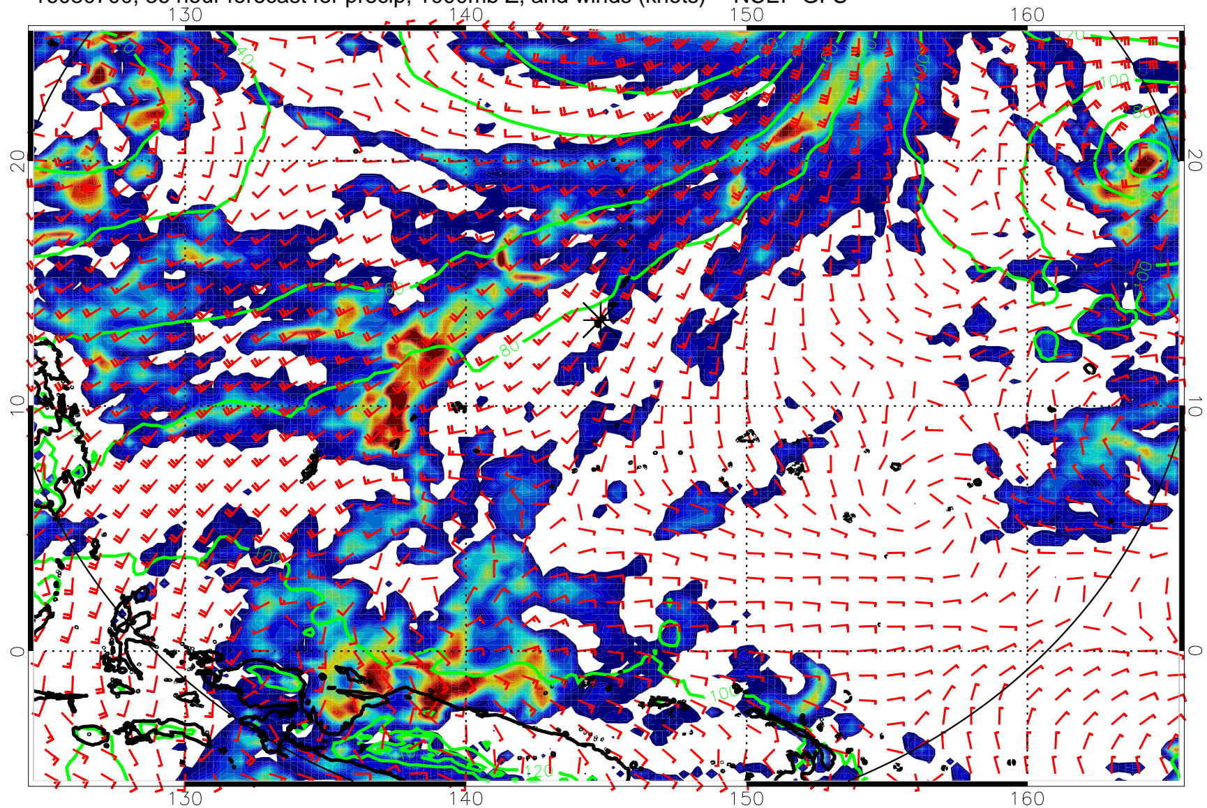
16080700, 36 hour forecast for precip, 1000mb Z, and winds (knots) -- NCEP GFS
