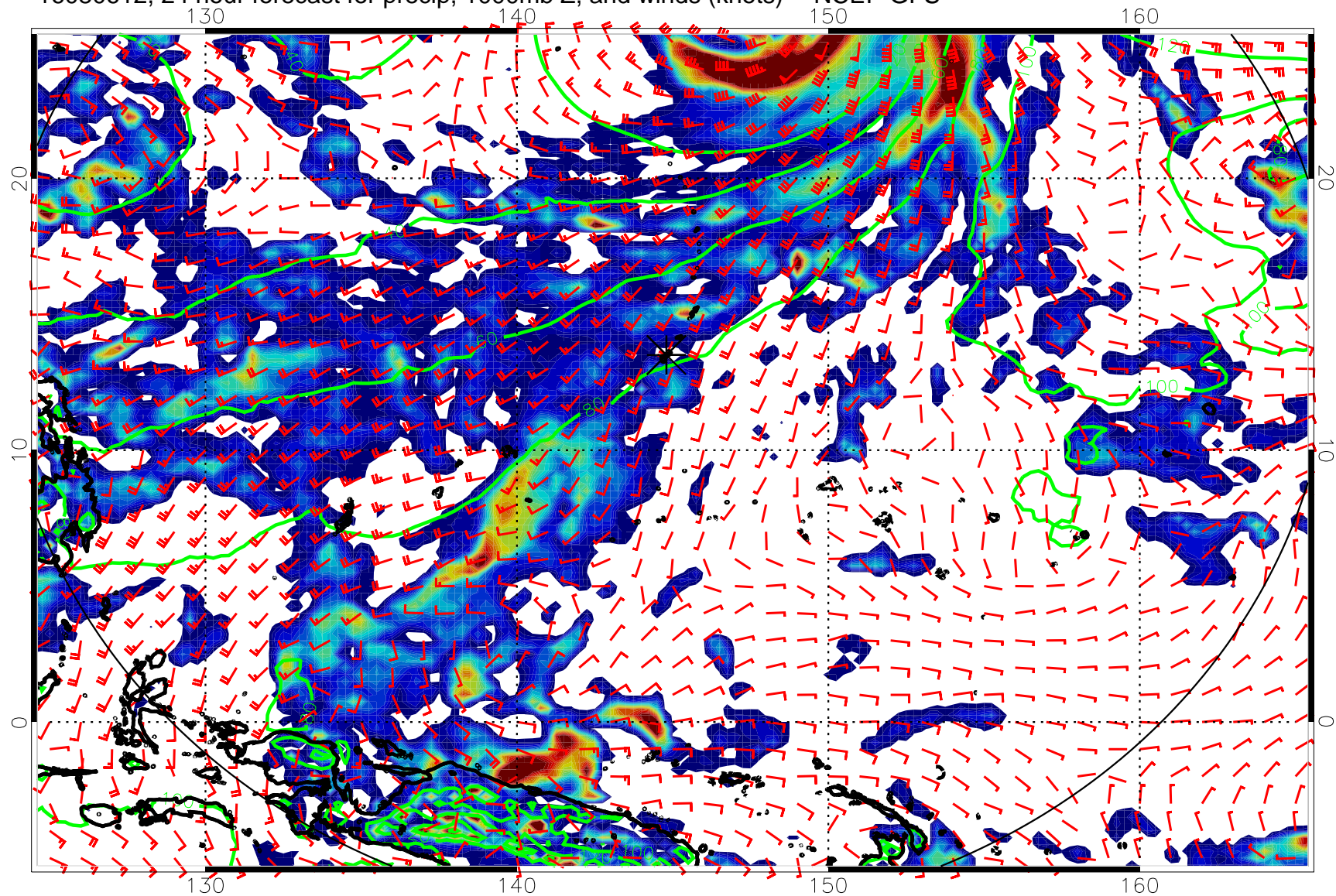
16080612, 24 hour forecast for precip, 1000mb Z, and winds (knots) -- NCEP GFS
