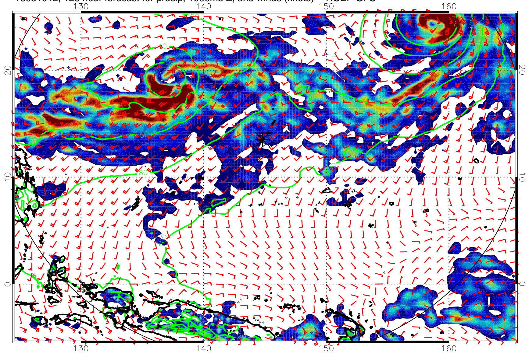
16081012, 120 hour forecast for precip, 1000mb Z, and winds (knots) -- NCEP GFS
