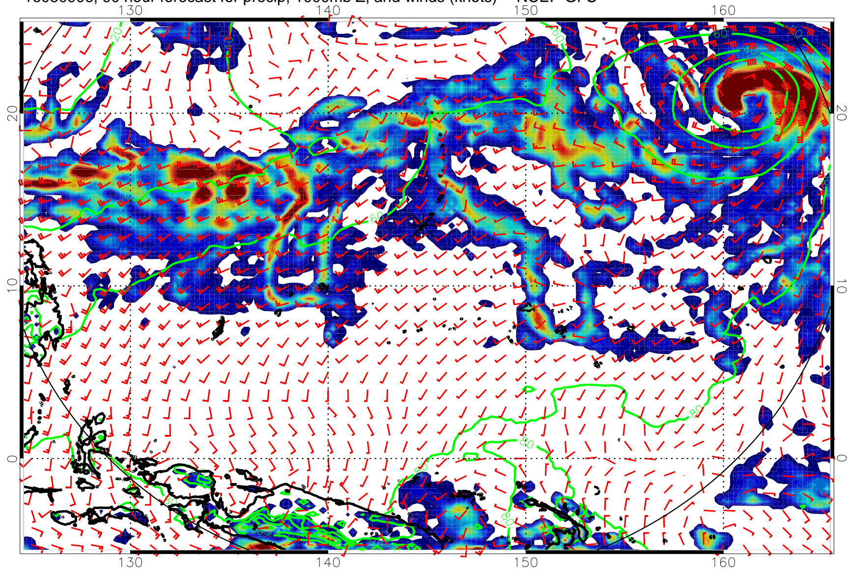
16080906, 90 hour forecast for precip, 1000mb Z, and winds (knots) -- NCEP GFS
