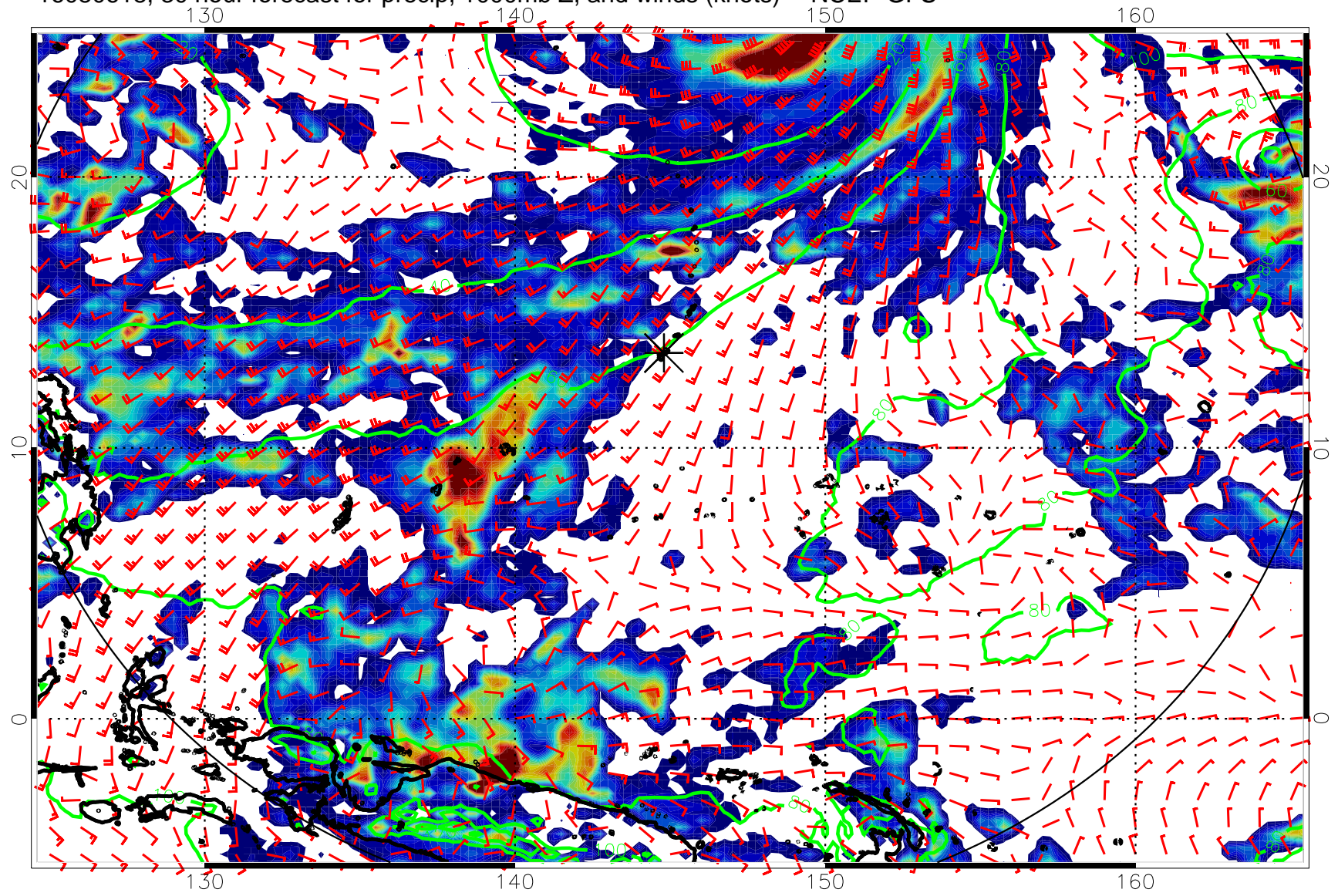
16080618, 30 hour forecast for precip, 1000mb Z, and winds (knots) -- NCEP GFS
