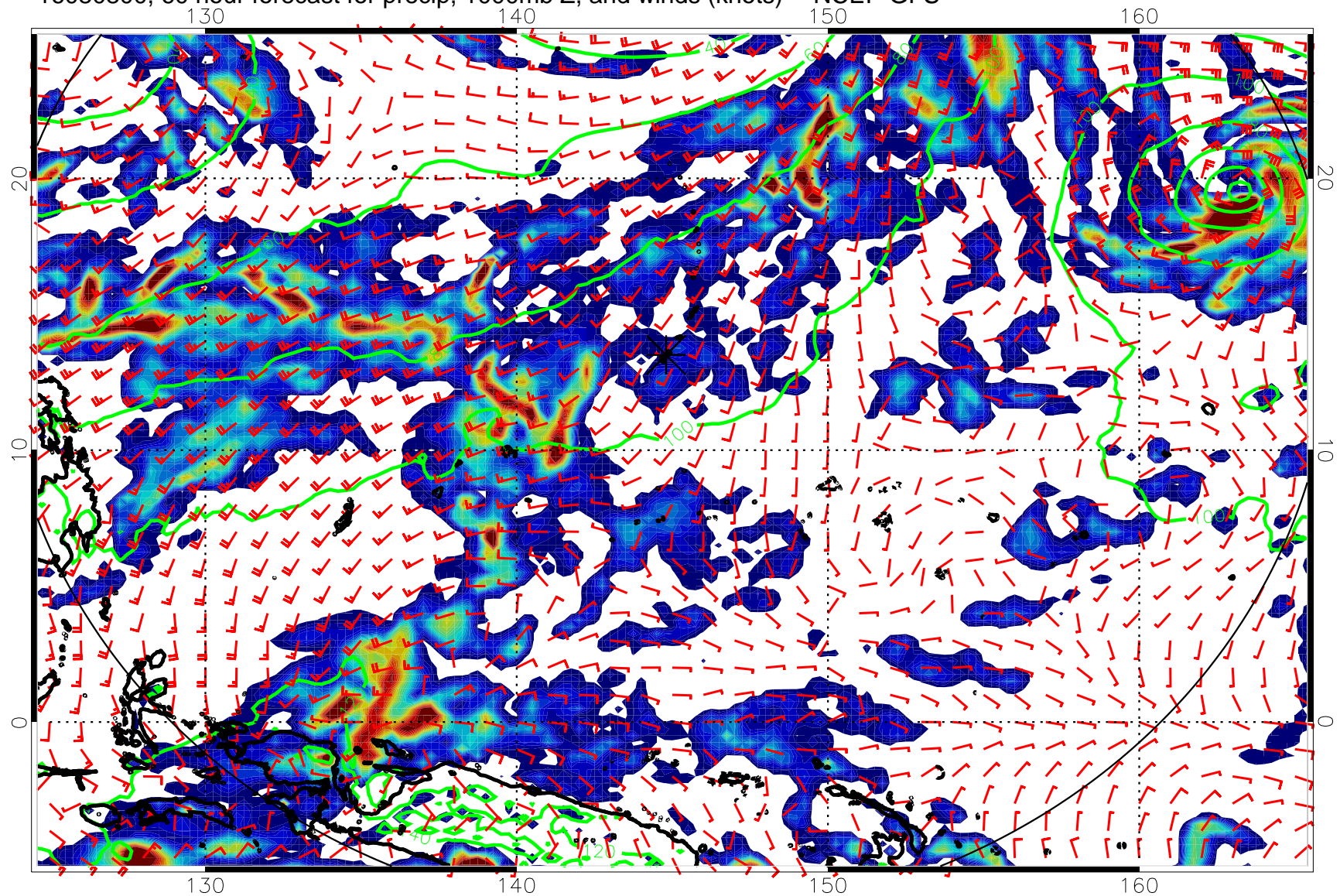
16080800, 60 hour forecast for precip, 1000mb Z, and winds (knots) -- NCEP GFS
