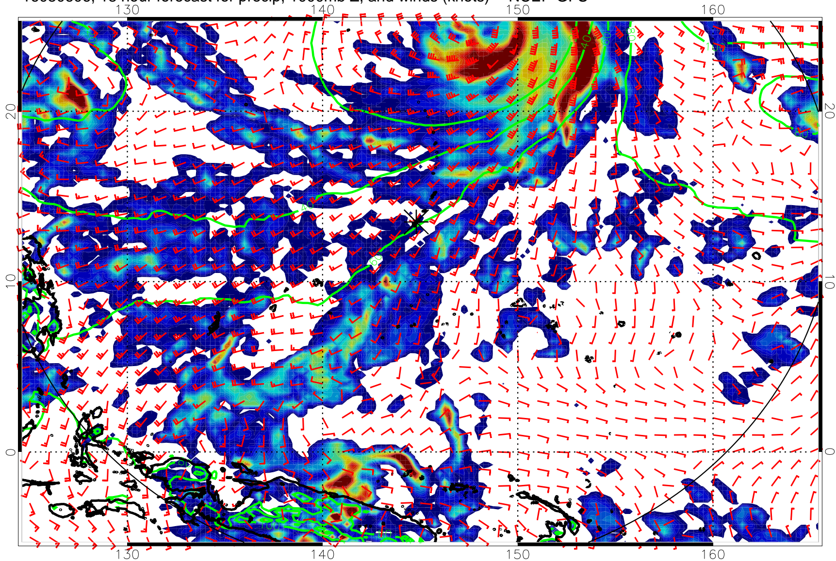
16080606, 18 hour forecast for precip, 1000mb Z, and winds (knots) -- NCEP GFS
