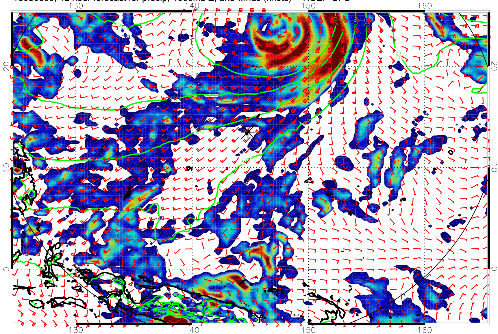
16080600, 12 hour forecast for precip, 1000mb Z, and winds (knots) -- NCEP GFS
