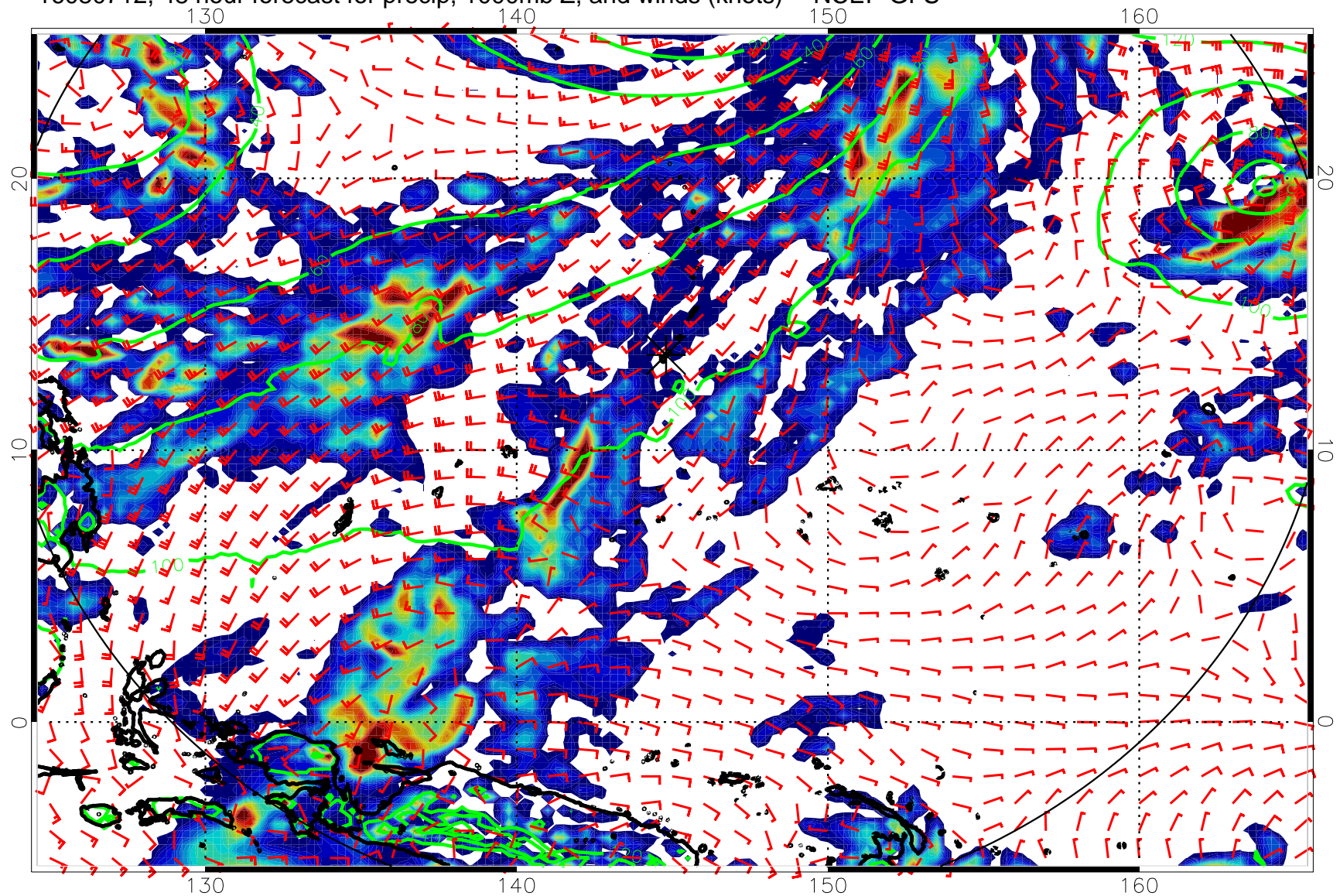
16080712, 48 hour forecast for precip, 1000mb Z, and winds (knots) -- NCEP GFS
