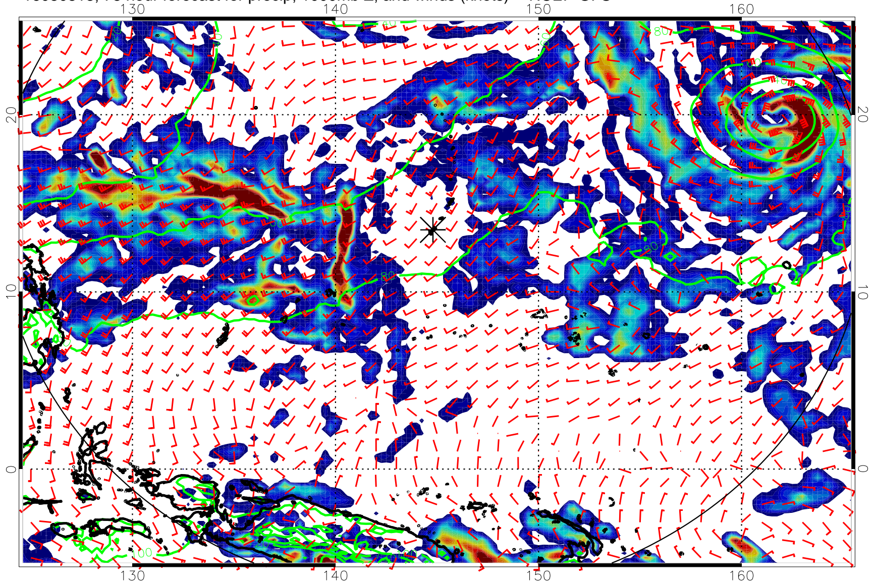
16080818, 78 hour forecast for precip, 1000mb Z, and winds (knots) -- NCEP GFS
