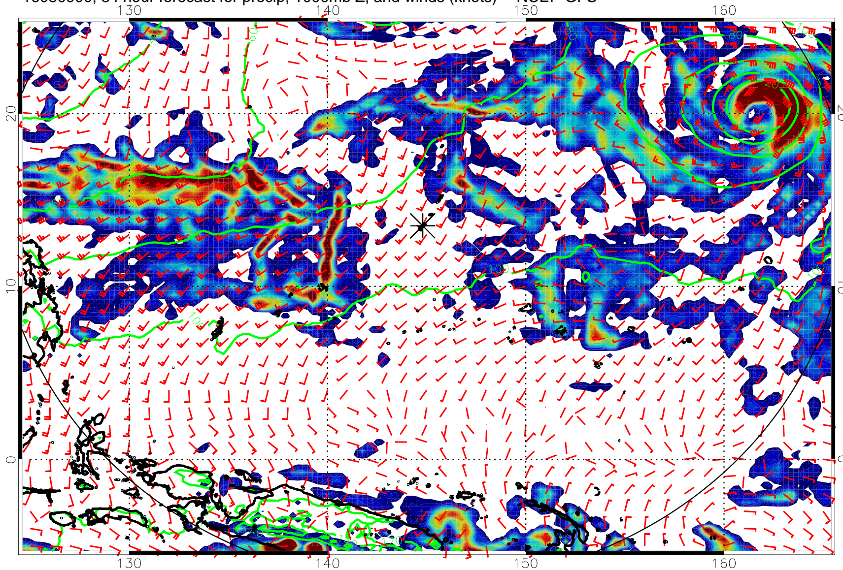
16080900, 84 hour forecast for precip, 1000mb Z, and winds (knots) -- NCEP GFS
