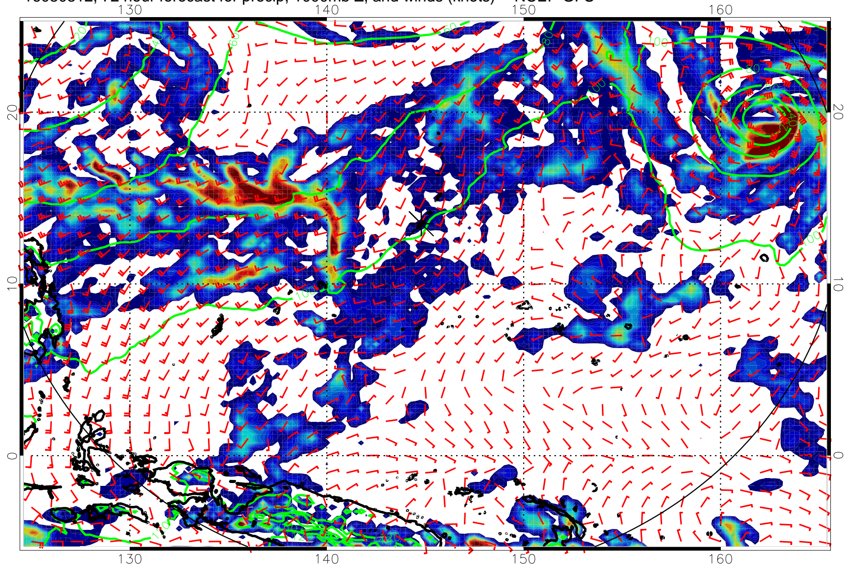
16080812, 72 hour forecast for precip, 1000mb Z, and winds (knots) -- NCEP GFS
