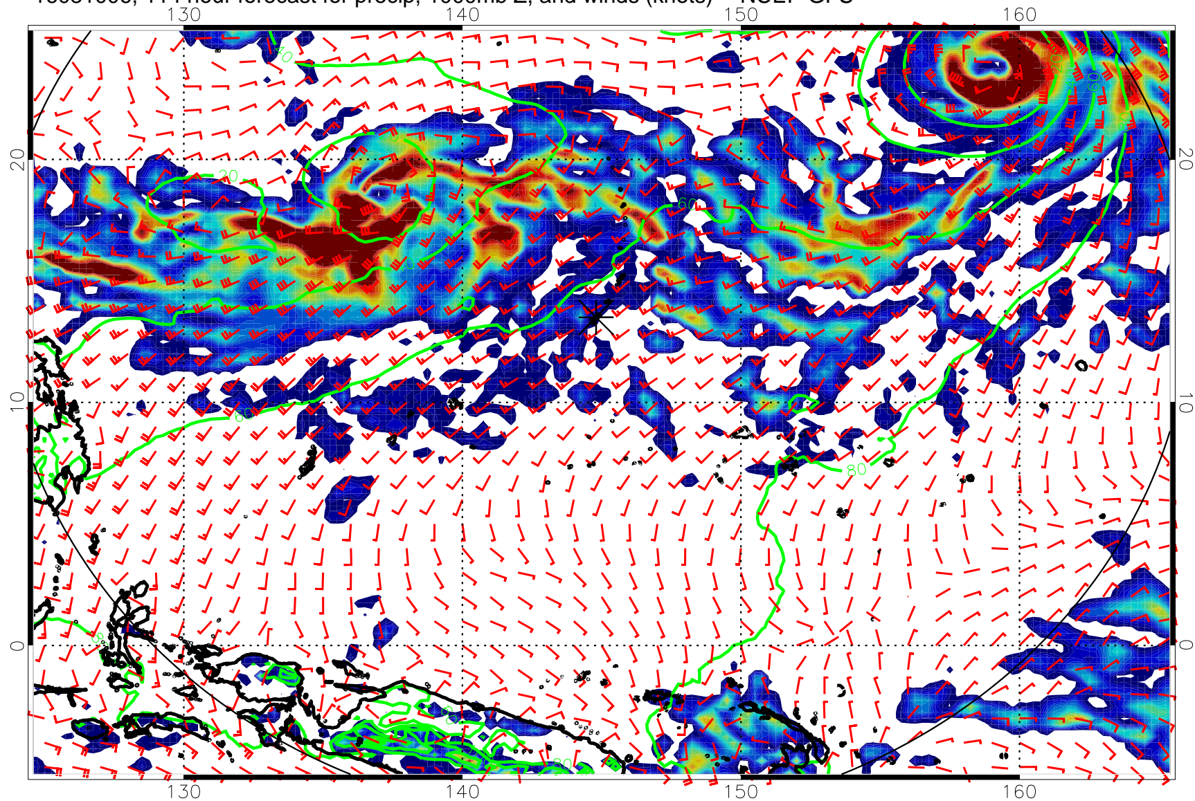
16081006, 114 hour forecast for precip, 1000mb Z, and winds (knots) -- NCEP GFS
