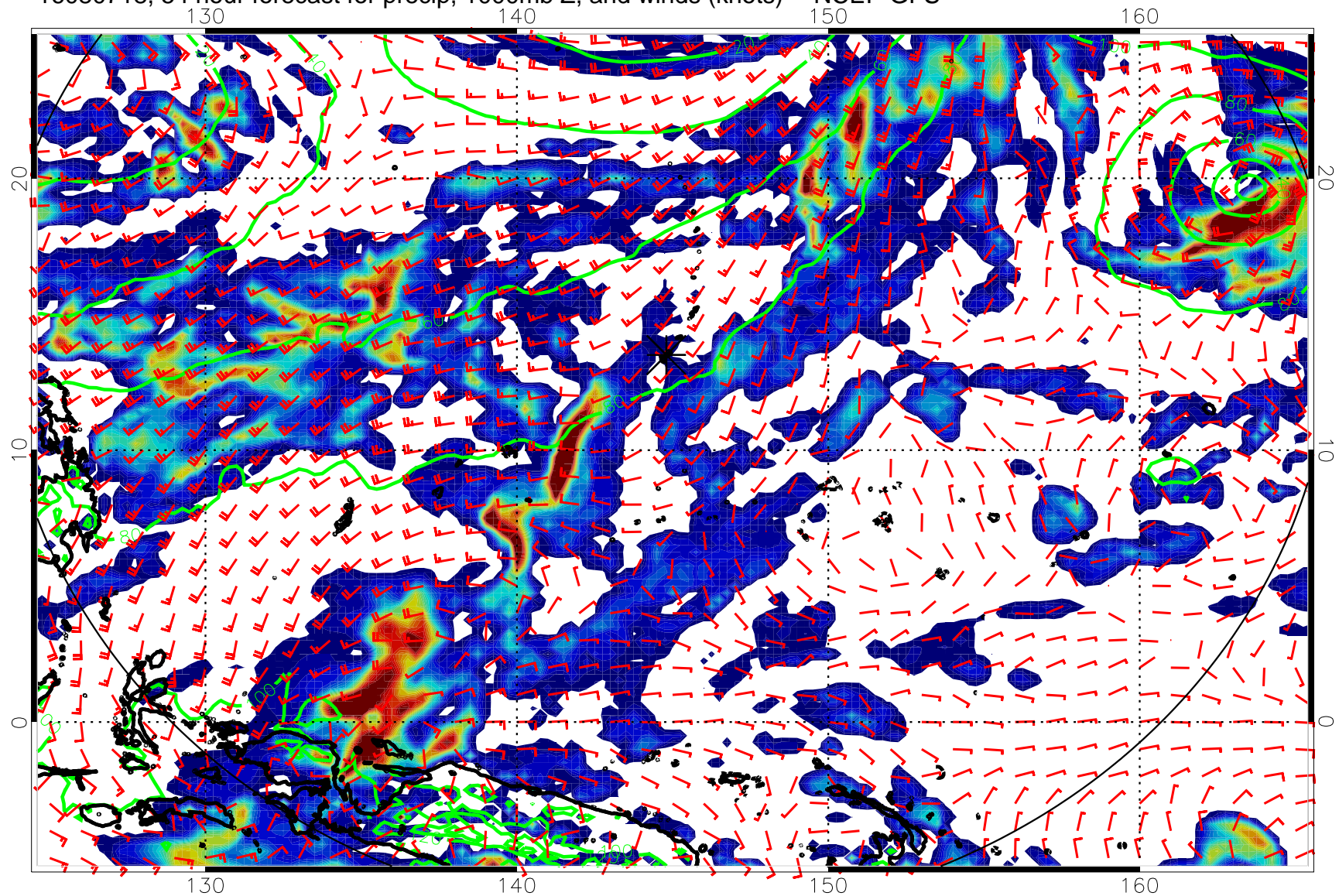
16080718, 54 hour forecast for precip, 1000mb Z, and winds (knots) -- NCEP GFS
