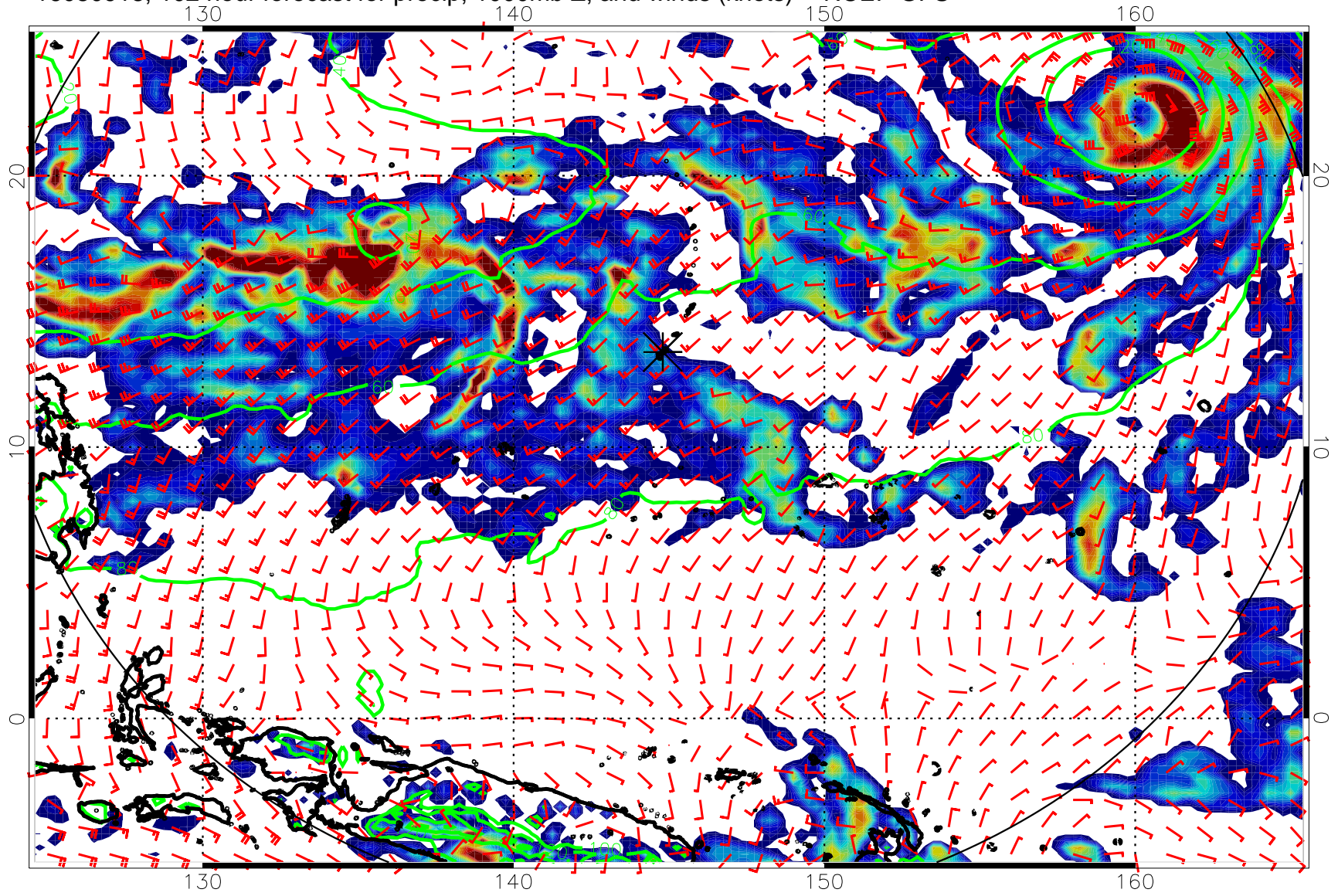
16080918, 102 hour forecast for precip, 1000mb Z, and winds (knots) -- NCEP GFS
