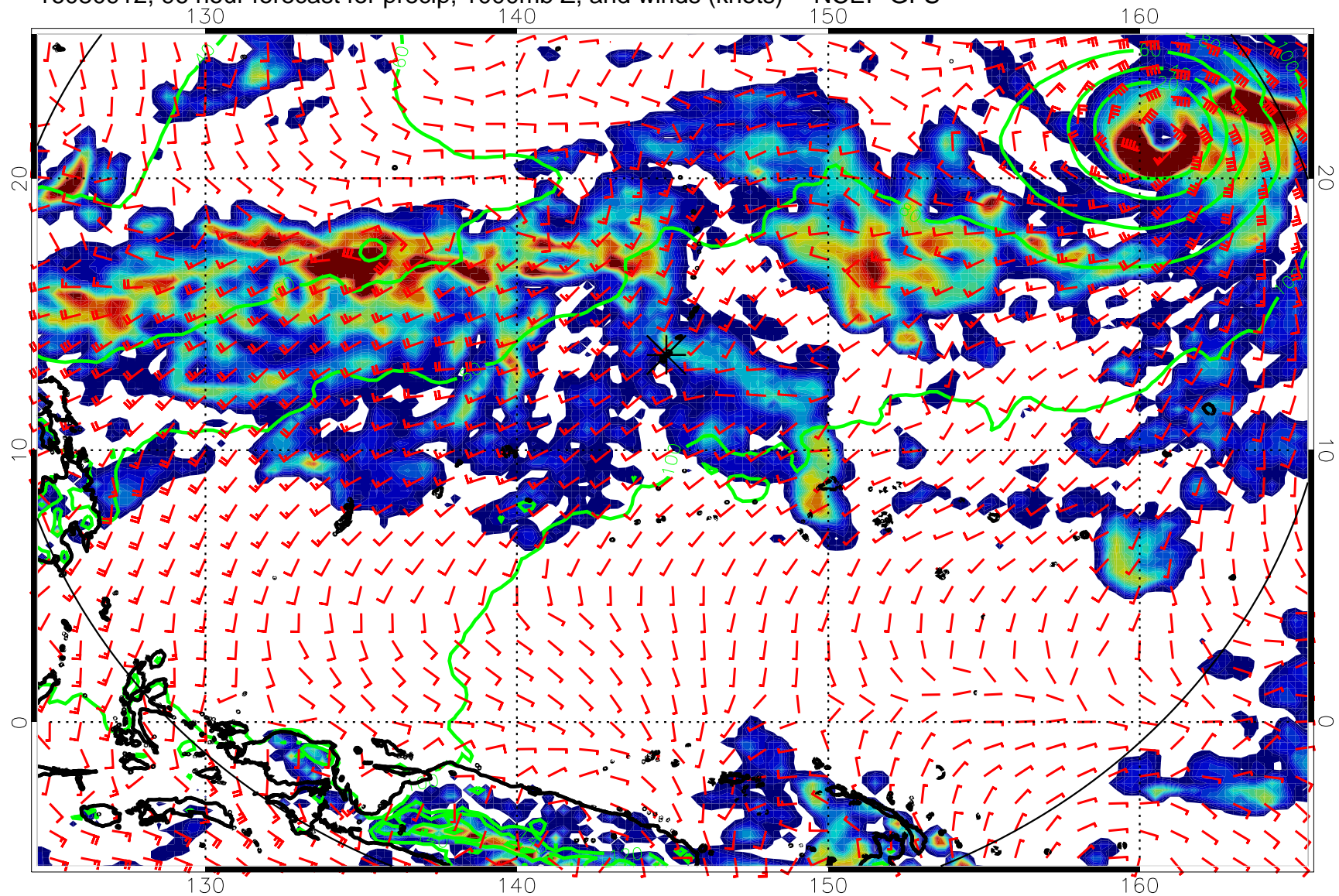
16080912, 96 hour forecast for precip, 1000mb Z, and winds (knots) -- NCEP GFS
