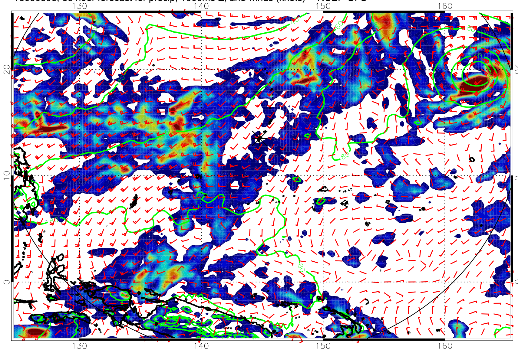
16080806, 66 hour forecast for precip, 1000mb Z, and winds (knots) -- NCEP GFS
