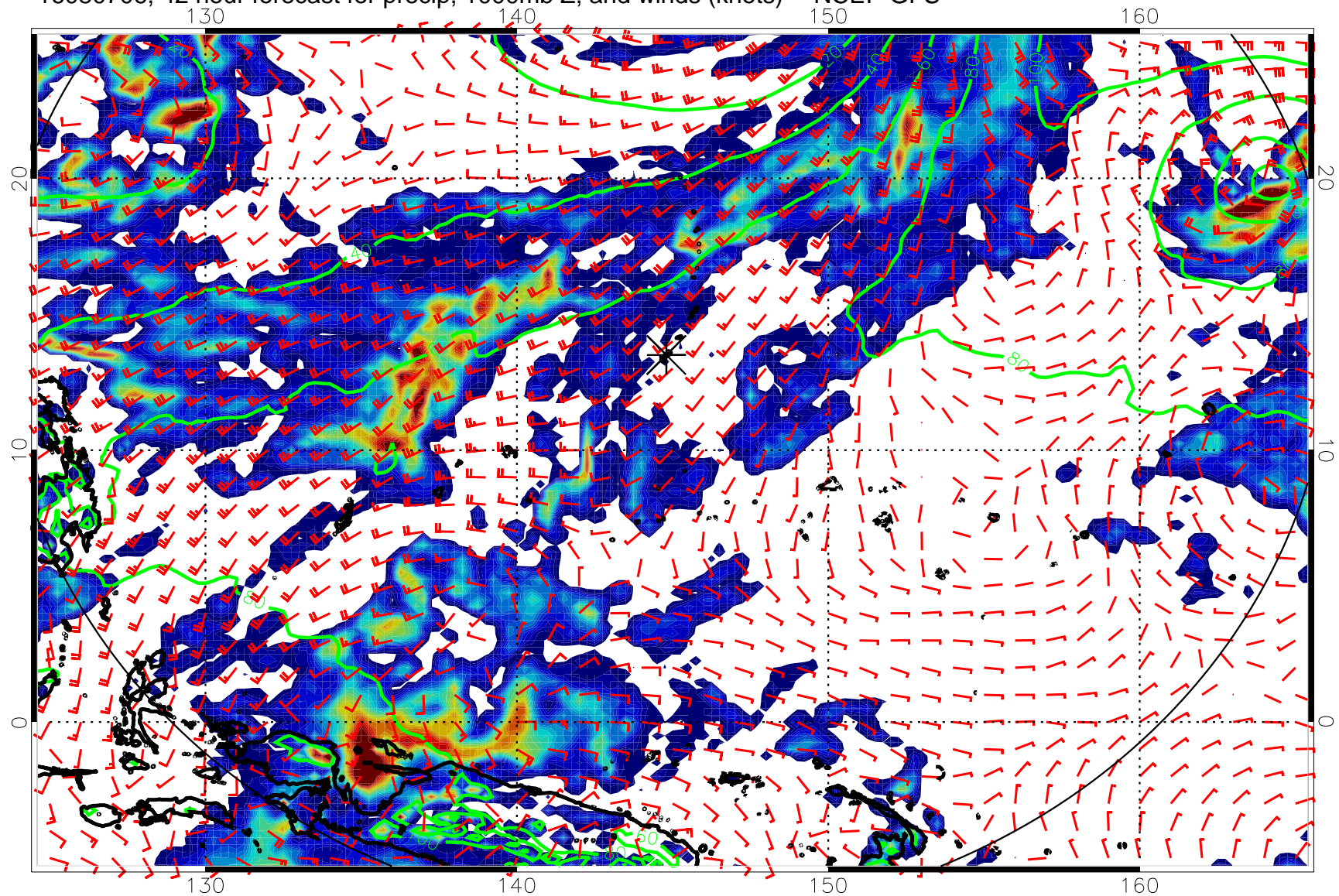
16080706, 42 hour forecast for precip, 1000mb Z, and winds (knots) -- NCEP GFS
