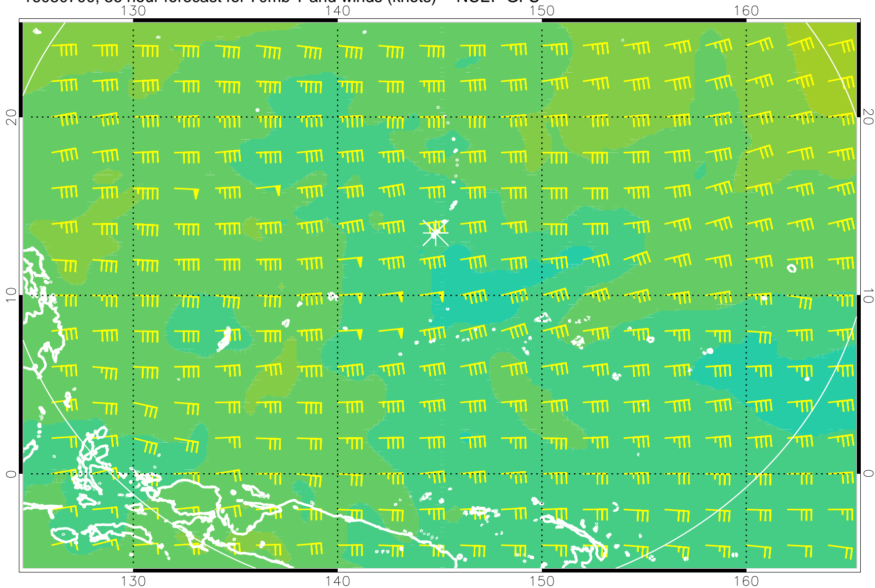
16080700, 36 hour forecast for 70mb T and winds (knots) -- NCEP GFS
