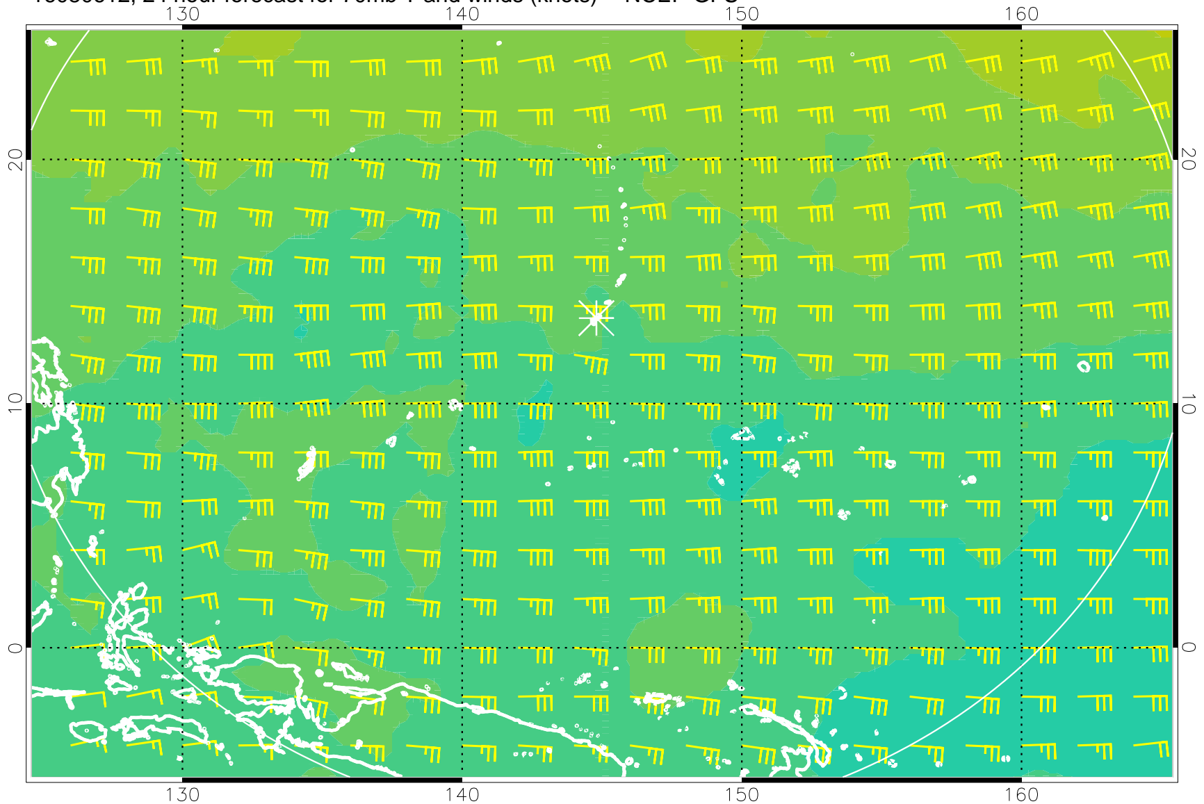
16080612, 24 hour forecast for 70mb T and winds (knots) -- NCEP GFS
