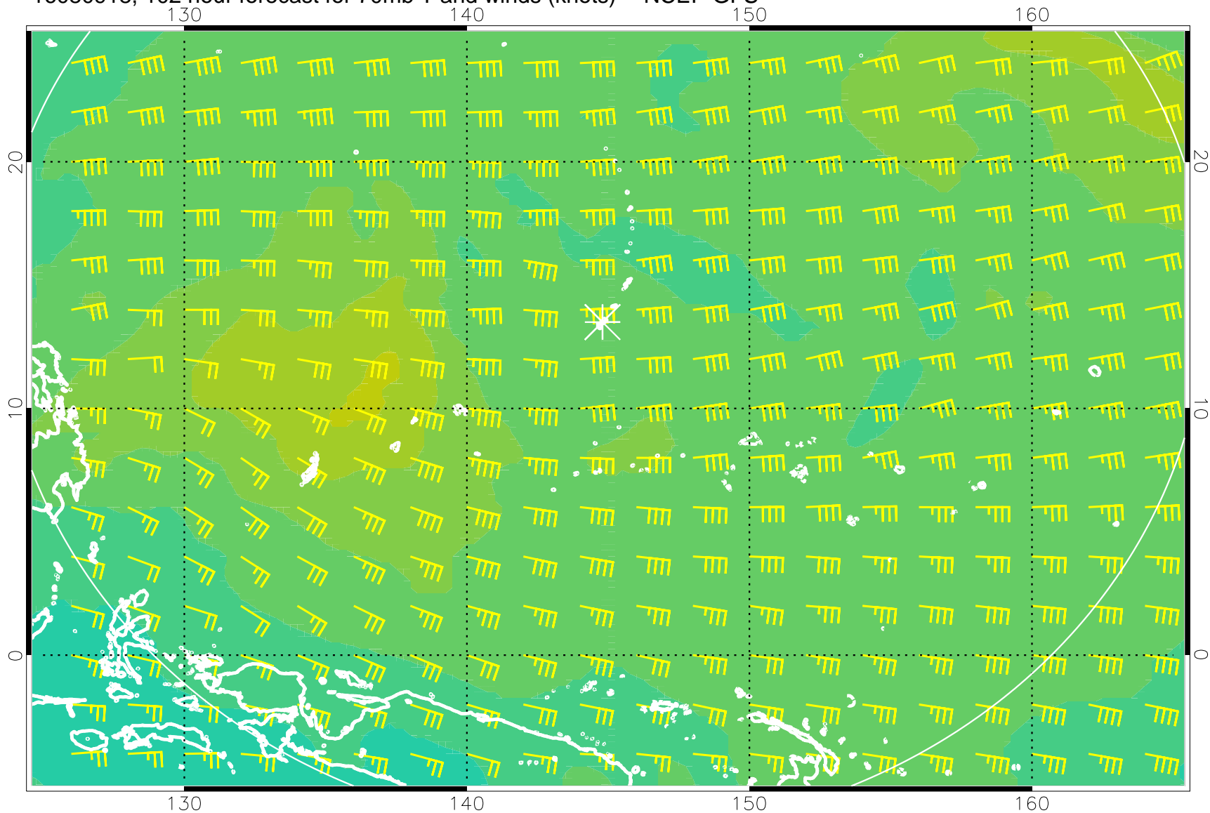
16080918, 102 hour forecast for 70mb T and winds (knots) -- NCEP GFS
