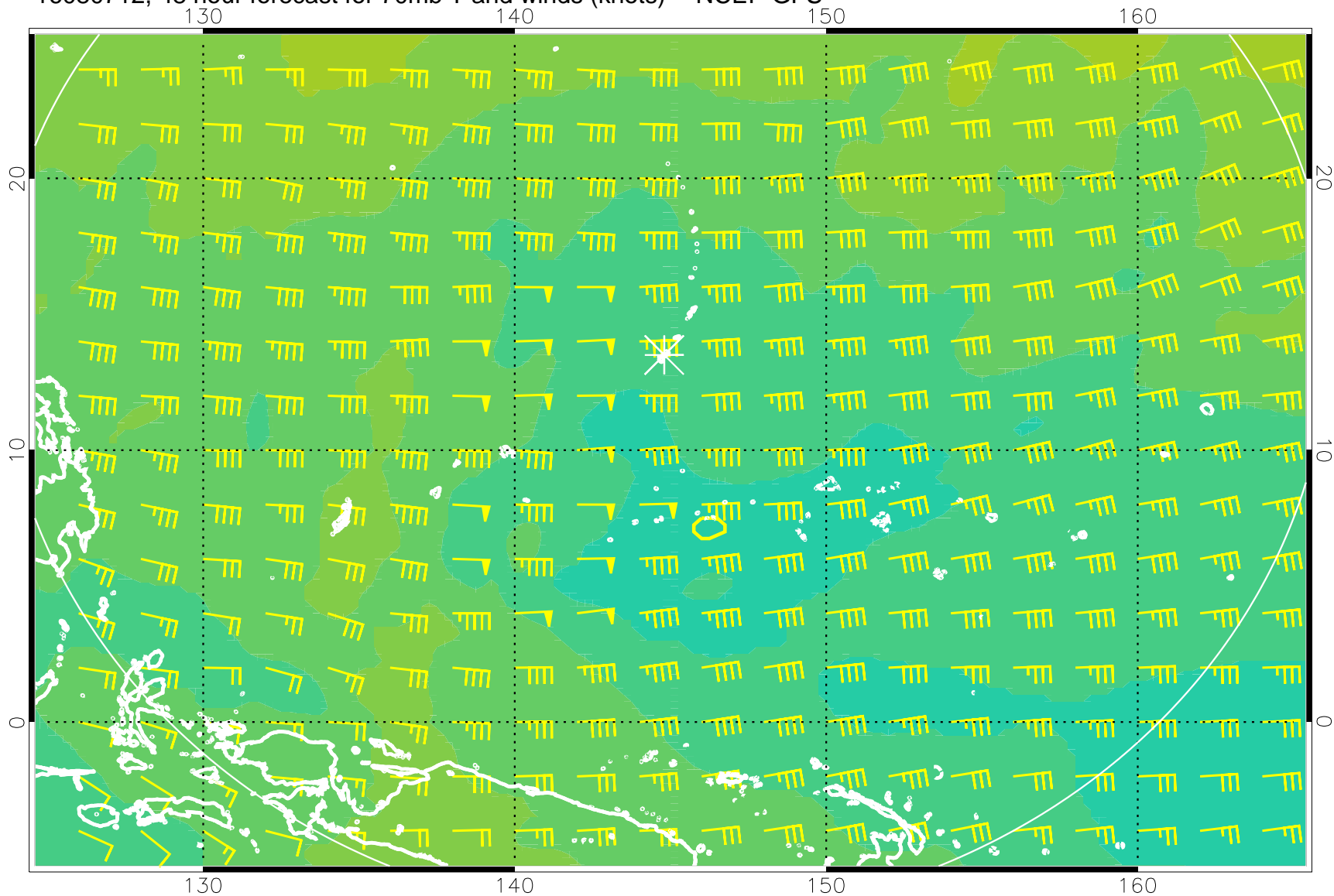
16080712, 48 hour forecast for 70mb T and winds (knots) -- NCEP GFS
