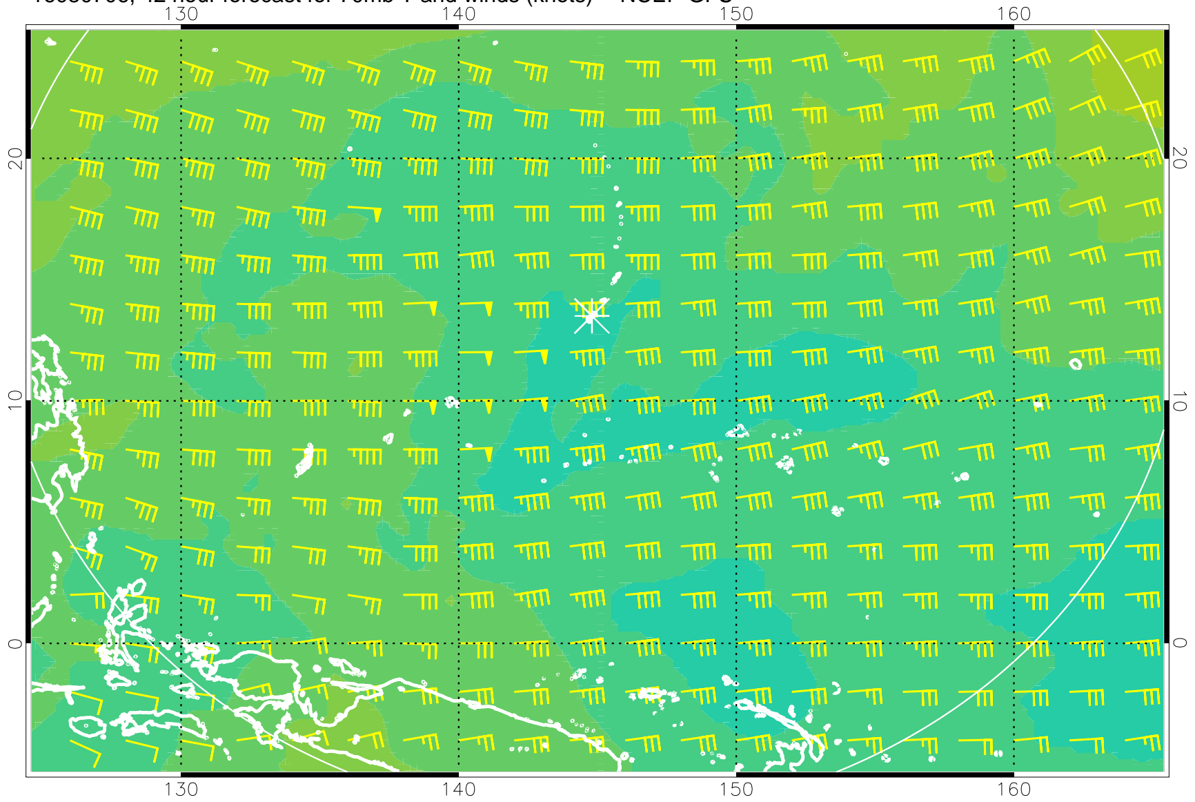
16080706, 42 hour forecast for 70mb T and winds (knots) -- NCEP GFS
