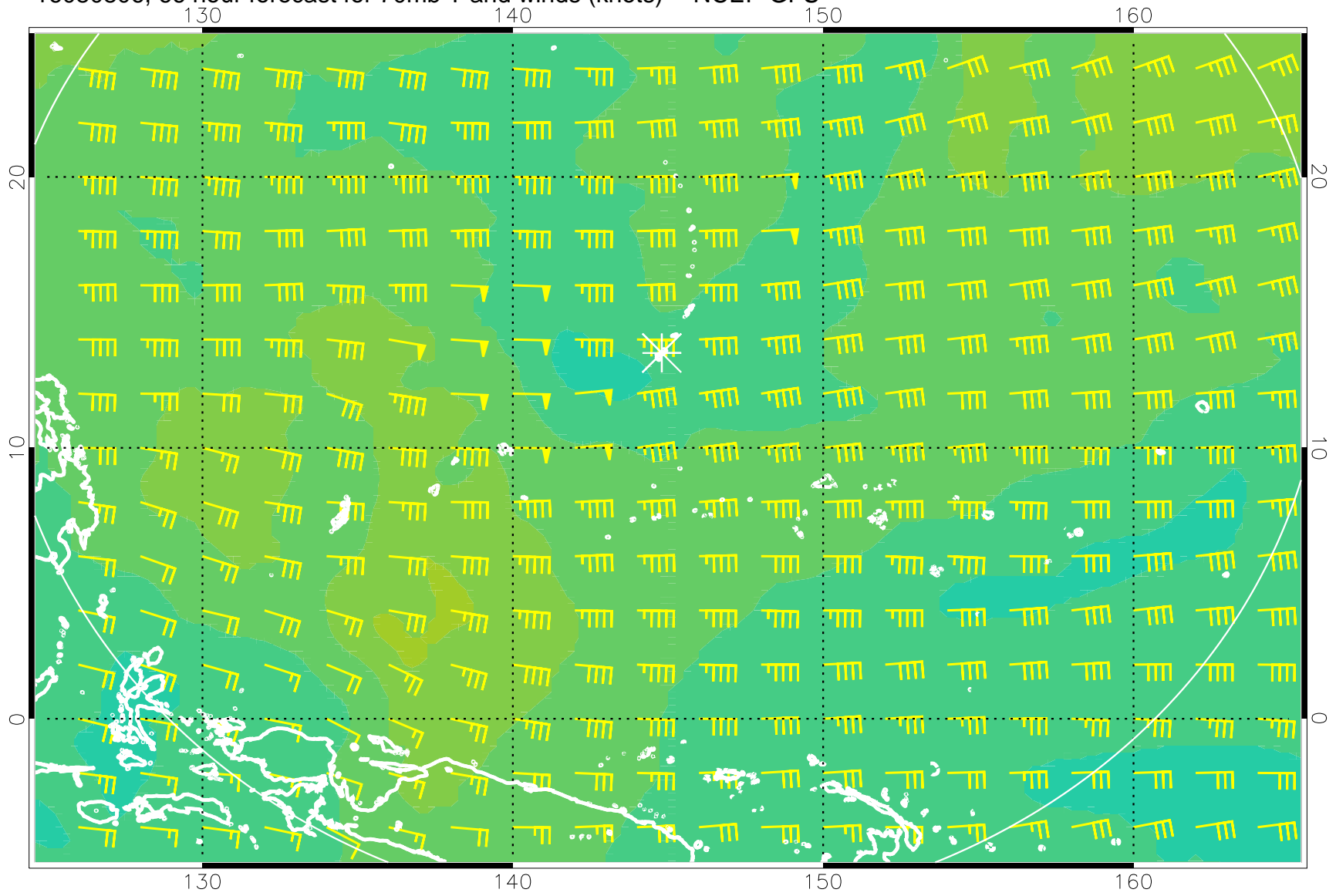
16080806, 66 hour forecast for 70mb T and winds (knots) -- NCEP GFS
