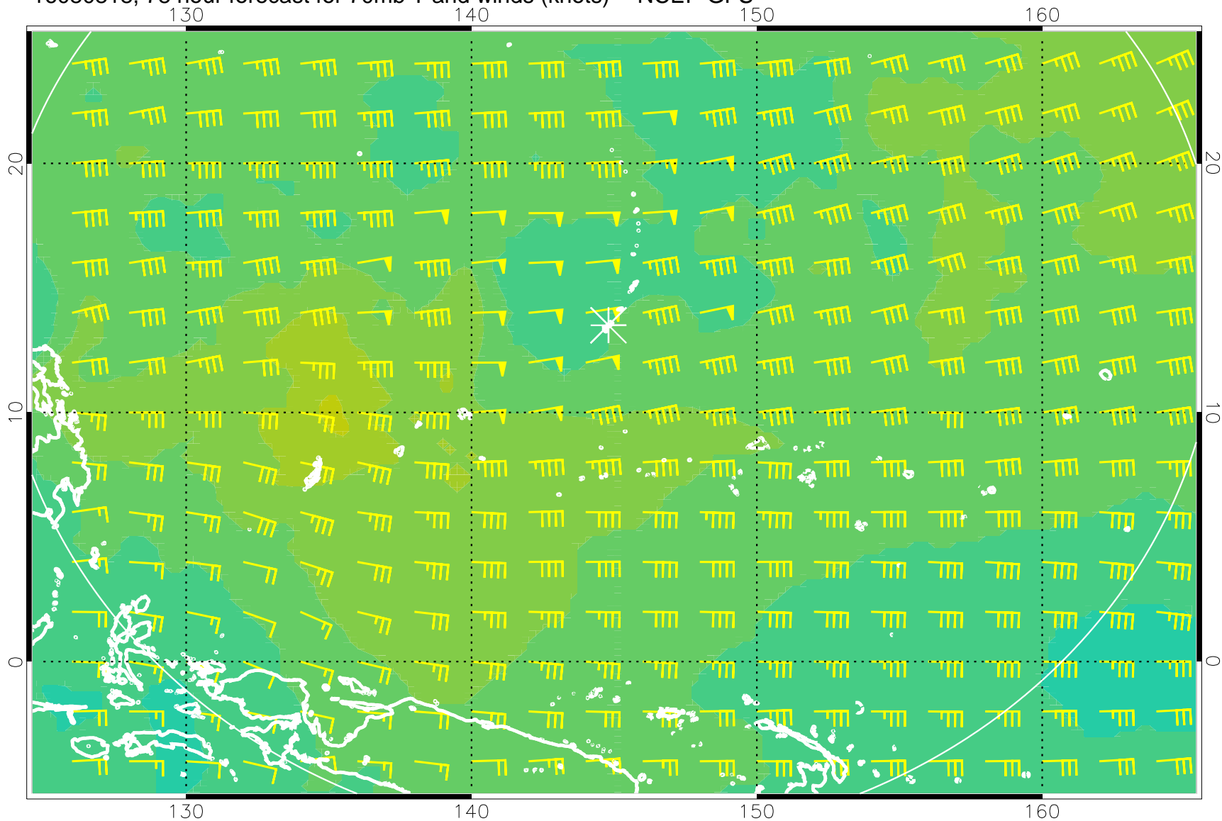
16080818, 78 hour forecast for 70mb T and winds (knots) -- NCEP GFS
