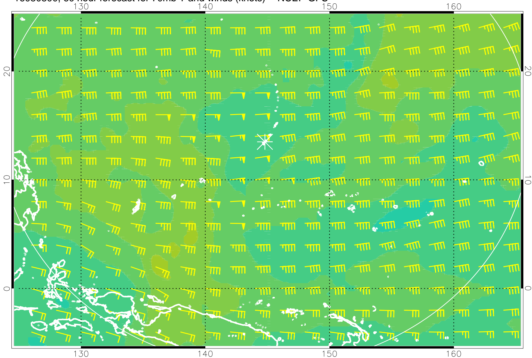
16080800, 60 hour forecast for 70mb T and winds (knots) -- NCEP GFS
