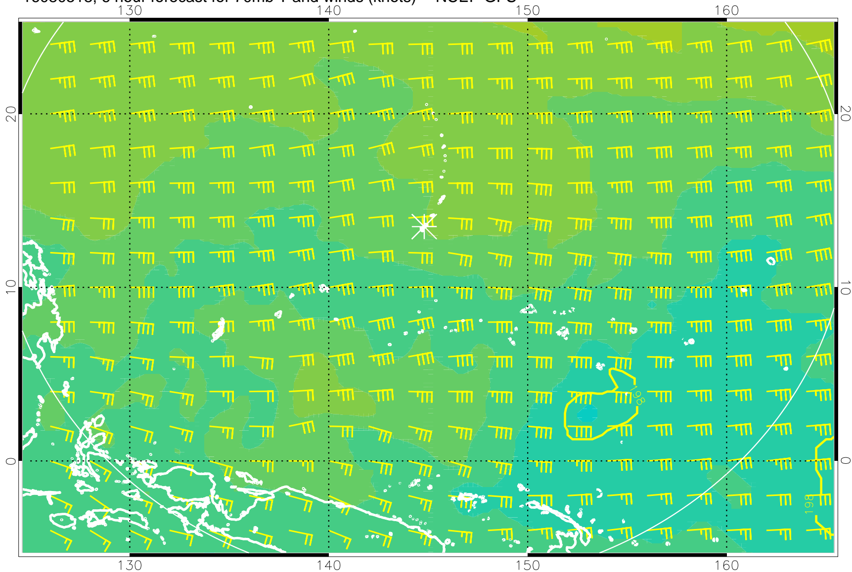
16080518, 6 hour forecast for 70mb T and winds (knots) -- NCEP GFS
