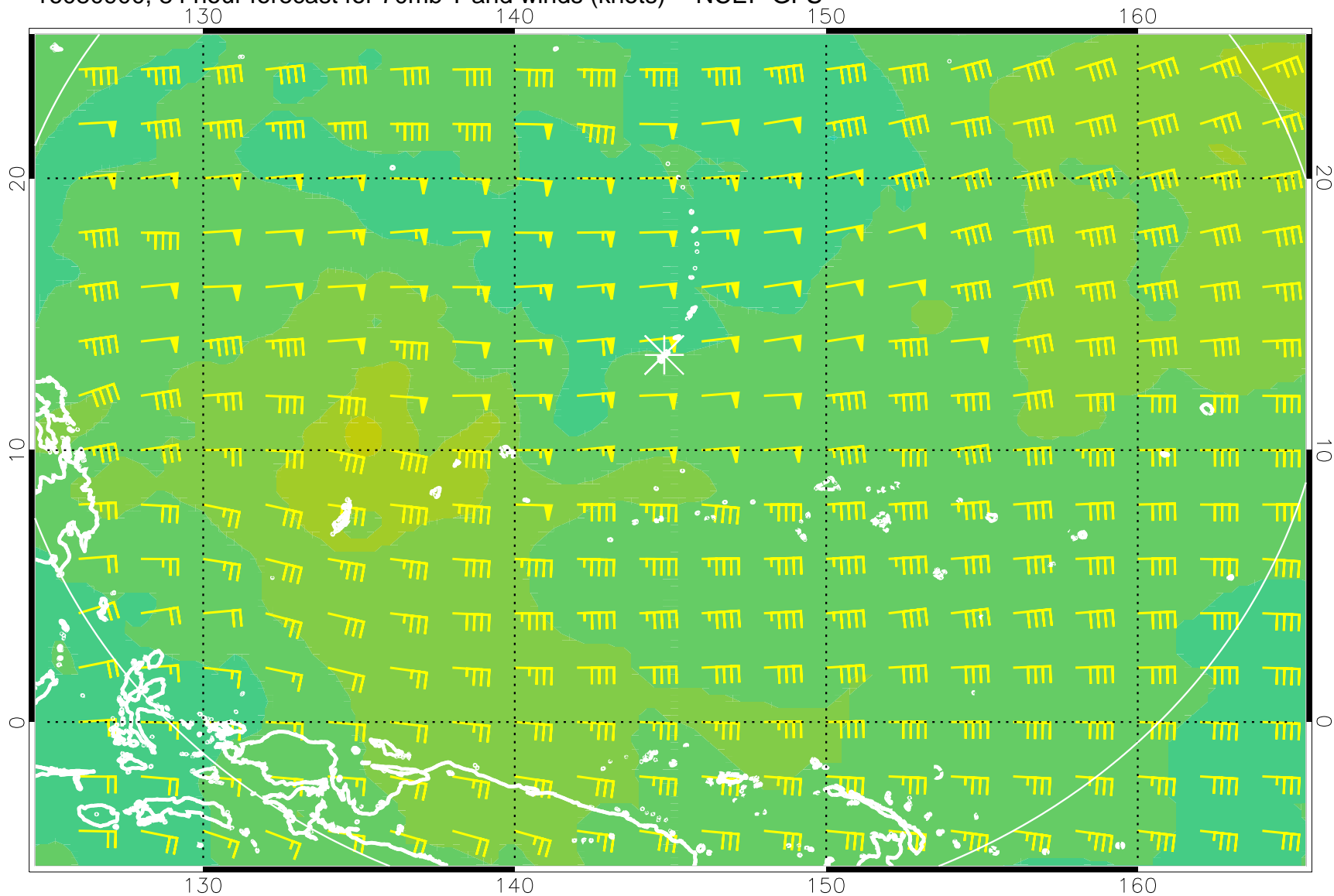
16080900, 84 hour forecast for 70mb T and winds (knots) -- NCEP GFS
