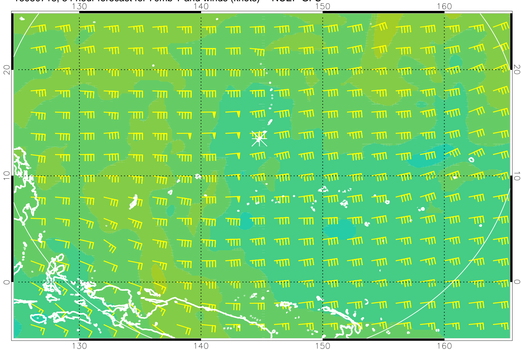
16080718, 54 hour forecast for 70mb T and winds (knots) -- NCEP GFS
