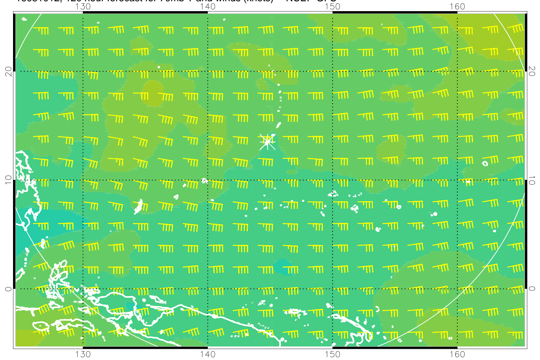
16081012, 120 hour forecast for 70mb T and winds (knots) -- NCEP GFS
