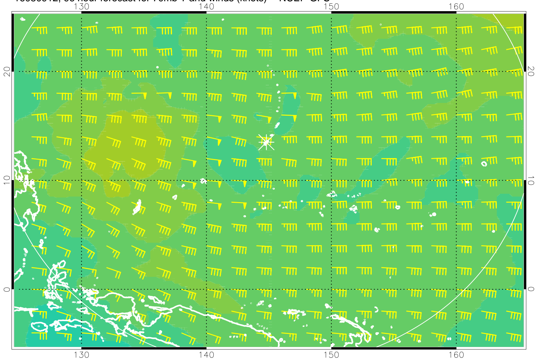
16080912, 96 hour forecast for 70mb T and winds (knots) -- NCEP GFS
