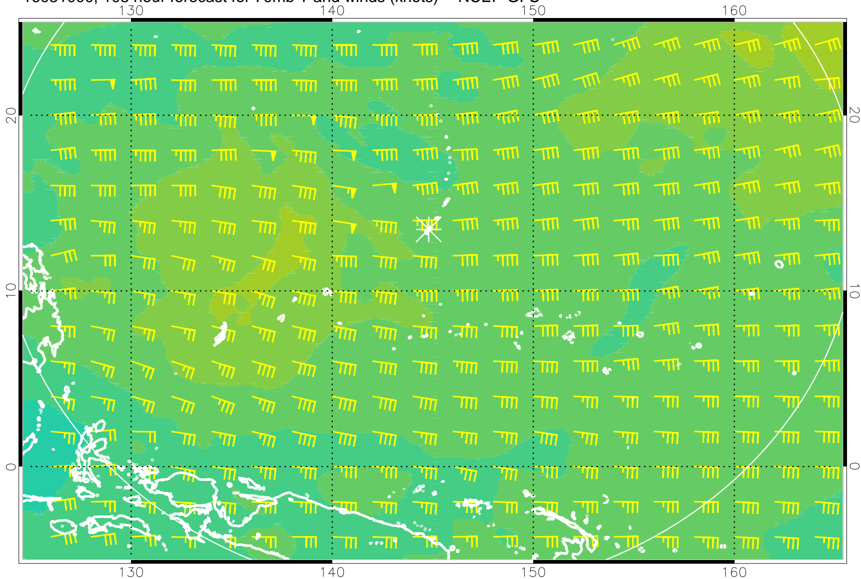
16081000, 108 hour forecast for 70mb T and winds (knots) -- NCEP GFS
