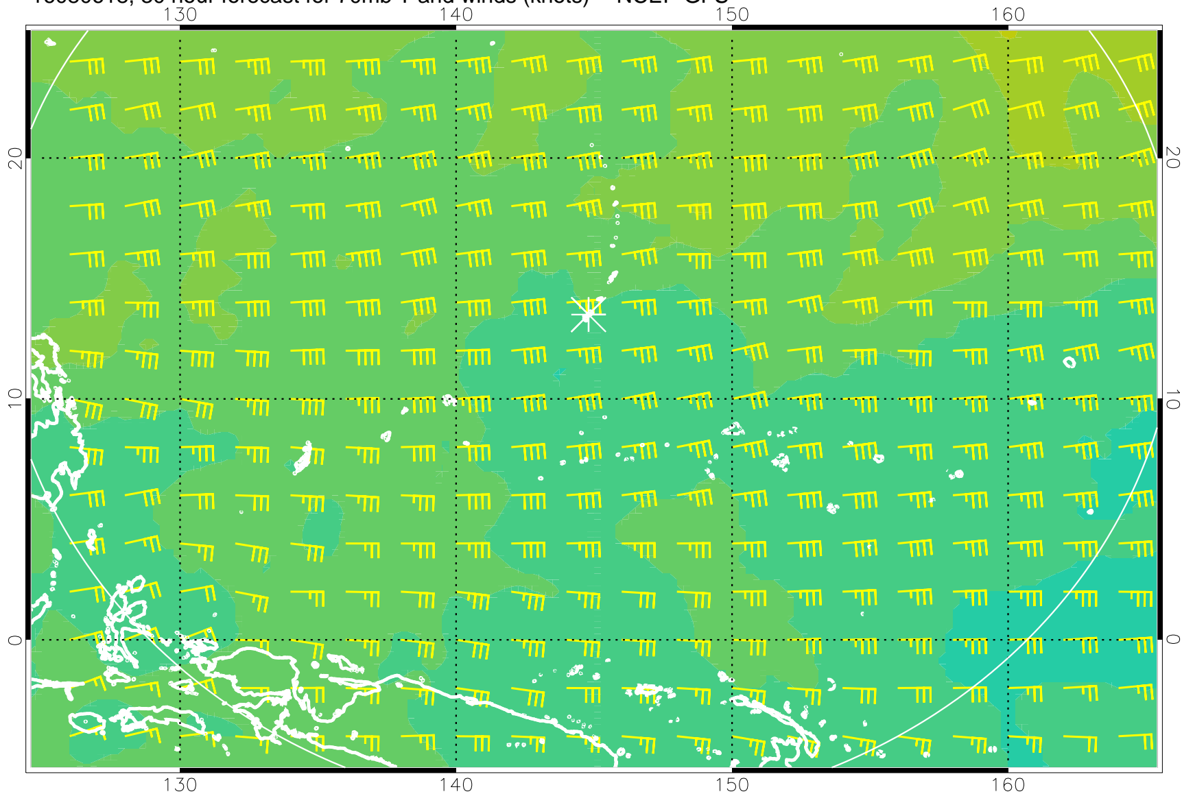
16080618, 30 hour forecast for 70mb T and winds (knots) -- NCEP GFS
