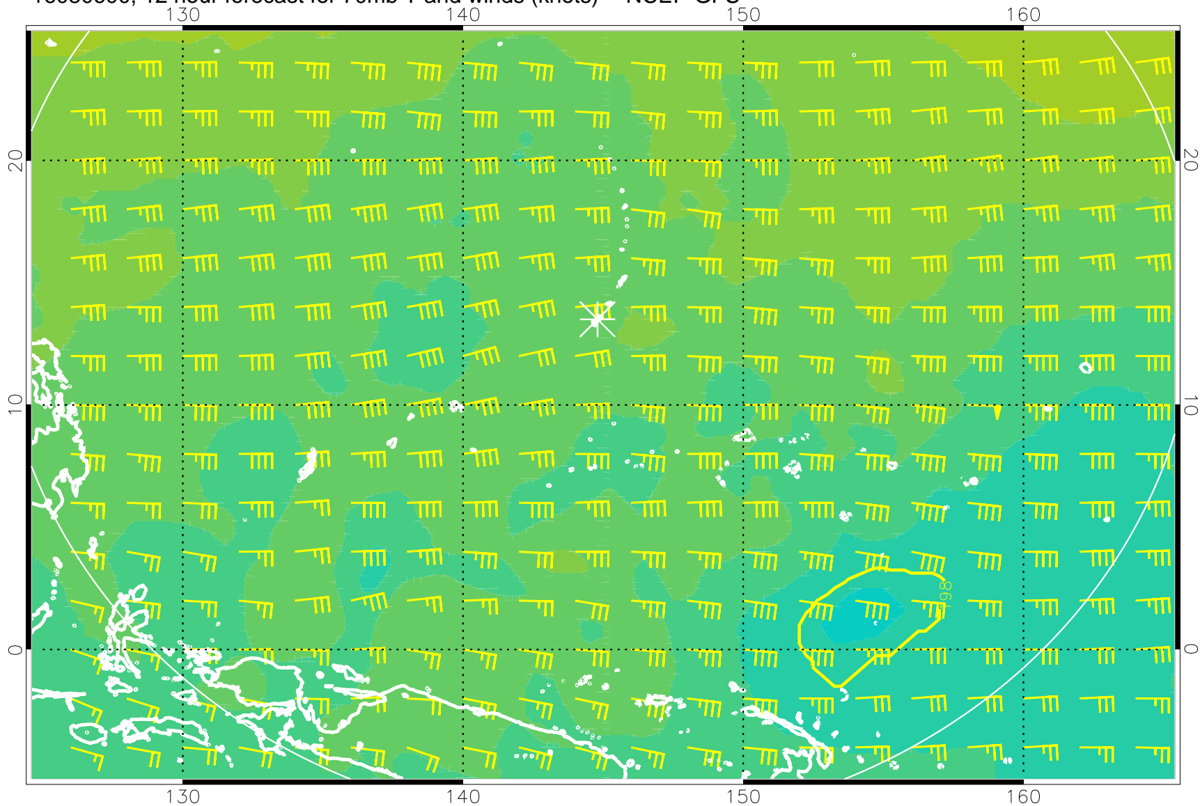
16080600, 12 hour forecast for 70mb T and winds (knots) -- NCEP GFS
