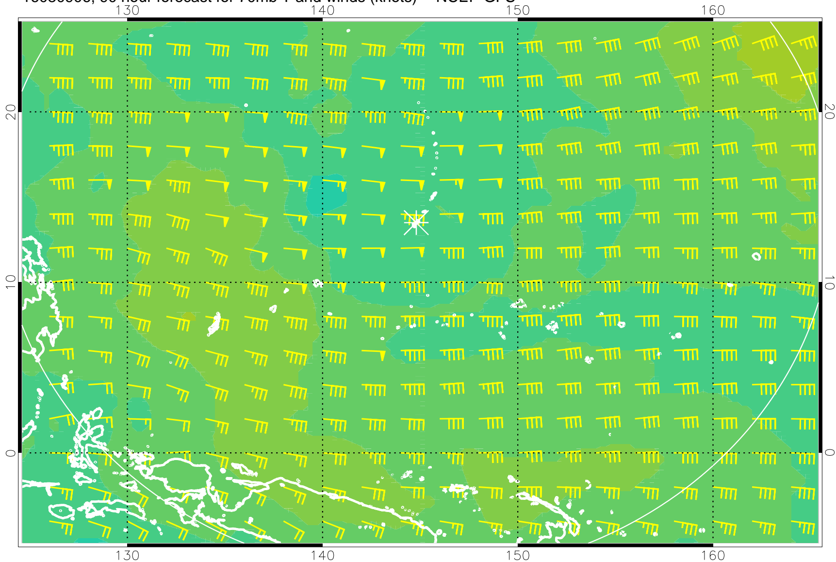
16080906, 90 hour forecast for 70mb T and winds (knots) -- NCEP GFS
