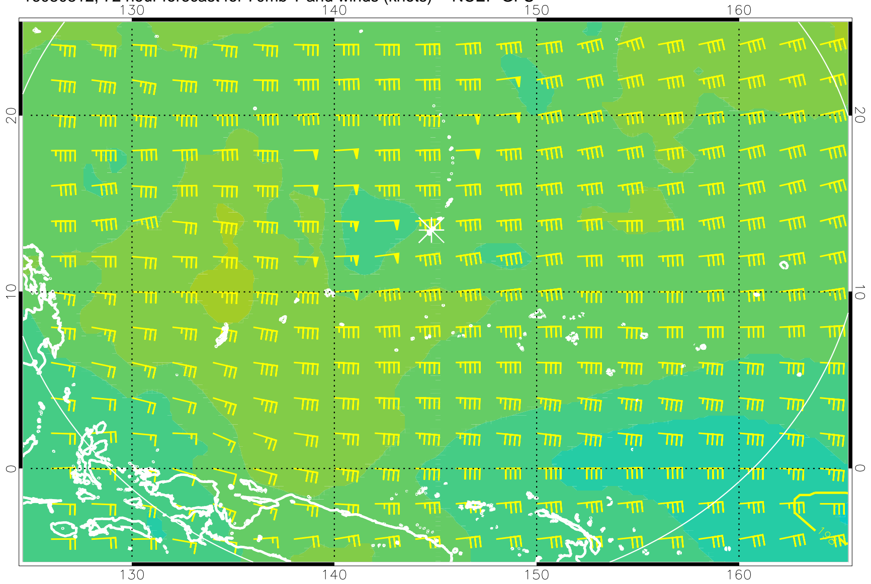
16080812, 72 hour forecast for 70mb T and winds (knots) -- NCEP GFS
