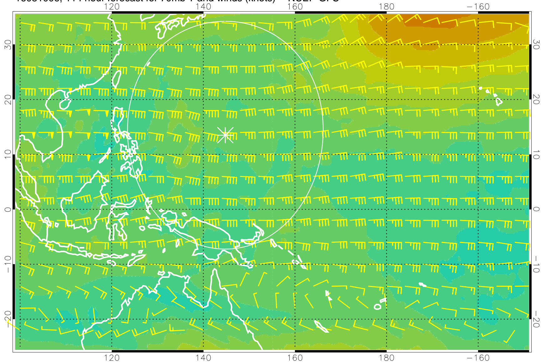
16081006, 114 hour forecast for 70mb T and winds (knots) -- NCEP GFS
