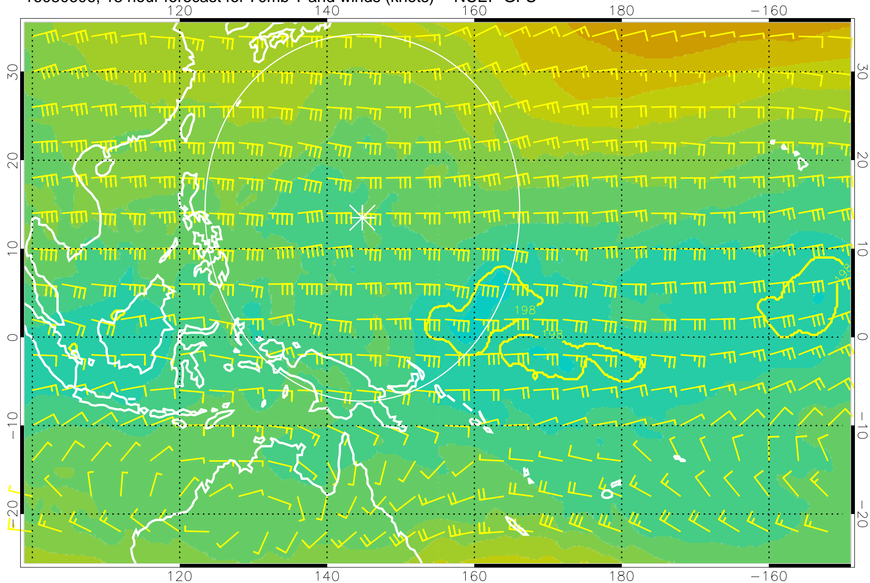
16080606, 18 hour forecast for 70mb T and winds (knots) -- NCEP GFS
