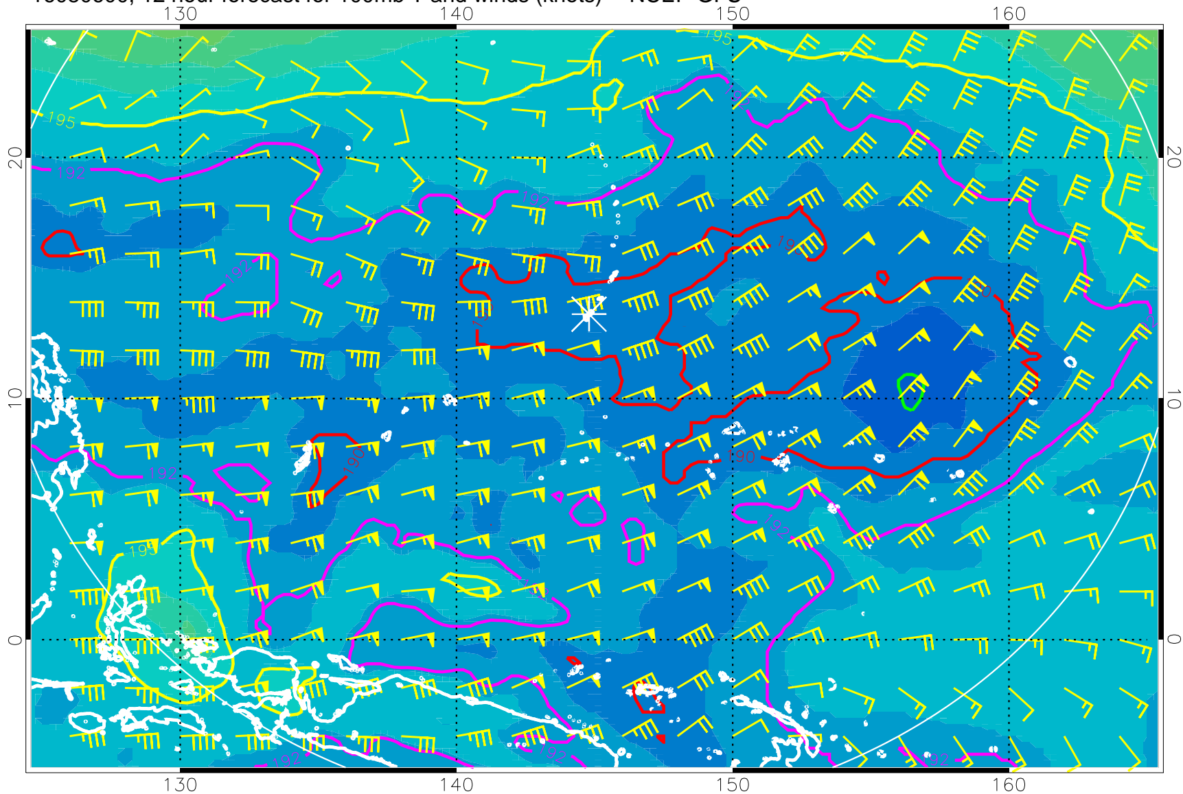
16080600, 12 hour forecast for 100mb T and winds (knots) -- NCEP GFS
