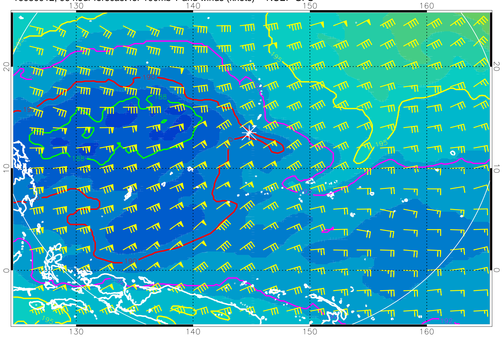
16080912, 96 hour forecast for 100mb T and winds (knots) -- NCEP GFS
