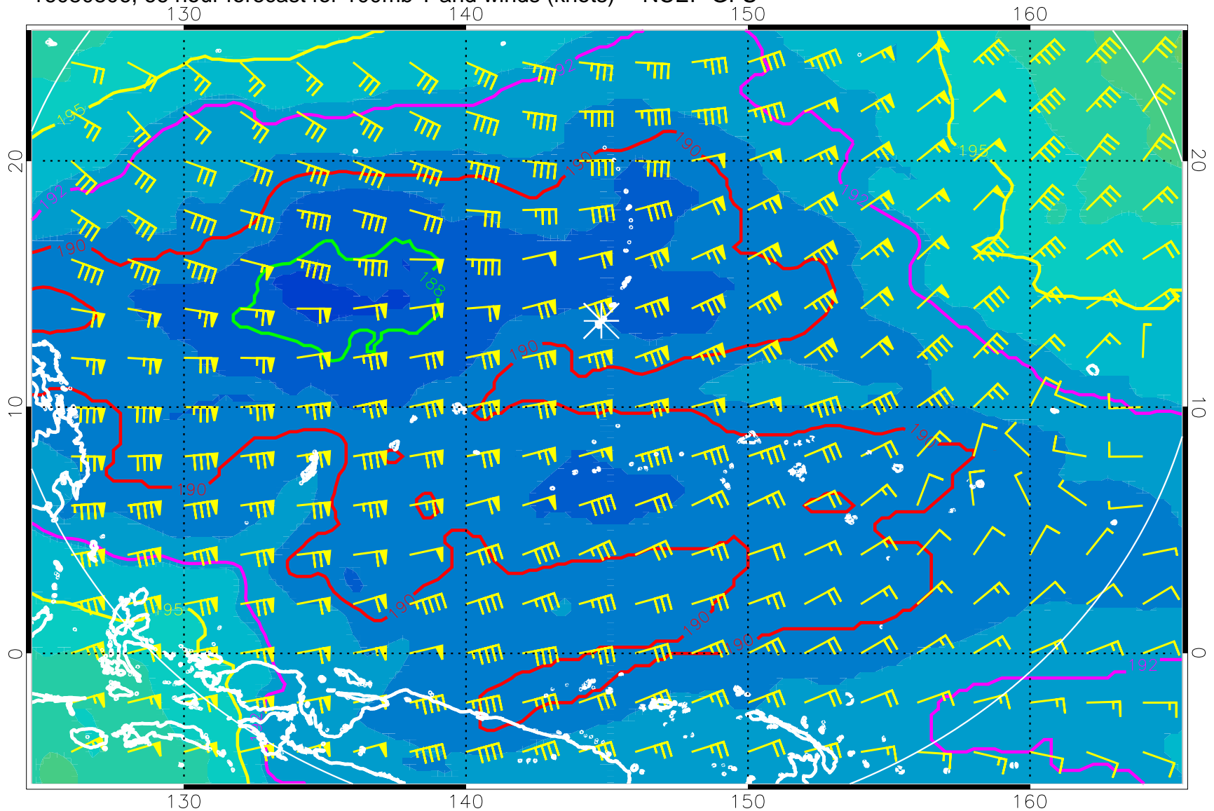
16080806, 66 hour forecast for 100mb T and winds (knots) -- NCEP GFS
