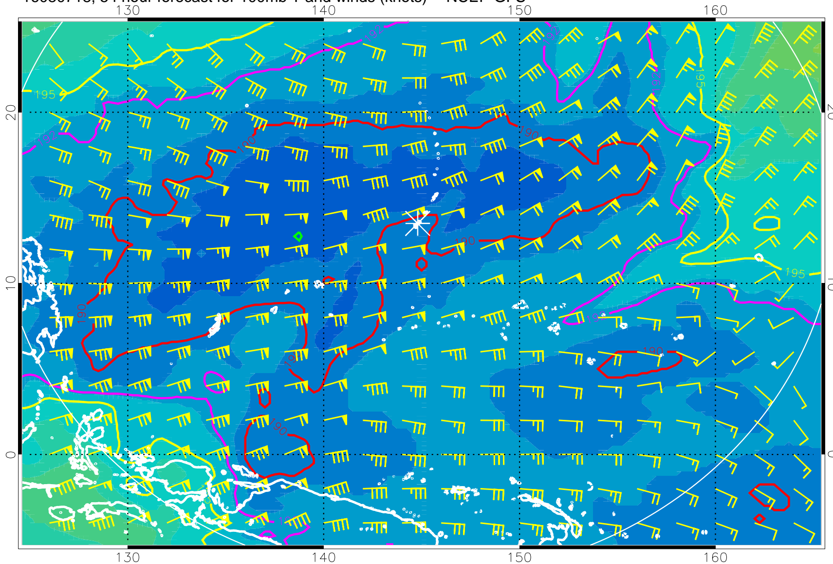
16080718, 54 hour forecast for 100mb T and winds (knots) -- NCEP GFS
