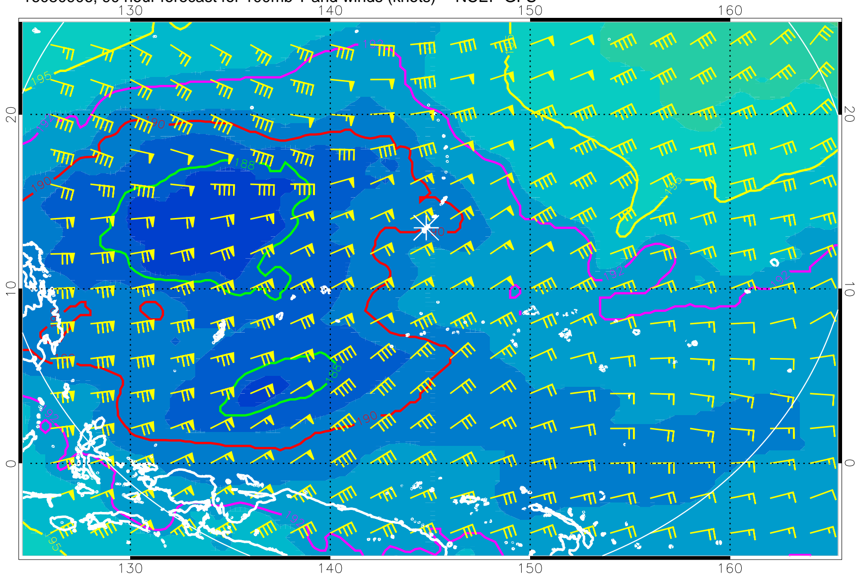
16080906, 90 hour forecast for 100mb T and winds (knots) -- NCEP GFS
