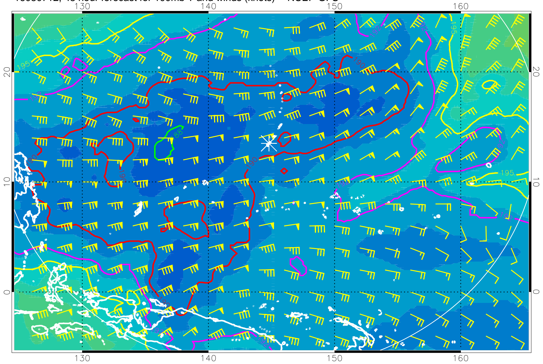
16080712, 48 hour forecast for 100mb T and winds (knots) -- NCEP GFS
