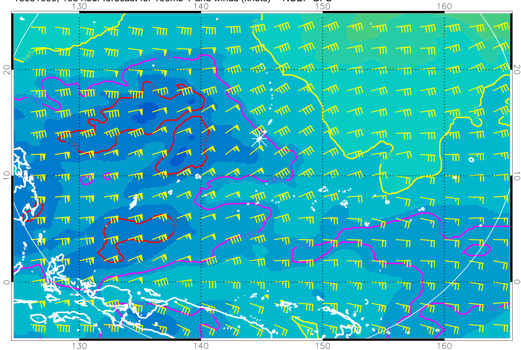
16081000, 108 hour forecast for 100mb T and winds (knots) -- NCEP GFS
