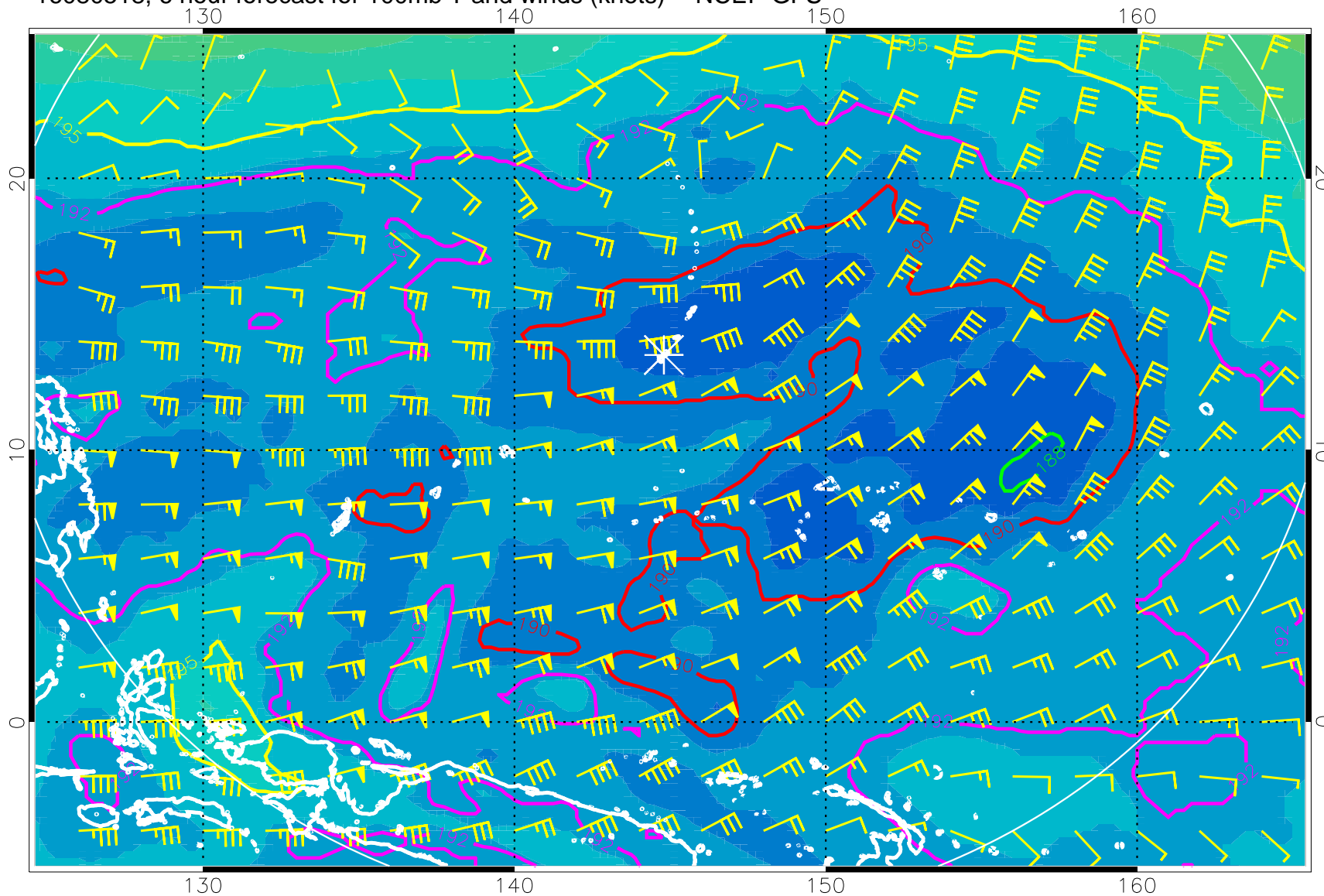
16080518, 6 hour forecast for 100mb T and winds (knots) -- NCEP GFS
