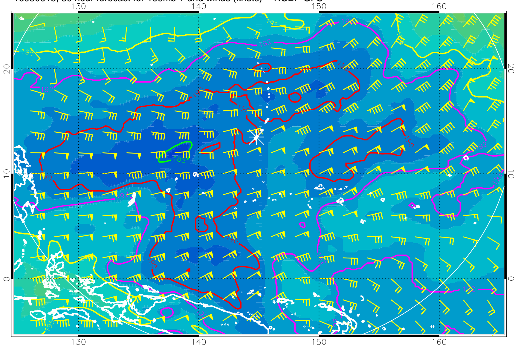
16080618, 30 hour forecast for 100mb T and winds (knots) -- NCEP GFS
