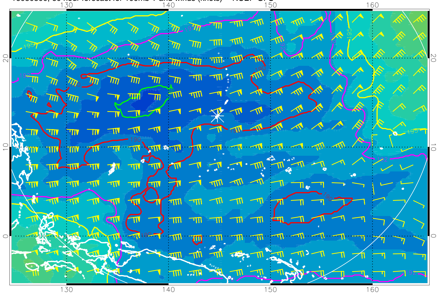
16080800, 60 hour forecast for 100mb T and winds (knots) -- NCEP GFS
