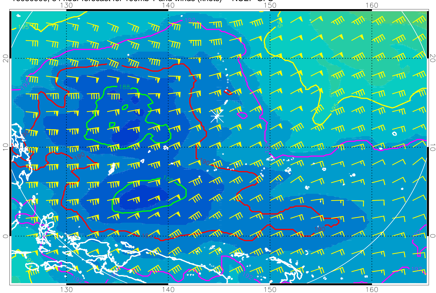
16080900, 84 hour forecast for 100mb T and winds (knots) -- NCEP GFS
