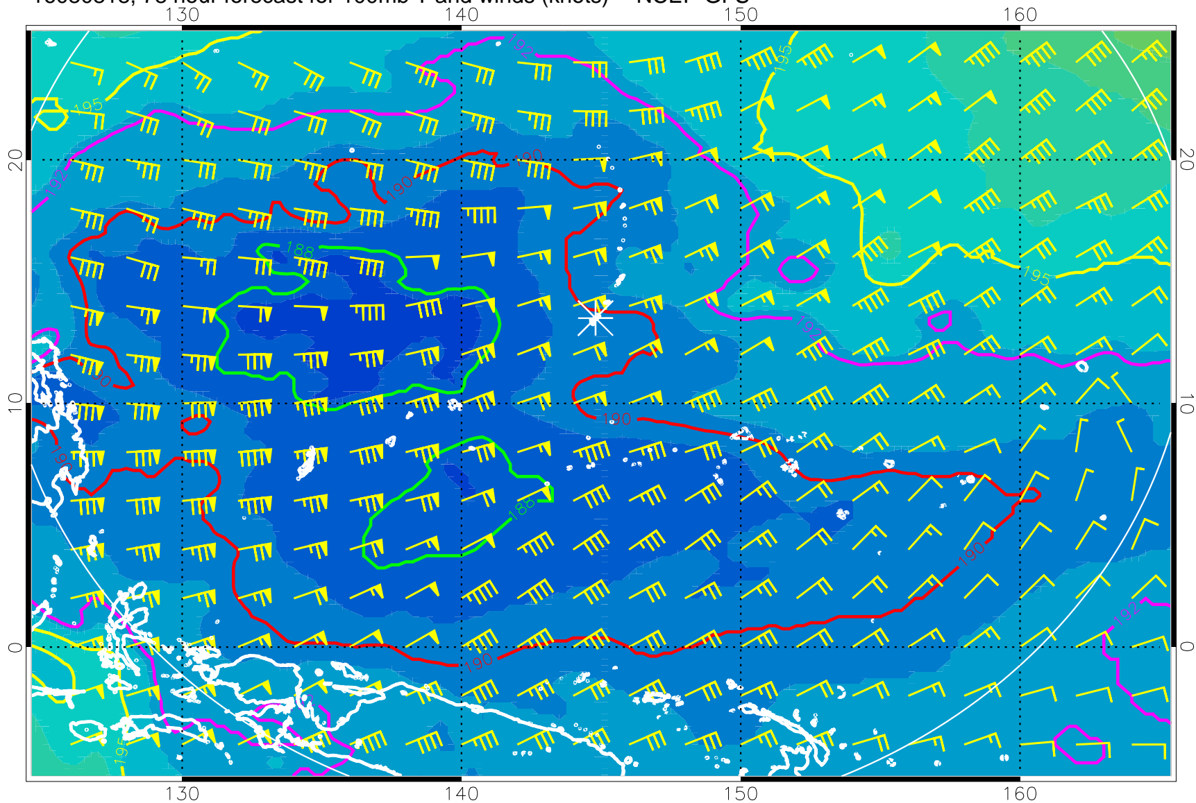
16080818, 78 hour forecast for 100mb T and winds (knots) -- NCEP GFS
