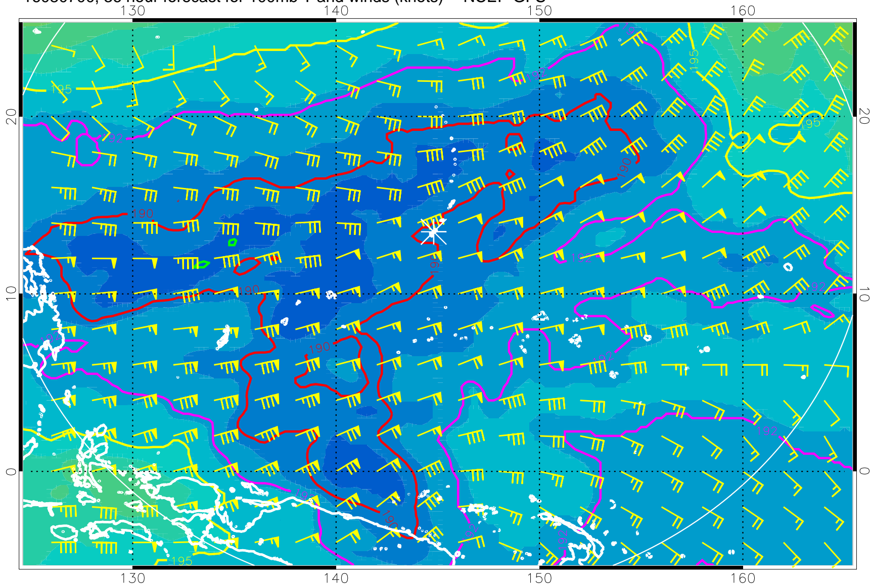
16080700, 36 hour forecast for 100mb T and winds (knots) -- NCEP GFS
