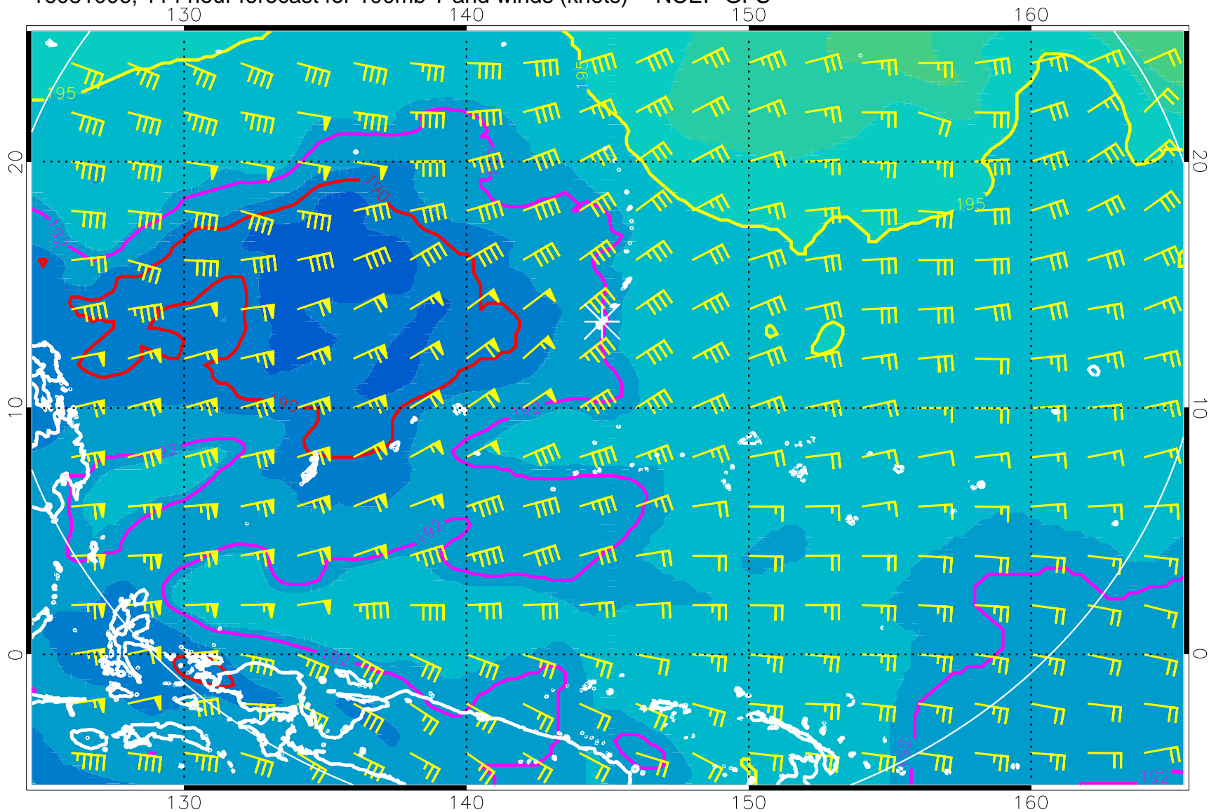
16081006, 114 hour forecast for 100mb T and winds (knots) -- NCEP GFS
