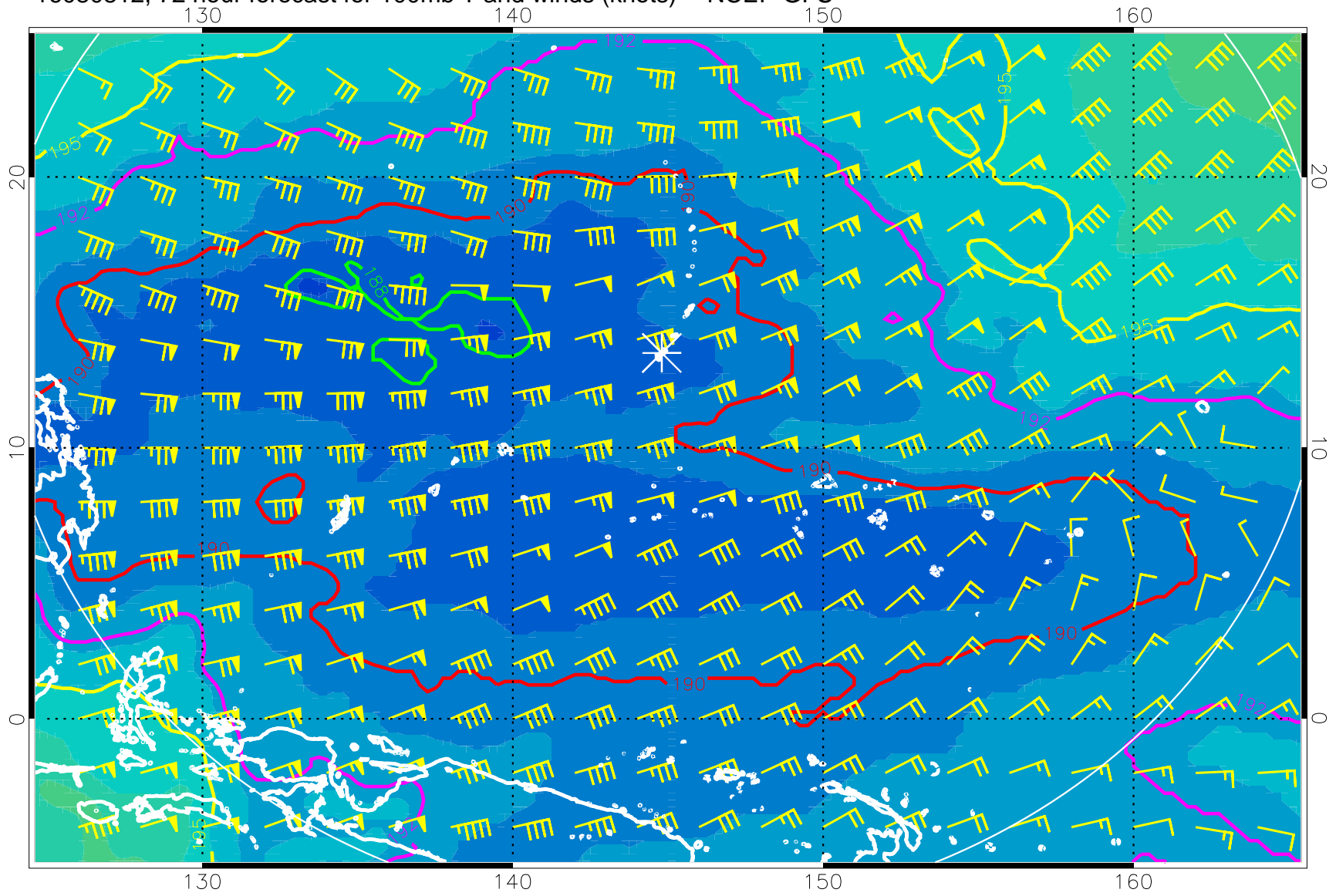
16080812, 72 hour forecast for 100mb T and winds (knots) -- NCEP GFS
