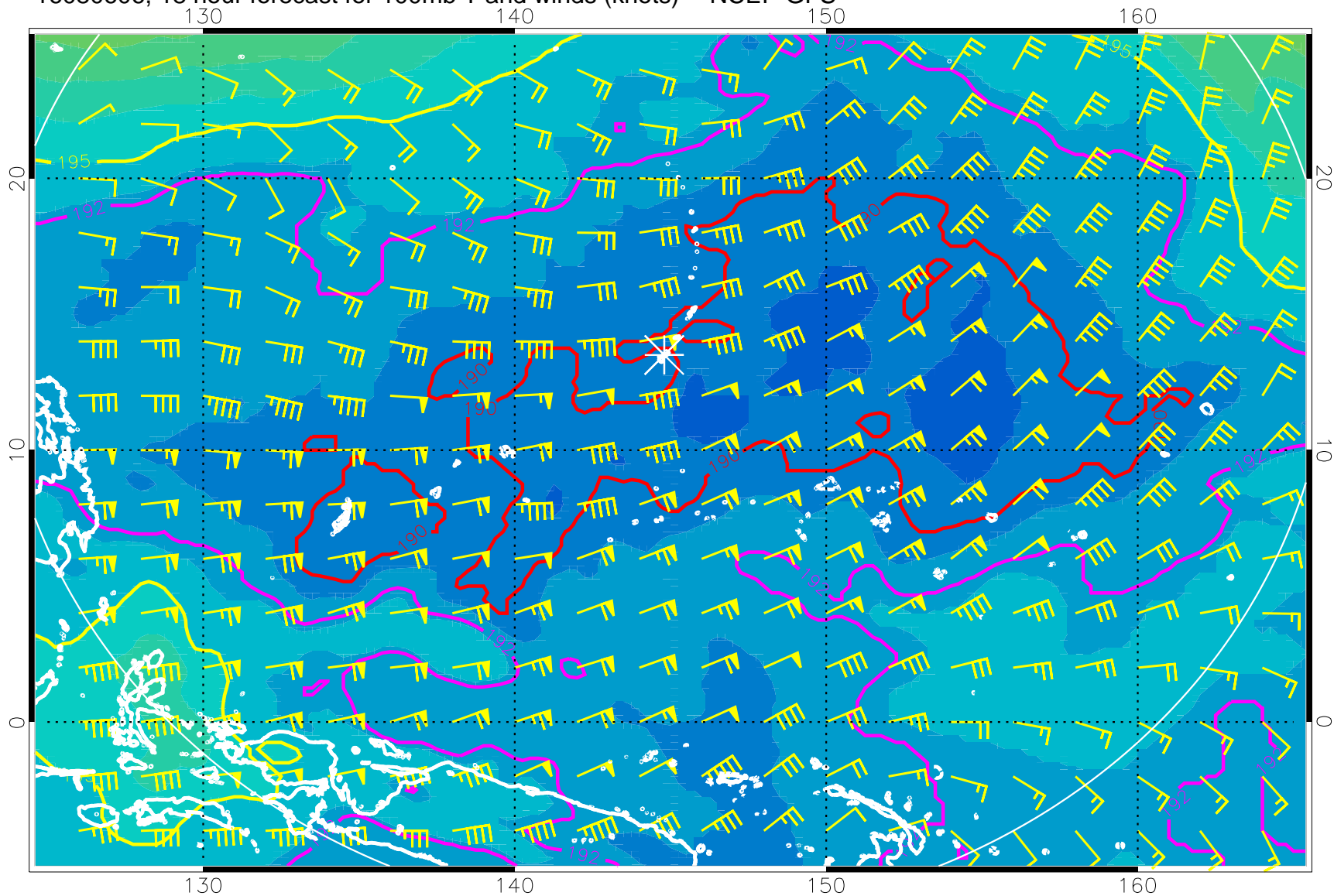
16080606, 18 hour forecast for 100mb T and winds (knots) -- NCEP GFS
