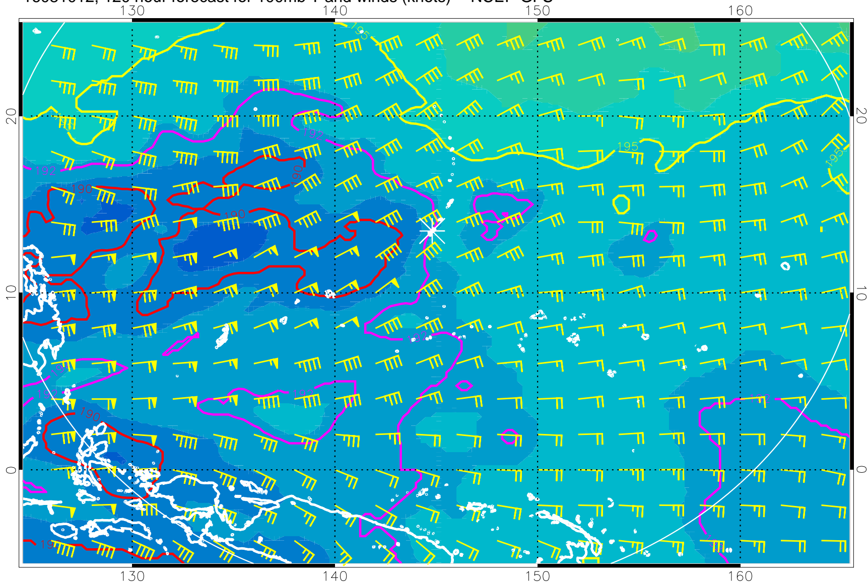
16081012, 120 hour forecast for 100mb T and winds (knots) -- NCEP GFS
