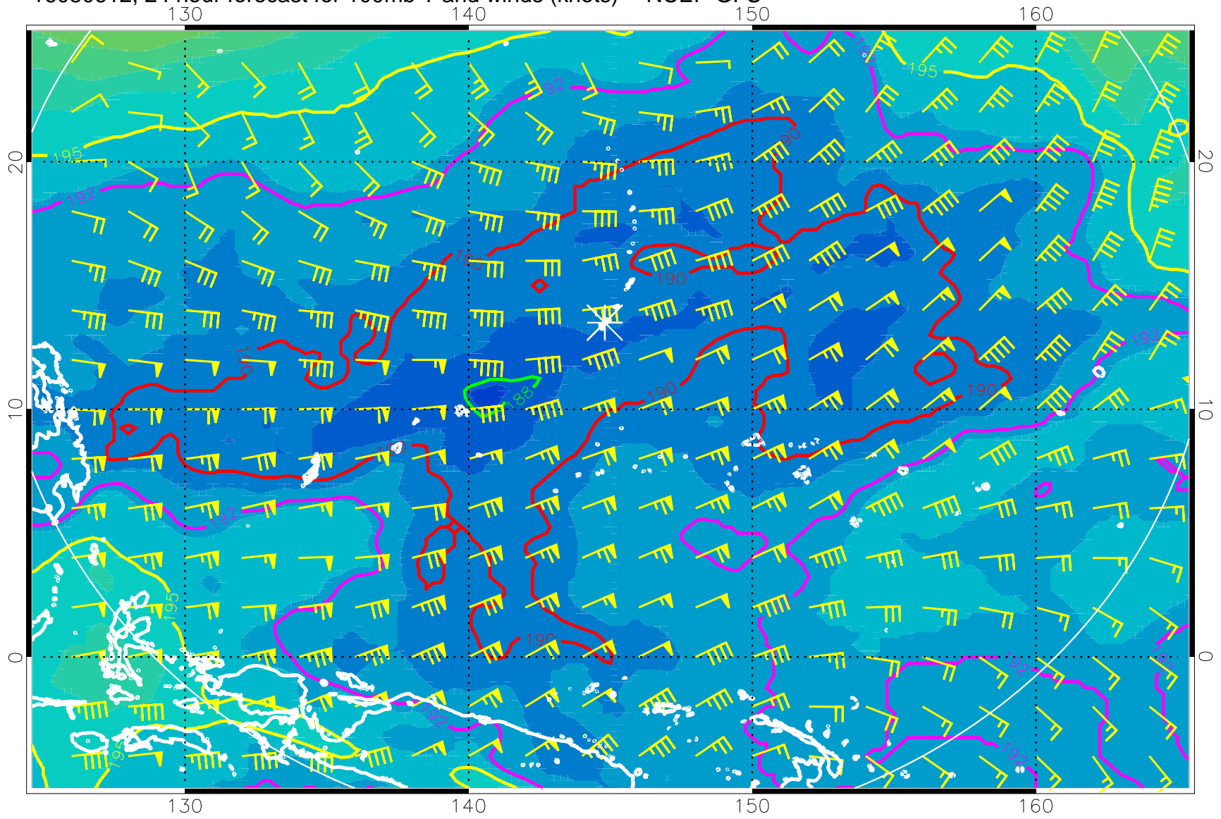
16080612, 24 hour forecast for 100mb T and winds (knots) -- NCEP GFS
