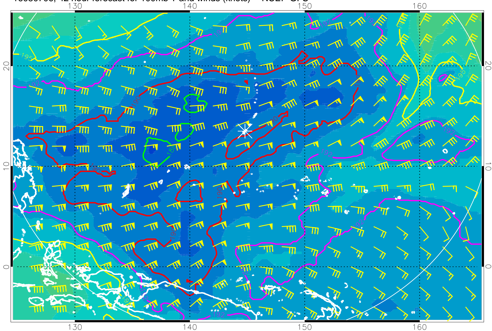
16080706, 42 hour forecast for 100mb T and winds (knots) -- NCEP GFS
