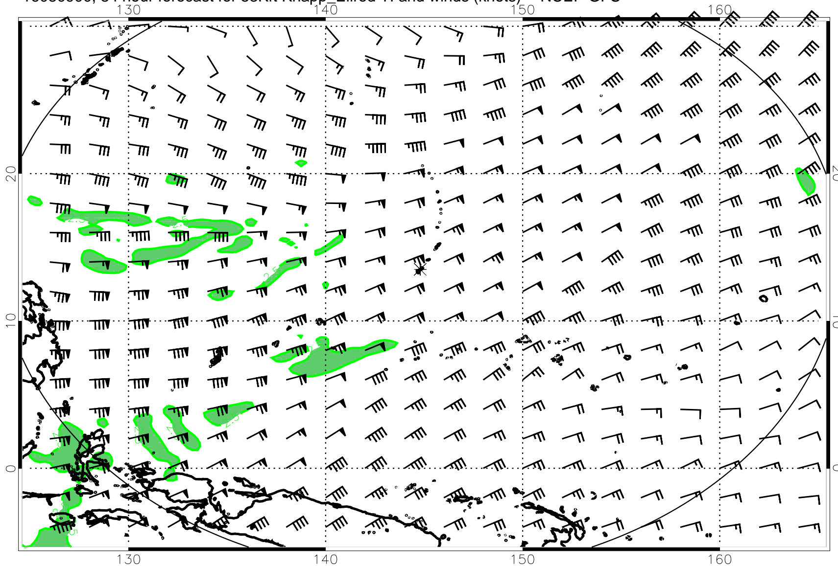
16080900, 84 hour forecast for 53Kft Knapp_Ellrod TI and winds (knots) -- NCEP GFS
