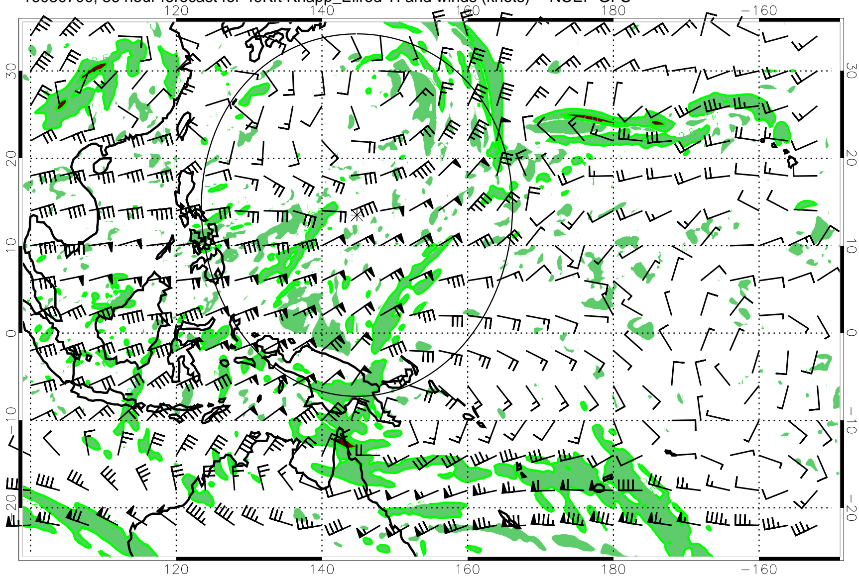
16080700, 36 hour forecast for 49Kft Knapp_Ellrod TI and winds (knots) -- NCEP GFS
