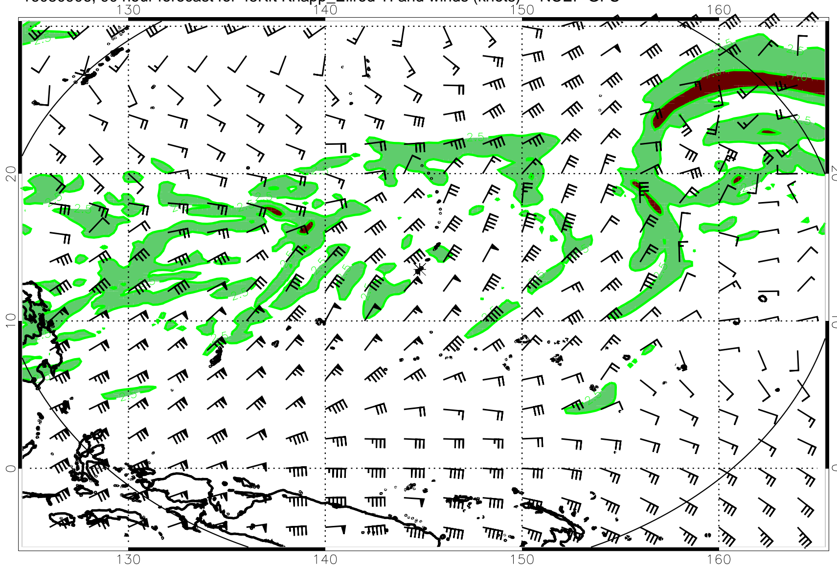
16080906, 90 hour forecast for 45Kft Knapp_Ellrod TI and winds (knots) -- NCEP GFS
