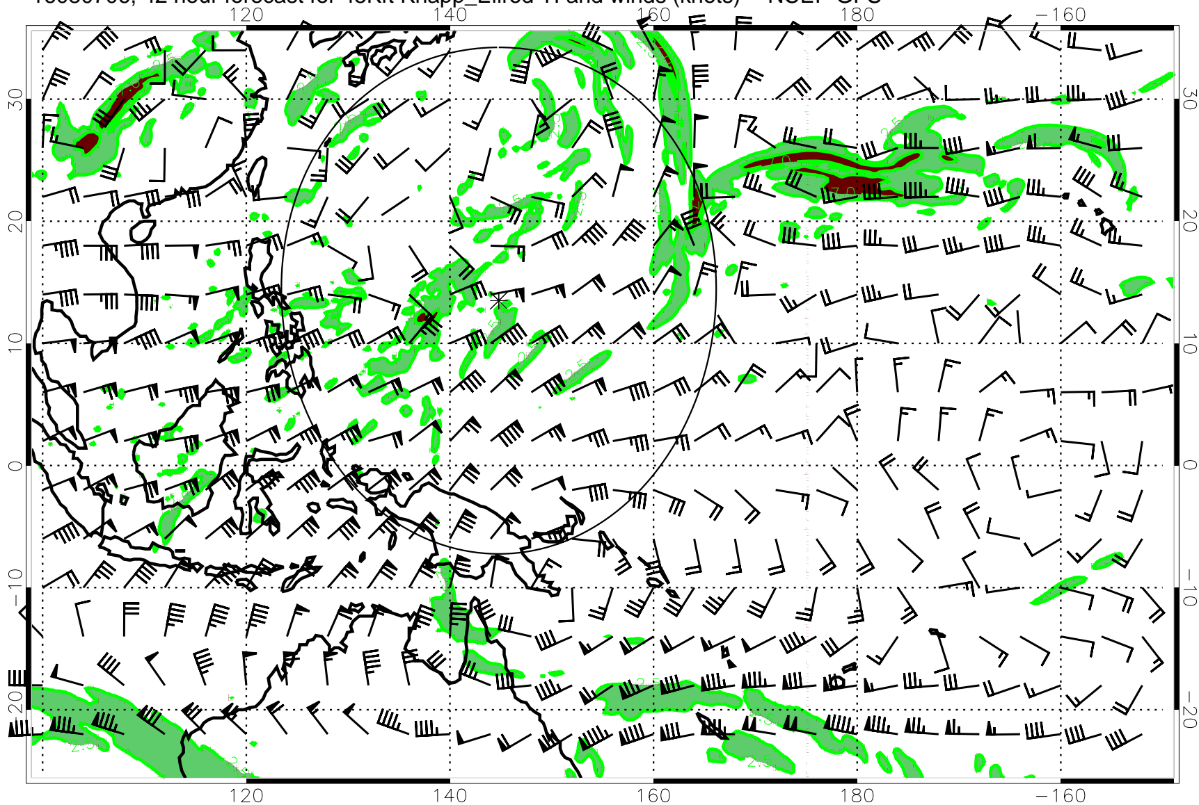
16080706, 42 hour forecast for 45Kft Knapp_Ellrod TI and winds (knots) -- NCEP GFS
