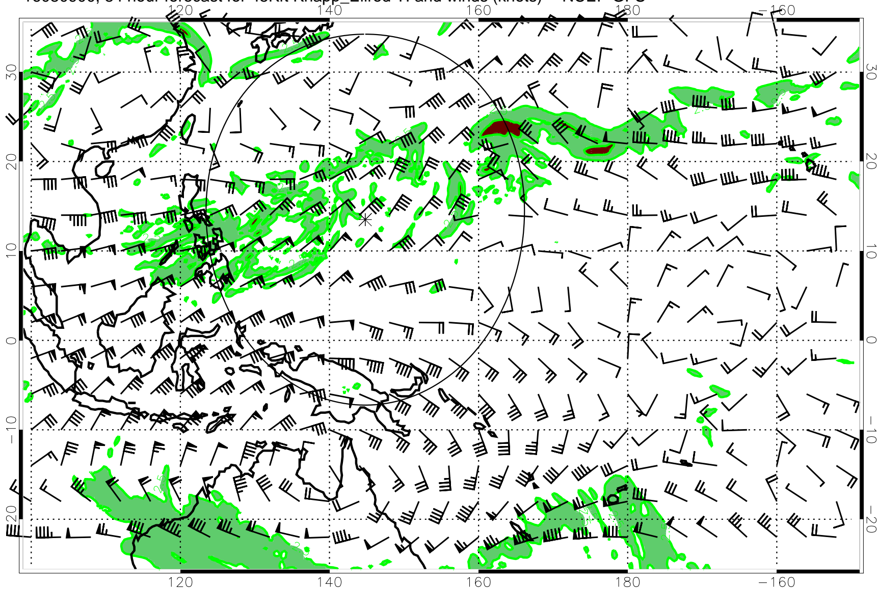
16080900, 84 hour forecast for 45Kft Knapp_Ellrod TI and winds (knots) -- NCEP GFS
