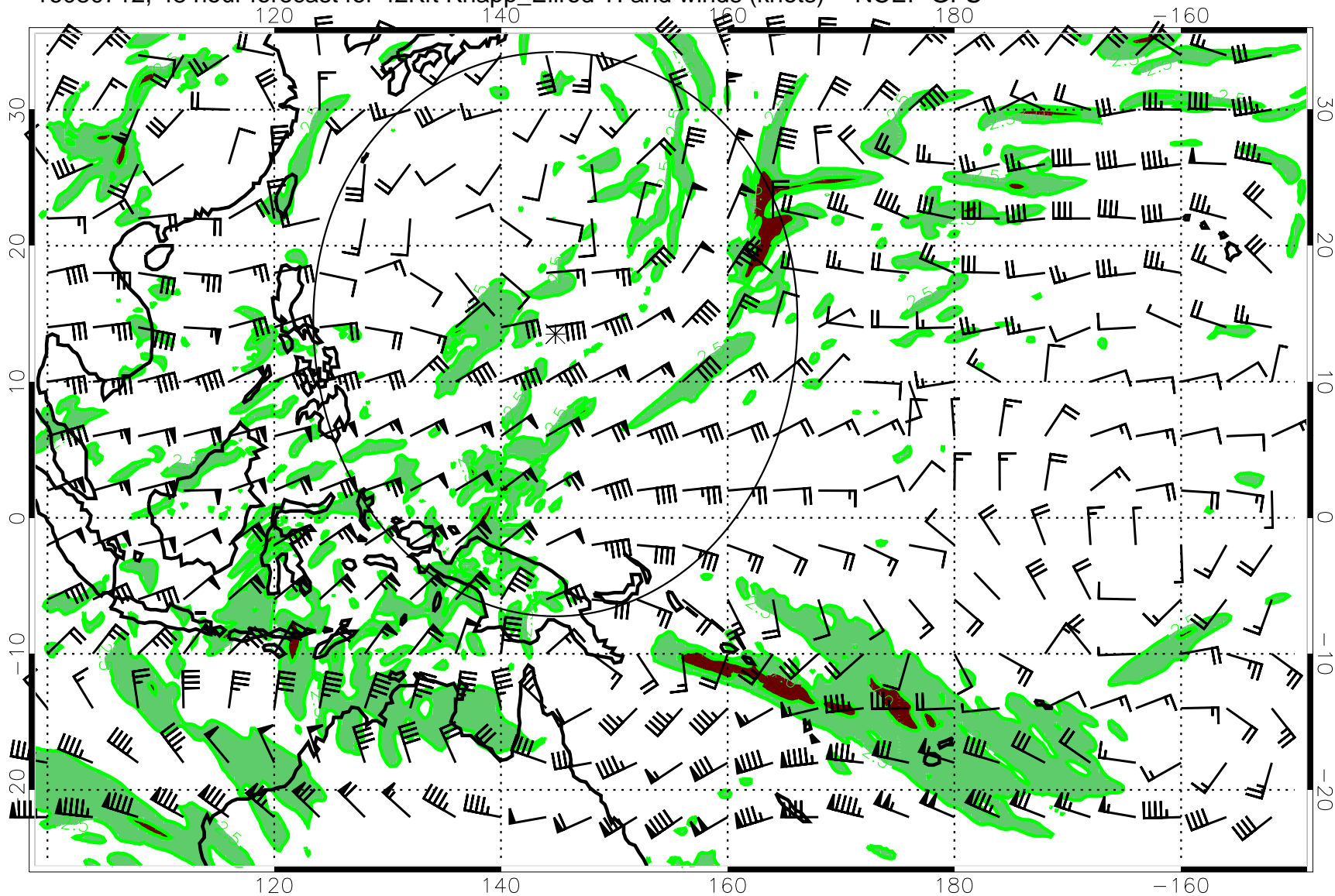
16080712, 48 hour forecast for 42Kft Knapp_Ellrod TI and winds (knots) -- NCEP GFS
