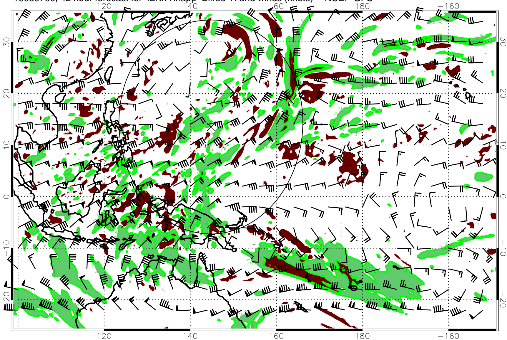
16080706, 42 hour forecast for 42Kft Knapp_Ellrod TI and winds (knots) -- NCEP GFS
