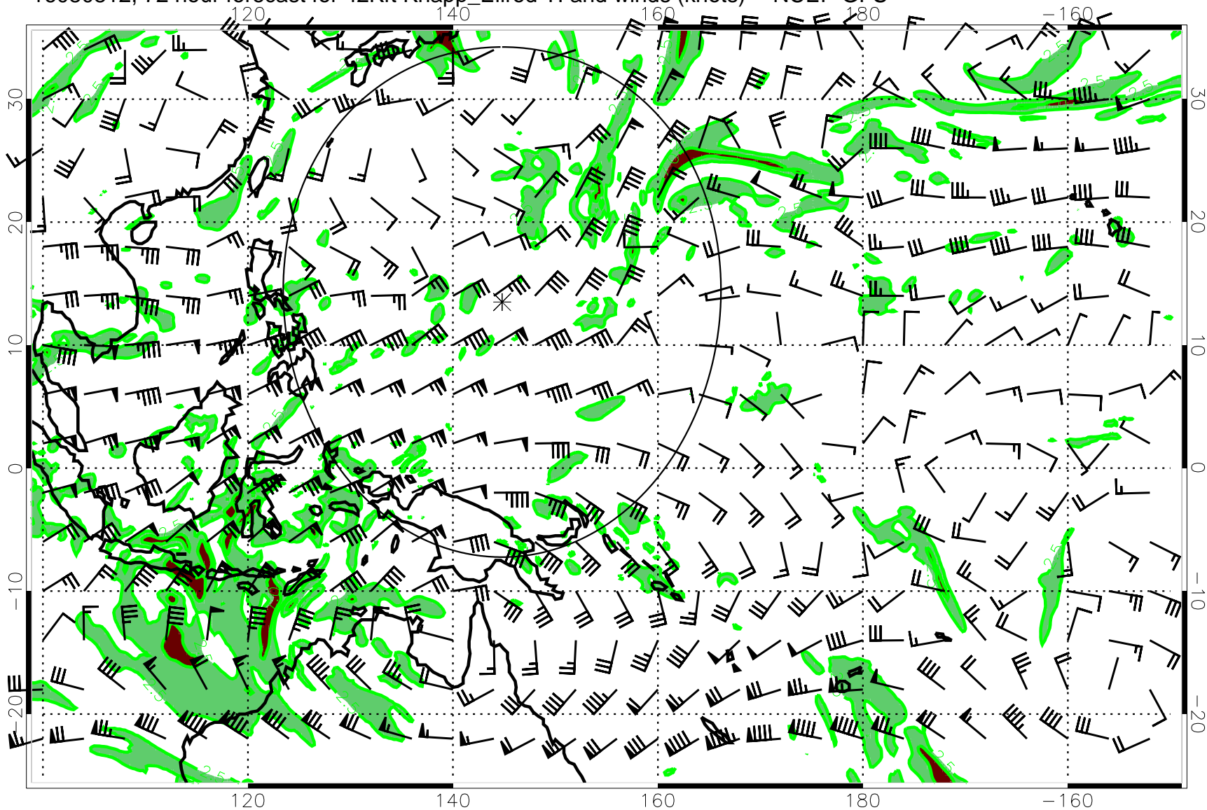
16080812, 72 hour forecast for 42Kft Knapp_Ellrod TI and winds (knots) -- NCEP GFS
