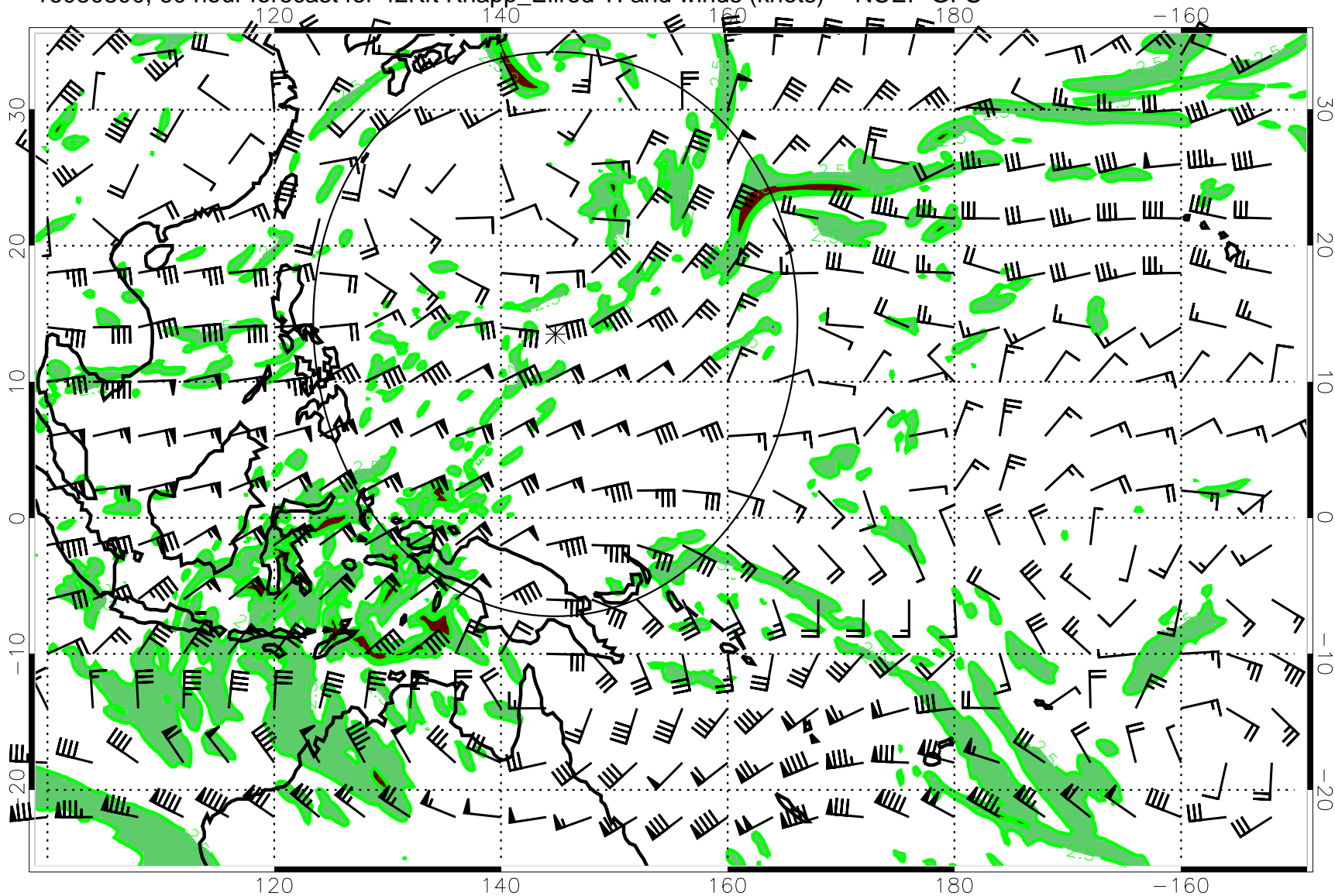
16080800, 60 hour forecast for 42Kft Knapp_Ellrod TI and winds (knots) -- NCEP GFS
