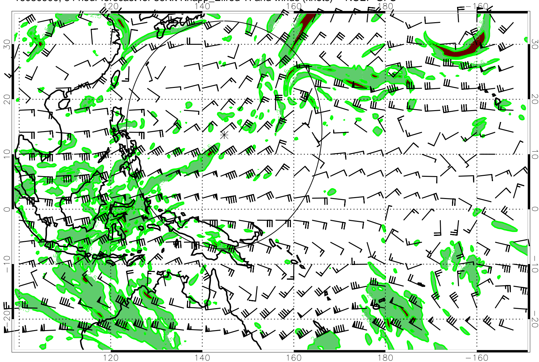
16080900, 84 hour forecast for 36Kft Knapp_Ellrod TI and winds (knots) -- NCEP GFS
