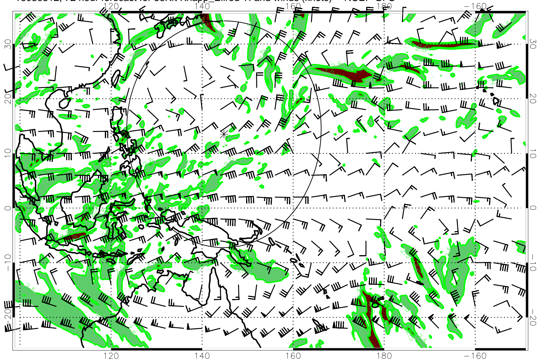
16080812, 72 hour forecast for 36Kft Knapp_Ellrod TI and winds (knots) -- NCEP GFS
