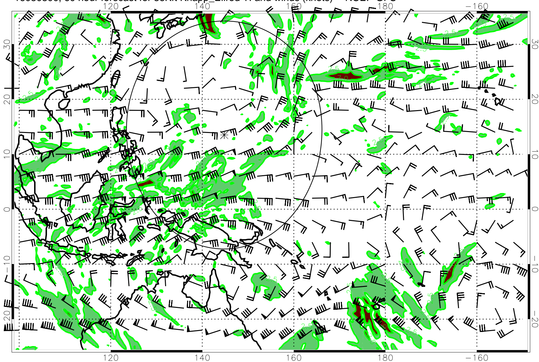
16080800, 60 hour forecast for 36Kft Knapp_Ellrod TI and winds (knots) -- NCEP GFS
