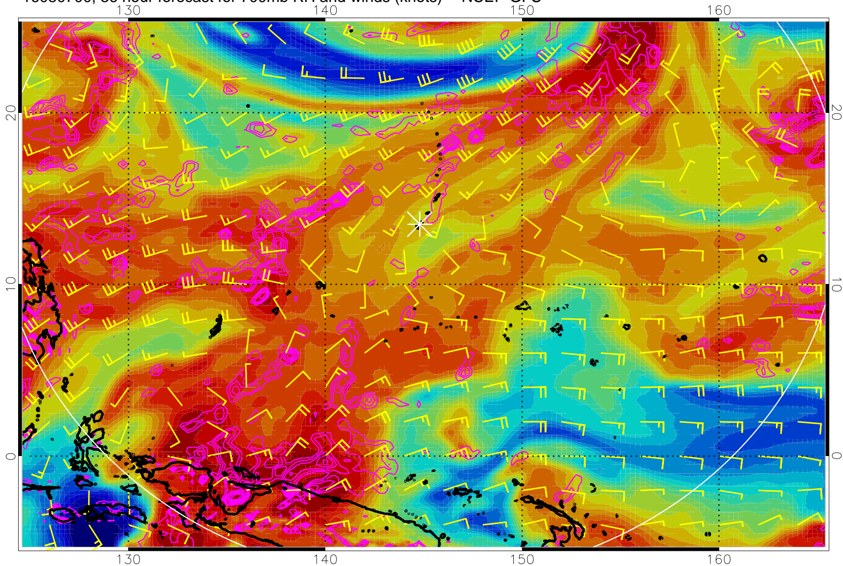
16080700, 36 hour forecast for 700mb RH and winds (knots) -- NCEP GFS
