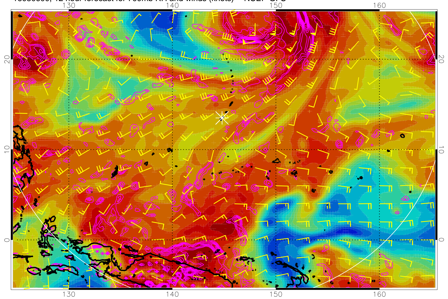
16080600, 12 hour forecast for 700mb RH and winds (knots) -- NCEP GFS
