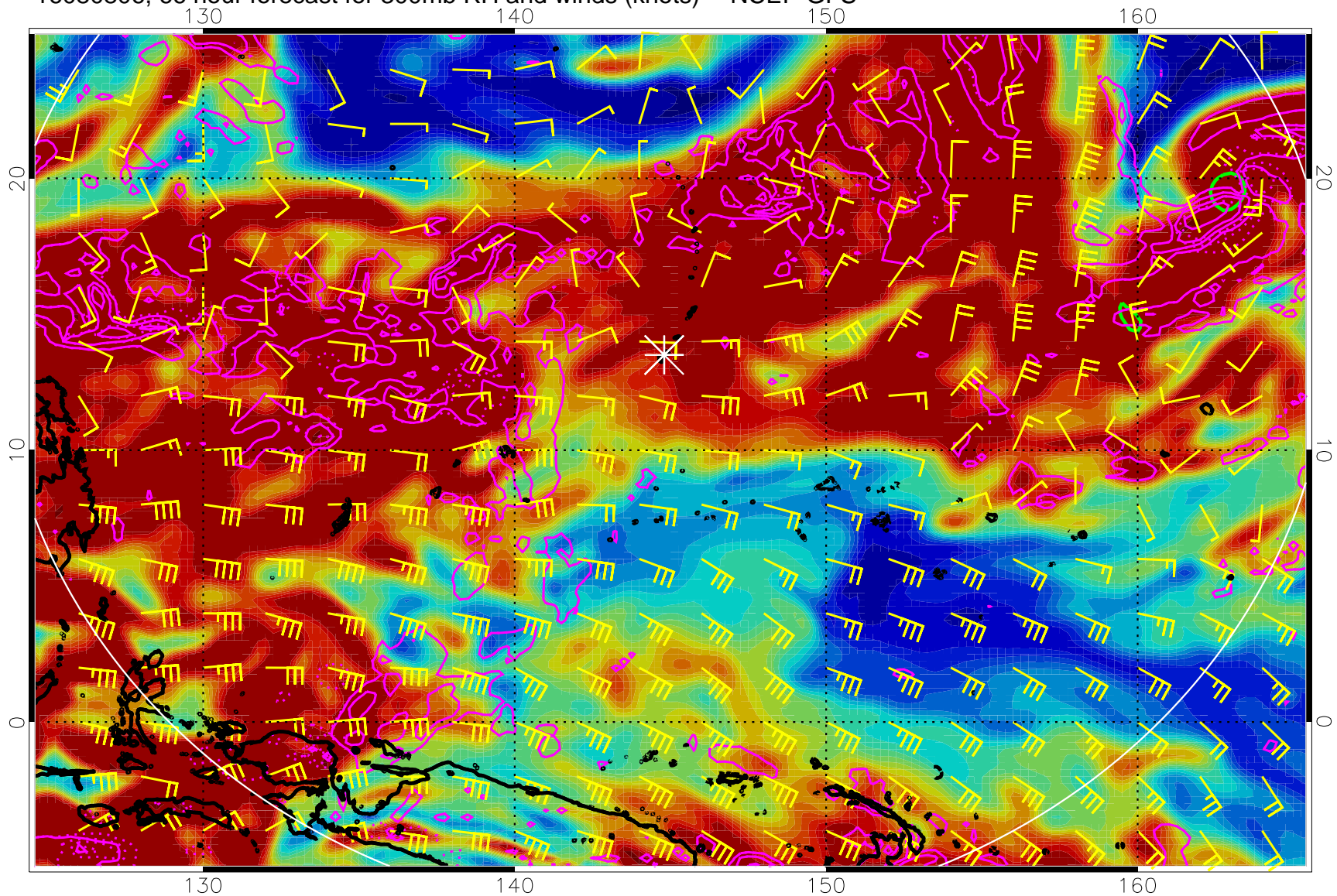
16080806, 66 hour forecast for 300mb RH and winds (knots) -- NCEP GFS
