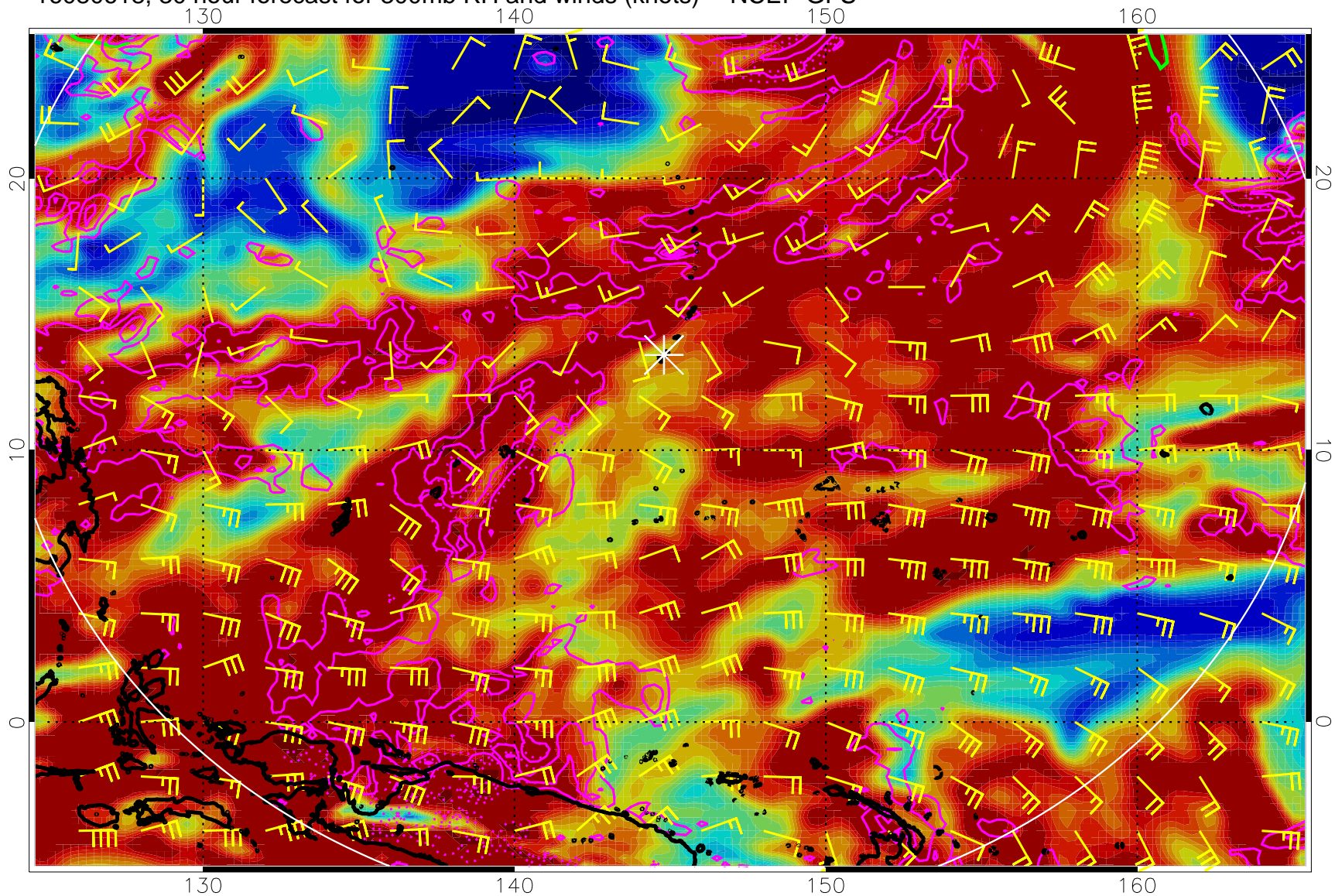
16080618, 30 hour forecast for 300mb RH and winds (knots) -- NCEP GFS
