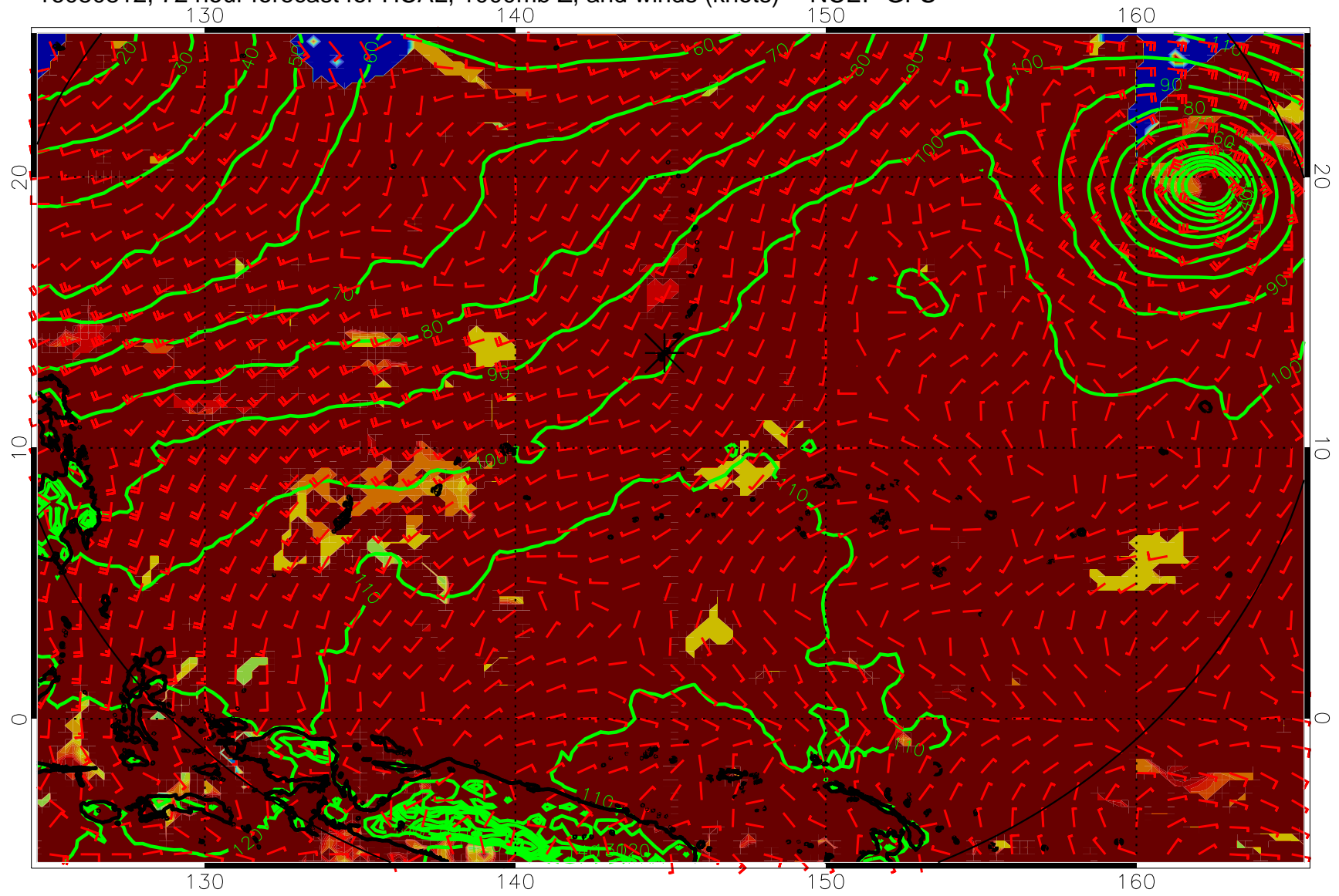
16080812, 72 hour forecast for HCAL, 1000mb Z, and winds (knots) -- NCEP GFS
