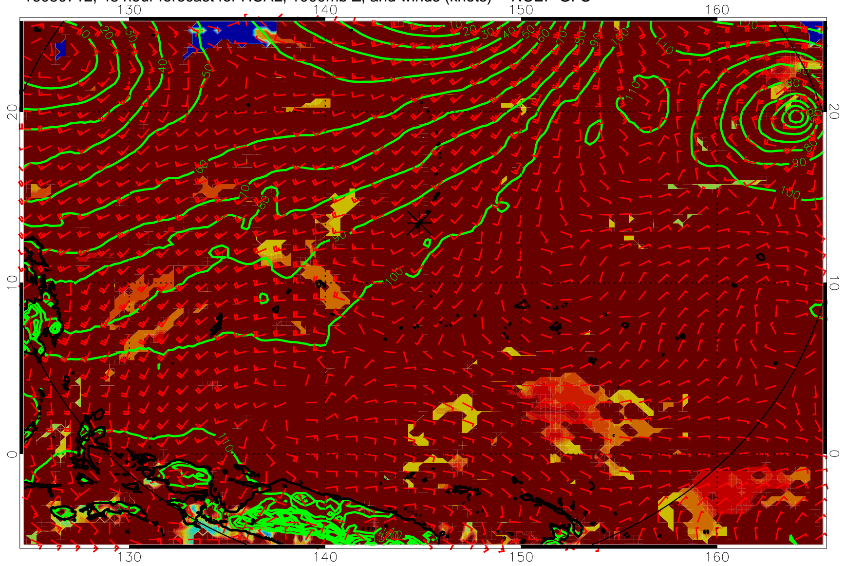
16080712, 48 hour forecast for HCAL, 1000mb Z, and winds (knots) -- NCEP GFS
