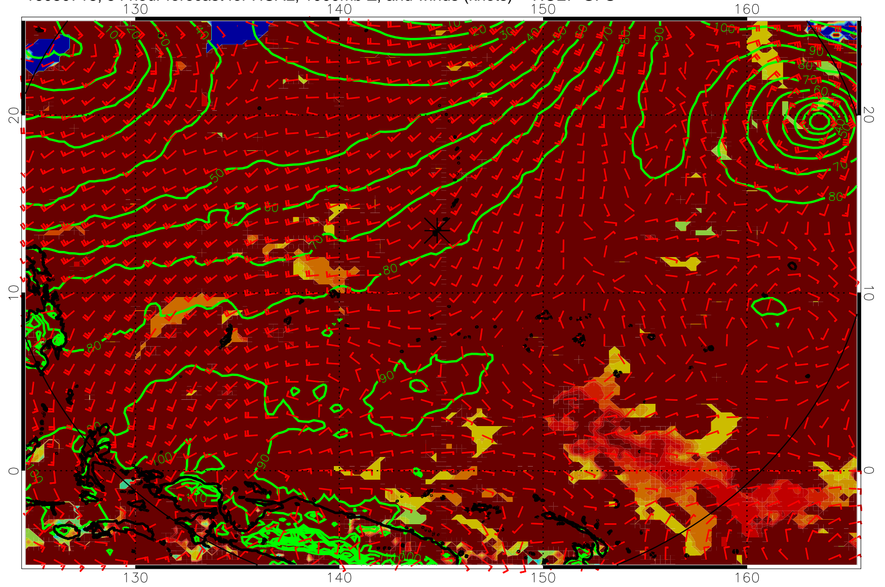
16080718, 54 hour forecast for HCAL, 1000mb Z, and winds (knots) -- NCEP GFS
