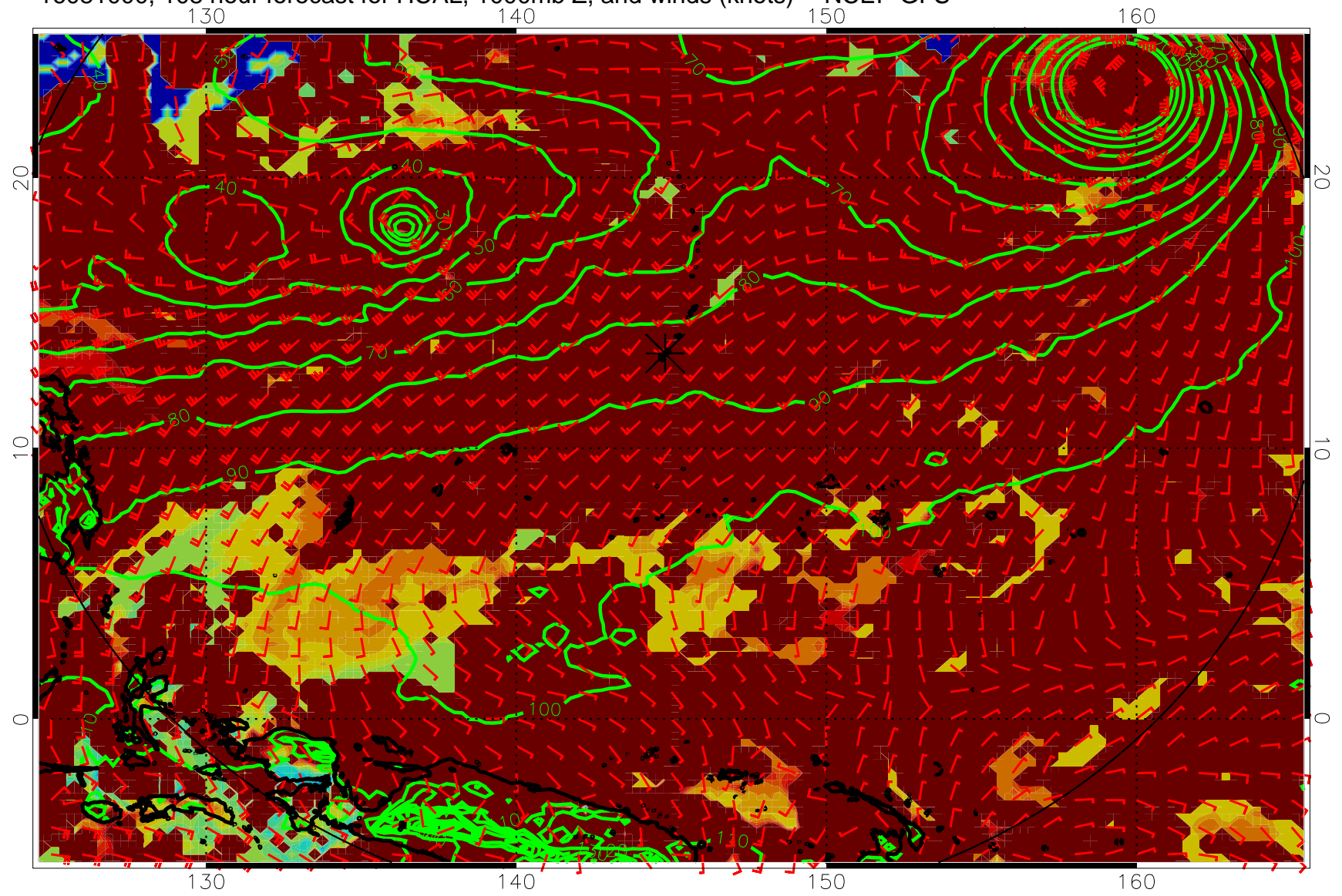
16081000, 108 hour forecast for HCAL, 1000mb Z, and winds (knots) -- NCEP GFS
