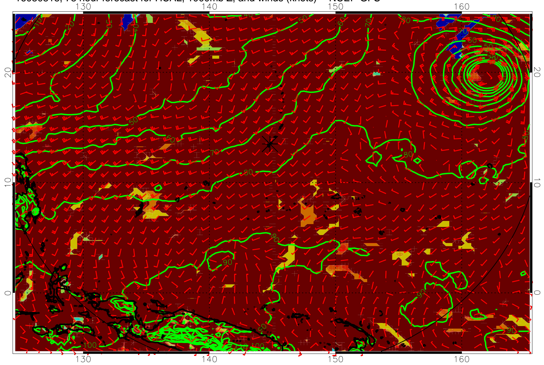
16080818, 78 hour forecast for HCAL, 1000mb Z, and winds (knots) -- NCEP GFS
