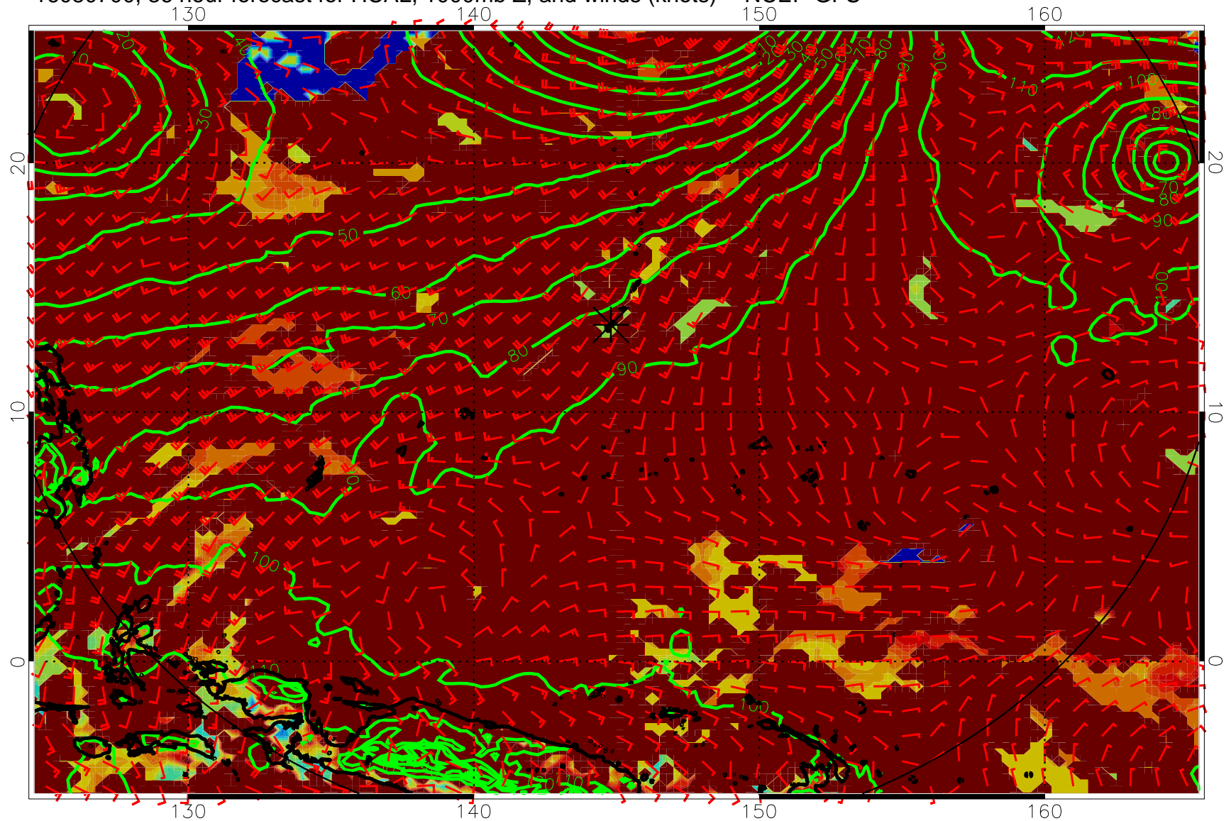
16080700, 36 hour forecast for HCAL, 1000mb Z, and winds (knots) -- NCEP GFS
