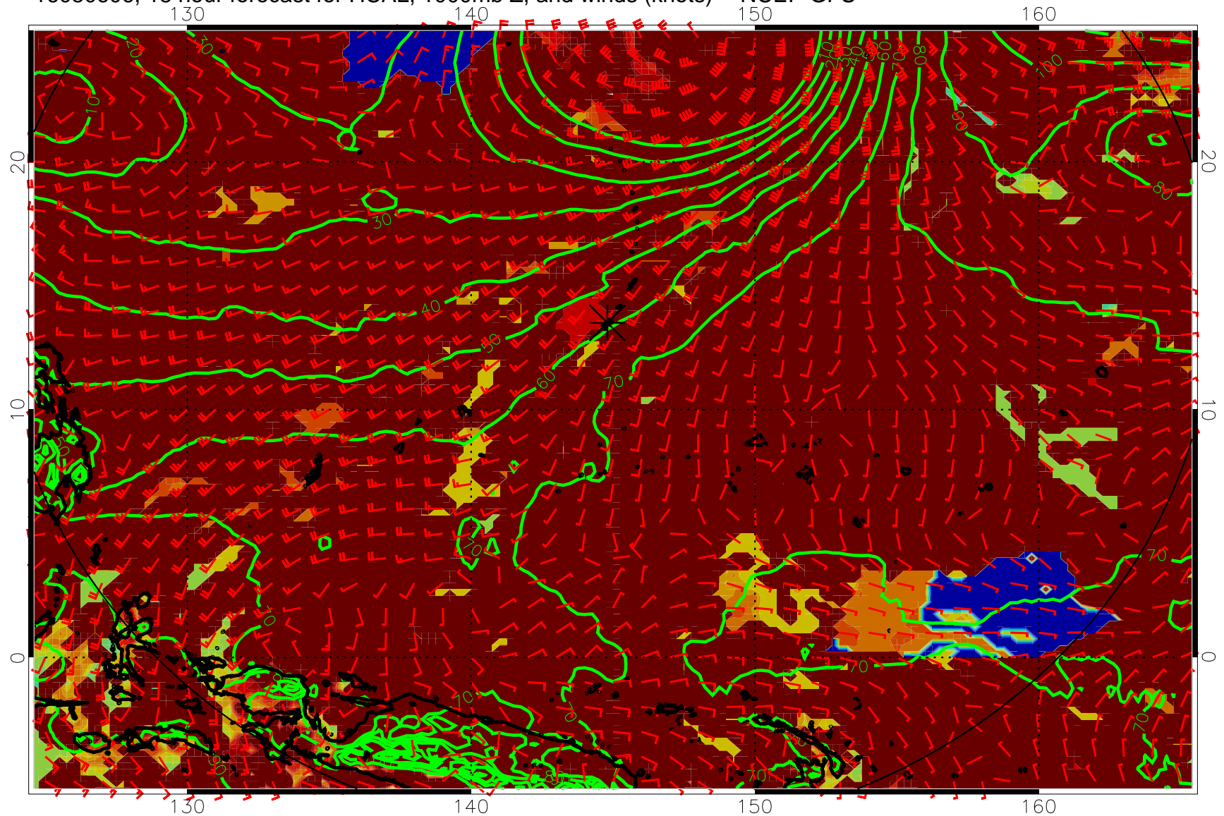
16080606, 18 hour forecast for HCAL, 1000mb Z, and winds (knots) -- NCEP GFS
