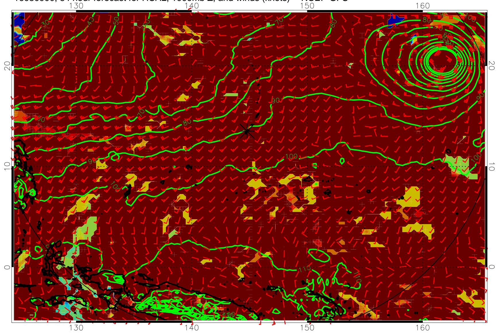
16080900, 84 hour forecast for HCAL, 1000mb Z, and winds (knots) -- NCEP GFS
