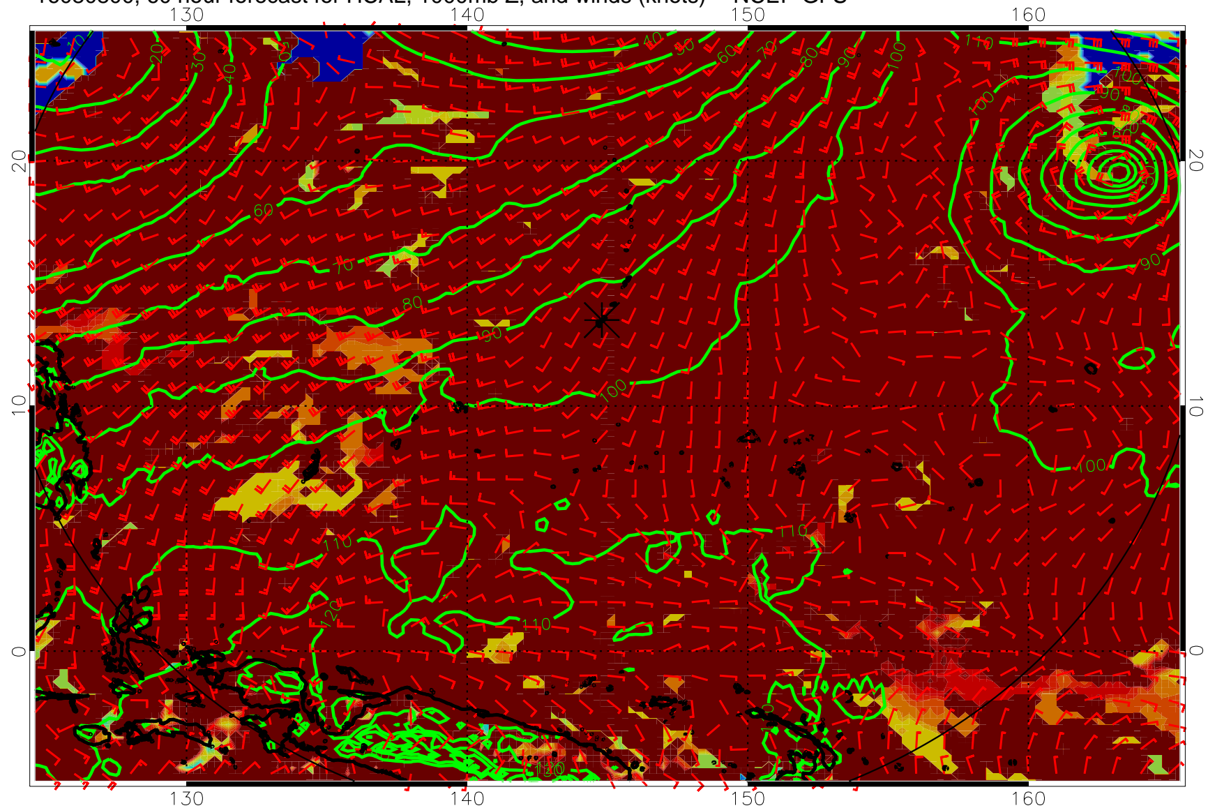
16080800, 60 hour forecast for HCAL, 1000mb Z, and winds (knots) -- NCEP GFS
