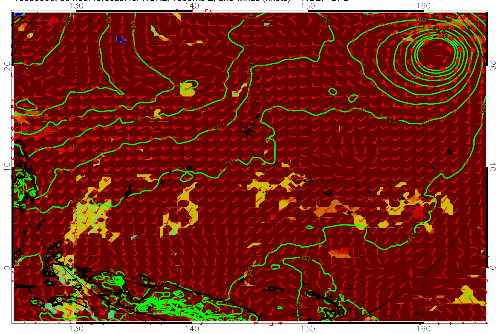
16080906, 90 hour forecast for HCAL, 1000mb Z, and winds (knots) -- NCEP GFS
