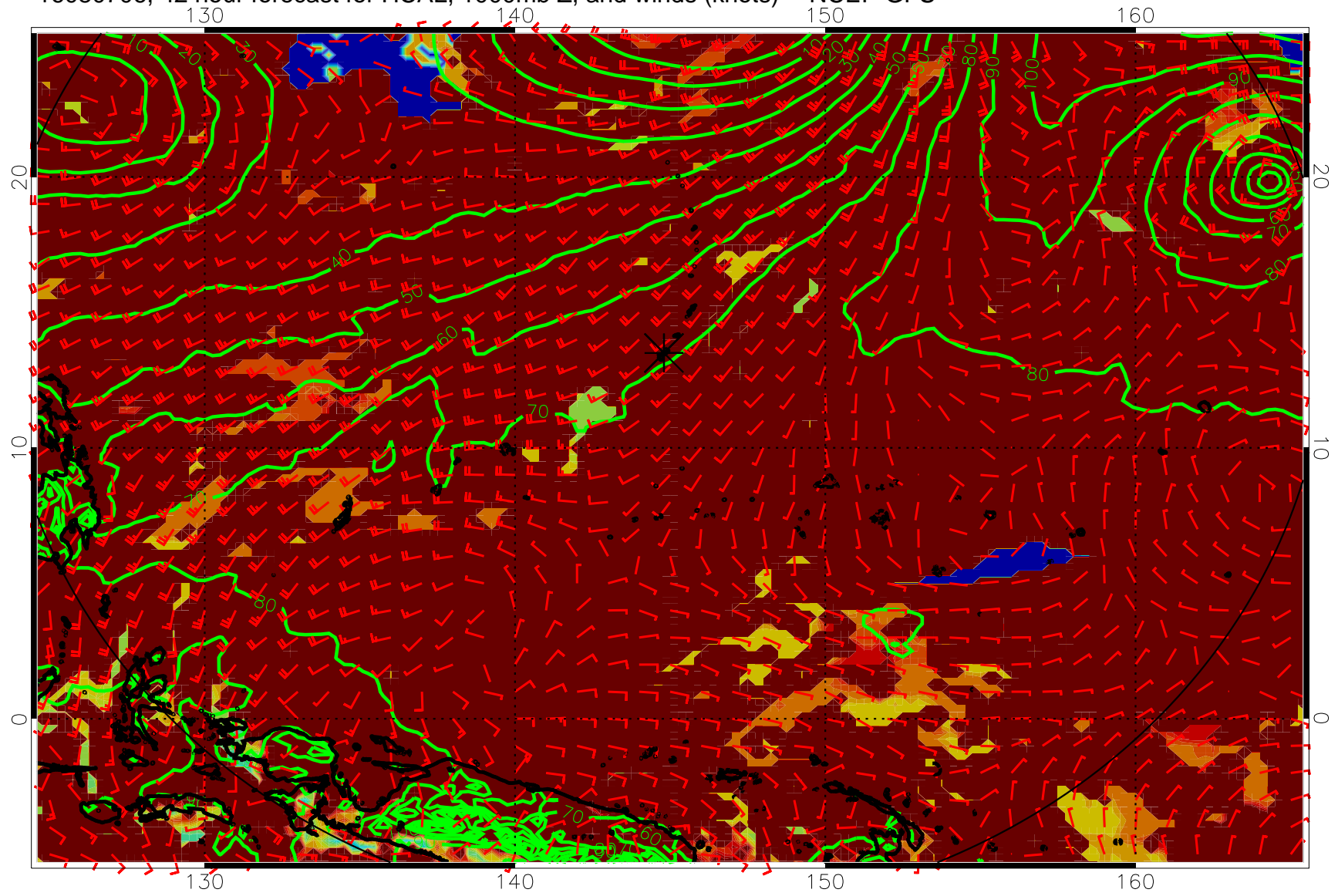
16080706, 42 hour forecast for HCAL, 1000mb Z, and winds (knots) -- NCEP GFS
