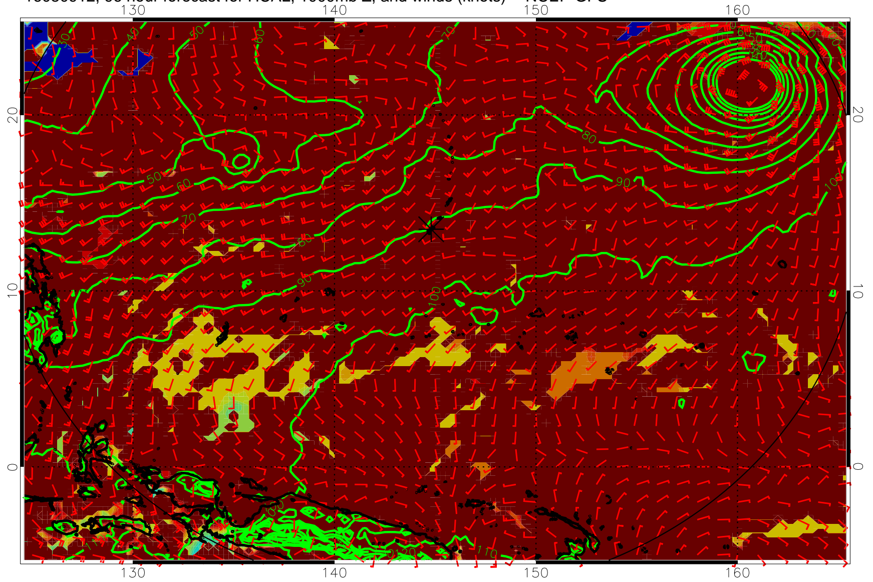
16080912, 96 hour forecast for HCAL, 1000mb Z, and winds (knots) -- NCEP GFS
