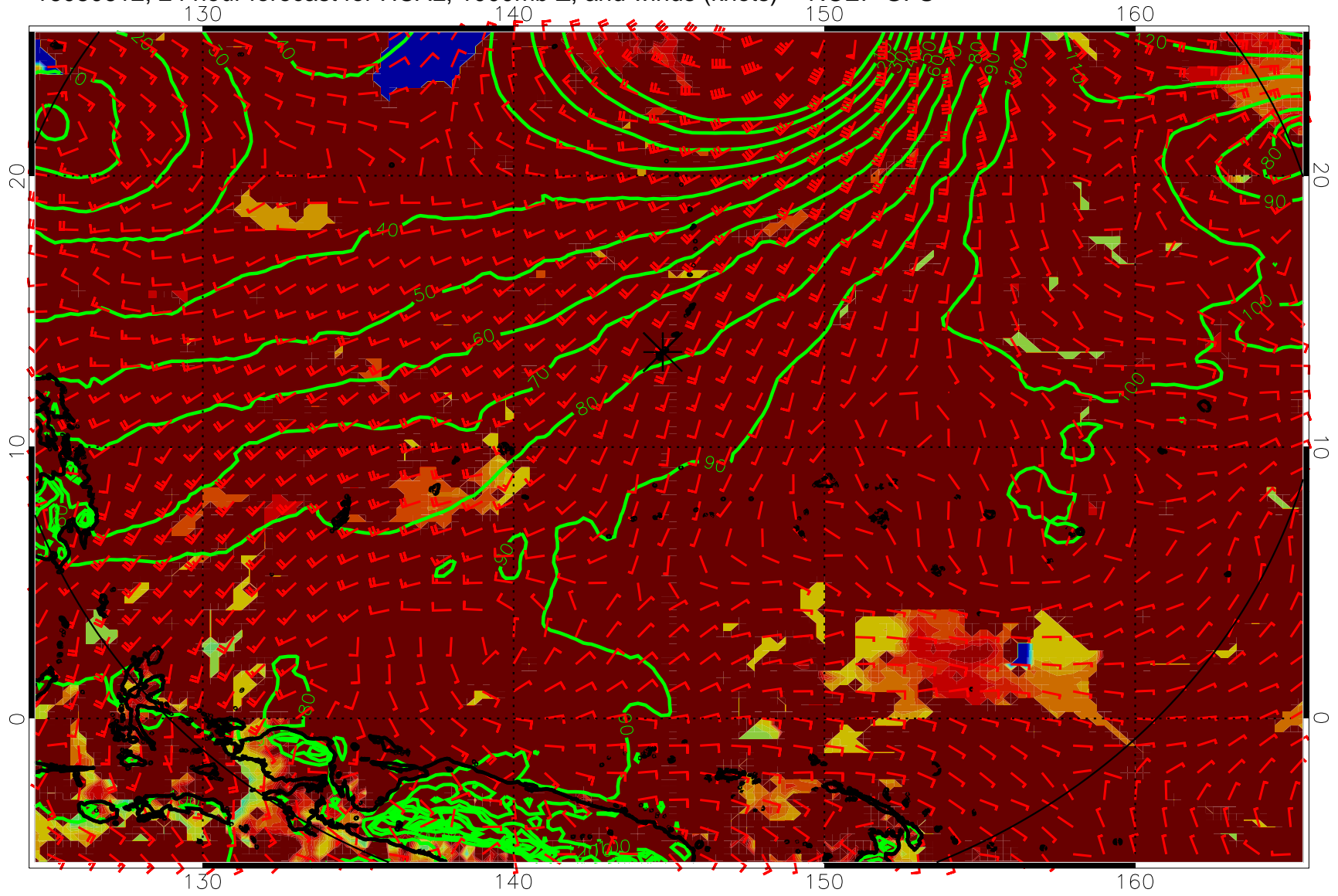
16080612, 24 hour forecast for HCAL, 1000mb Z, and winds (knots) -- NCEP GFS
