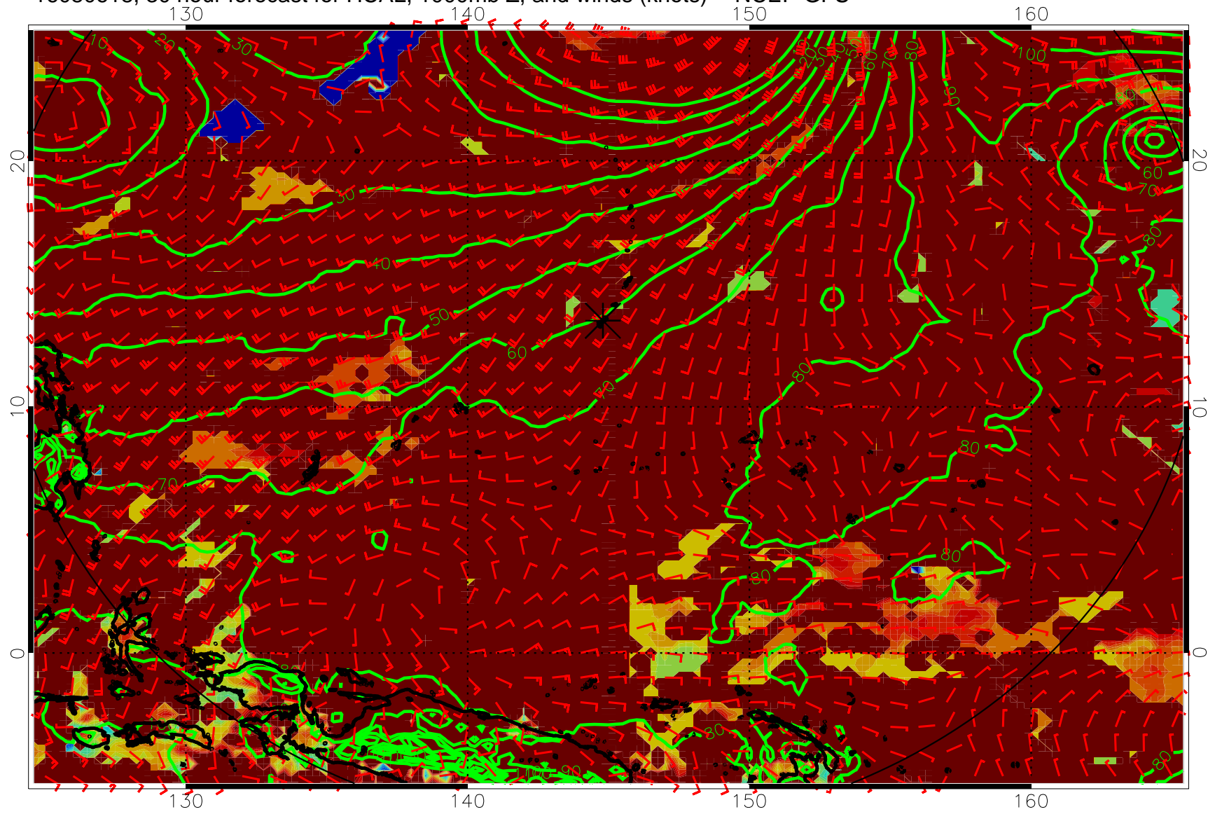
16080618, 30 hour forecast for HCAL, 1000mb Z, and winds (knots) -- NCEP GFS
