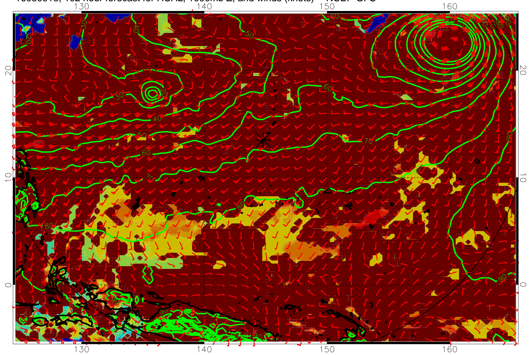
16080918, 102 hour forecast for HCAL, 1000mb Z, and winds (knots) -- NCEP GFS
