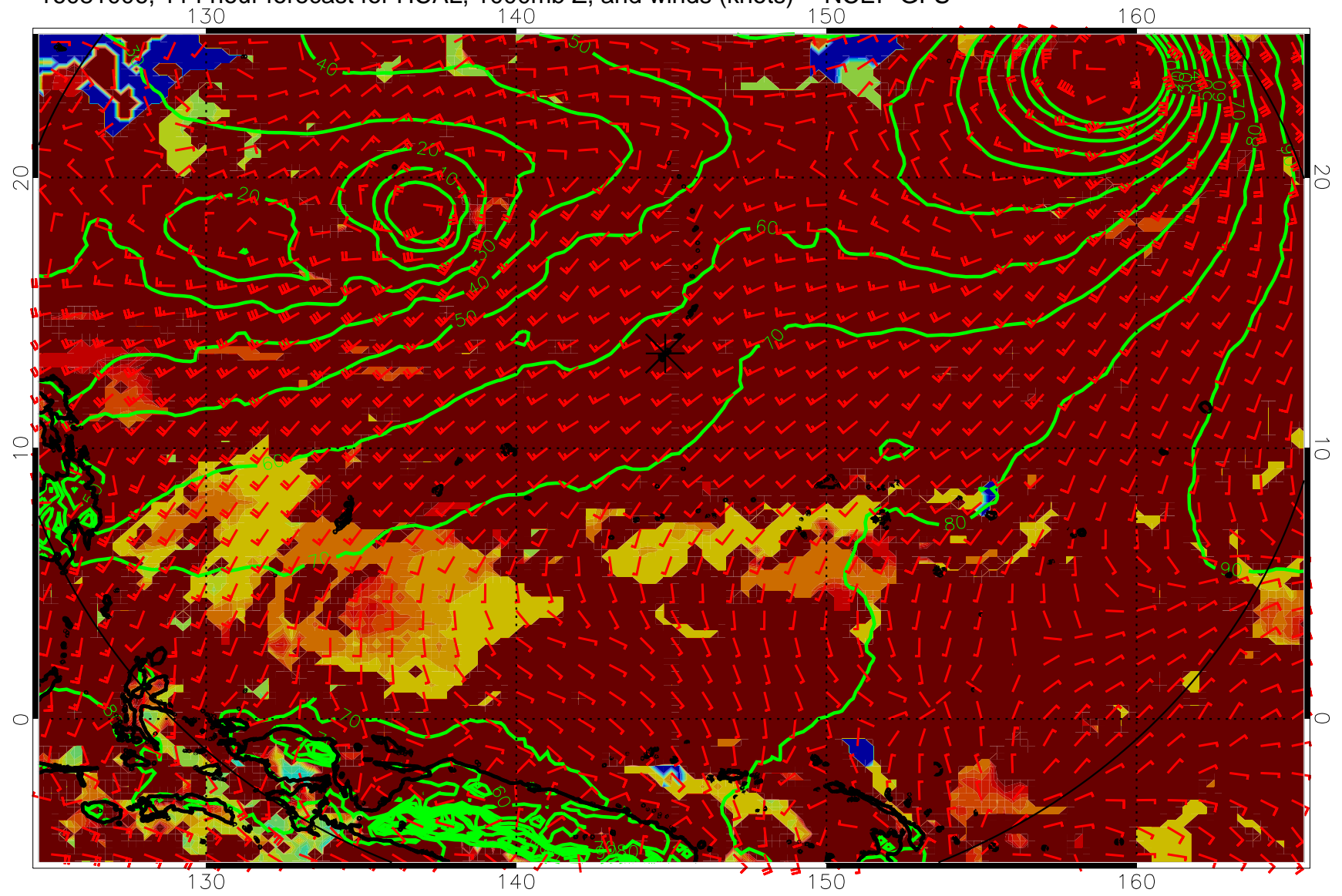
16081006, 114 hour forecast for HCAL, 1000mb Z, and winds (knots) -- NCEP GFS
