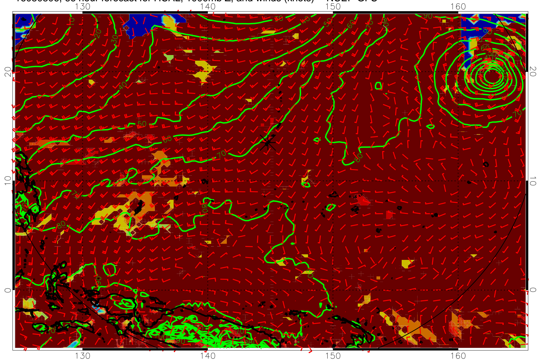
16080806, 66 hour forecast for HCAL, 1000mb Z, and winds (knots) -- NCEP GFS
