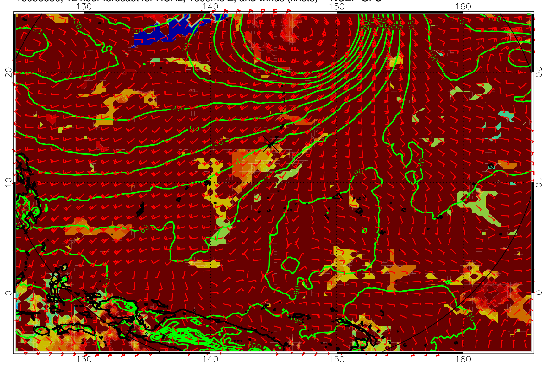
16080600, 12 hour forecast for HCAL, 1000mb Z, and winds (knots) -- NCEP GFS
