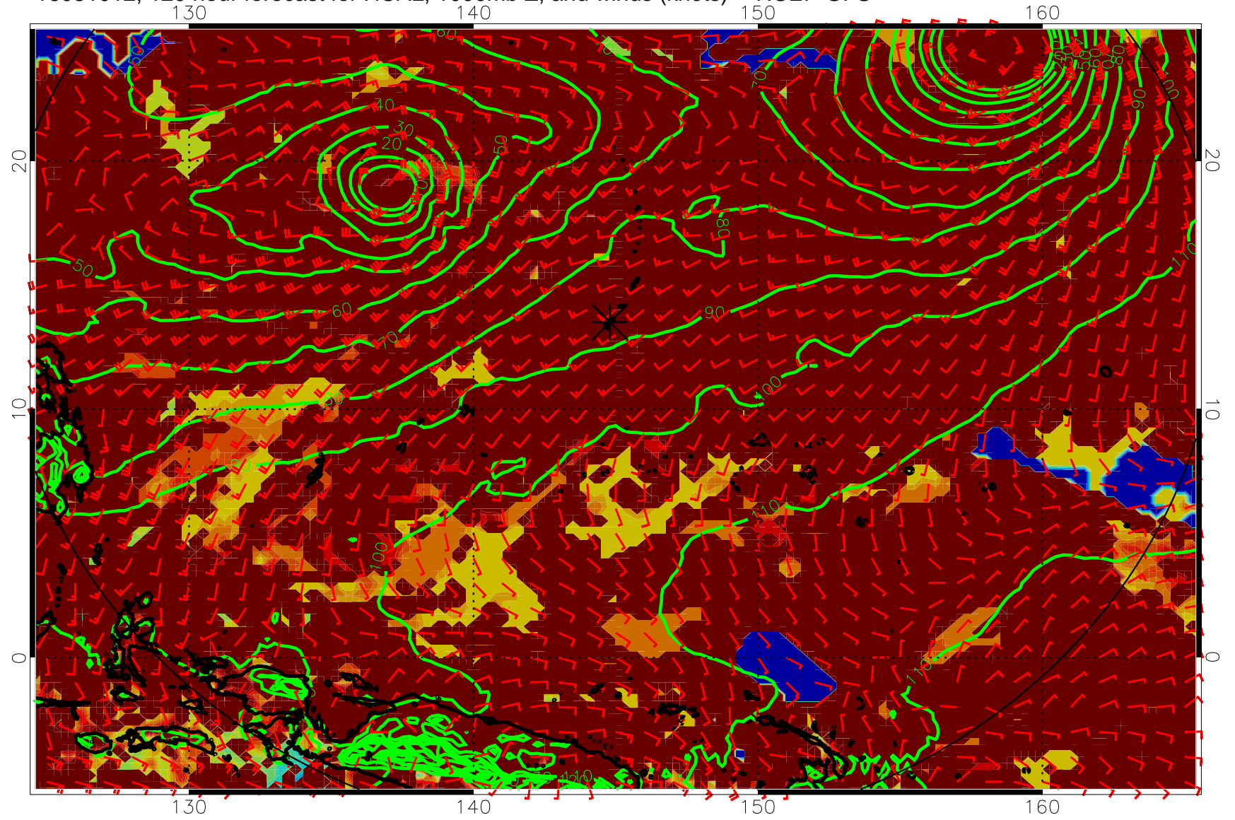
16081012, 120 hour forecast for HCAL, 1000mb Z, and winds (knots) -- NCEP GFS
