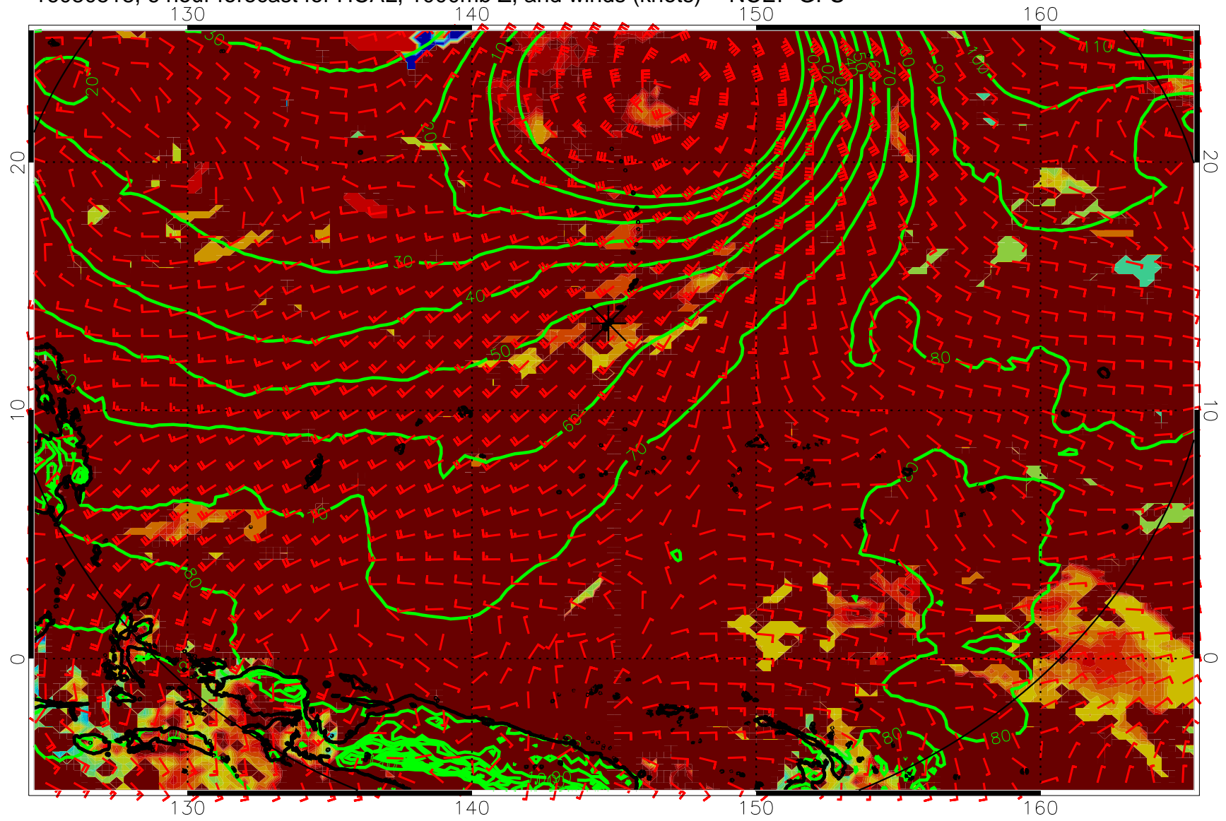
16080518, 6 hour forecast for HCAL, 1000mb Z, and winds (knots) -- NCEP GFS
