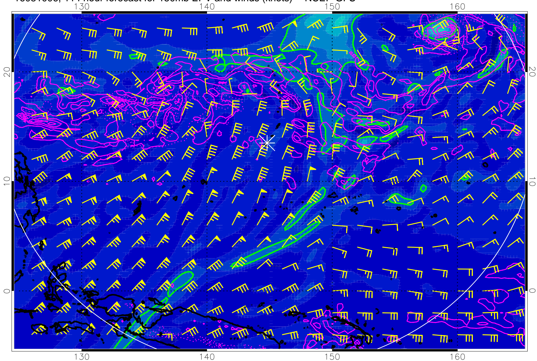
16081006, 114 hour forecast for 150mb EPV and winds (knots) -- NCEP GFS
