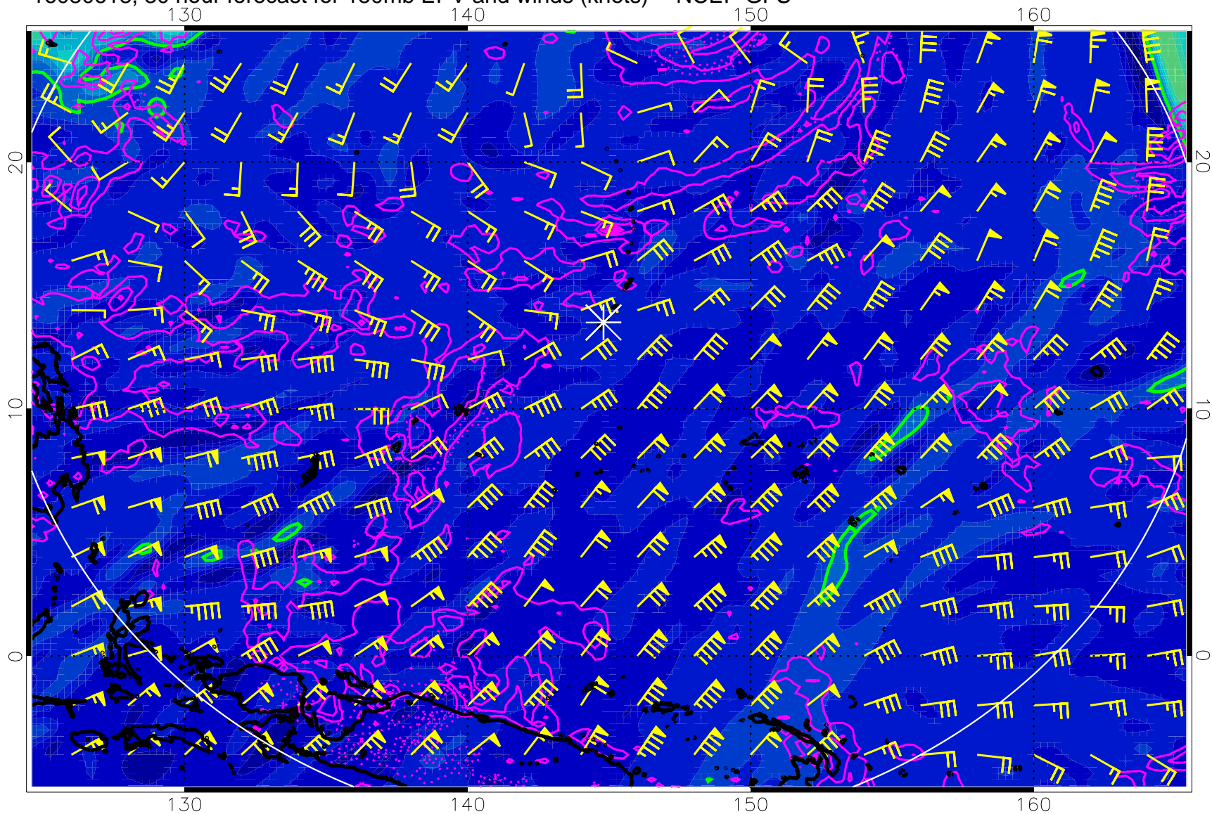
16080618, 30 hour forecast for 150mb EPV and winds (knots) -- NCEP GFS
