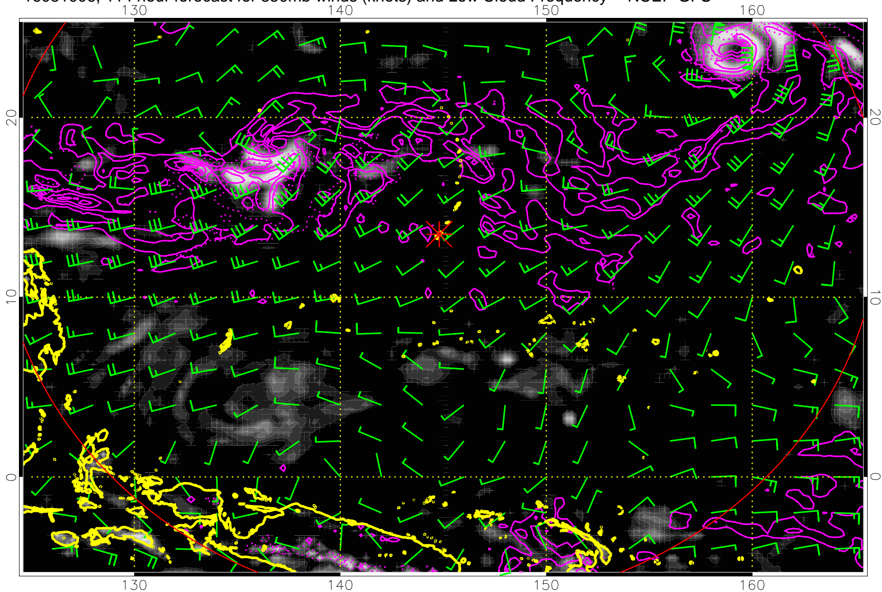
16081006, 114 hour forecast for 850mb winds (knots) and Low Cloud Frequency -- NCEP GFS
