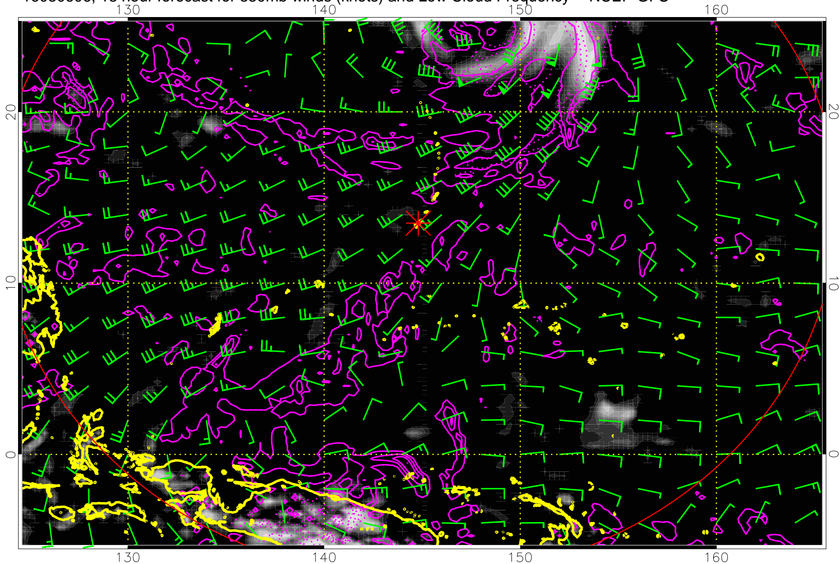
16080606, 18 hour forecast for 850mb winds (knots) and Low Cloud Frequency -- NCEP GFS
