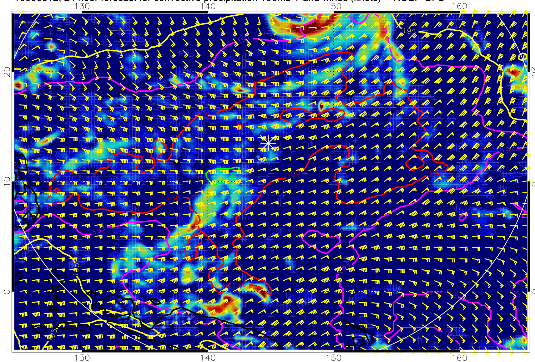
16080612, 24 hour forecast for convective precipitation 100mb T and winds (knots) -- NCEP GFS
