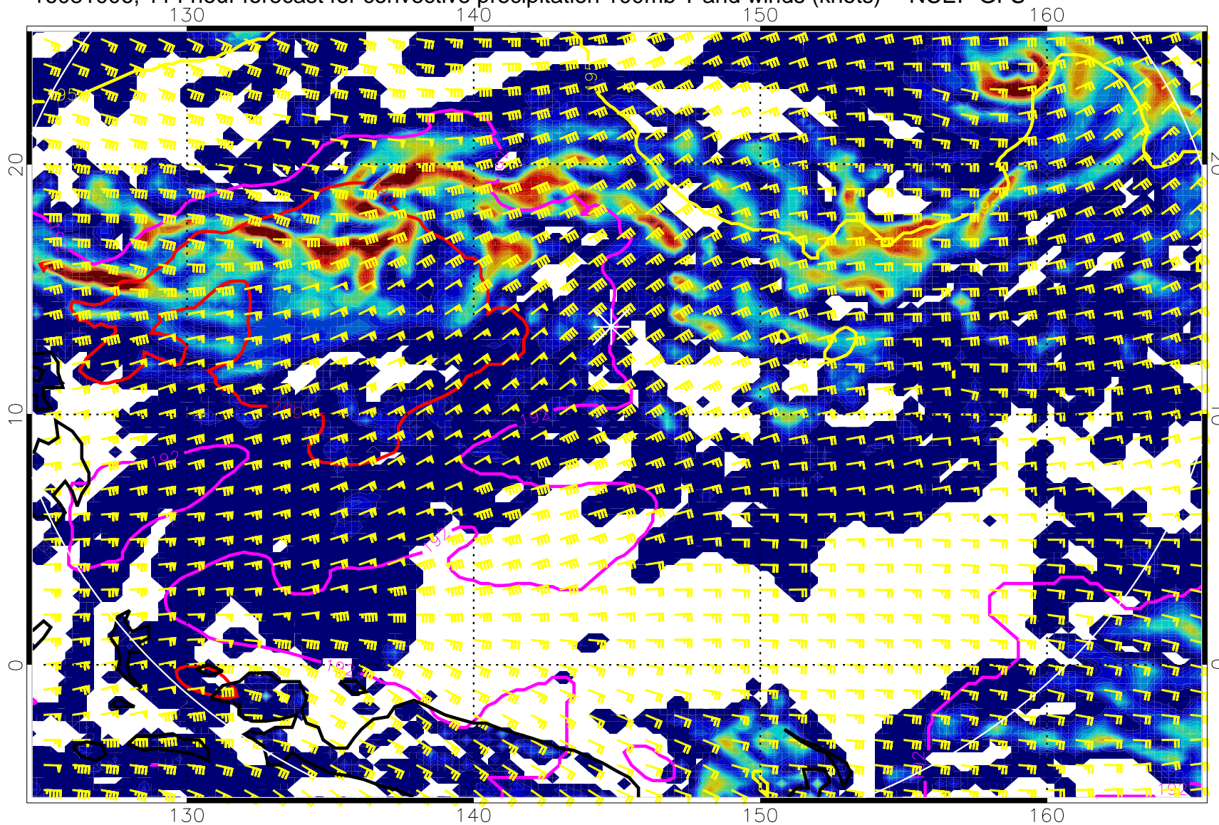
16081006, 114 hour forecast for convective precipitation 100mb T and winds (knots) -- NCEP GFS
