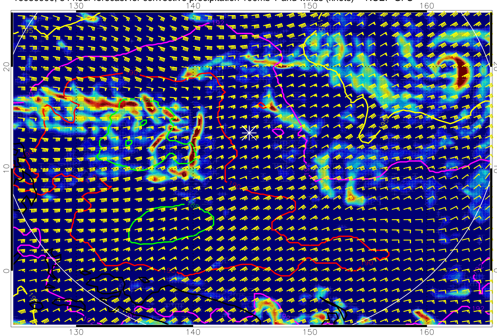
16080900, 84 hour forecast for convective precipitation 100mb T and winds (knots) -- NCEP GFS
