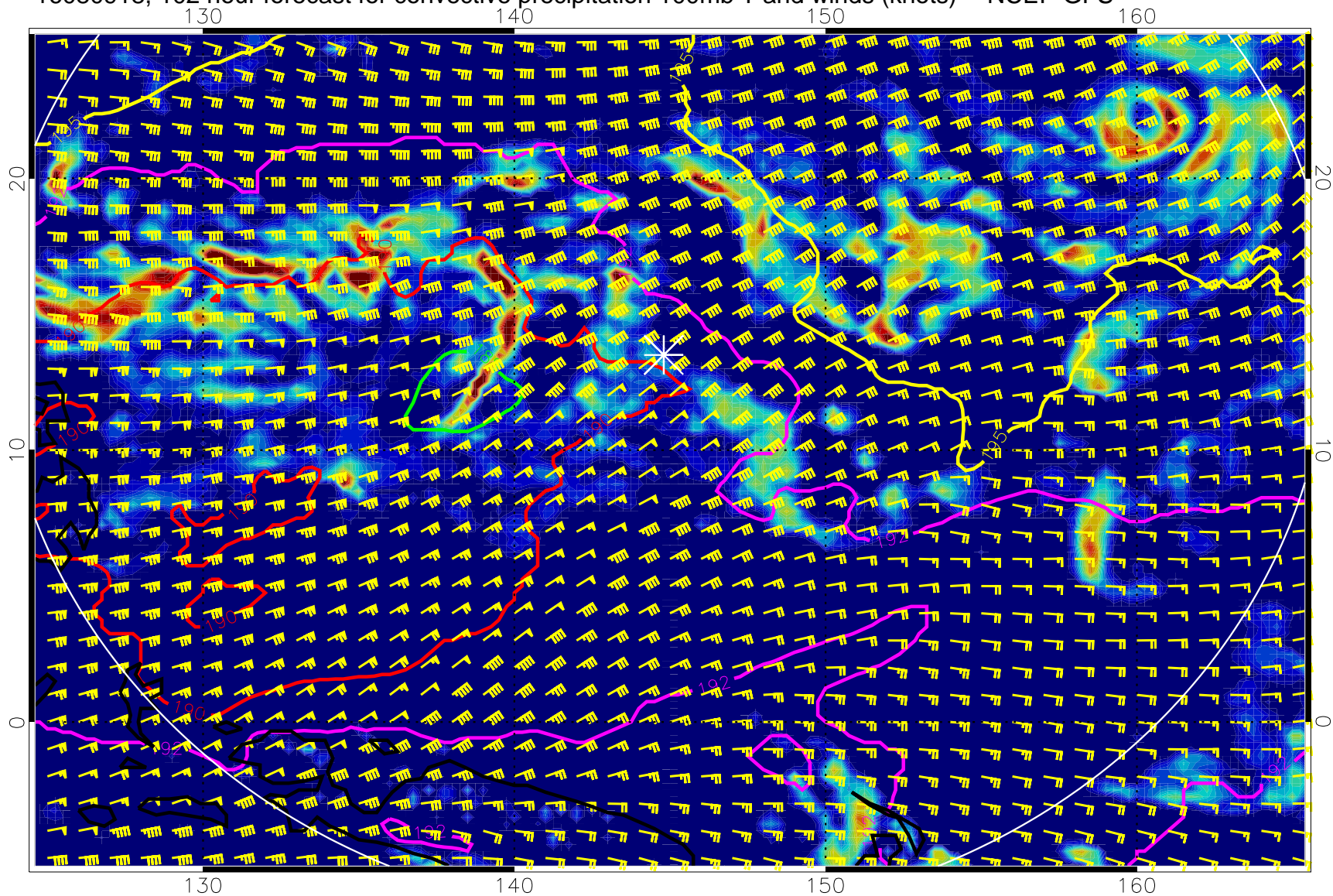
16080918, 102 hour forecast for convective precipitation 100mb T and winds (knots) -- NCEP GFS
