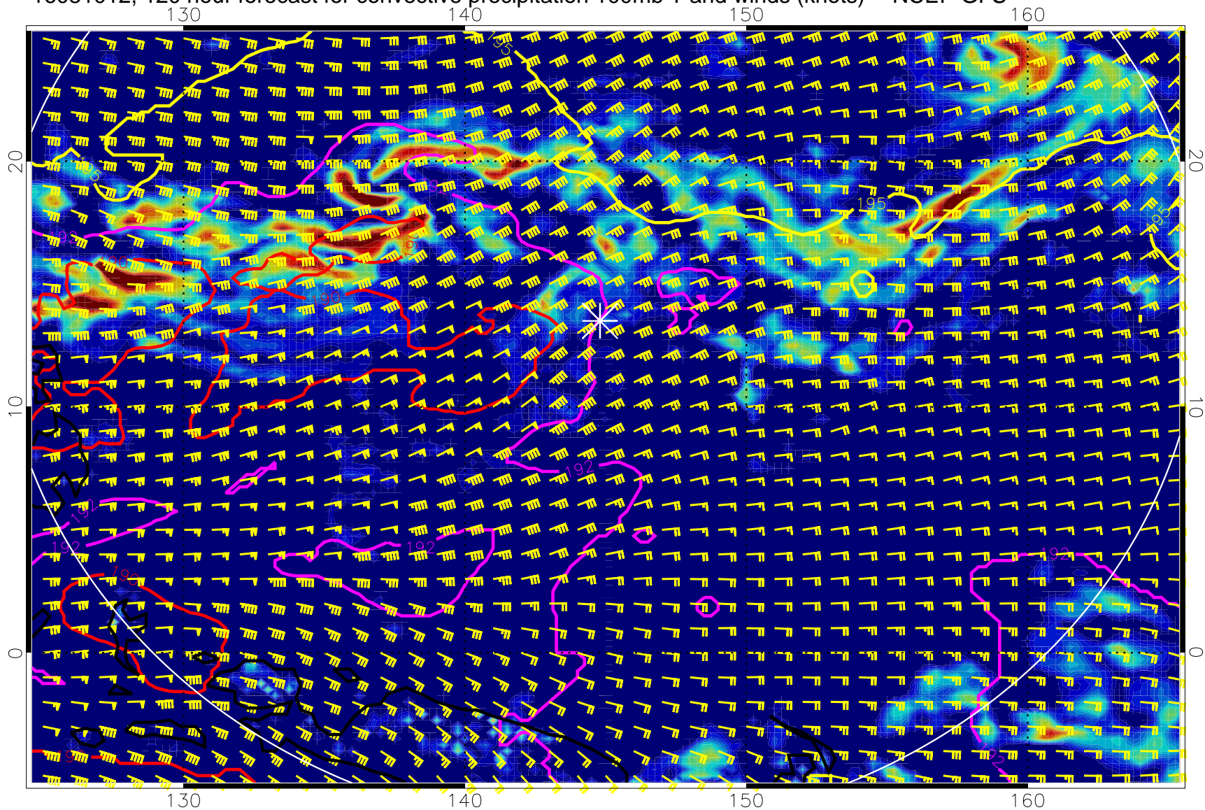
16081012, 120 hour forecast for convective precipitation 100mb T and winds (knots) -- NCEP GFS
