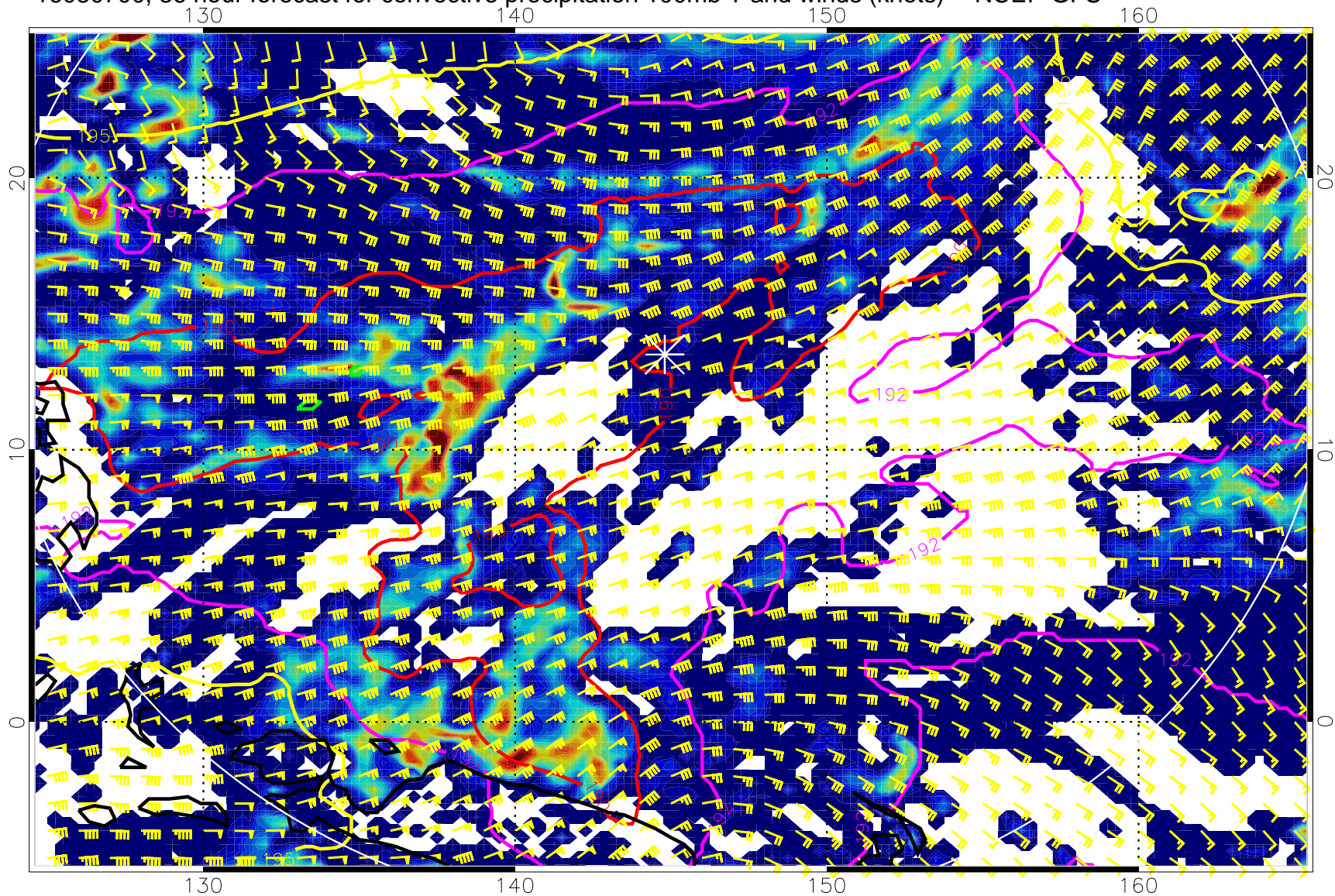
16080700, 36 hour forecast for convective precipitation 100mb T and winds (knots) -- NCEP GFS
