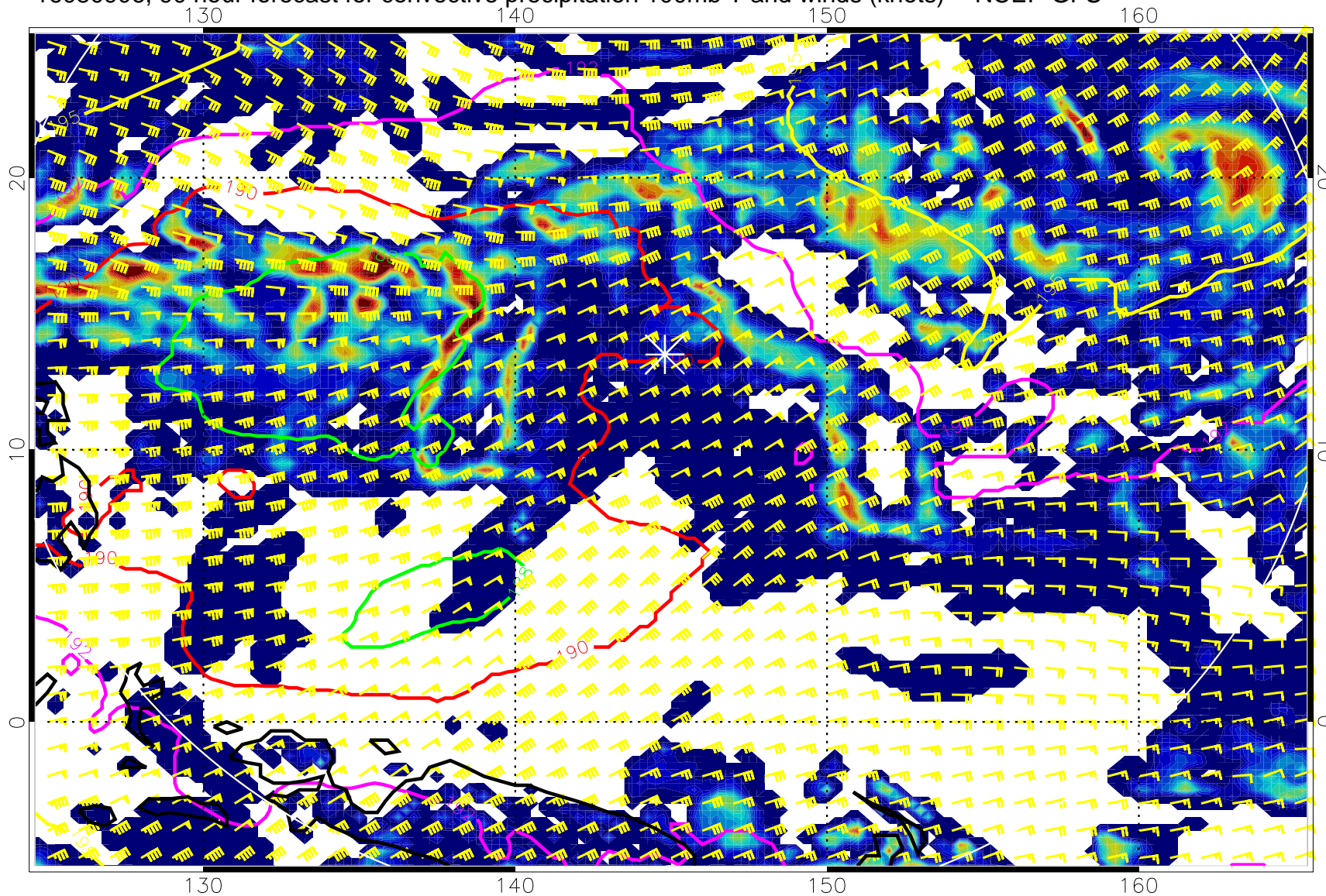
16080906, 90 hour forecast for convective precipitation 100mb T and winds (knots) -- NCEP GFS
