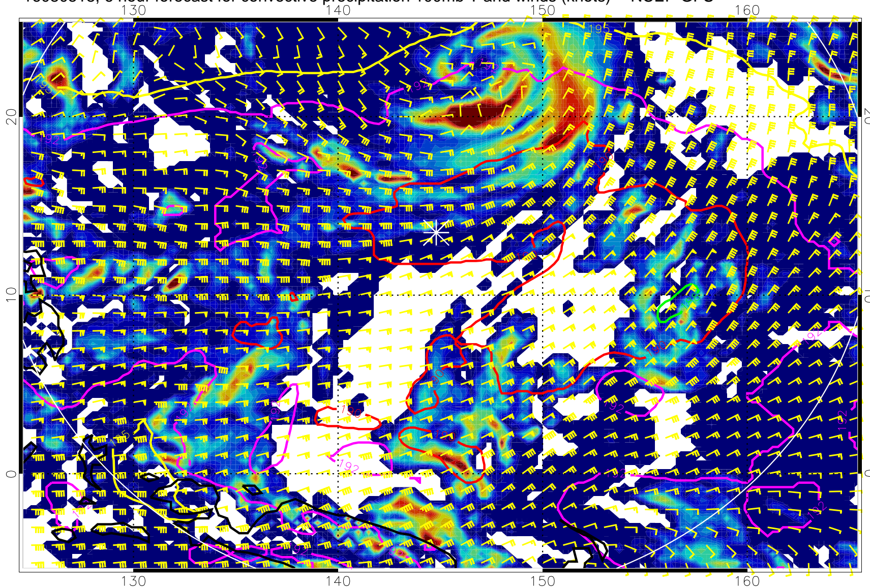
16080518, 6 hour forecast for convective precipitation 100mb T and winds (knots) -- NCEP GFS
