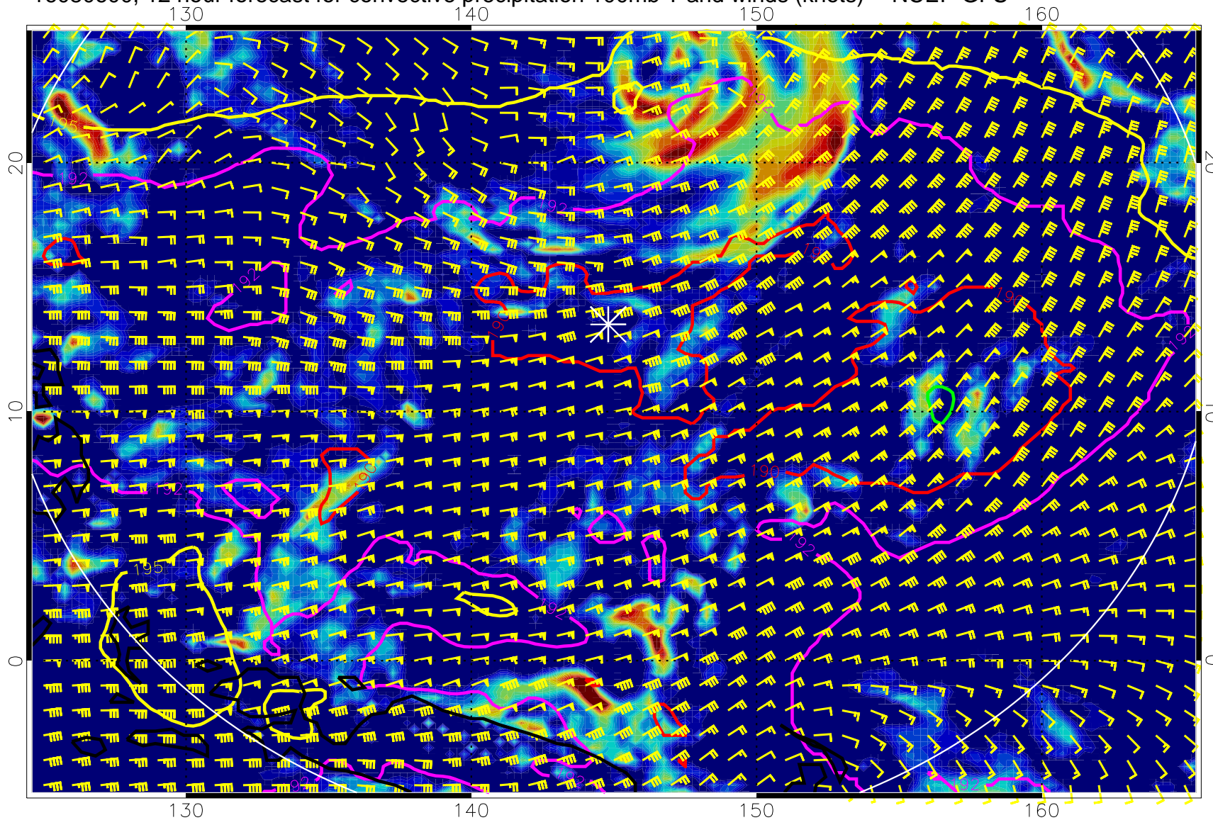
16080600, 12 hour forecast for convective precipitation 100mb T and winds (knots) -- NCEP GFS
