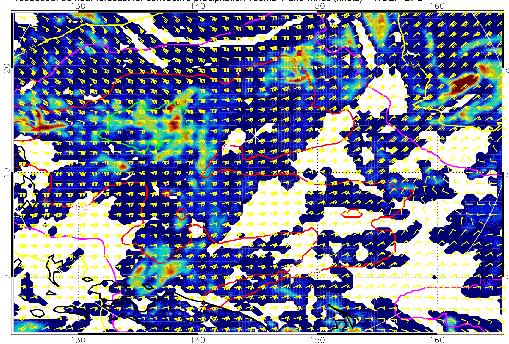
16080806, 66 hour forecast for convective precipitation 100mb T and winds (knots) -- NCEP GFS
