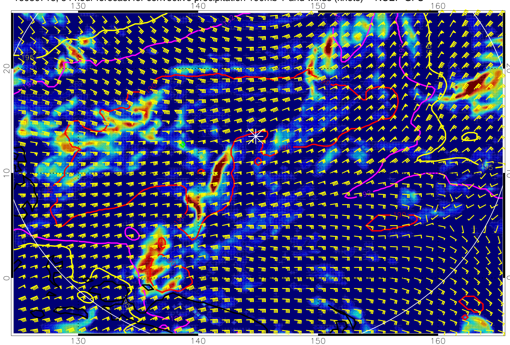
16080718, 54 hour forecast for convective precipitation 100mb T and winds (knots) -- NCEP GFS
