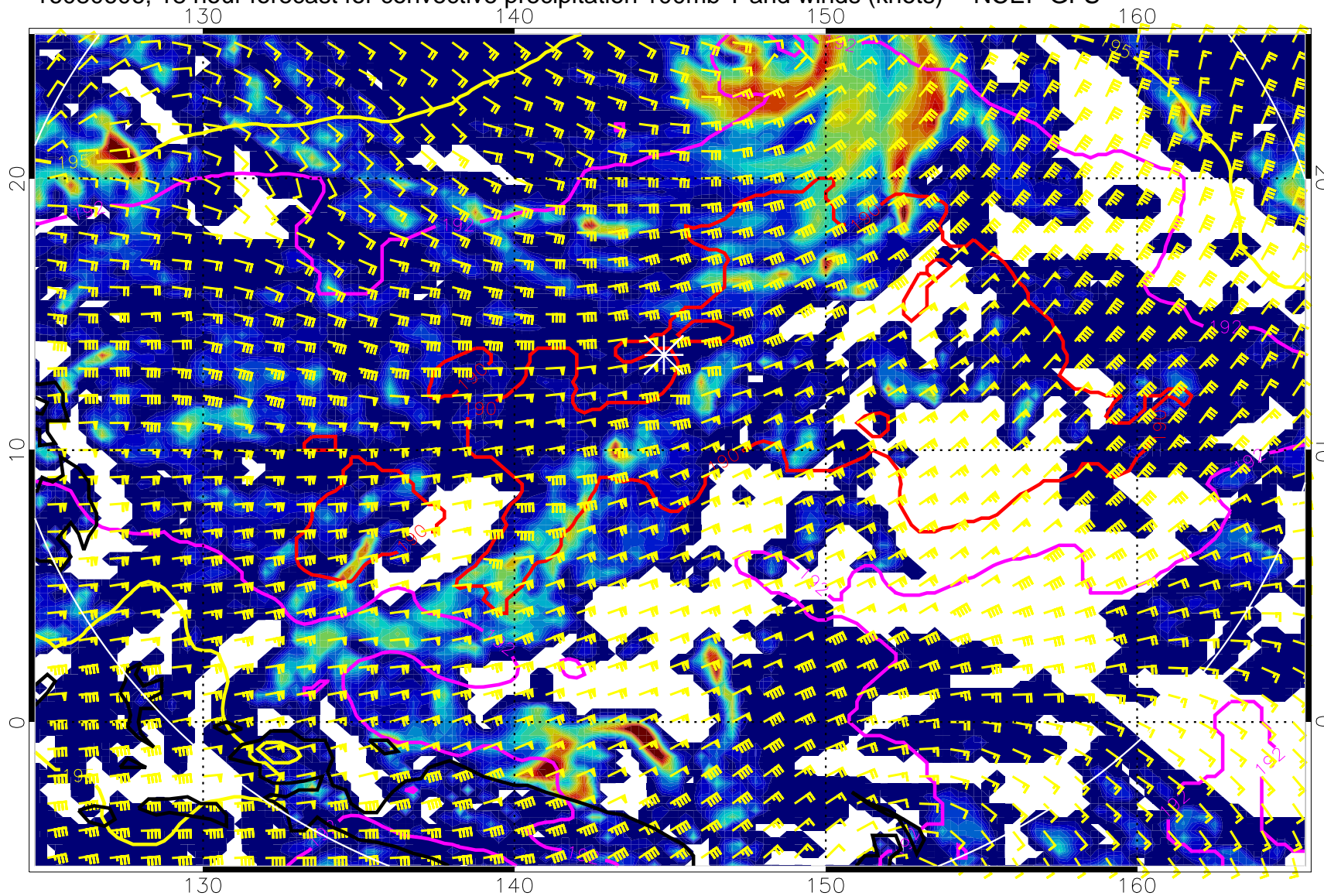
16080606, 18 hour forecast for convective precipitation 100mb T and winds (knots) -- NCEP GFS
