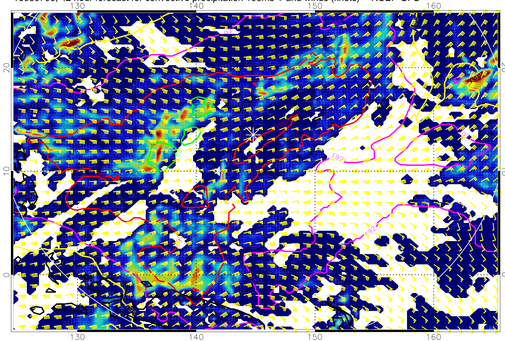
16080706, 42 hour forecast for convective precipitation 100mb T and winds (knots) -- NCEP GFS
