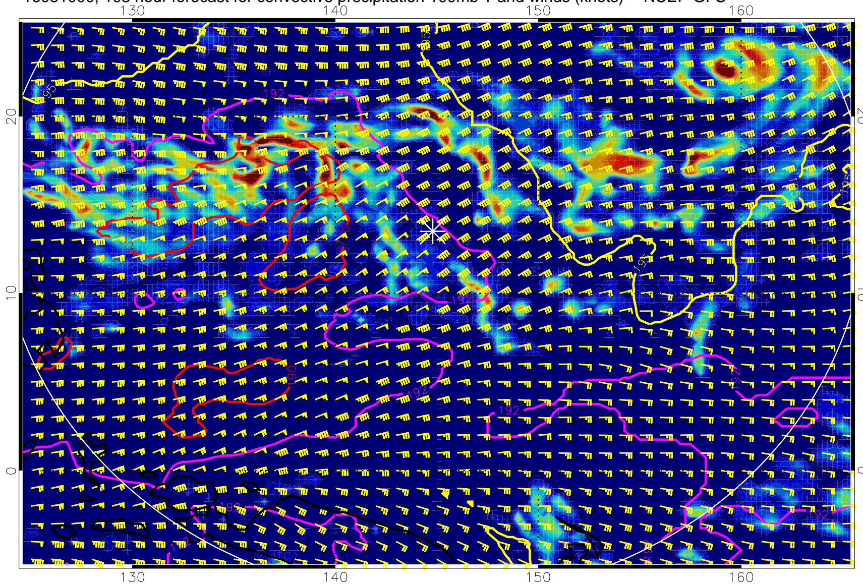
16081000, 108 hour forecast for convective precipitation 100mb T and winds (knots) -- NCEP GFS
