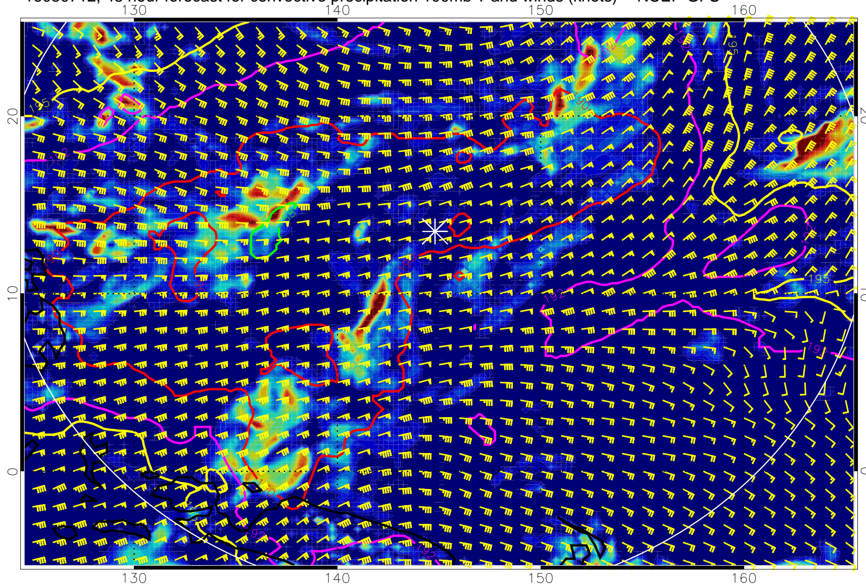
16080712, 48 hour forecast for convective precipitation 100mb T and winds (knots) -- NCEP GFS
