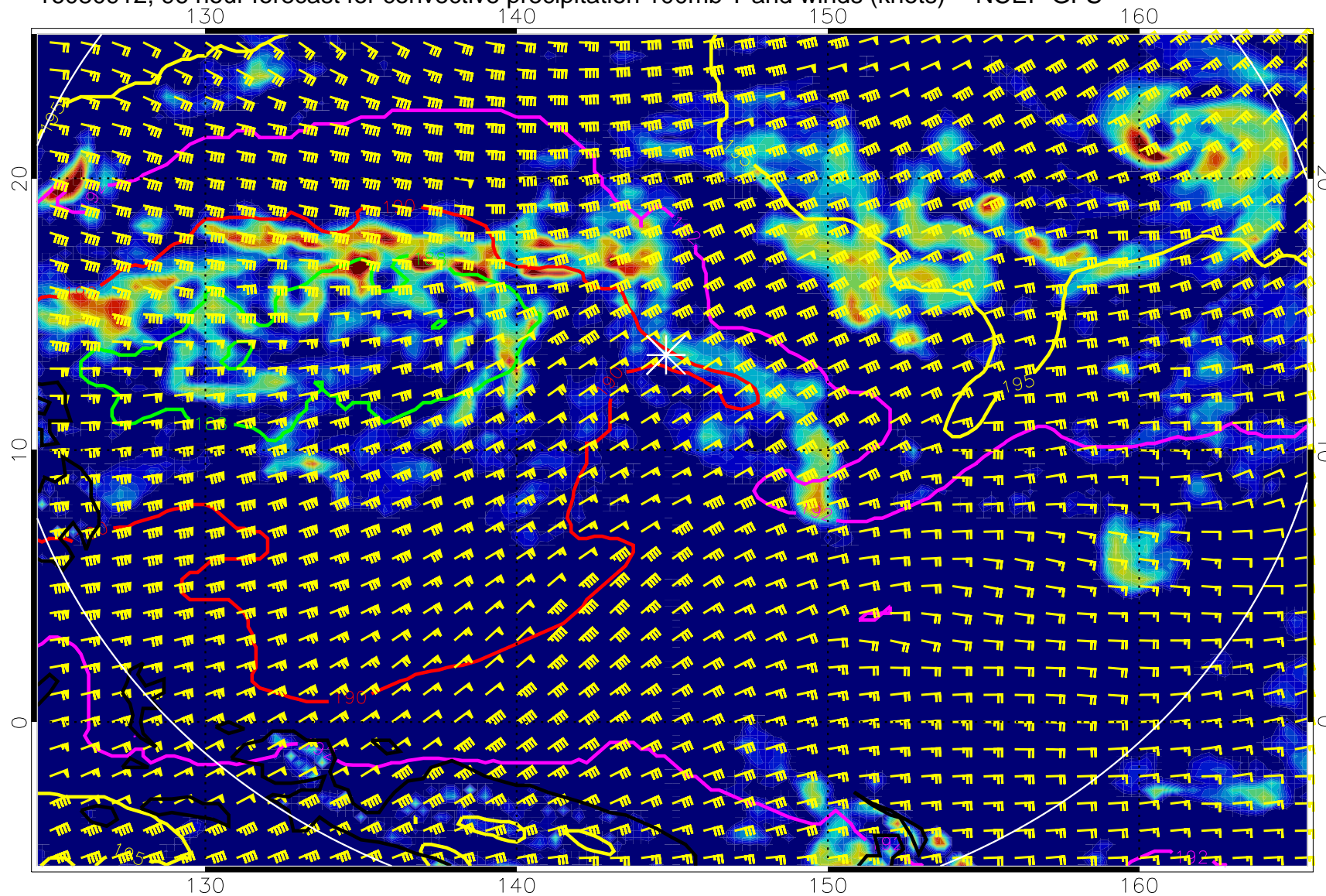
16080912, 96 hour forecast for convective precipitation 100mb T and winds (knots) -- NCEP GFS
