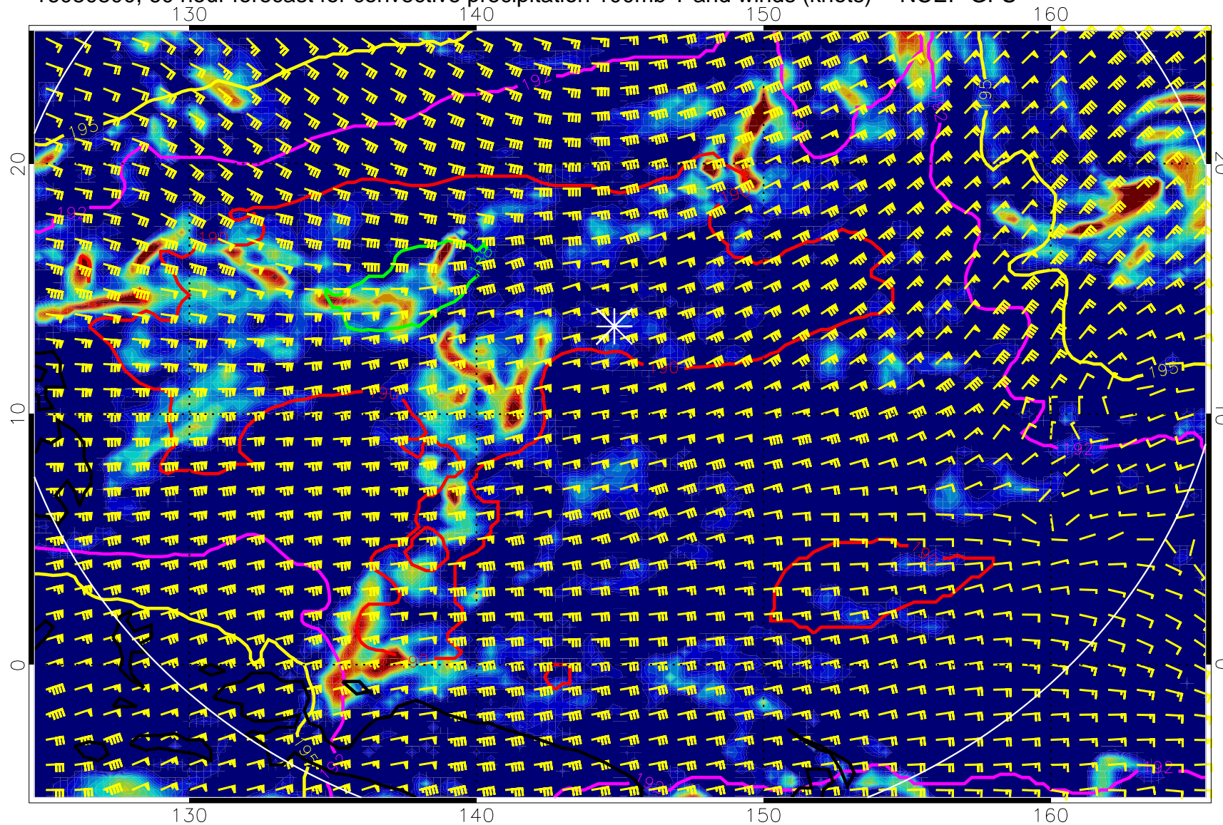
16080800, 60 hour forecast for convective precipitation 100mb T and winds (knots) -- NCEP GFS
