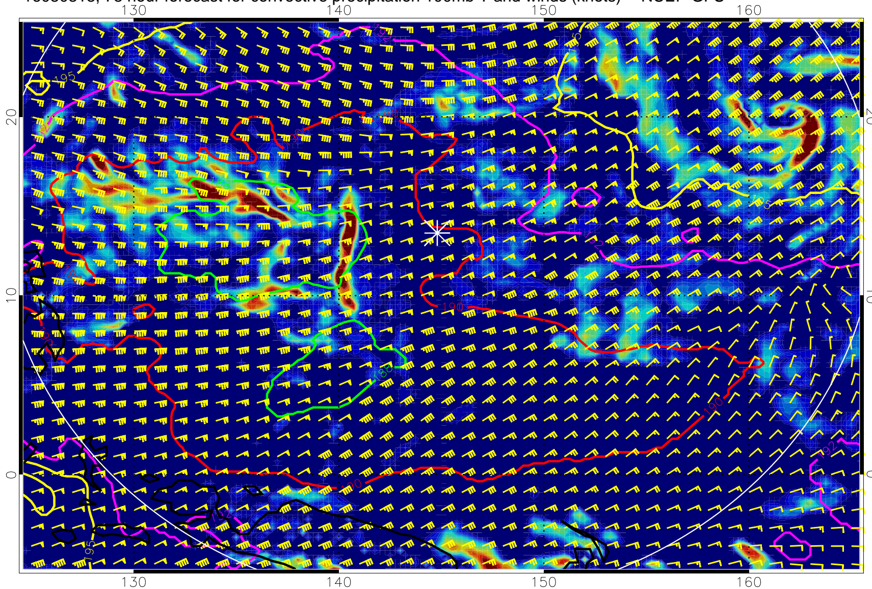
16080818, 78 hour forecast for convective precipitation 100mb T and winds (knots) -- NCEP GFS
