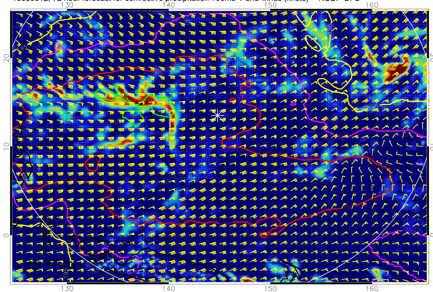
16080812, 72 hour forecast for convective precipitation 100mb T and winds (knots) -- NCEP GFS
