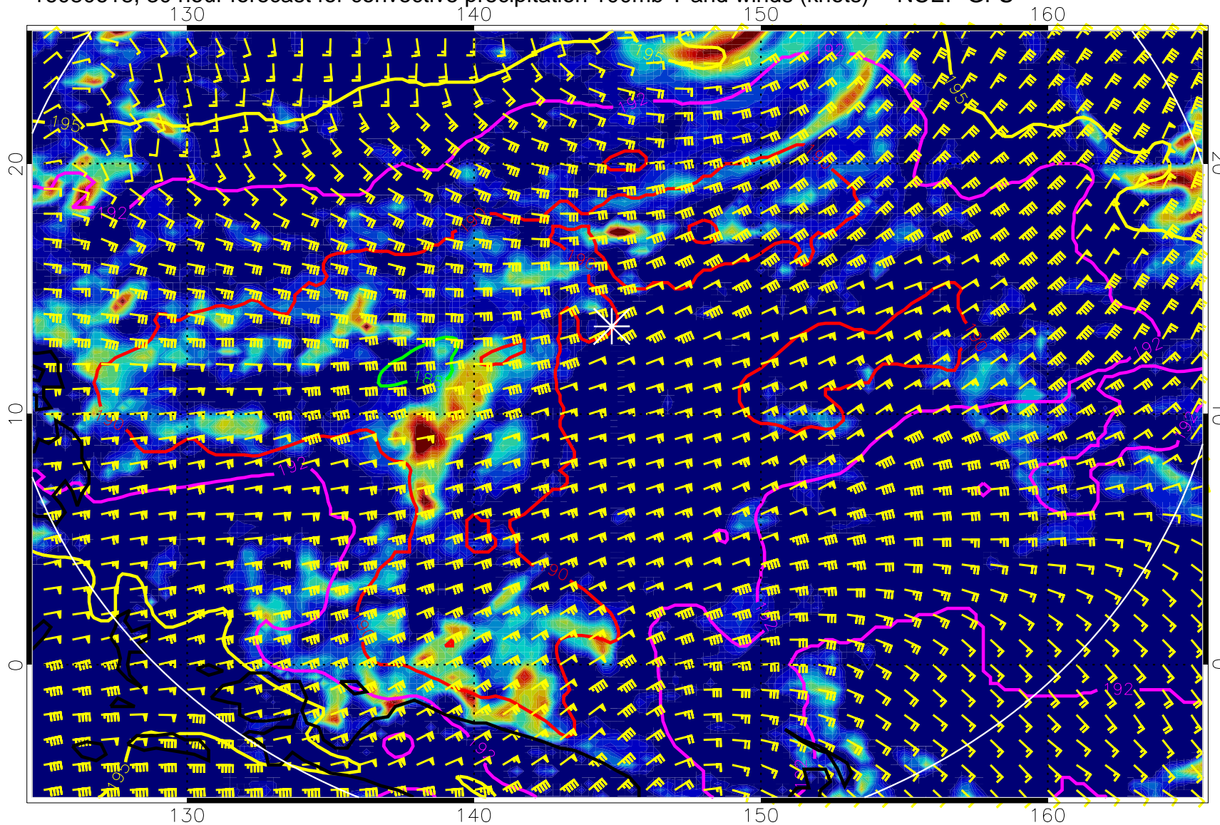
16080618, 30 hour forecast for convective precipitation 100mb T and winds (knots) -- NCEP GFS
