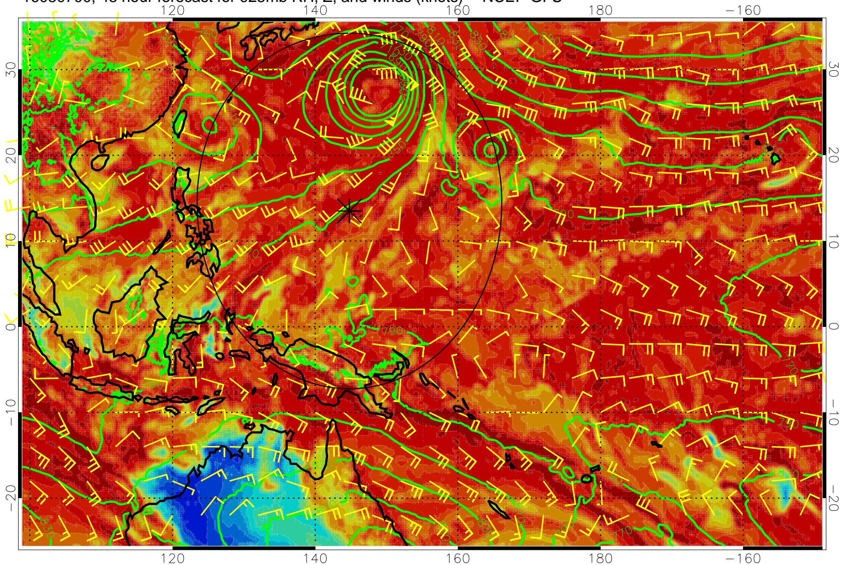
16080700, 48 hour forecast for 925mb RH, Z, and winds (knots) -- NCEP GFS
