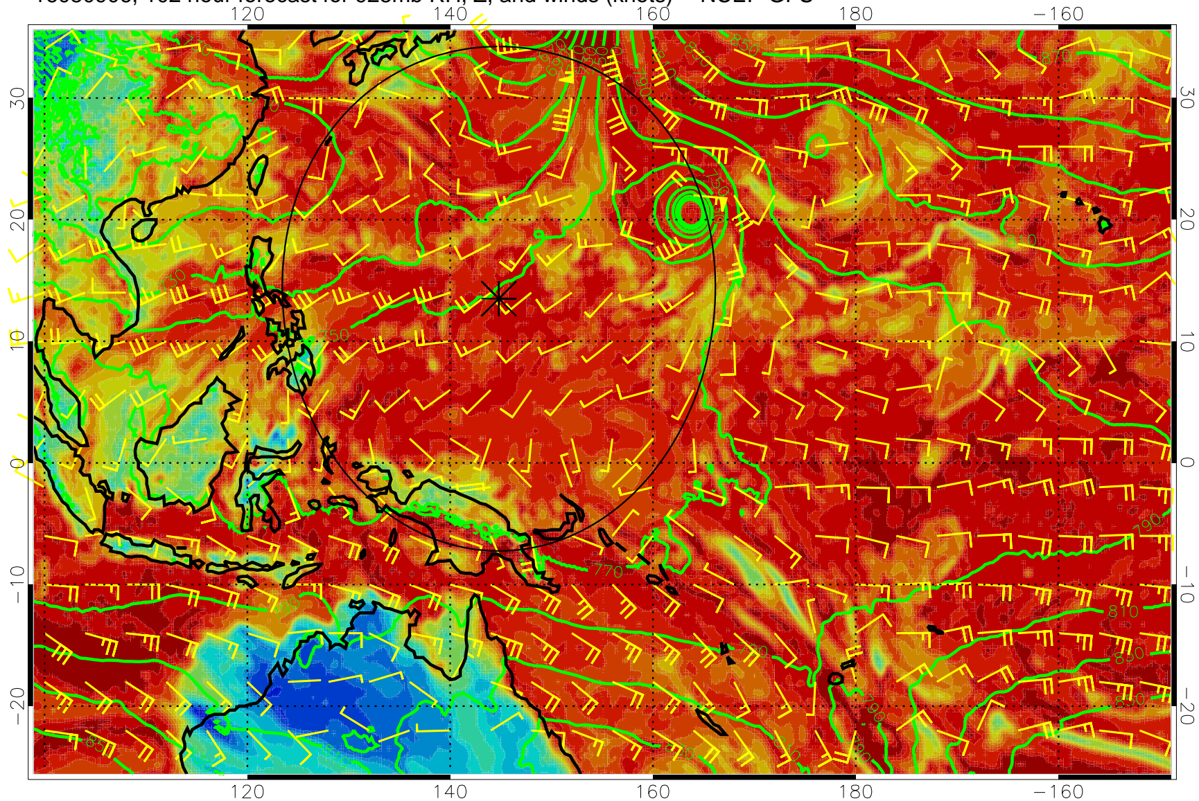
16080906, 102 hour forecast for 925mb RH, Z, and winds (knots) -- NCEP GFS
