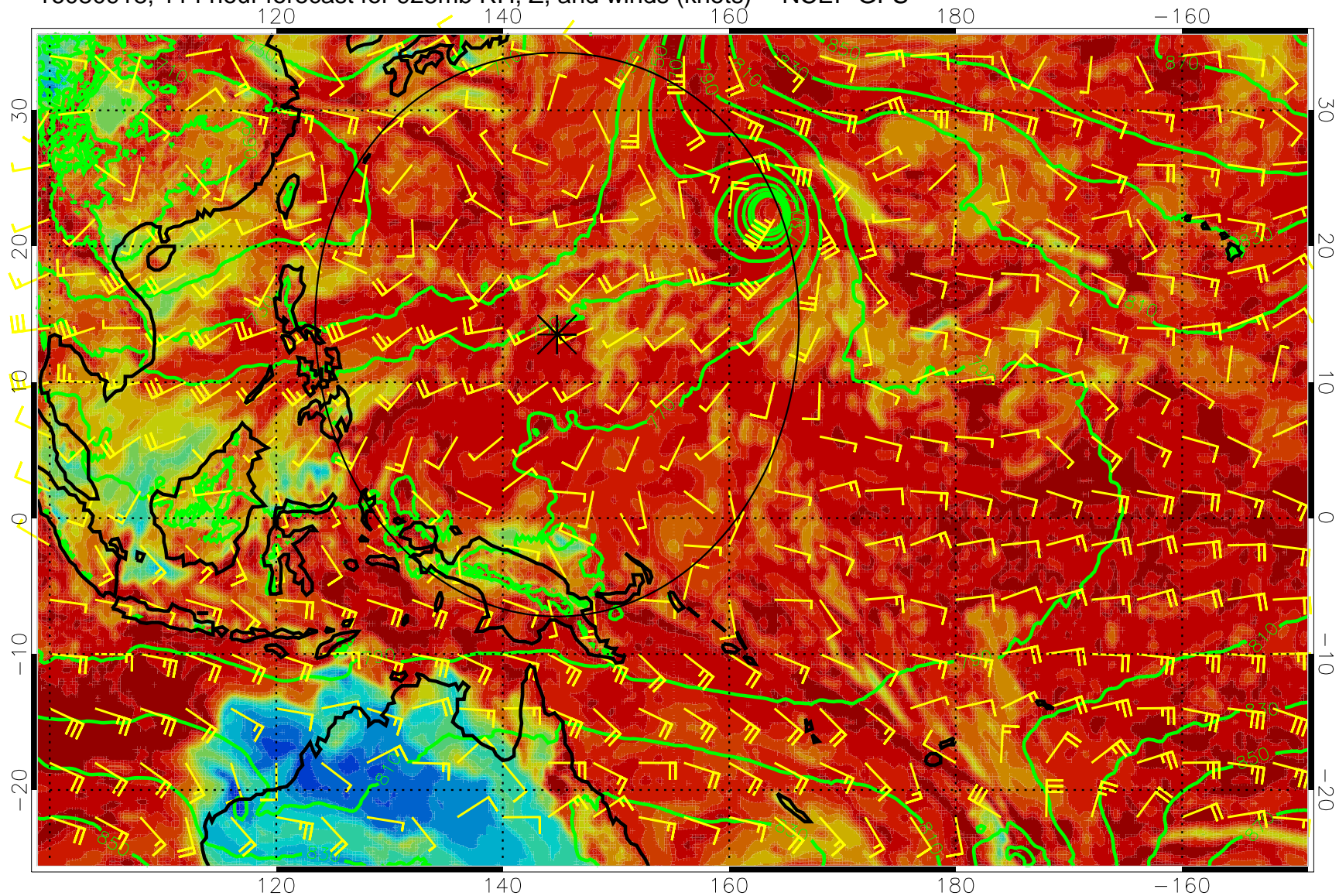
16080918, 114 hour forecast for 925mb RH, Z, and winds (knots) -- NCEP GFS
