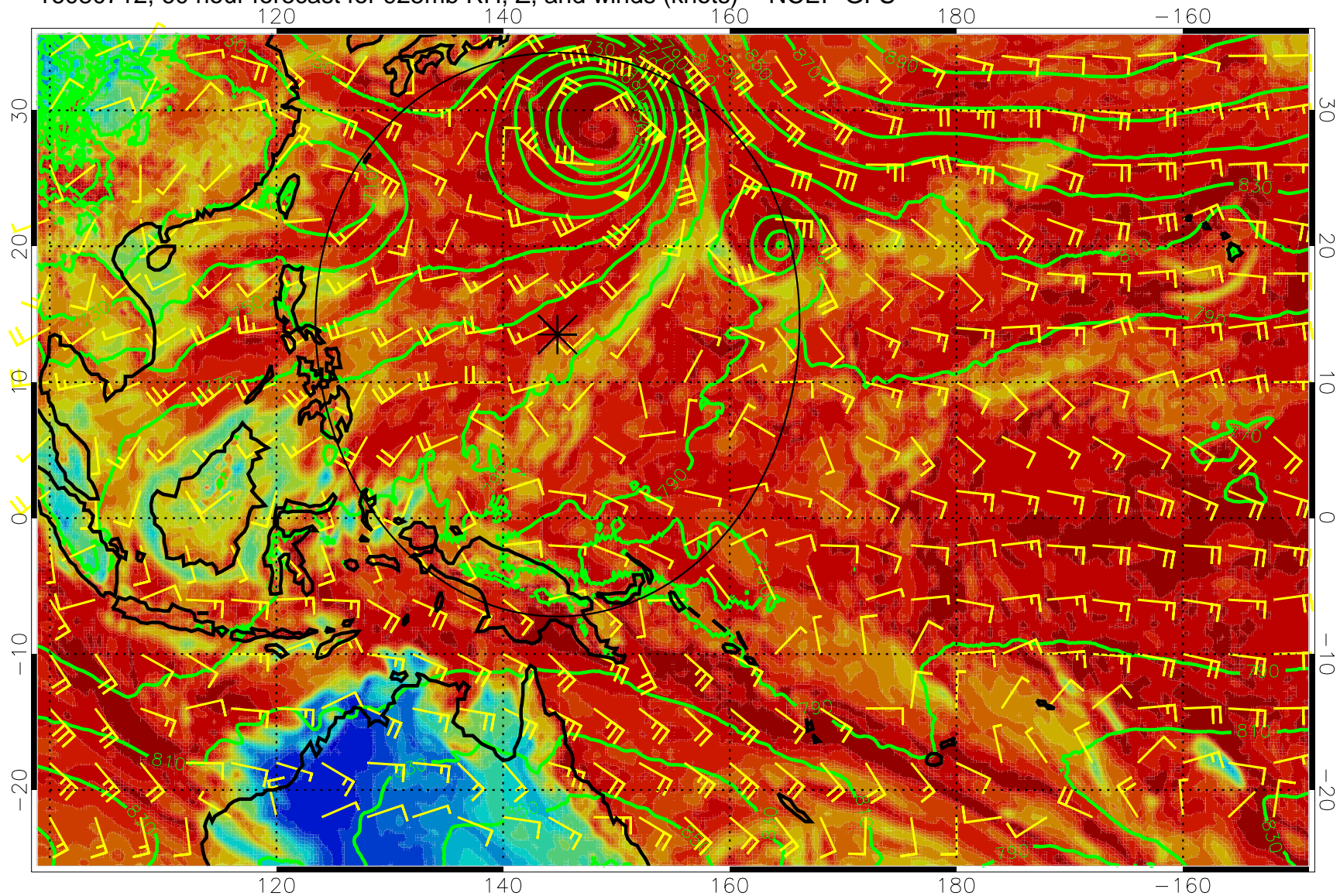
16080712, 60 hour forecast for 925mb RH, Z, and winds (knots) -- NCEP GFS
