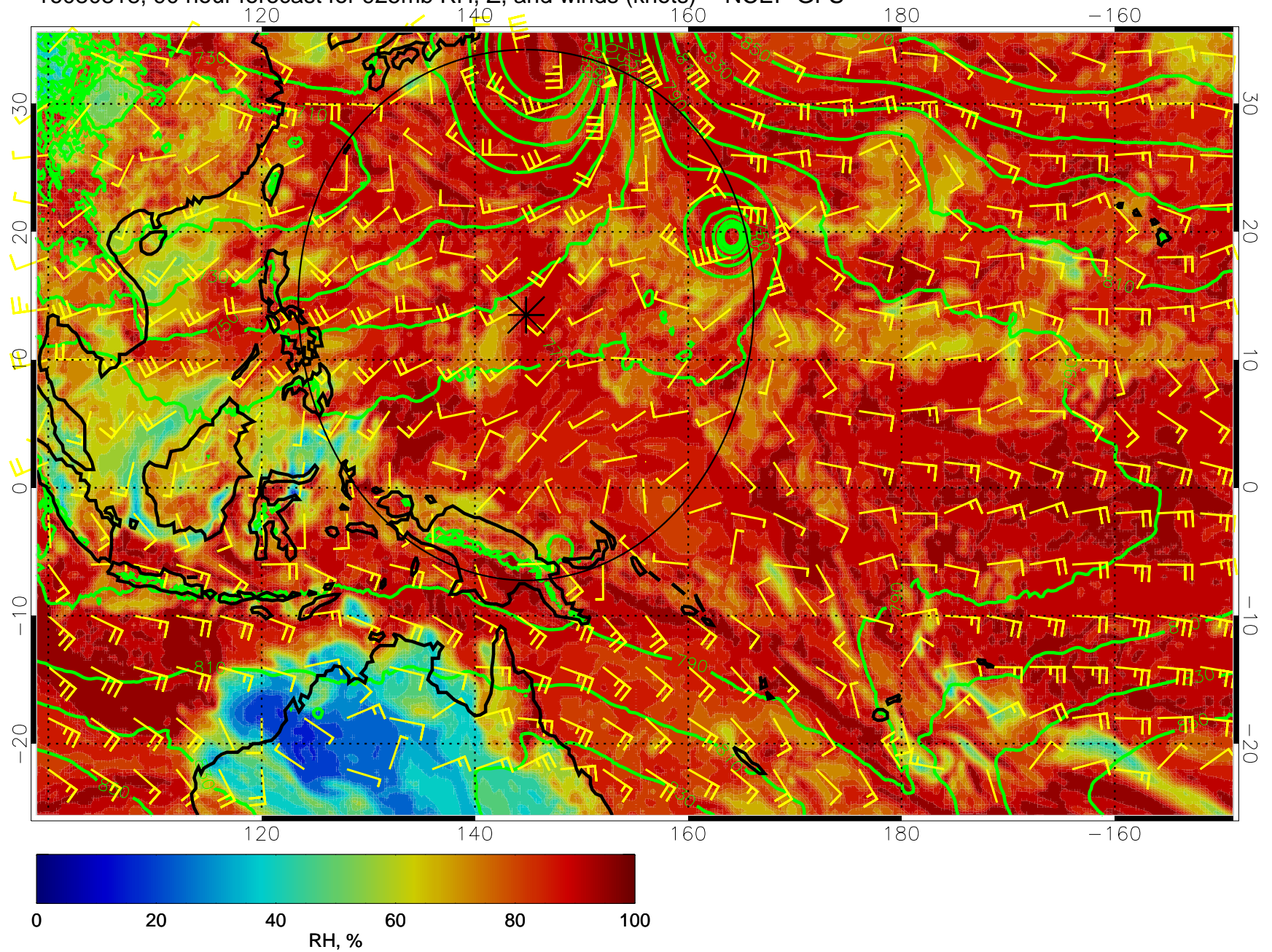
16080818, 90 hour forecast for 925mb RH, Z, and winds (knots) -- NCEP GFS
