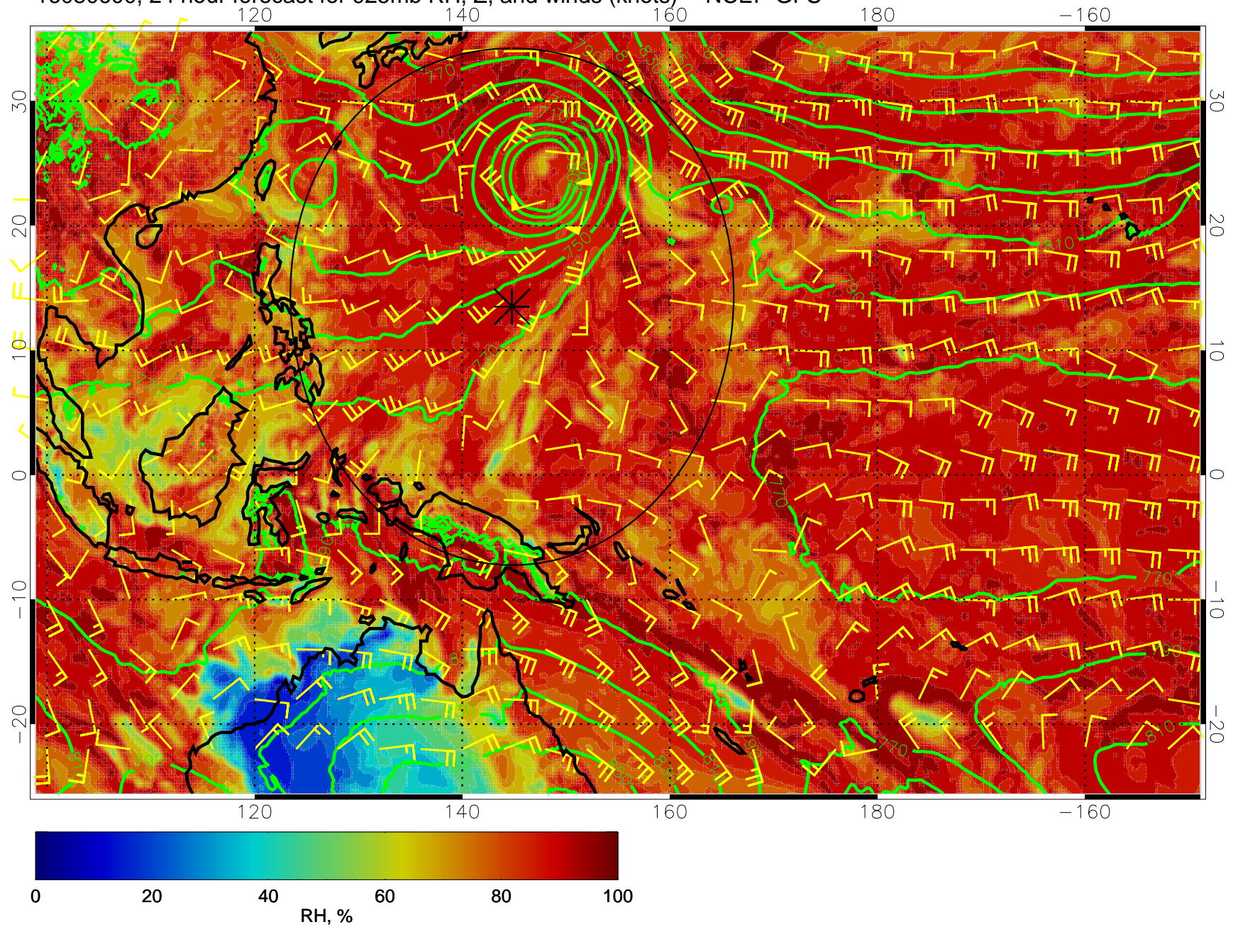
16080600, 24 hour forecast for 925mb RH, Z, and winds (knots) -- NCEP GFS
