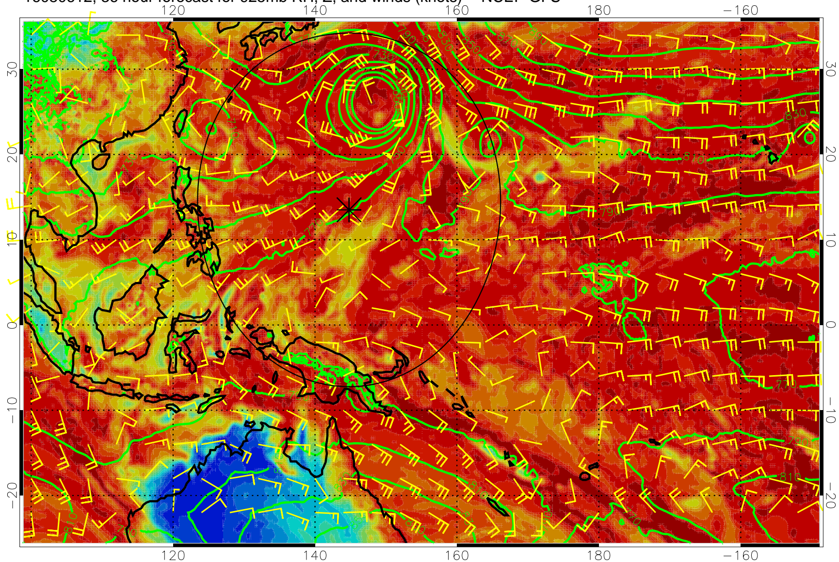
16080612, 36 hour forecast for 925mb RH, Z, and winds (knots) -- NCEP GFS
