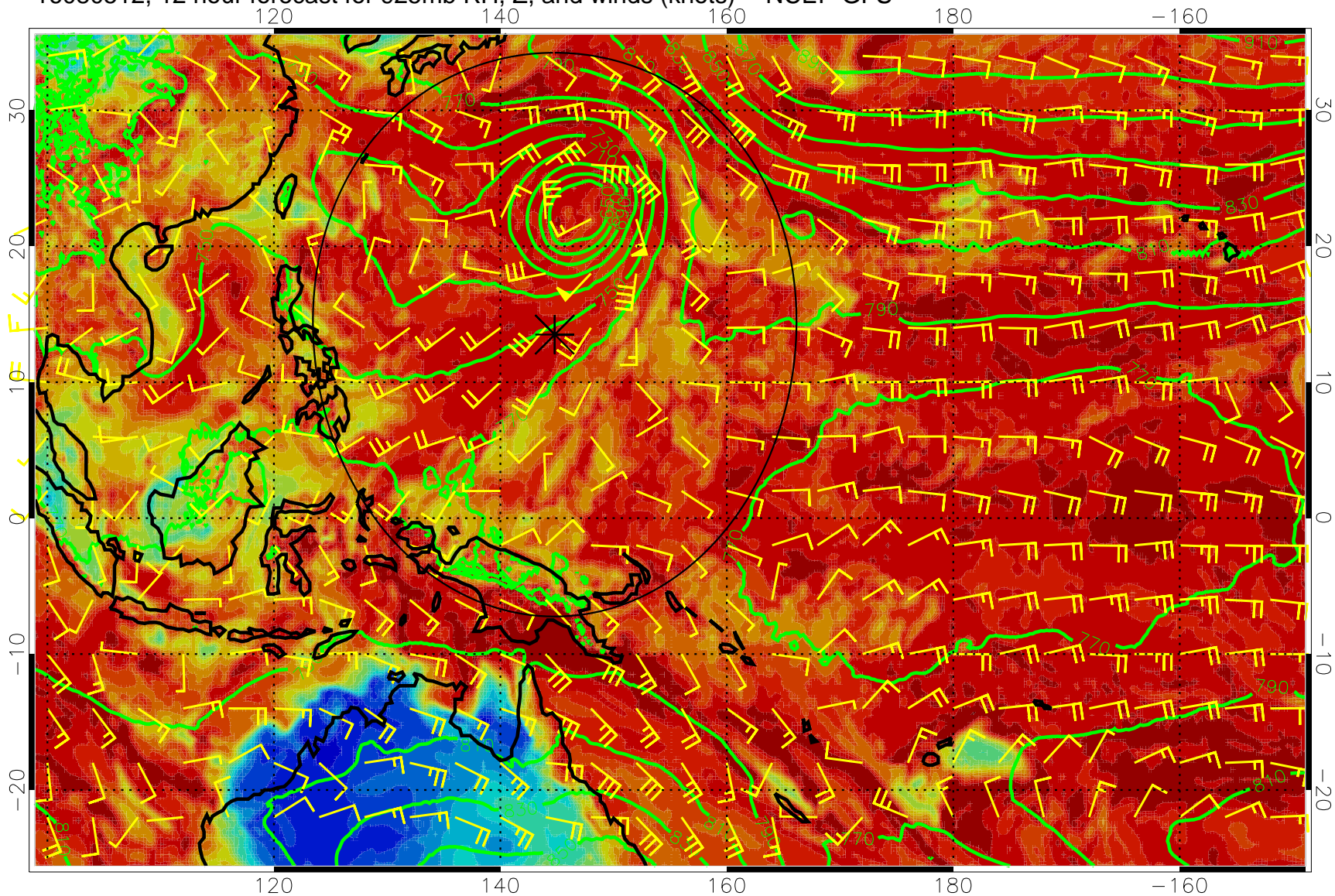
16080512, 12 hour forecast for 925mb RH, Z, and winds (knots) -- NCEP GFS
