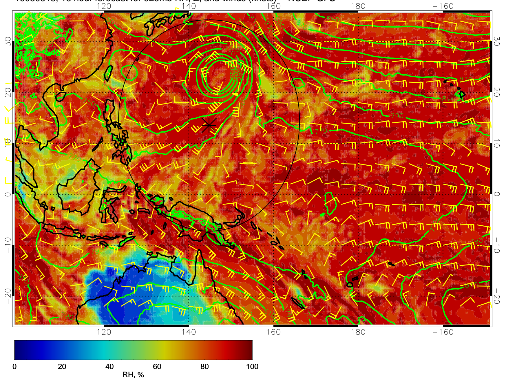
16080518, 18 hour forecast for 925mb RH, Z, and winds (knots) -- NCEP GFS
