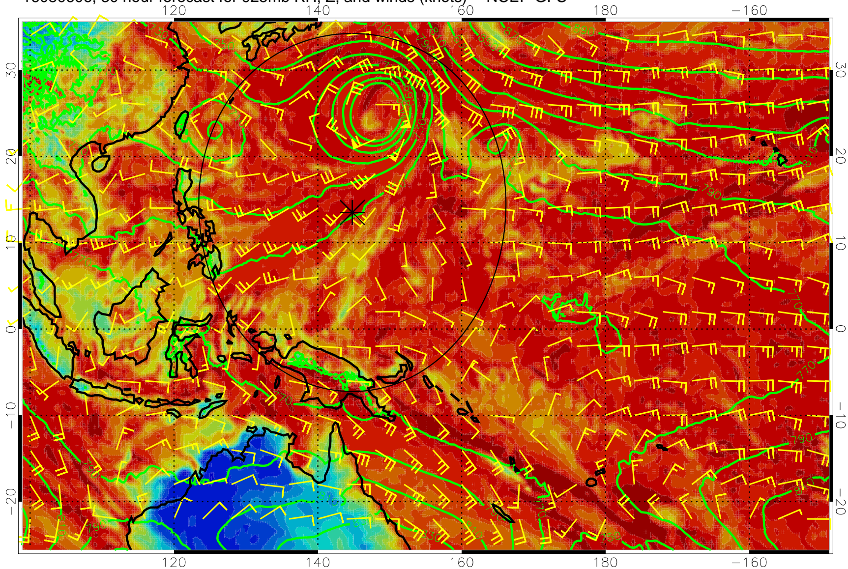
16080606, 30 hour forecast for 925mb RH, Z, and winds (knots) -- NCEP GFS
