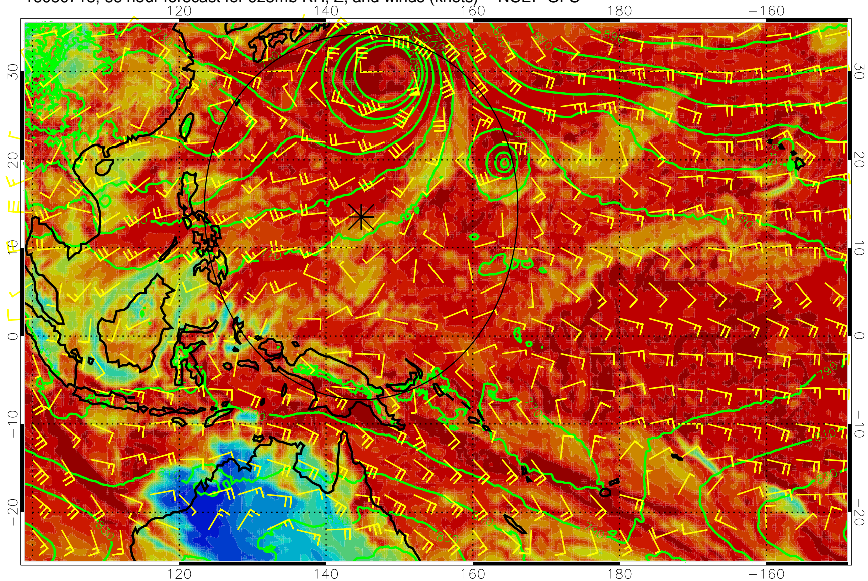
16080718, 66 hour forecast for 925mb RH, Z, and winds (knots) -- NCEP GFS
