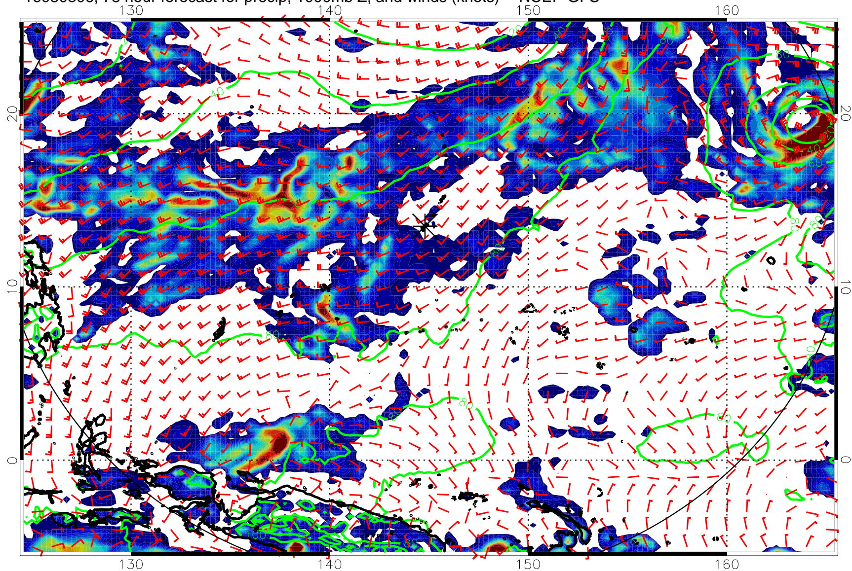
16080806, 78 hour forecast for precip, 1000mb Z, and winds (knots) -- NCEP GFS
