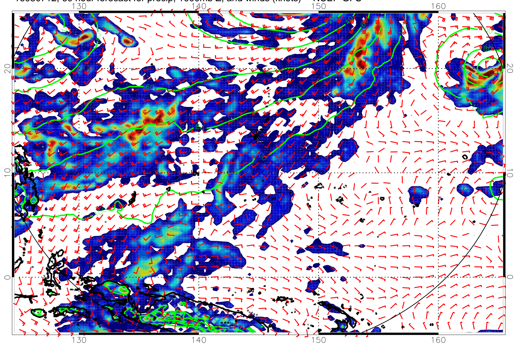
16080712, 60 hour forecast for precip, 1000mb Z, and winds (knots) -- NCEP GFS
