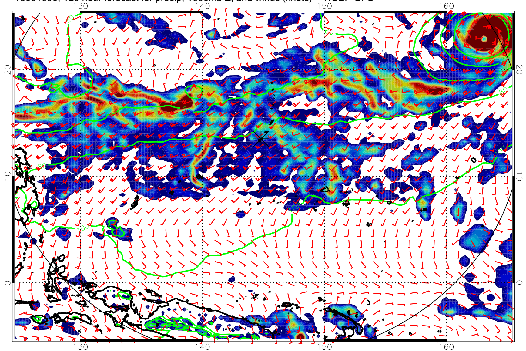
16081000, 120 hour forecast for precip, 1000mb Z, and winds (knots) -- NCEP GFS
