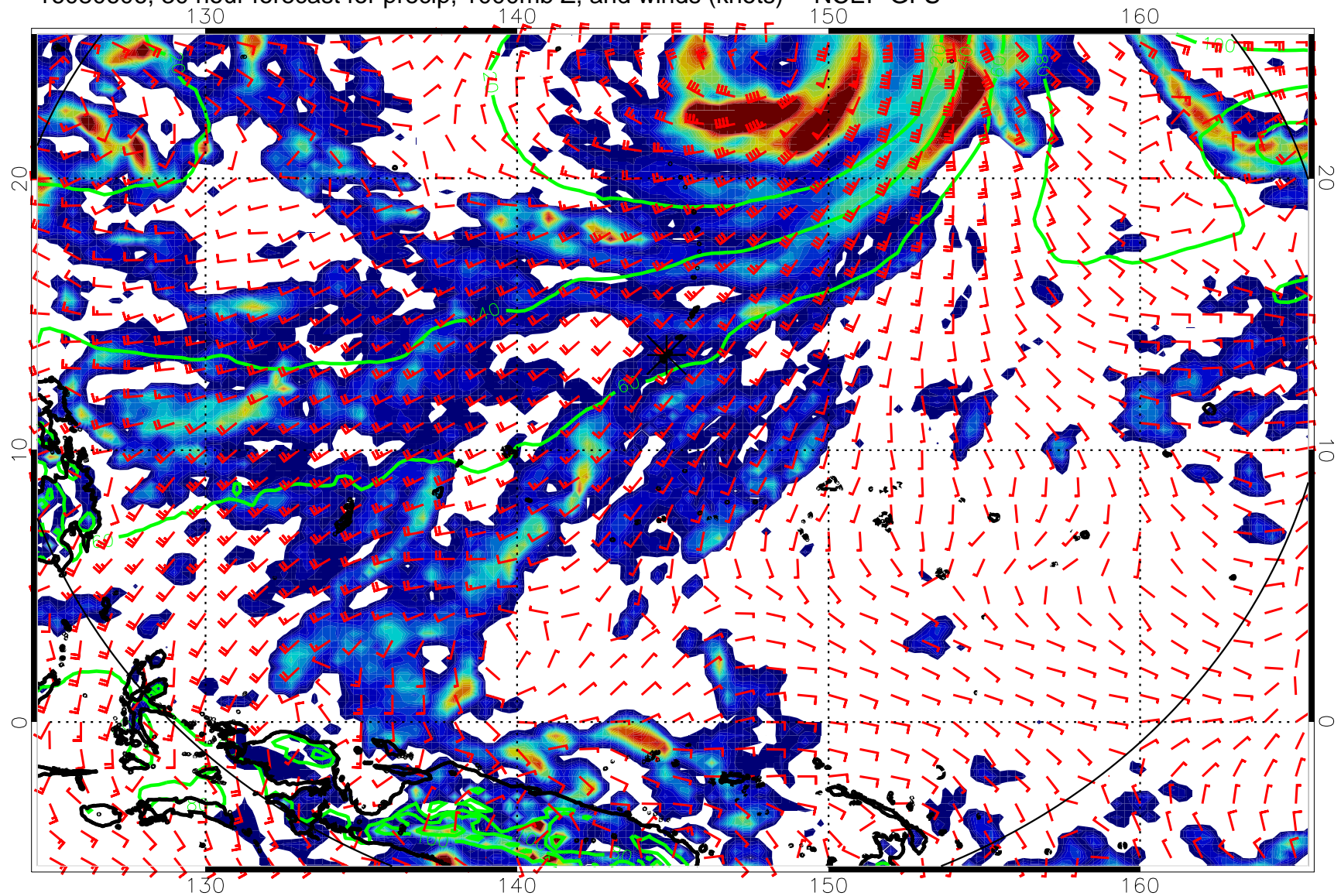
16080606, 30 hour forecast for precip, 1000mb Z, and winds (knots) -- NCEP GFS
