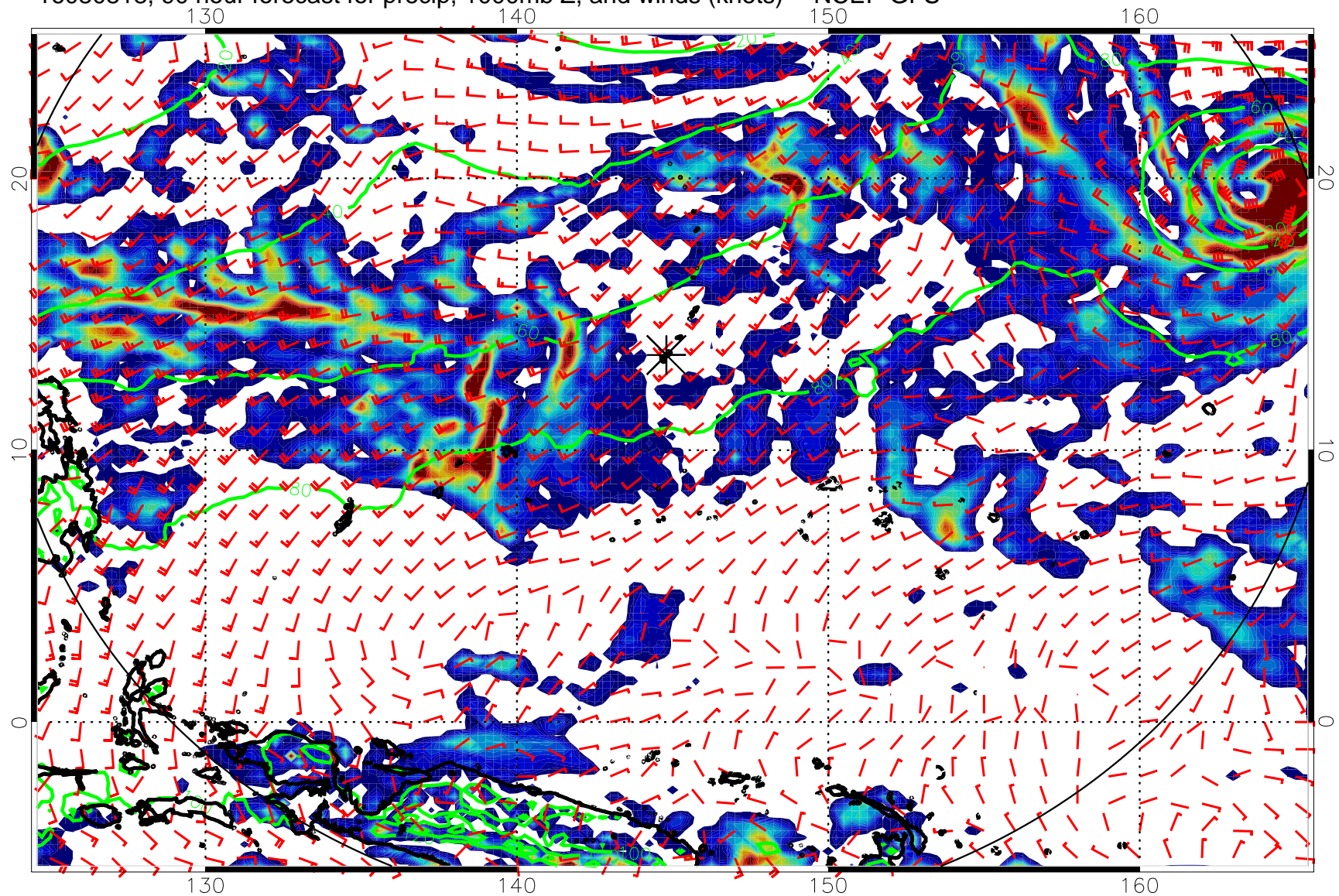
16080818, 90 hour forecast for precip, 1000mb Z, and winds (knots) -- NCEP GFS
