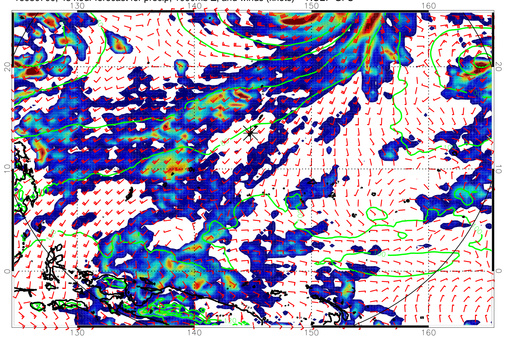
16080700, 48 hour forecast for precip, 1000mb Z, and winds (knots) -- NCEP GFS
