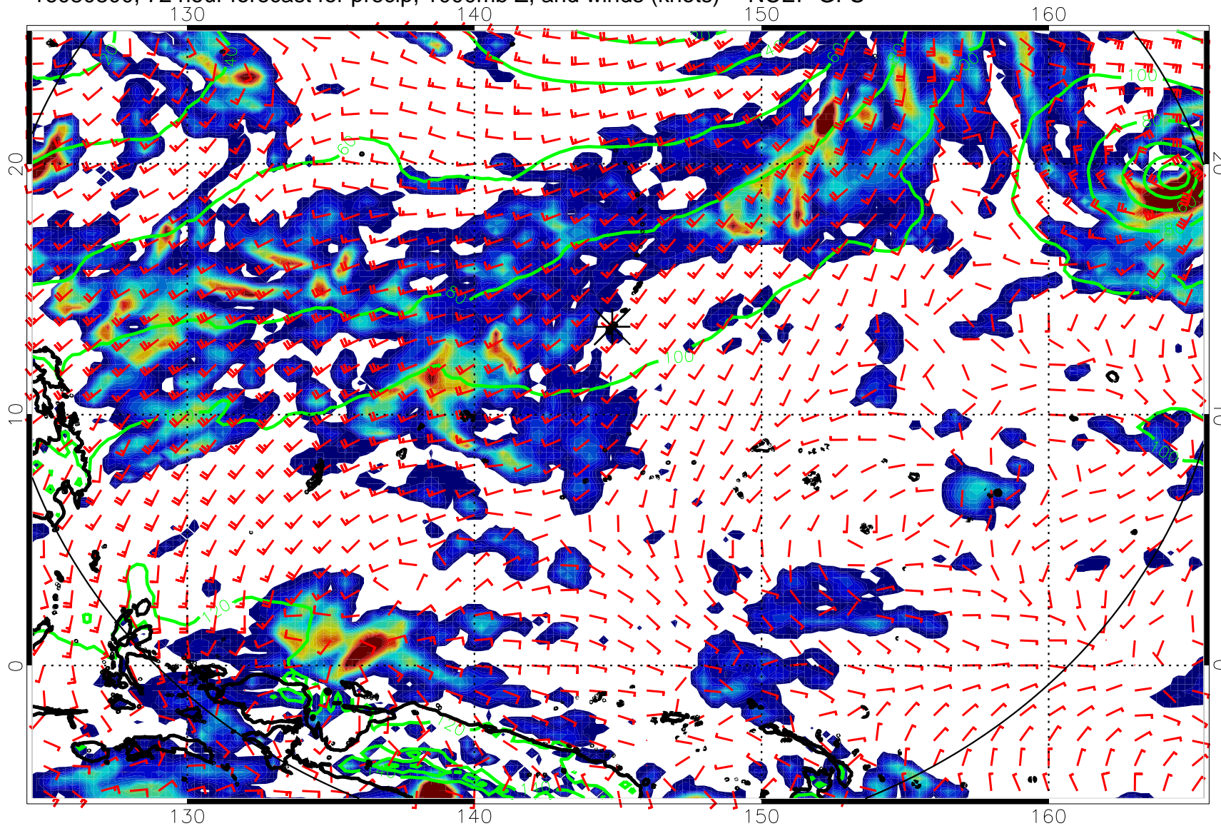
16080800, 72 hour forecast for precip, 1000mb Z, and winds (knots) -- NCEP GFS
