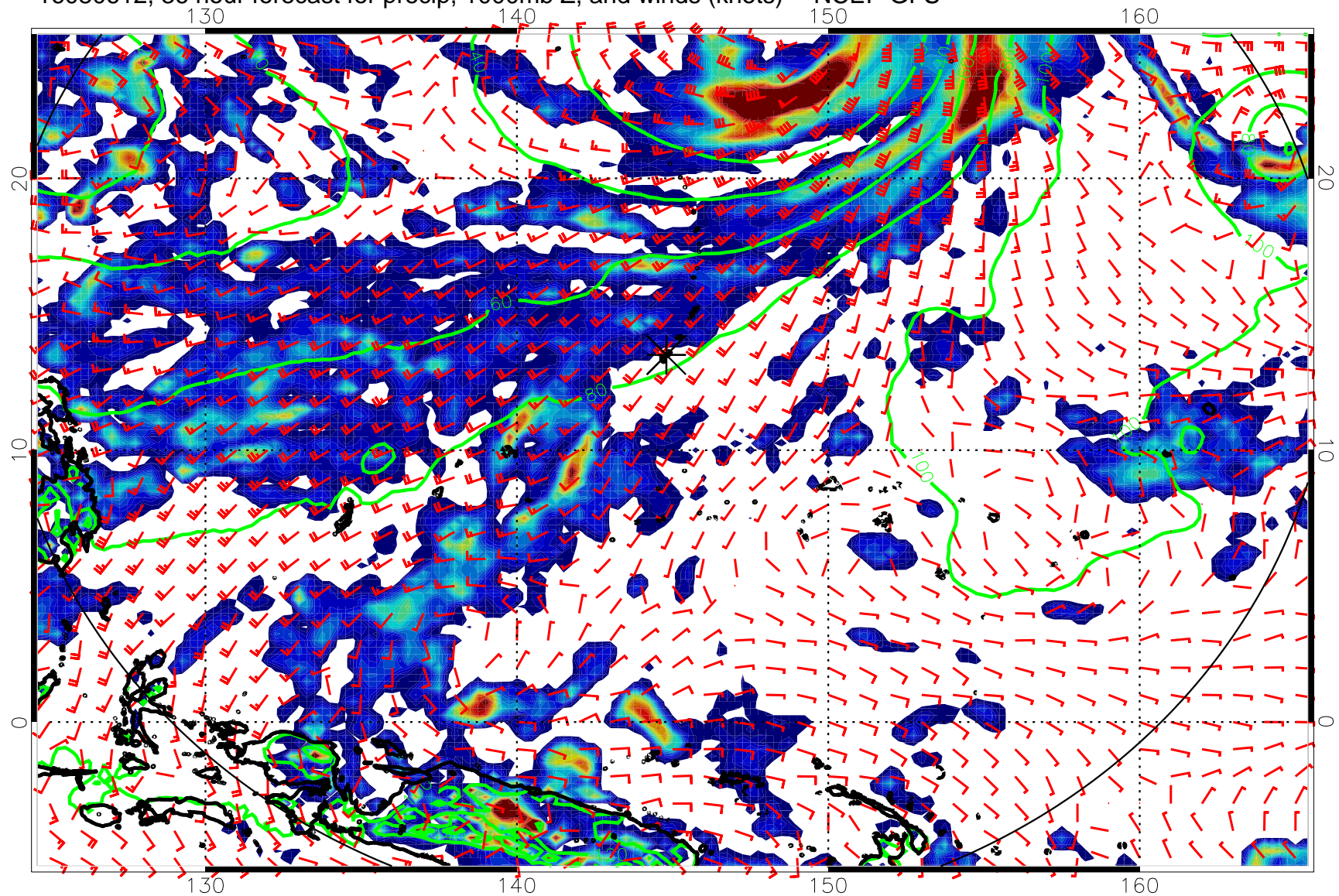
16080612, 36 hour forecast for precip, 1000mb Z, and winds (knots) -- NCEP GFS
