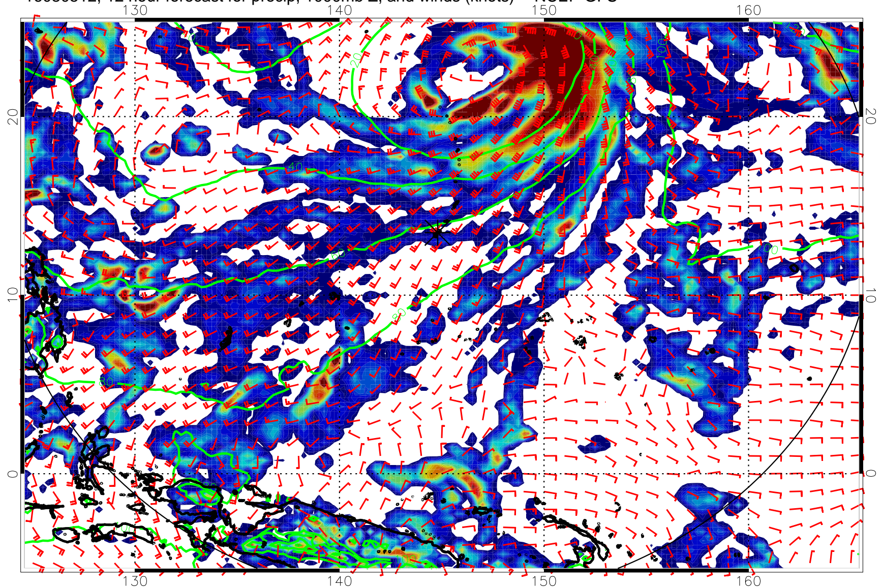
16080512, 12 hour forecast for precip, 1000mb Z, and winds (knots) -- NCEP GFS
