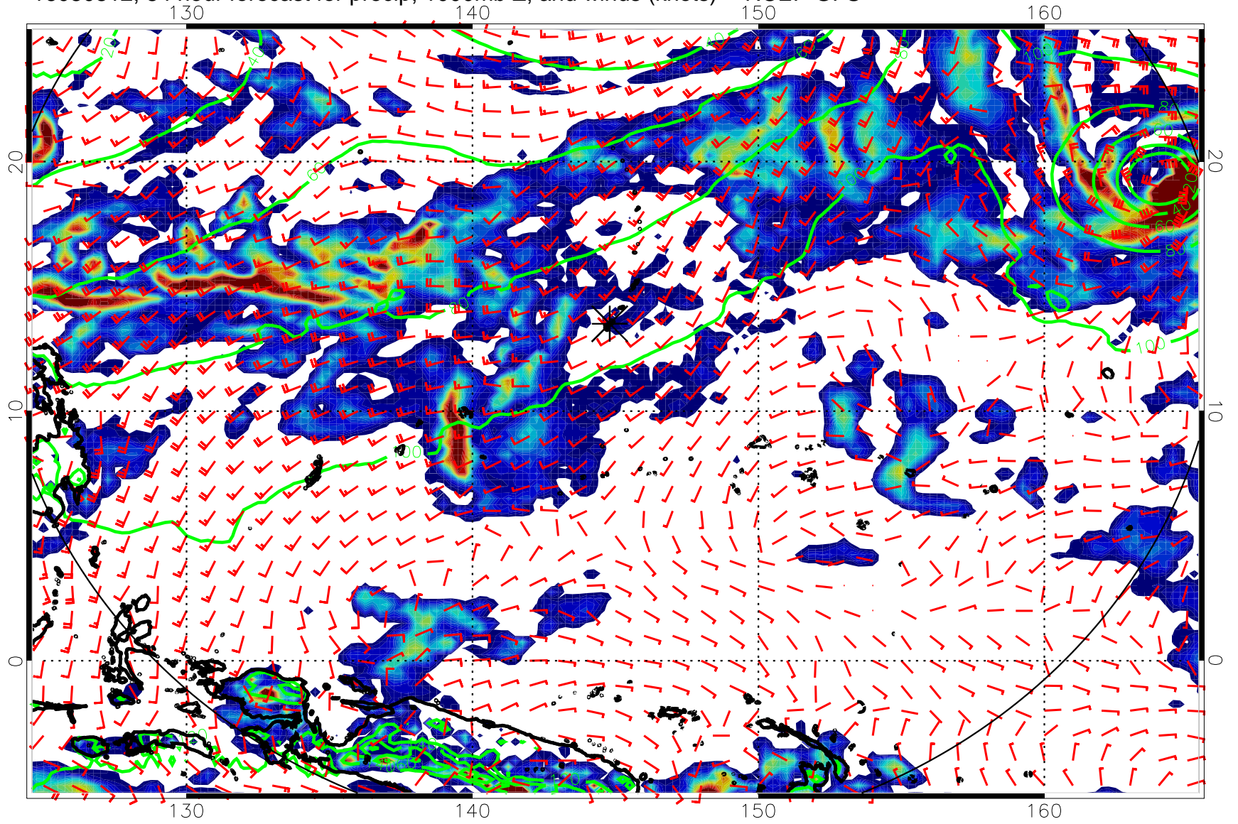
16080812, 84 hour forecast for precip, 1000mb Z, and winds (knots) -- NCEP GFS
