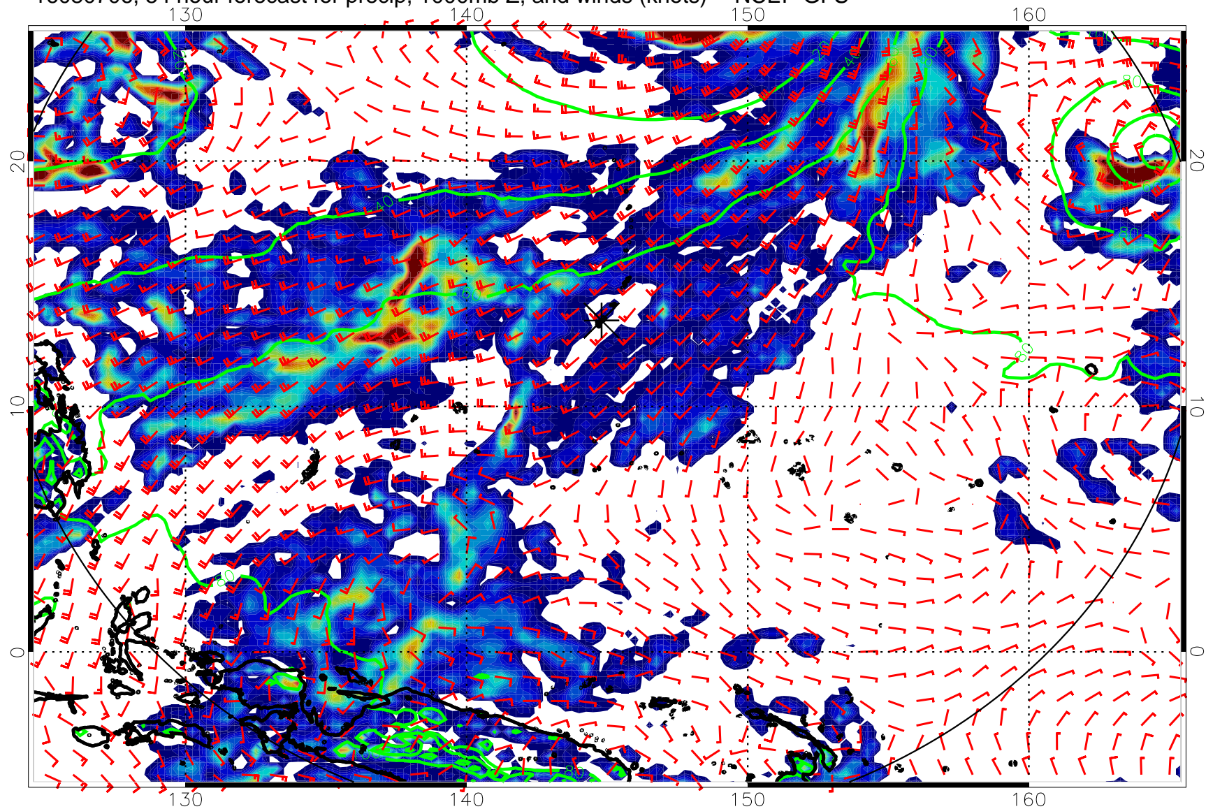
16080706, 54 hour forecast for precip, 1000mb Z, and winds (knots) -- NCEP GFS
