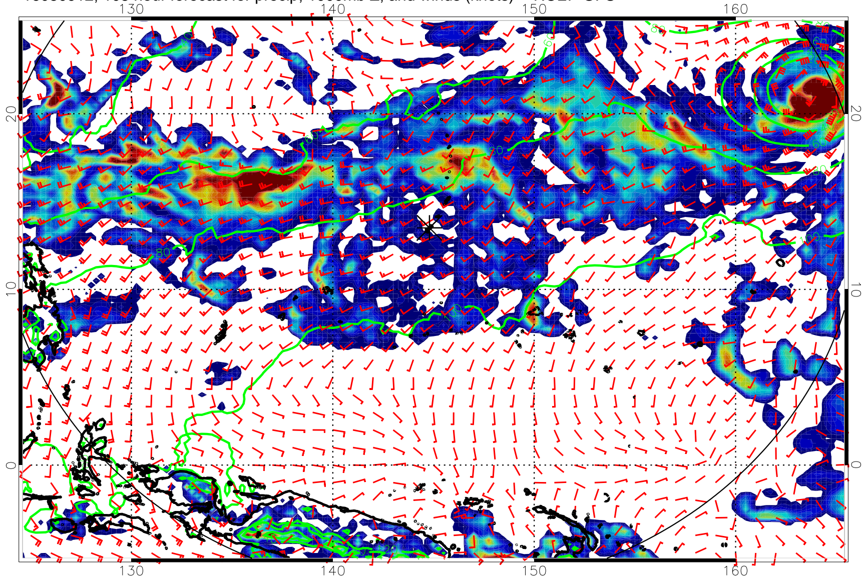
16080912, 108 hour forecast for precip, 1000mb Z, and winds (knots) -- NCEP GFS
