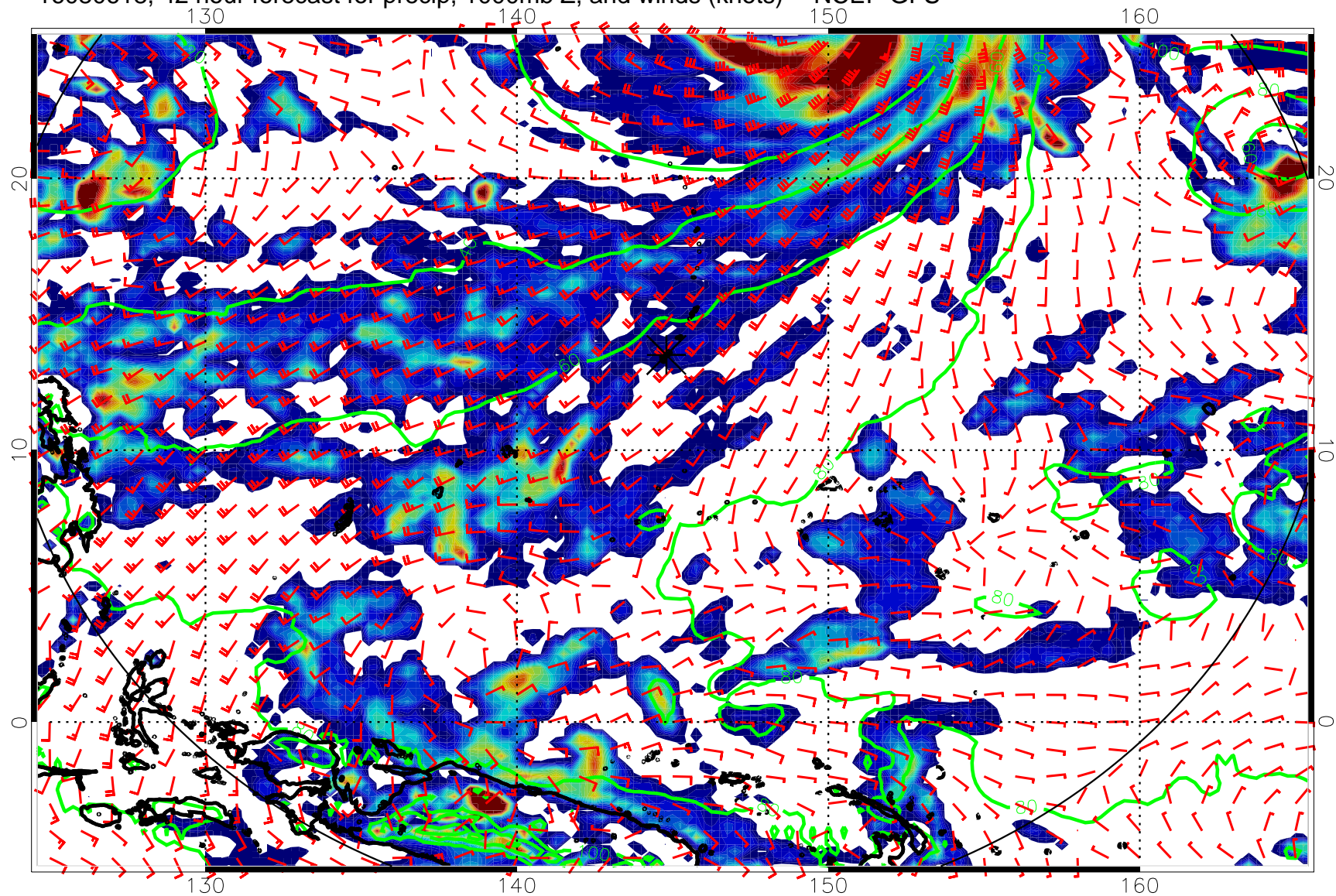
16080618, 42 hour forecast for precip, 1000mb Z, and winds (knots) -- NCEP GFS
