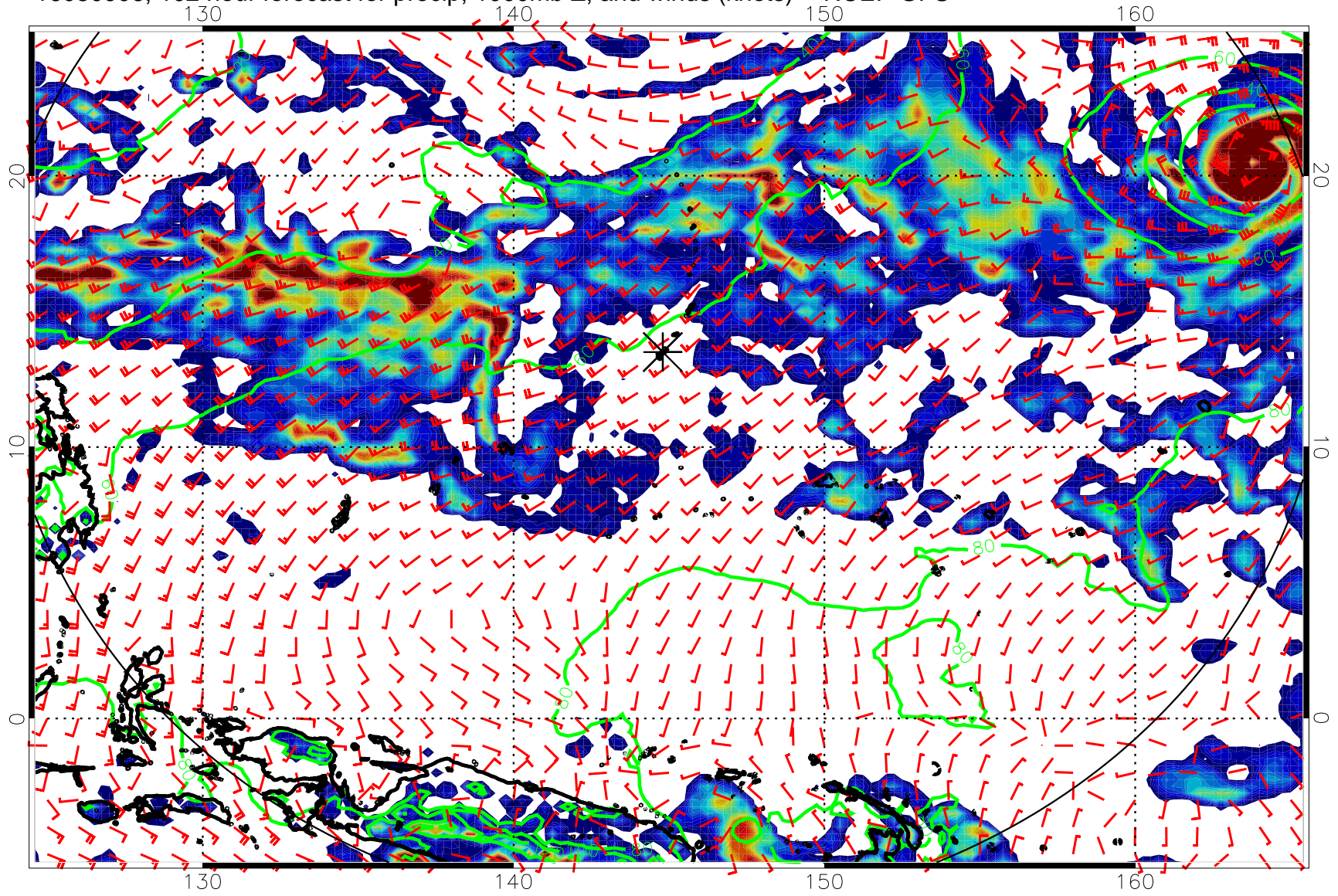
16080906, 102 hour forecast for precip, 1000mb Z, and winds (knots) -- NCEP GFS
