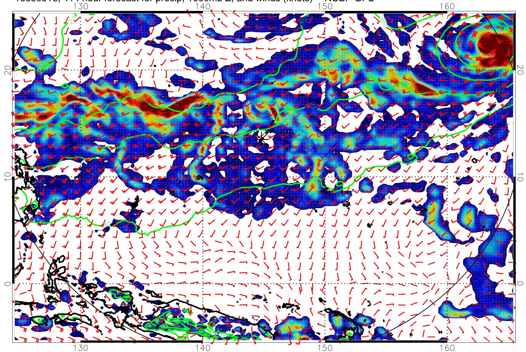
16080918, 114 hour forecast for precip, 1000mb Z, and winds (knots) -- NCEP GFS
