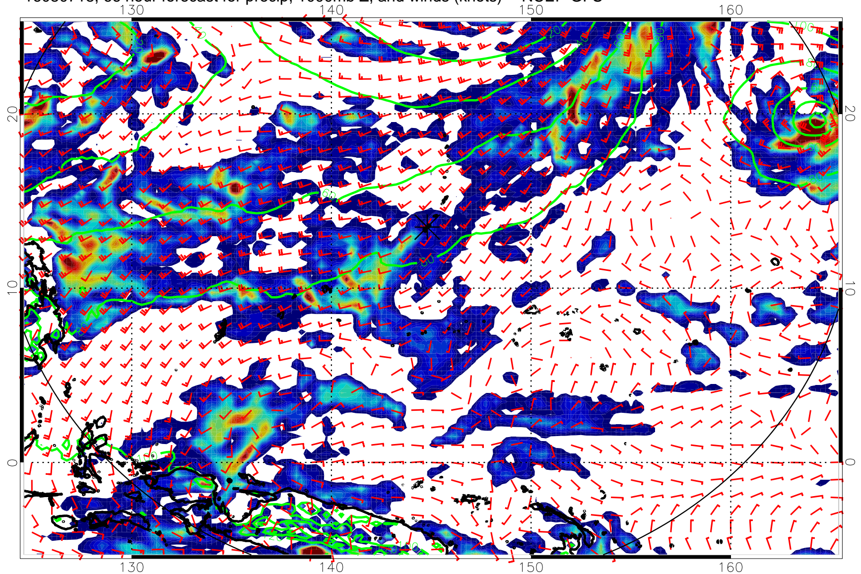
16080718, 66 hour forecast for precip, 1000mb Z, and winds (knots) -- NCEP GFS
