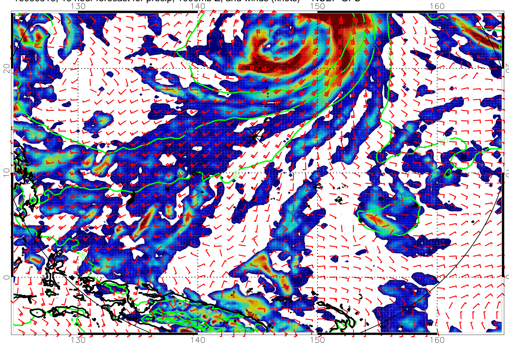
16080518, 18 hour forecast for precip, 1000mb Z, and winds (knots) -- NCEP GFS
