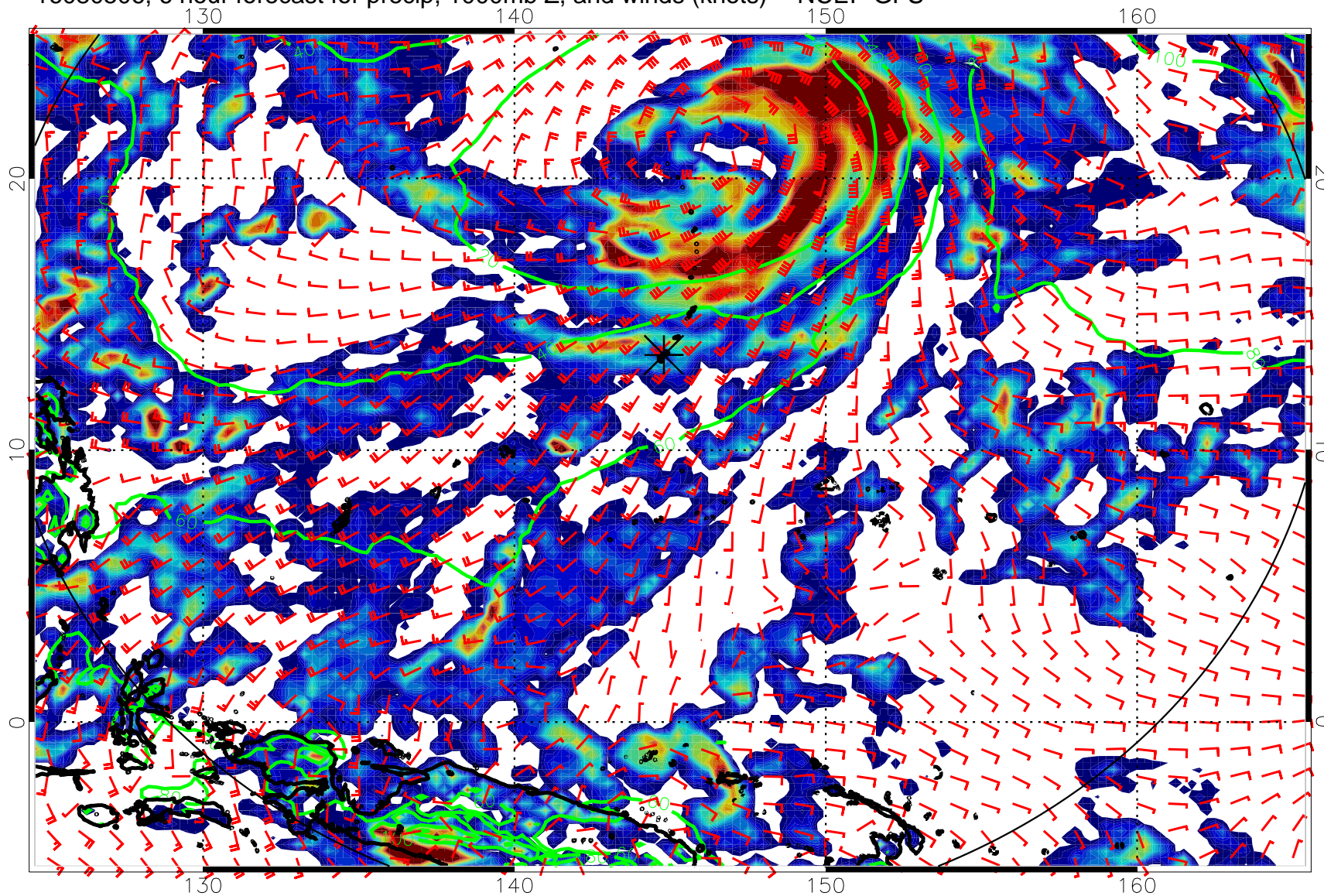
16080506, 6 hour forecast for precip, 1000mb Z, and winds (knots) -- NCEP GFS
