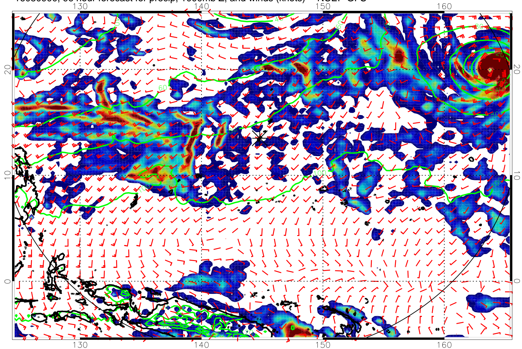
16080900, 96 hour forecast for precip, 1000mb Z, and winds (knots) -- NCEP GFS
