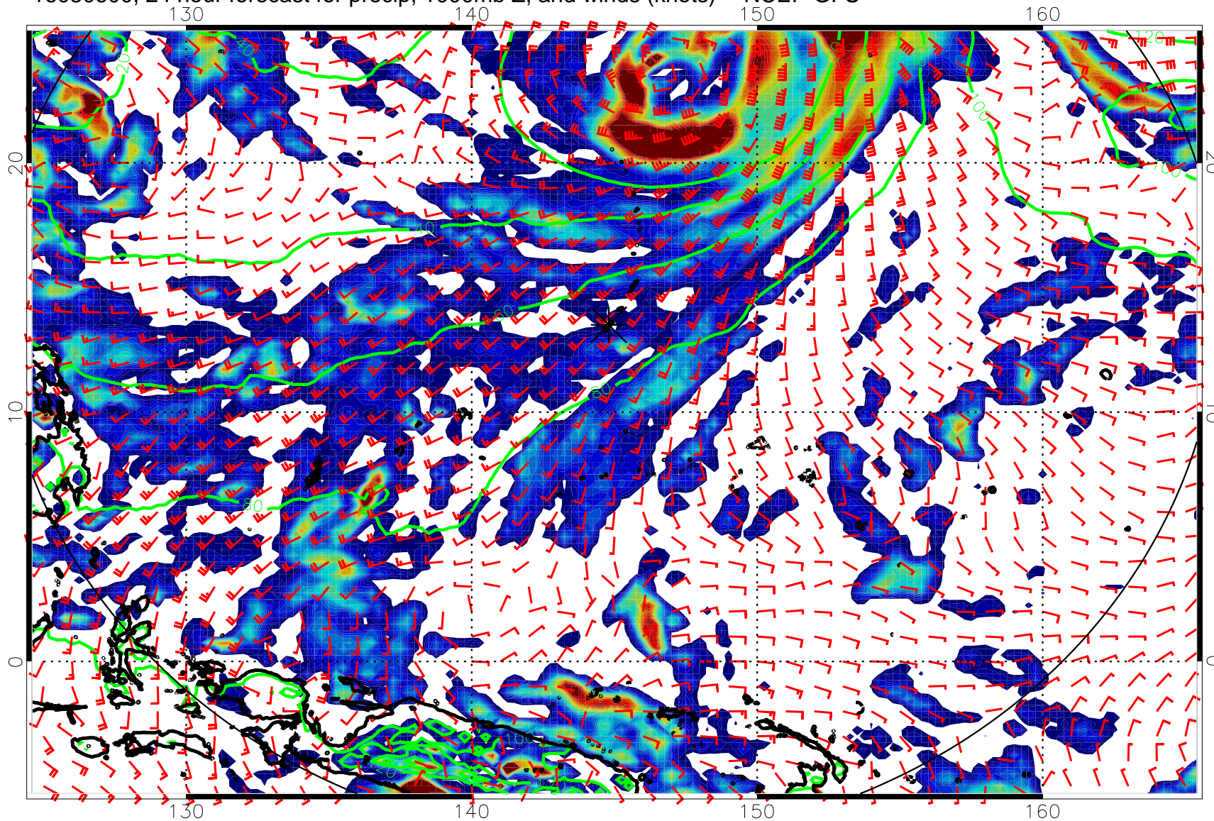
16080600, 24 hour forecast for precip, 1000mb Z, and winds (knots) -- NCEP GFS
