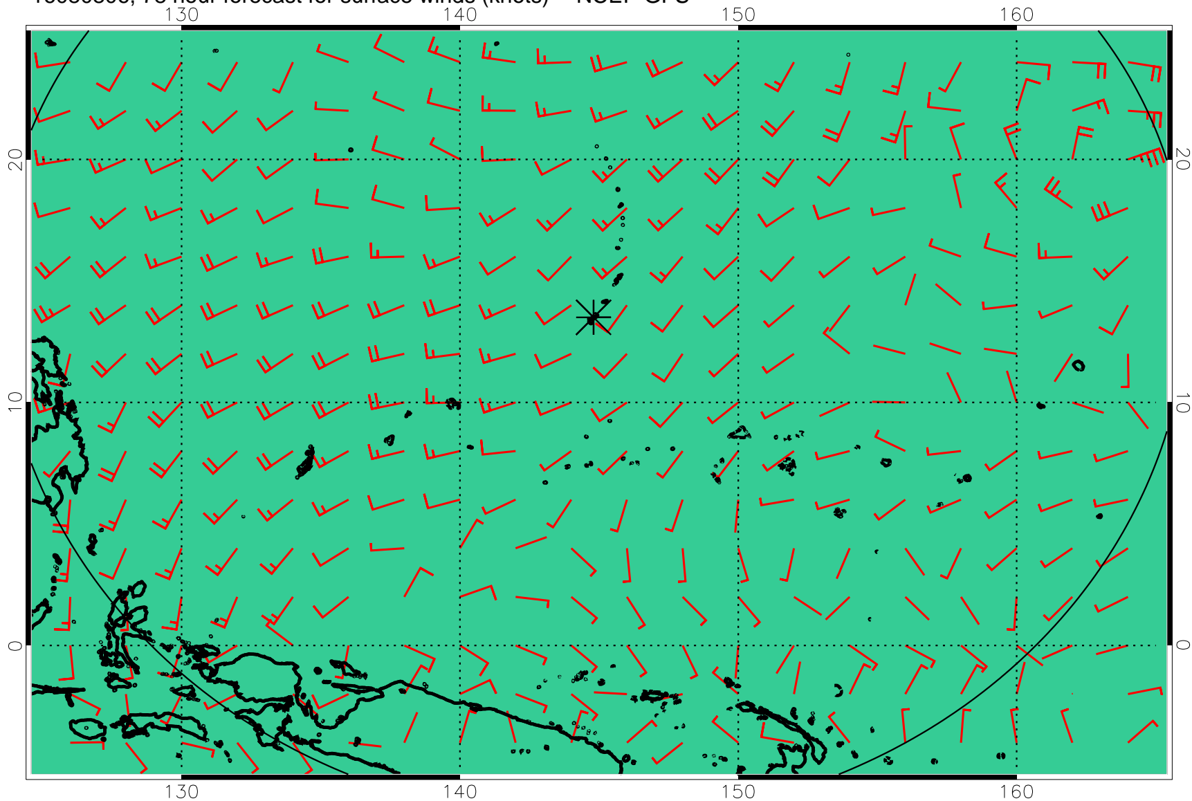
16080806, 78 hour forecast for surface winds (knots) -- NCEP GFS
