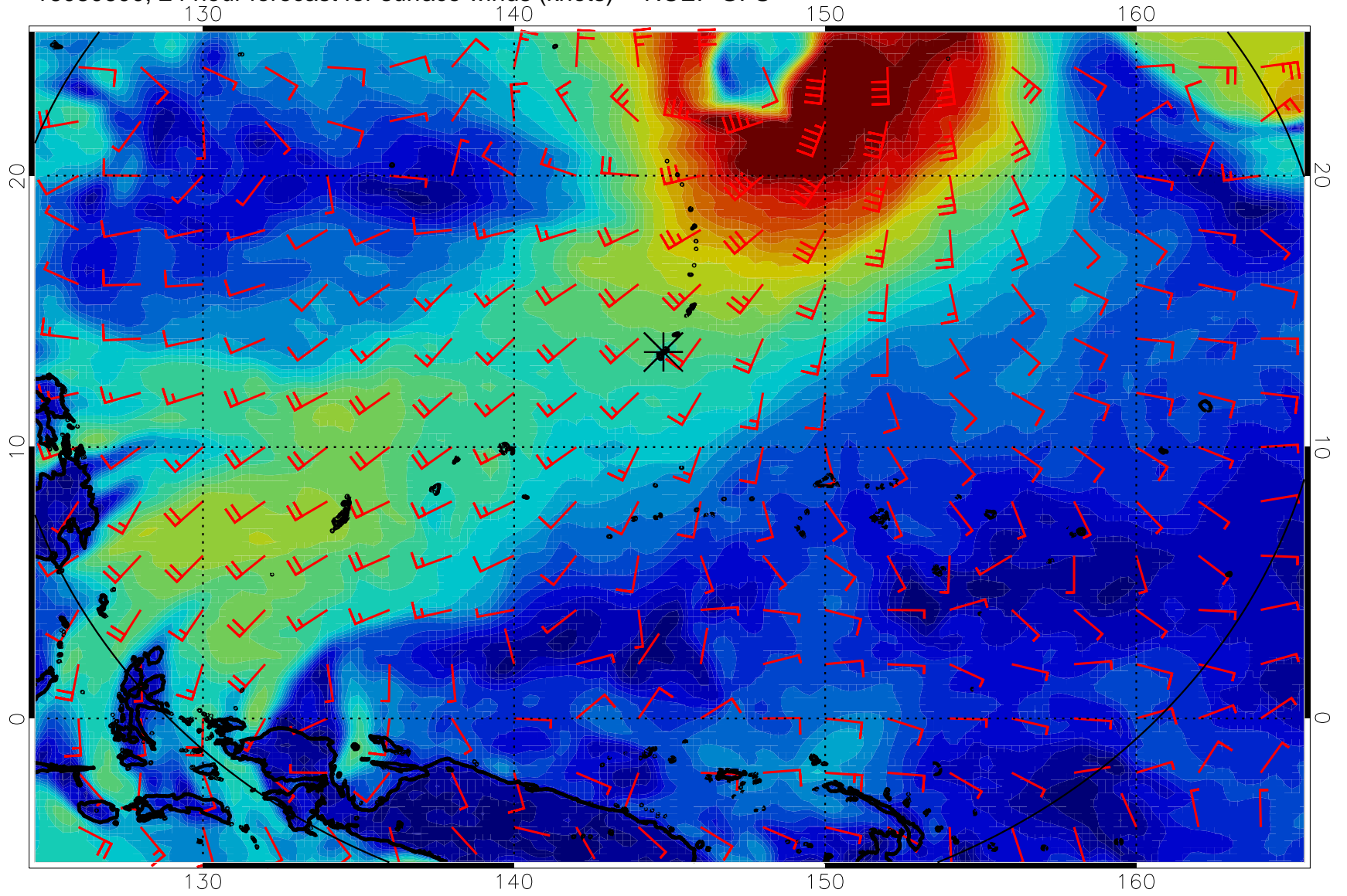
16080600, 24 hour forecast for surface winds (knots) -- NCEP GFS
