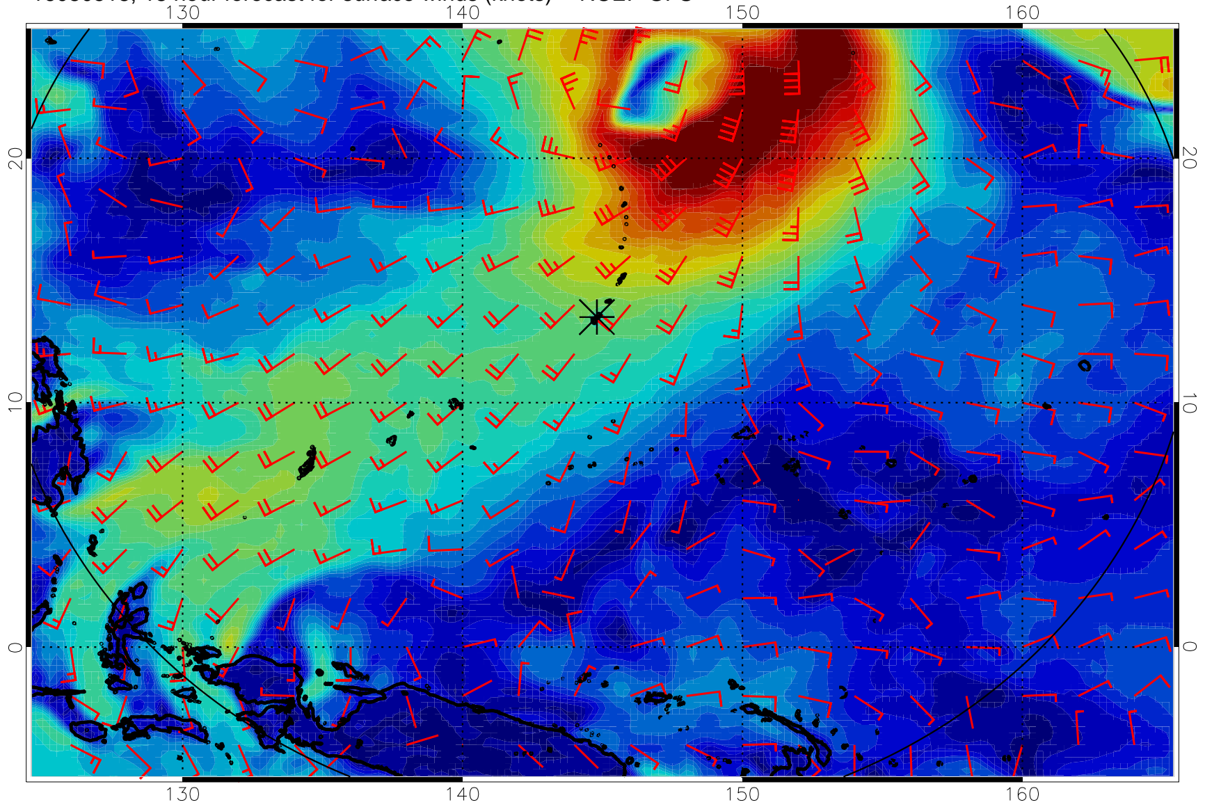
16080518, 18 hour forecast for surface winds (knots) -- NCEP GFS
