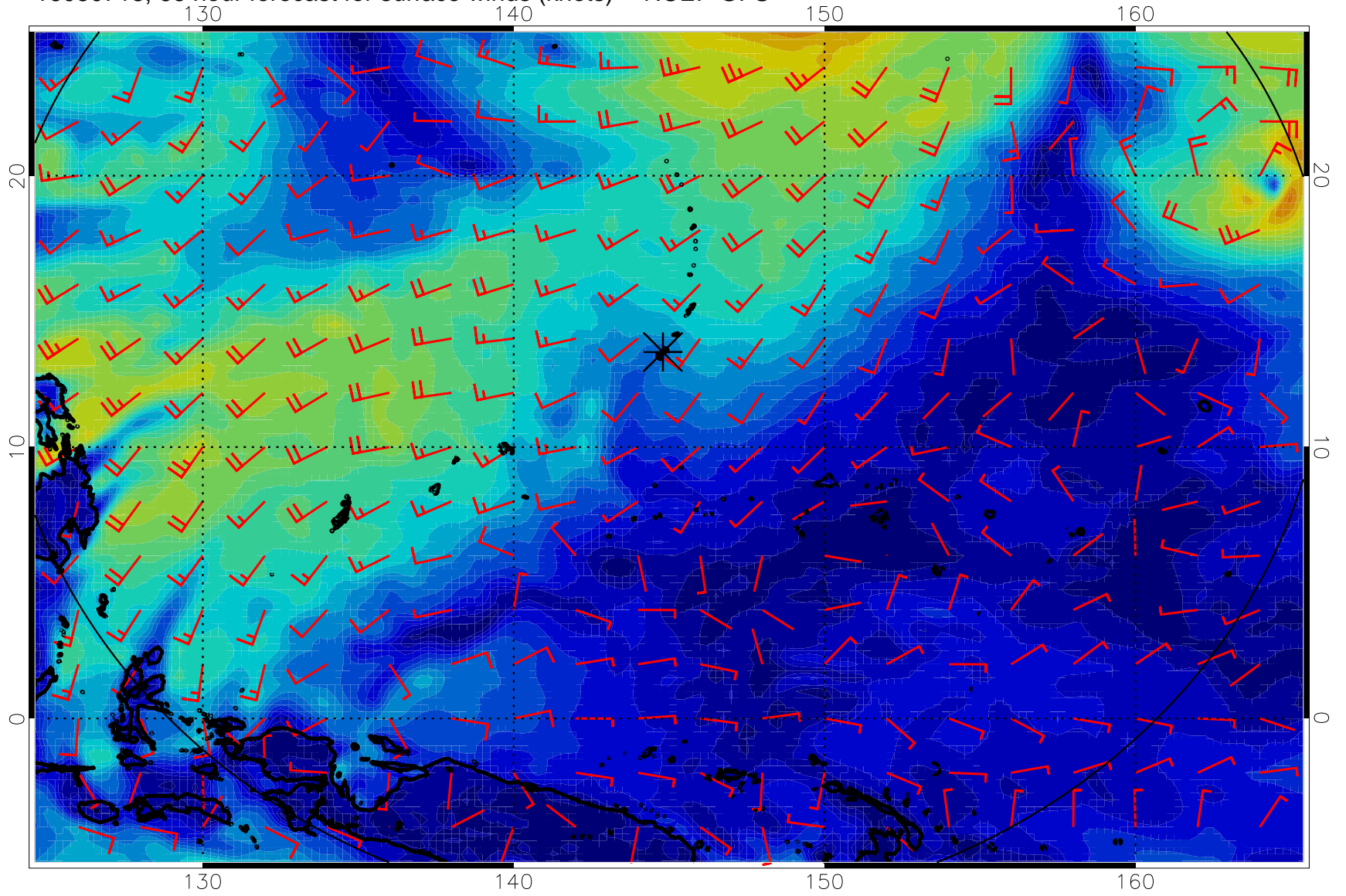
16080718, 66 hour forecast for surface winds (knots) -- NCEP GFS
