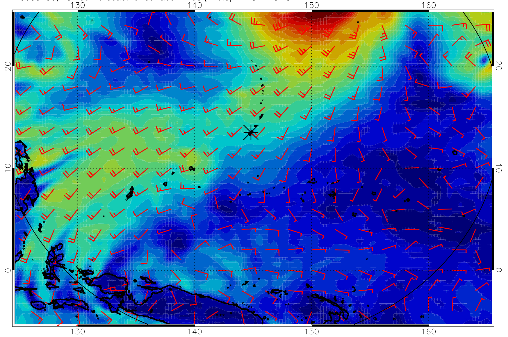
16080700, 48 hour forecast for surface winds (knots) -- NCEP GFS
