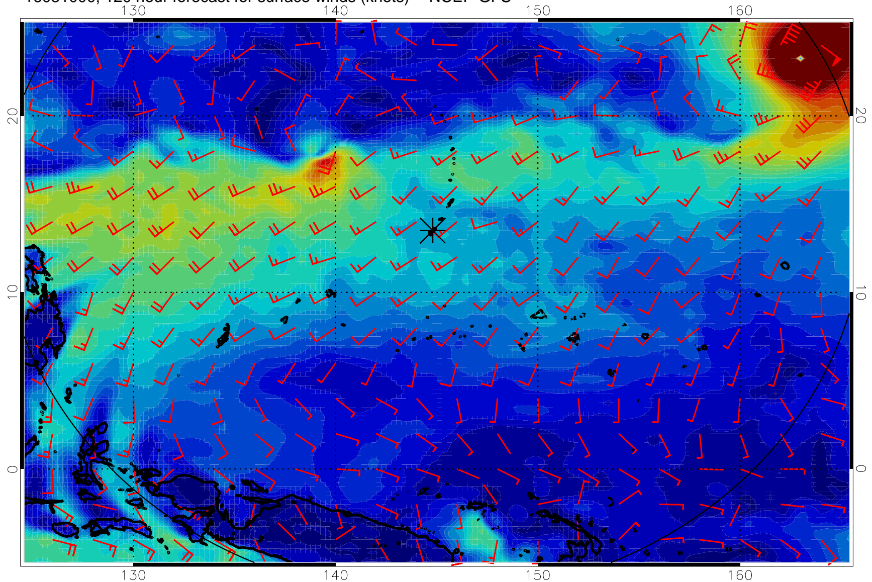
16081000, 120 hour forecast for surface winds (knots) -- NCEP GFS
