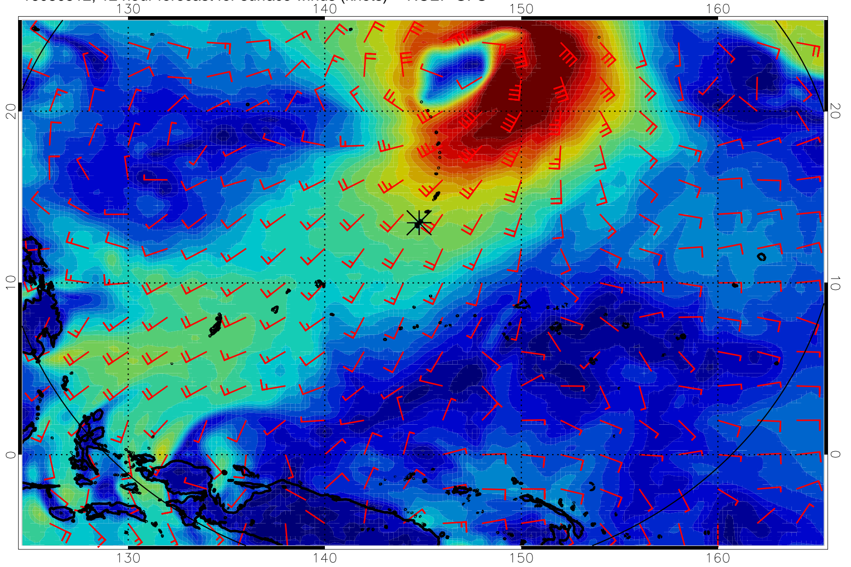
16080512, 12 hour forecast for surface winds (knots) -- NCEP GFS
