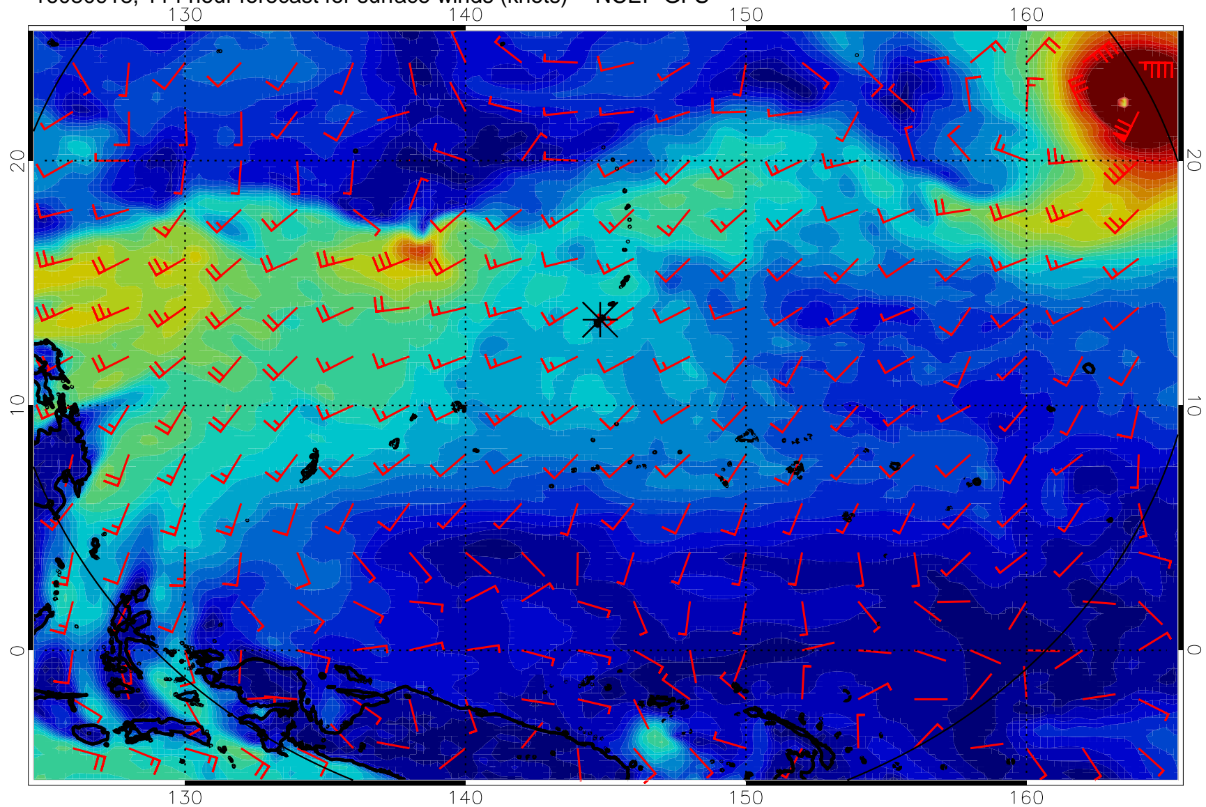
16080918, 114 hour forecast for surface winds (knots) -- NCEP GFS
