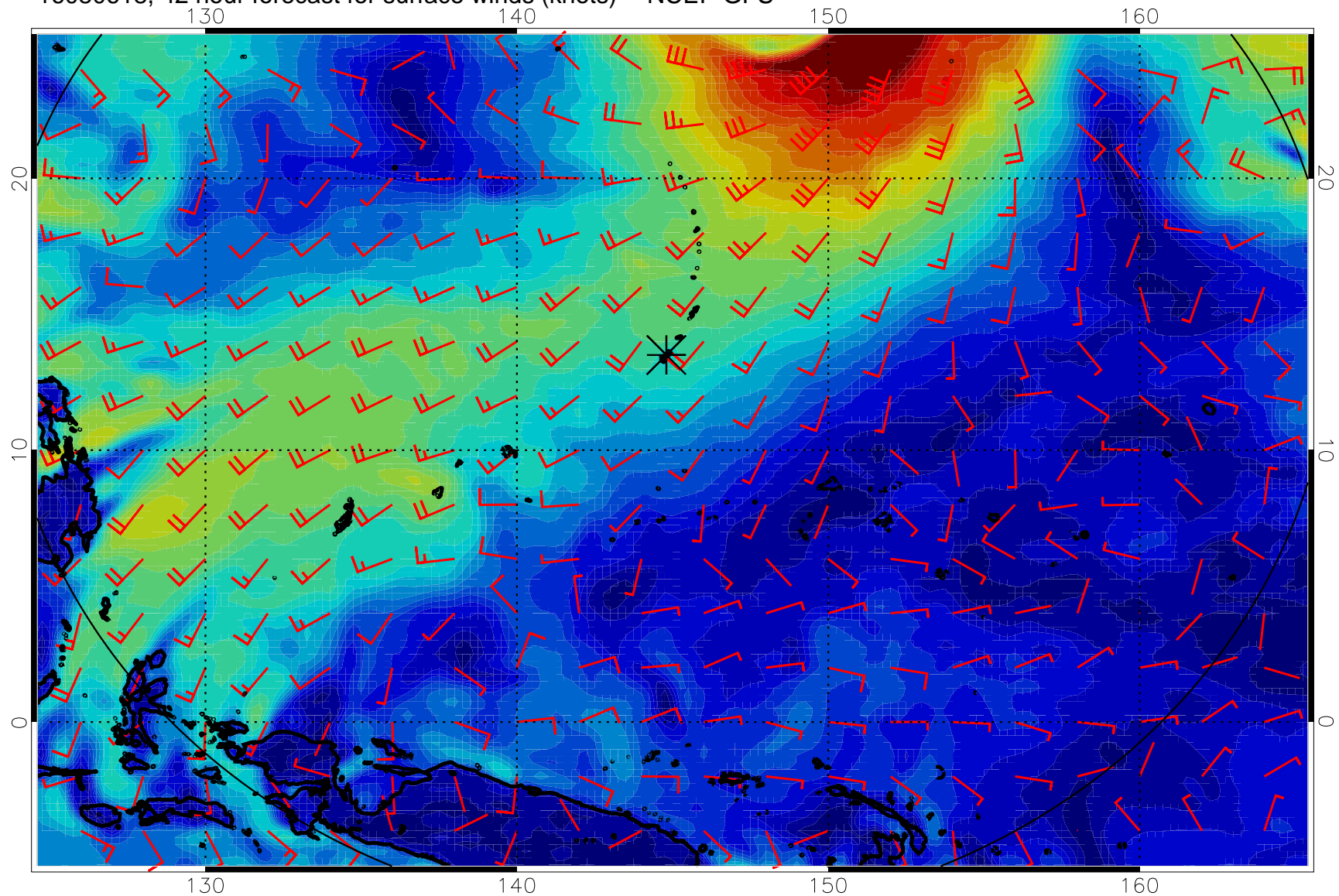
16080618, 42 hour forecast for surface winds (knots) -- NCEP GFS
