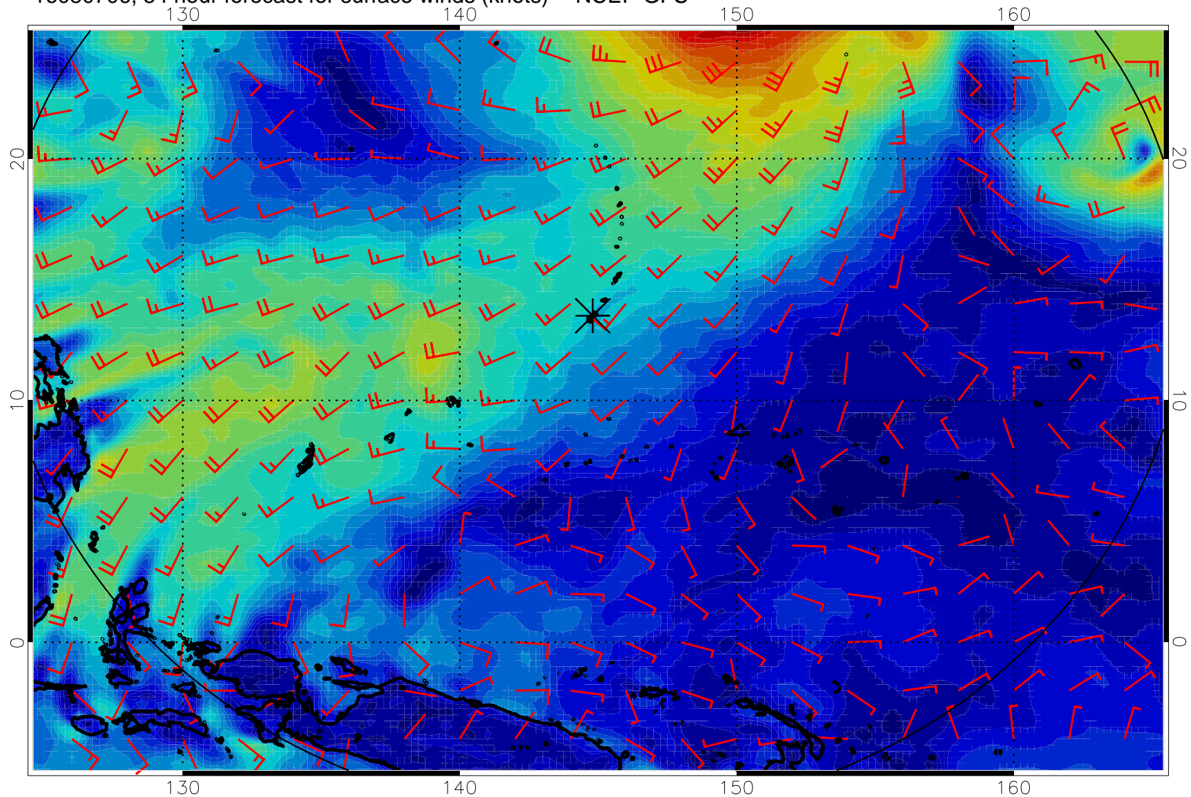
16080706, 54 hour forecast for surface winds (knots) -- NCEP GFS
