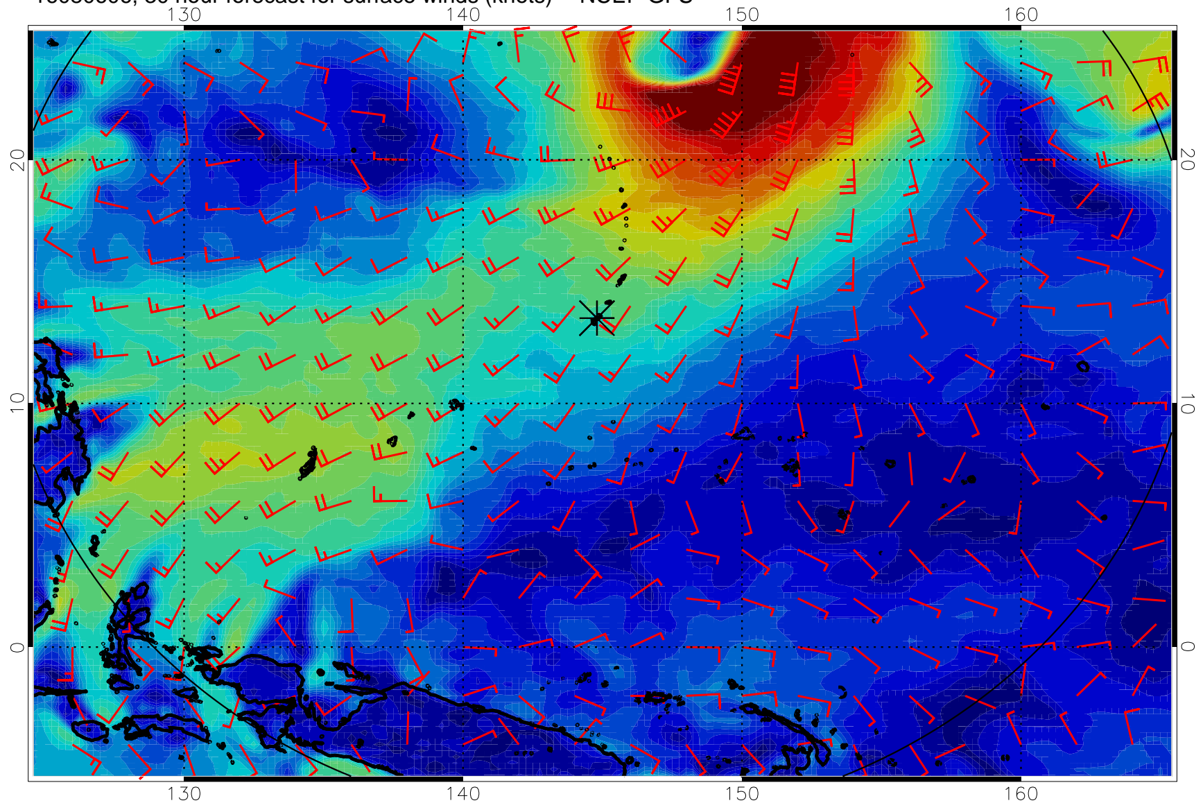
16080606, 30 hour forecast for surface winds (knots) -- NCEP GFS
