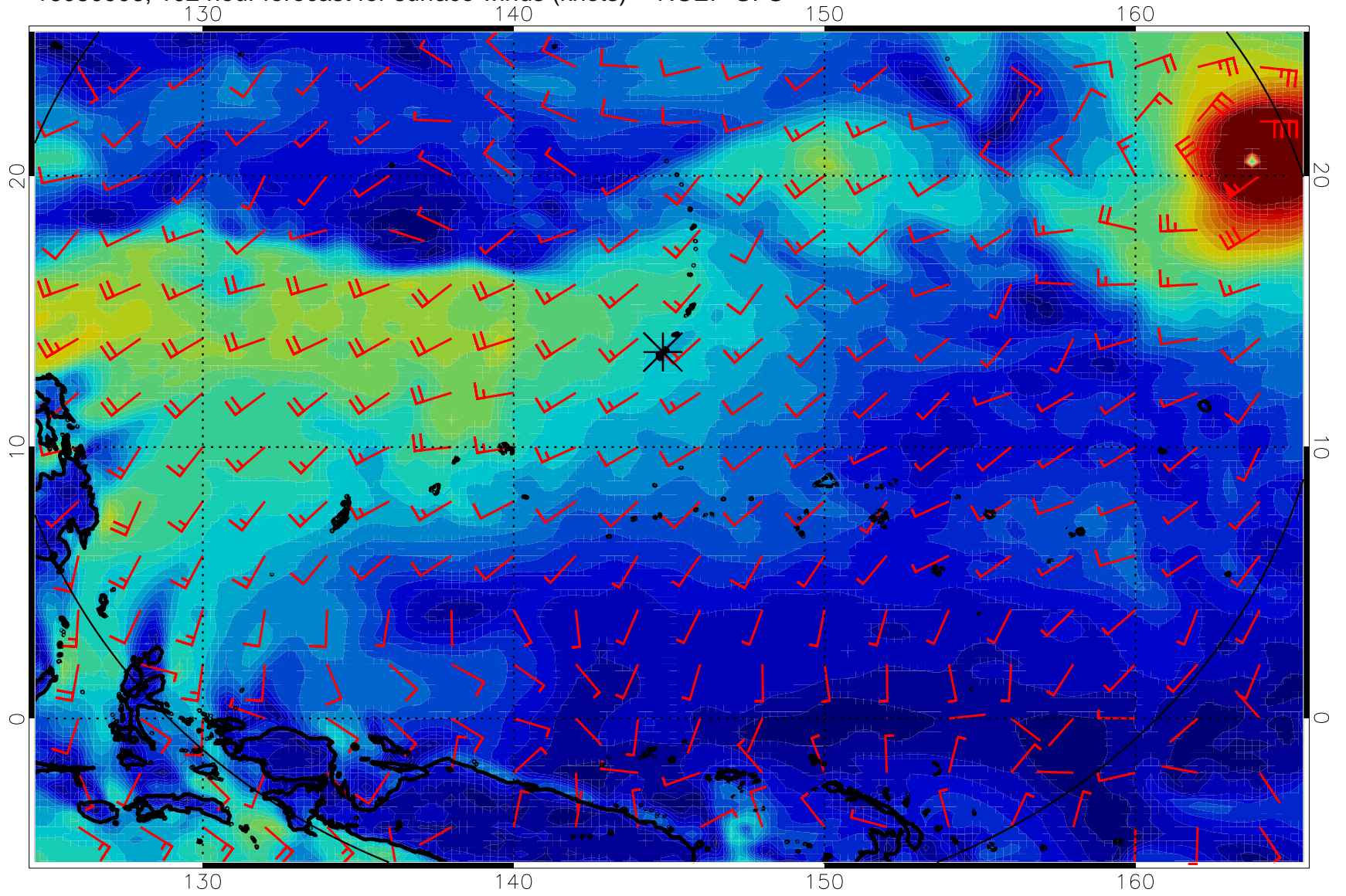
16080906, 102 hour forecast for surface winds (knots) -- NCEP GFS
