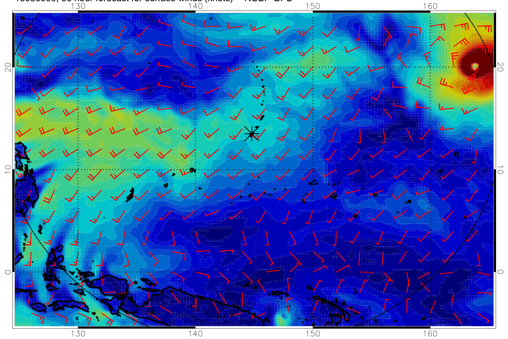
16080900, 96 hour forecast for surface winds (knots) -- NCEP GFS
