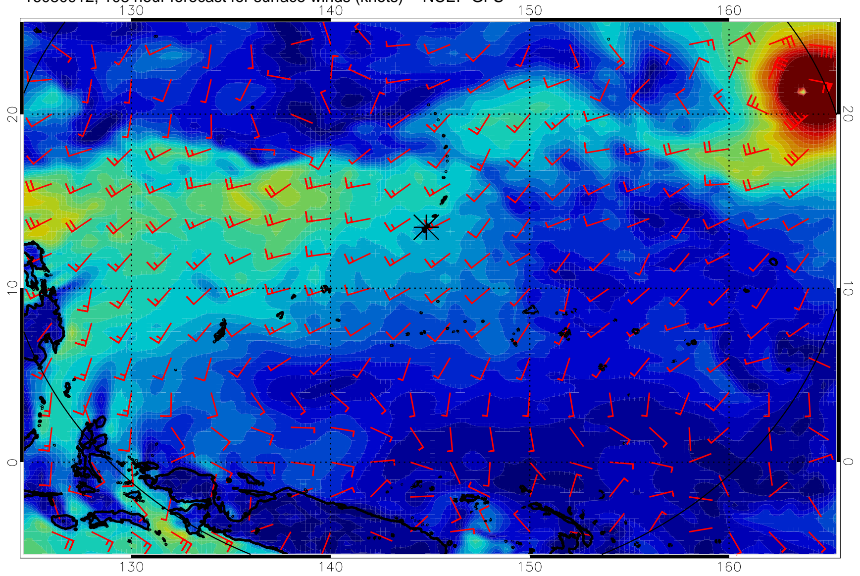
16080912, 108 hour forecast for surface winds (knots) -- NCEP GFS
