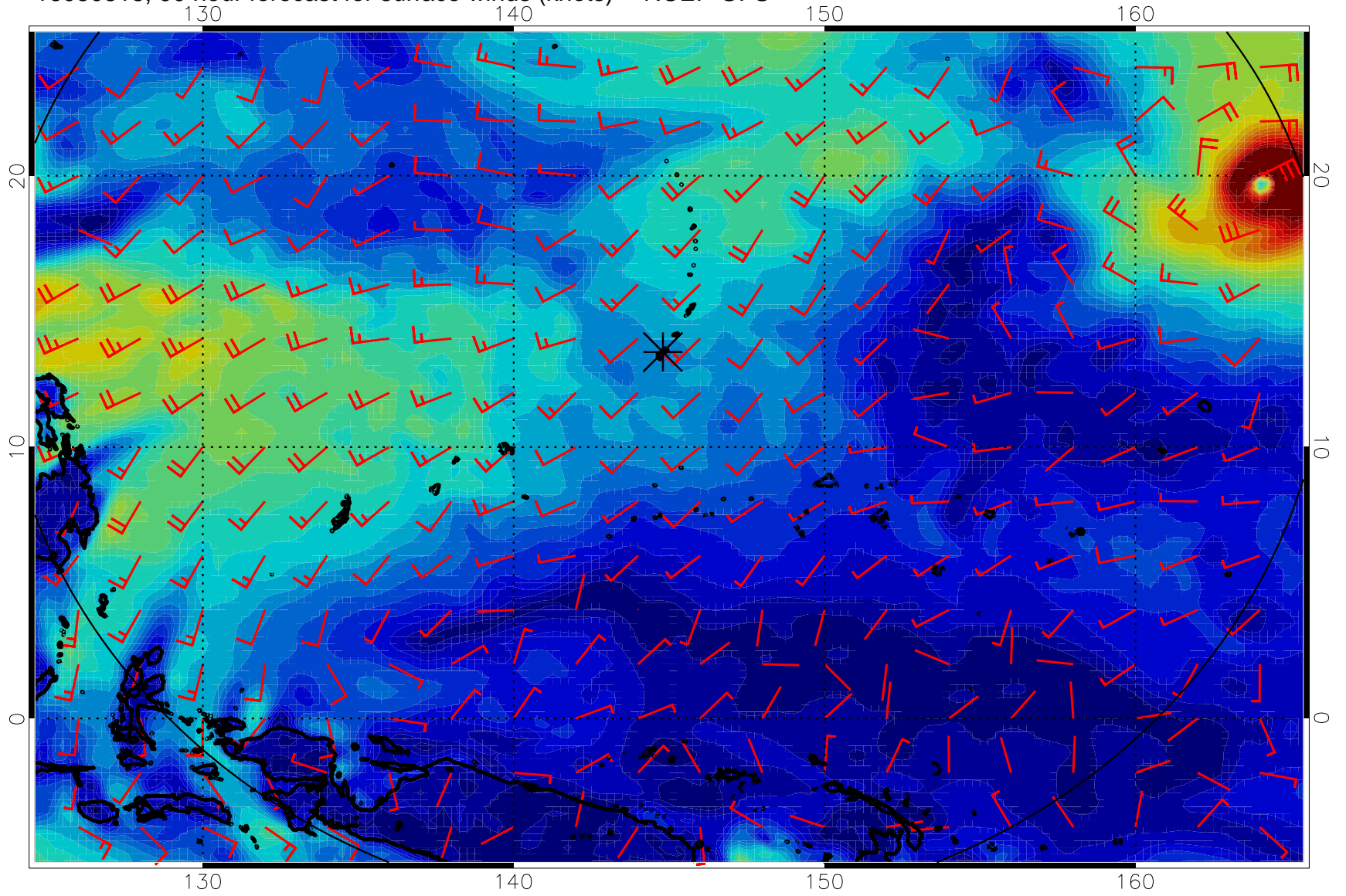
16080818, 90 hour forecast for surface winds (knots) -- NCEP GFS
