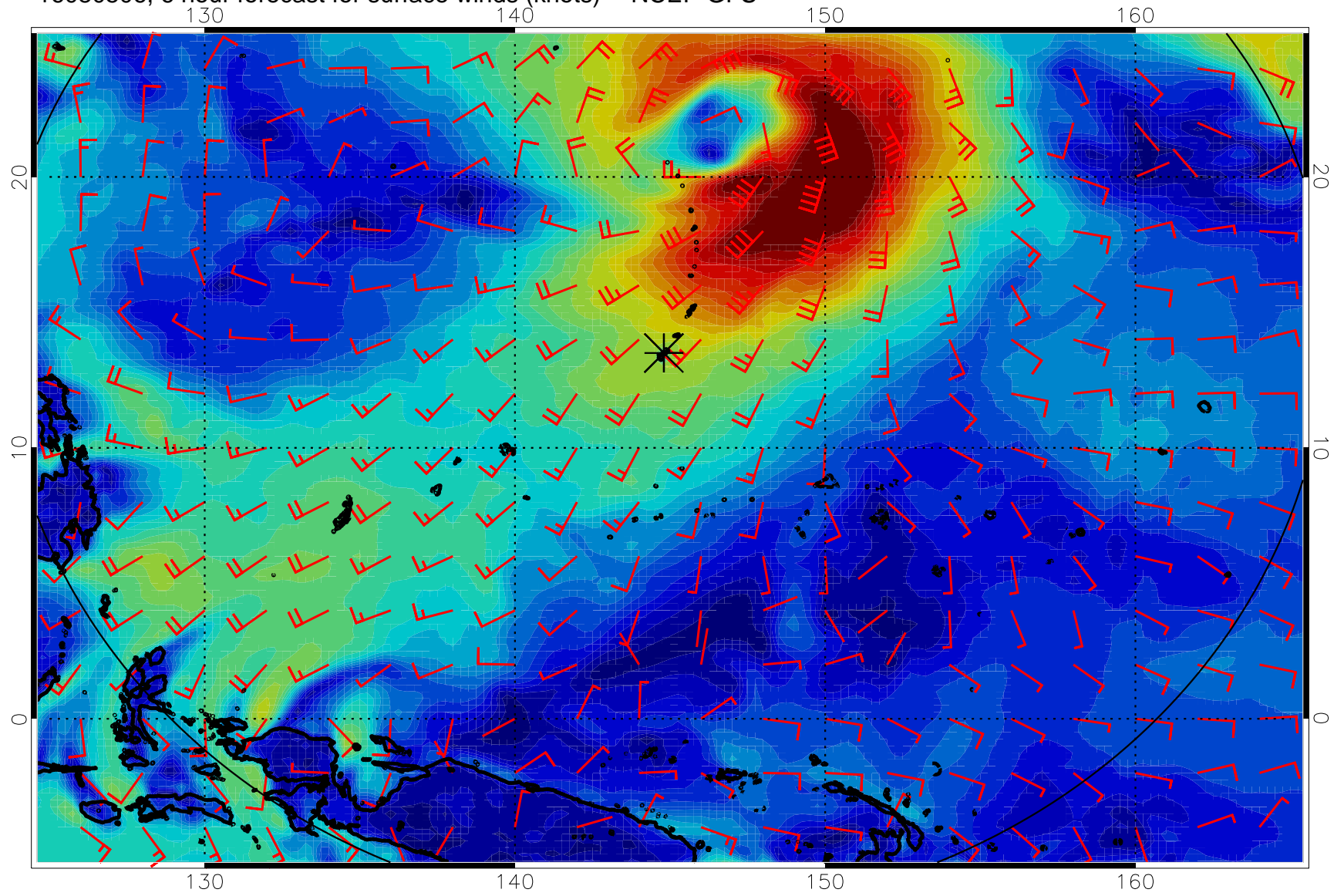
16080506, 6 hour forecast for surface winds (knots) -- NCEP GFS
