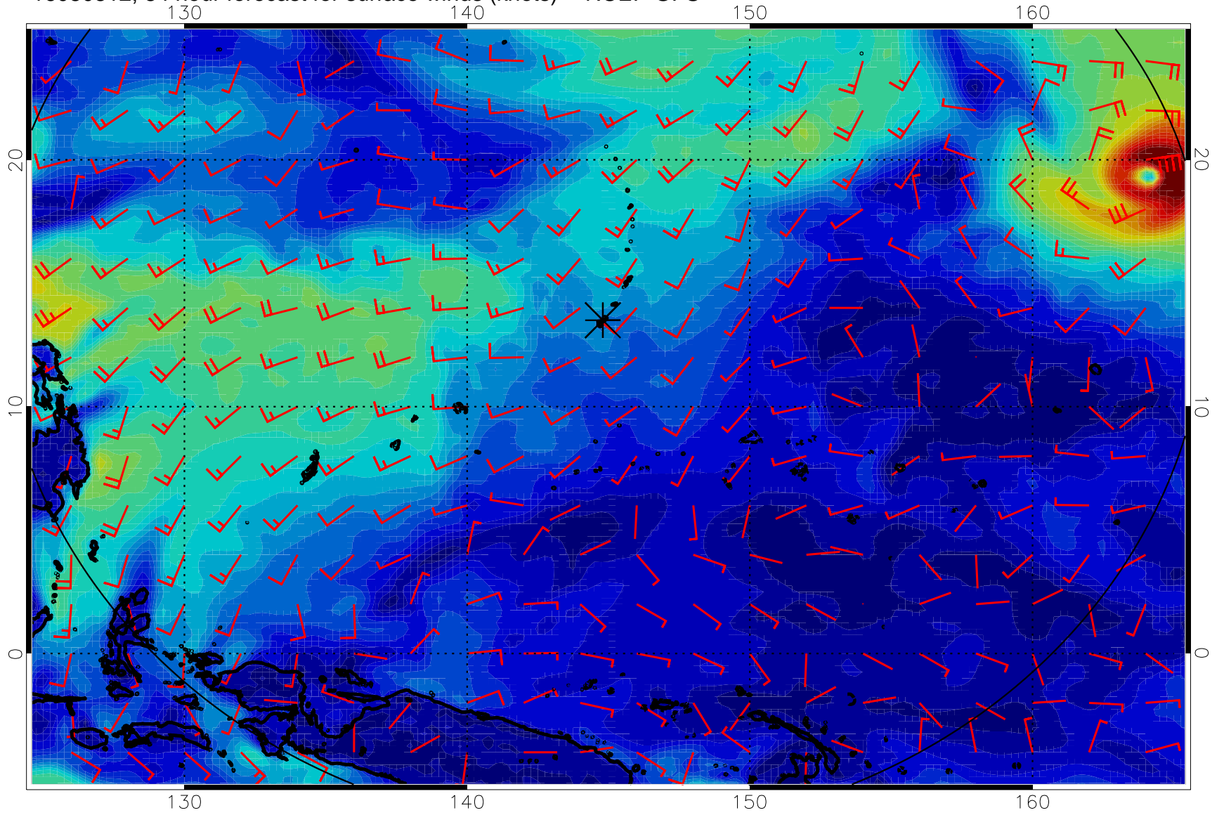
16080812, 84 hour forecast for surface winds (knots) -- NCEP GFS
