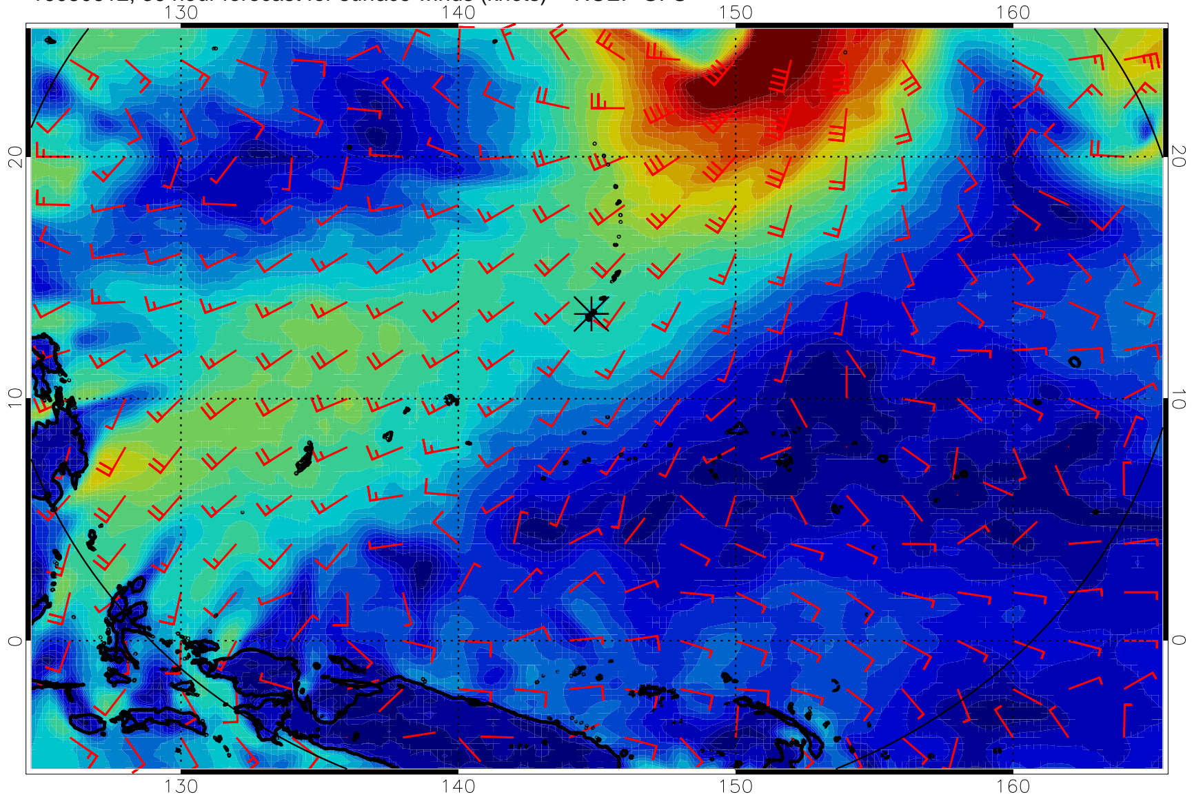
16080612, 36 hour forecast for surface winds (knots) -- NCEP GFS
