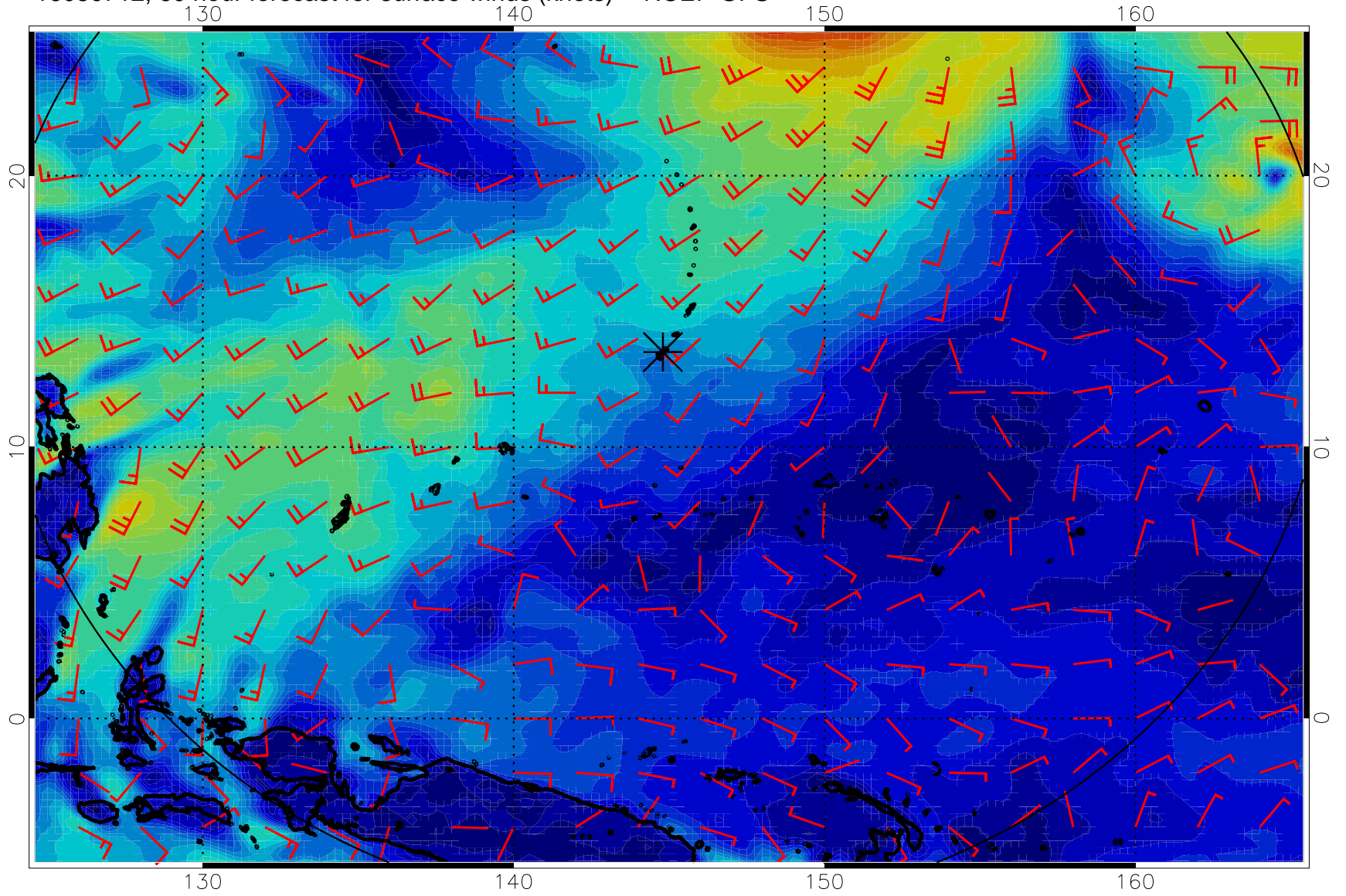
16080712, 60 hour forecast for surface winds (knots) -- NCEP GFS
