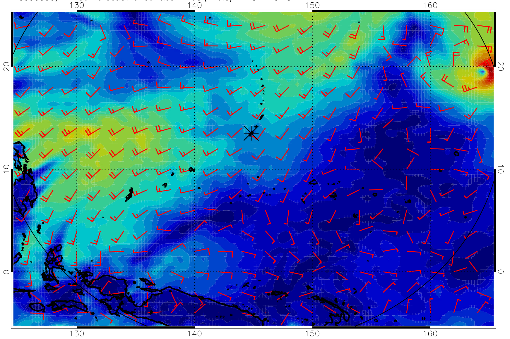
16080800, 72 hour forecast for surface winds (knots) -- NCEP GFS
