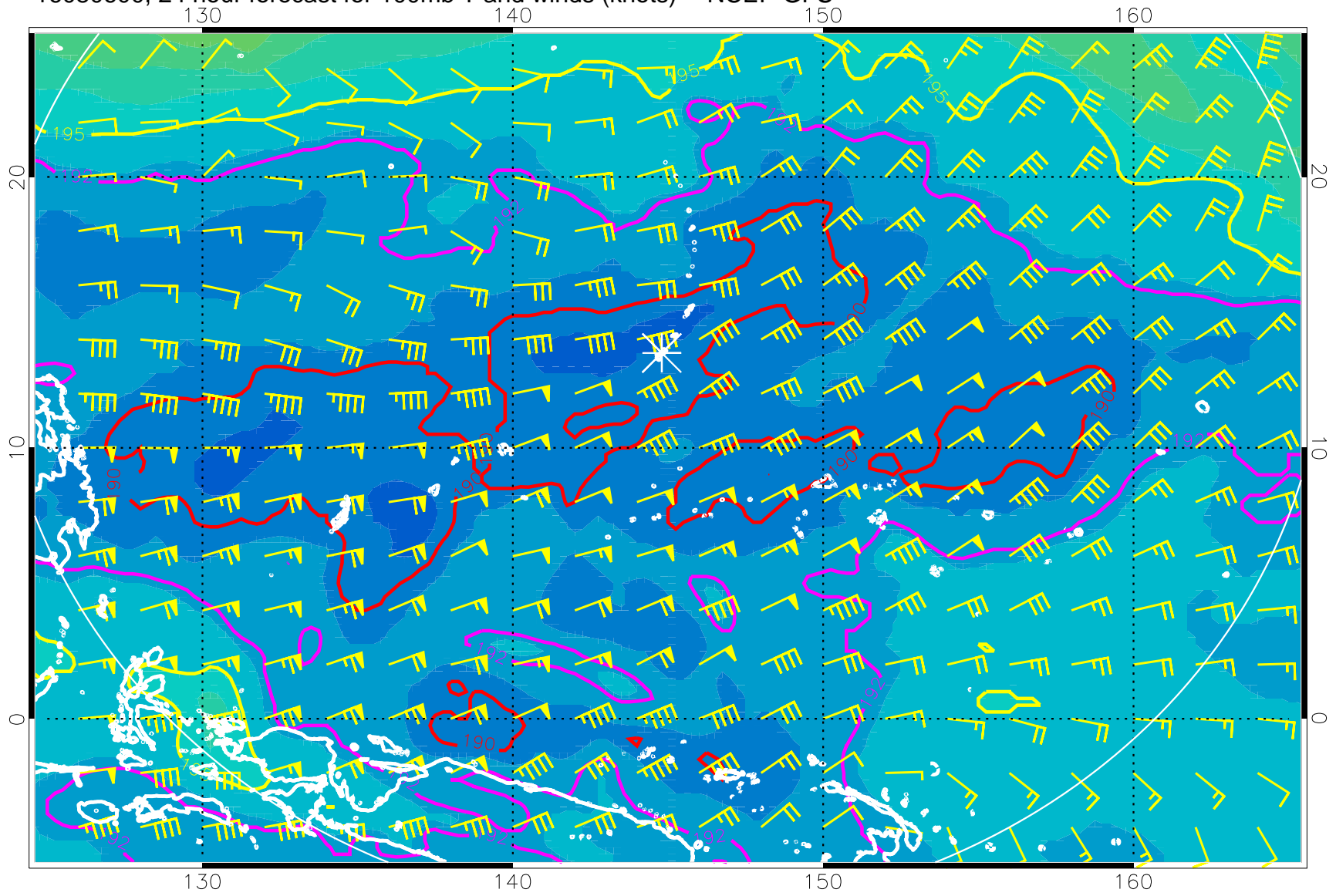
16080600, 24 hour forecast for 100mb T and winds (knots) -- NCEP GFS
