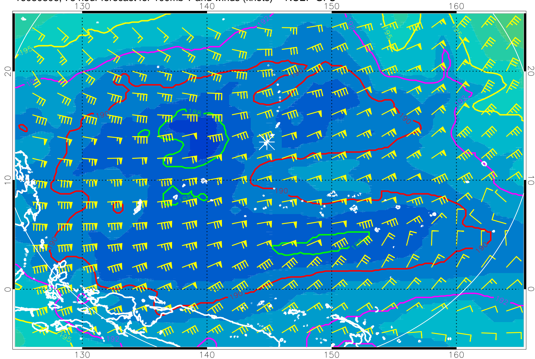
16080806, 78 hour forecast for 100mb T and winds (knots) -- NCEP GFS
