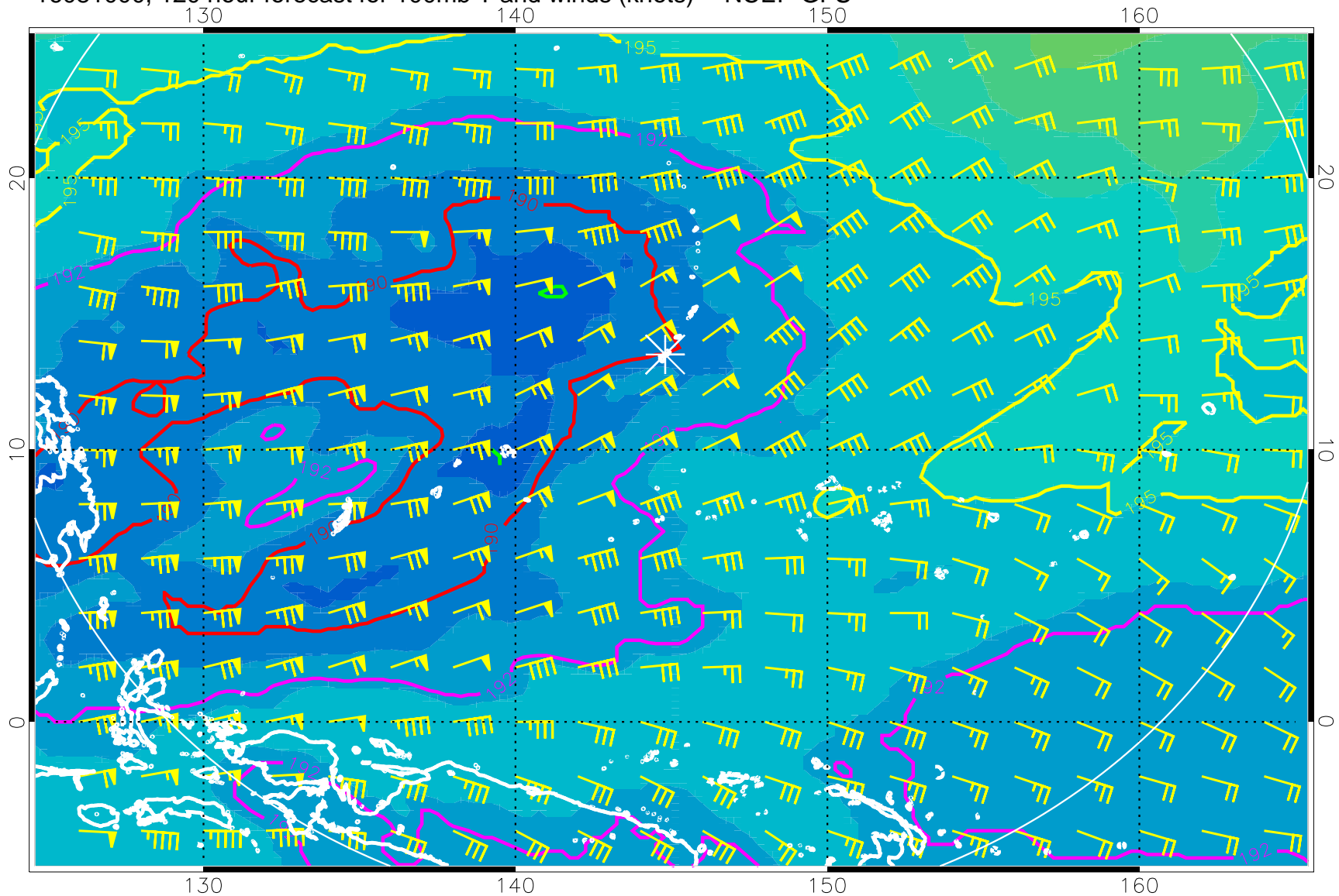
16081000, 120 hour forecast for 100mb T and winds (knots) -- NCEP GFS
