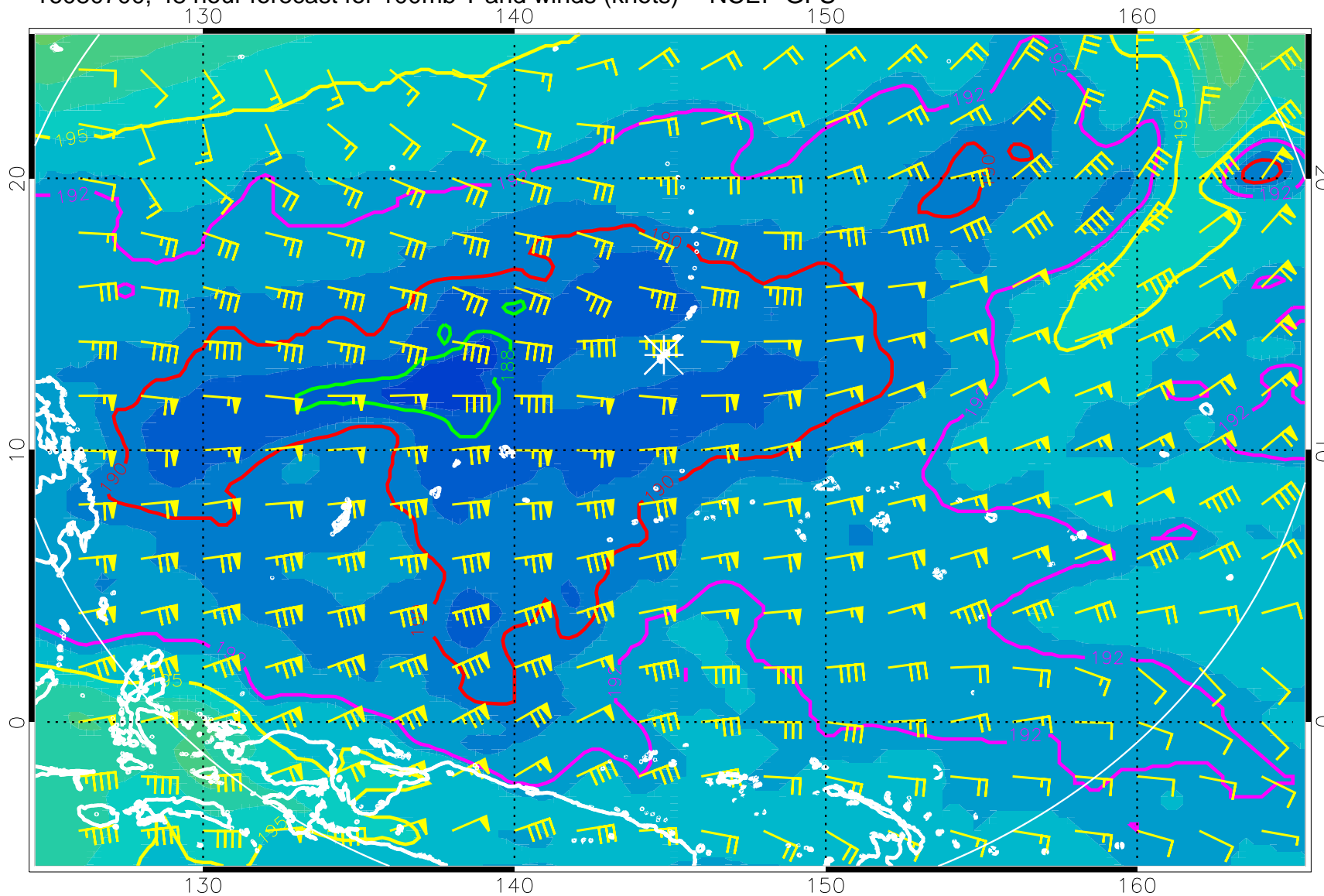
16080700, 48 hour forecast for 100mb T and winds (knots) -- NCEP GFS
