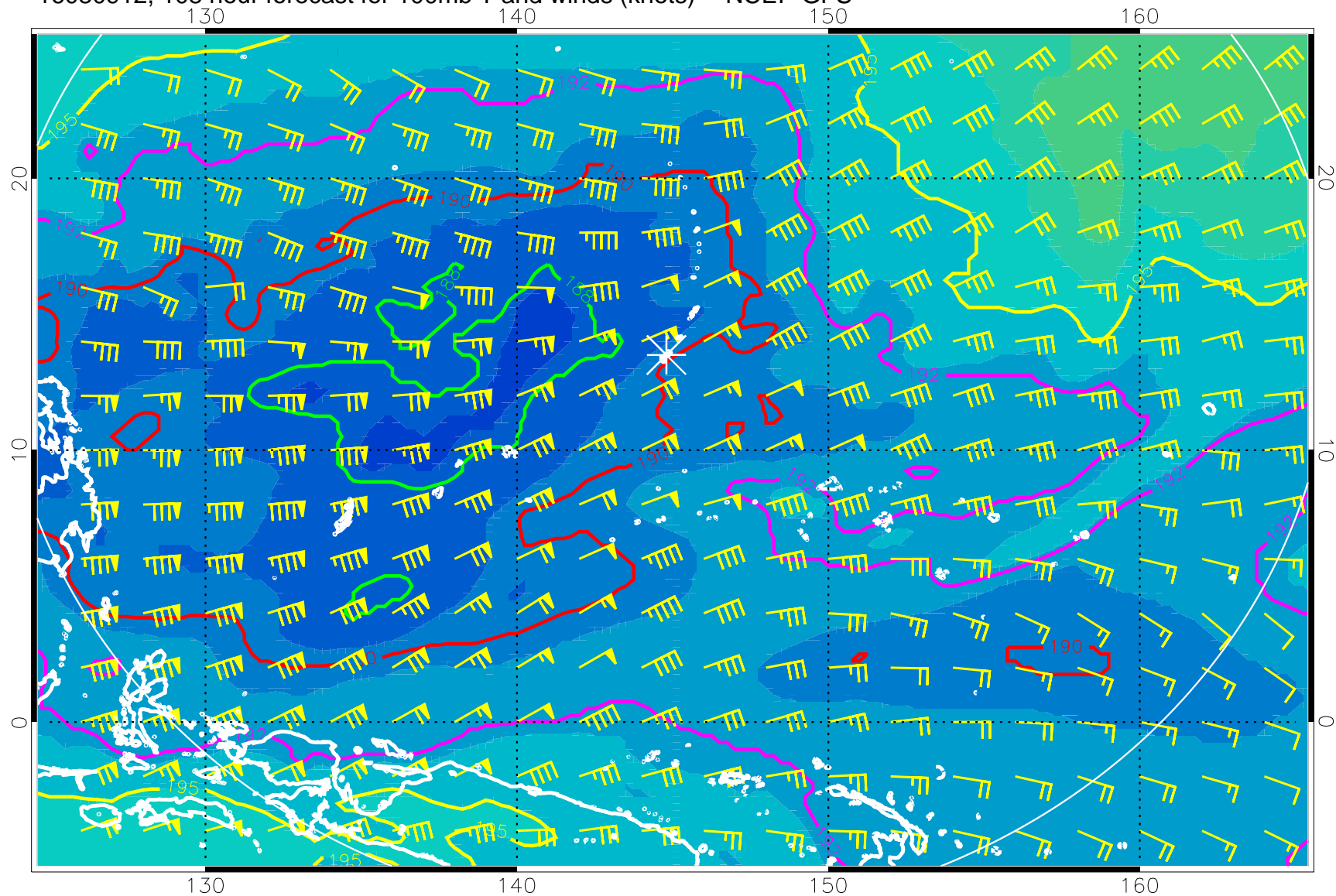
16080912, 108 hour forecast for 100mb T and winds (knots) -- NCEP GFS
