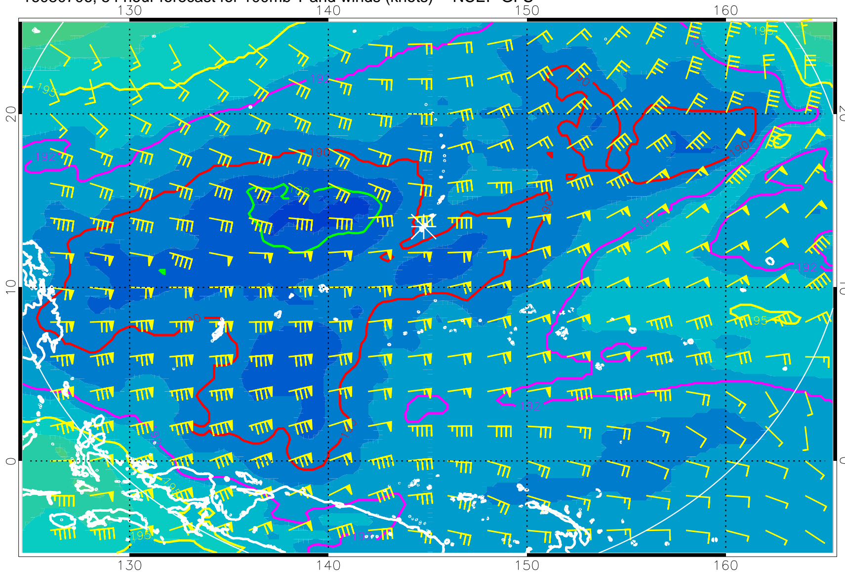
16080706, 54 hour forecast for 100mb T and winds (knots) -- NCEP GFS
