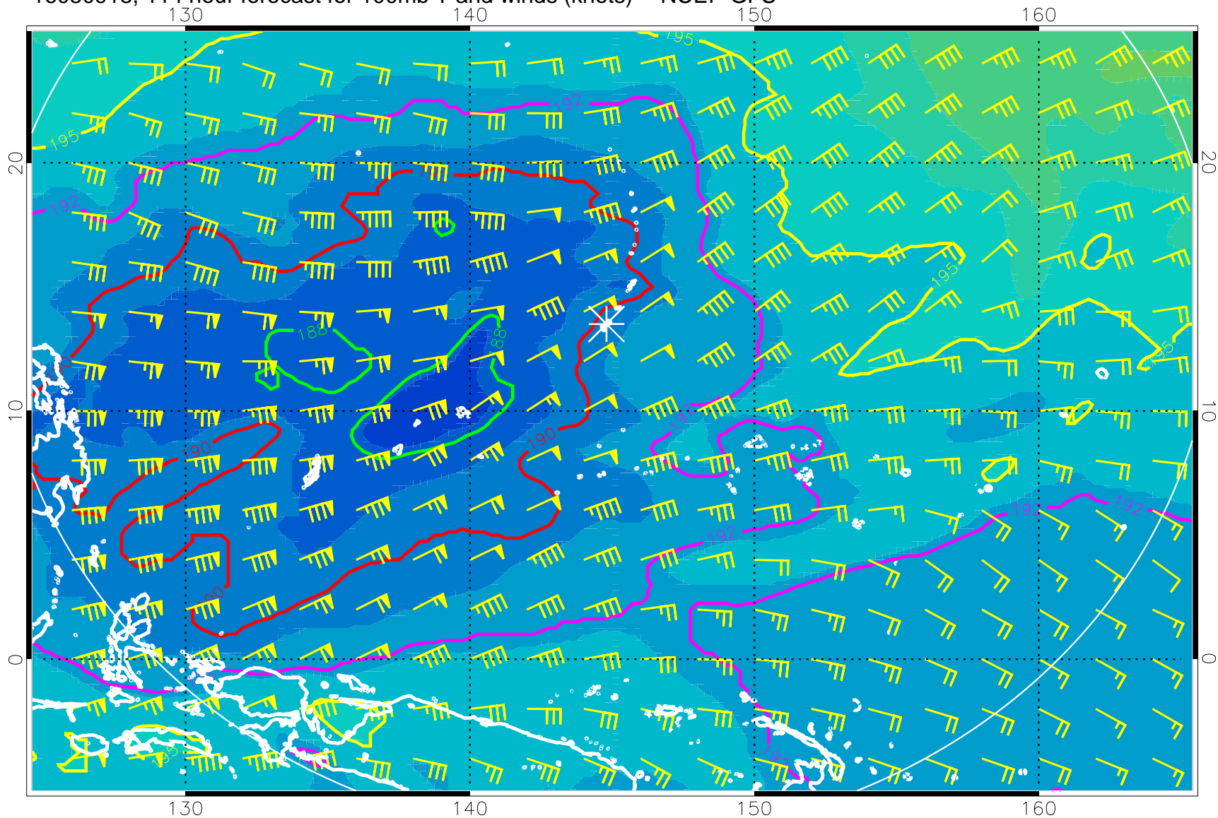
16080918, 114 hour forecast for 100mb T and winds (knots) -- NCEP GFS
