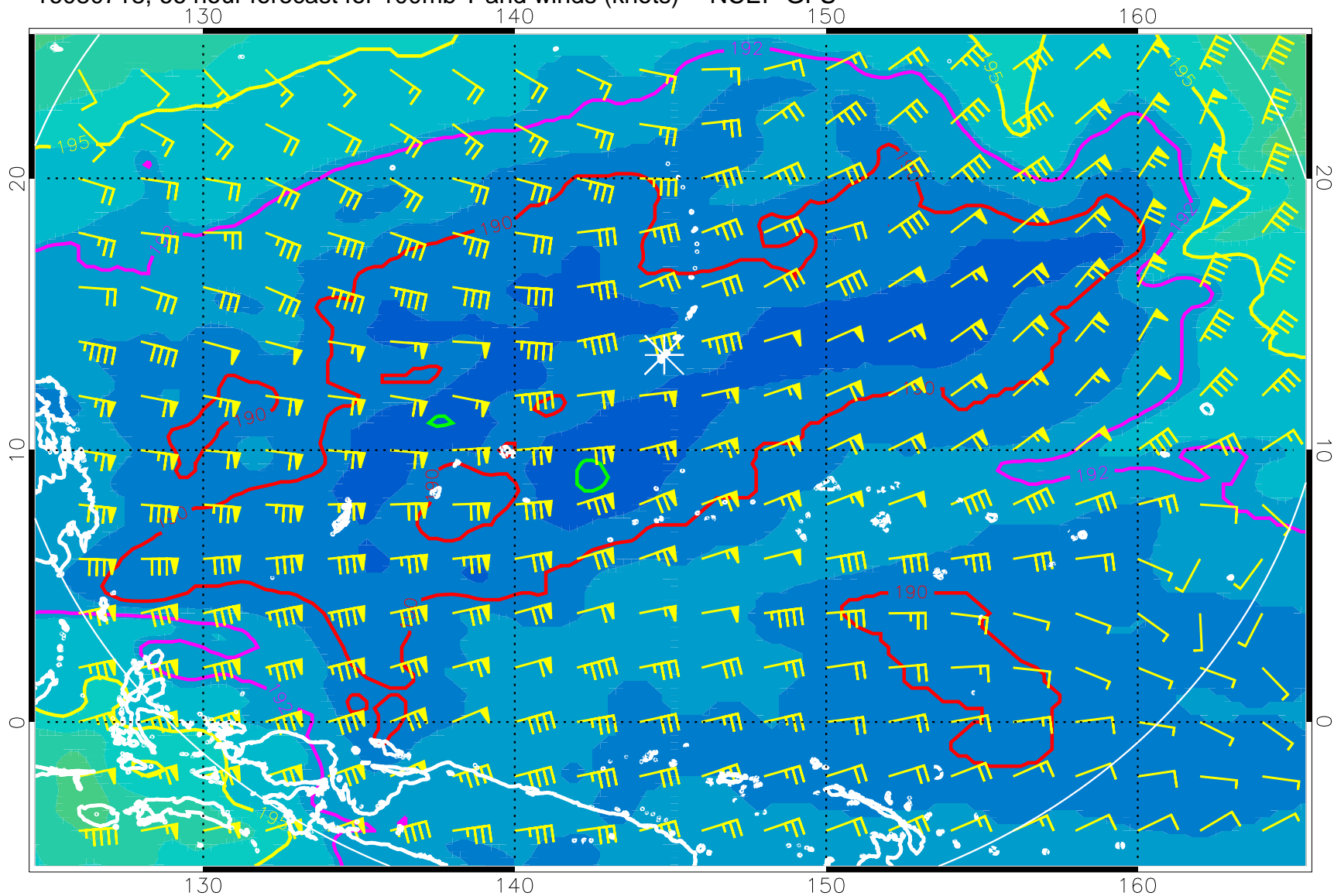
16080718, 66 hour forecast for 100mb T and winds (knots) -- NCEP GFS
