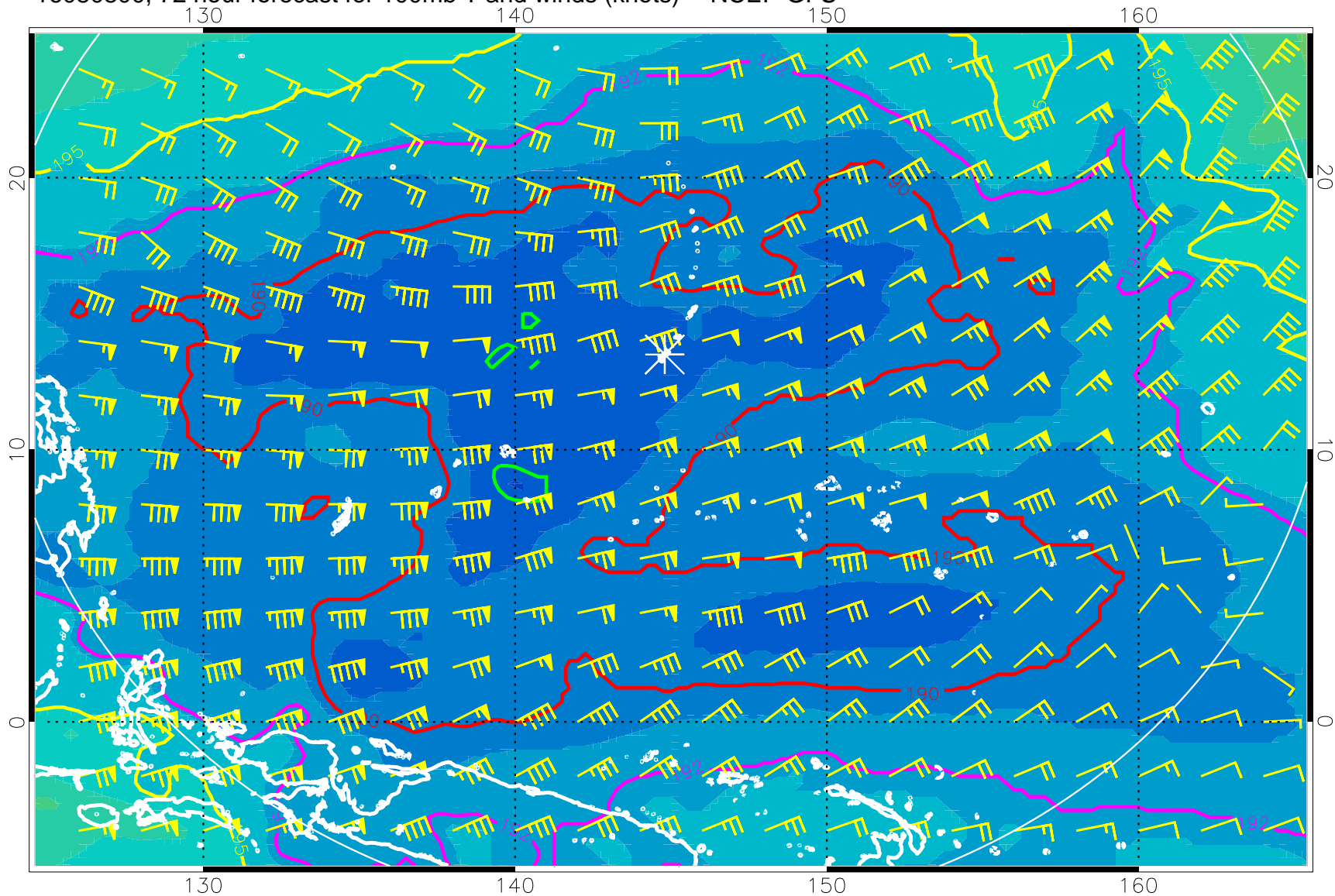
16080800, 72 hour forecast for 100mb T and winds (knots) -- NCEP GFS
