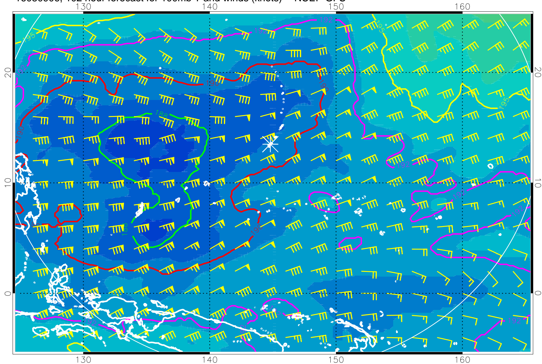
16080906, 102 hour forecast for 100mb T and winds (knots) -- NCEP GFS
