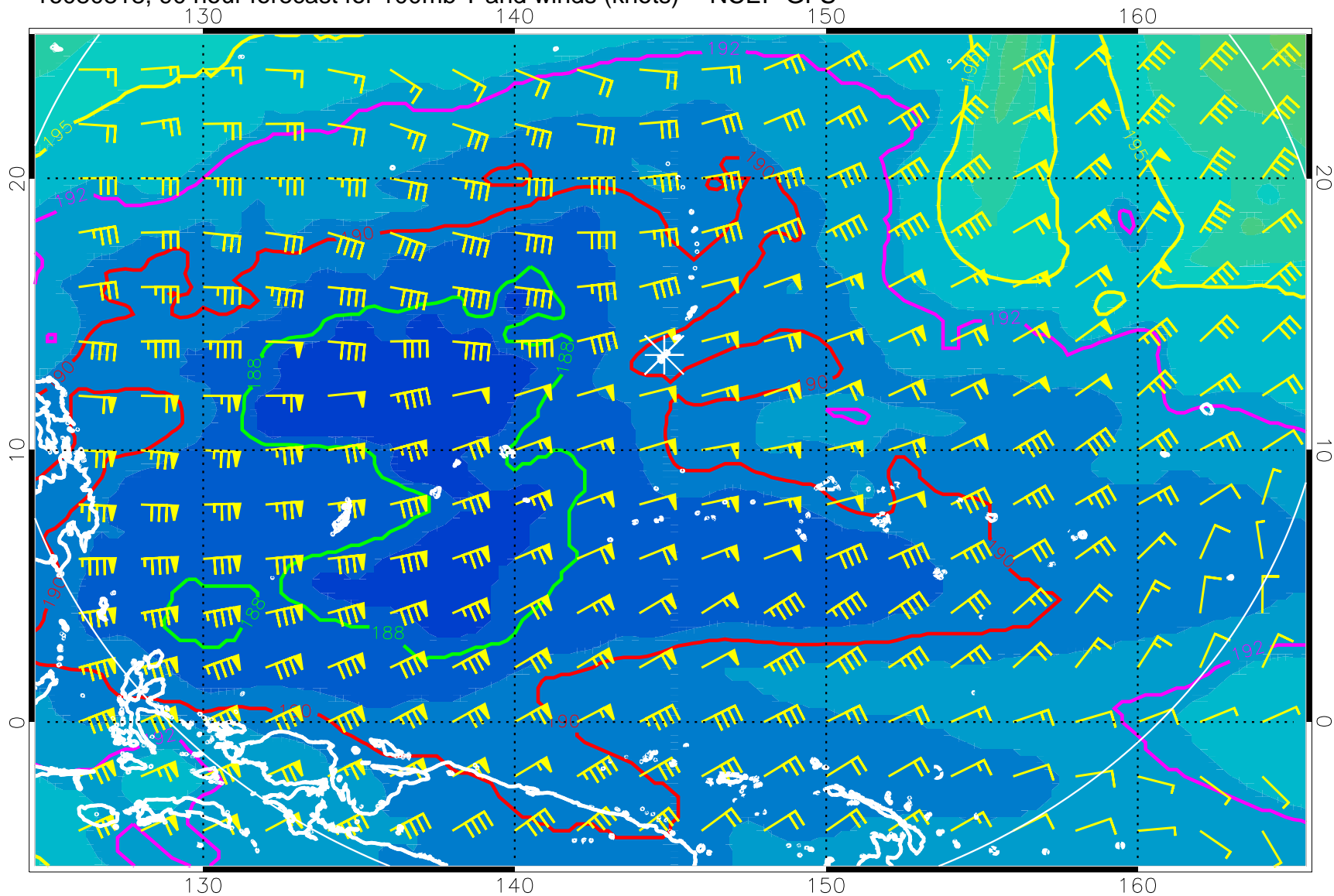
16080818, 90 hour forecast for 100mb T and winds (knots) -- NCEP GFS
