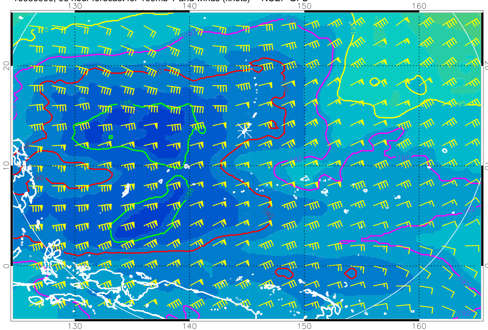
16080900, 96 hour forecast for 100mb T and winds (knots) -- NCEP GFS
