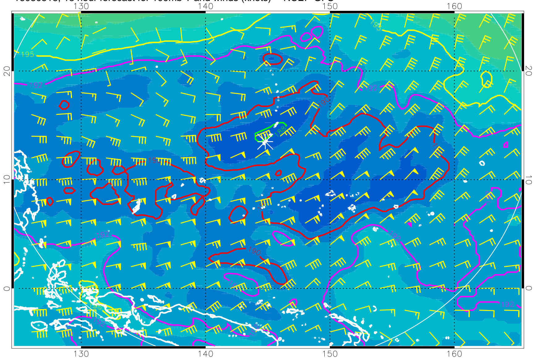
16080518, 18 hour forecast for 100mb T and winds (knots) -- NCEP GFS
