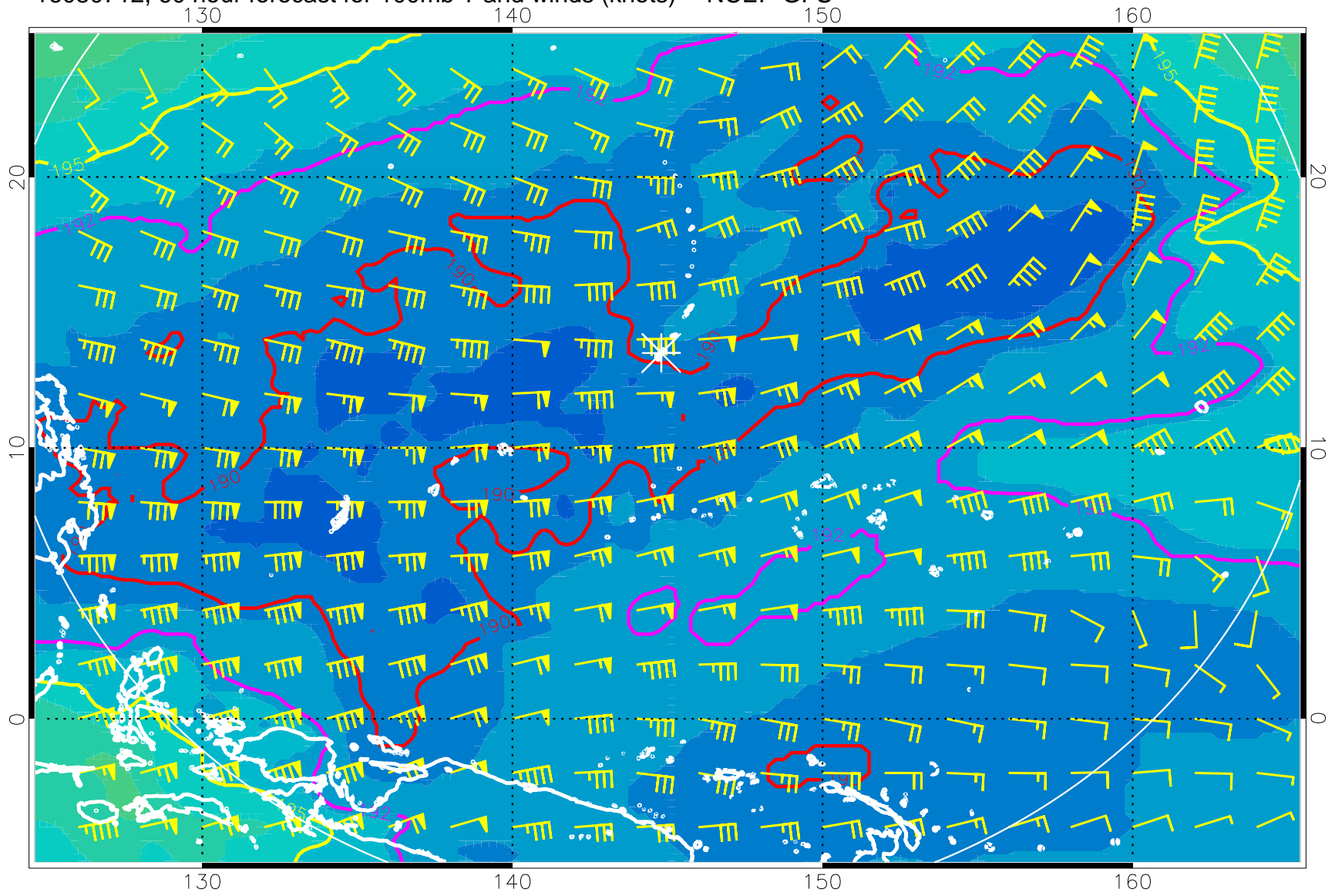
16080712, 60 hour forecast for 100mb T and winds (knots) -- NCEP GFS
