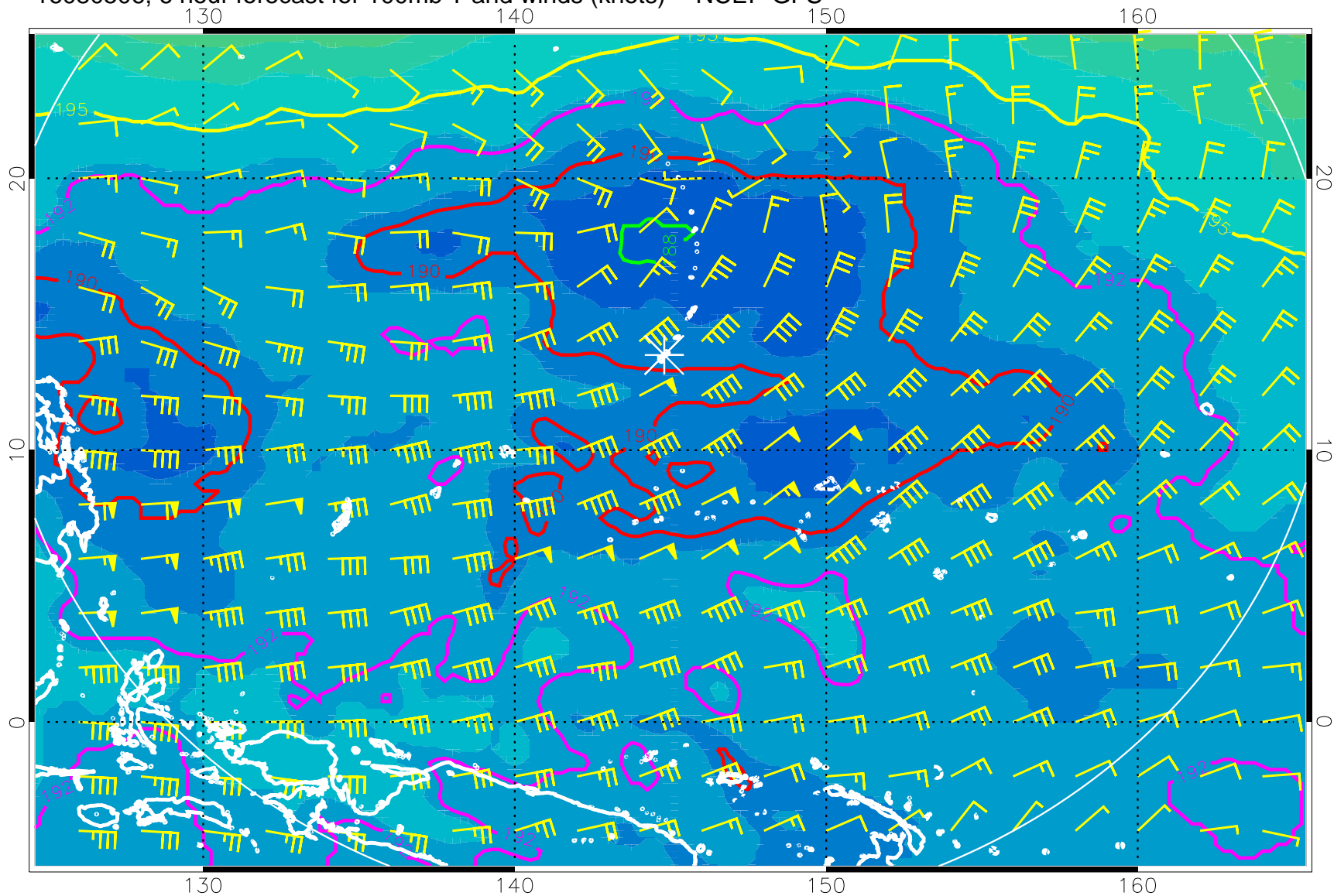
16080506, 6 hour forecast for 100mb T and winds (knots) -- NCEP GFS
