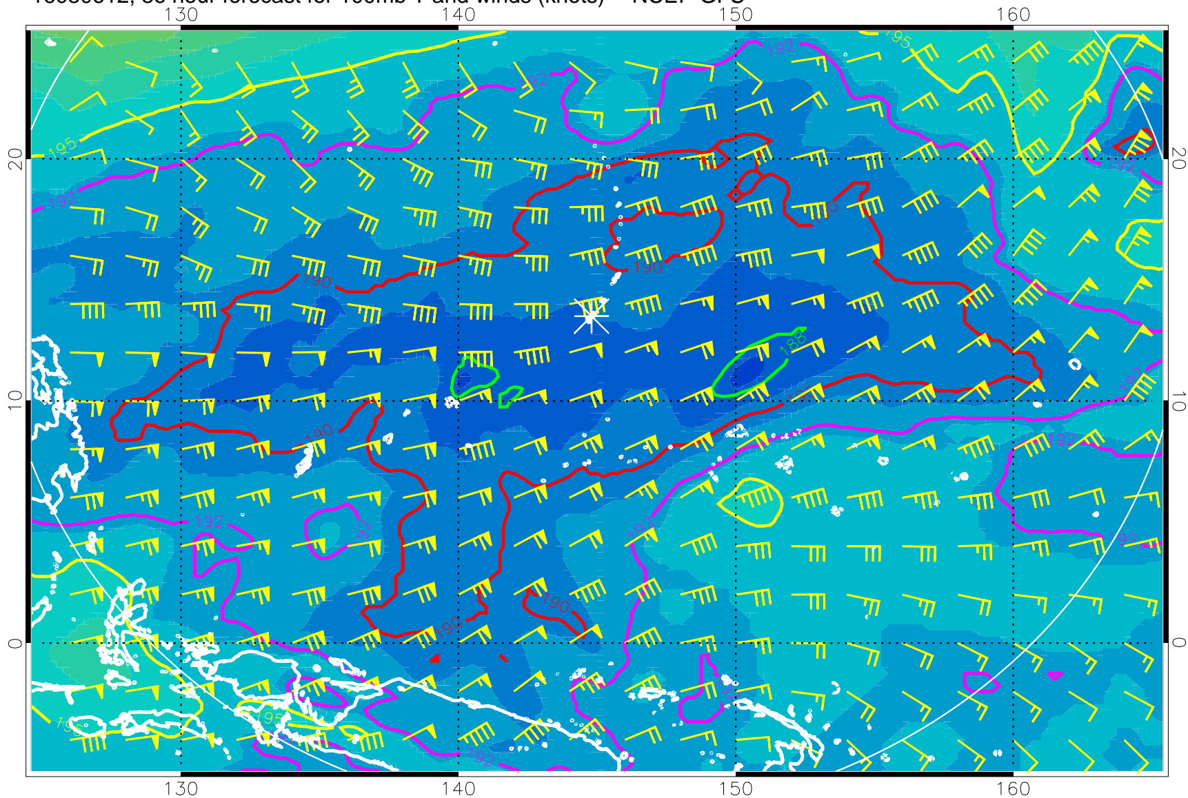
16080612, 36 hour forecast for 100mb T and winds (knots) -- NCEP GFS
