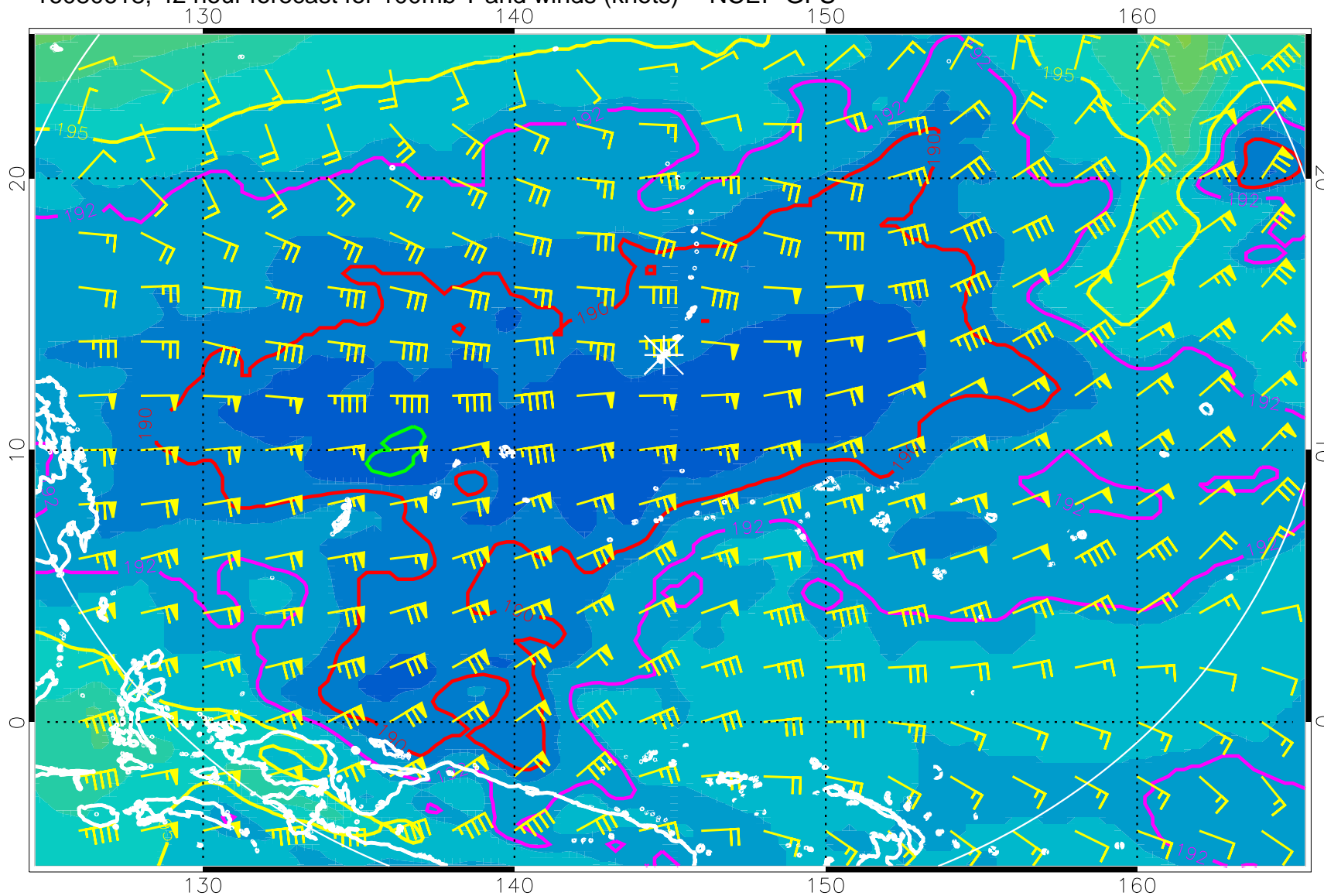
16080618, 42 hour forecast for 100mb T and winds (knots) -- NCEP GFS
