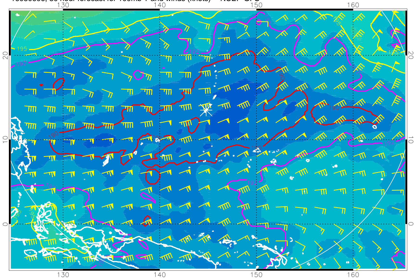
16080606, 30 hour forecast for 100mb T and winds (knots) -- NCEP GFS
