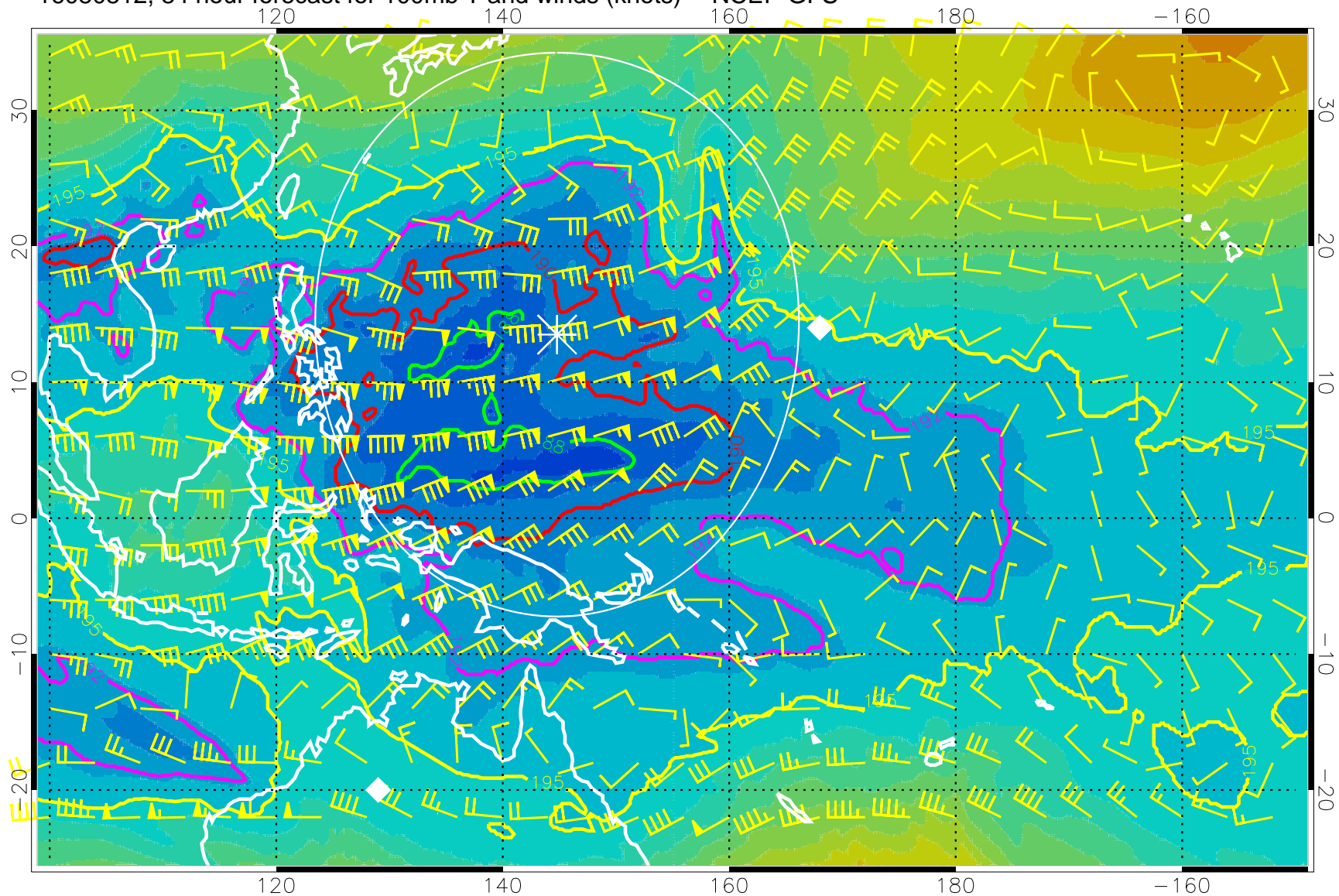
16080812, 84 hour forecast for 100mb T and winds (knots) -- NCEP GFS
