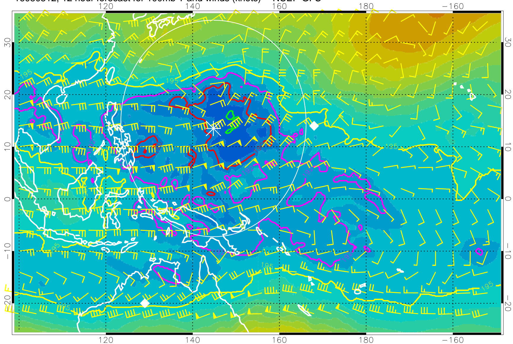
16080512, 12 hour forecast for 100mb T and winds (knots) -- NCEP GFS
