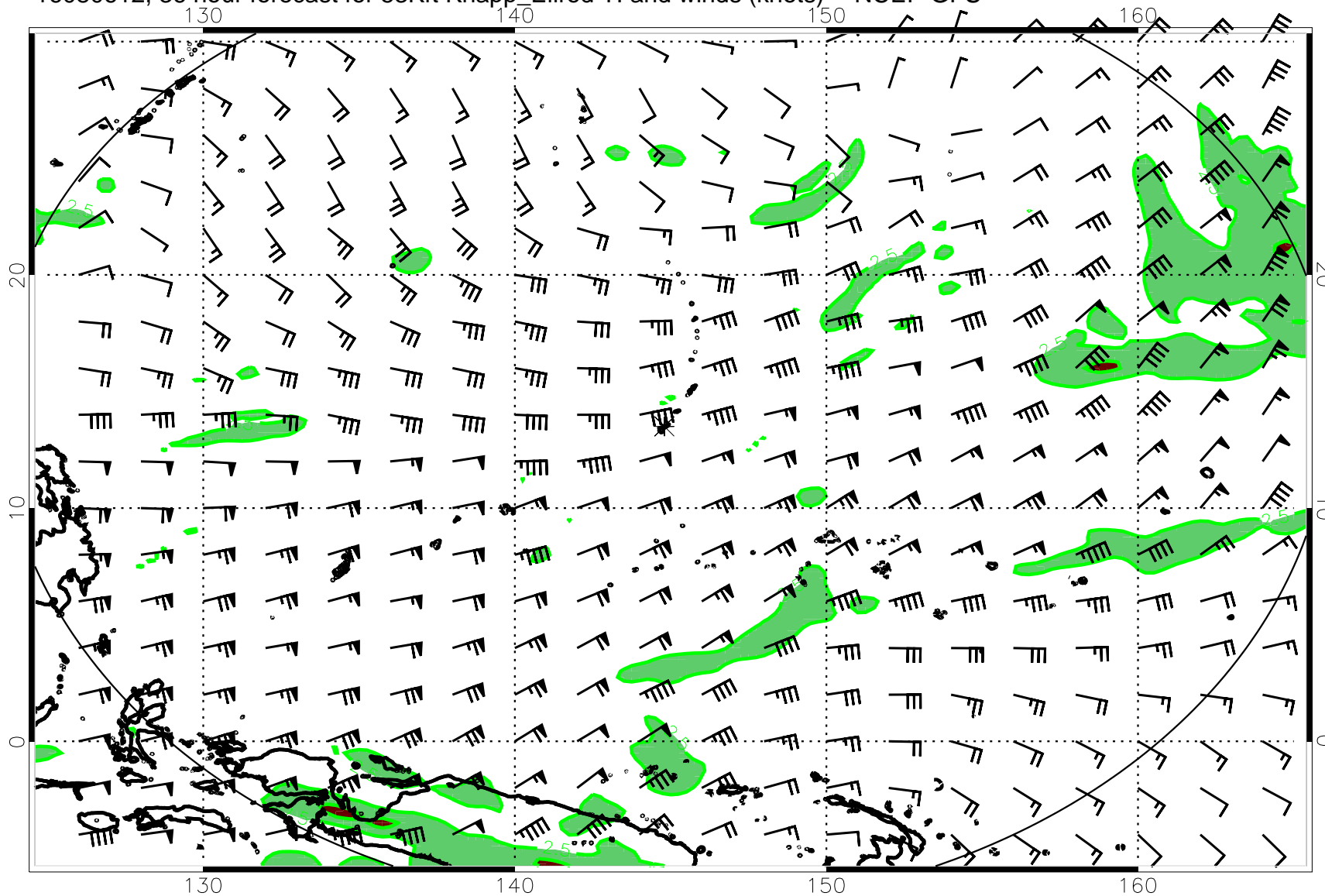
16080612, 36 hour forecast for 53Kft Knapp_Ellrod TI and winds (knots) -- NCEP GFS
