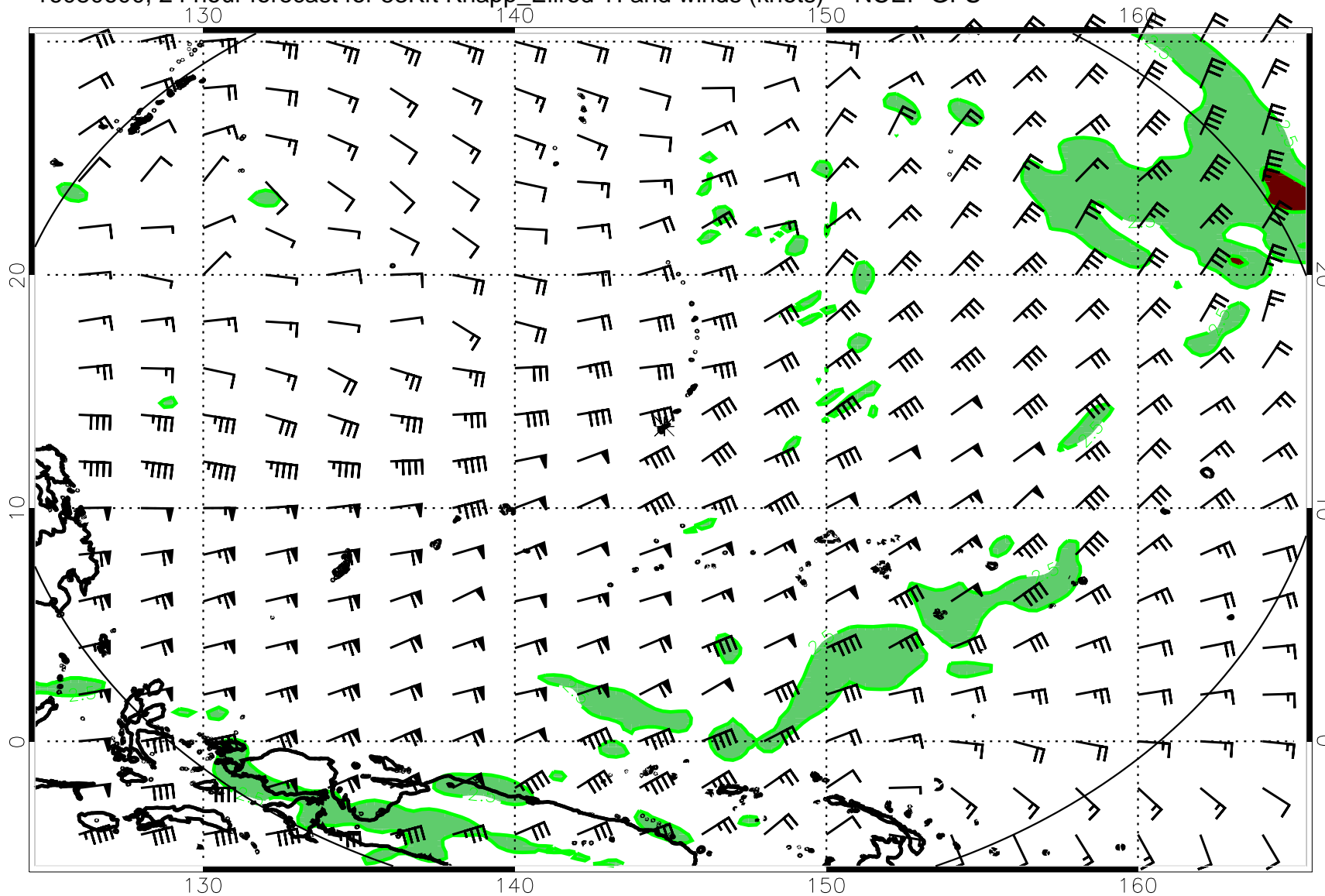
16080600, 24 hour forecast for 53Kft Knapp_Ellrod TI and winds (knots) -- NCEP GFS
