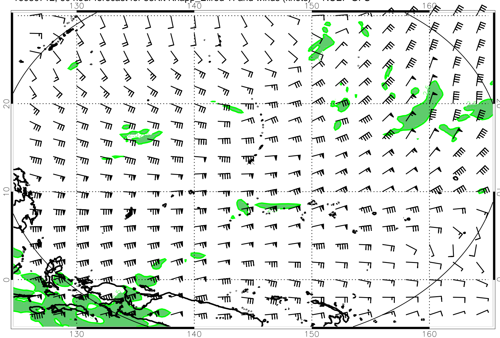
16080712, 60 hour forecast for 53Kft Knapp_Ellrod TI and winds (knots) -- NCEP GFS
