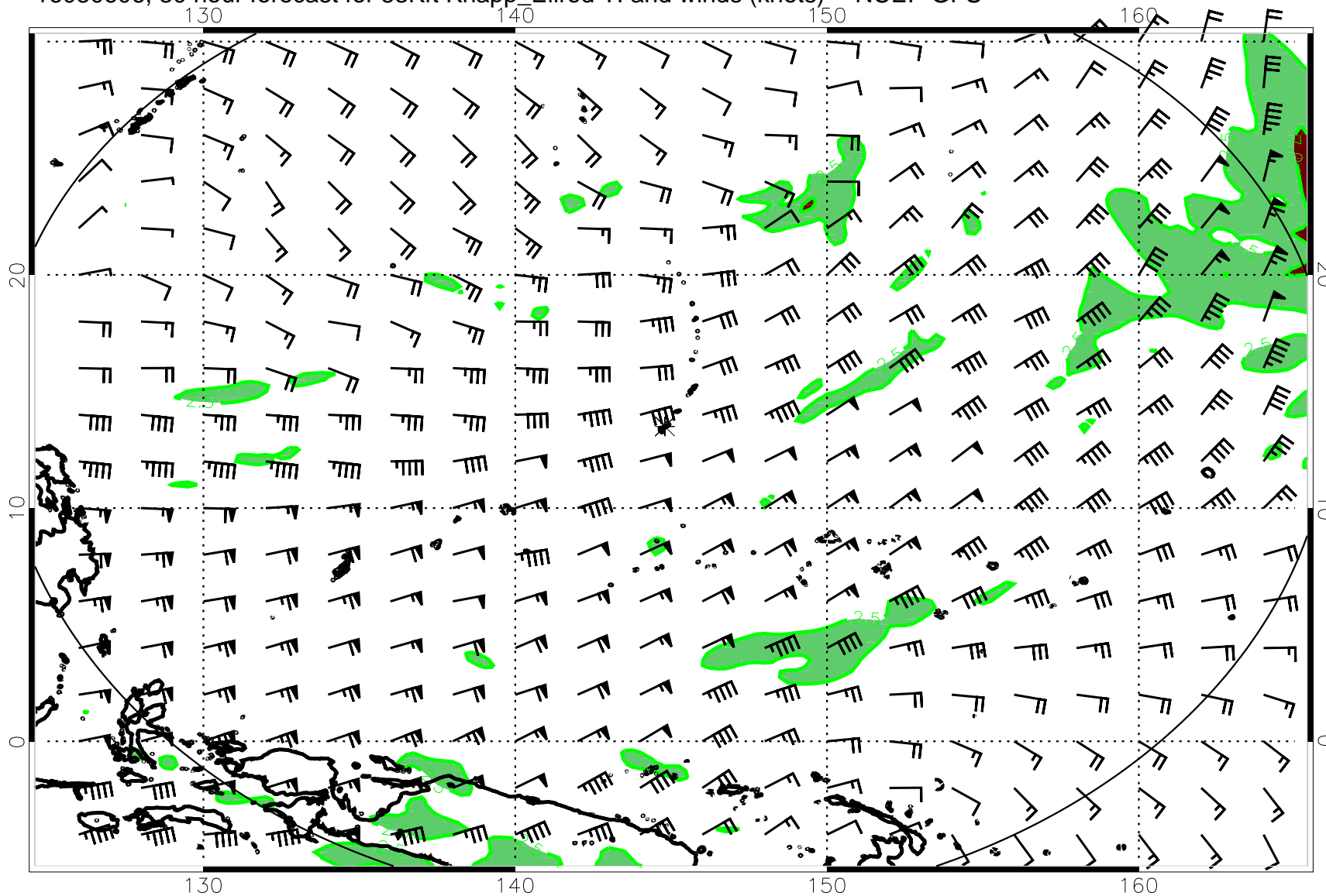
16080606, 30 hour forecast for 53Kft Knapp_Ellrod TI and winds (knots) -- NCEP GFS
