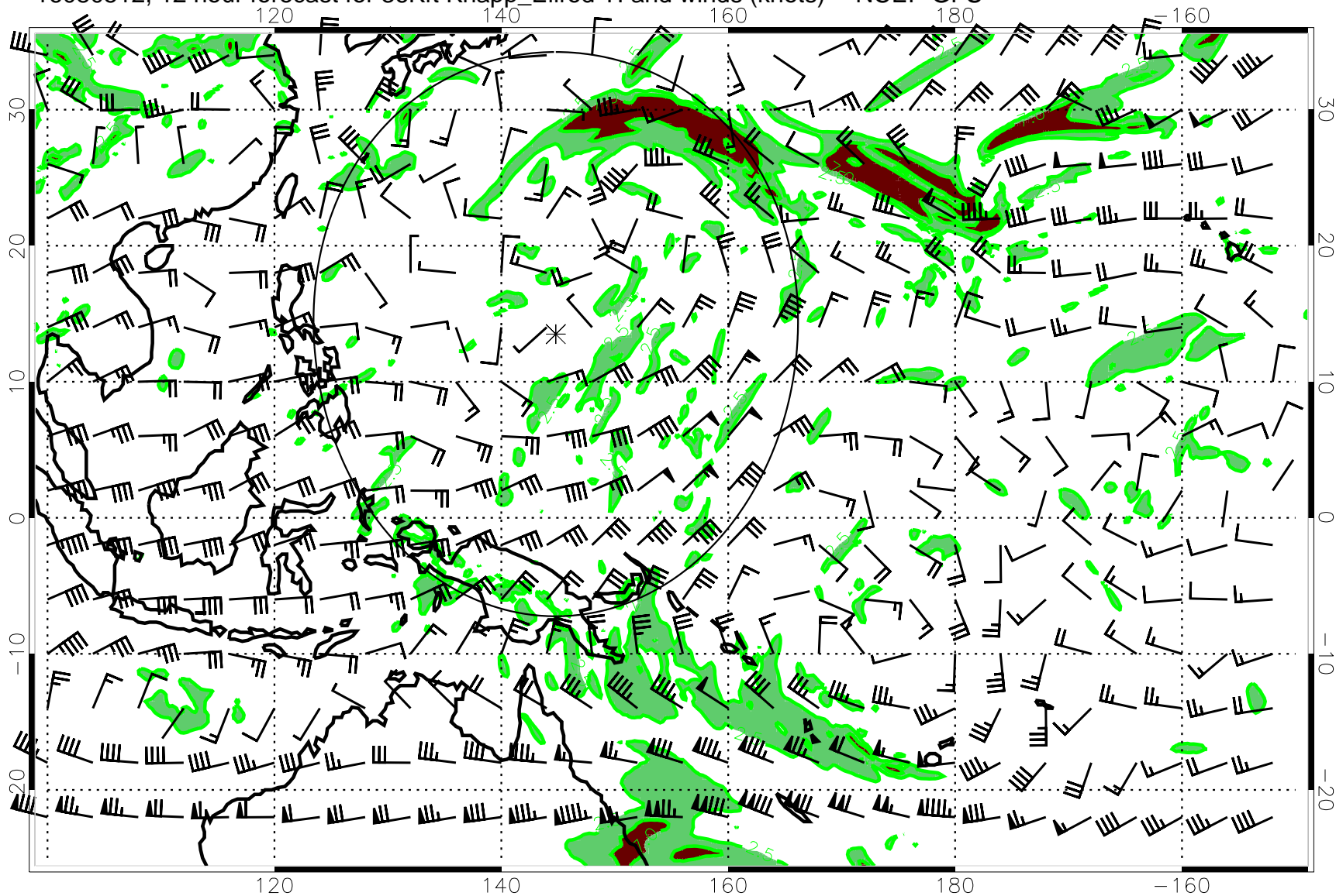
16080512, 12 hour forecast for 36Kft Knapp_Ellrod TI and winds (knots) -- NCEP GFS
