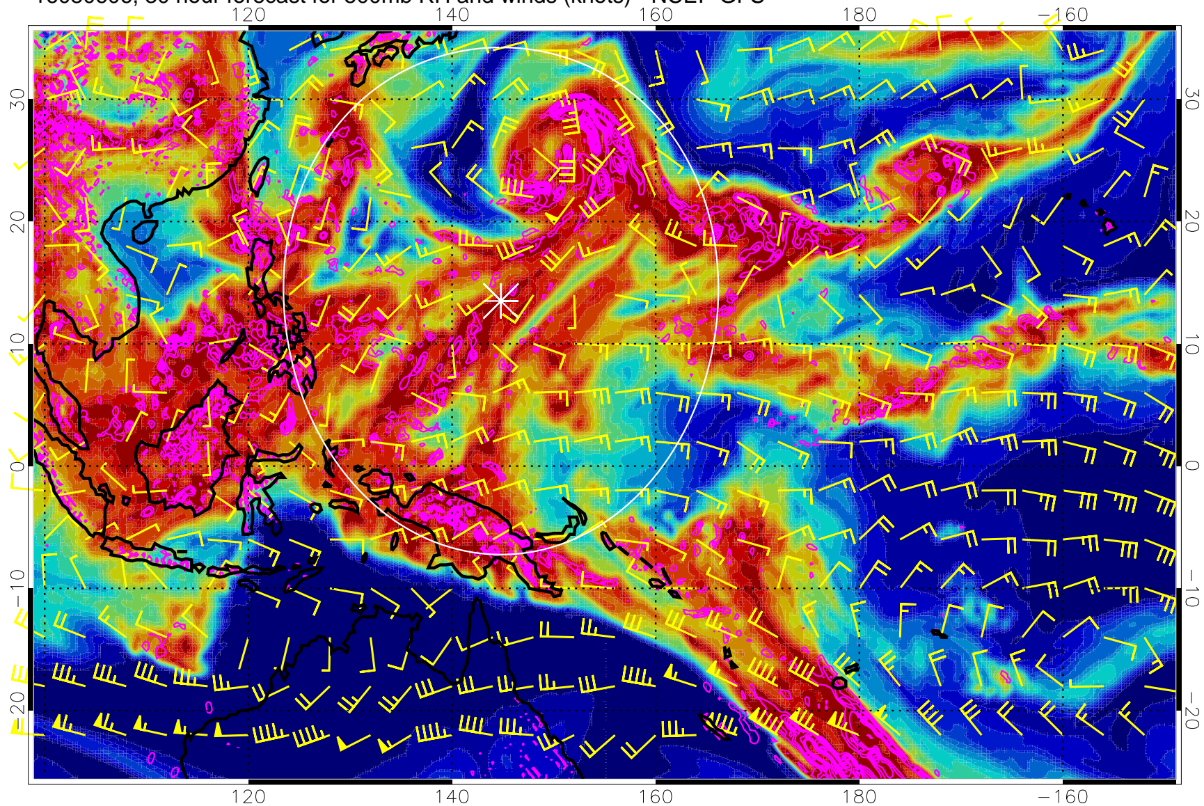
16080606, 30 hour forecast for 500mb RH and winds (knots) - NCEP GFS
