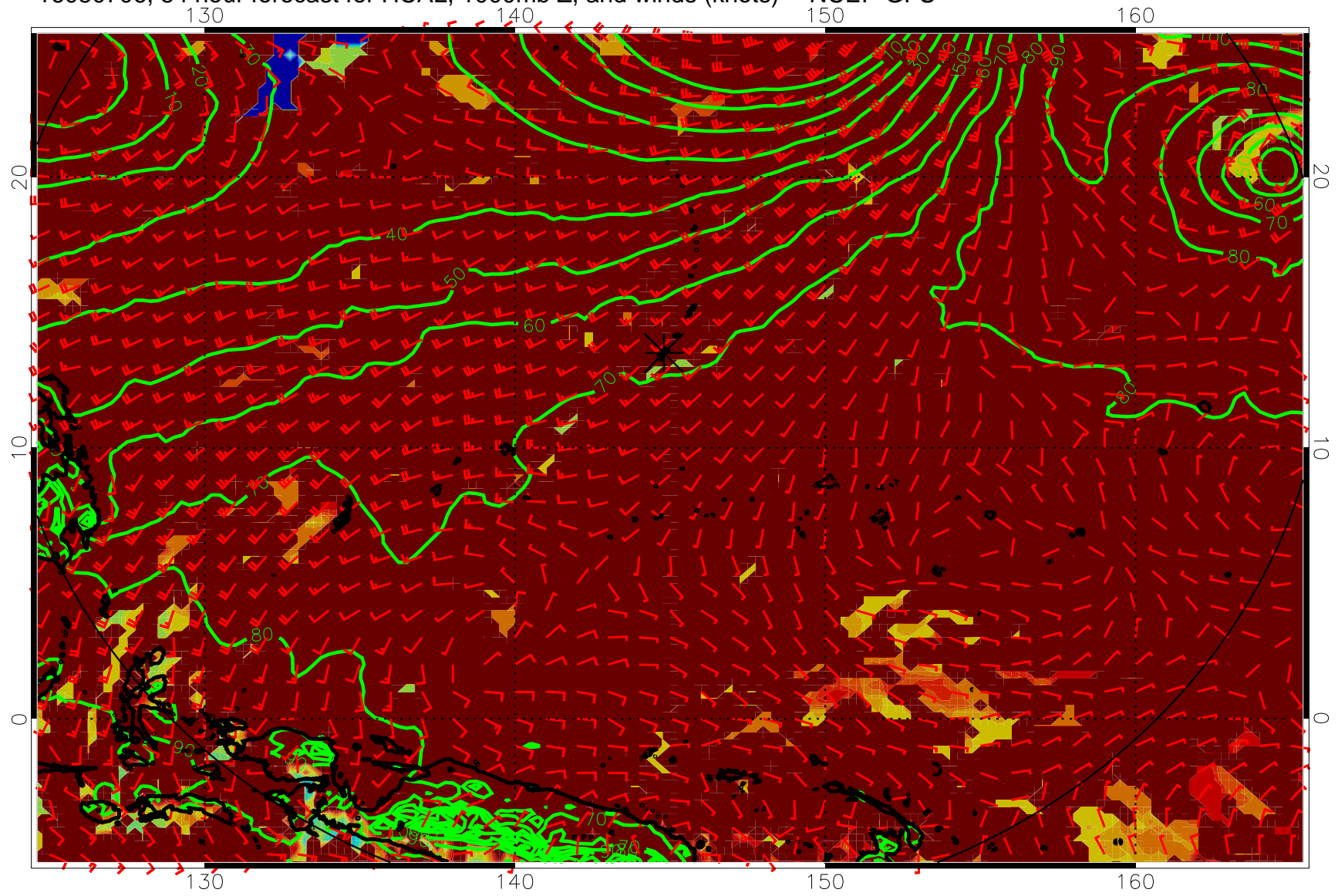
16080706, 54 hour forecast for HCAL, 1000mb Z, and winds (knots) -- NCEP GFS
