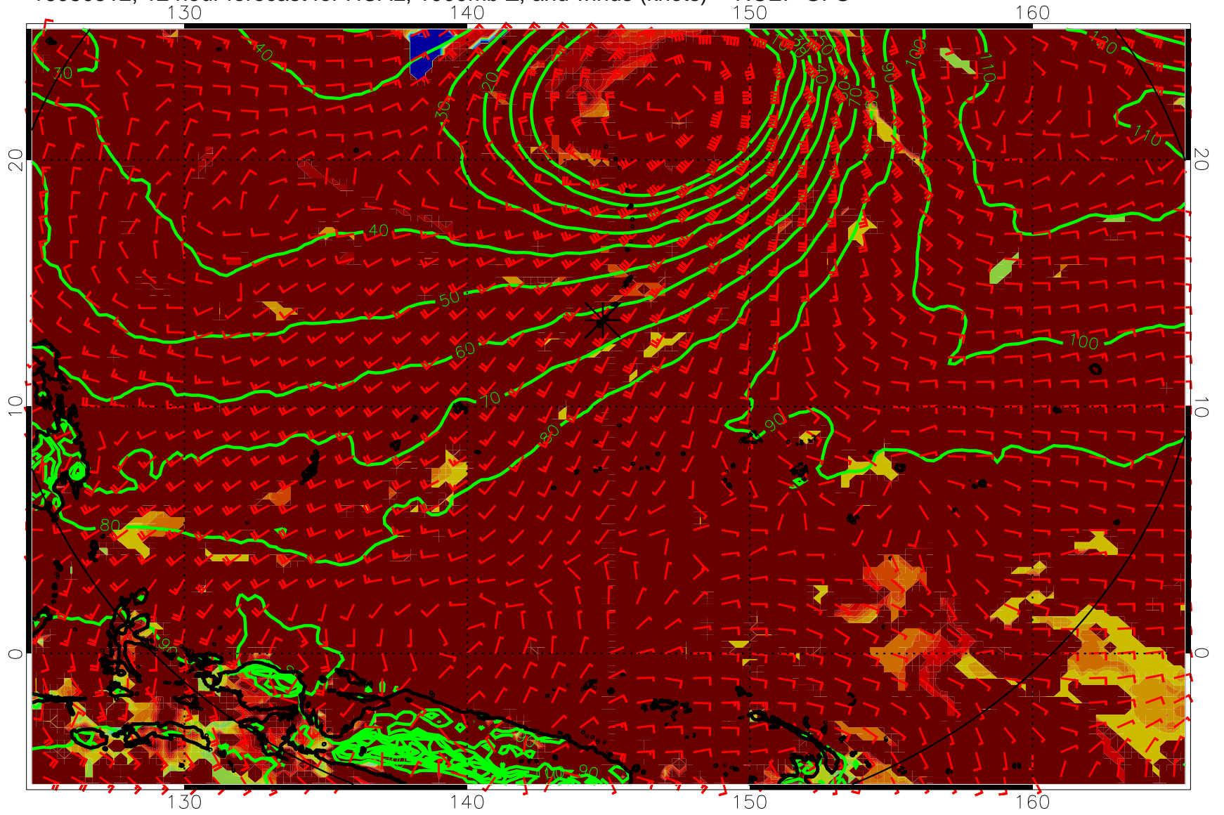
16080512, 12 hour forecast for HCAL, 1000mb Z, and winds (knots) -- NCEP GFS
