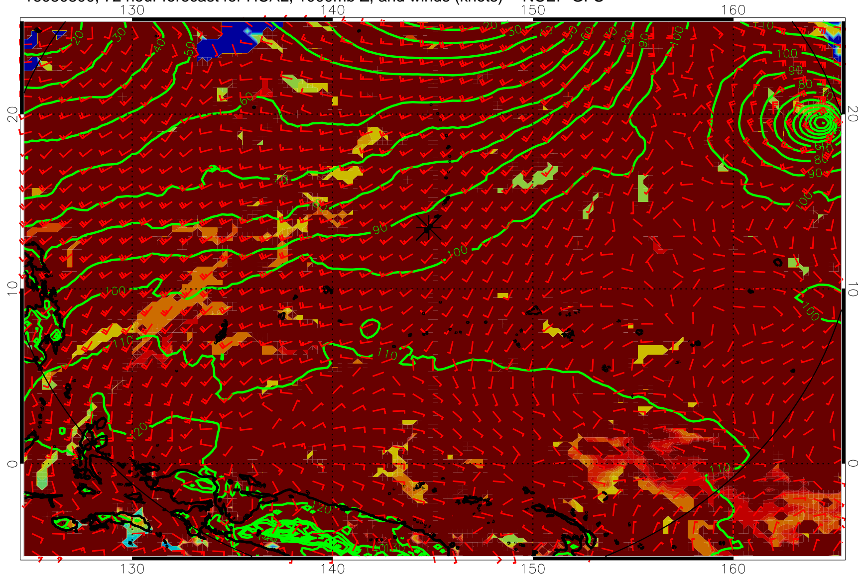
16080800, 72 hour forecast for HCAL, 1000mb Z, and winds (knots) -- NCEP GFS
