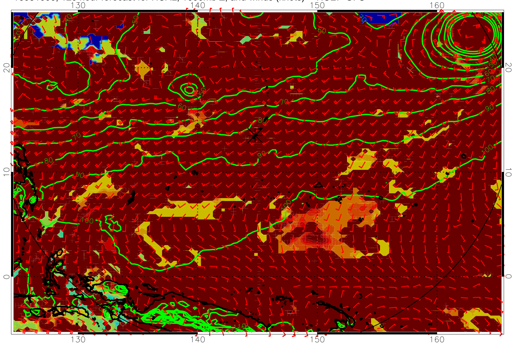
16081000, 120 hour forecast for HCAL, 1000mb Z, and winds (knots) -- NCEP GFS
