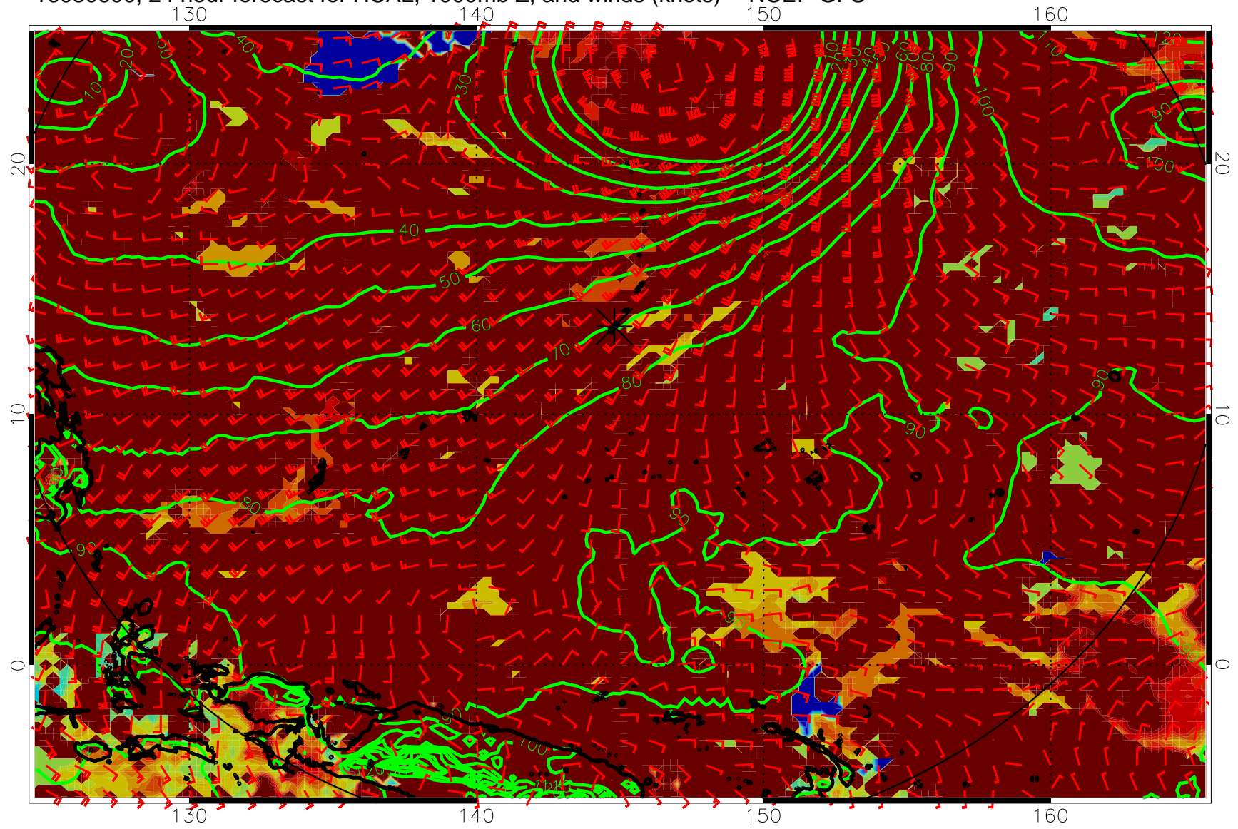
16080600, 24 hour forecast for HCAL, 1000mb Z, and winds (knots) -- NCEP GFS
