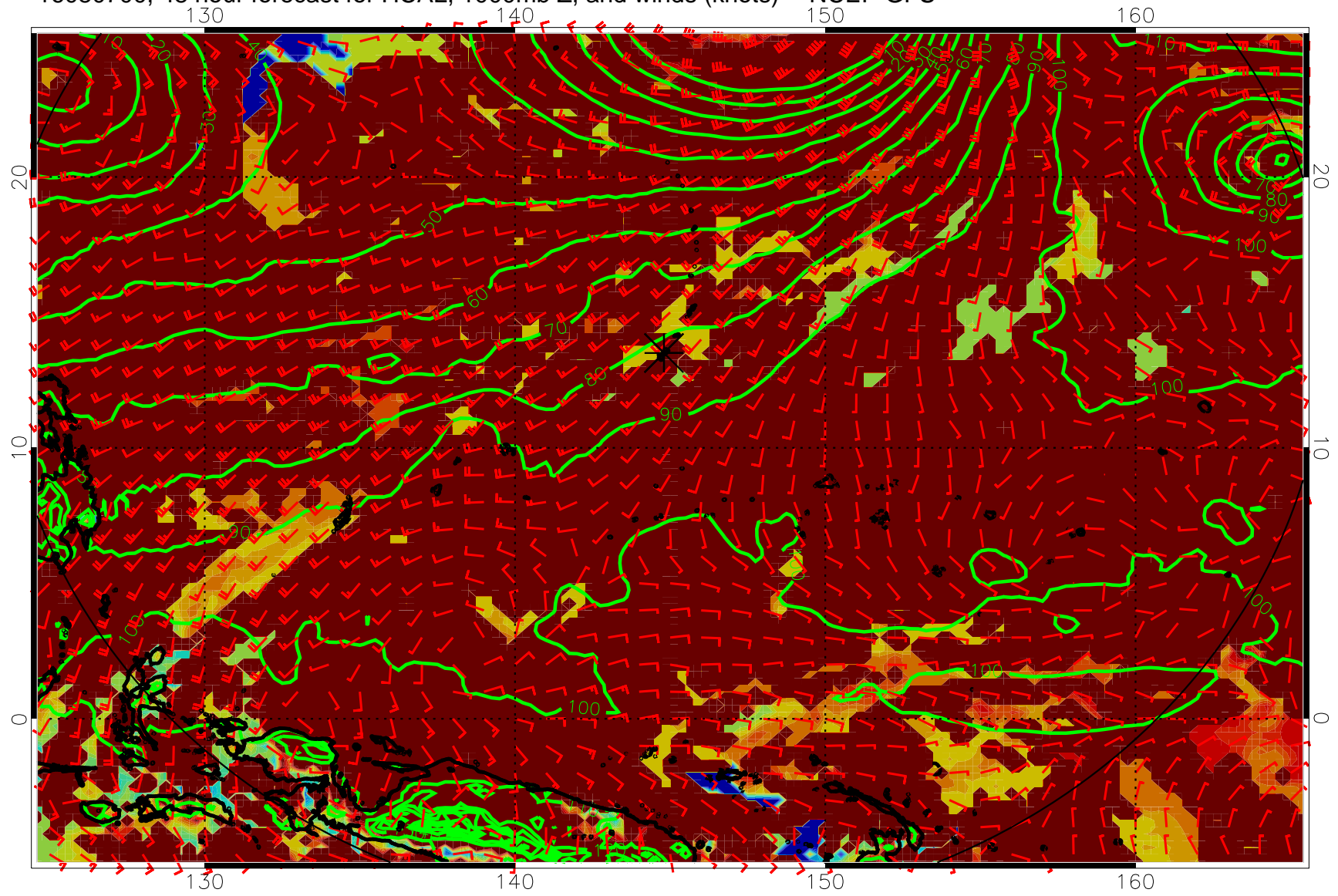
16080700, 48 hour forecast for HCAL, 1000mb Z, and winds (knots) -- NCEP GFS
