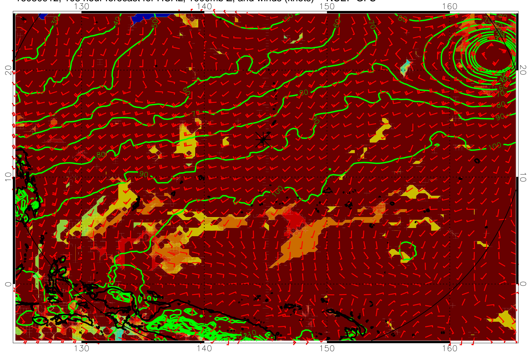
16080912, 108 hour forecast for HCAL, 1000mb Z, and winds (knots) -- NCEP GFS
