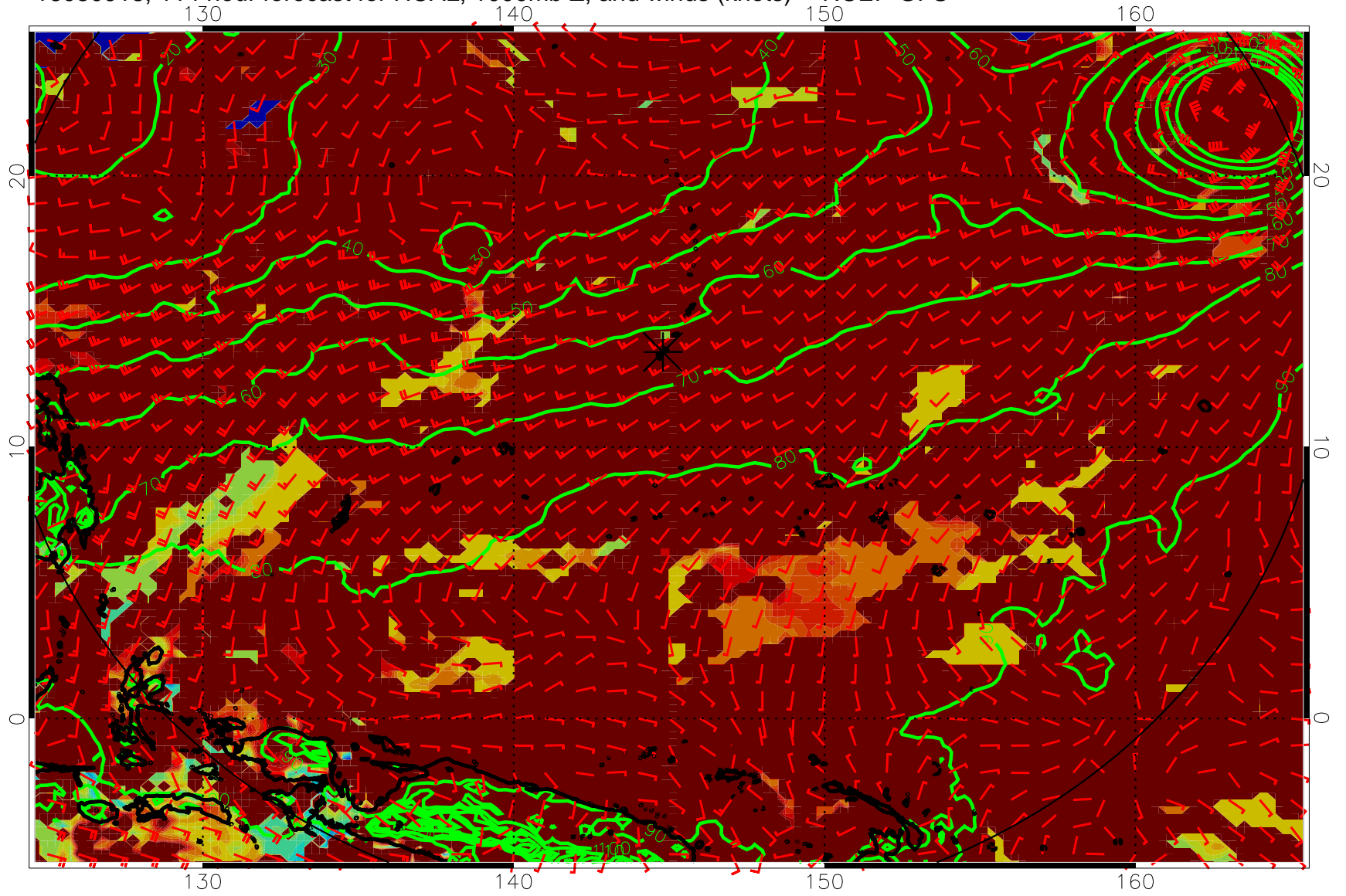
16080918, 114 hour forecast for HCAL, 1000mb Z, and winds (knots) -- NCEP GFS
