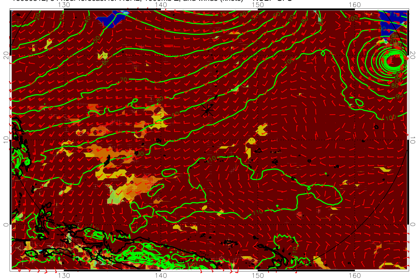
16080812, 84 hour forecast for HCAL, 1000mb Z, and winds (knots) -- NCEP GFS
