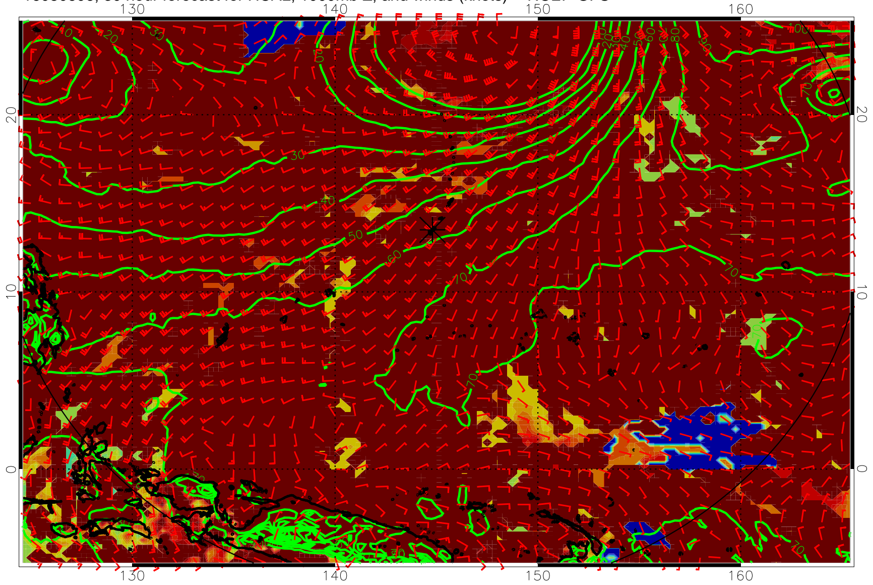
16080606, 30 hour forecast for HCAL, 1000mb Z, and winds (knots) -- NCEP GFS
