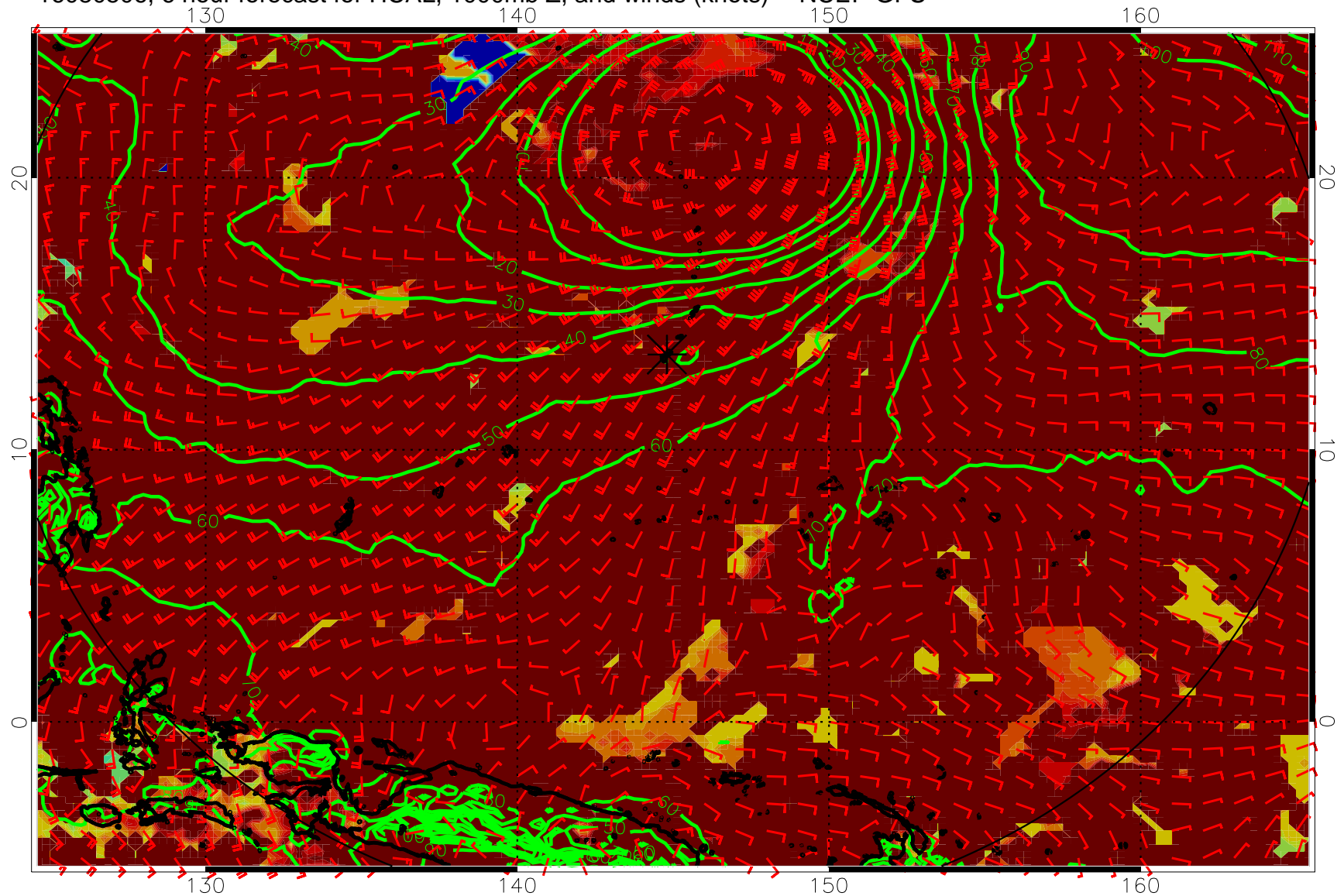
16080506, 6 hour forecast for HCAL, 1000mb Z, and winds (knots) -- NCEP GFS
