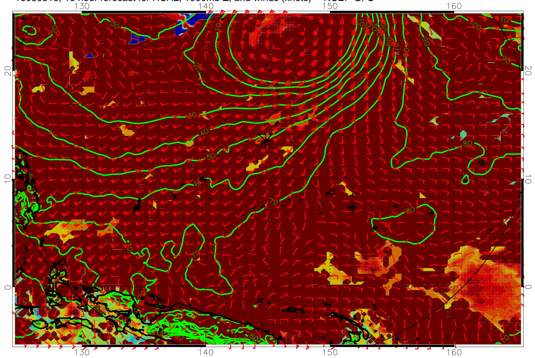
16080518, 18 hour forecast for HCAL, 1000mb Z, and winds (knots) -- NCEP GFS
