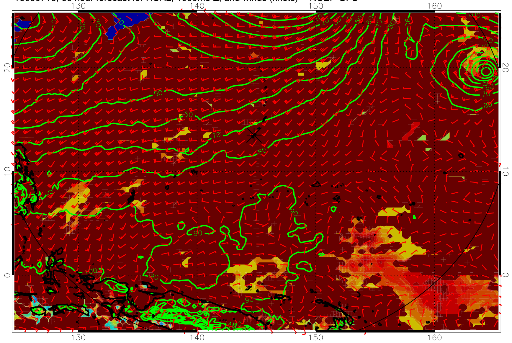
16080718, 66 hour forecast for HCAL, 1000mb Z, and winds (knots) -- NCEP GFS
