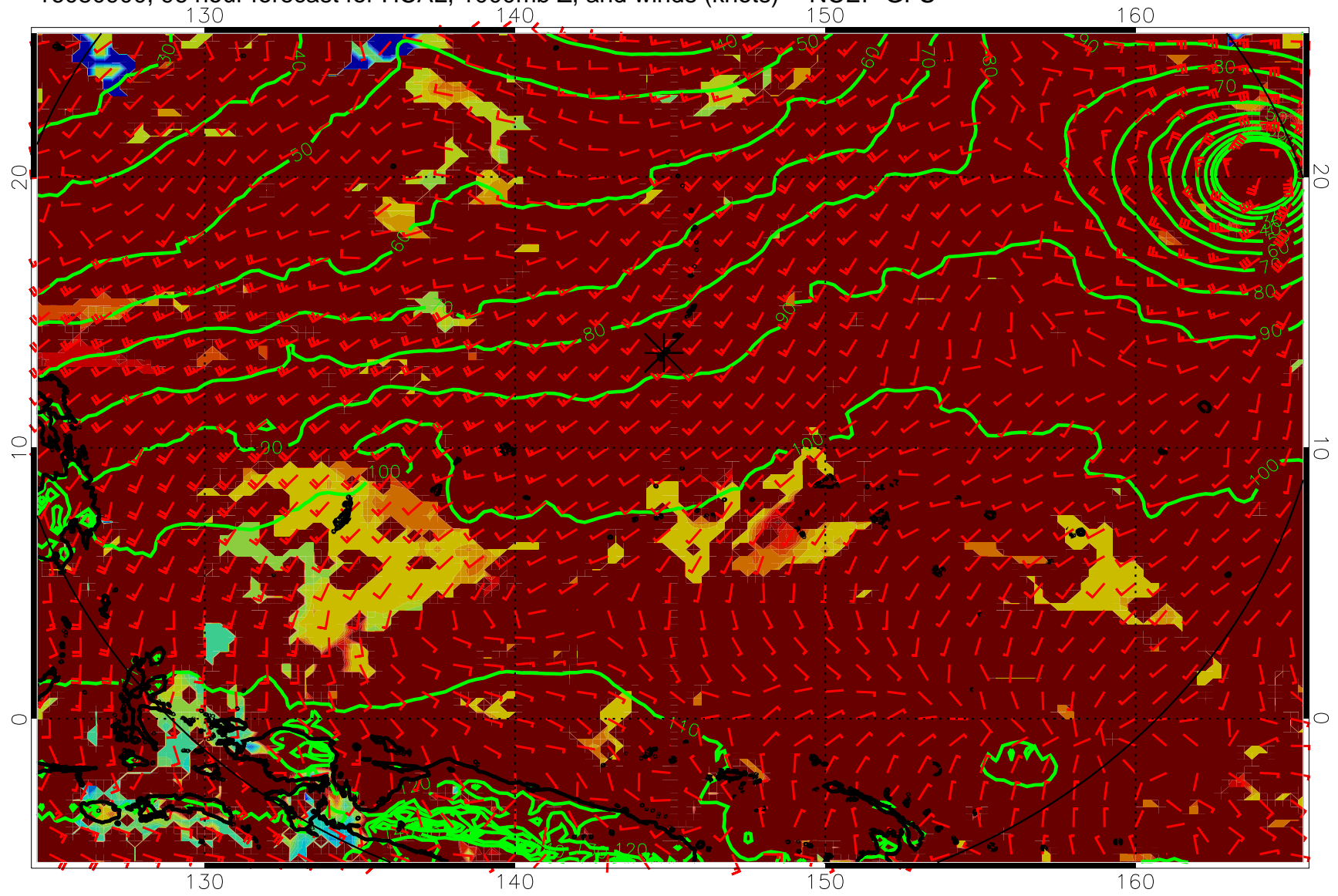
16080900, 96 hour forecast for HCAL, 1000mb Z, and winds (knots) -- NCEP GFS
