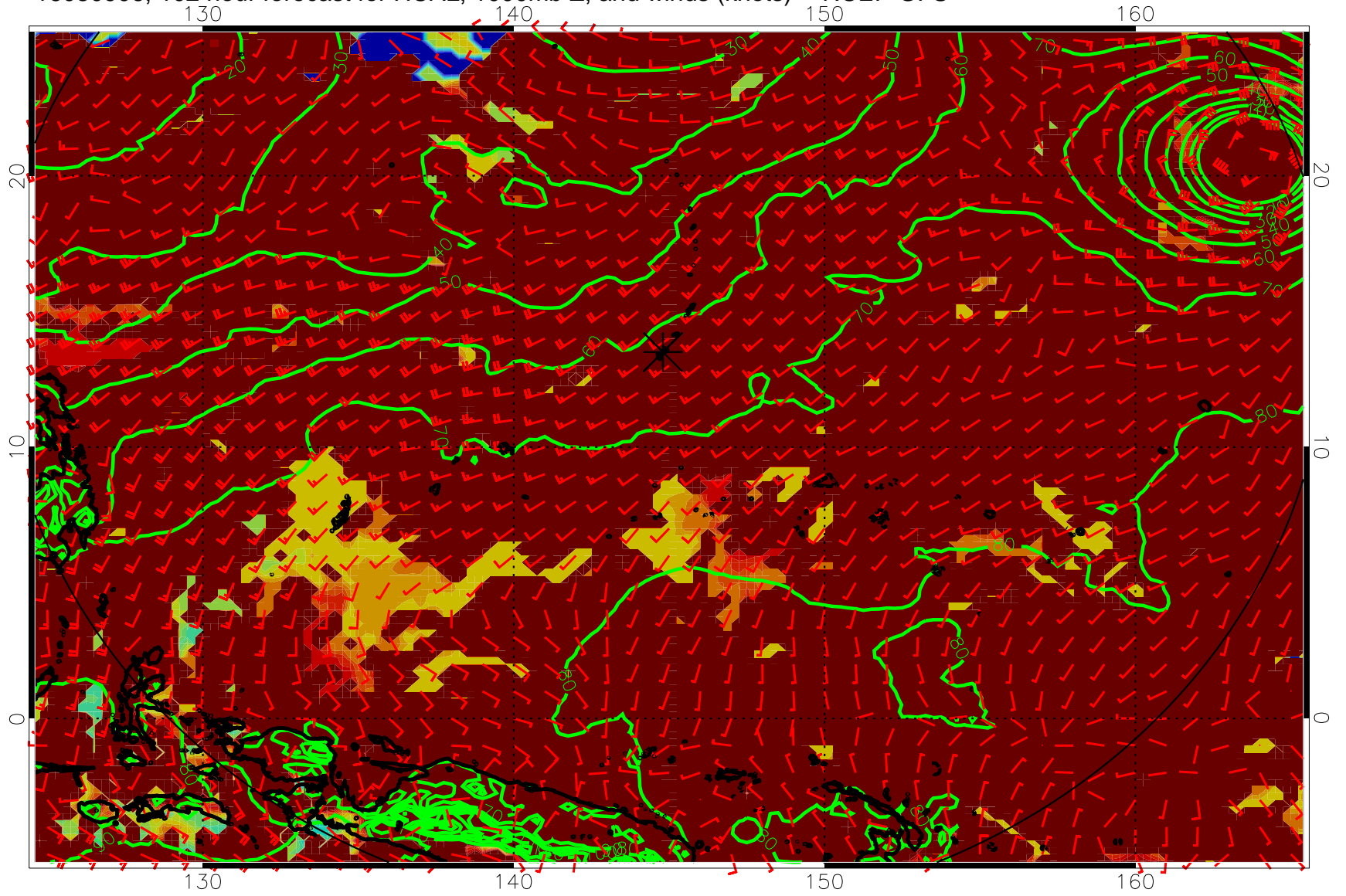
16080906, 102 hour forecast for HCAL, 1000mb Z, and winds (knots) -- NCEP GFS
