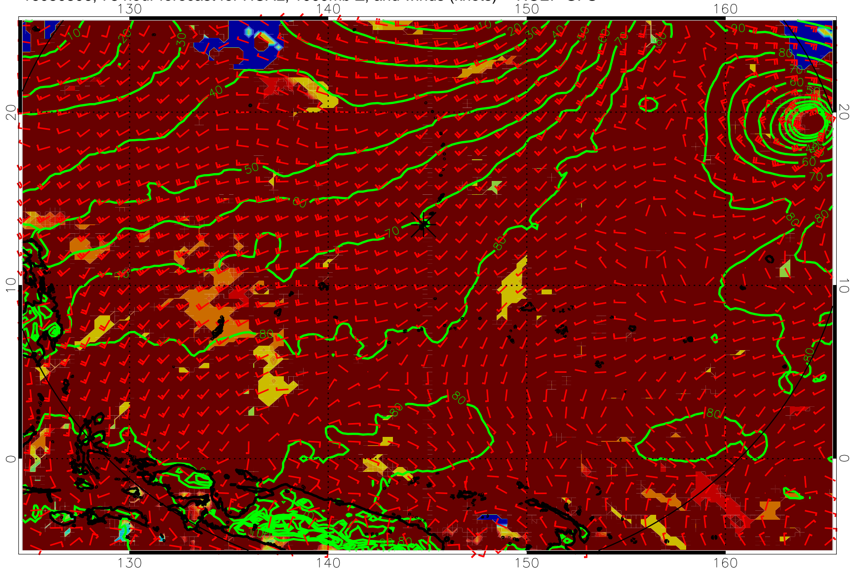
16080806, 78 hour forecast for HCAL, 1000mb Z, and winds (knots) -- NCEP GFS
