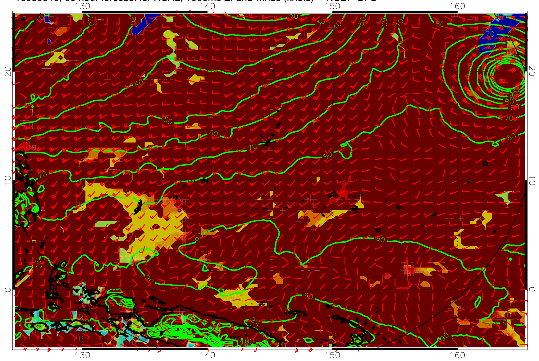
16080818, 90 hour forecast for HCAL, 1000mb Z, and winds (knots) -- NCEP GFS
