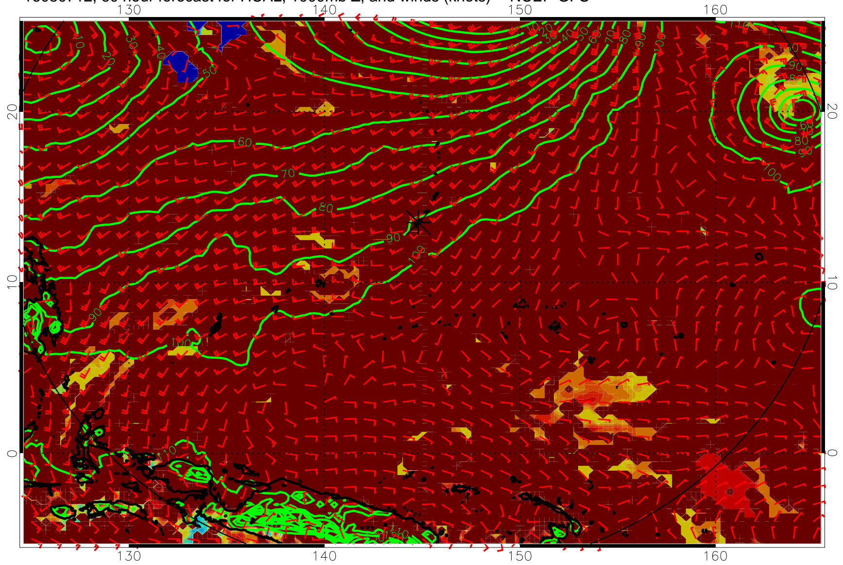
16080712, 60 hour forecast for HCAL, 1000mb Z, and winds (knots) -- NCEP GFS
