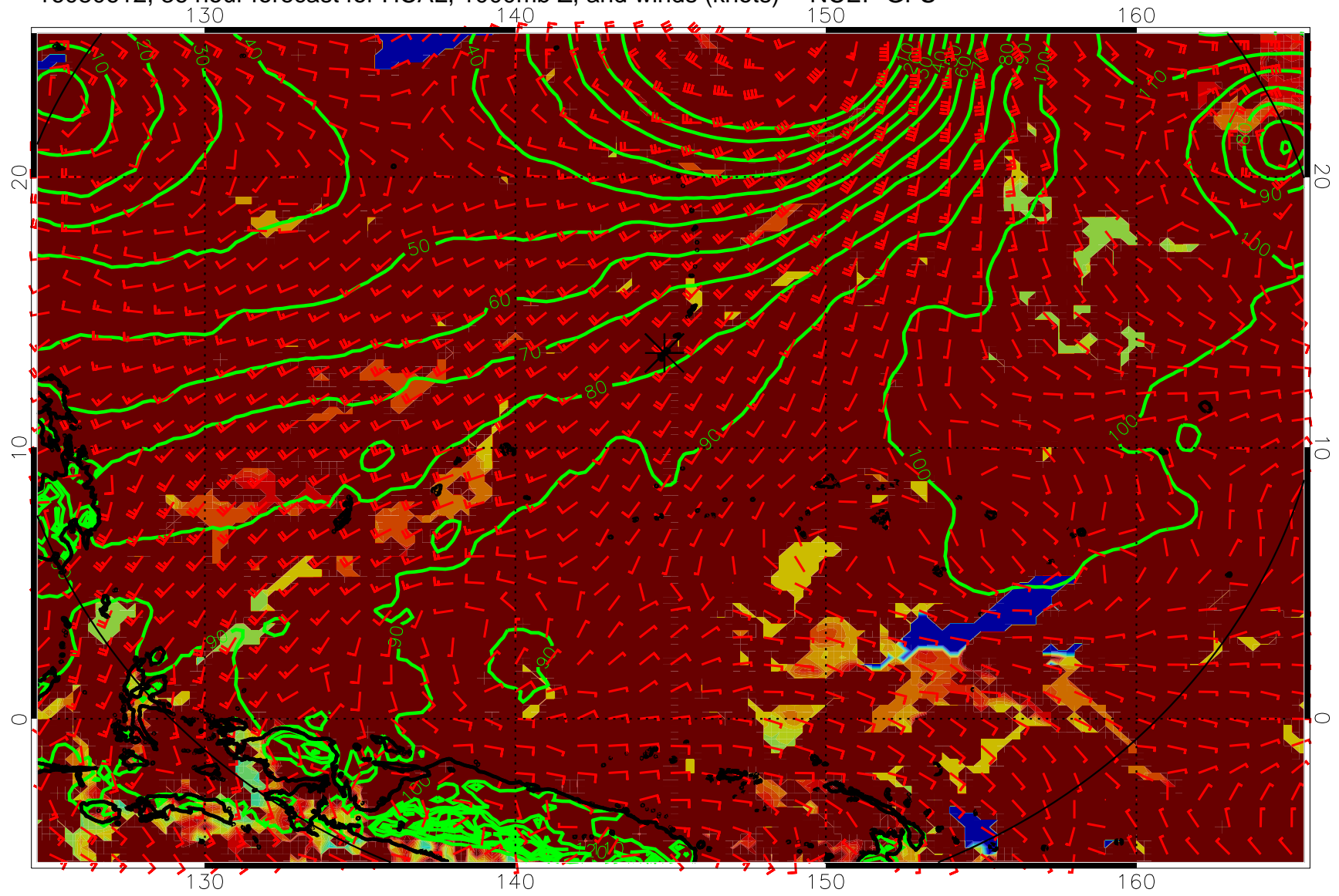
16080612, 36 hour forecast for HCAL, 1000mb Z, and winds (knots) -- NCEP GFS
