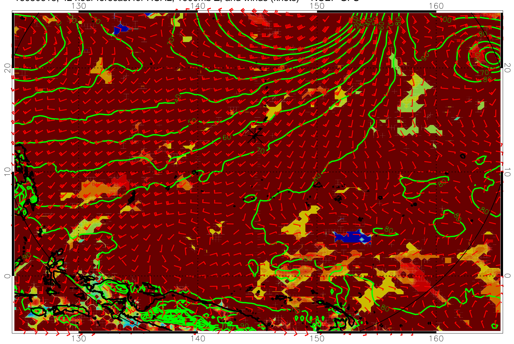
16080618, 42 hour forecast for HCAL, 1000mb Z, and winds (knots) -- NCEP GFS
