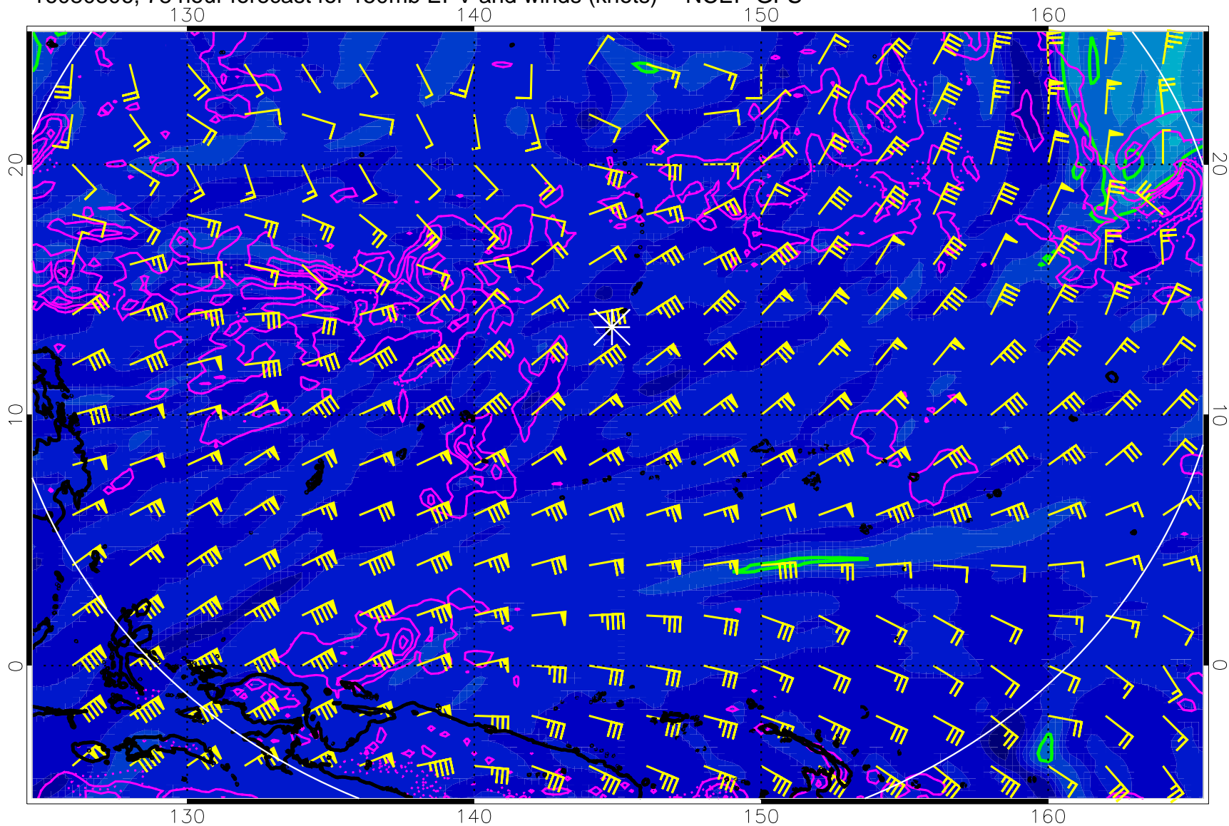
16080806, 78 hour forecast for 150mb EPV and winds (knots) -- NCEP GFS
