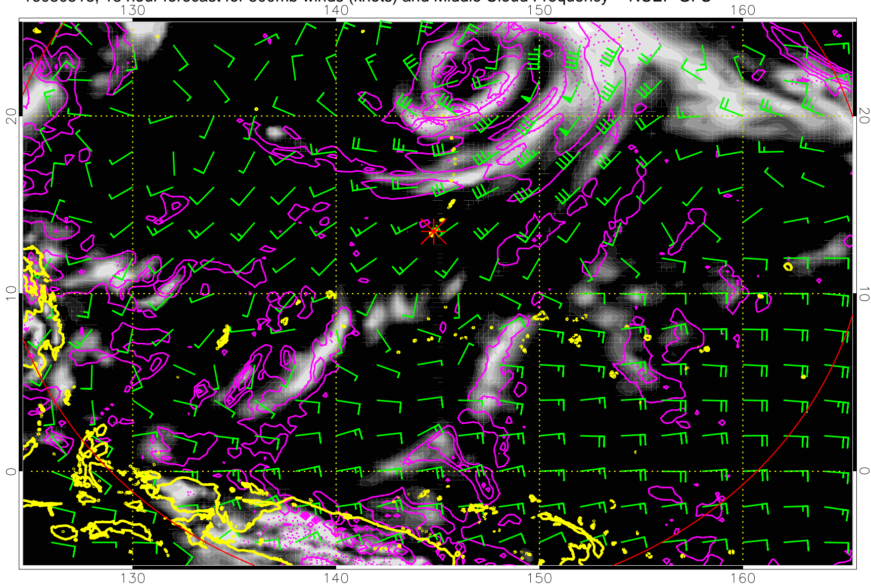
16080518, 18 hour forecast for 500mb winds (knots) and Middle Cloud Frequency -- NCEP GFS
