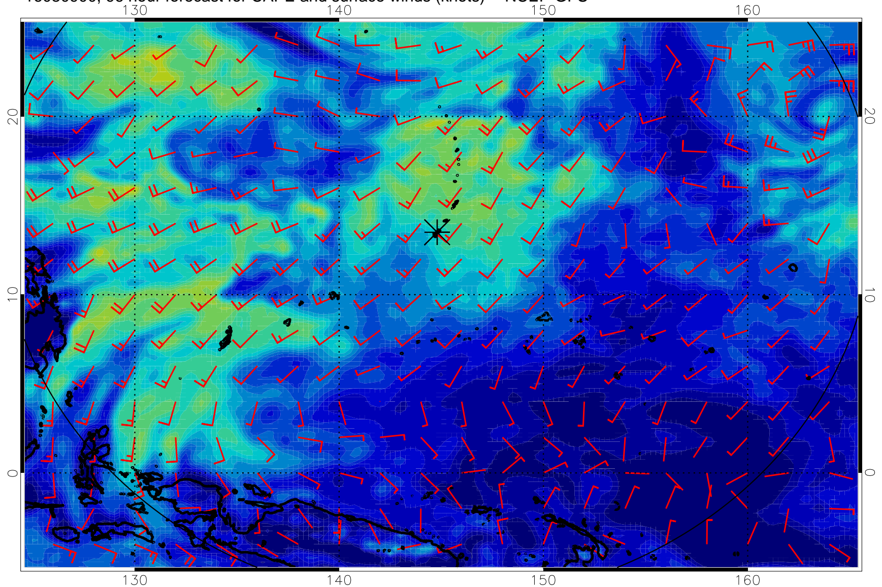
16080900, 96 hour forecast for CAPE and surface winds (knots) -- NCEP GFS
