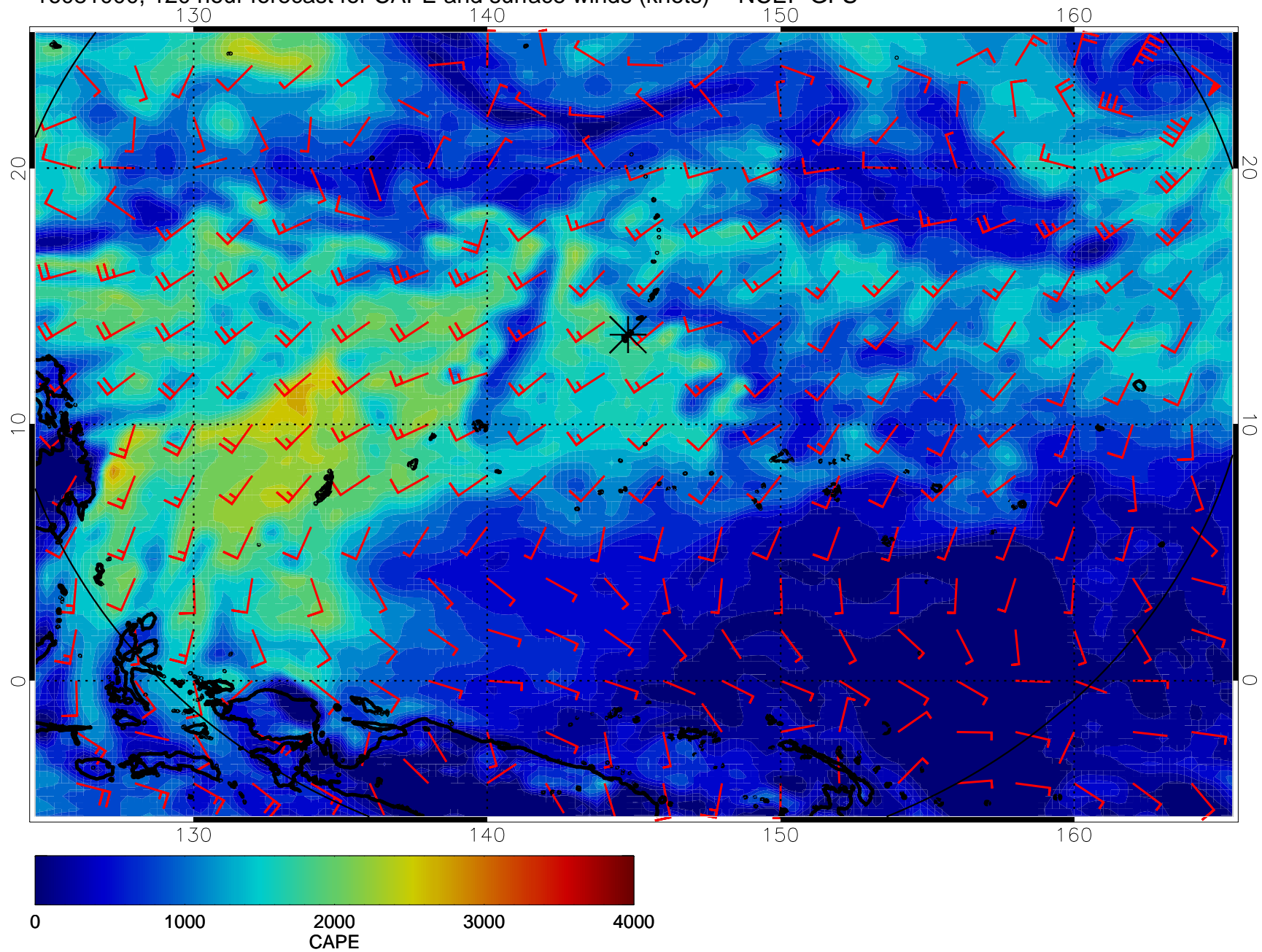
16081000, 120 hour forecast for CAPE and surface winds (knots) -- NCEP GFS
