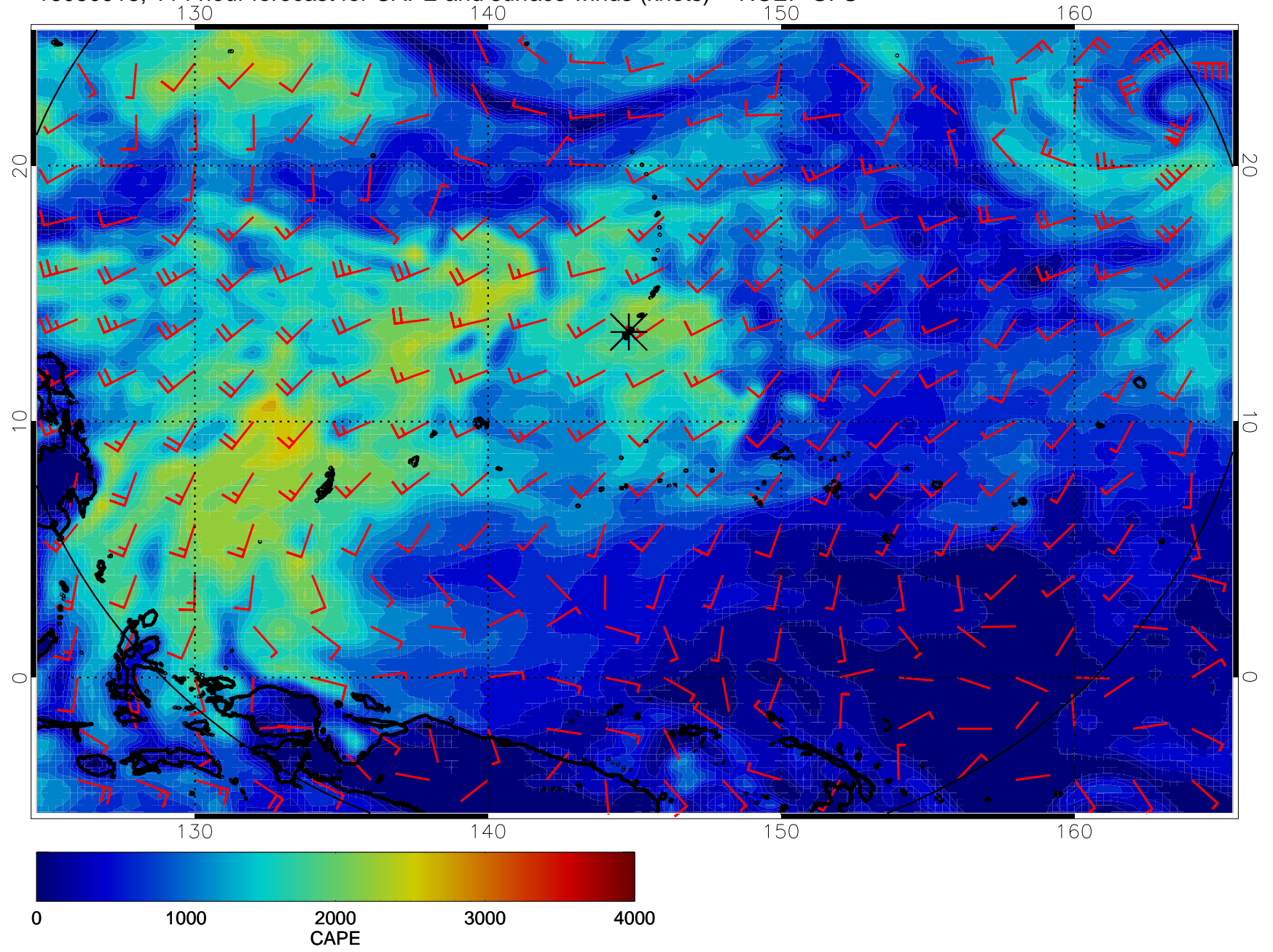
16080918, 114 hour forecast for CAPE and surface winds (knots) -- NCEP GFS
