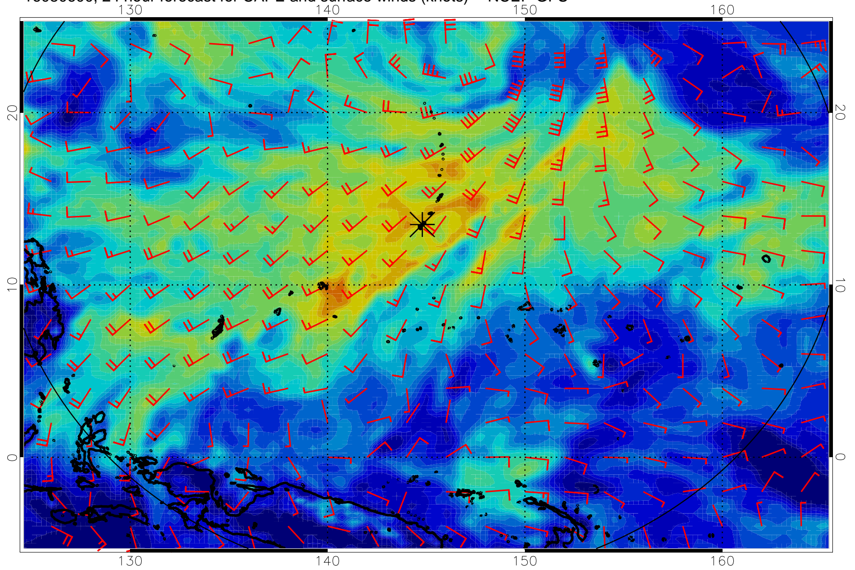
16080600, 24 hour forecast for CAPE and surface winds (knots) -- NCEP GFS
