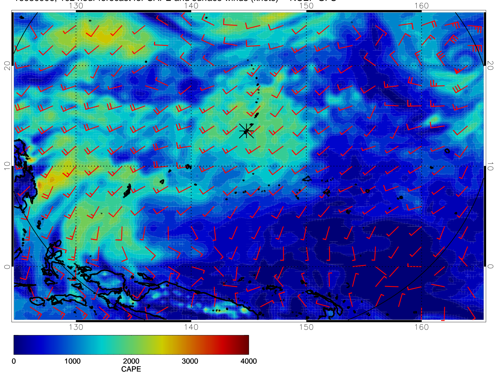
16080906, 102 hour forecast for CAPE and surface winds (knots) -- NCEP GFS
