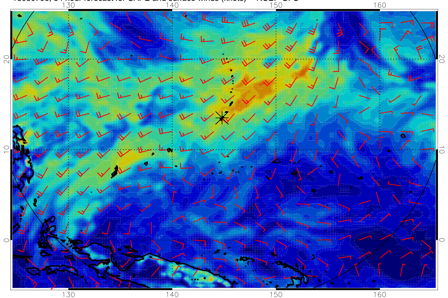
16080706, 54 hour forecast for CAPE and surface winds (knots) -- NCEP GFS
