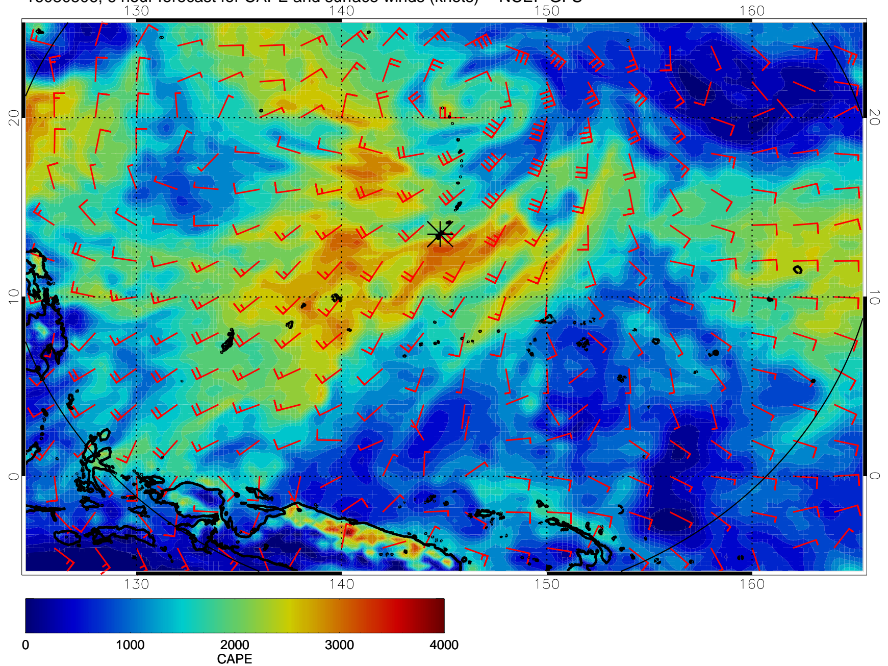
16080506, 6 hour forecast for CAPE and surface winds (knots) -- NCEP GFS
