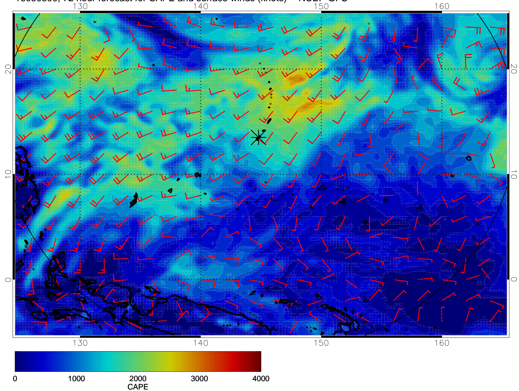
16080800, 72 hour forecast for CAPE and surface winds (knots) -- NCEP GFS
