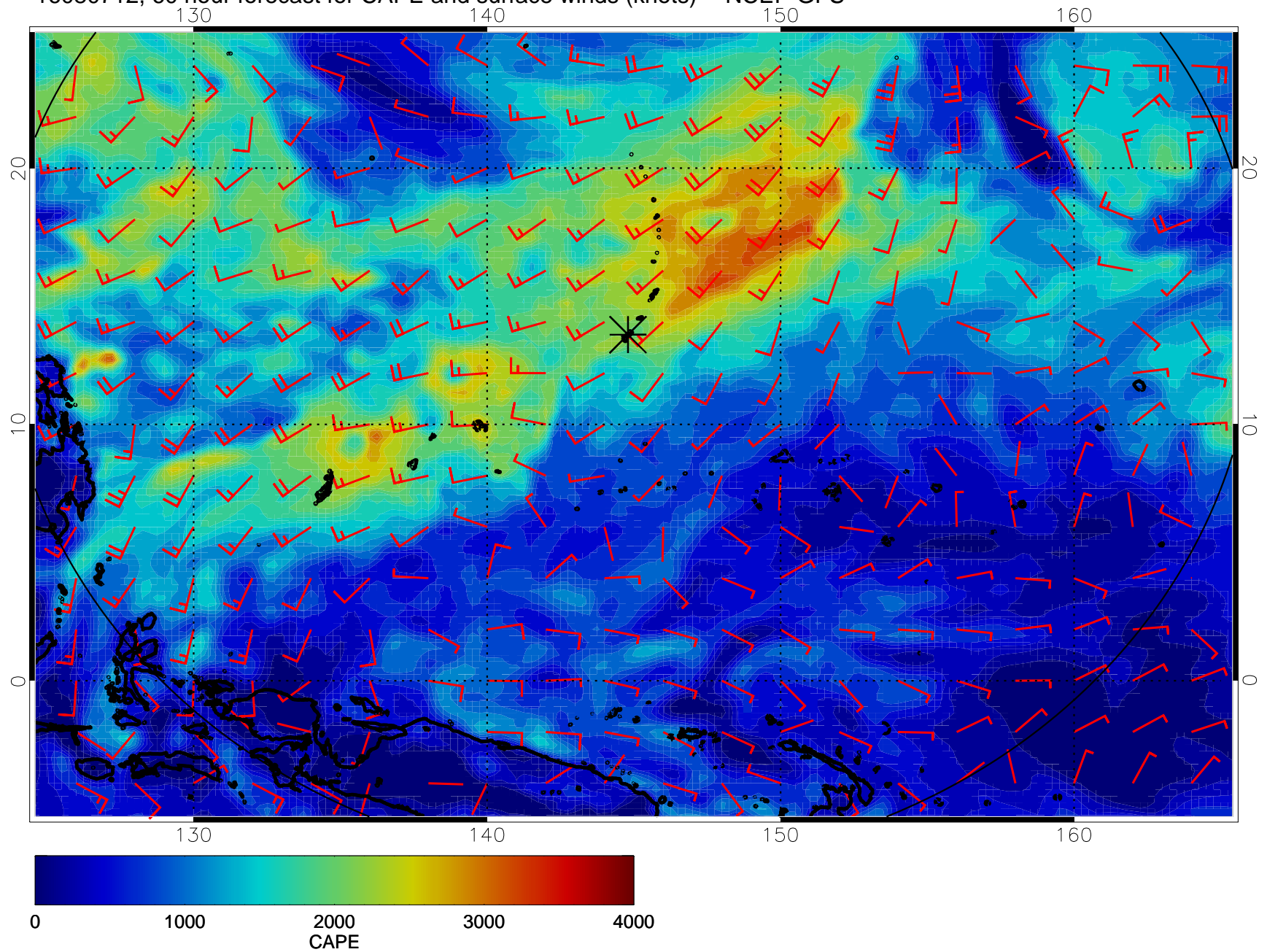
16080712, 60 hour forecast for CAPE and surface winds (knots) -- NCEP GFS
