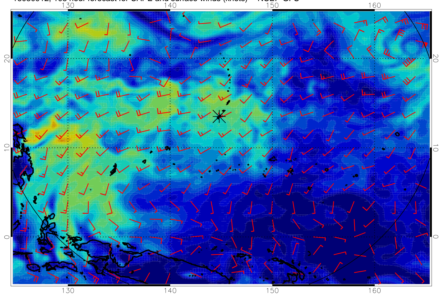
16080912, 108 hour forecast for CAPE and surface winds (knots) -- NCEP GFS
