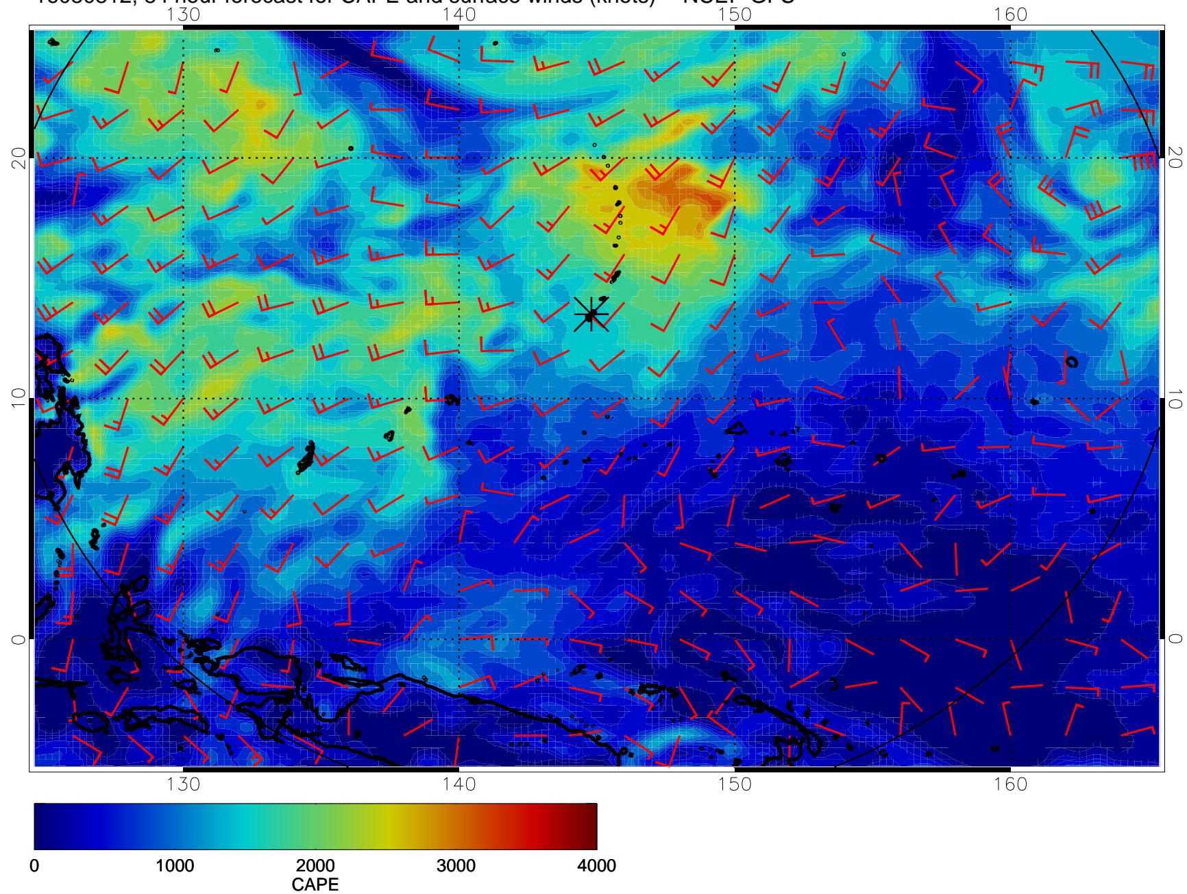
16080812, 84 hour forecast for CAPE and surface winds (knots) -- NCEP GFS
