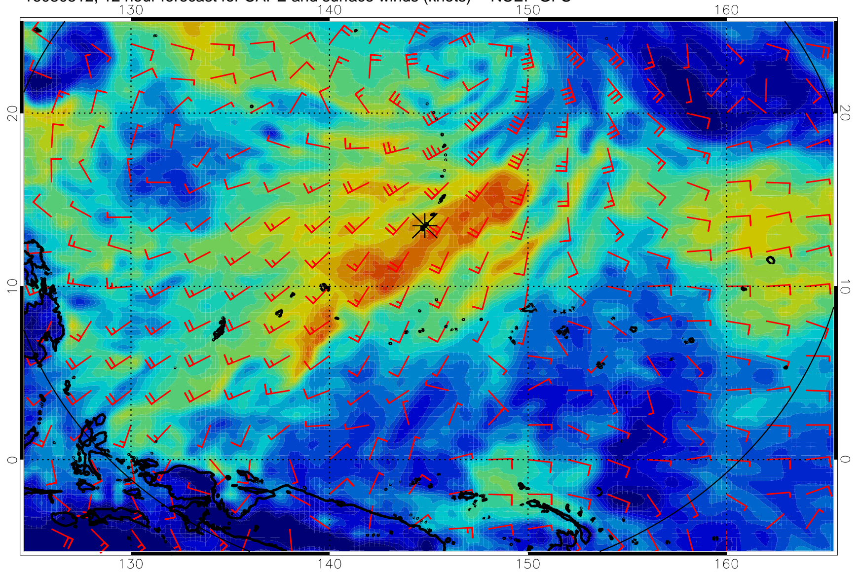
16080512, 12 hour forecast for CAPE and surface winds (knots) -- NCEP GFS
