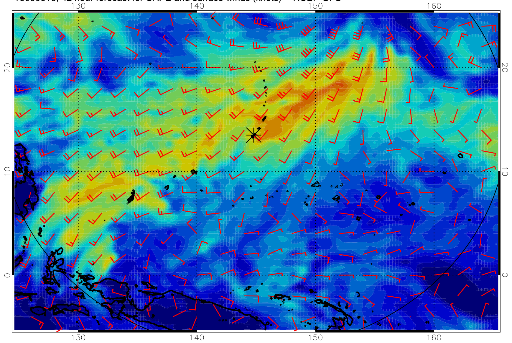
16080618, 42 hour forecast for CAPE and surface winds (knots) -- NCEP GFS
