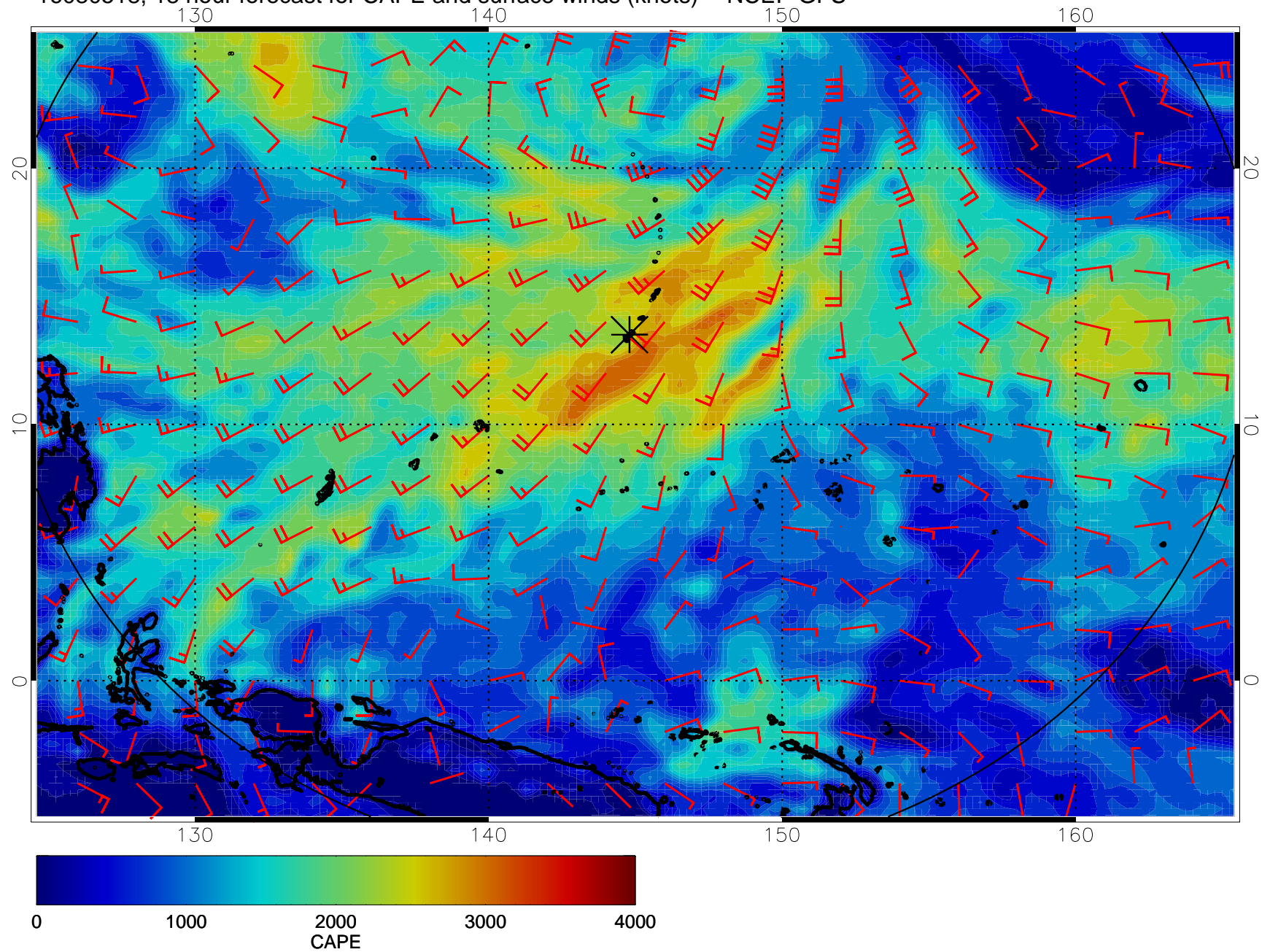
16080518, 18 hour forecast for CAPE and surface winds (knots) -- NCEP GFS
