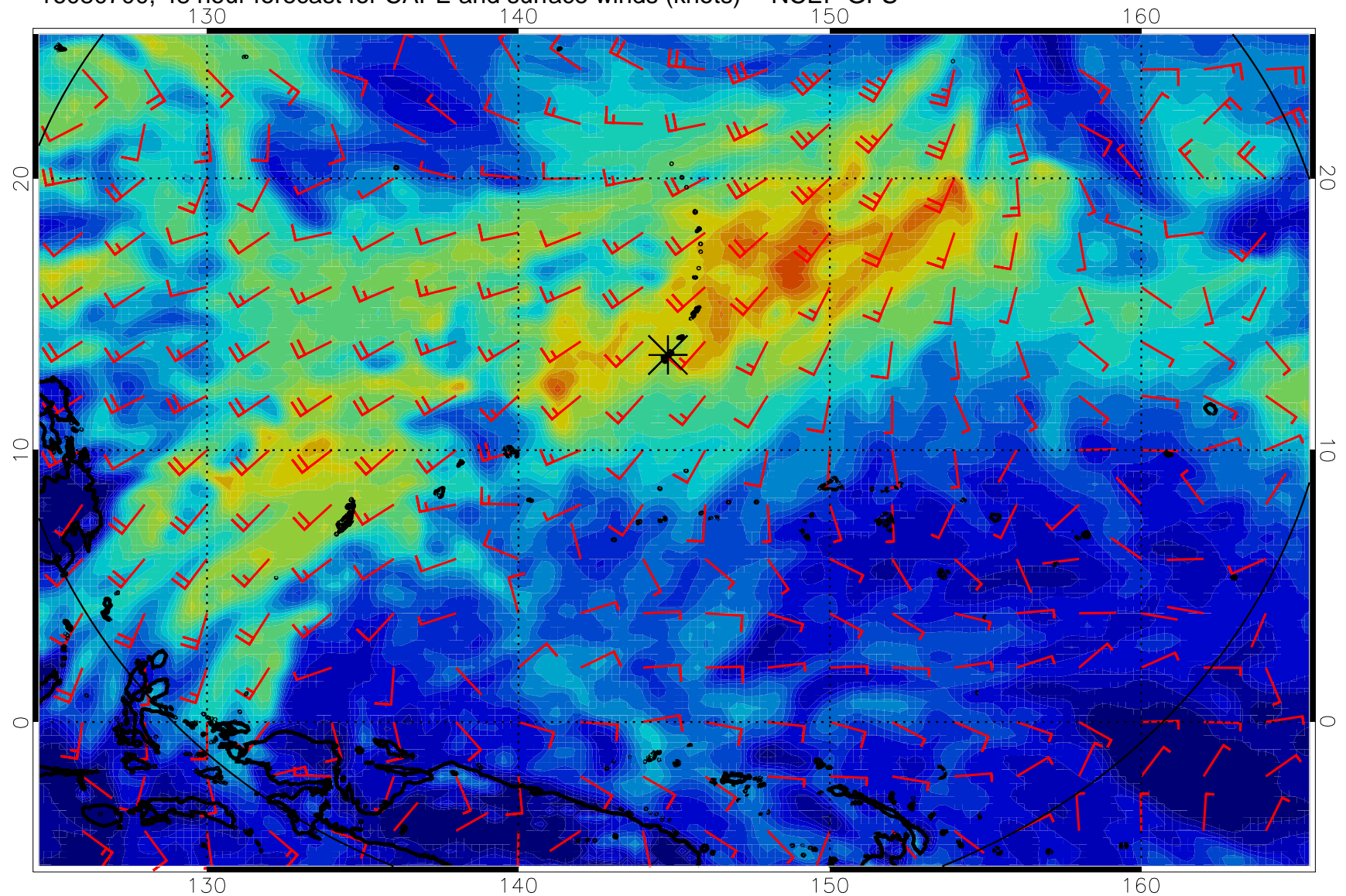
16080700, 48 hour forecast for CAPE and surface winds (knots) -- NCEP GFS
