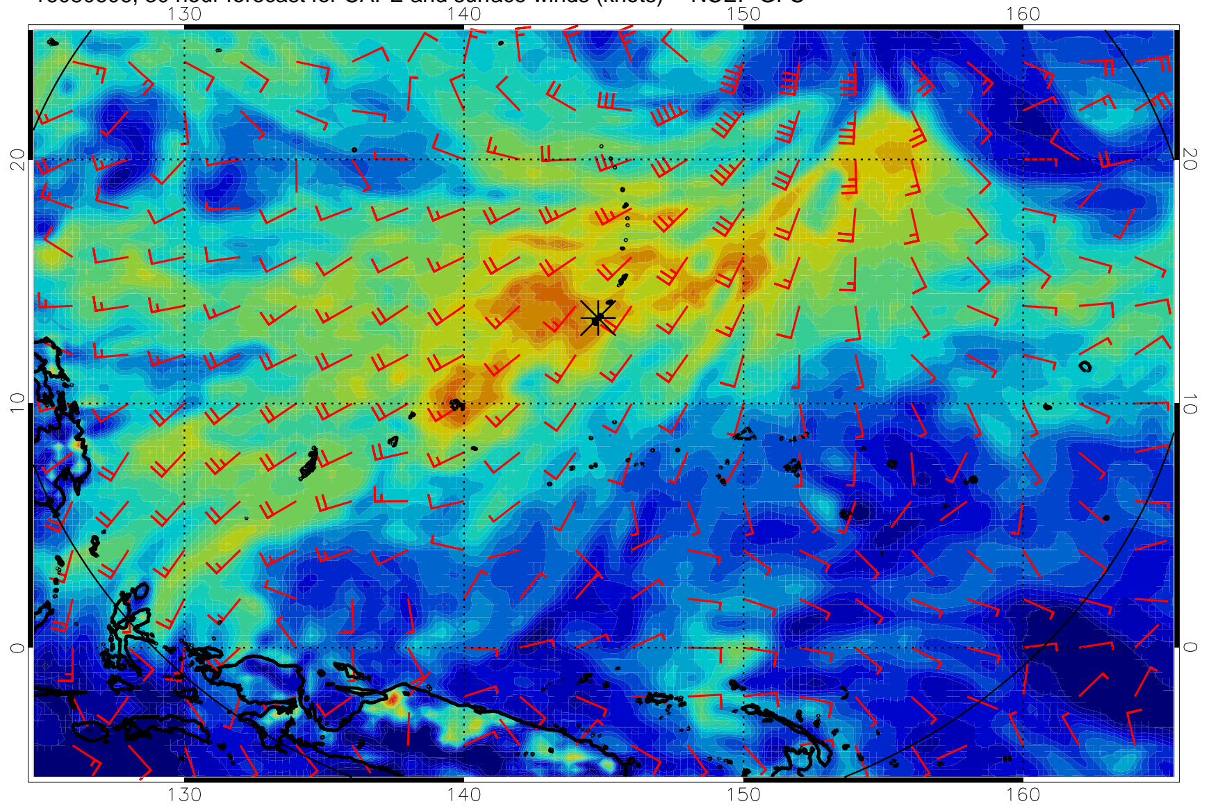
16080606, 30 hour forecast for CAPE and surface winds (knots) -- NCEP GFS
