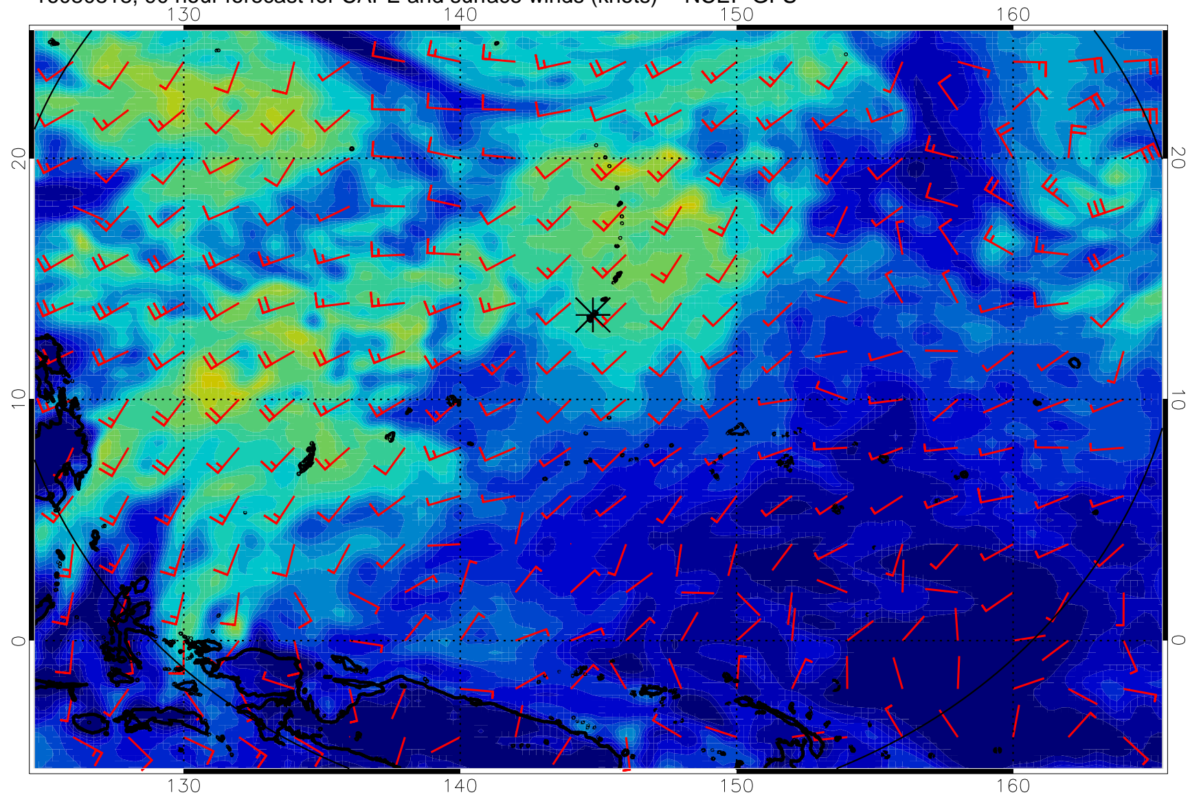
16080818, 90 hour forecast for CAPE and surface winds (knots) -- NCEP GFS
