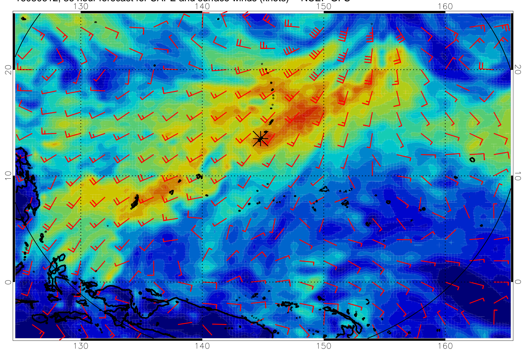
16080612, 36 hour forecast for CAPE and surface winds (knots) -- NCEP GFS
