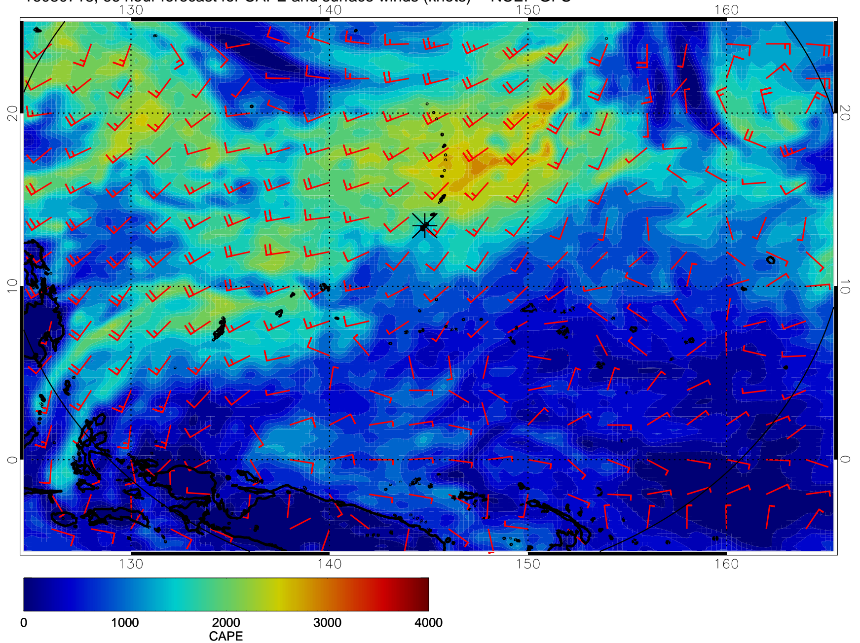
16080718, 66 hour forecast for CAPE and surface winds (knots) -- NCEP GFS
