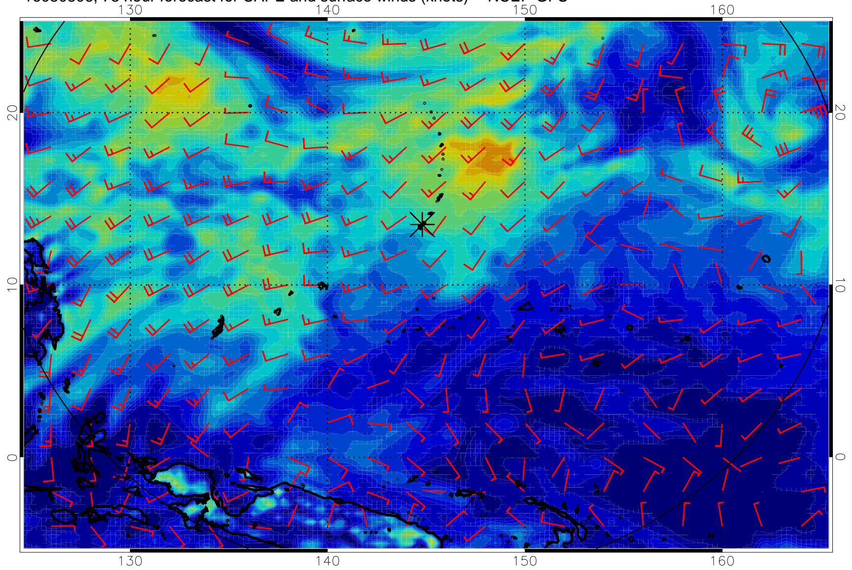
16080806, 78 hour forecast for CAPE and surface winds (knots) -- NCEP GFS
