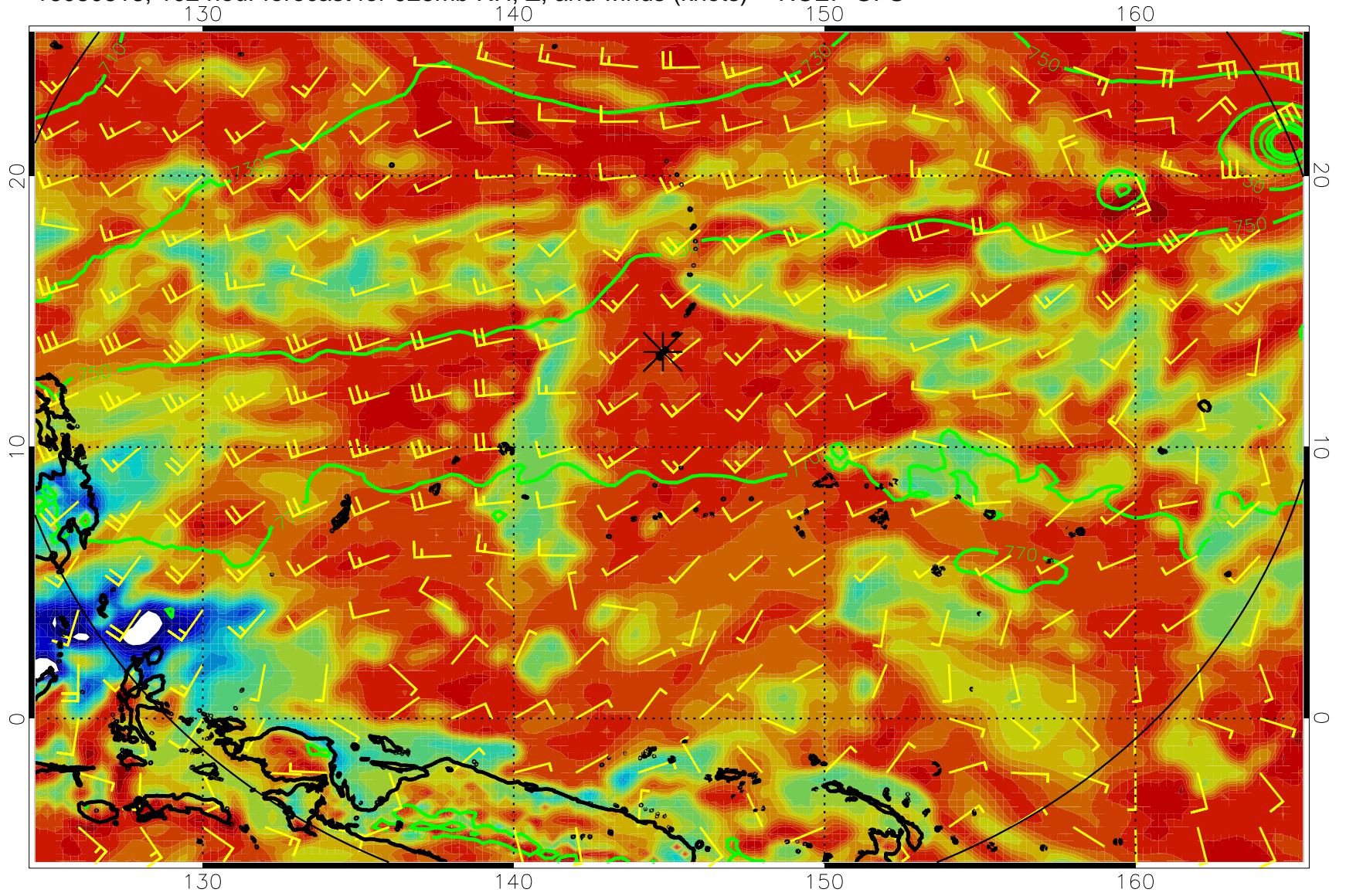
16080818, 102 hour forecast for 925mb RH, Z, and winds (knots) -- NCEP GFS
