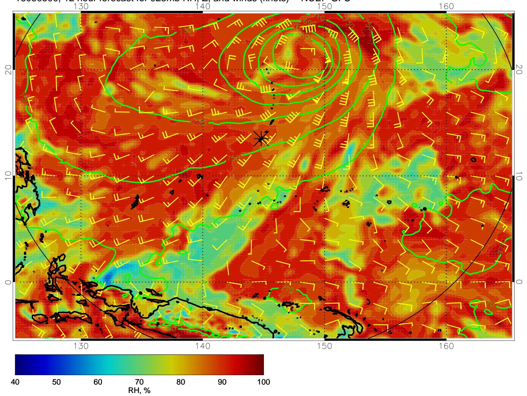
16080500, 12 hour forecast for 925mb RH, Z, and winds (knots) -- NCEP GFS
