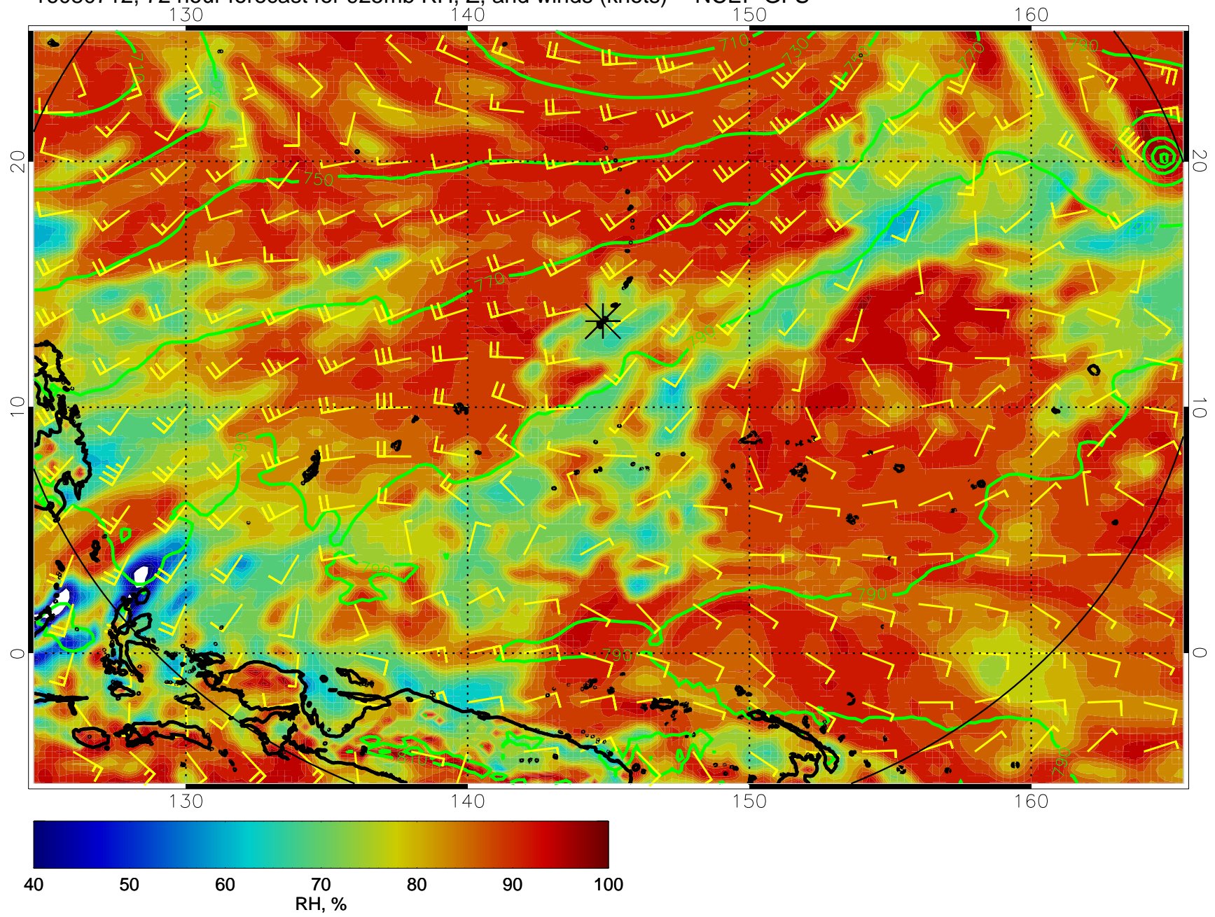
16080712, 72 hour forecast for 925mb RH, Z, and winds (knots) -- NCEP GFS
