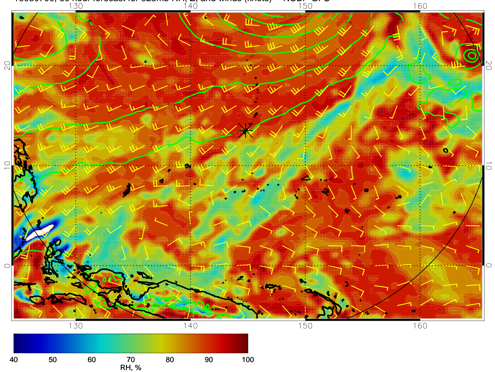
16080700, 60 hour forecast for 925mb RH, Z, and winds (knots) -- NCEP GFS
