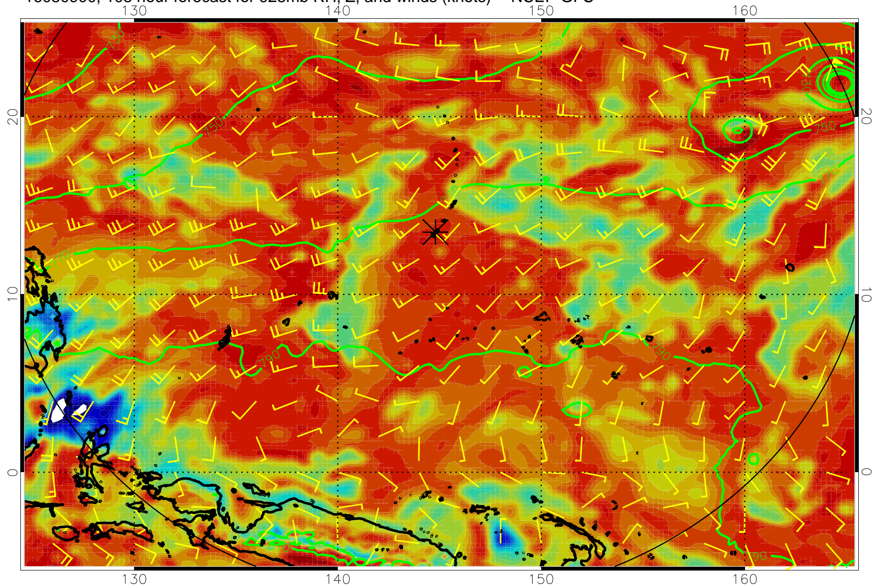
16080900, 108 hour forecast for 925mb RH, Z, and winds (knots) -- NCEP GFS
