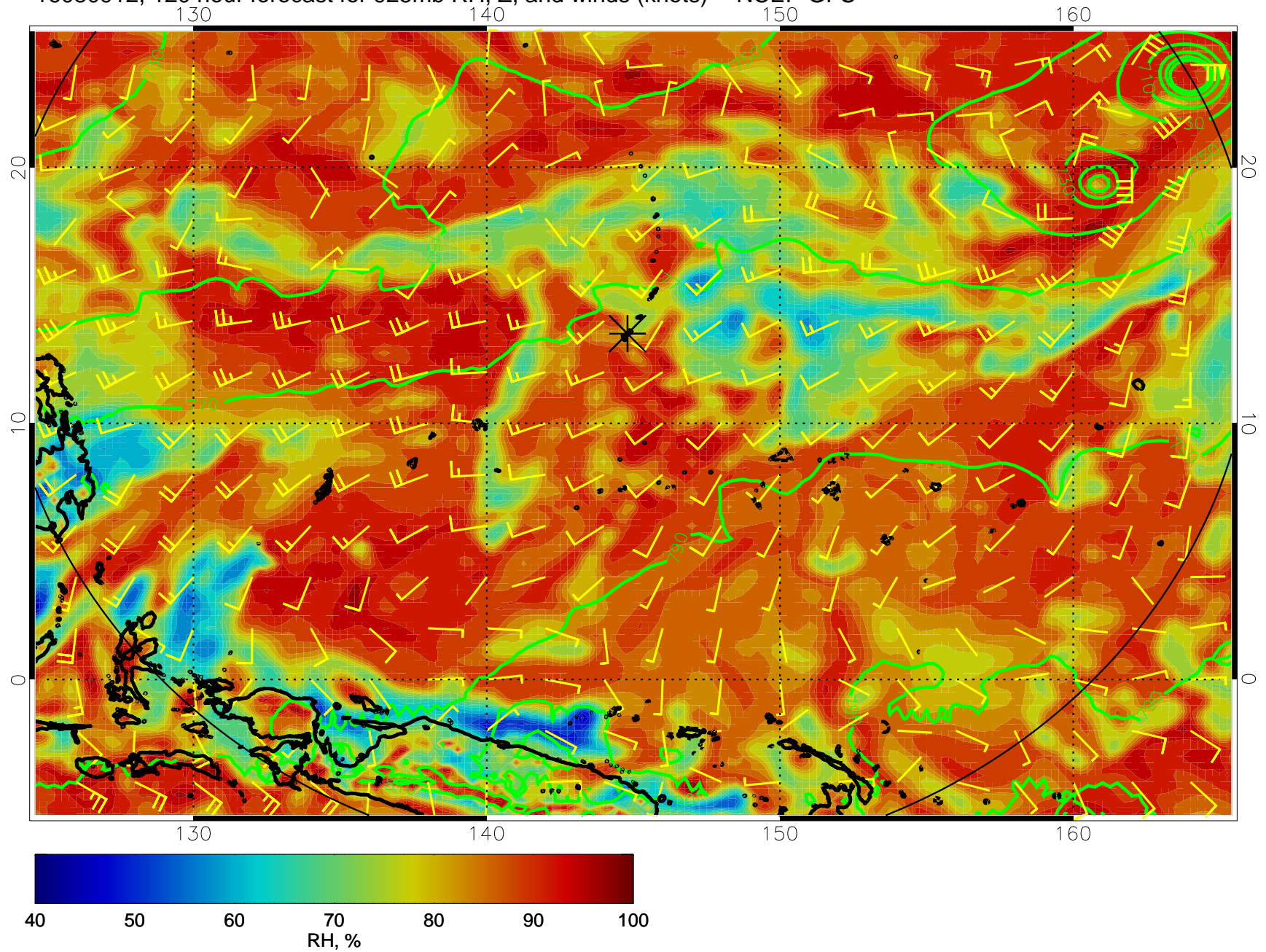
16080912, 120 hour forecast for 925mb RH, Z, and winds (knots) -- NCEP GFS
