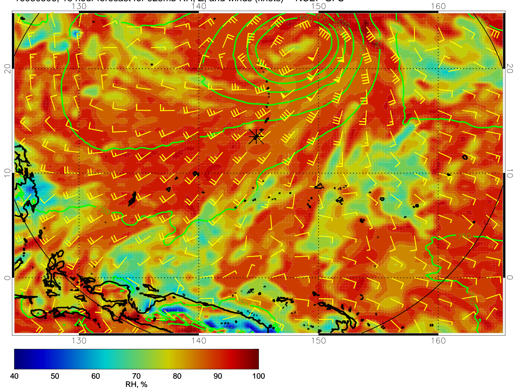
16080506, 18 hour forecast for 925mb RH, Z, and winds (knots) -- NCEP GFS
