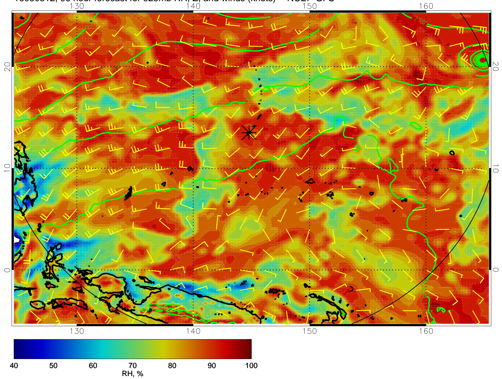
16080812, 96 hour forecast for 925mb RH, Z, and winds (knots) -- NCEP GFS
