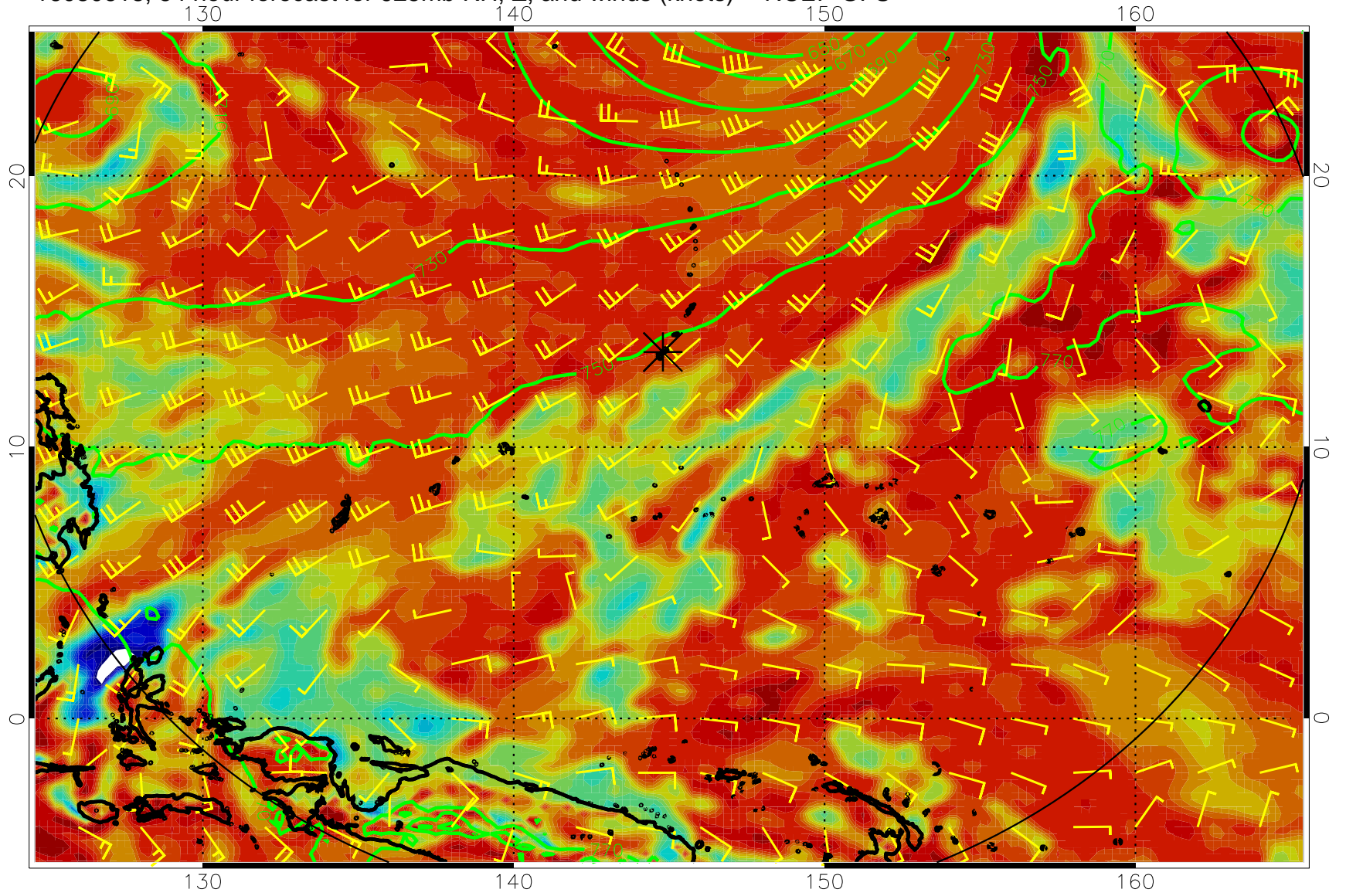
16080618, 54 hour forecast for 925mb RH, Z, and winds (knots) -- NCEP GFS
