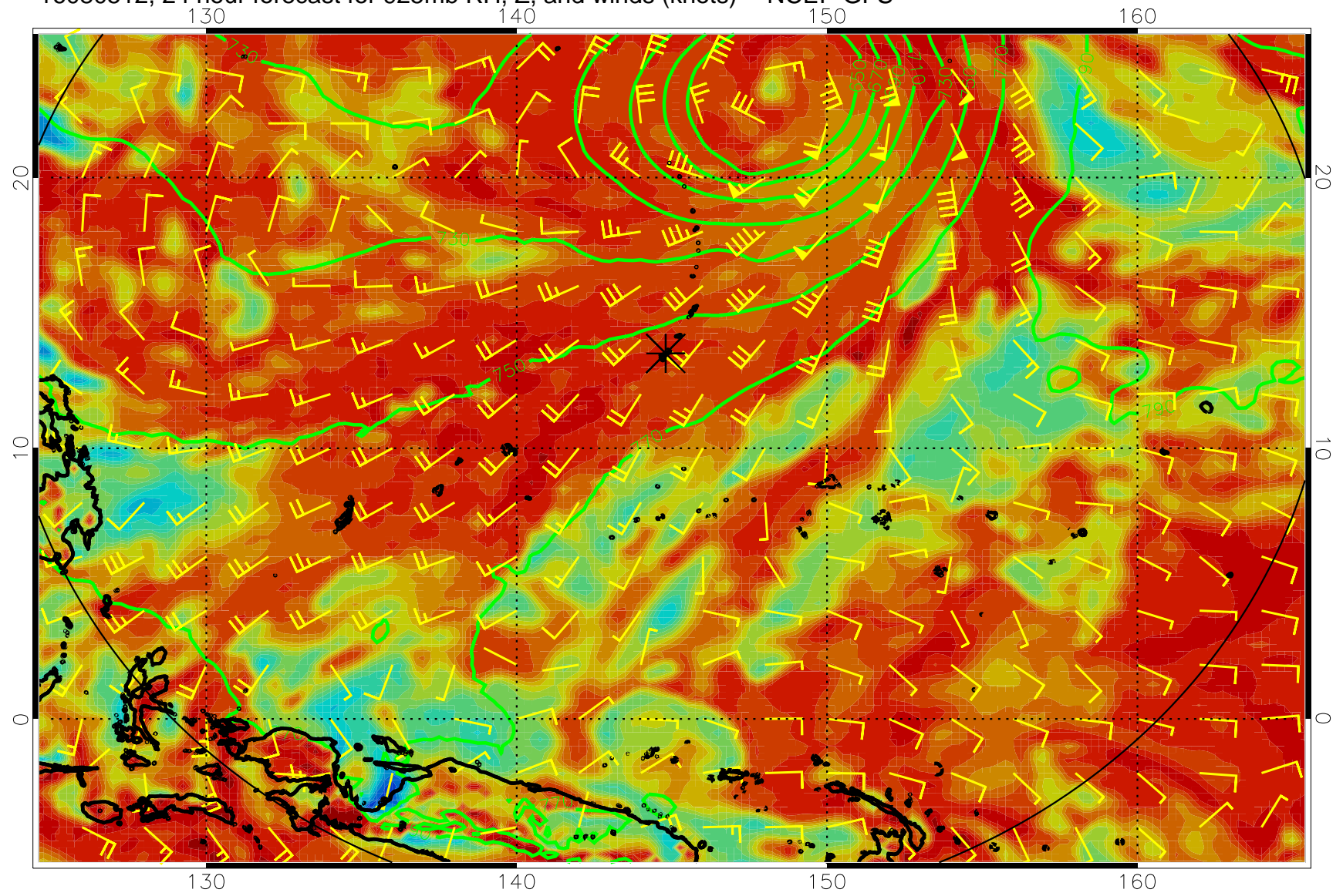
16080512, 24 hour forecast for 925mb RH, Z, and winds (knots) -- NCEP GFS
