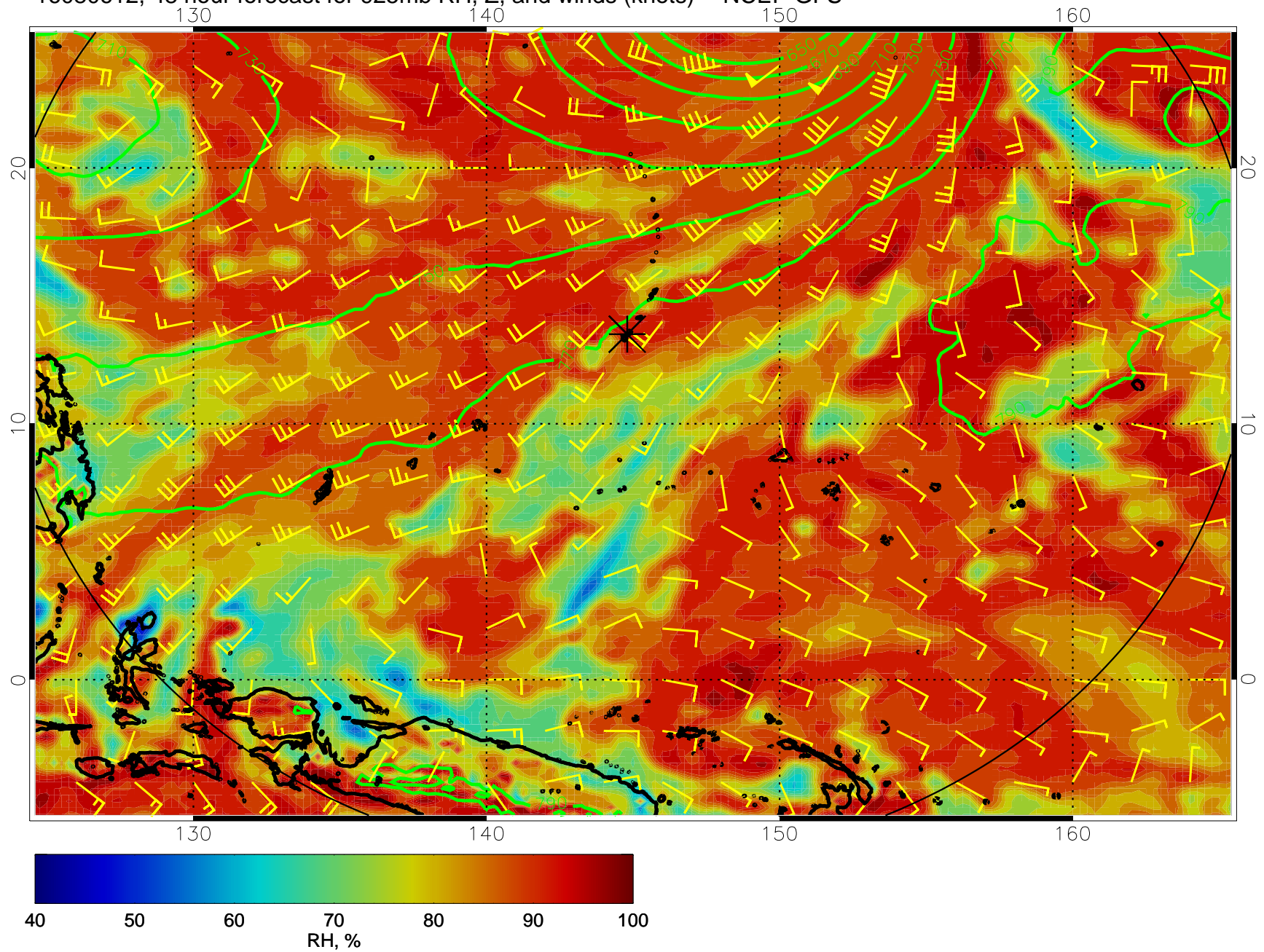
16080612, 48 hour forecast for 925mb RH, Z, and winds (knots) -- NCEP GFS
