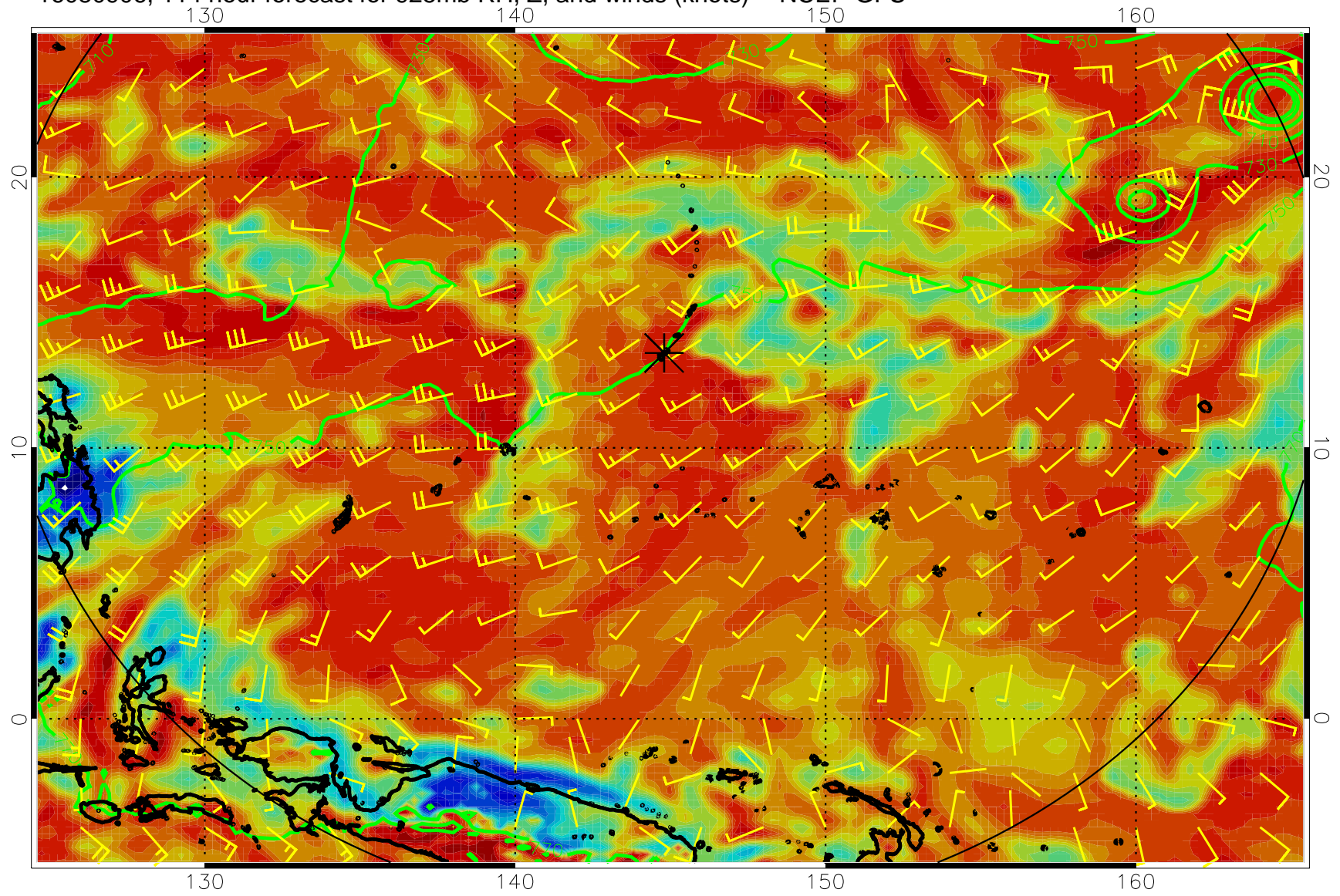
16080906, 114 hour forecast for 925mb RH, Z, and winds (knots) -- NCEP GFS
