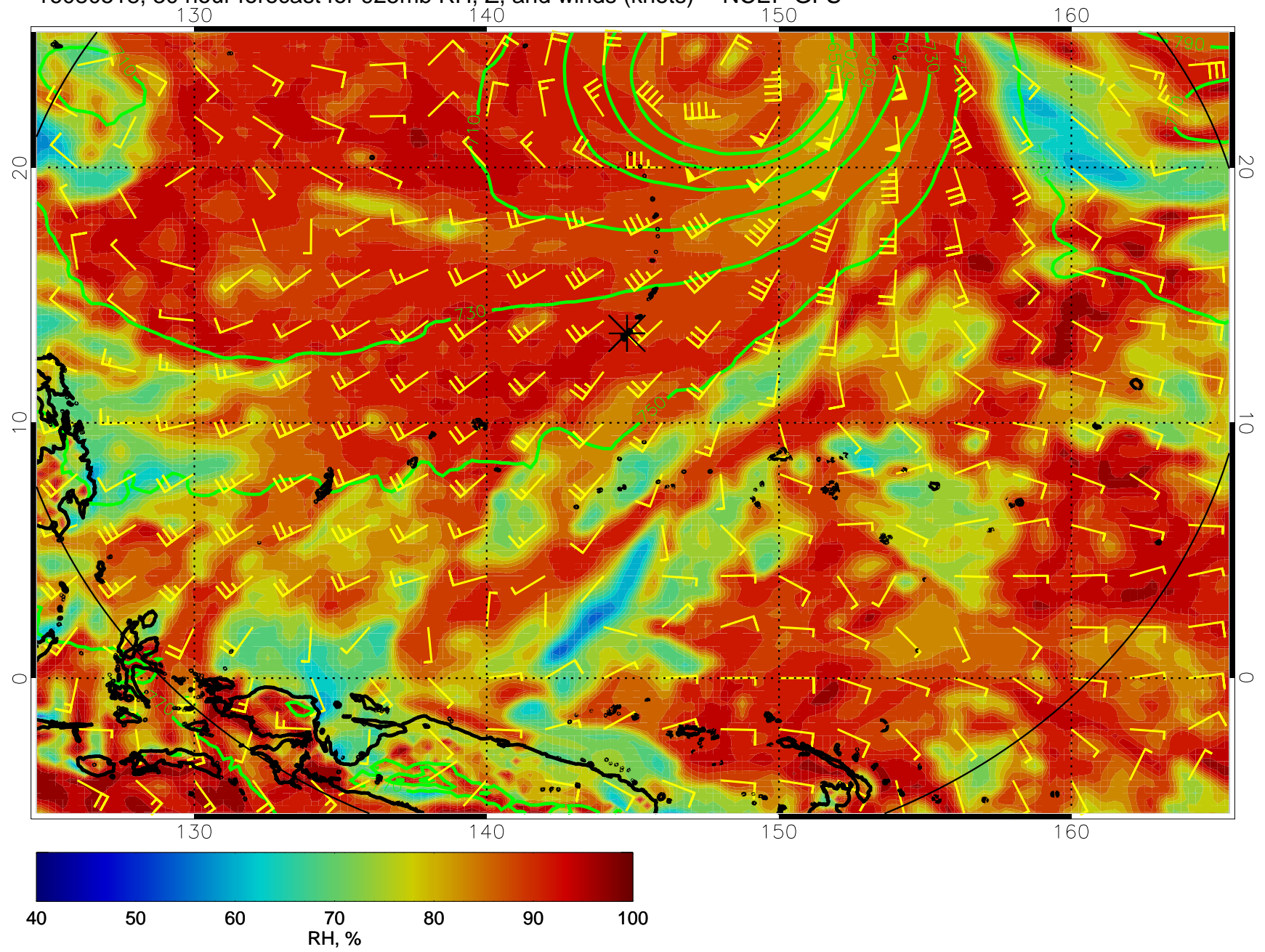
16080518, 30 hour forecast for 925mb RH, Z, and winds (knots) -- NCEP GFS
