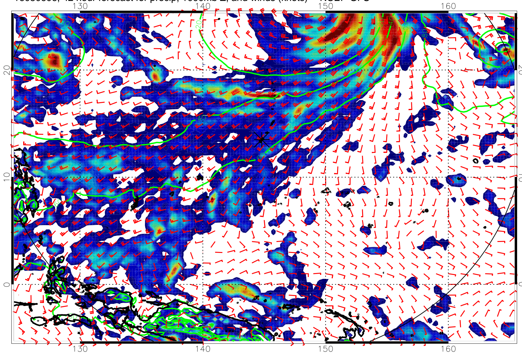
16080606, 42 hour forecast for precip, 1000mb Z, and winds (knots) -- NCEP GFS
