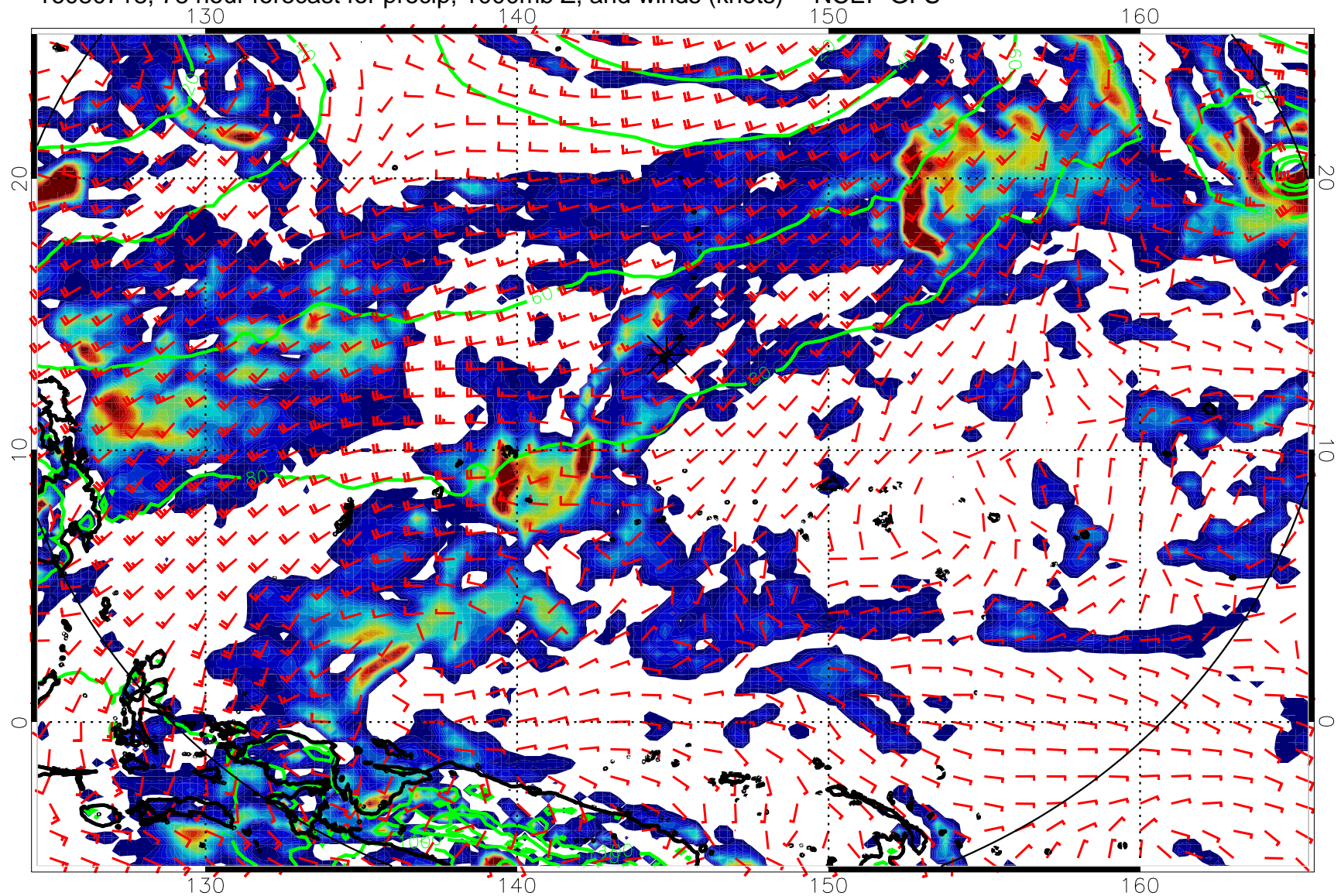
16080718, 78 hour forecast for precip, 1000mb Z, and winds (knots) -- NCEP GFS
