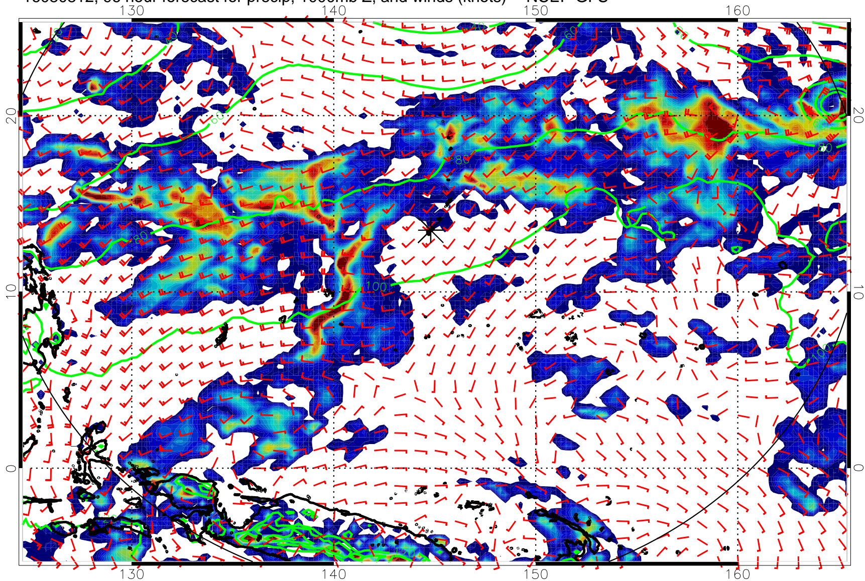
16080812, 96 hour forecast for precip, 1000mb Z, and winds (knots) -- NCEP GFS
