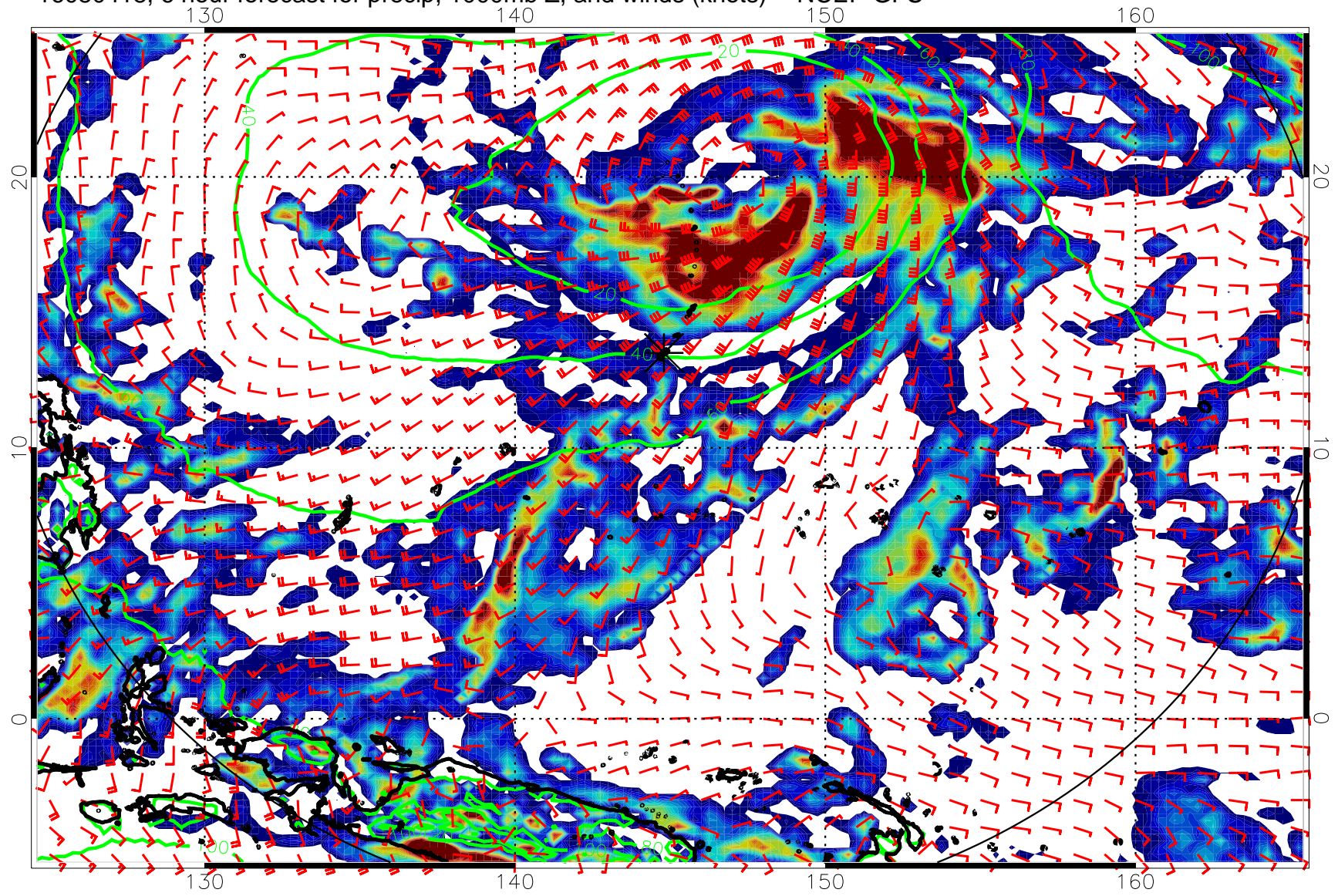
16080418, 6 hour forecast for precip, 1000mb Z, and winds (knots) -- NCEP GFS
