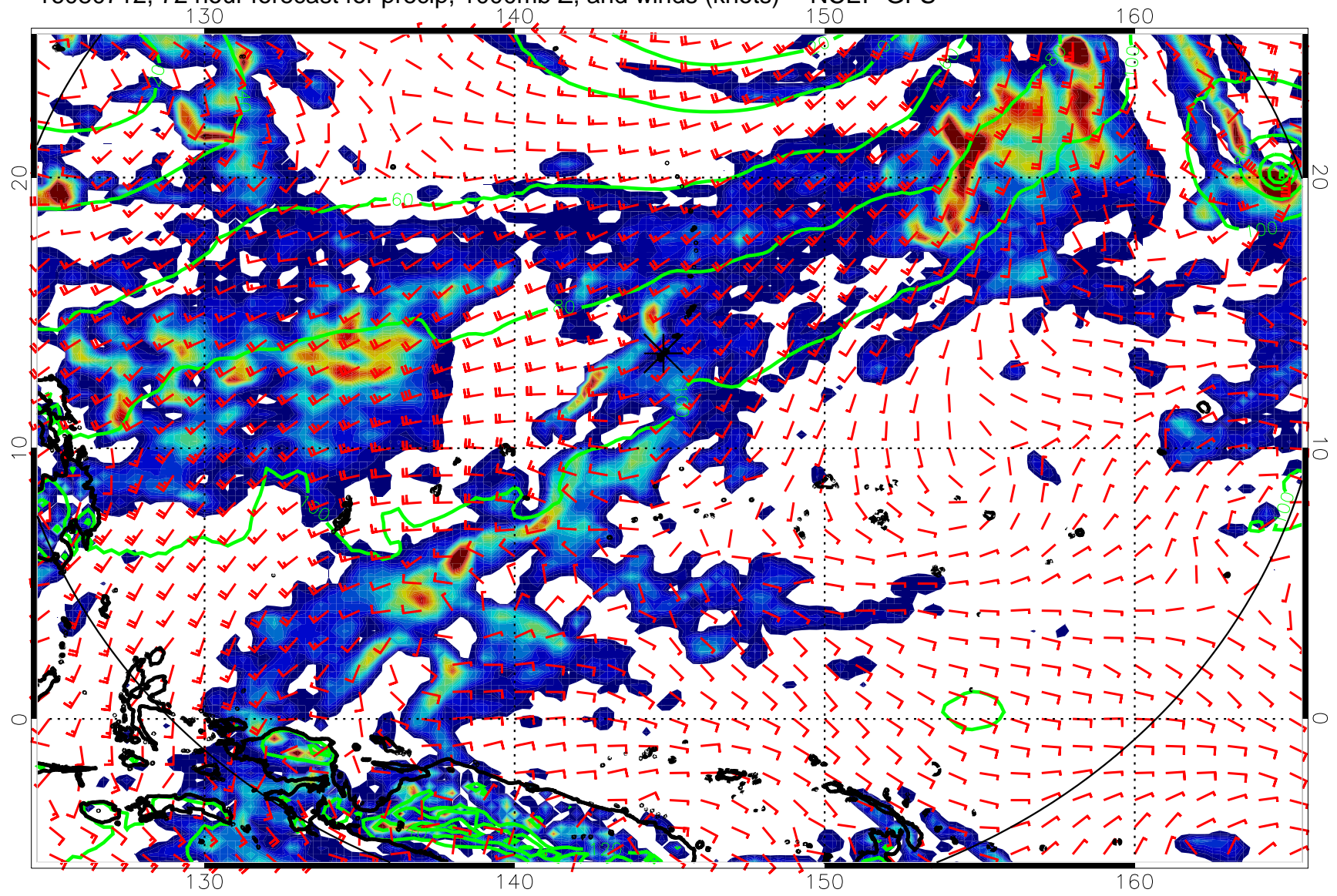
16080712, 72 hour forecast for precip, 1000mb Z, and winds (knots) -- NCEP GFS
