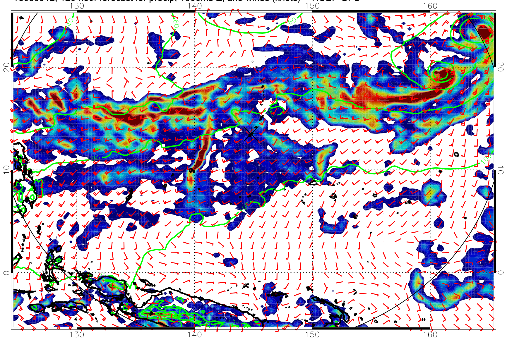
16080912, 120 hour forecast for precip, 1000mb Z, and winds (knots) -- NCEP GFS
