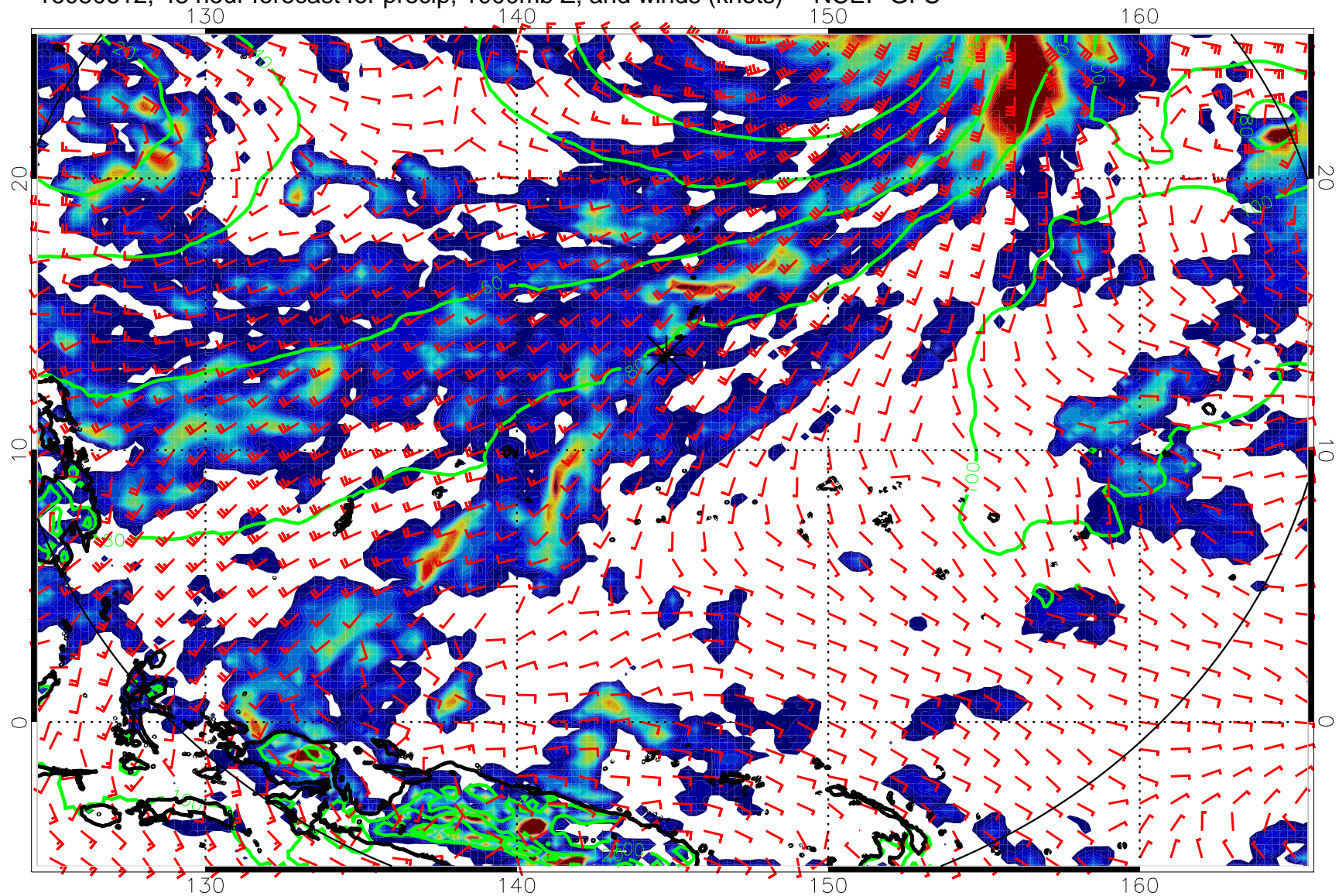
16080612, 48 hour forecast for precip, 1000mb Z, and winds (knots) -- NCEP GFS
