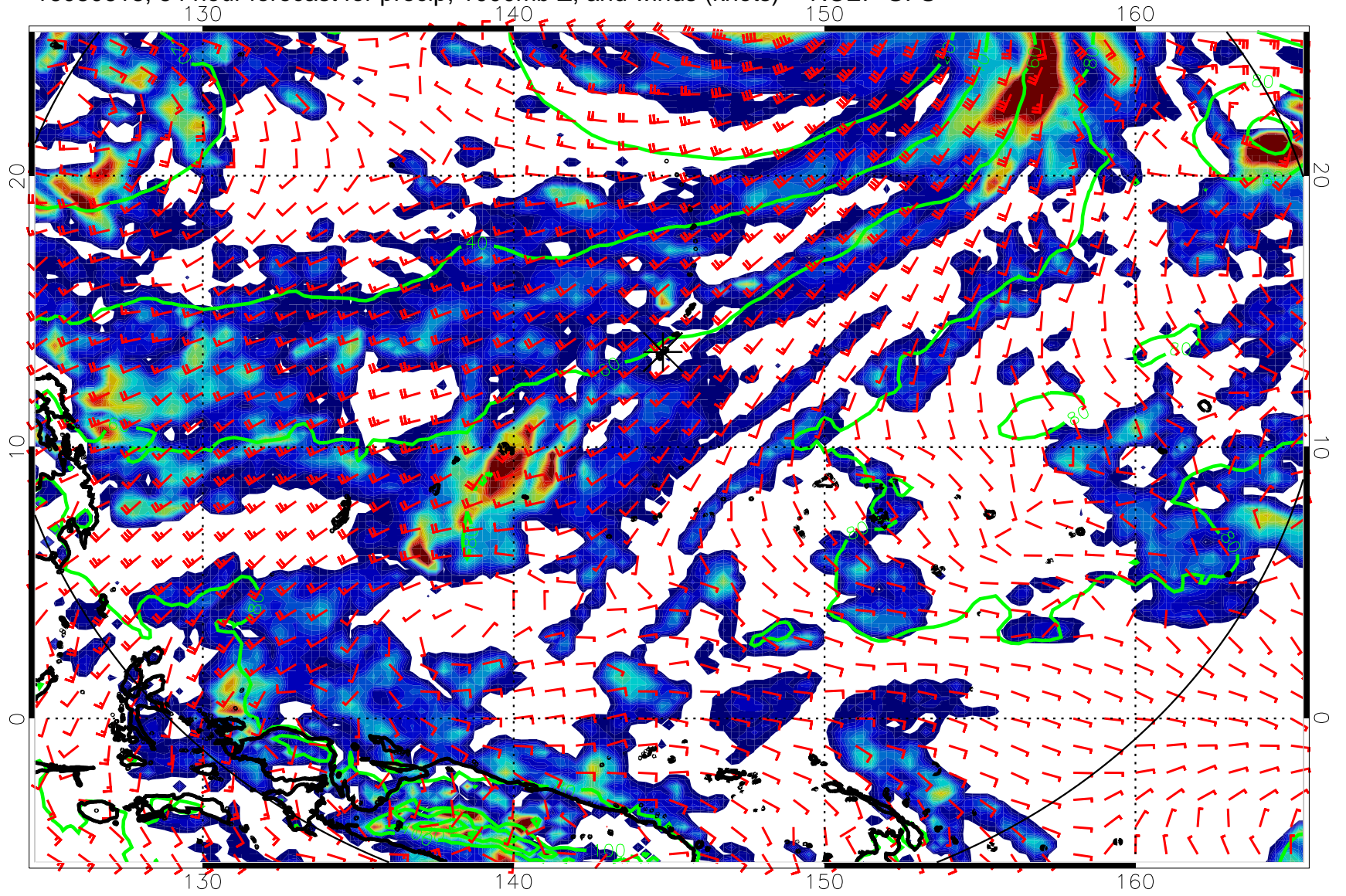
16080618, 54 hour forecast for precip, 1000mb Z, and winds (knots) -- NCEP GFS
