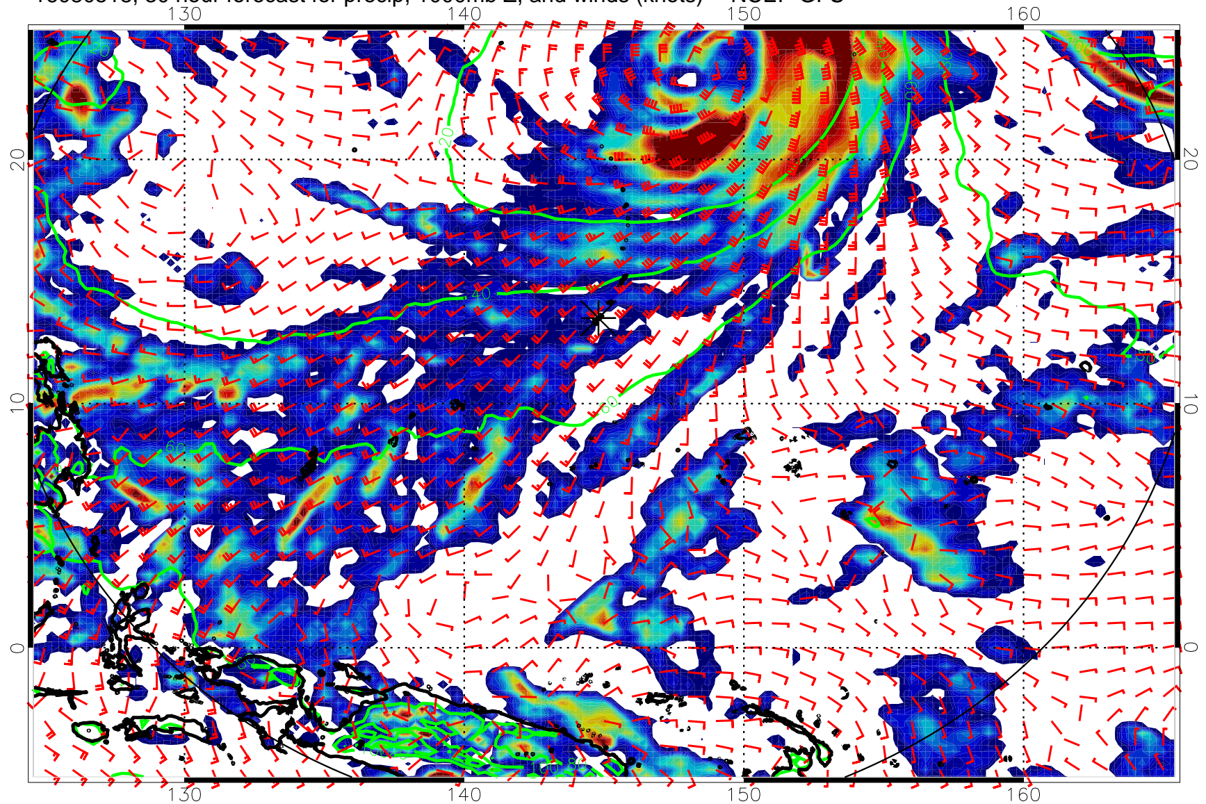
16080518, 30 hour forecast for precip, 1000mb Z, and winds (knots) -- NCEP GFS
