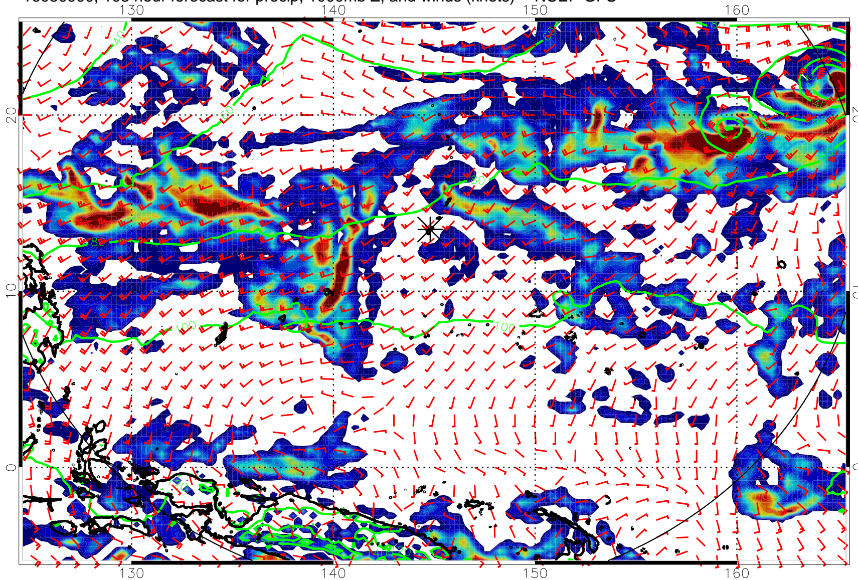
16080900, 108 hour forecast for precip, 1000mb Z, and winds (knots) -- NCEP GFS
