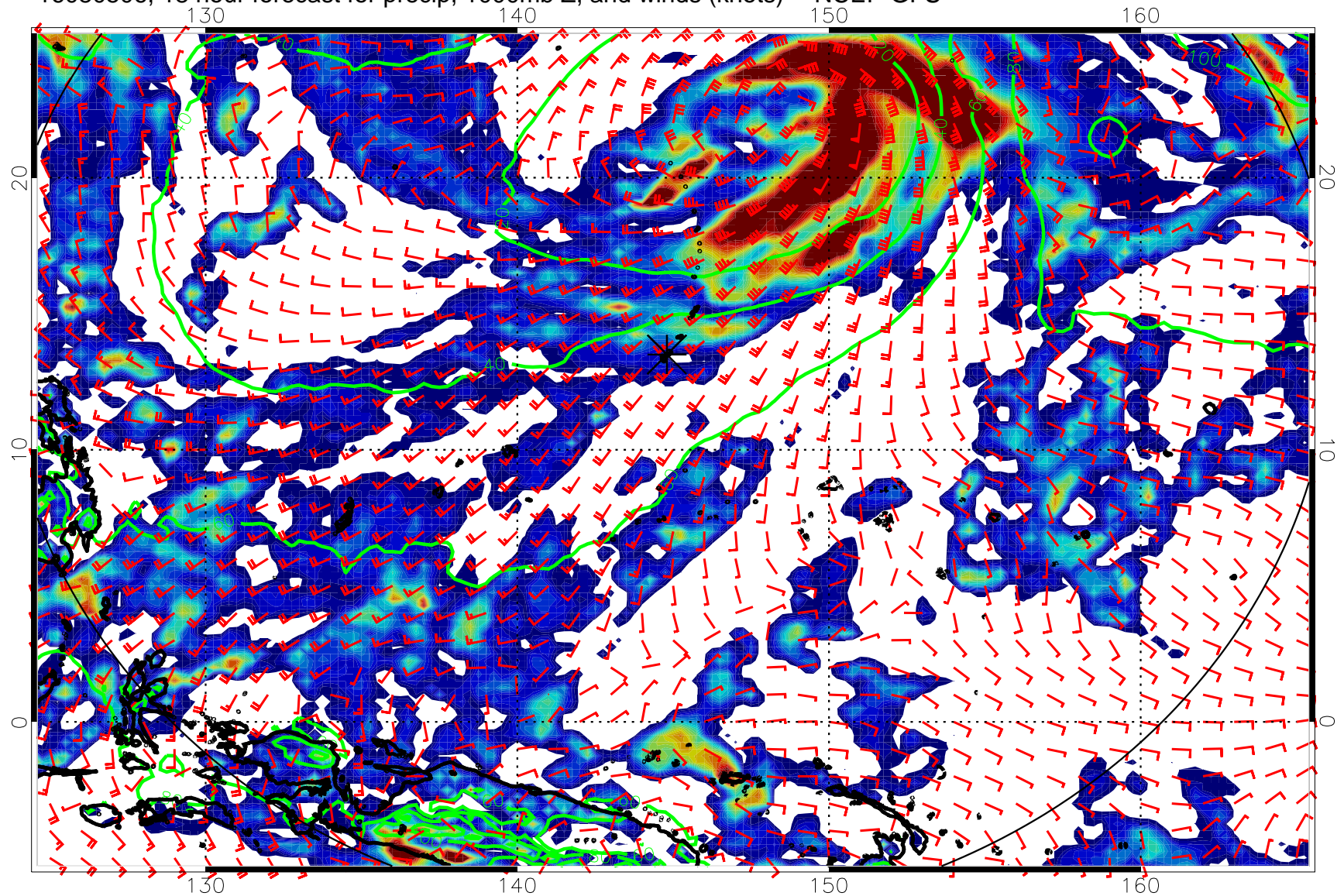
16080506, 18 hour forecast for precip, 1000mb Z, and winds (knots) -- NCEP GFS
