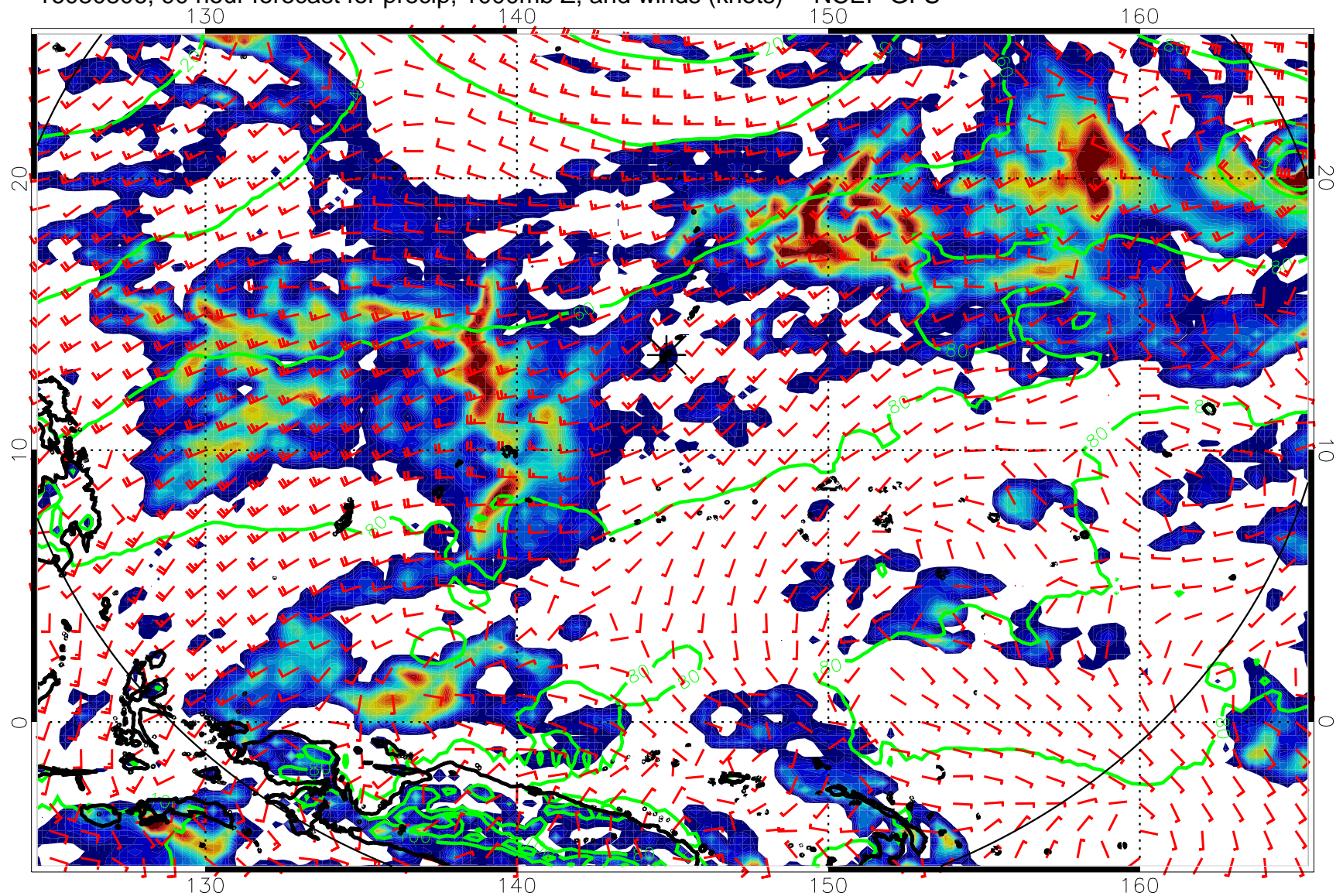
16080806, 90 hour forecast for precip, 1000mb Z, and winds (knots) -- NCEP GFS
