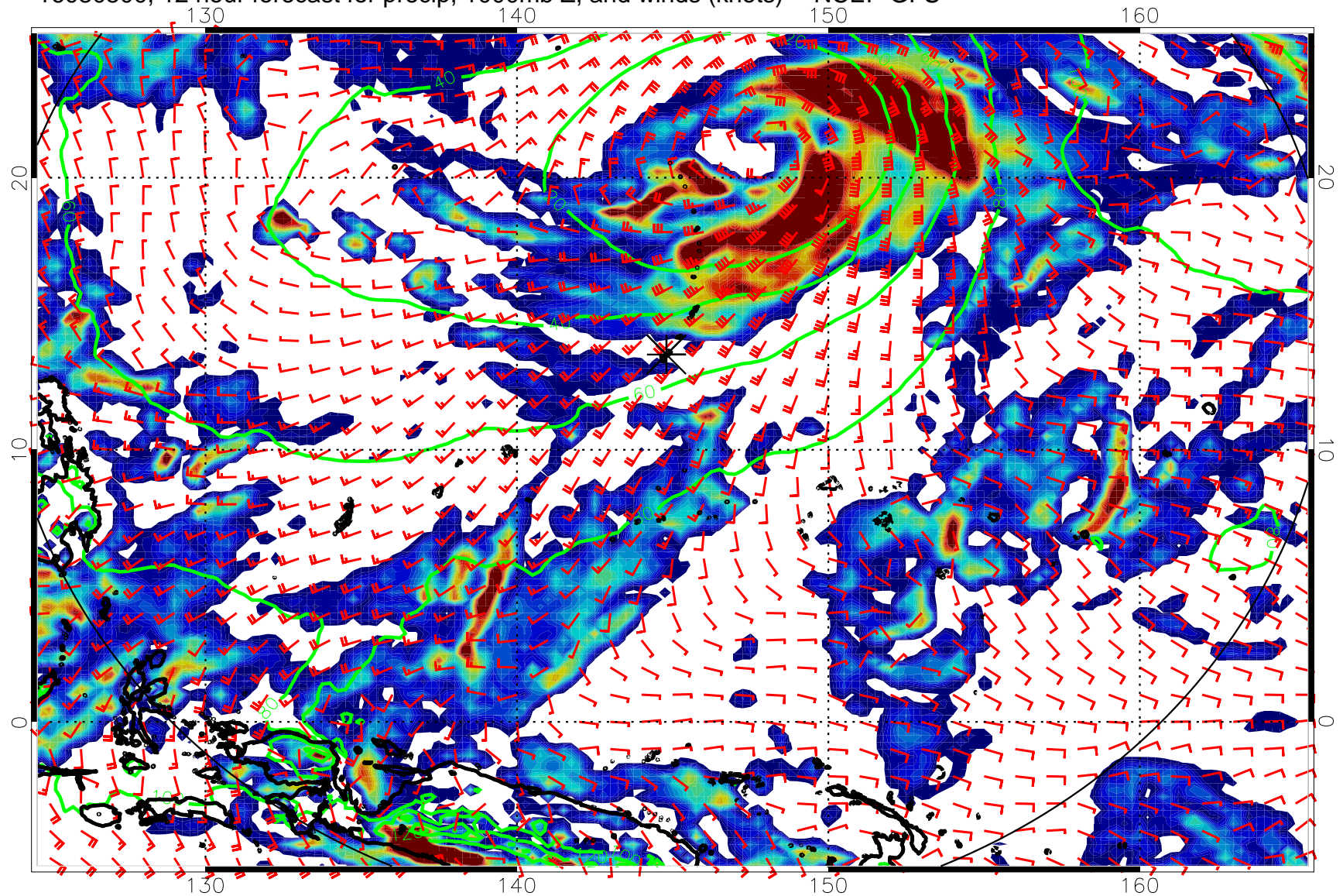
16080500, 12 hour forecast for precip, 1000mb Z, and winds (knots) -- NCEP GFS
