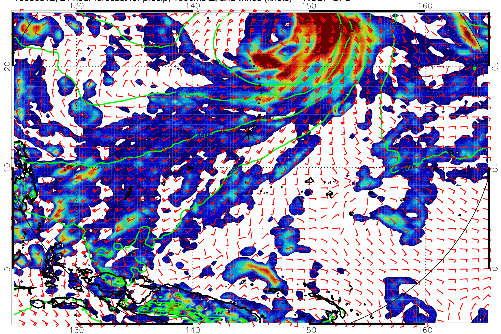
16080512, 24 hour forecast for precip, 1000mb Z, and winds (knots) -- NCEP GFS
