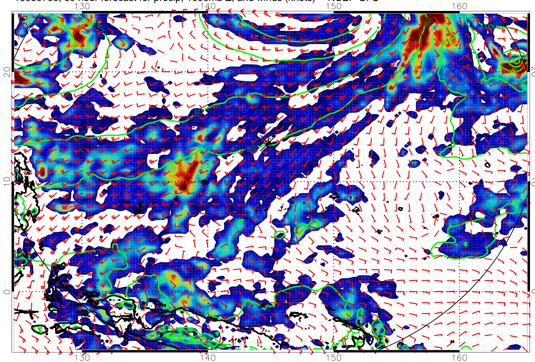
16080700, 60 hour forecast for precip, 1000mb Z, and winds (knots) -- NCEP GFS
