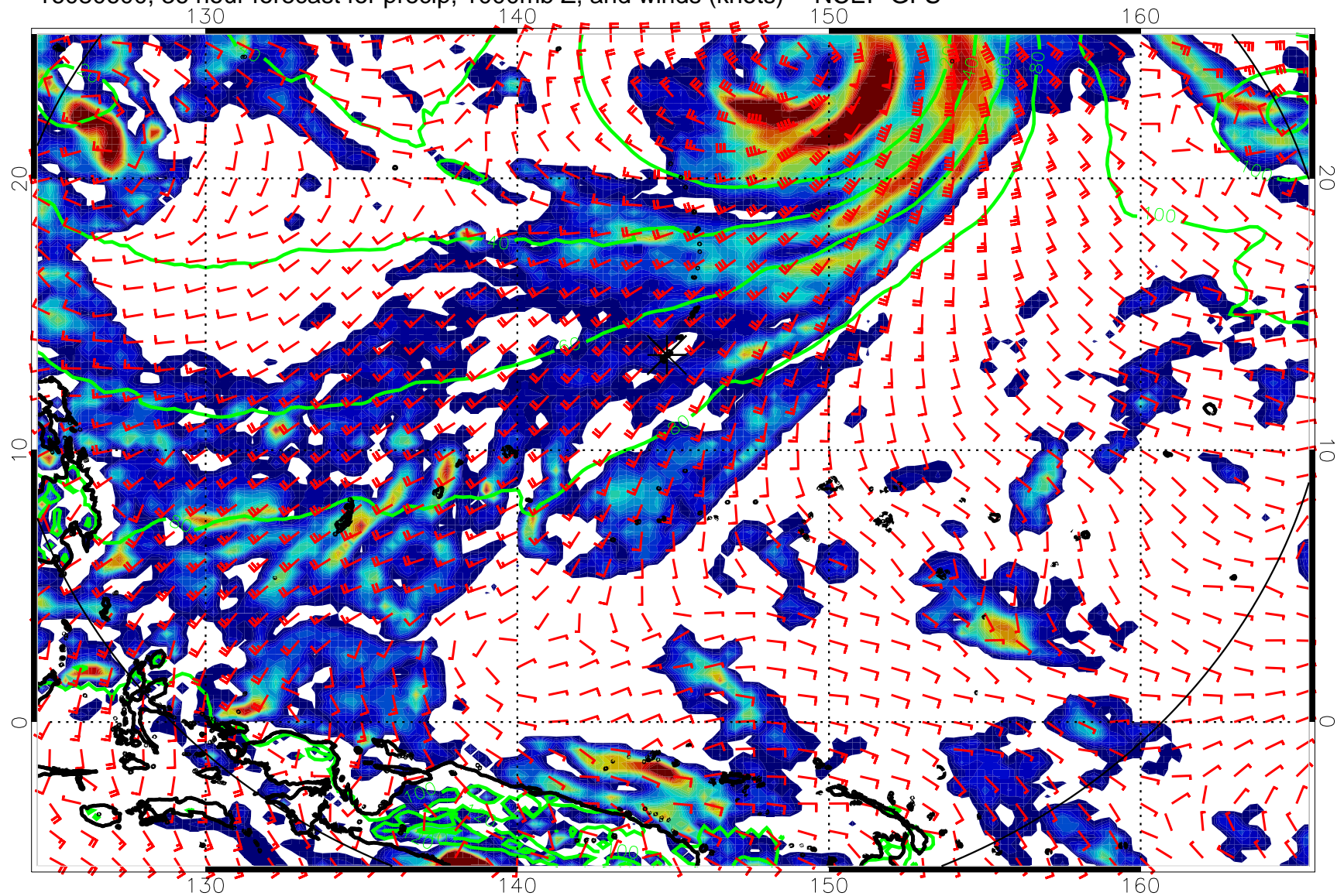
16080600, 36 hour forecast for precip, 1000mb Z, and winds (knots) -- NCEP GFS
