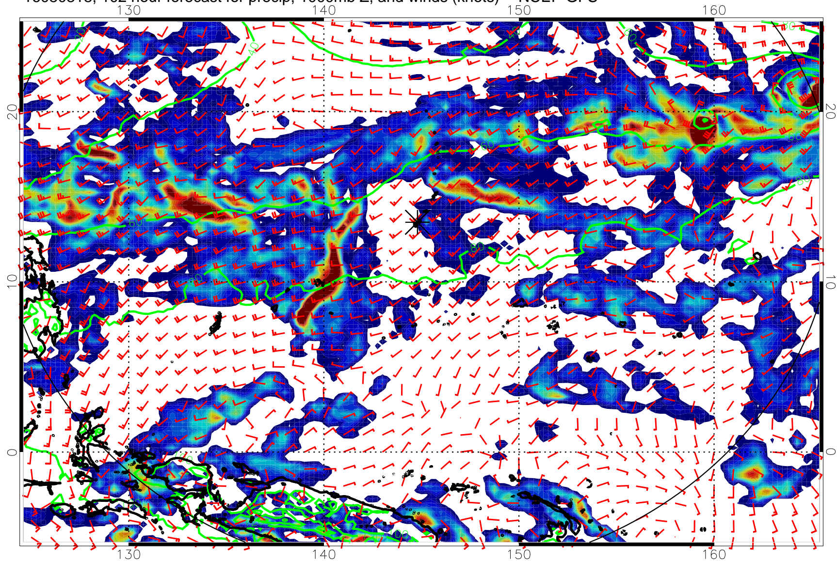
16080818, 102 hour forecast for precip, 1000mb Z, and winds (knots) -- NCEP GFS
