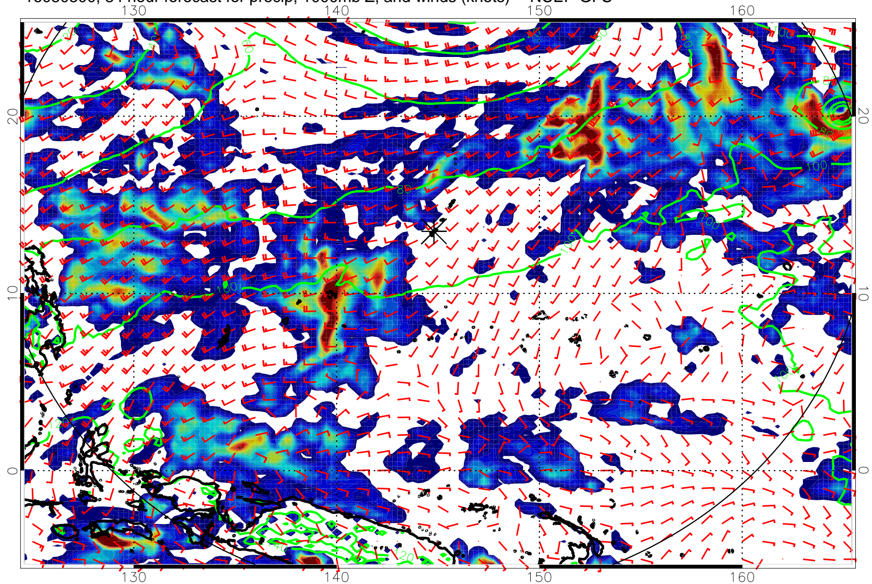
16080800, 84 hour forecast for precip, 1000mb Z, and winds (knots) -- NCEP GFS
