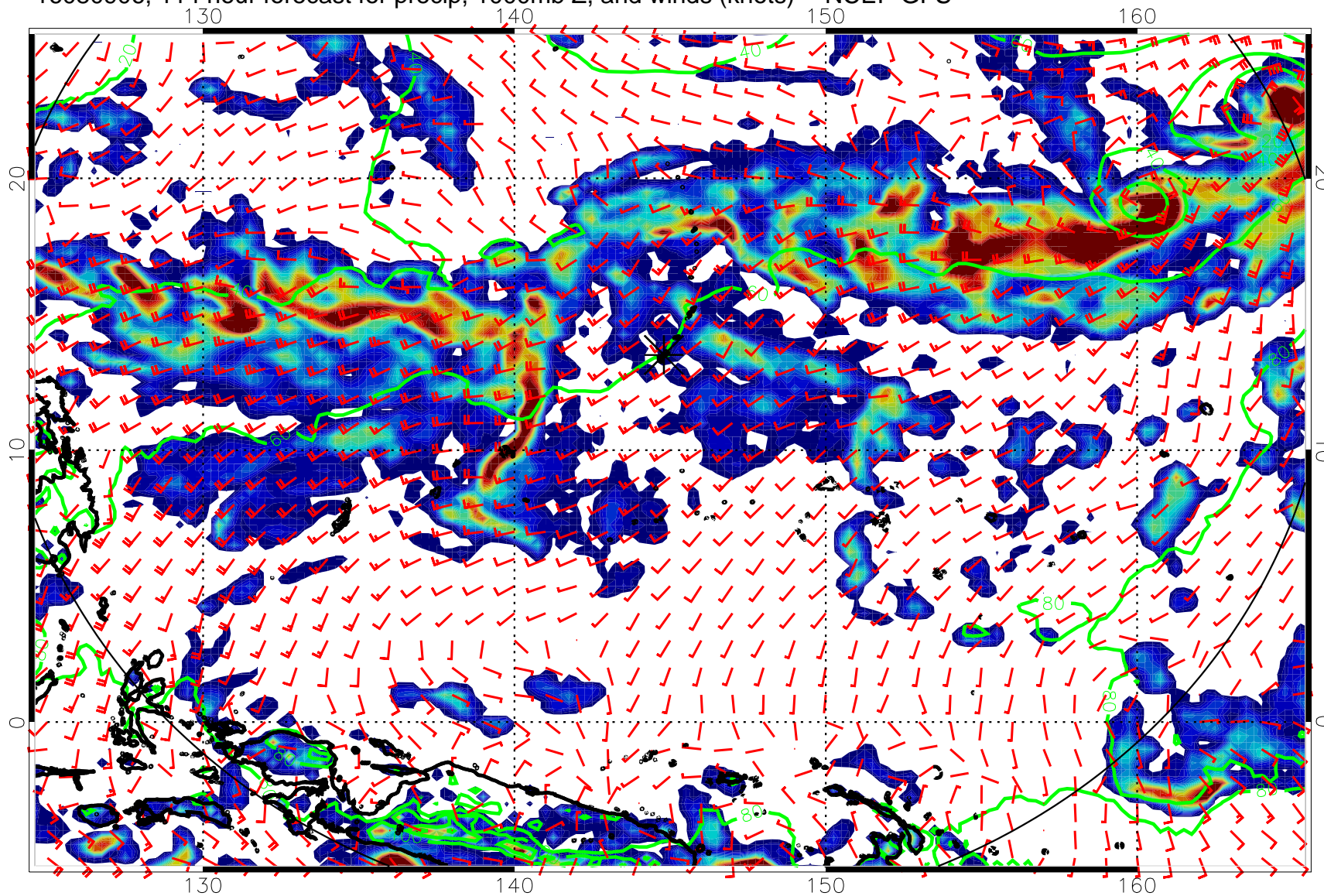
16080906, 114 hour forecast for precip, 1000mb Z, and winds (knots) -- NCEP GFS
