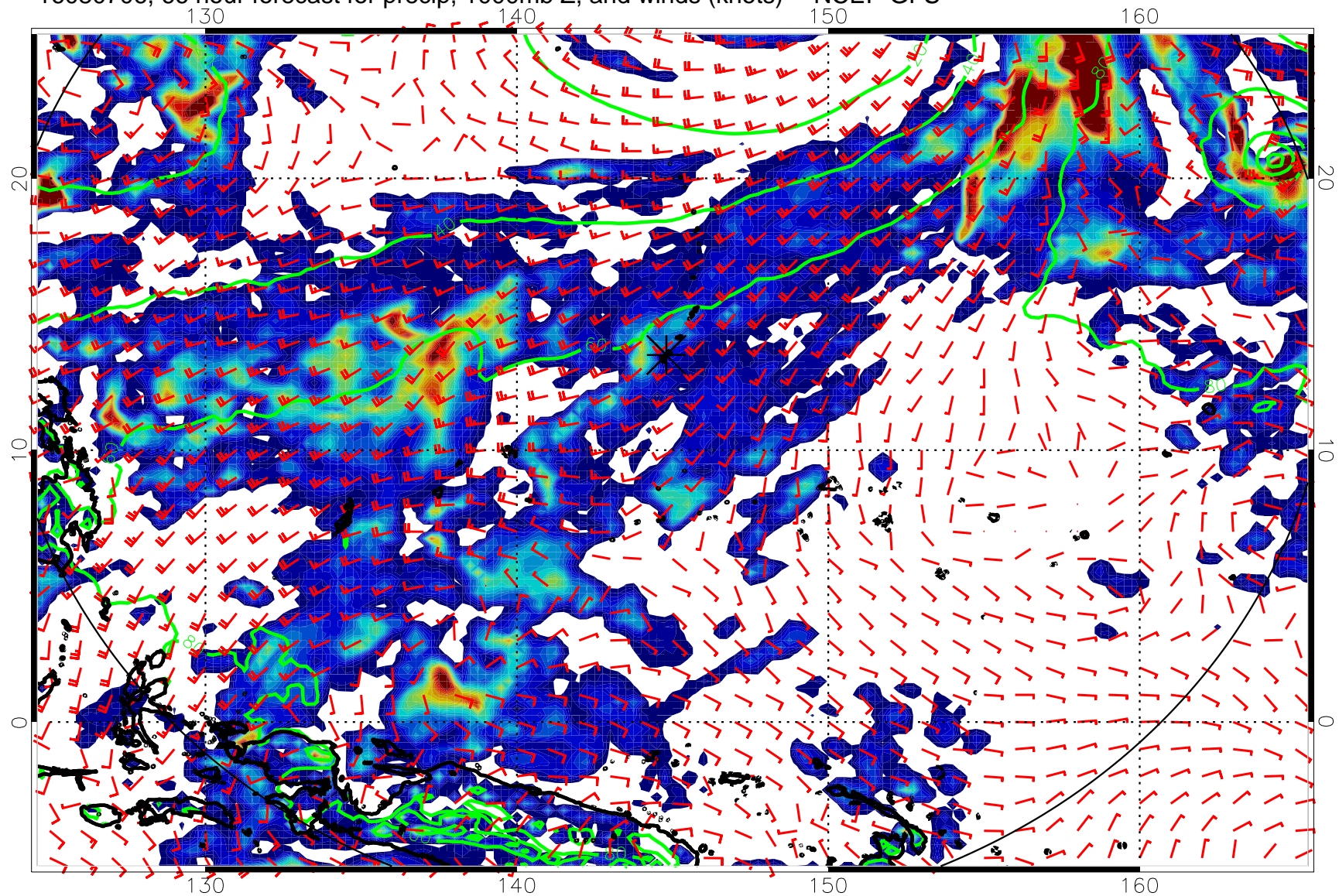
16080706, 66 hour forecast for precip, 1000mb Z, and winds (knots) -- NCEP GFS
