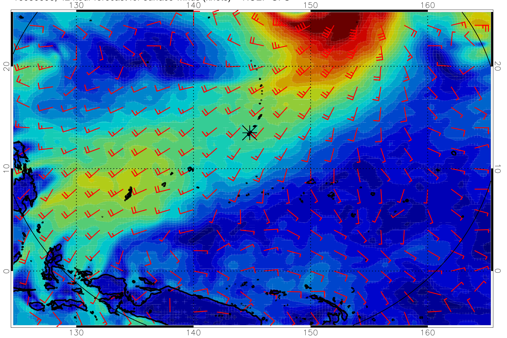
16080606, 42 hour forecast for surface winds (knots) -- NCEP GFS
