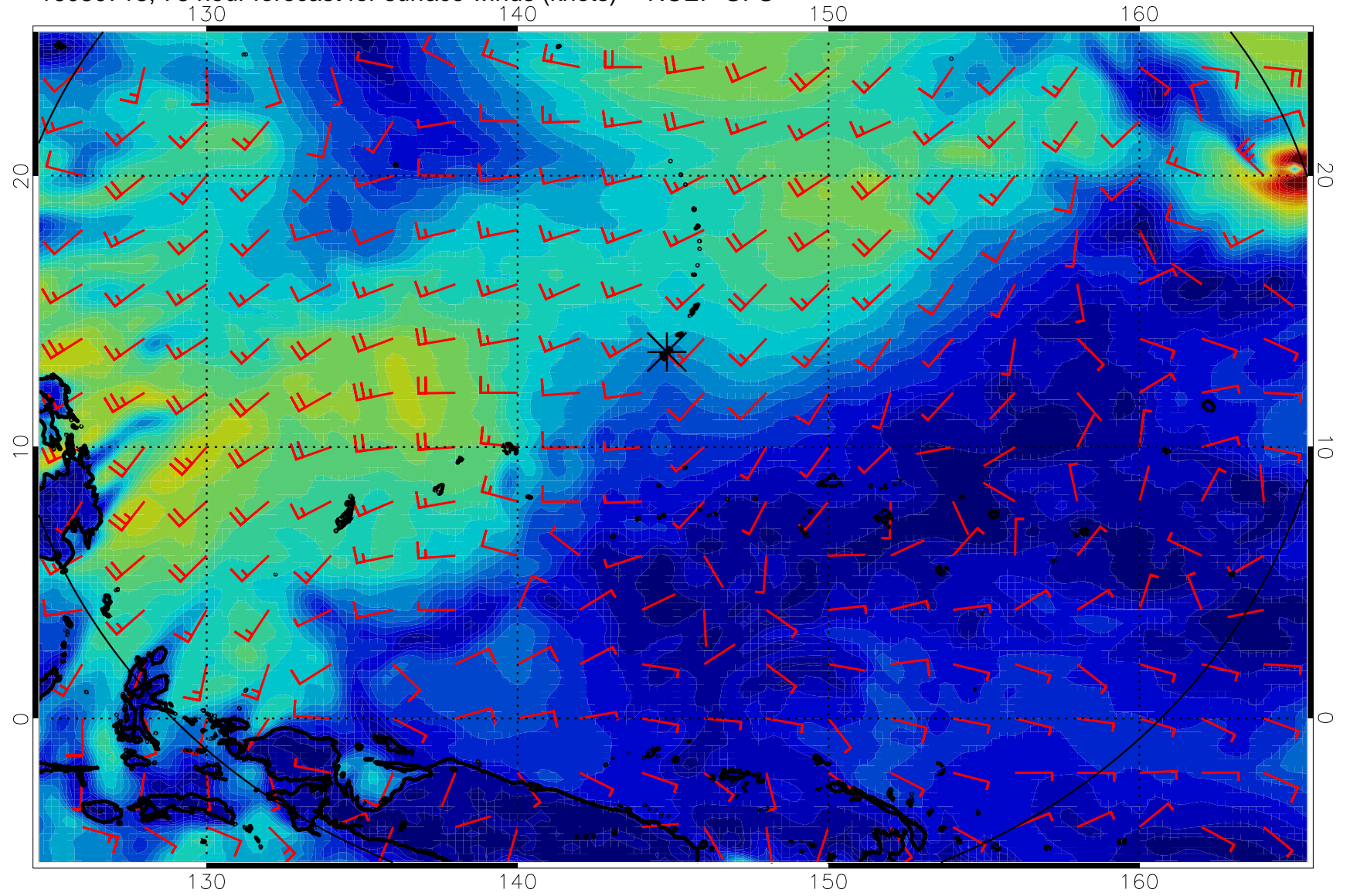
16080718, 78 hour forecast for surface winds (knots) -- NCEP GFS
