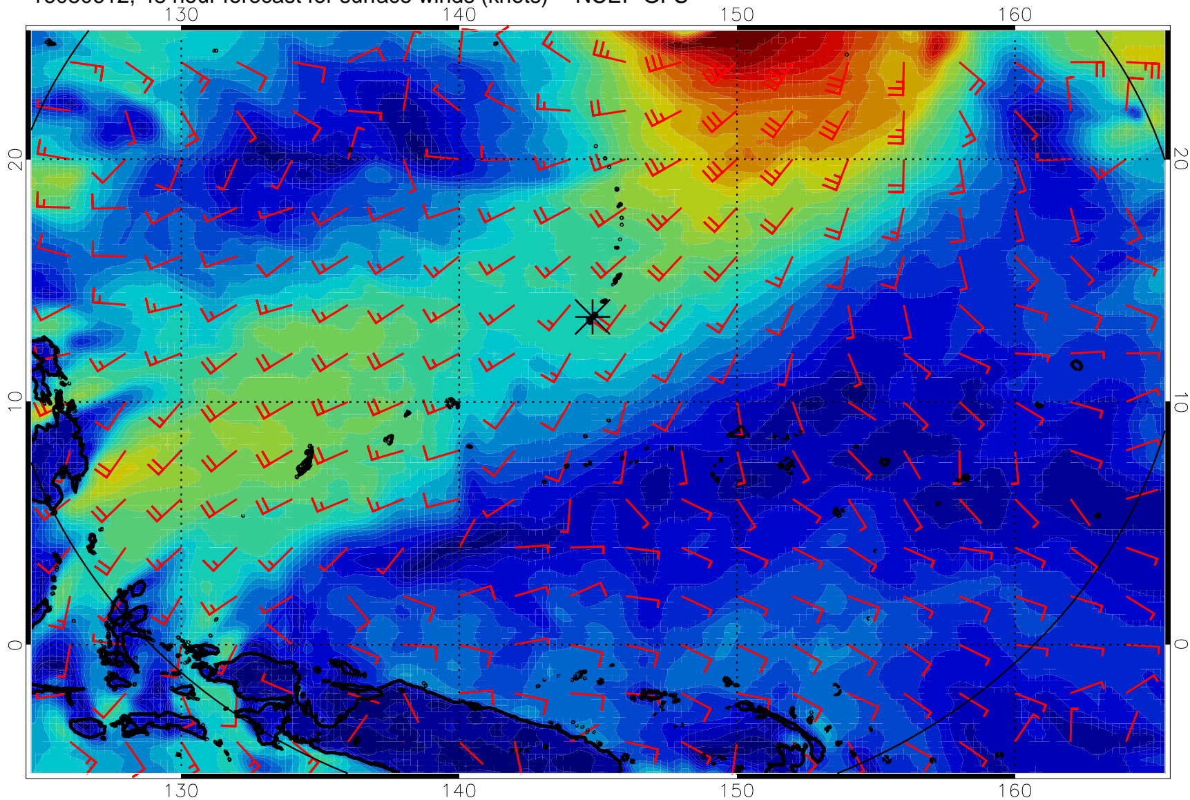
16080612, 48 hour forecast for surface winds (knots) -- NCEP GFS
