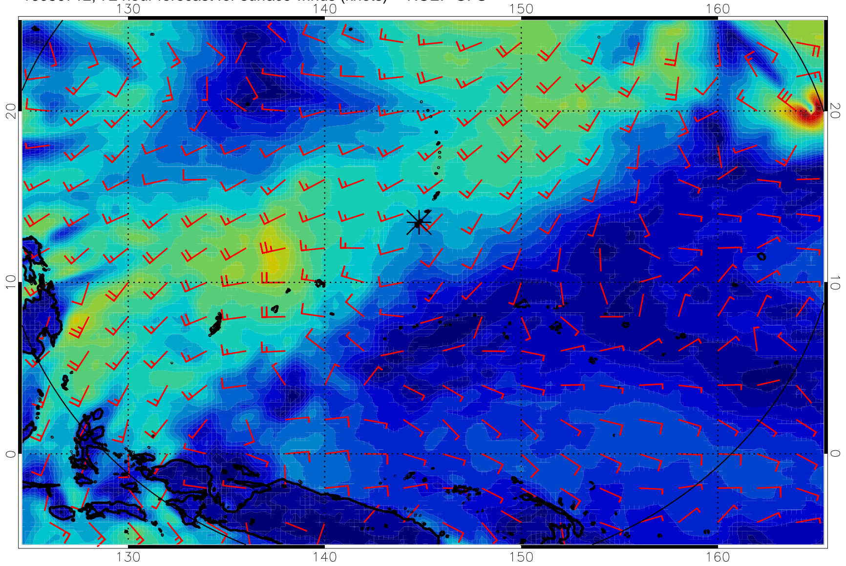
16080712, 72 hour forecast for surface winds (knots) -- NCEP GFS
