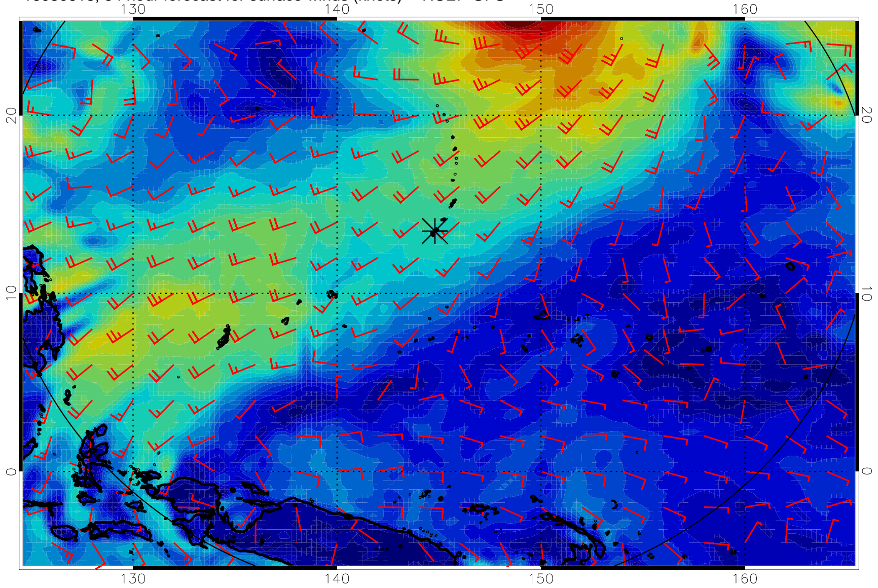
16080618, 54 hour forecast for surface winds (knots) -- NCEP GFS
