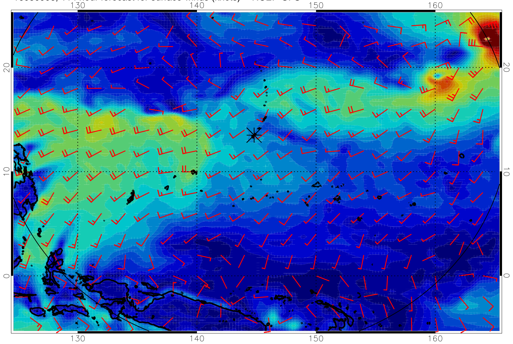
16080906, 114 hour forecast for surface winds (knots) -- NCEP GFS
