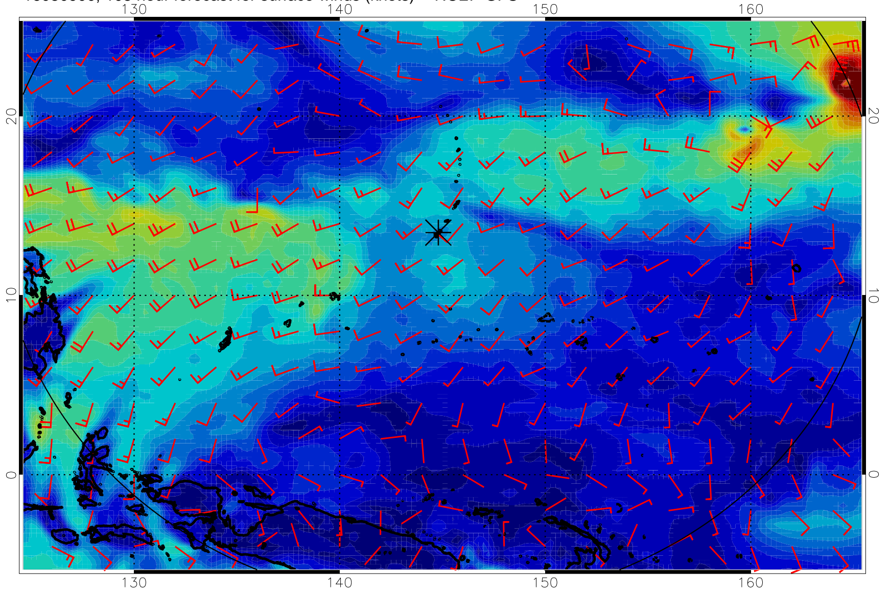
16080900, 108 hour forecast for surface winds (knots) -- NCEP GFS
