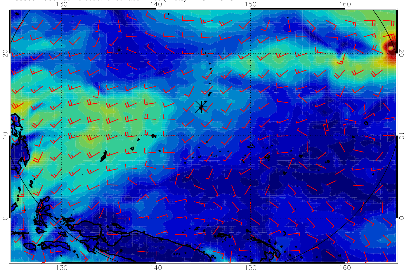
16080812, 96 hour forecast for surface winds (knots) -- NCEP GFS
