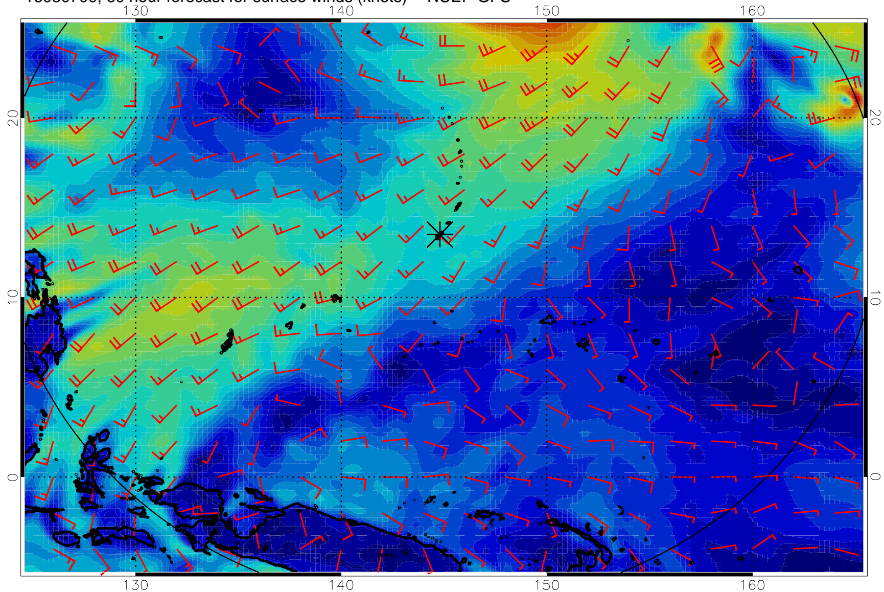
16080700, 60 hour forecast for surface winds (knots) -- NCEP GFS
