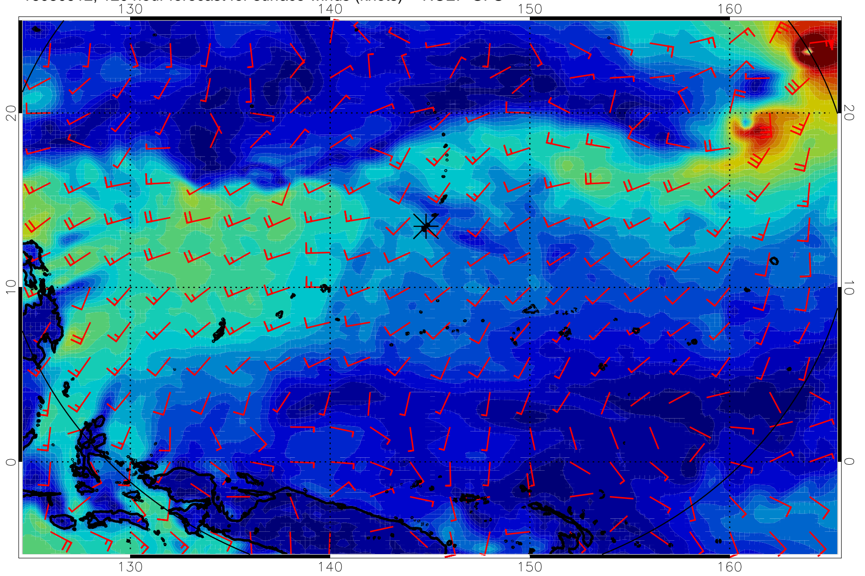
16080912, 120 hour forecast for surface winds (knots) -- NCEP GFS
