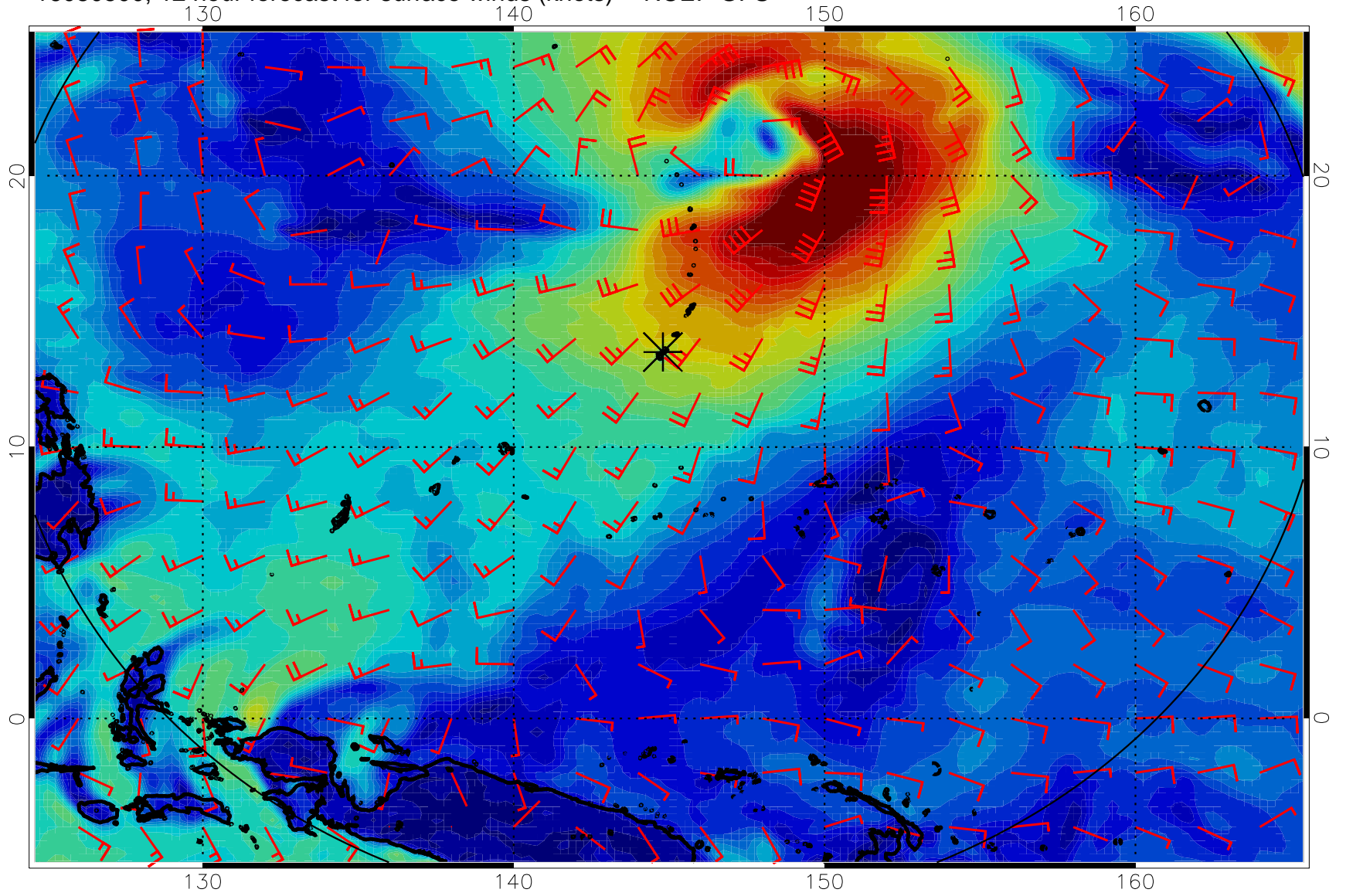
16080500, 12 hour forecast for surface winds (knots) -- NCEP GFS
