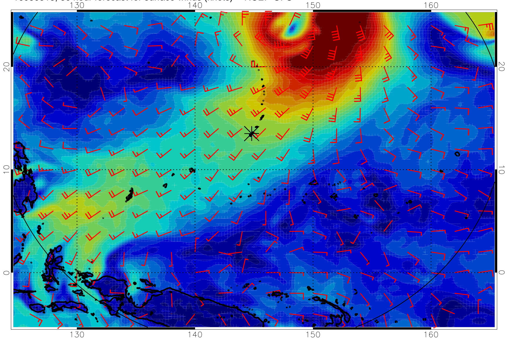
16080518, 30 hour forecast for surface winds (knots) -- NCEP GFS
