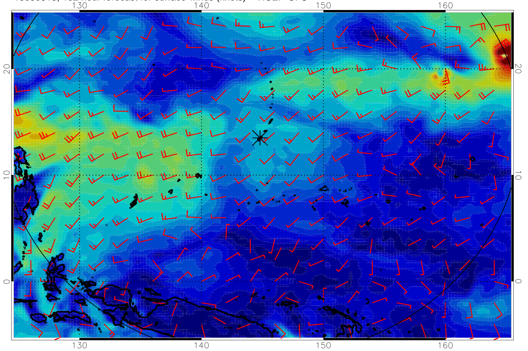
16080818, 102 hour forecast for surface winds (knots) -- NCEP GFS
