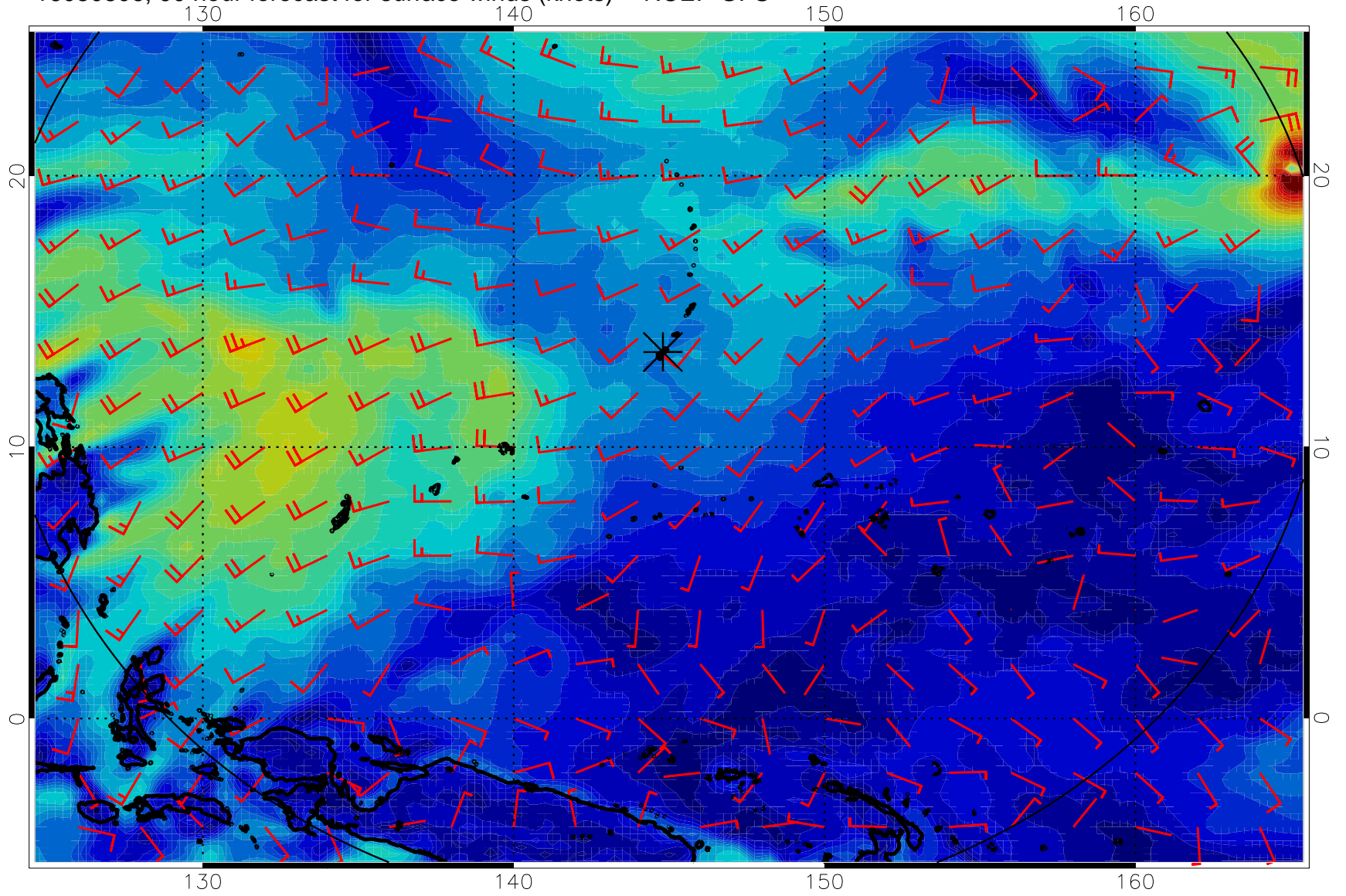
16080806, 90 hour forecast for surface winds (knots) -- NCEP GFS
