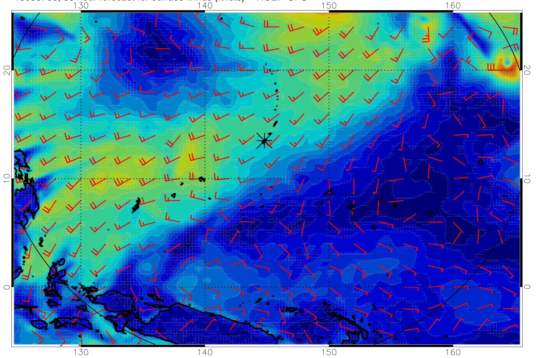
16080706, 66 hour forecast for surface winds (knots) -- NCEP GFS
