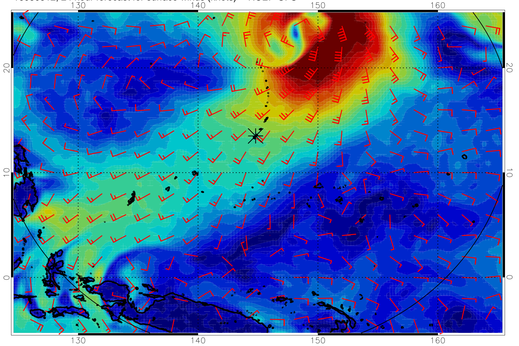
16080512, 24 hour forecast for surface winds (knots) -- NCEP GFS
