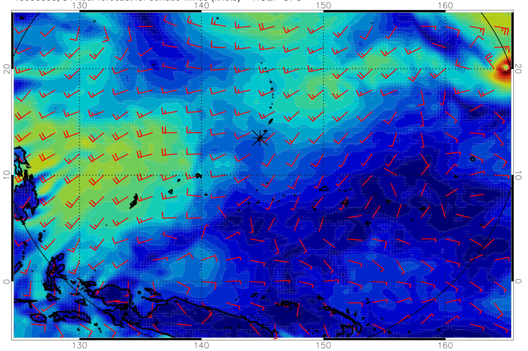
16080800, 84 hour forecast for surface winds (knots) -- NCEP GFS
