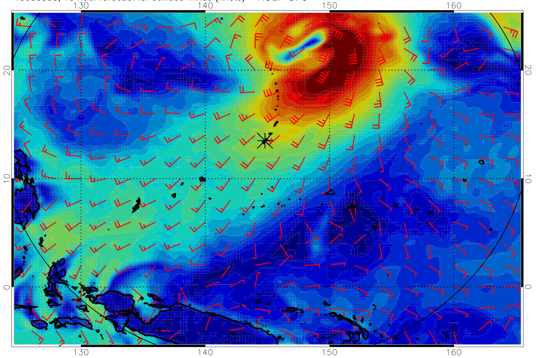
16080506, 18 hour forecast for surface winds (knots) -- NCEP GFS
