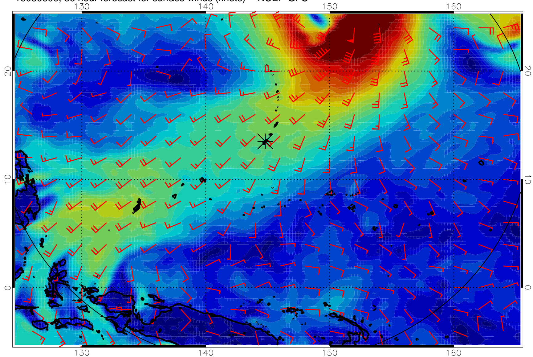
16080600, 36 hour forecast for surface winds (knots) -- NCEP GFS
