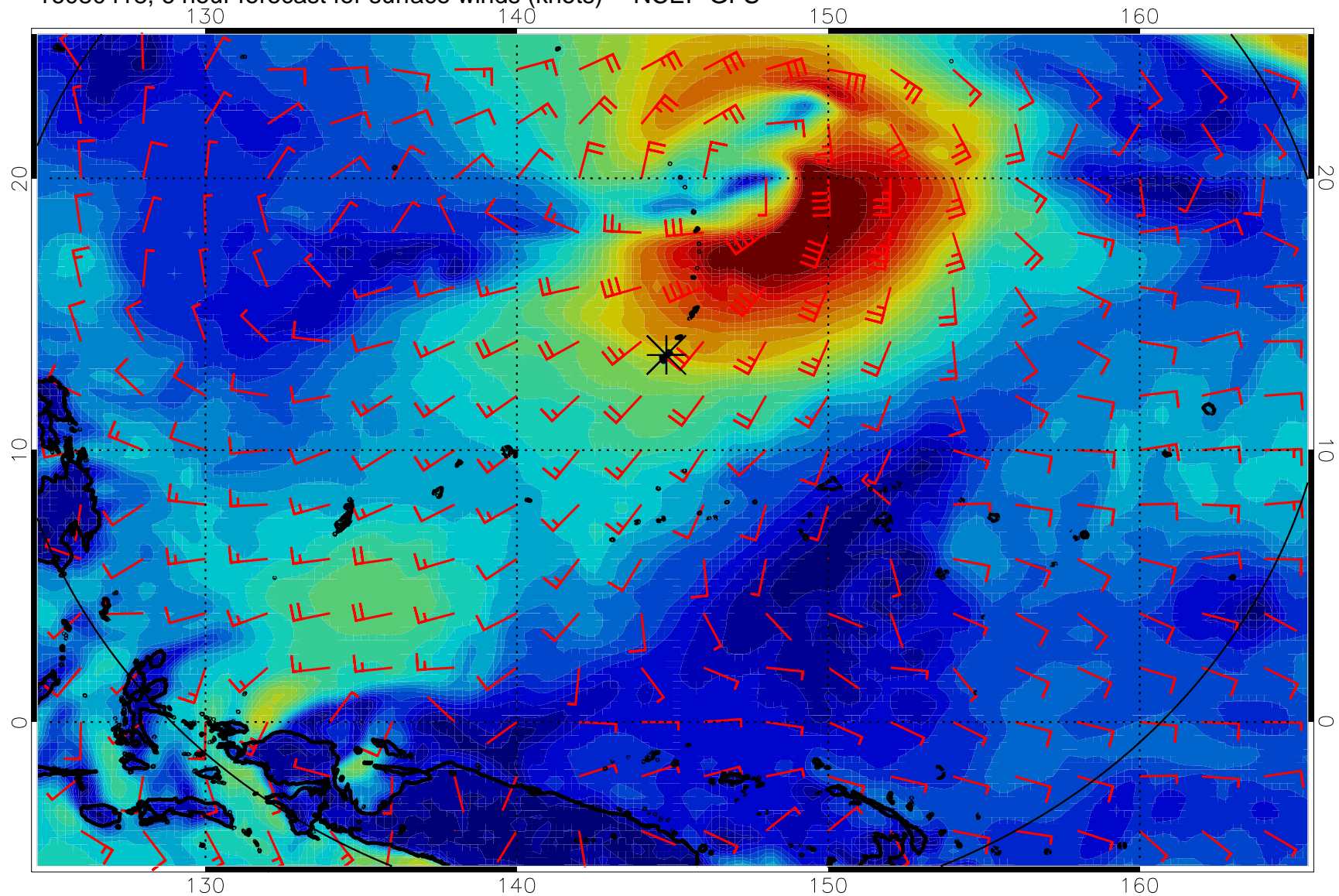
16080418, 6 hour forecast for surface winds (knots) -- NCEP GFS
