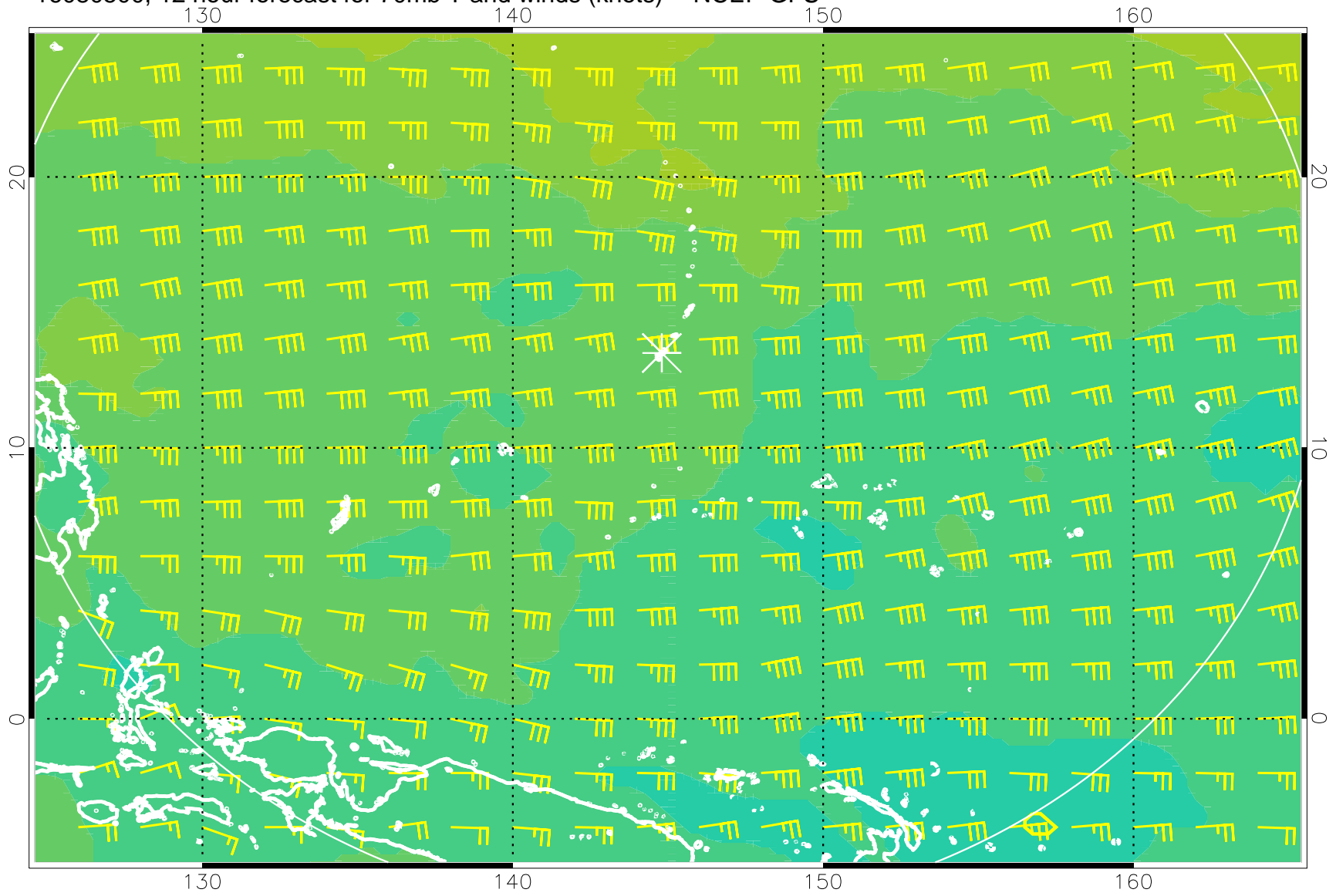
16080500, 12 hour forecast for 70mb T and winds (knots) -- NCEP GFS
