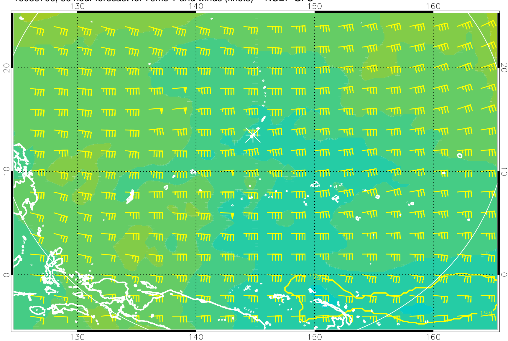
16080706, 66 hour forecast for 70mb T and winds (knots) -- NCEP GFS
