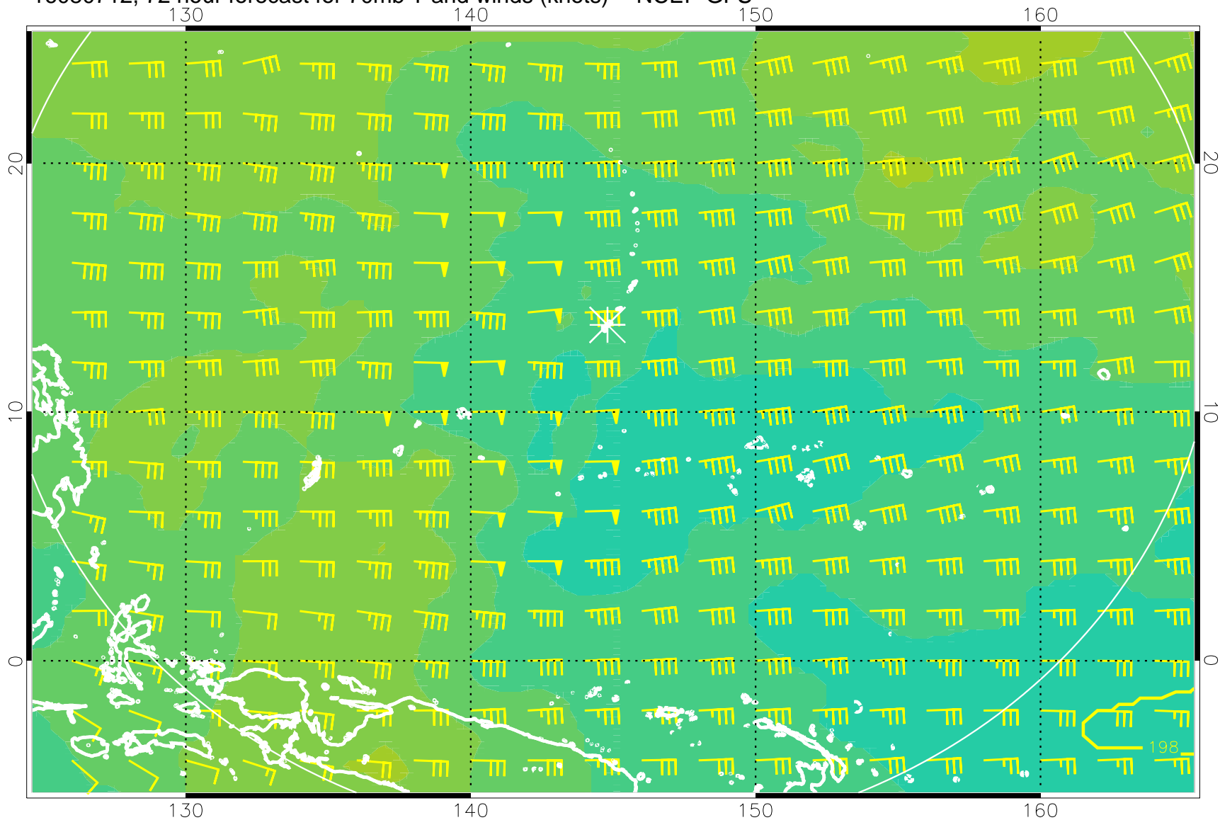
16080712, 72 hour forecast for 70mb T and winds (knots) -- NCEP GFS
