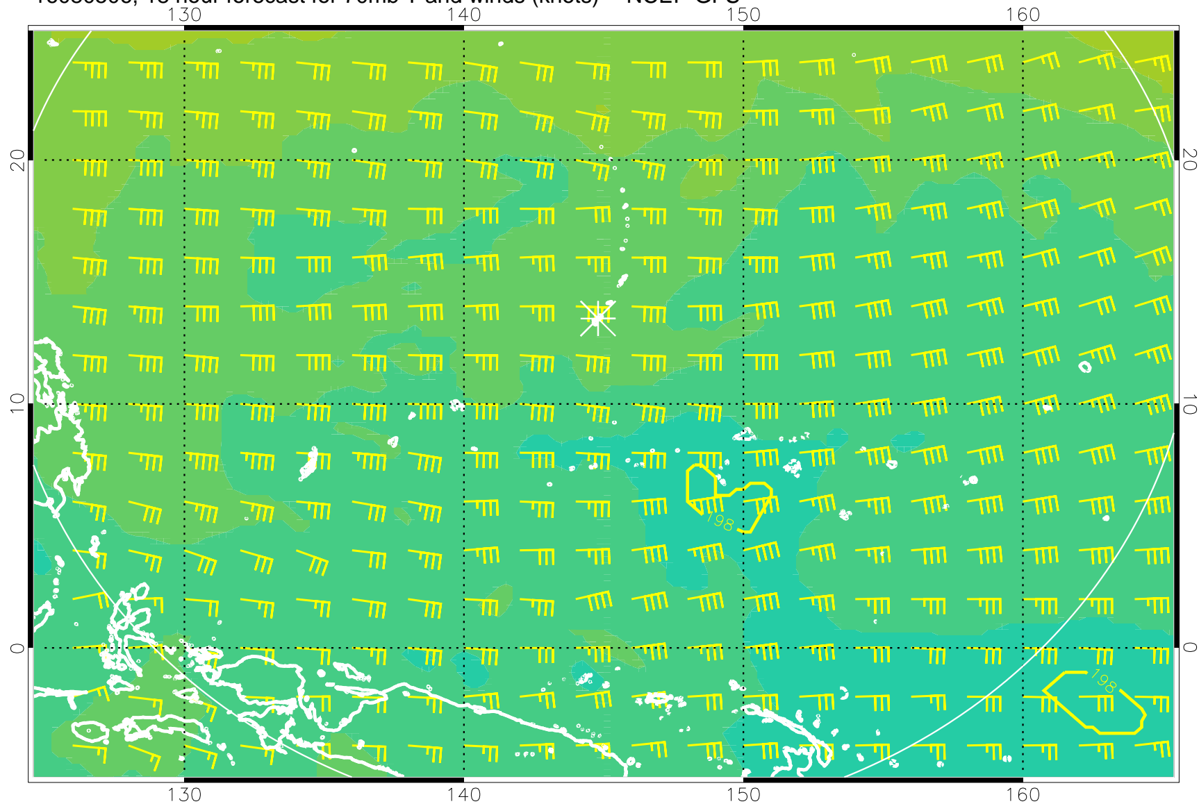
16080506, 18 hour forecast for 70mb T and winds (knots) -- NCEP GFS
