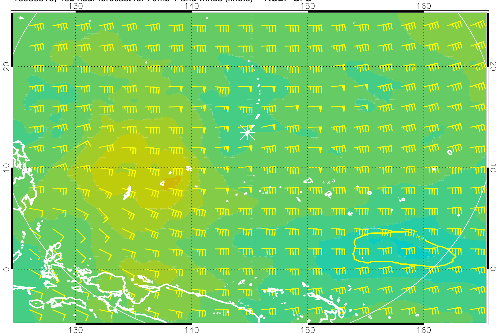
16080818, 102 hour forecast for 70mb T and winds (knots) -- NCEP GFS
