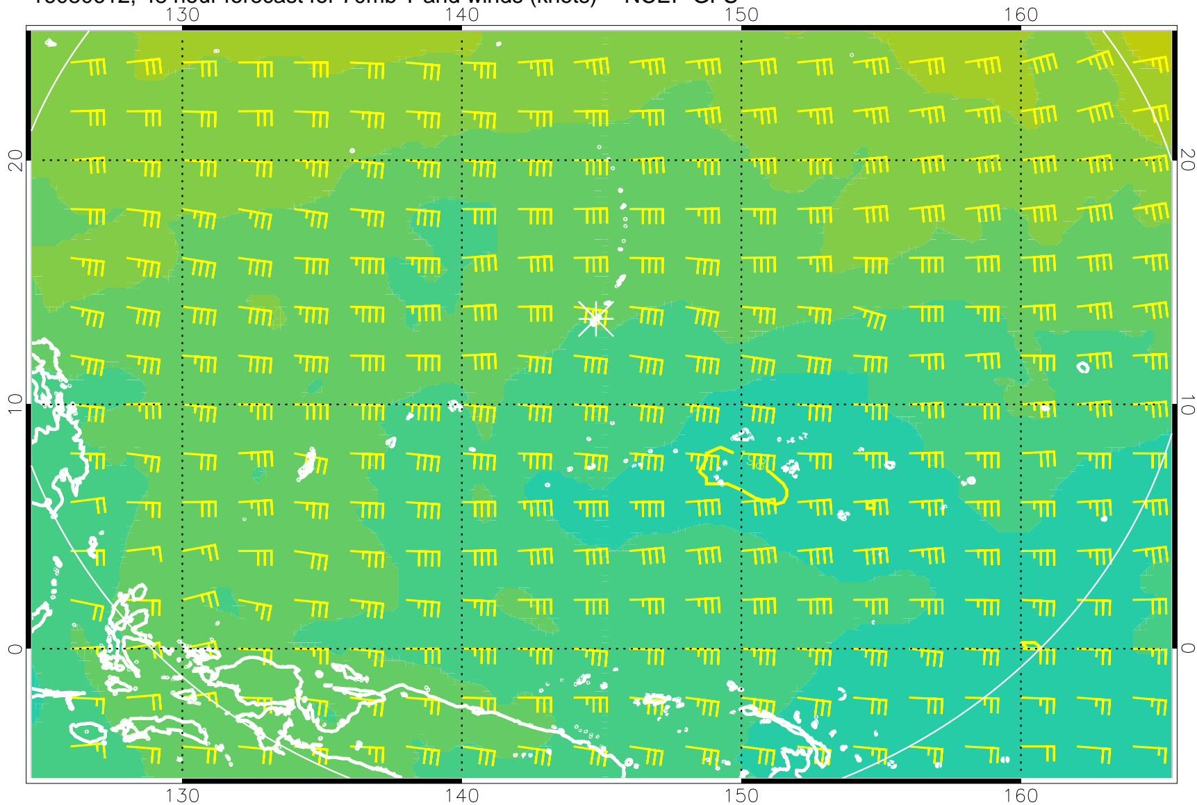
16080612, 48 hour forecast for 70mb T and winds (knots) -- NCEP GFS
