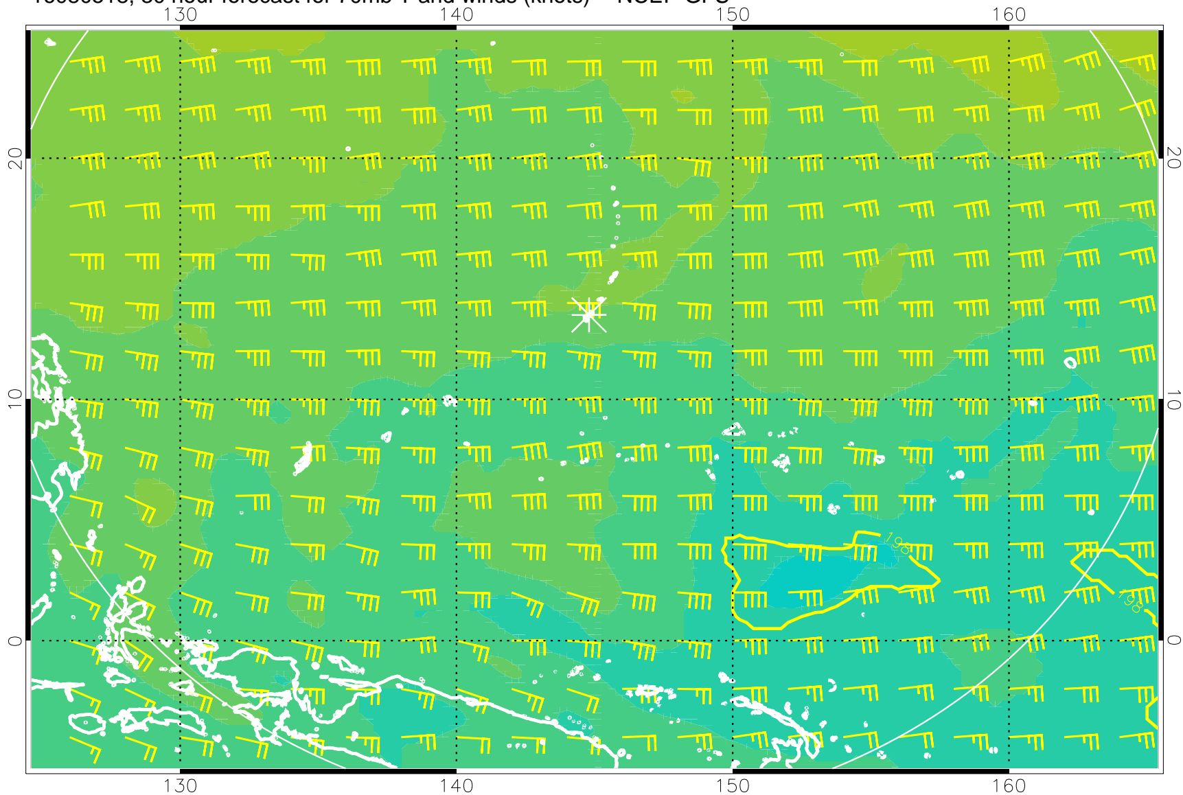
16080518, 30 hour forecast for 70mb T and winds (knots) -- NCEP GFS
