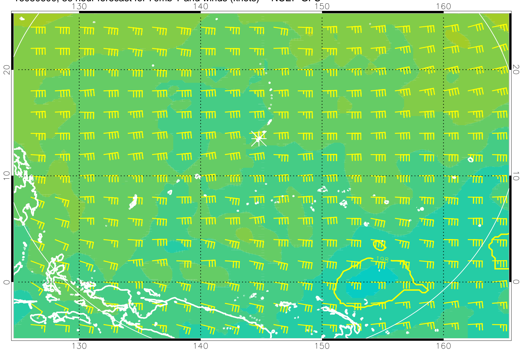
16080600, 36 hour forecast for 70mb T and winds (knots) -- NCEP GFS
