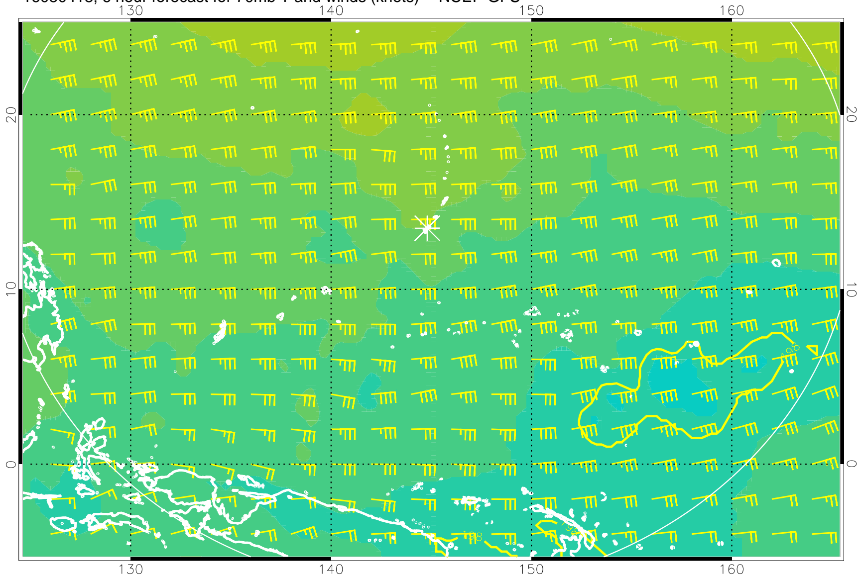
16080418, 6 hour forecast for 70mb T and winds (knots) -- NCEP GFS
