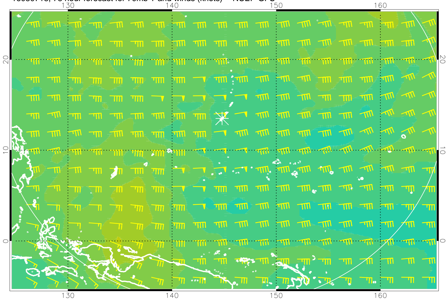
16080718, 78 hour forecast for 70mb T and winds (knots) -- NCEP GFS
