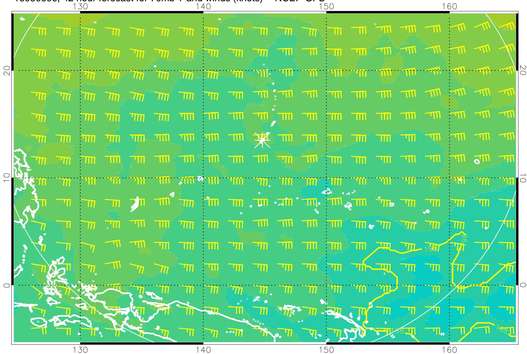
16080606, 42 hour forecast for 70mb T and winds (knots) -- NCEP GFS
