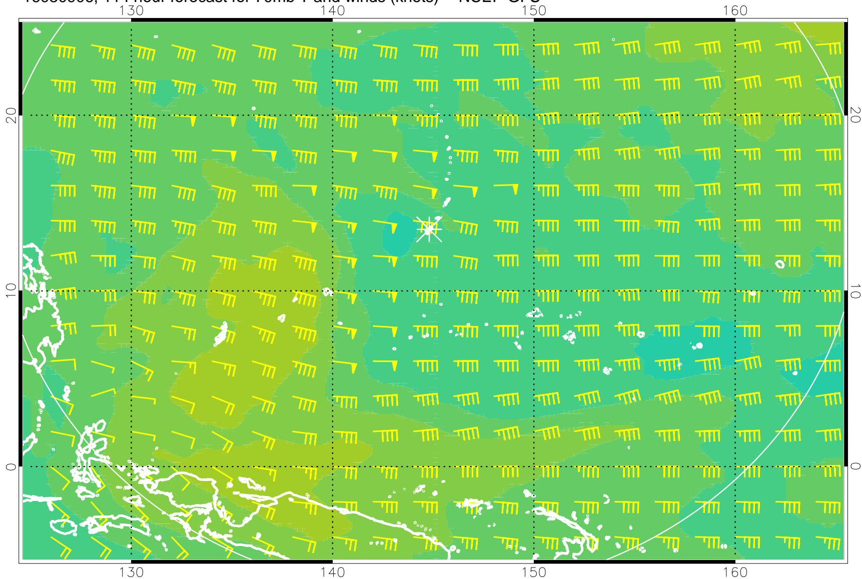
16080906, 114 hour forecast for 70mb T and winds (knots) -- NCEP GFS
