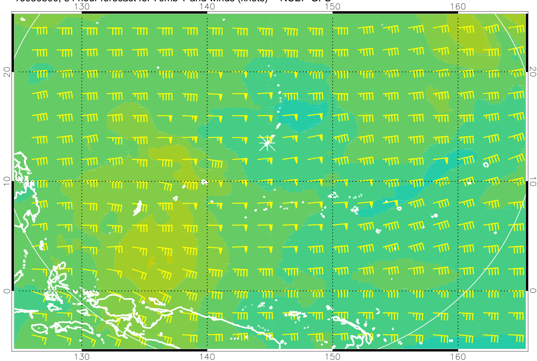
16080800, 84 hour forecast for 70mb T and winds (knots) -- NCEP GFS
