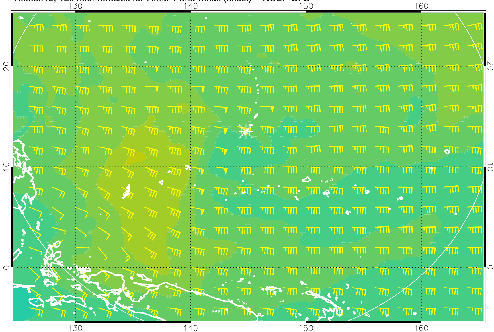
16080912, 120 hour forecast for 70mb T and winds (knots) -- NCEP GFS
