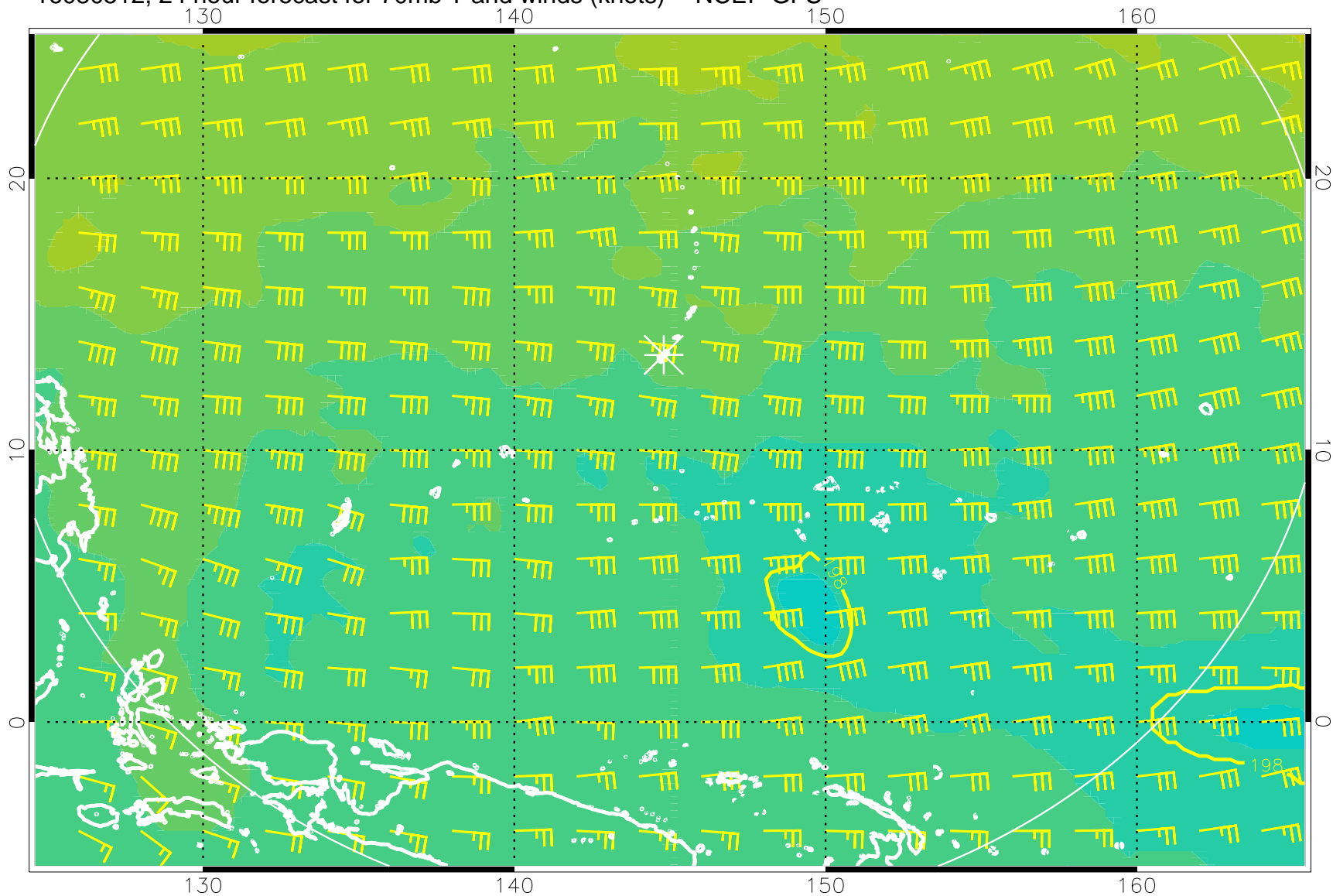
16080512, 24 hour forecast for 70mb T and winds (knots) -- NCEP GFS
