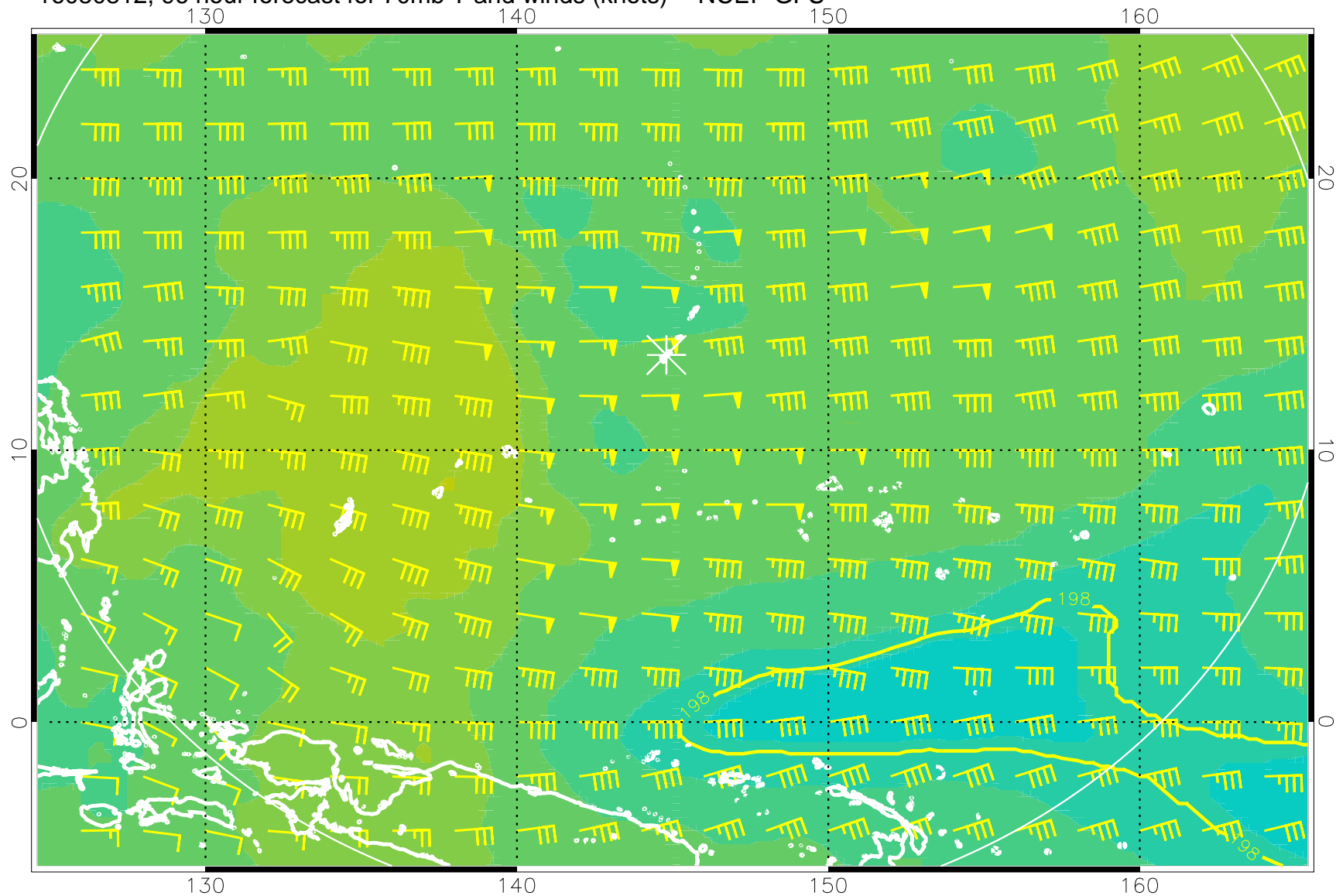
16080812, 96 hour forecast for 70mb T and winds (knots) -- NCEP GFS
