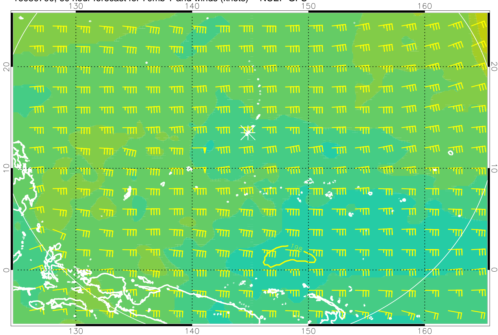
16080700, 60 hour forecast for 70mb T and winds (knots) -- NCEP GFS
