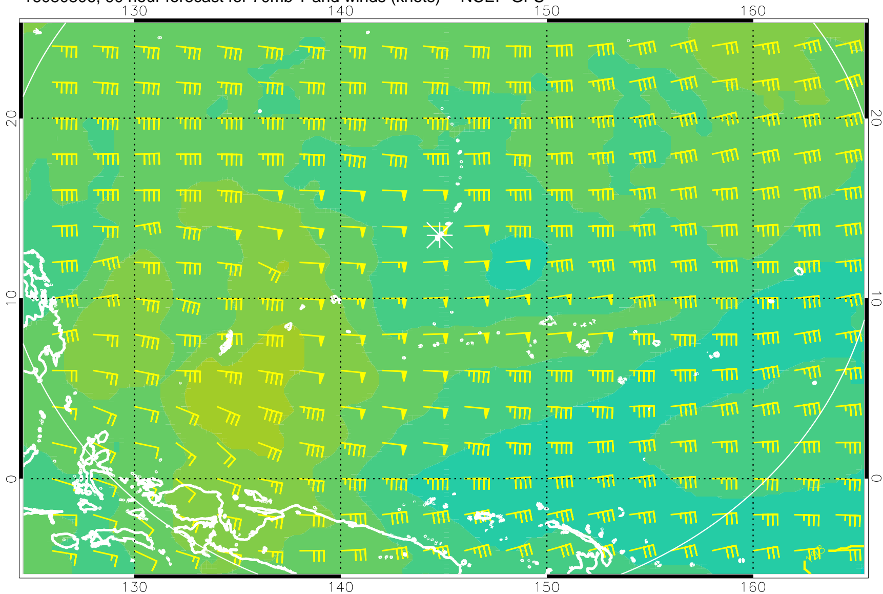
16080806, 90 hour forecast for 70mb T and winds (knots) -- NCEP GFS
