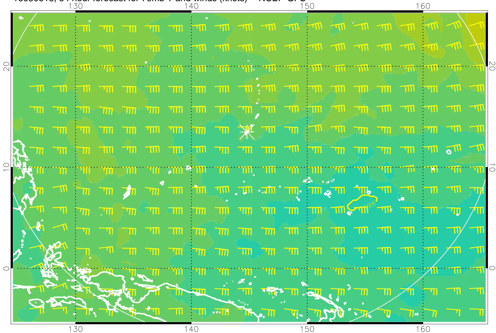
16080618, 54 hour forecast for 70mb T and winds (knots) -- NCEP GFS
