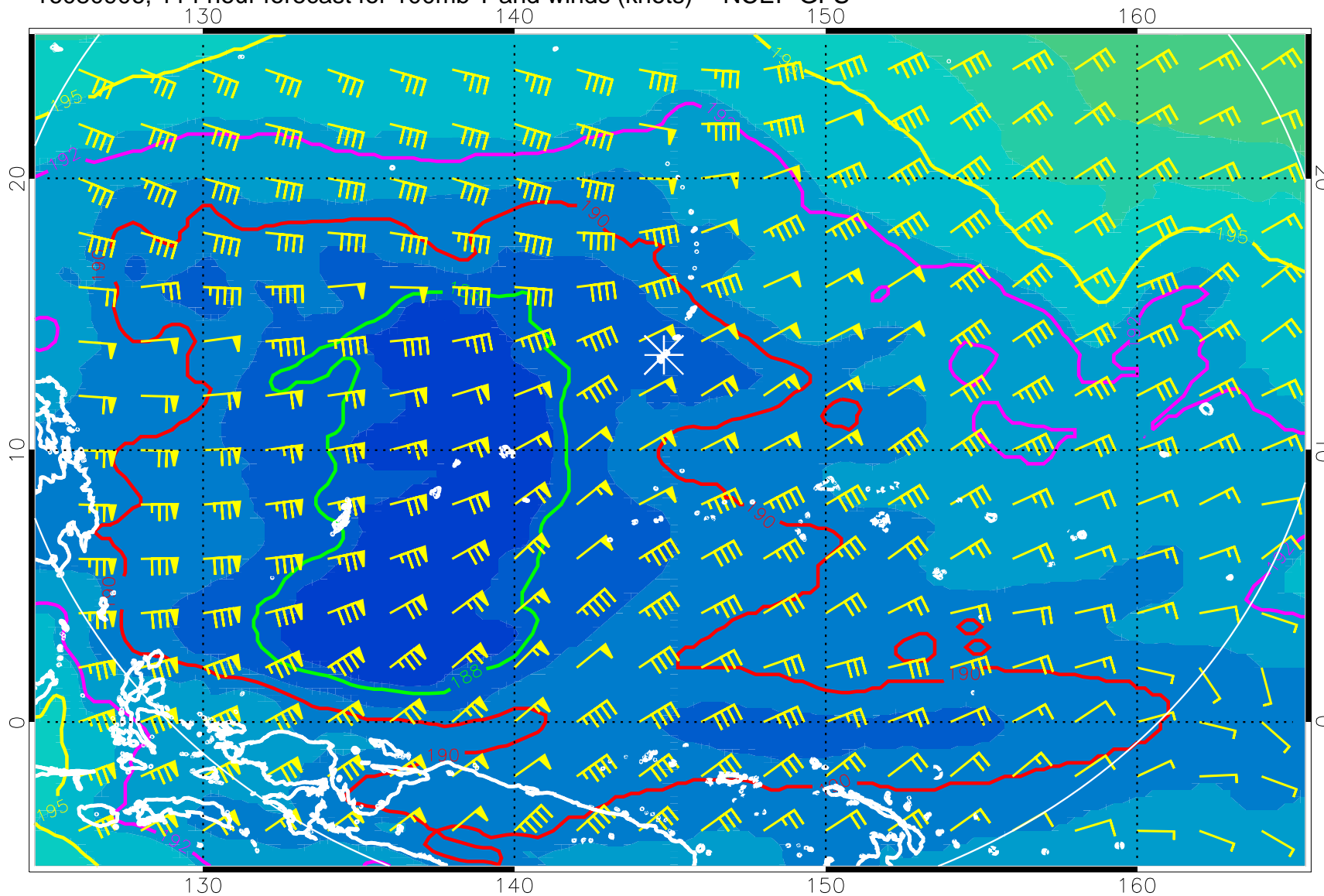
16080906, 114 hour forecast for 100mb T and winds (knots) -- NCEP GFS
