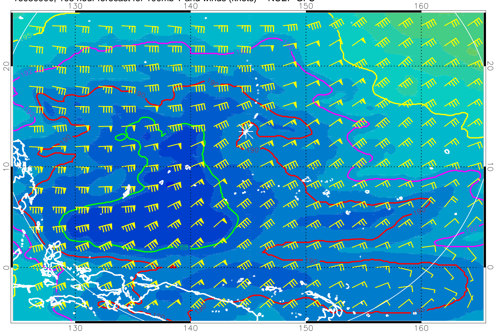
16080900, 108 hour forecast for 100mb T and winds (knots) -- NCEP GFS
