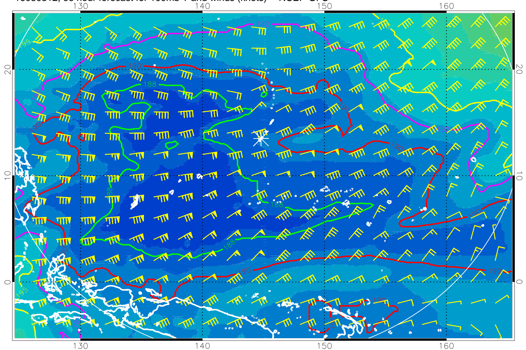
16080812, 96 hour forecast for 100mb T and winds (knots) -- NCEP GFS
