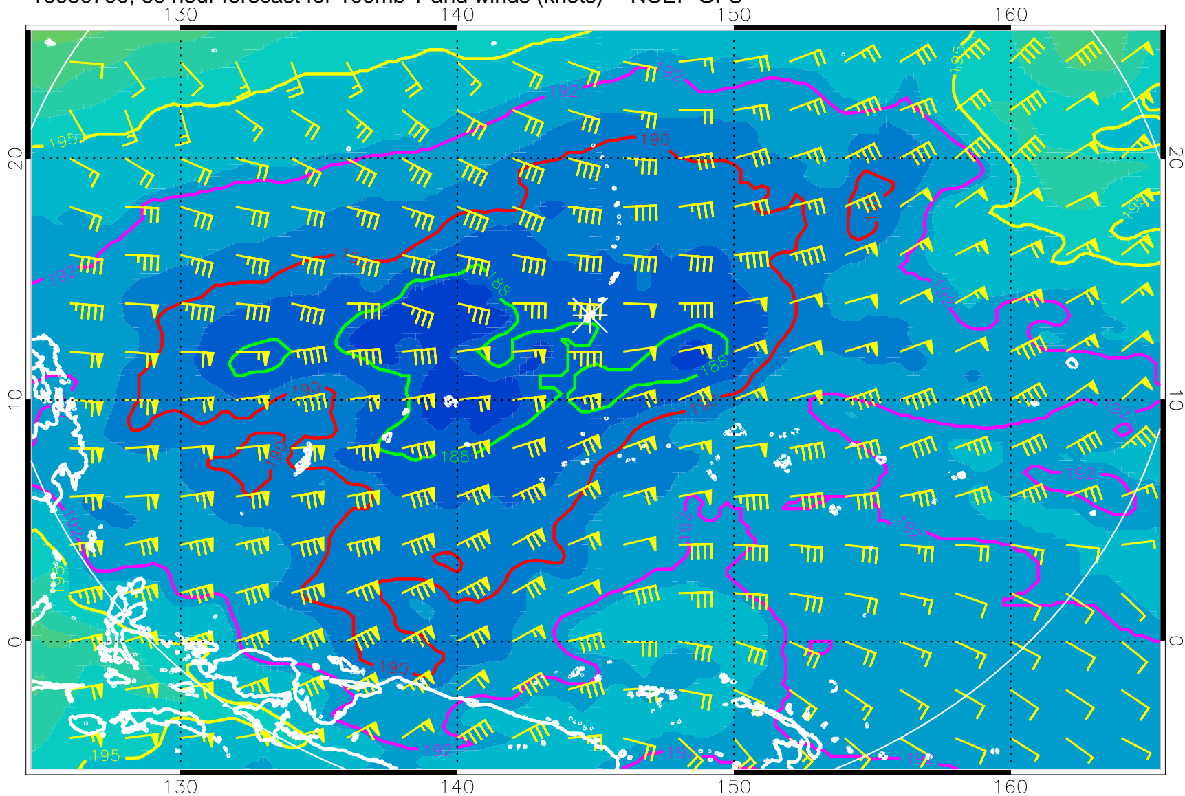
16080700, 60 hour forecast for 100mb T and winds (knots) -- NCEP GFS
