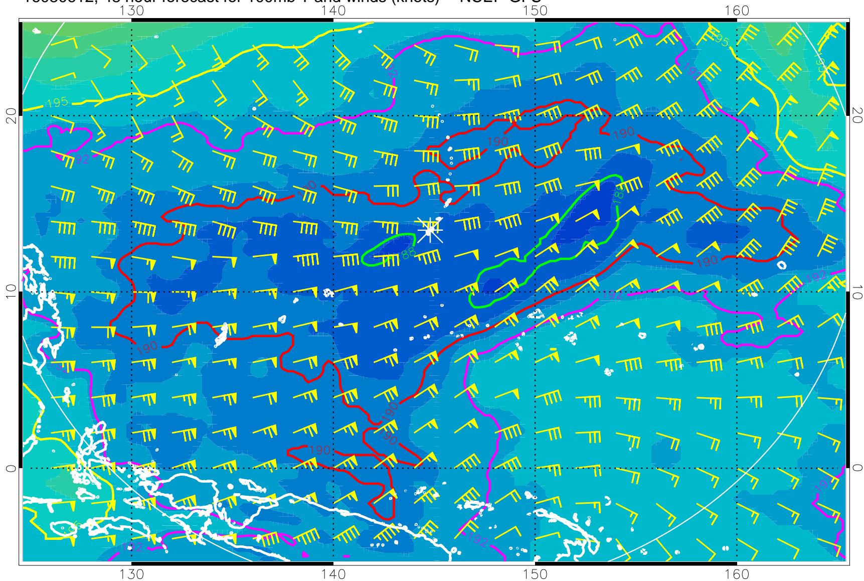
16080612, 48 hour forecast for 100mb T and winds (knots) -- NCEP GFS
