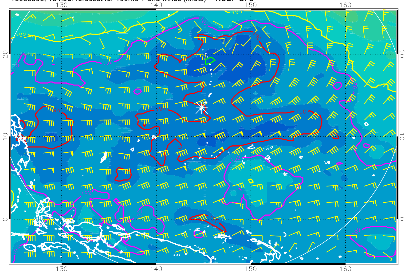
16080506, 18 hour forecast for 100mb T and winds (knots) -- NCEP GFS
