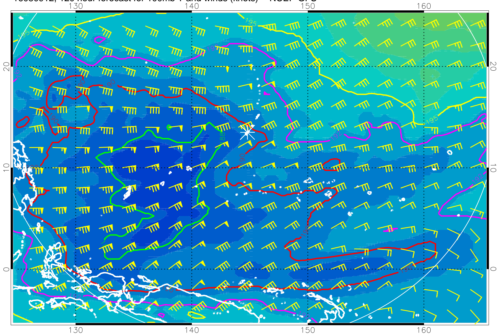
16080912, 120 hour forecast for 100mb T and winds (knots) -- NCEP GFS
