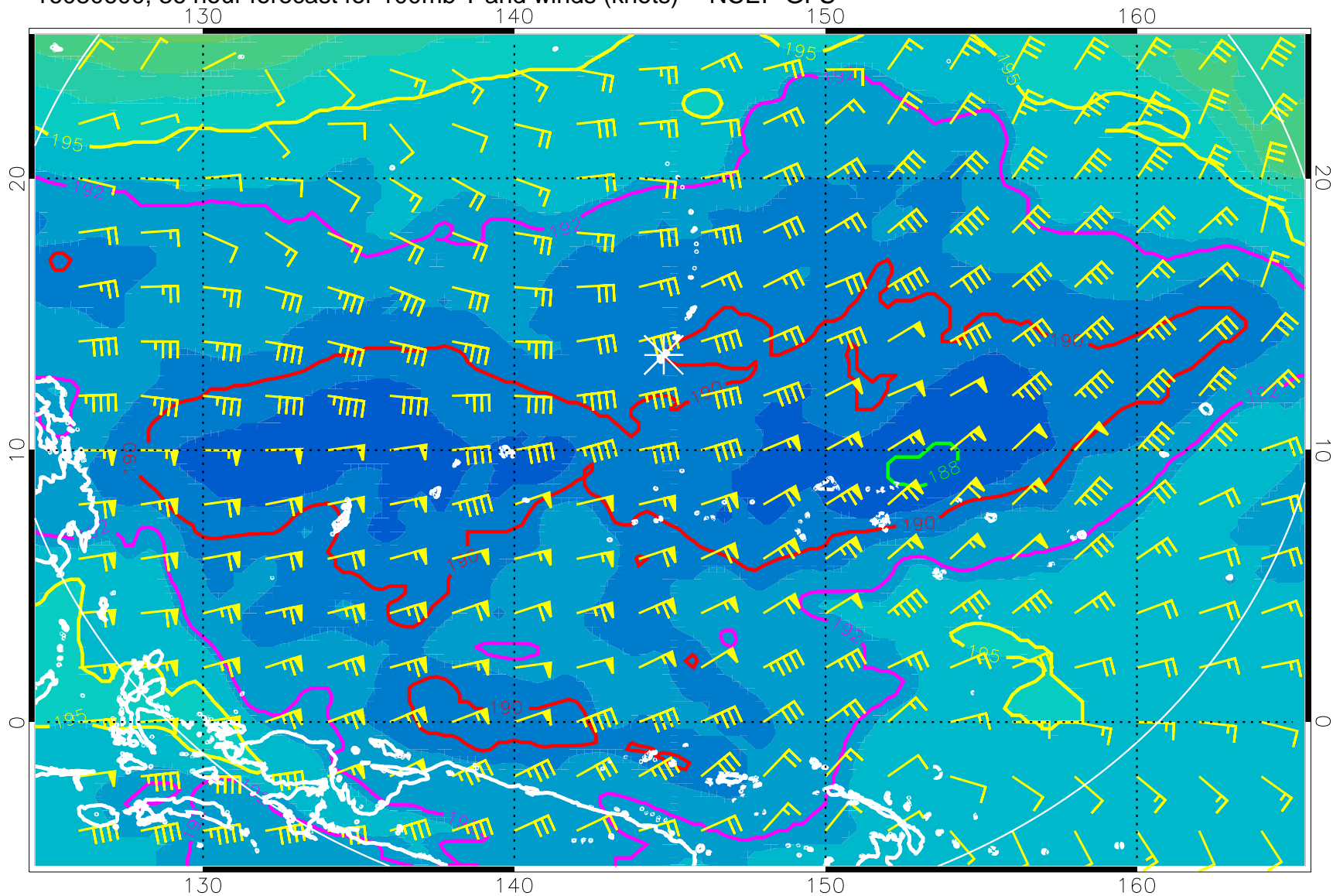
16080600, 36 hour forecast for 100mb T and winds (knots) -- NCEP GFS
