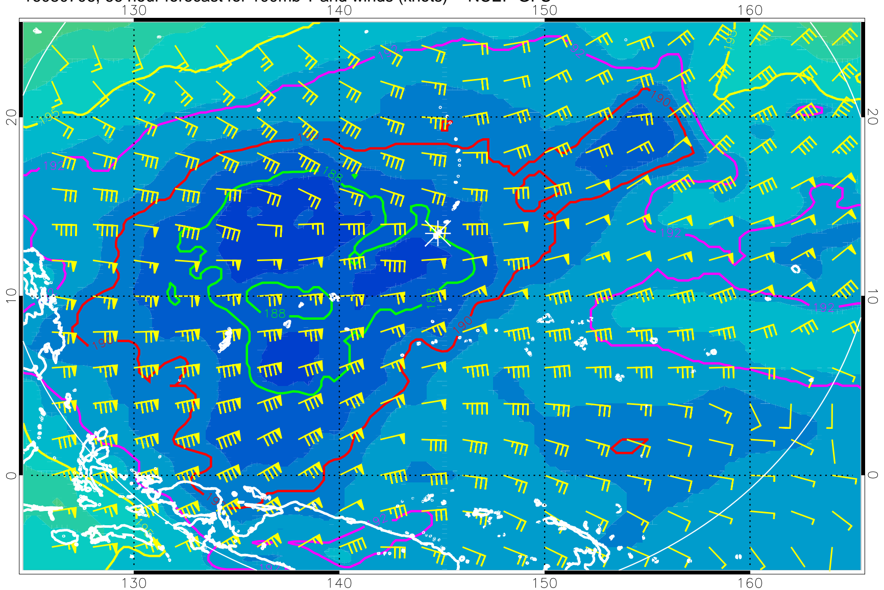
16080706, 66 hour forecast for 100mb T and winds (knots) -- NCEP GFS
