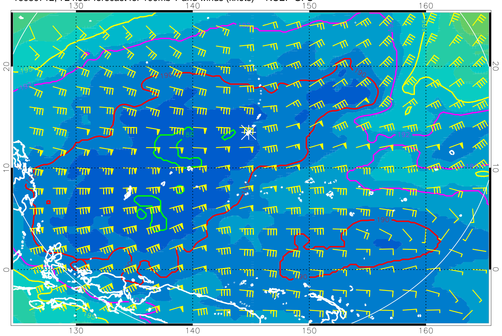
16080712, 72 hour forecast for 100mb T and winds (knots) -- NCEP GFS
