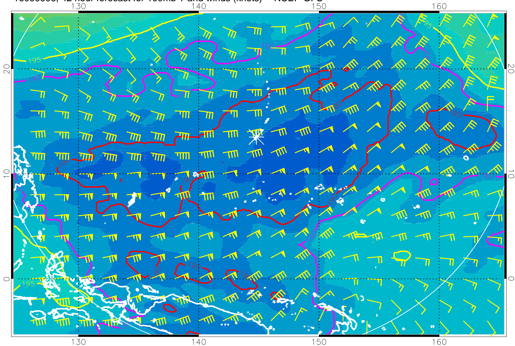
16080606, 42 hour forecast for 100mb T and winds (knots) -- NCEP GFS
