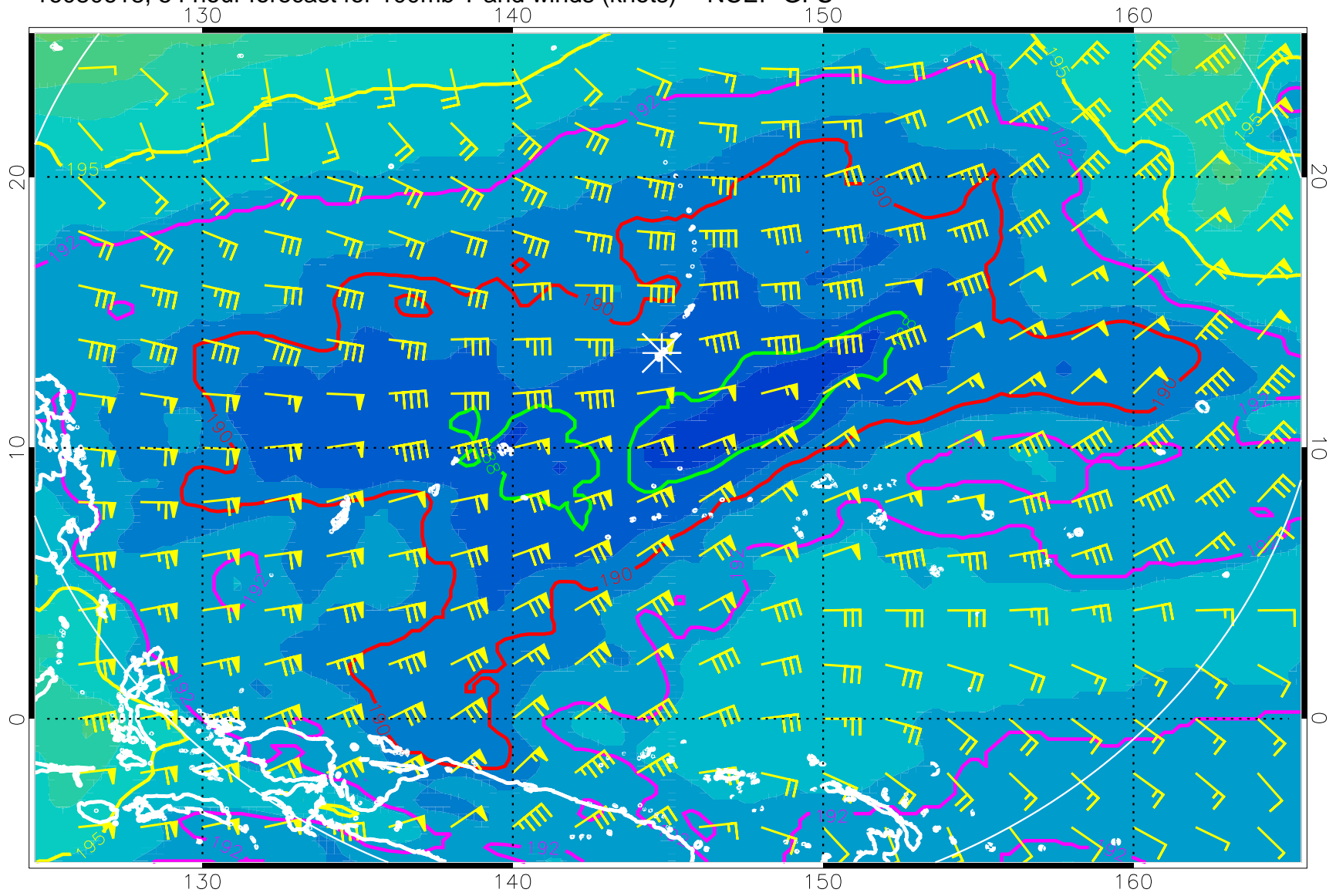
16080618, 54 hour forecast for 100mb T and winds (knots) -- NCEP GFS
