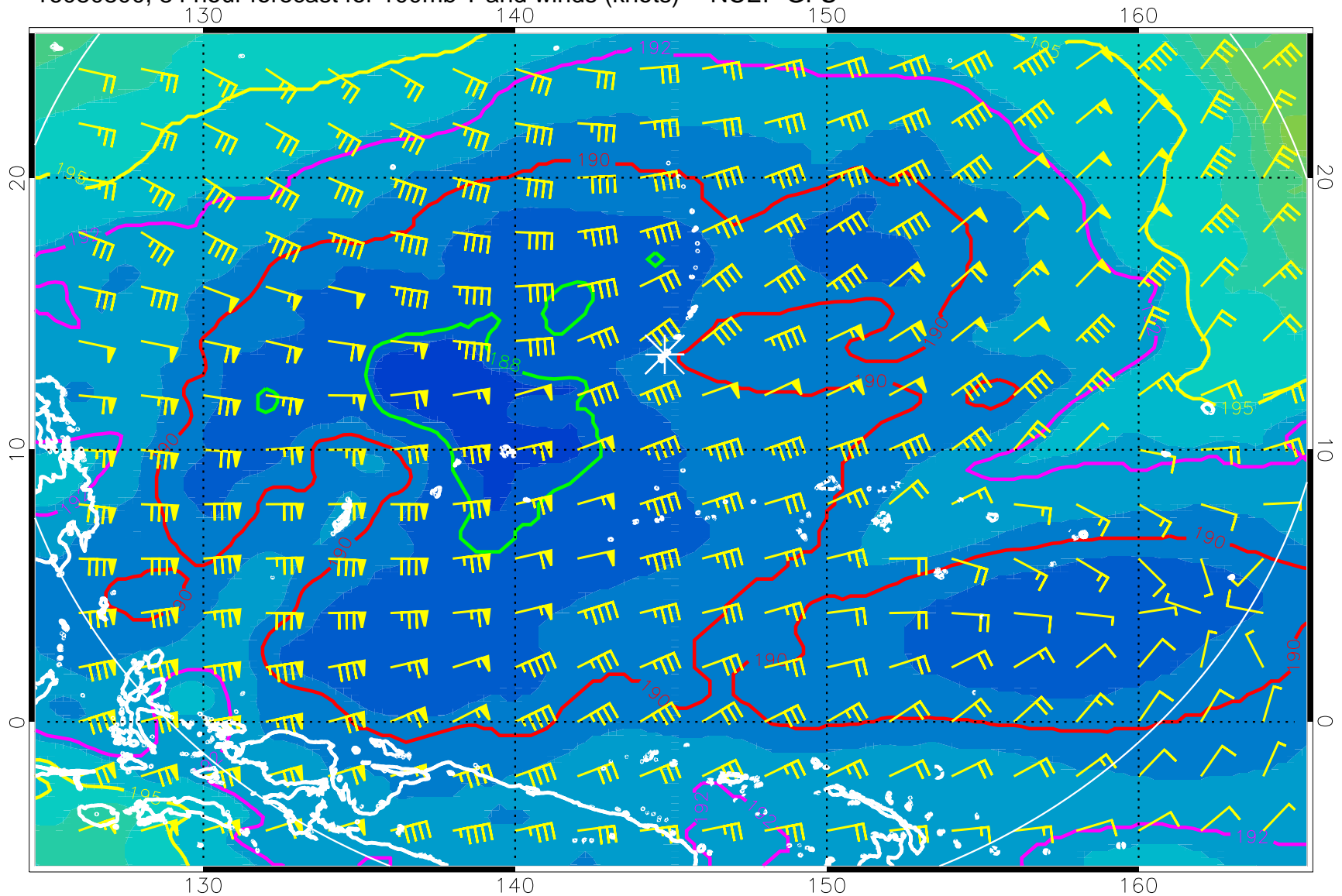
16080800, 84 hour forecast for 100mb T and winds (knots) -- NCEP GFS
