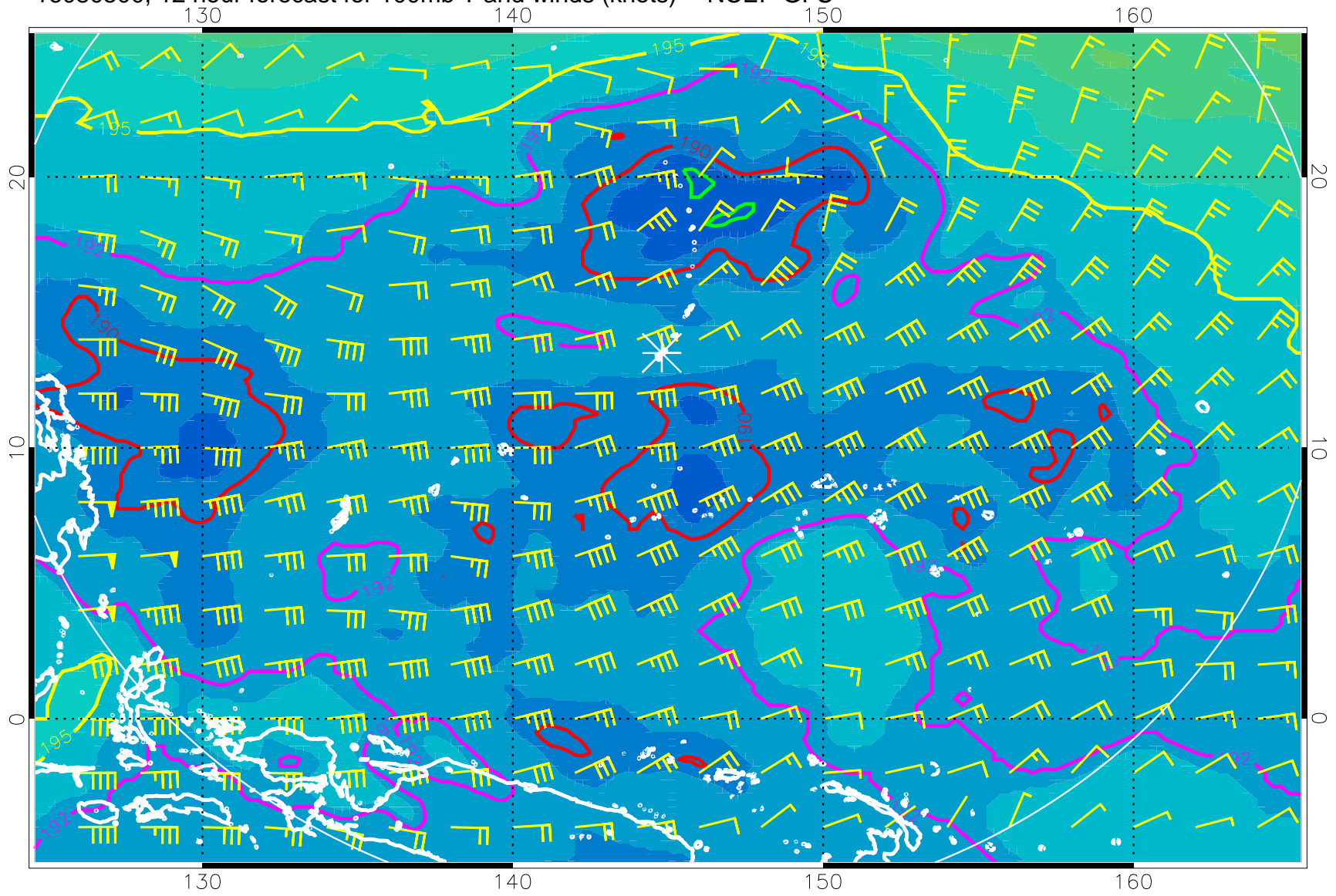
16080500, 12 hour forecast for 100mb T and winds (knots) -- NCEP GFS
