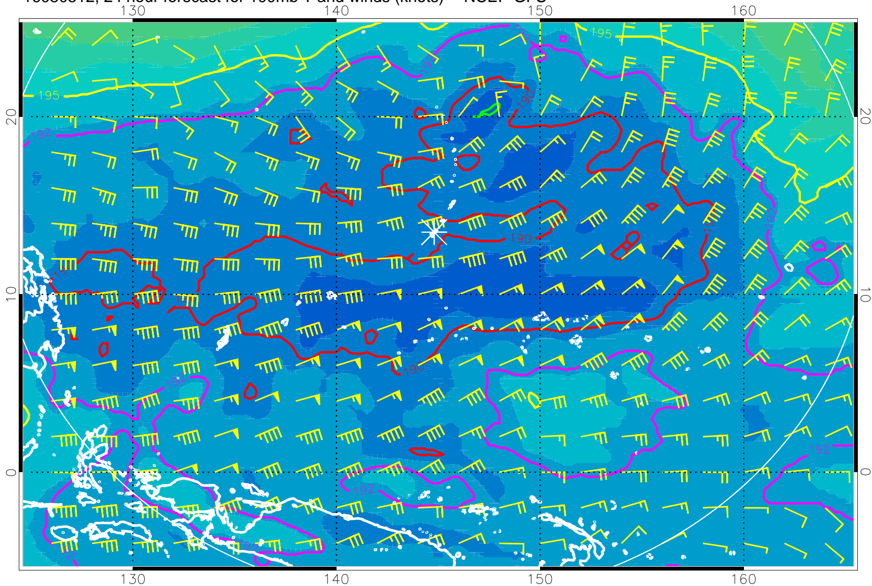
16080512, 24 hour forecast for 100mb T and winds (knots) -- NCEP GFS
