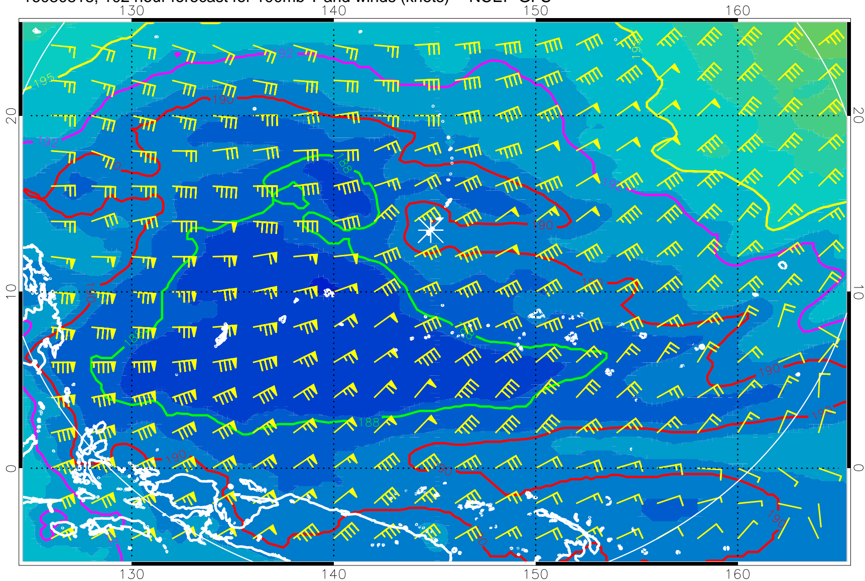
16080818, 102 hour forecast for 100mb T and winds (knots) -- NCEP GFS
