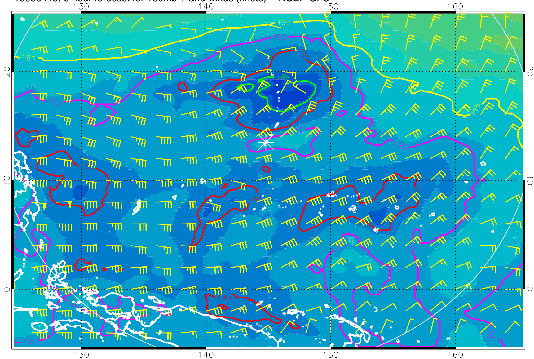
16080418, 6 hour forecast for 100mb T and winds (knots) -- NCEP GFS
