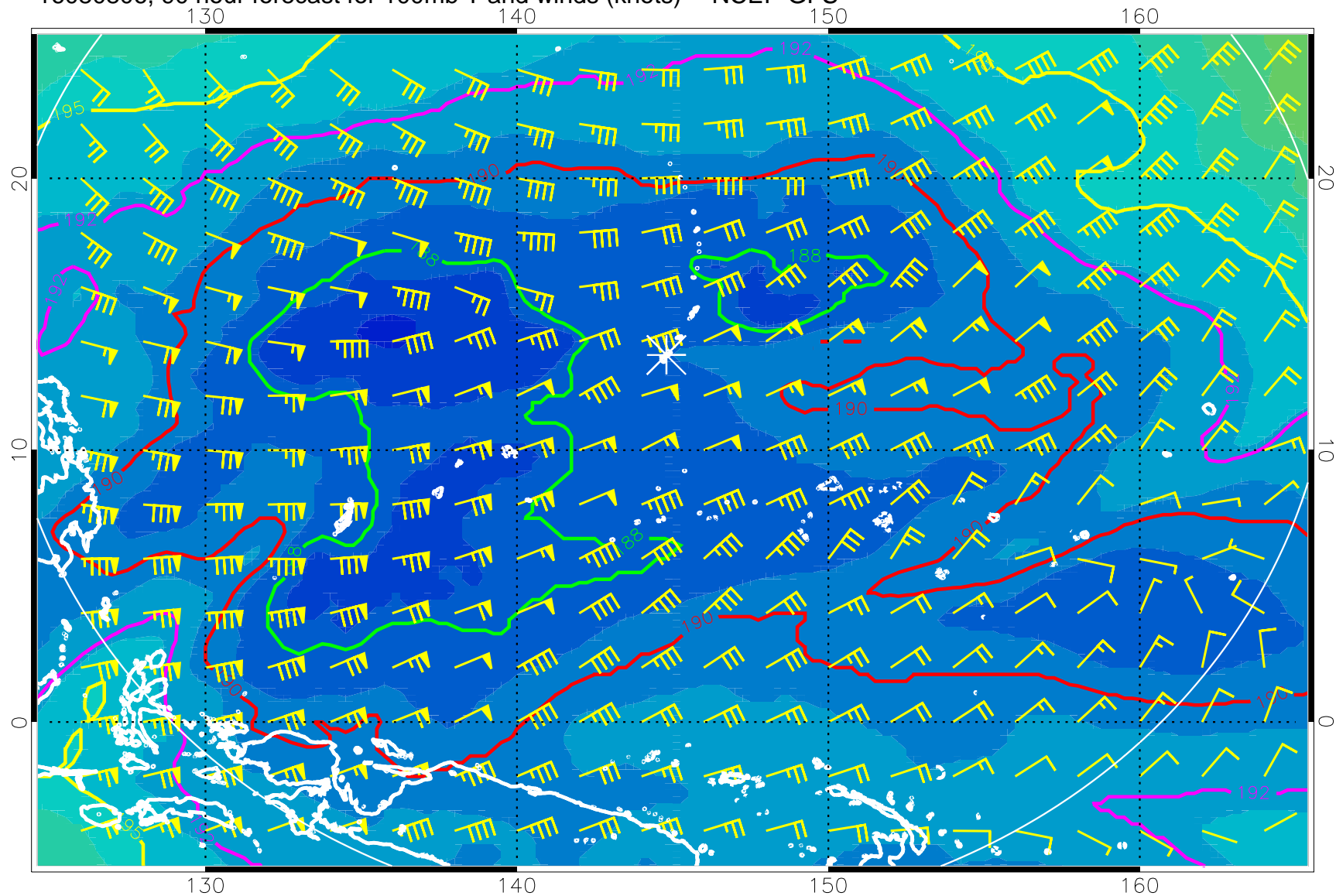
16080806, 90 hour forecast for 100mb T and winds (knots) -- NCEP GFS
