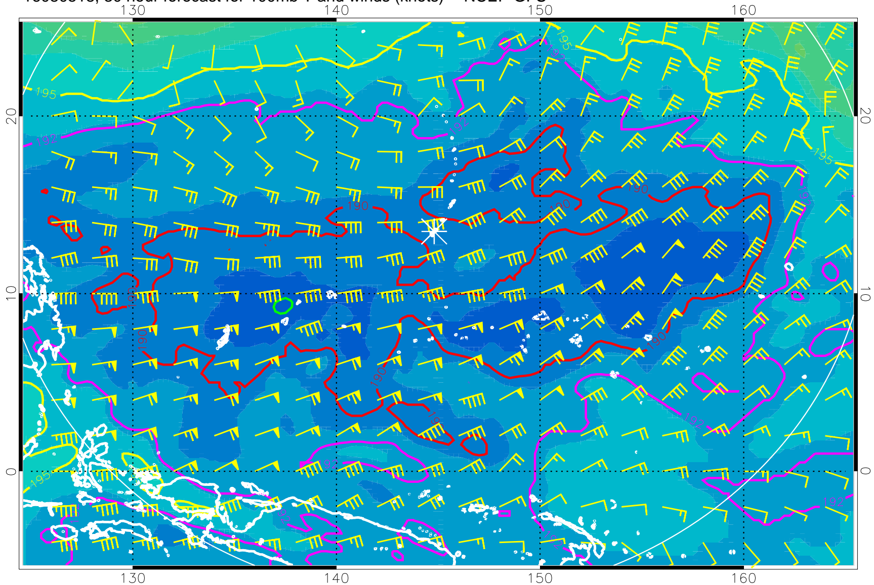
16080518, 30 hour forecast for 100mb T and winds (knots) -- NCEP GFS
