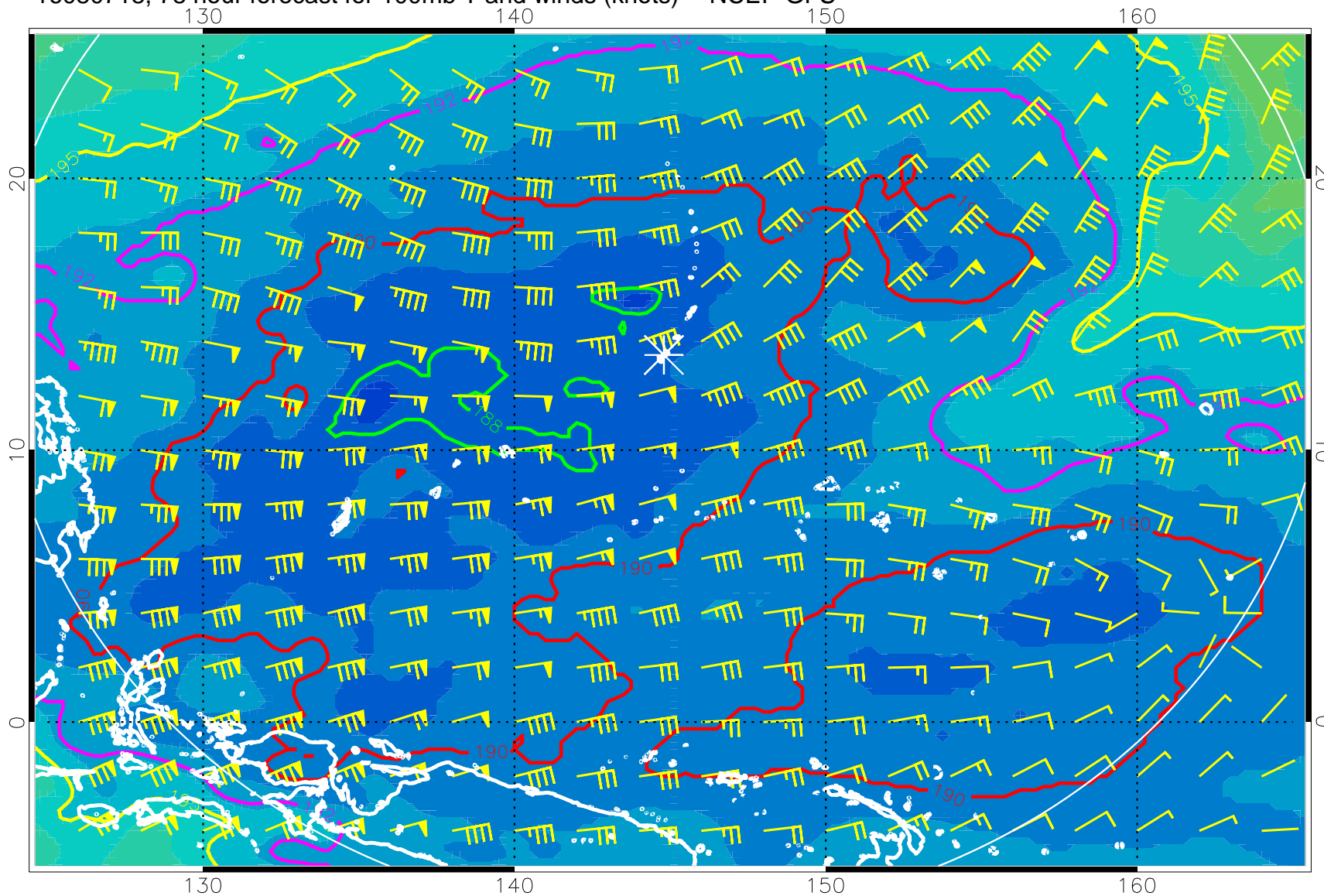
16080718, 78 hour forecast for 100mb T and winds (knots) -- NCEP GFS
